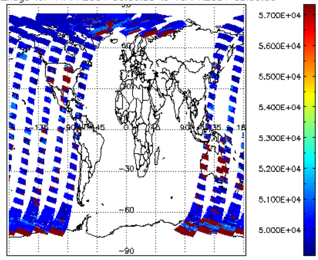
cloud_flags for 14APR2004 00:00:00 to 15APR2004 00:00:00
