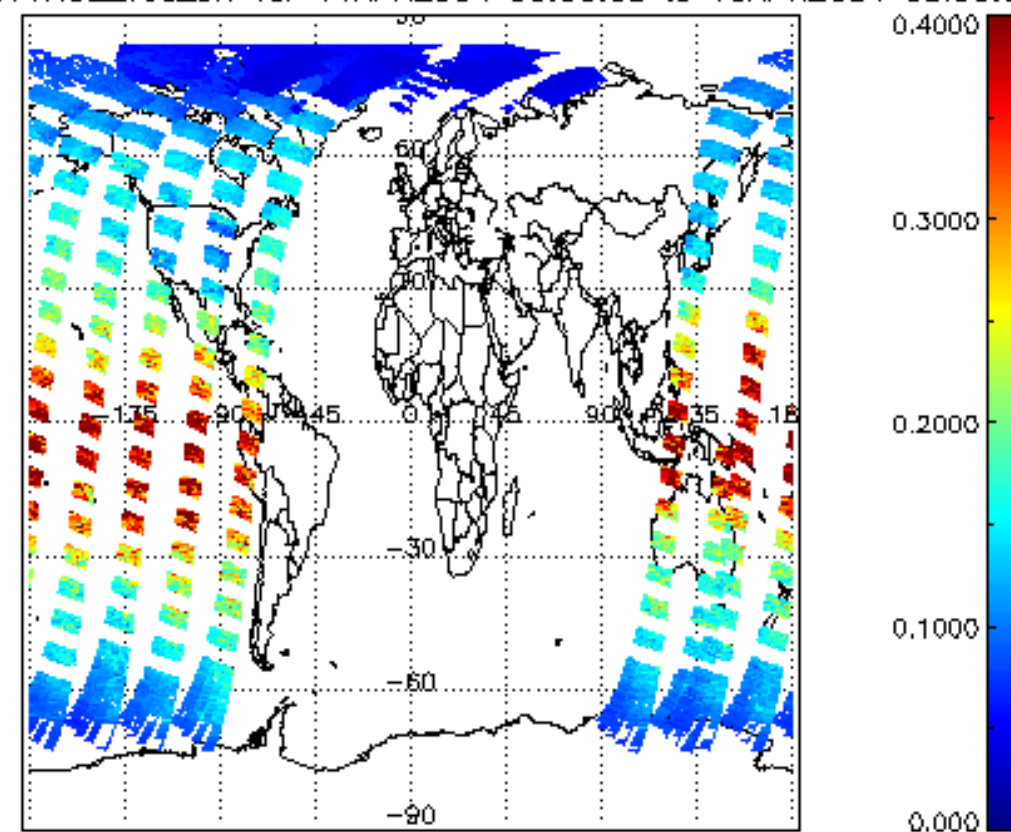
iCIOL2P_NADUV1NO2_vcd_err for 14APR2004 00:00:00 to 15APR2004 00:00:00
