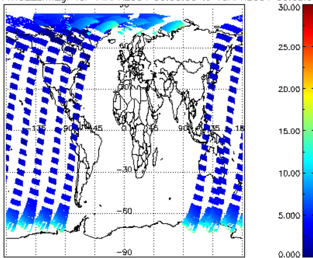
iCIOL2P_NADUV1NO2_amf_gr for 14APR2004 00:00:00 to 15APR2004 00:00:00
