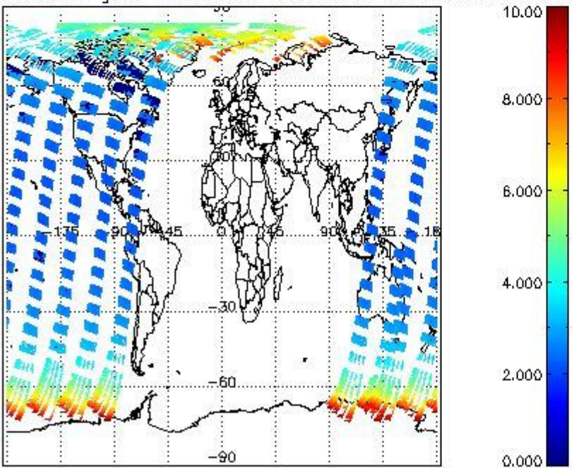
SCIOL2P_NADUV003_amf_gr for 14APR2004 00:00:00 to 15APR2004 00:00:00
