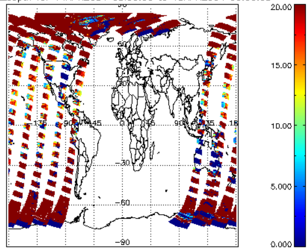
cl_opt_depth for 14APR2004 00:00:00 to 15APR2004 00:00:00
