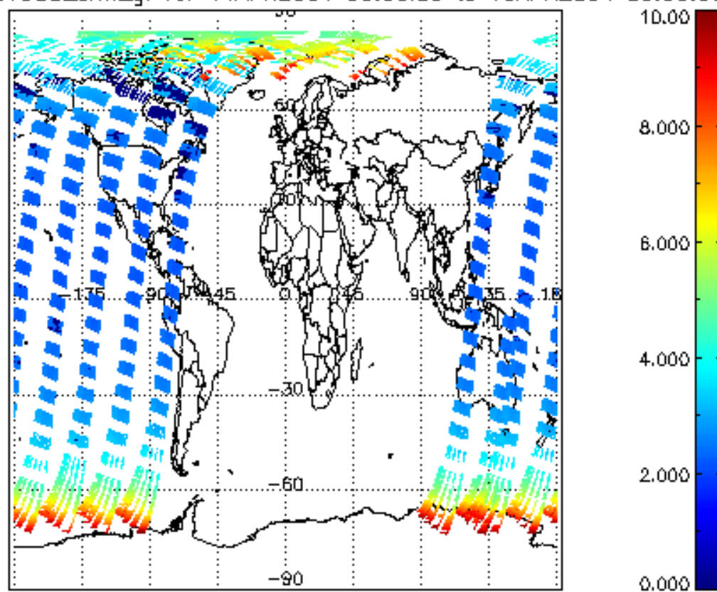
SCIOL2P_NADUV003_amf_gr for 14APR2004 00:00:00 to 15APR2004 00:00:00
