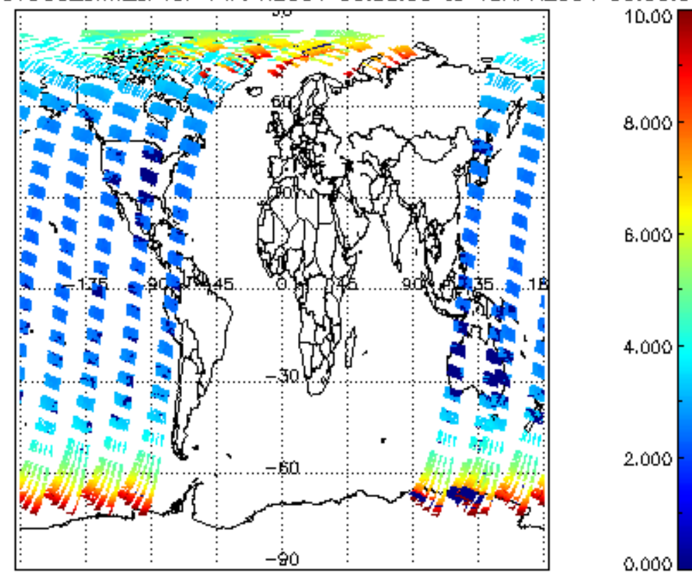
SCIOL2P_NADUV003_amf_cl for 14APR2004 00:00:00 to 15APR2004 00:00:00
