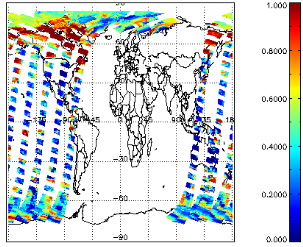
cl_frac for 14APR2004 00:00:00 to 15APR2004 00:00:00
