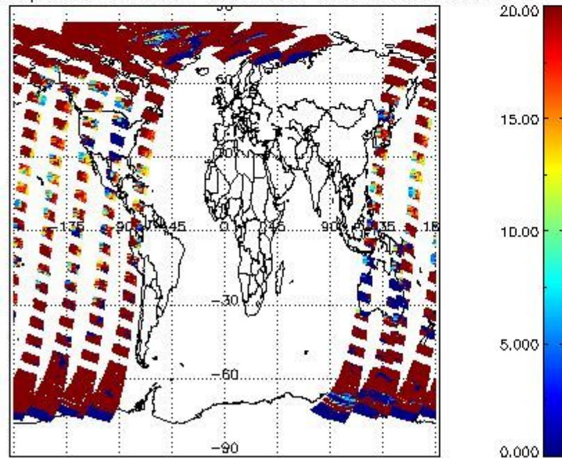
cL_opt_depth for 14APR2004 00:00:00 to 15APR2004 00:00:00
