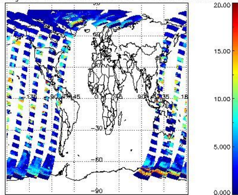
cL_top_height for 14APR2004 00:00:00 to 15APR2004 00:00:00
