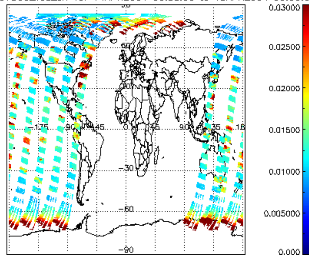
SCIOL2P_NADUV003_vcd_err for 14APR2004 00:00:00 to 15APR2004 00:00:00
