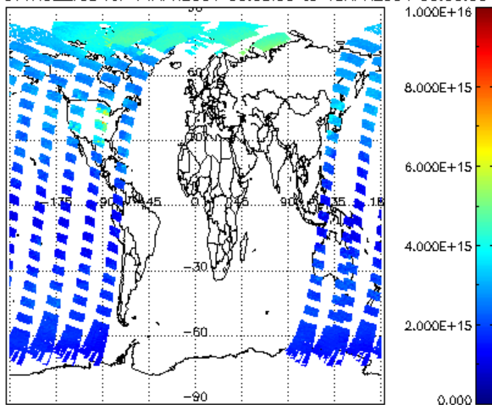
SCIOL2P_NADUV1NO2_vcd for 14APR2004 00:00:00 to 15APR2004 00:00:00
