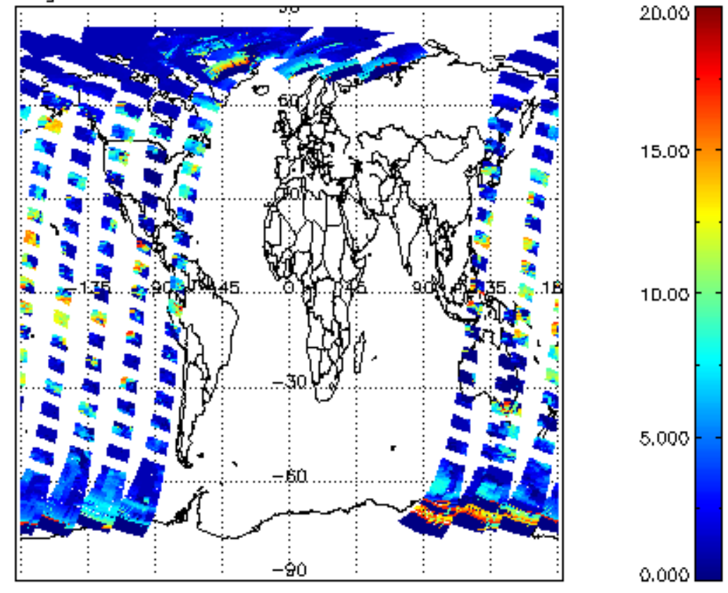
cl_top_height for 14APR2004 00:00:00 to 15APR2004 00:00:00
