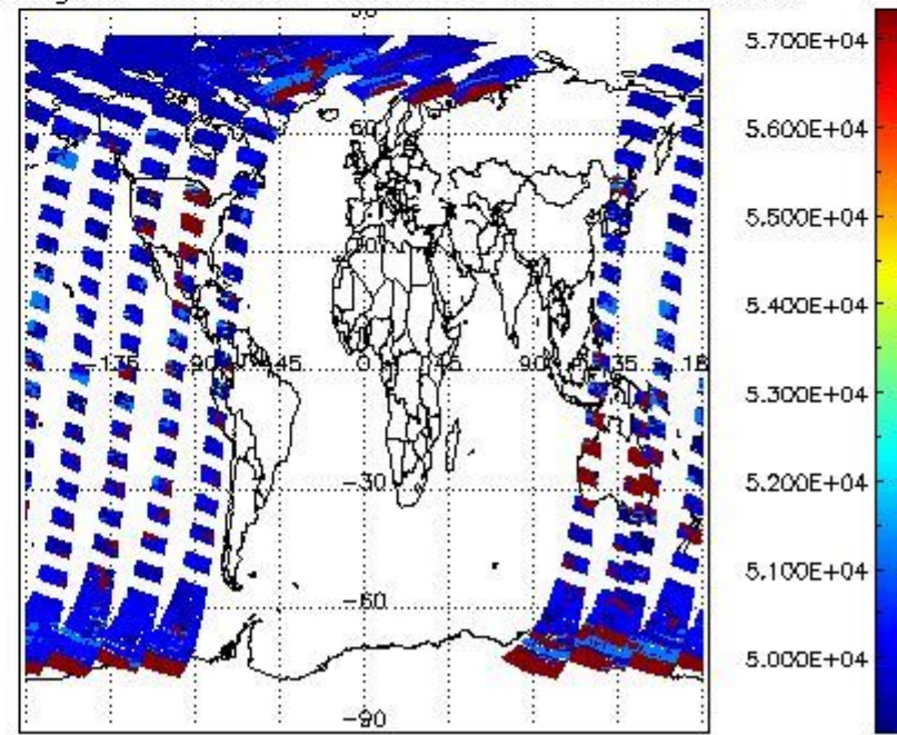
cloud_flags for 14APR2004 00:00:00 to 15APR2004 00:00:00
