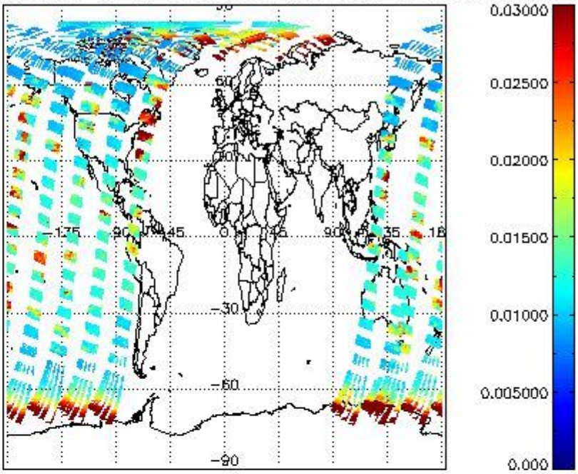
SCIOL2P_NADUV003_vcd_err for 14APR2004 00:00:00 to 15APR2004 00:00:00
