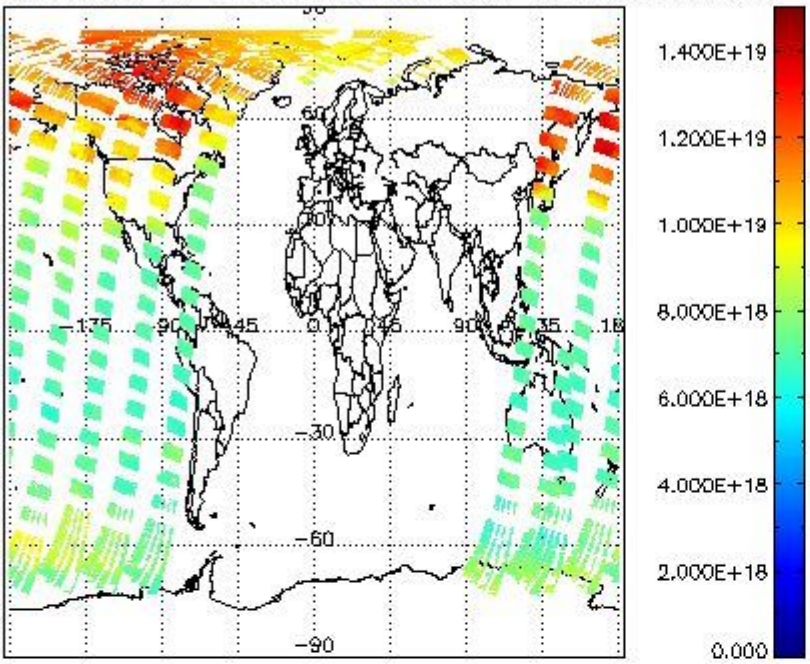
SCIOL2P_NADUV003_vcd for 14APR2004 00:00:00 to 15APR2004 00:00:00
