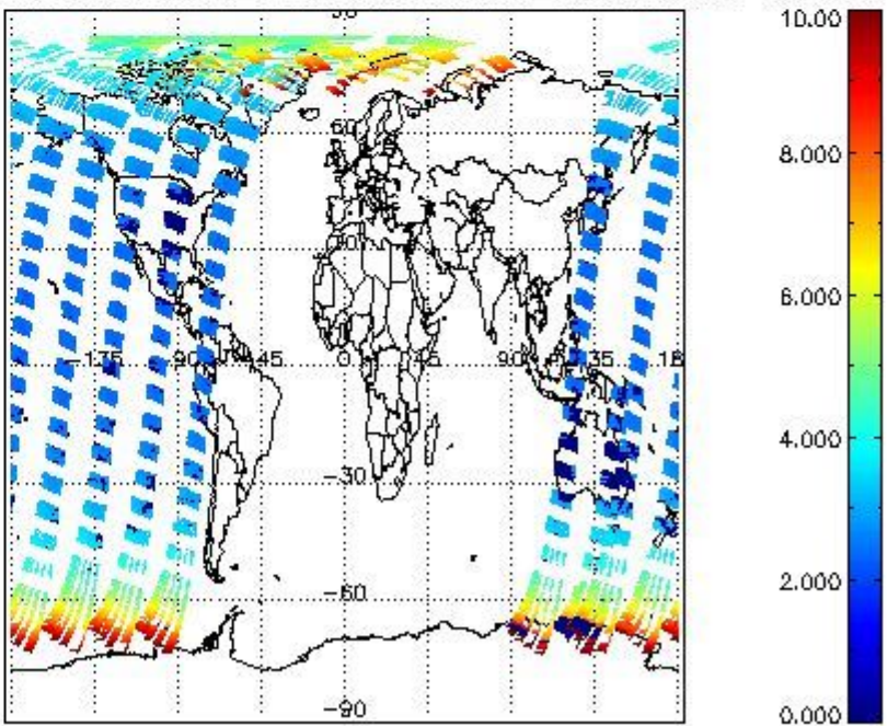
SCIOL2P_NADUV003_amf_cl for 14APR2004 00:00:00 to 15APR2004 00:00:00
