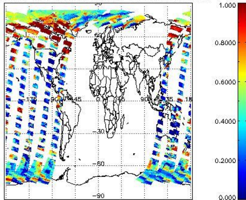
cL_frac for 14APR2004 00:00:00 to 15APR2004 00:00:00
