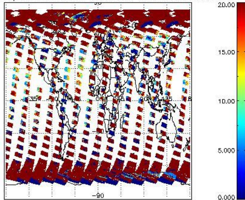
cLopt_depth for 12APR2004 00:00:00 to 13APR2004 00:00:00
