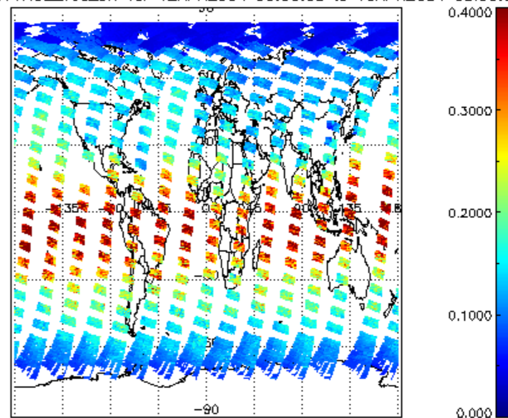
iCIOL2P_NADUV1NO2_vcd_err for 12APR2004 00:00:00 to 13APR2004 00:00:00
