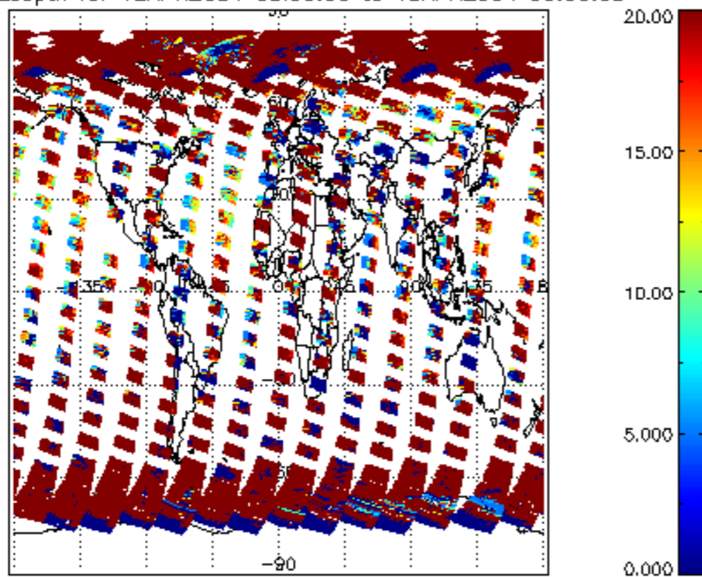
cl_opt_depth for 12APR2004 00:00:00 to 13APR2004 00:00:00
