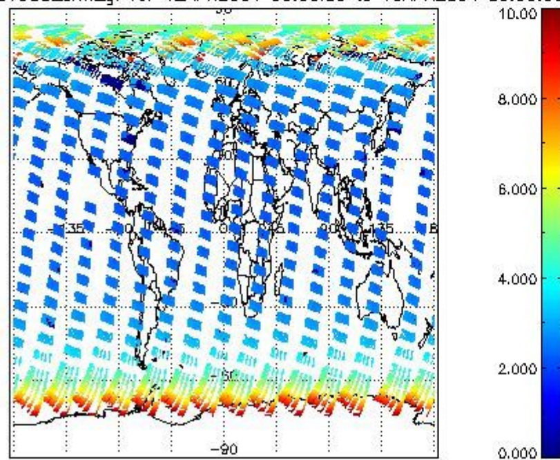
SCIOL2P_NADUV003_amf_gr for 12APR2004 00:00:00 to 13APR2004 00:00:00
