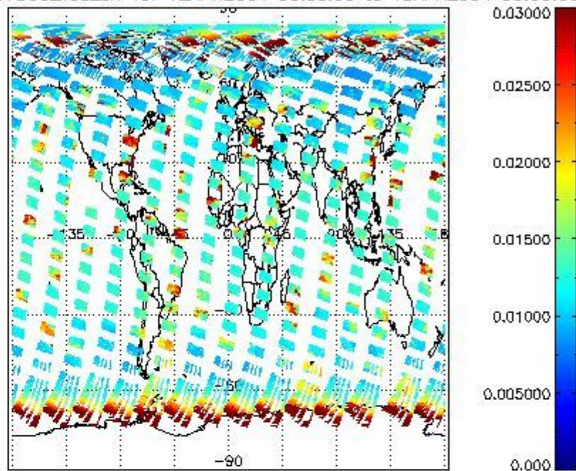
SCIOL2P_NADUV003_vcd_err for 12APR2004 00:00:00 to 13APR2004 00:00:00
