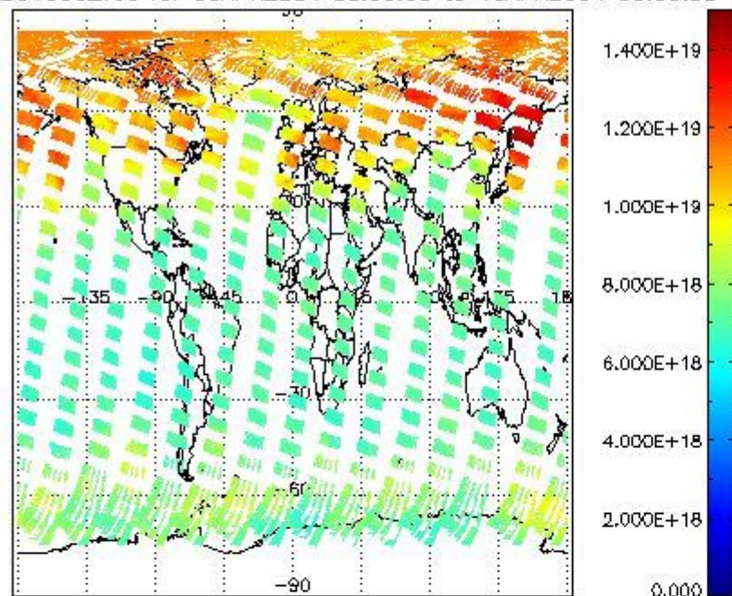
SCIOL2P_NADUV003_vcd for 09APR2004 00:00:00 to 10APR2004 00:00:00
