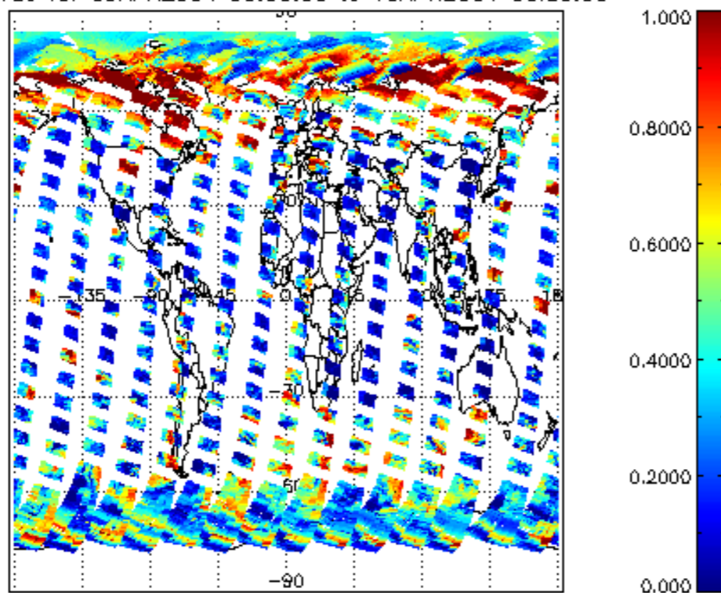
cl_frac for 09APR2004 00:00:00 to 10APR2004 00:00:00
