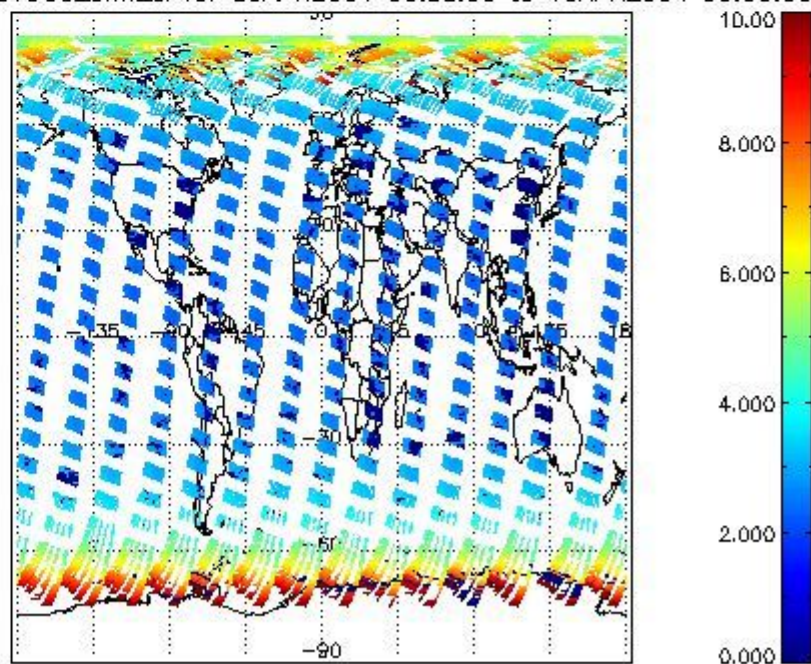
SCIOL2P_NADUV003_amf_cl for 09APR2004 00:00:00 to 10APR2004 00:00:00
