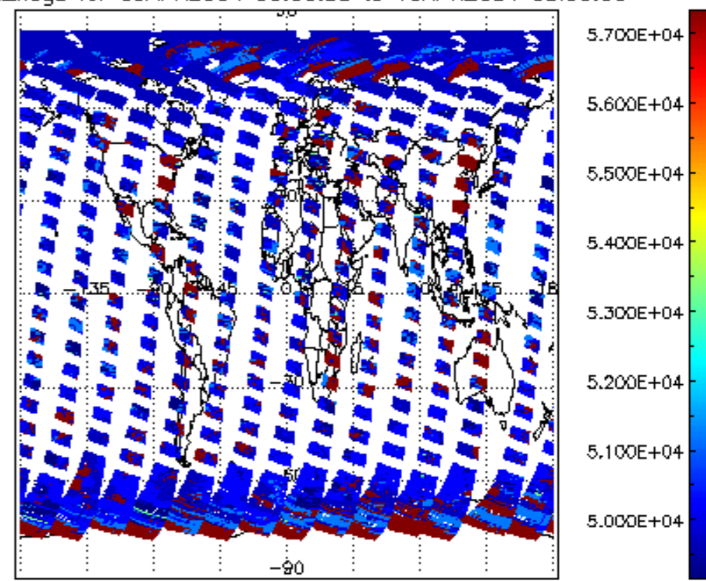
cloud_flags for 09APR2004 00:00:00 to 10APR2004 00:00:00
