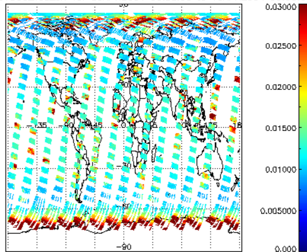
SCIOL2P_NADUV003_vcd_err for 09APR2004 00:00:00 to 10APR2004 00:00:00
