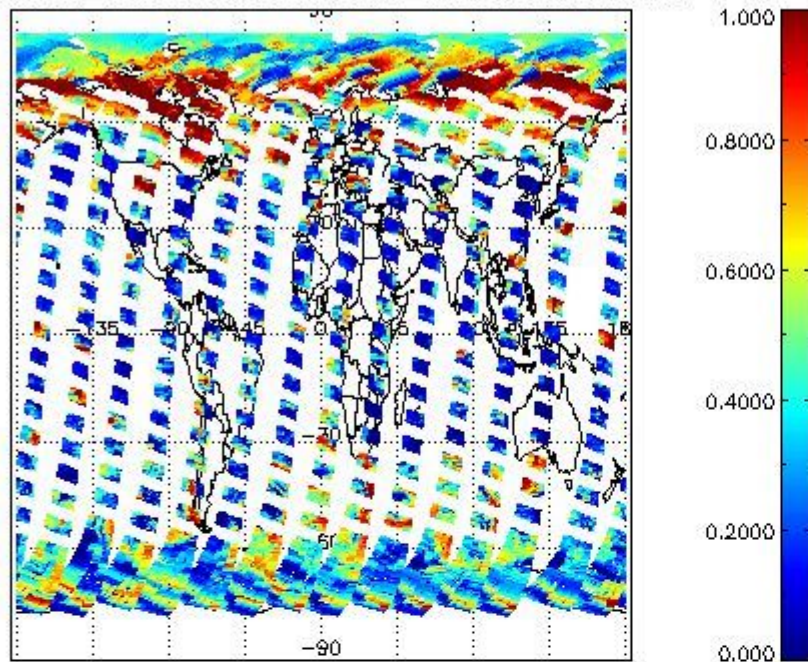
cLfrac for 09APR2004 00:00:00 to 10APR2004 00:00:00
