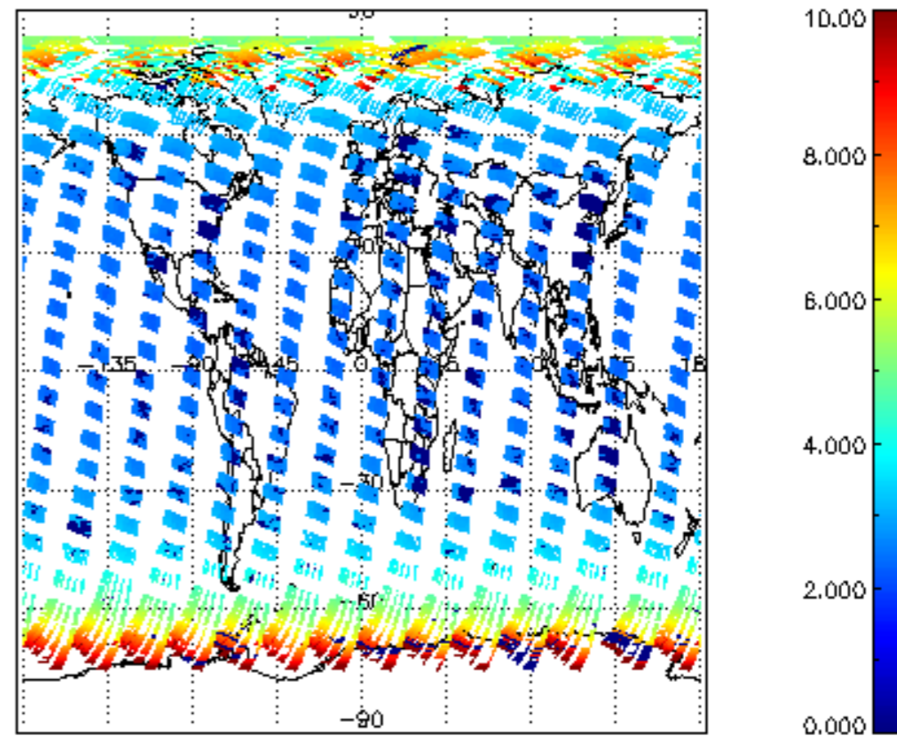
SCIOL2P_NADUV003_amf_cl for 09APR2004 00:00:00 to 10APR2004 00:00:00
