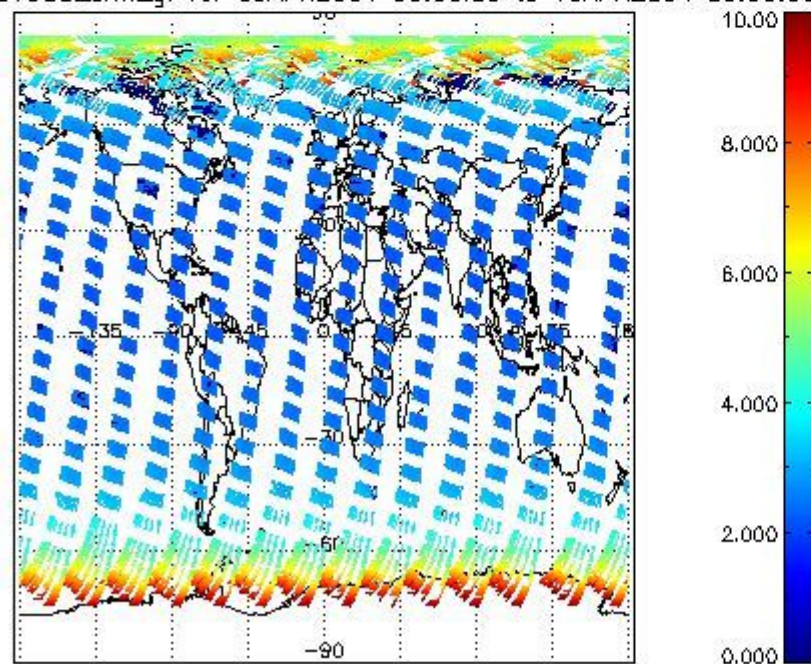
SCIOL2P_NADUV003_amf_gr for 09APR2004 00:00:00 to 10APR2004 00:00:00
