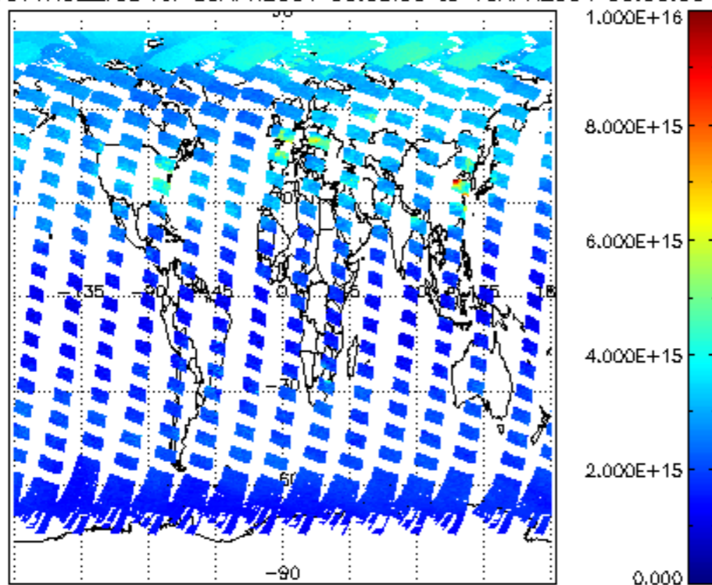
SCIOL2P_NADUV1NO2_vcd for 09APR2004 00:00:00 to 10APR2004 00:00:00
