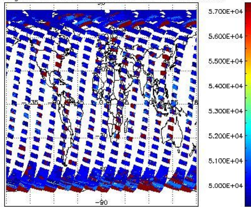
cloud_flags for 09APR2004 00:00:00 to 10APR2004 00:00:00
