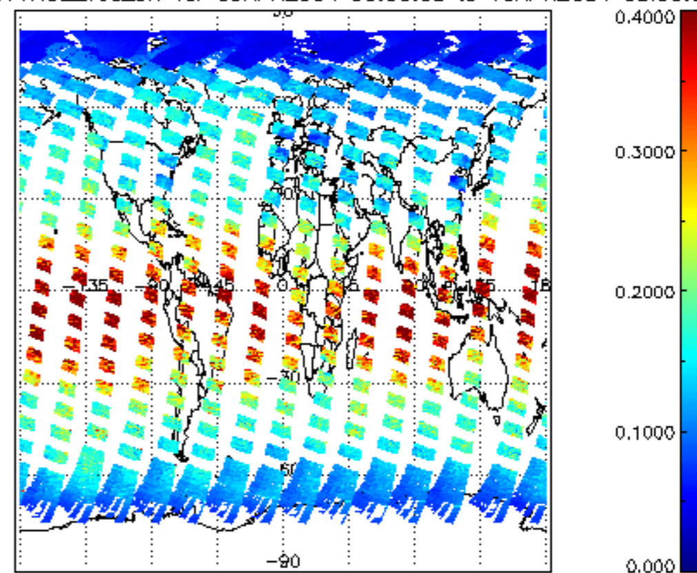
iCIOL2P_NADUV1NO2_vcd_err for 09APR2004 00:00:00 to 10APR2004 00:00:00
