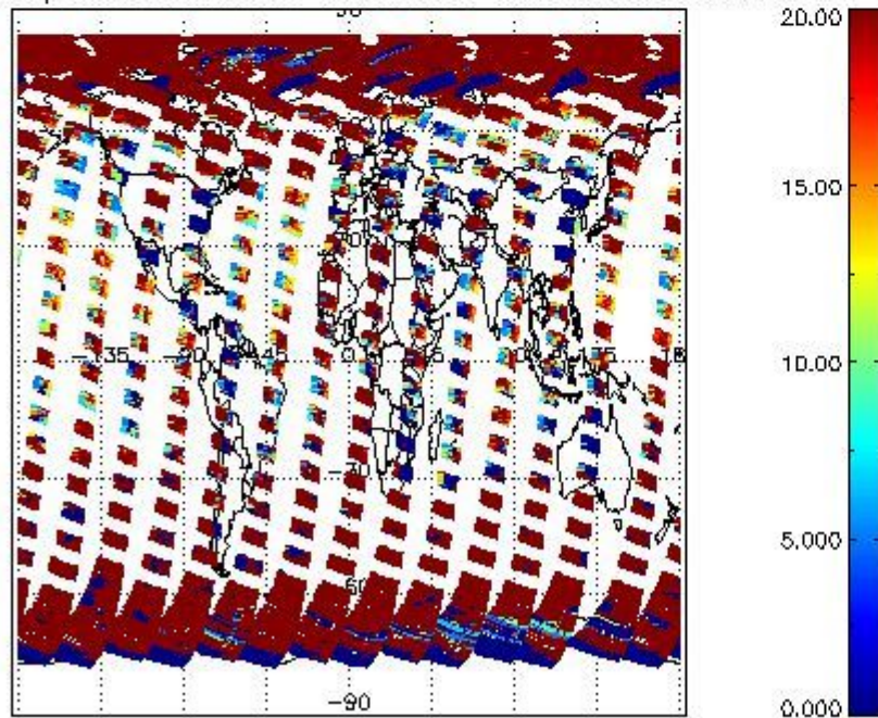
cLopt_depth for 09APR2004 00:00:00 to 10APR2004 00:00:00
