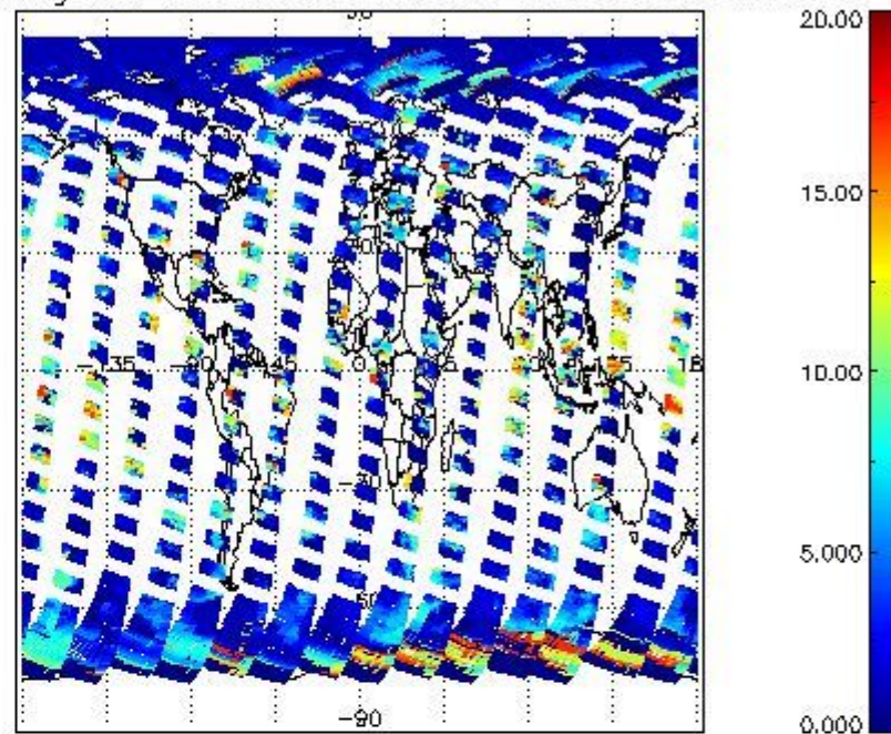
cL_top_height for 09APR2004 00:00:00 to 10APR2004 00:00:00
