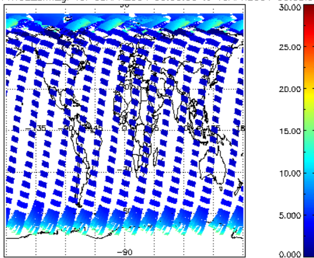
iCIOL2P_NADUV1NO2_amf_gr for 09APR2004 00:00:00 to 10APR2004 00:00:00
