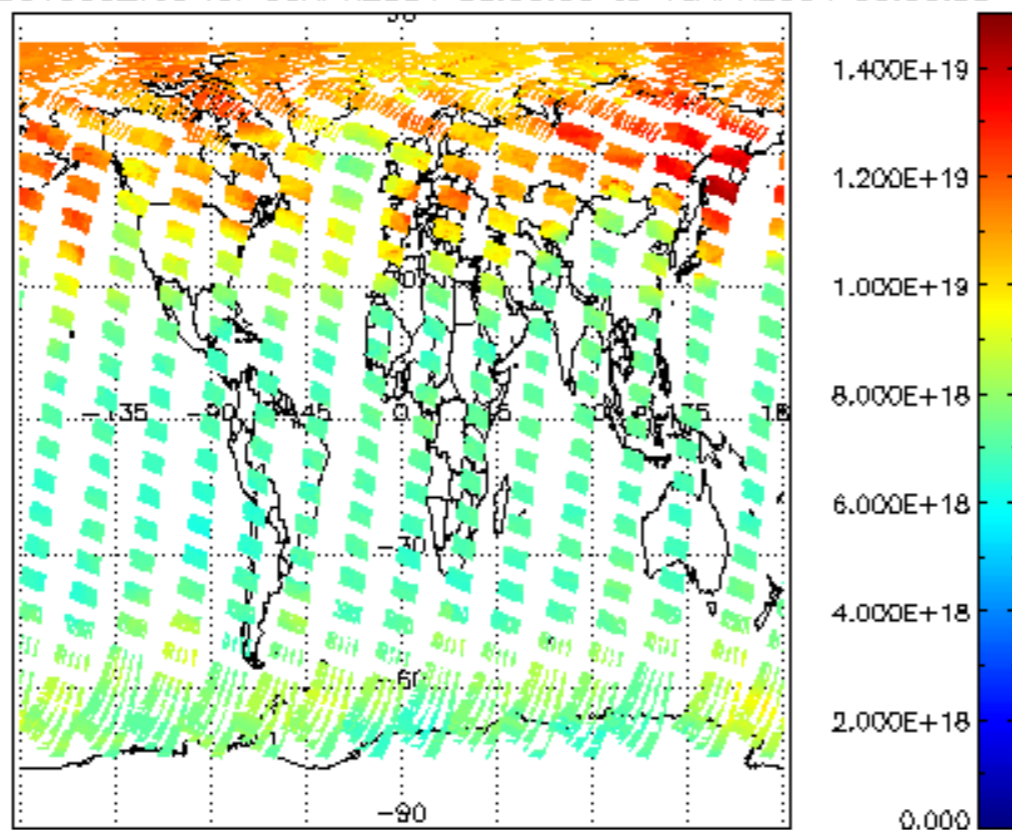
SCIOL2P_NADUV003_vcd for 09APR2004 00:00:00 to 10APR2004 00:00:00
