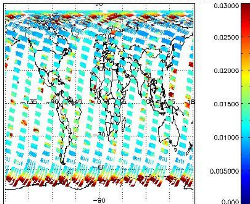
SCIOL2P_NADUV003_vcd_err for 09APR2004 00:00:00 to 10APR2004 00:00:00
