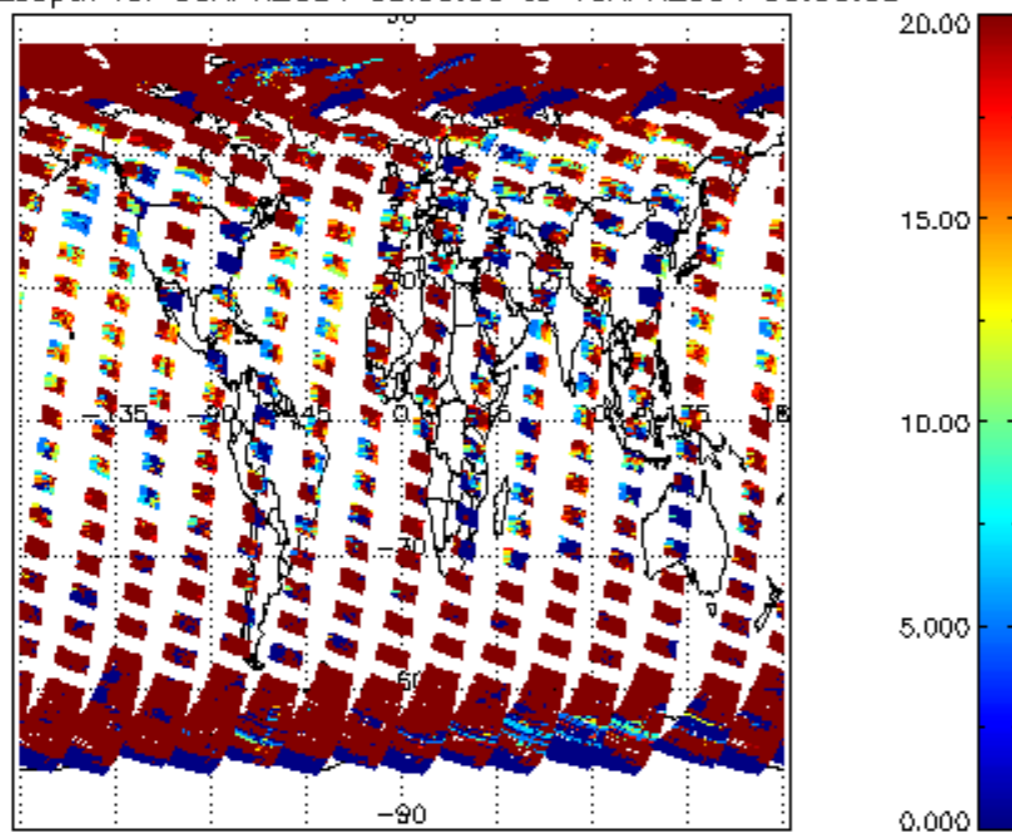
cl_opt_depth for 09APR2004 00:00:00 to 10APR2004 00:00:00
