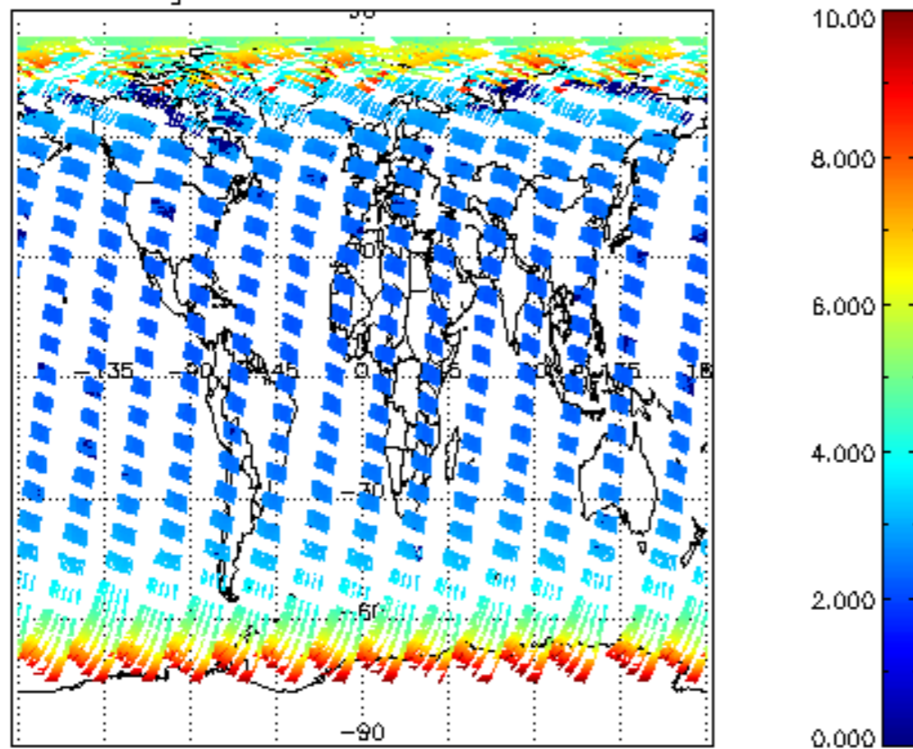
SCIOL2P_NADUV003_amf_gr for 09APR2004 00:00:00 to 10APR2004 00:00:00
