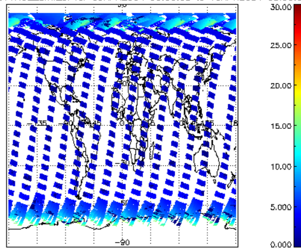
iCIOL2P_NADUV1NO2_amf_cl for 09APR2004 00:00:00 to 10APR2004 00:00:00
