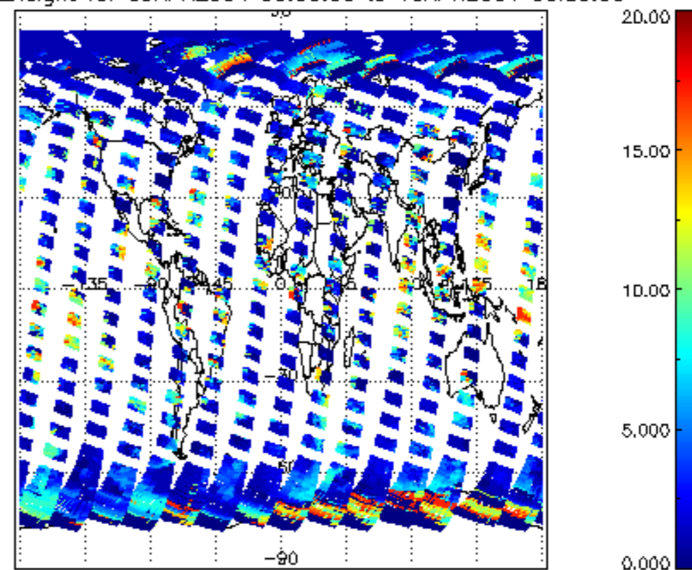
cl_top_height for 09APR2004 00:00:00 to 10APR2004 00:00:00
