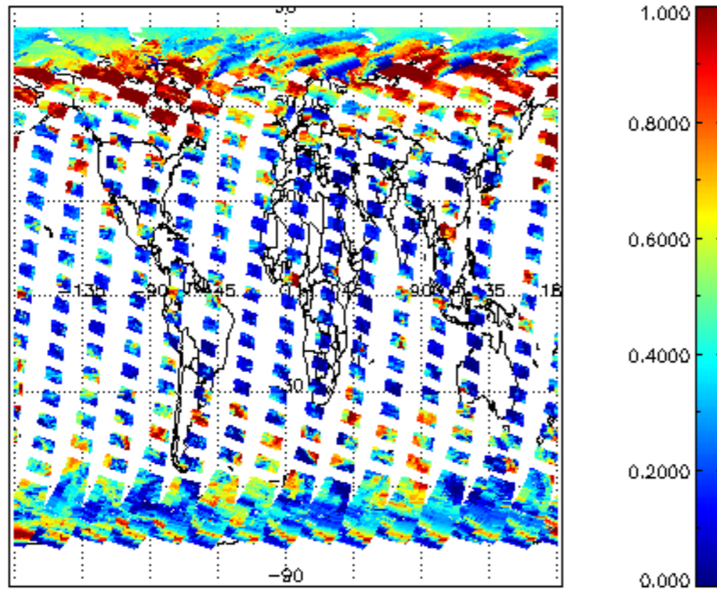
cl_frac for 08APR2004 00:00:00 to 09APR2004 00:00:00
