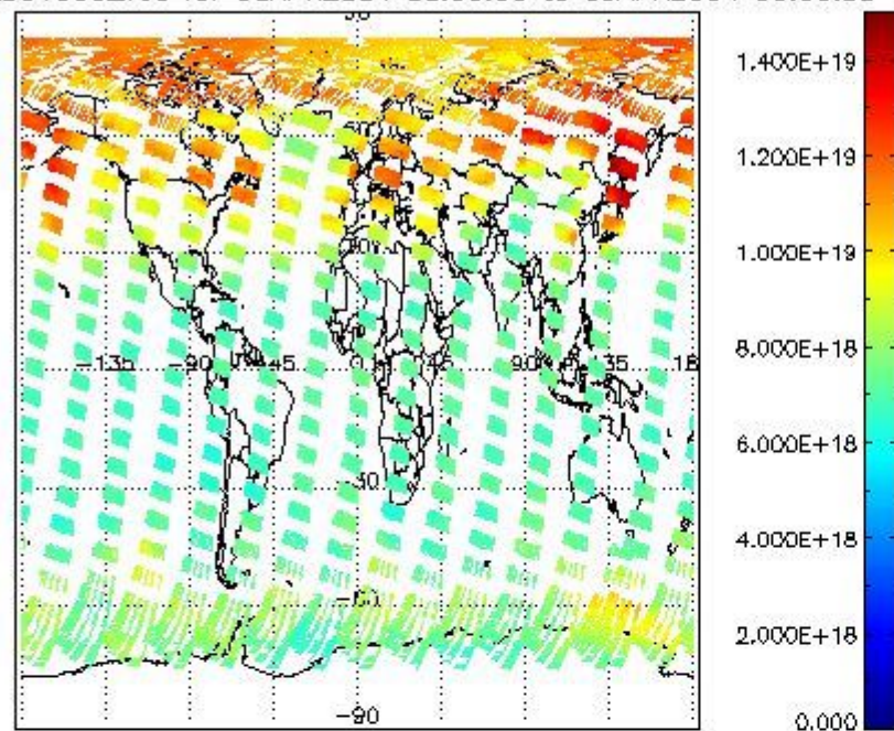
SCIOL2P_NADUV003_vcd for 08APR2004 00:00:00 to 09APR2004 00:00:00
