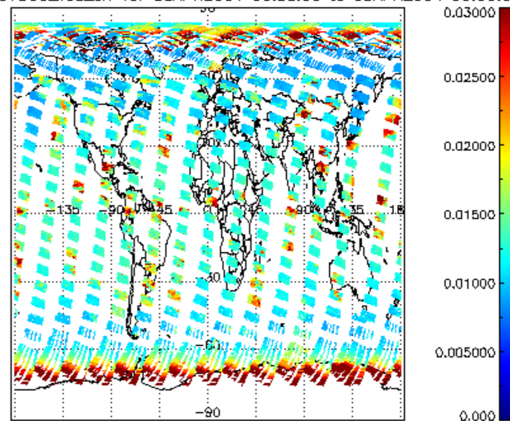
SCIOL2P_NADUV003_vcd_err for 08APR2004 00:00:00 to 09APR2004 00:00:00
