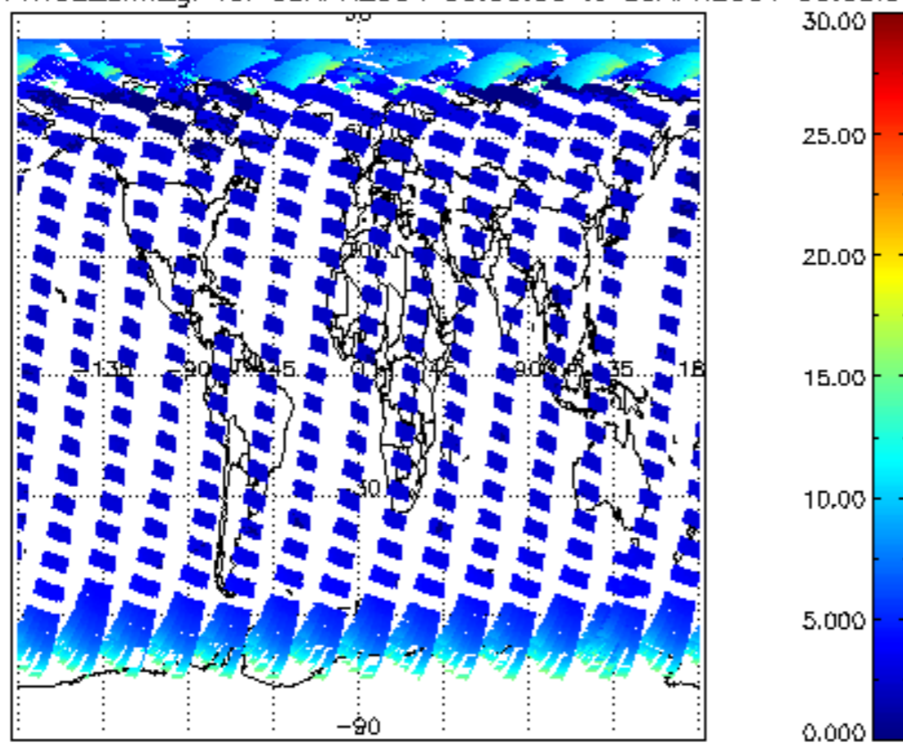
iCIOL2P_NADUV1NO2_amf_gr for 08APR2004 00:00:00 to 09APR2004 00:00:00
