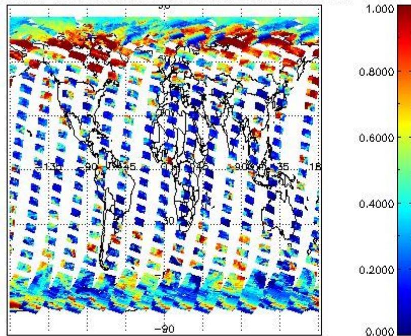
cL_frac for 08APR2004 00:00:00 to 09APR2004 00:00:00
