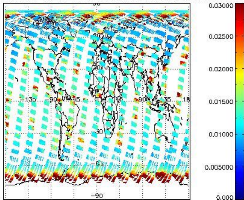
SCIOL2P_NADUV003_vcd_err for 08APR2004 00:00:00 to 09APR2004 00:00:00
