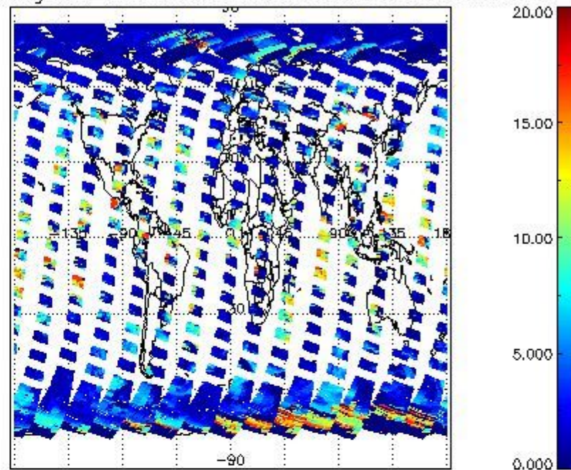
cL_top_height for 08APR2004 00:00:00 to 09APR2004 00:00:00
