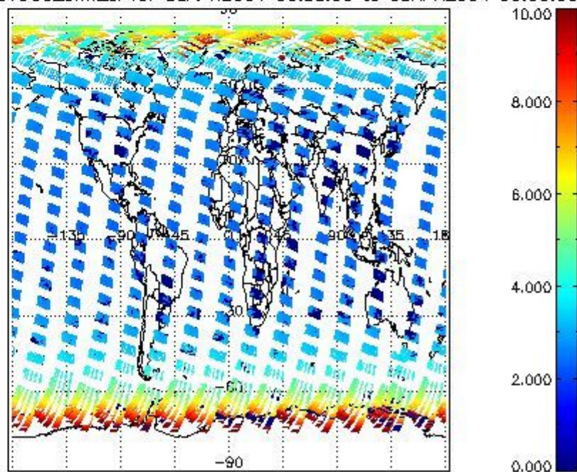
SCIOL2P_NADUV003_amf_cl for 08APR2004 00:00:00 to 09APR2004 00:00:00
