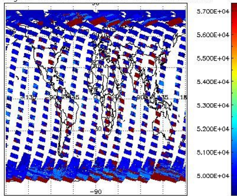
cloud_flags for 08APR2004 00:00:00 to 09APR2004 00:00:00
