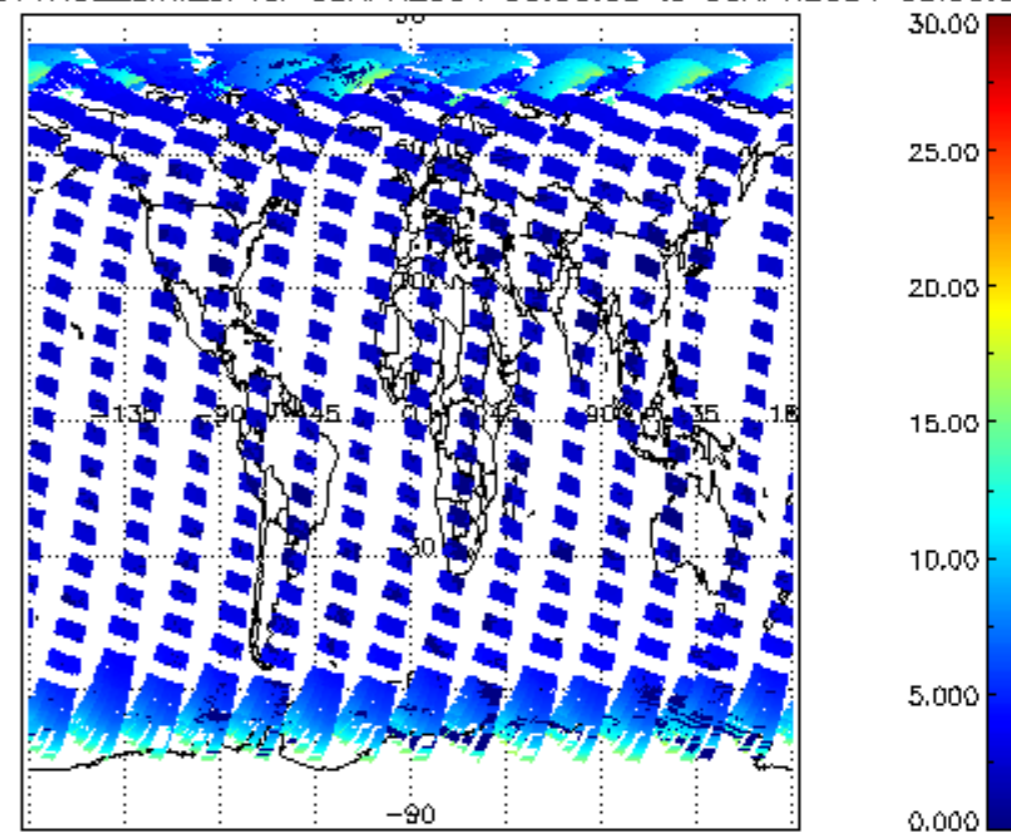
iCIOL2P_NADUV1NO2_amf_cl for 08APR2004 00:00:00 to 09APR2004 00:00:00
