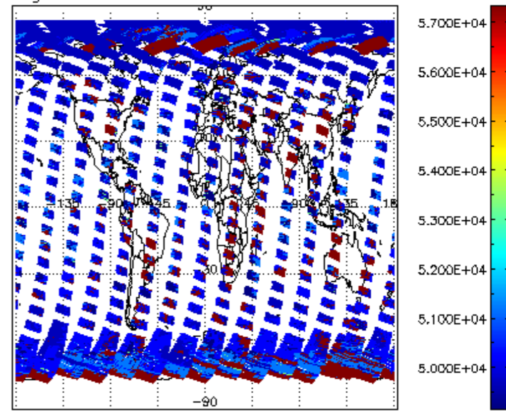
cloud_flags for 08APR2004 00:00:00 to 09APR2004 00:00:00
