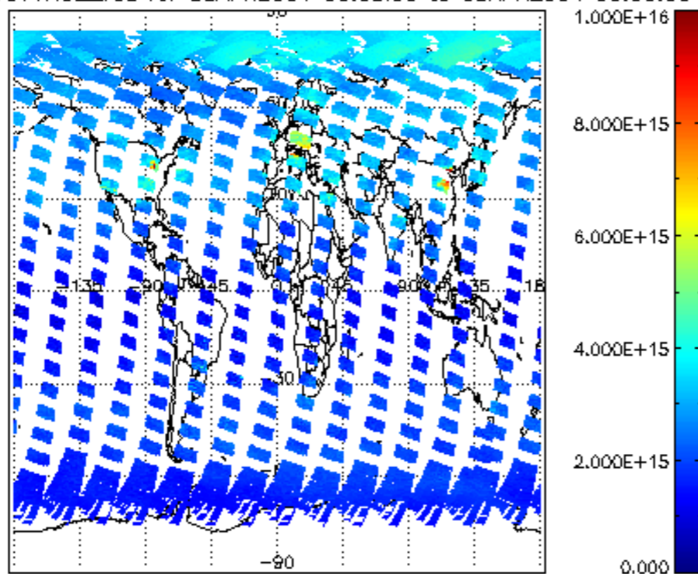
SCIOL2P_NADUV1NO2_vcd for 08APR2004 00:00:00 to 09APR2004 00:00:00
