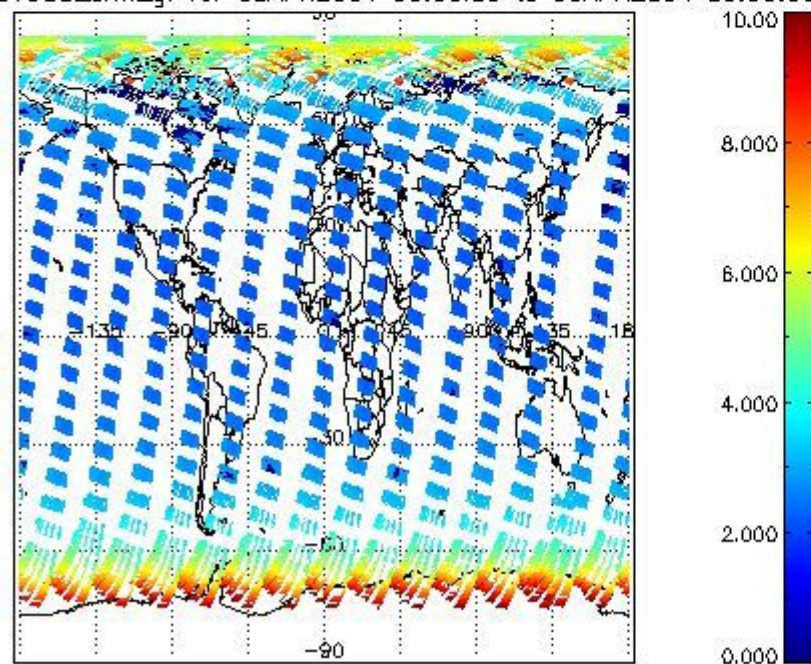
SCIOL2P_NADUV003_amf_gr for 08APR2004 00:00:00 to 09APR2004 00:00:00
