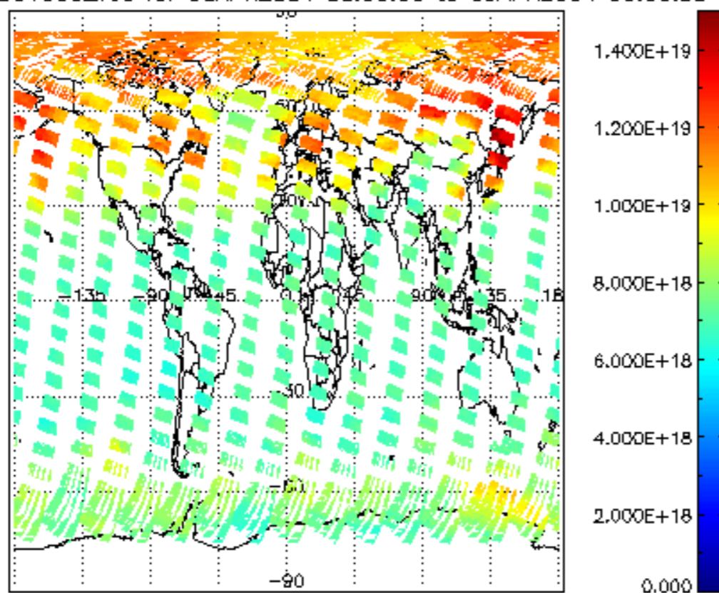
SCIOL2P_NADUV003_vcd for 08APR2004 00:00:00 to 09APR2004 00:00:00
