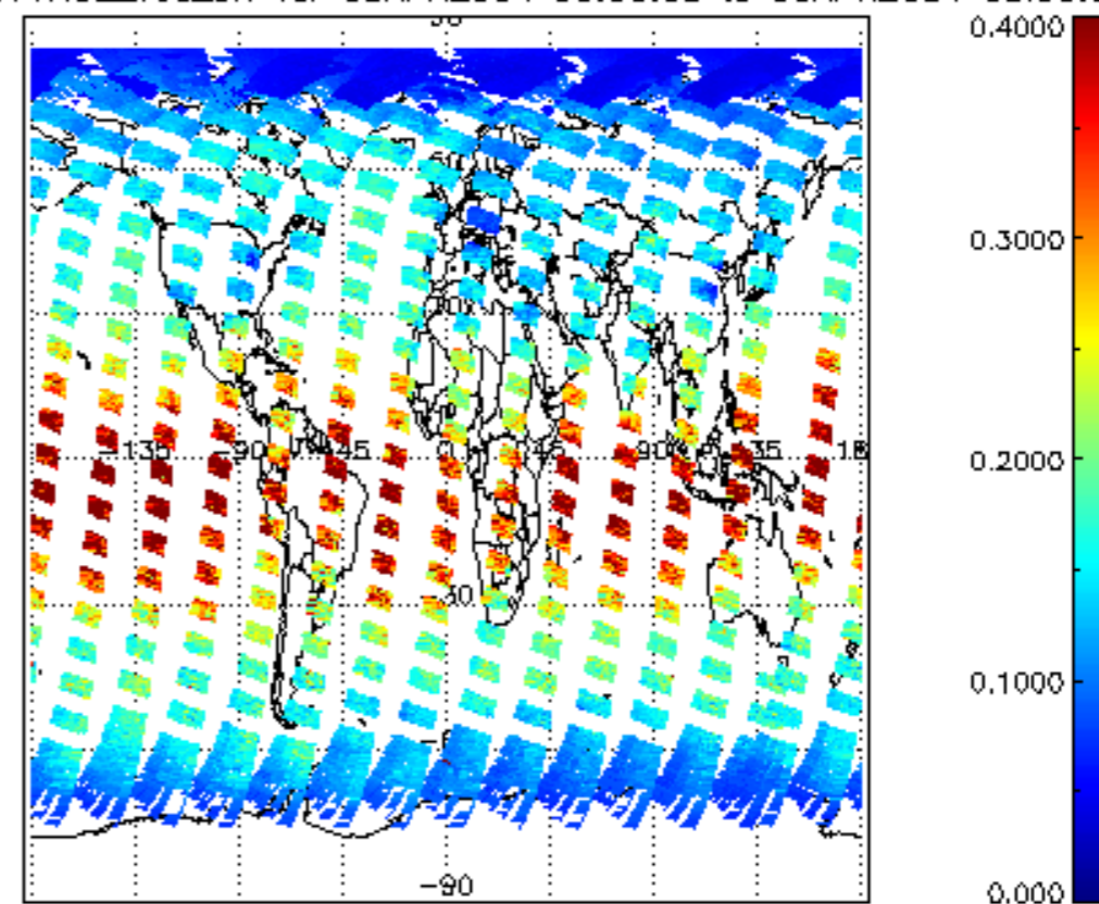
iCIOL2P_NADUV1NO2_vcd_err for 08APR2004 00:00:00 to 09APR2004 00:00:00
