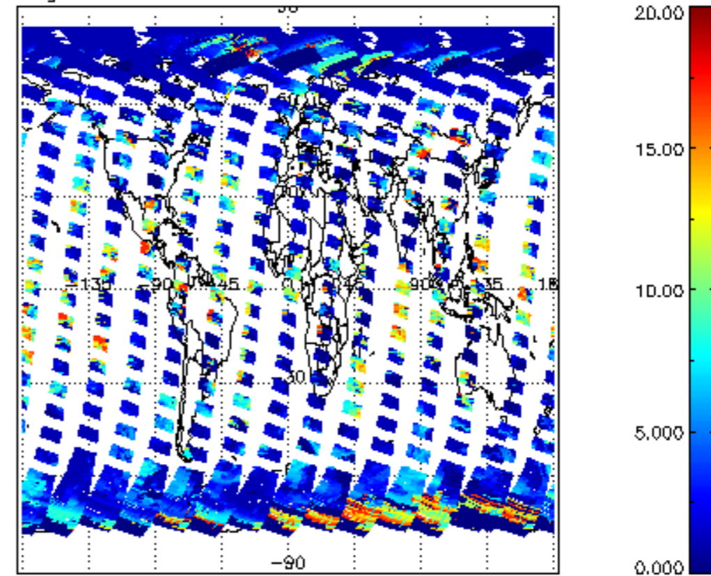
cl_top_height for 08APR2004 00:00:00 to 09APR2004 00:00:00
