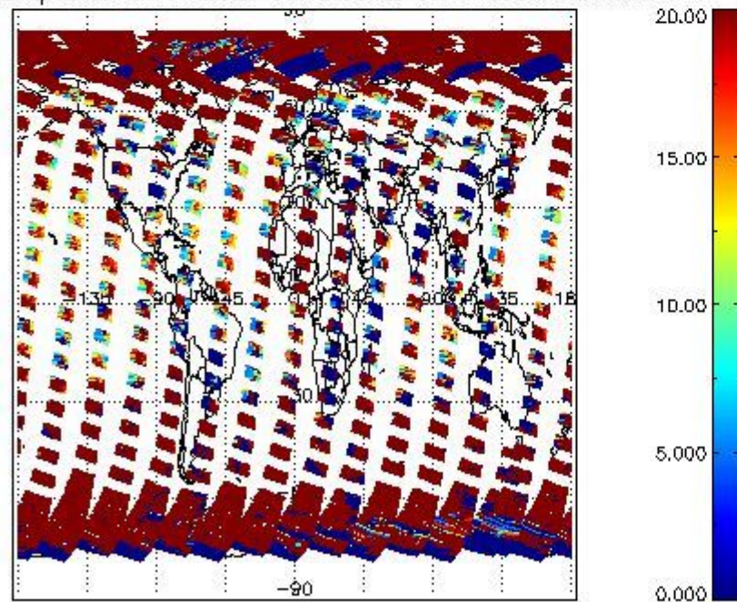
cL_opt_depth for 08APR2004 00:00:00 to 09APR2004 00:00:00
