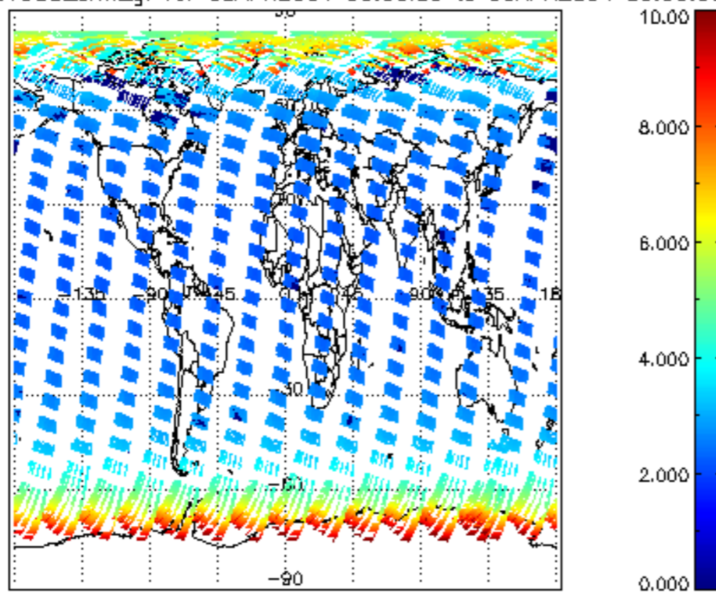
SCIOL2P_NADUV003_amf_gr for 08APR2004 00:00:00 to 09APR2004 00:00:00
