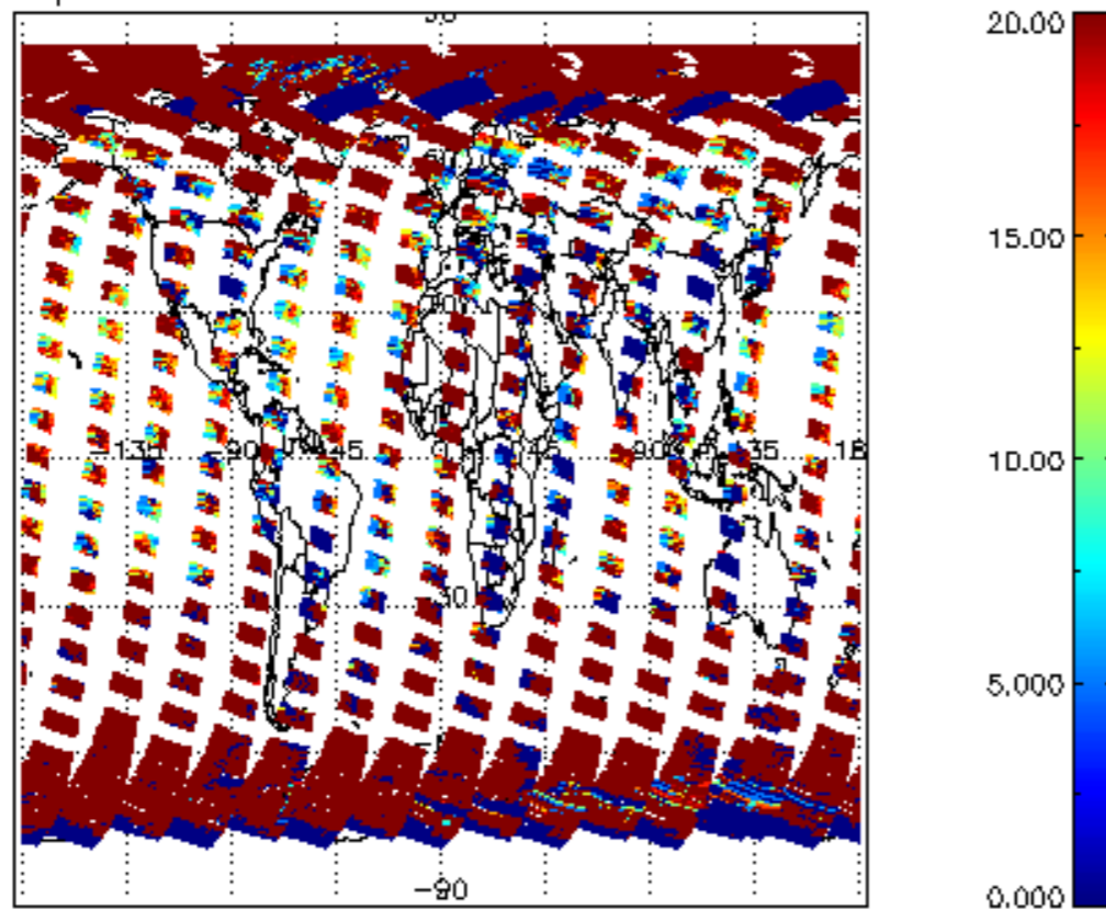
cl_opt_depth for 08APR2004 00:00:00 to 09APR2004 00:00:00
