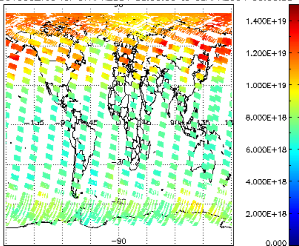
SCIOL2P_NADUV003_vcd for 07APR2004 00:00:00 to 08APR2004 00:00:00
