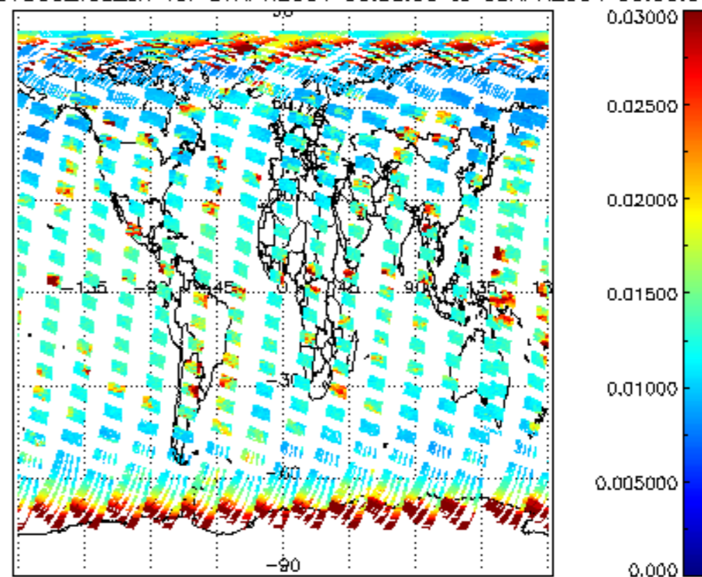
SCIOL2P_NADUV003_vcd_err for 07APR2004 00:00:00 to 08APR2004 00:00:00
