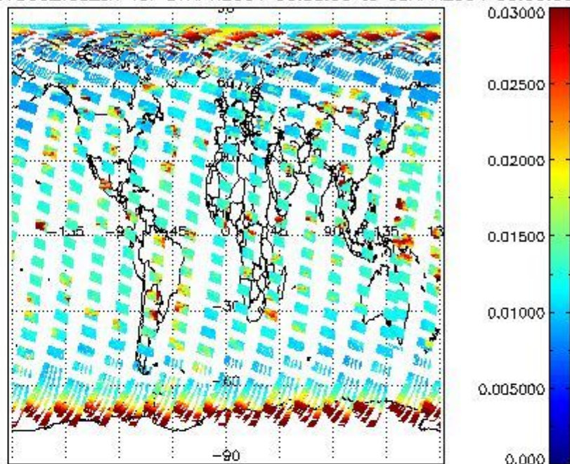
SCIOL2P_NADUV003_vcd_err for 07APR2004 00:00:00 to 08APR2004 00:00:00
