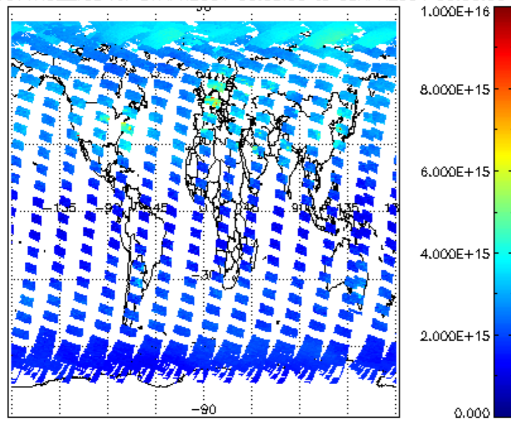
SCIOL2P_NADUV1NO2_vcd for 07APR2004 00:00:00 to 08APR2004 00:00:00
