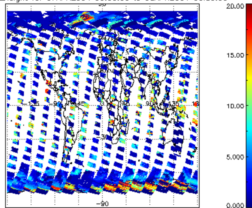
cL_top_height for 07APR2004 00:00:00 to 08APR2004 00:00:00
