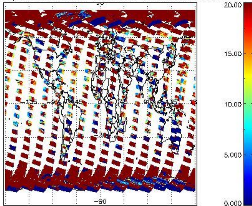
cL_opt_depth for 07APR2004 00:00:00 to 08APR2004 00:00:00
