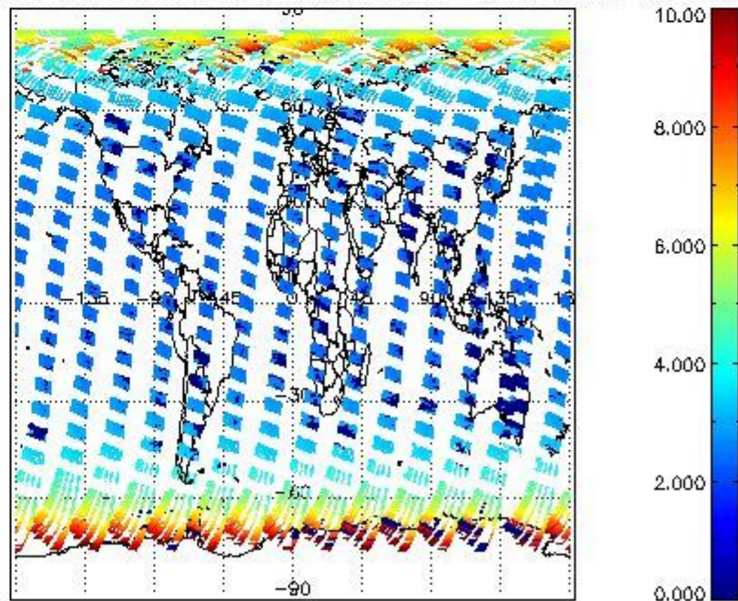
SCIOL2P_NADUV003_amf_cl for 07APR2004 00:00:00 to 08APR2004 00:00:00
