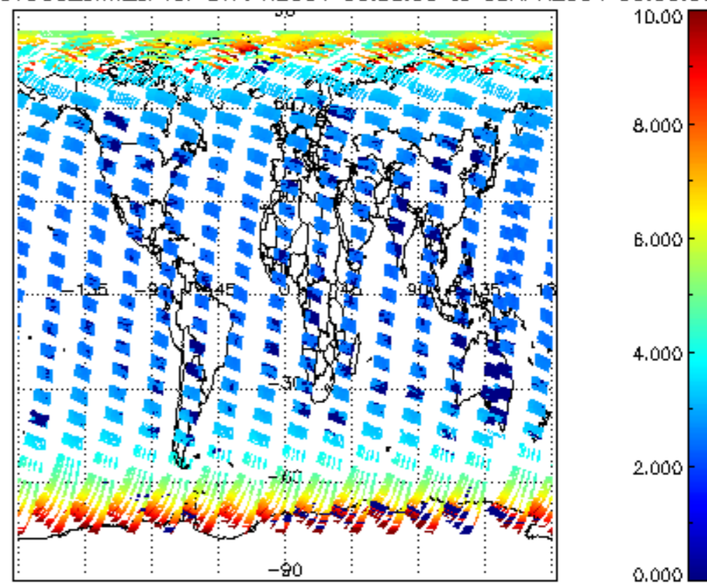
SCIOL2P_NADUV003_amf_cl for 07APR2004 00:00:00 to 08APR2004 00:00:00
