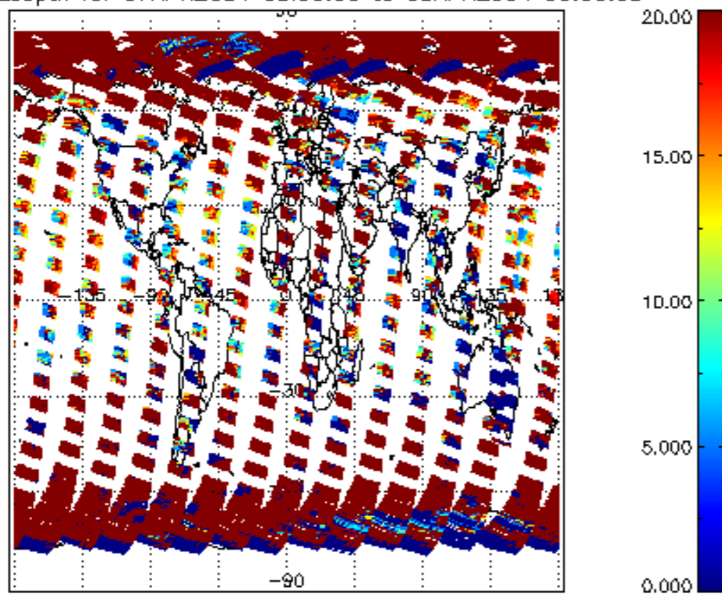
cL_opt_depth for 07APR2004 00:00:00 to 08APR2004 00:00:00
