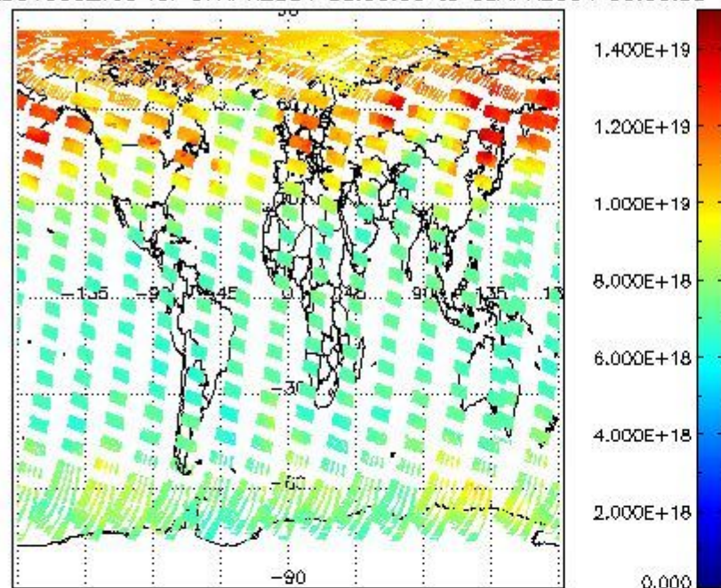
SCIOL2P_NADUV003_vcd for 07APR2004 00:00:00 to 08APR2004 00:00:00
