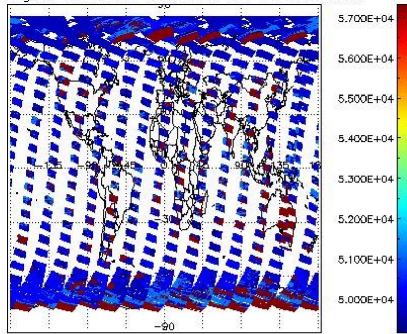
cloud_flags for 07APR2004 00:00:00 to 08APR2004 00:00:00
