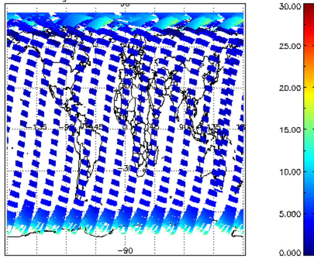
iCIOL2P_NADUV1NO2_amf_gr for 07APR2004 00:00:00 to 08APR2004 00:00:00
