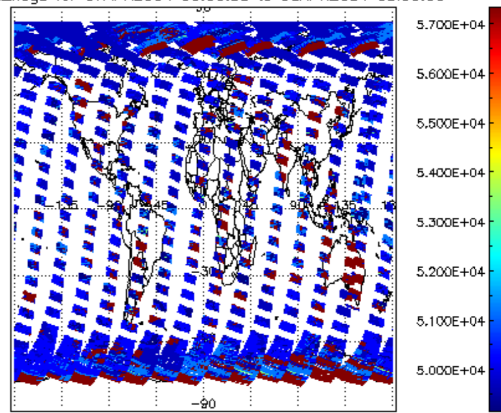
cloud_flags for 07APR2004 00:00:00 to 08APR2004 00:00:00
