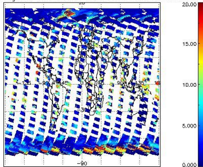
cL_top_height for 07APR2004 00:00:00 to 08APR2004 00:00:00
