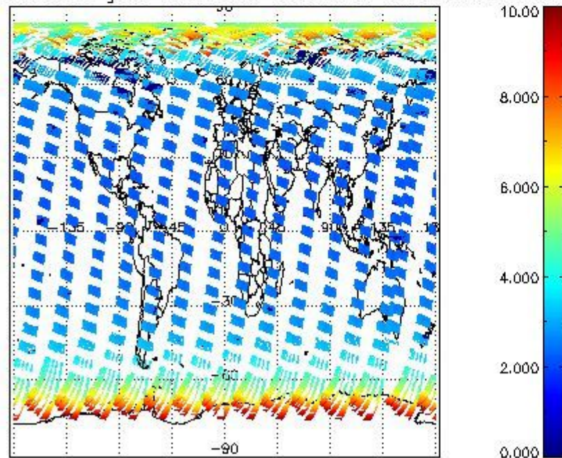
SCIOL2P_NADUV003_amf_gr for 07APR2004 00:00:00 to 08APR2004 00:00:00
