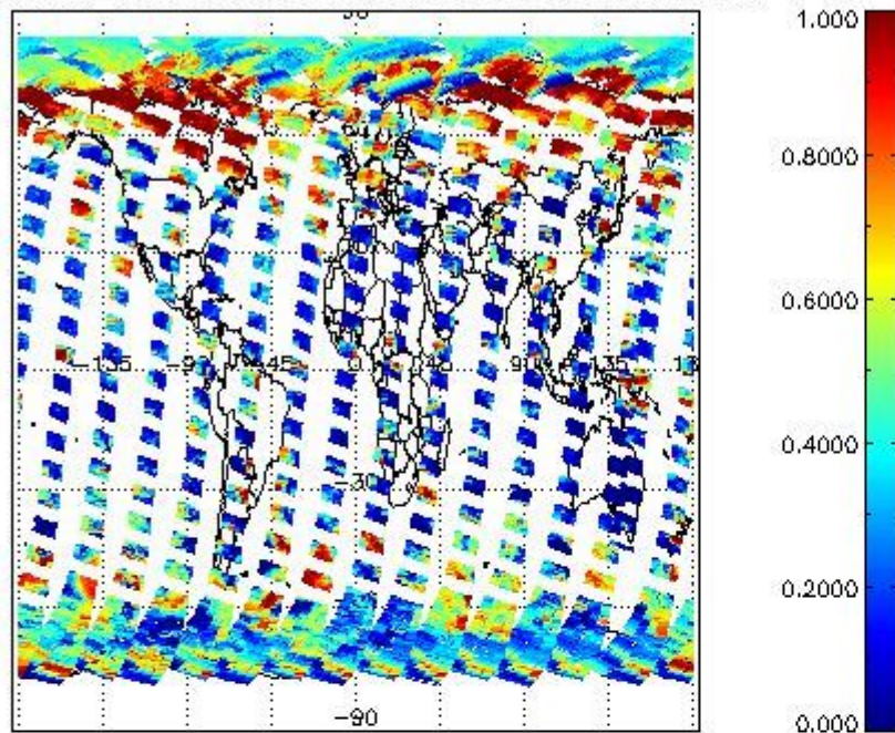
cL_frac for 07APR2004 00:00:00 to 08APR2004 00:00:00
