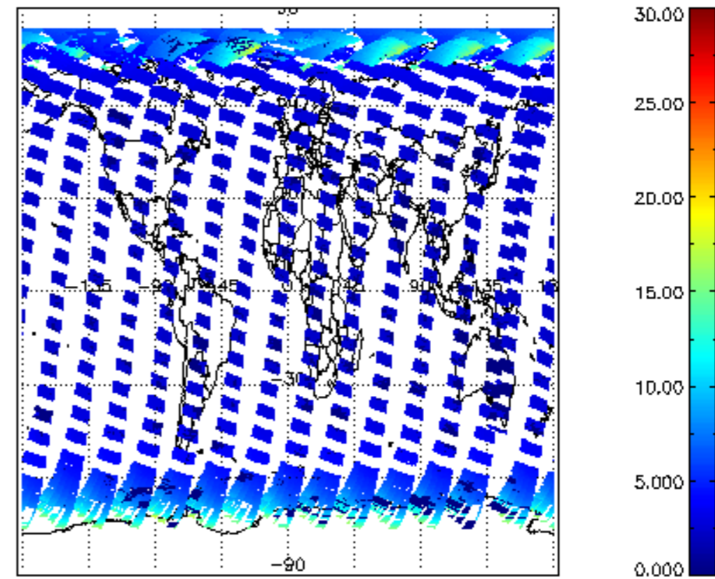
iCIOL2P_NADUV1NO2_amf_cl for 07APR2004 00:00:00 to 08APR2004 00:00:00
