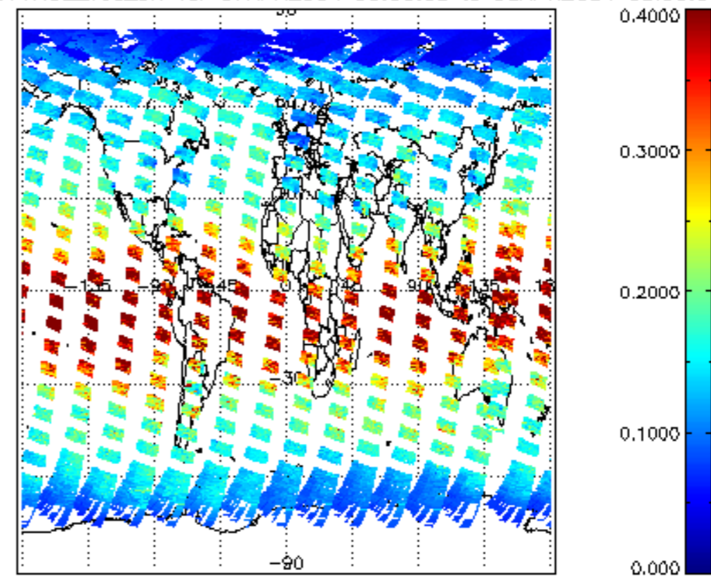
iCIOL2P_NADUV1NO2_vcd_err for 07APR2004 00:00:00 to 08APR2004 00:00:00
