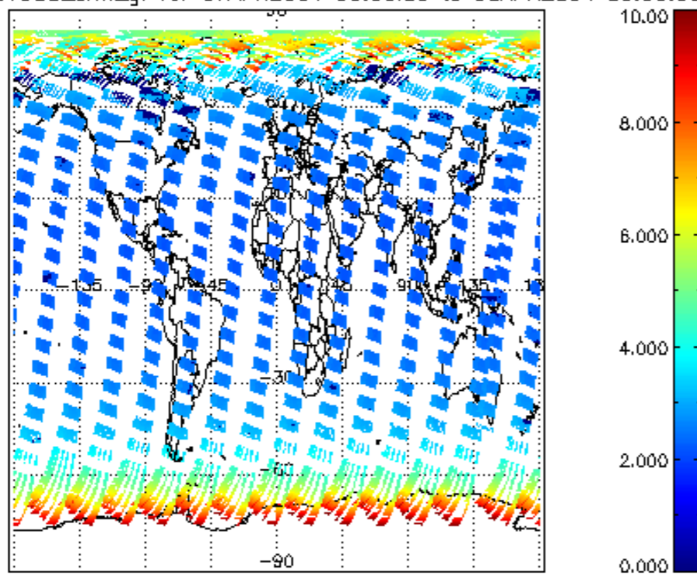
SCIOL2P_NADUV003_amf_gr for 07APR2004 00:00:00 to 08APR2004 00:00:00
