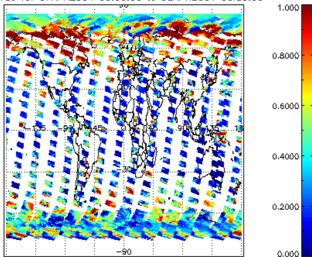
cL_frac for 07APR2004 00:00:00 to 08APR2004 00:00:00
