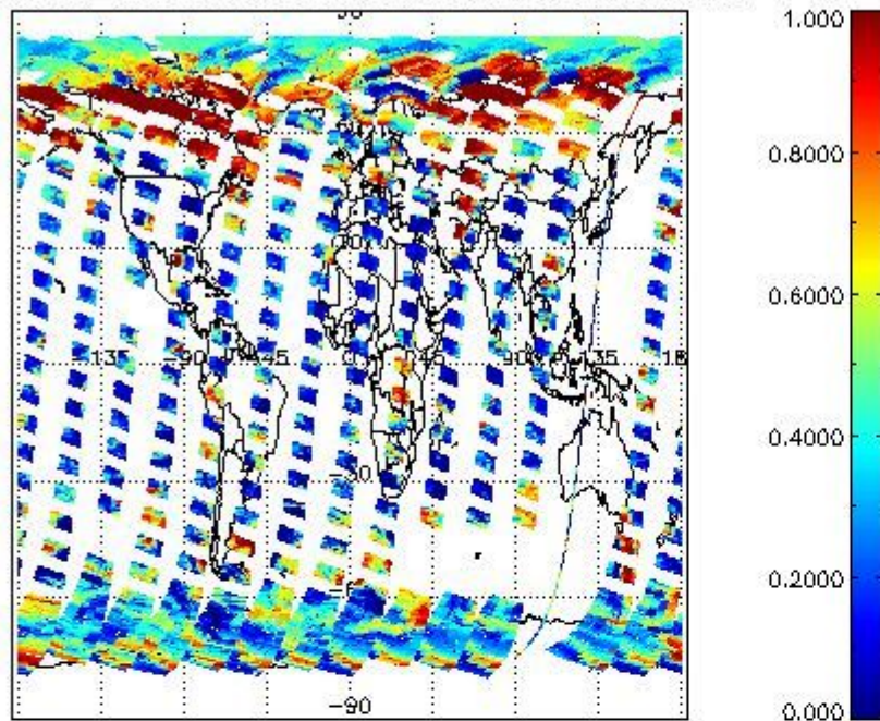
cL_frac for 05APR2004 00:00:00 to 06APR2004 00:00:00
