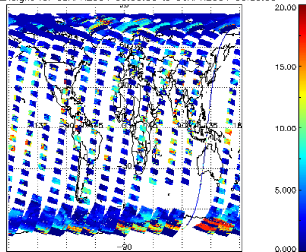
cl_top_height for 05APR2004 00:00:00 to 06APR2004 00:00:00
