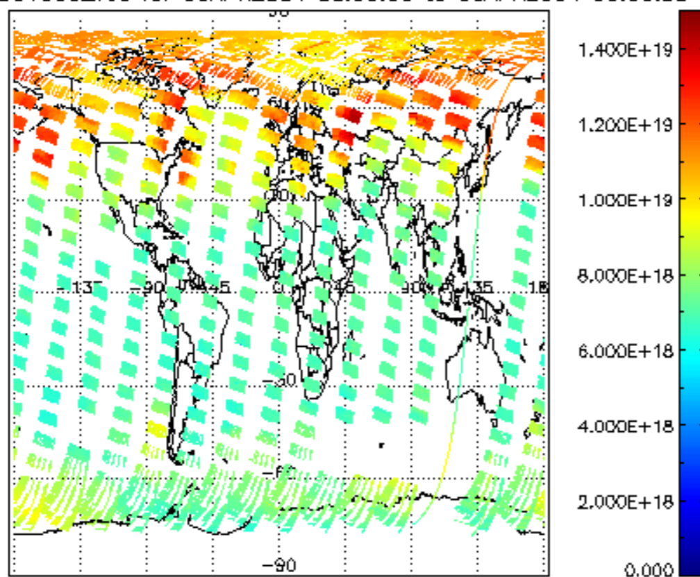
SCIOL2P_NADUV003_vcd for 05APR2004 00:00:00 to 06APR2004 00:00:00
