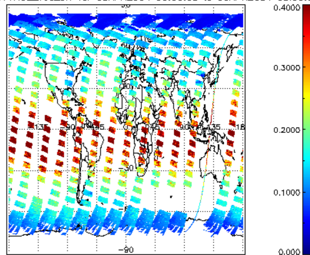
iCIOL2P_NADUV1NO2_vcd_err for 05APR2004 00:00:00 to 06APR2004 00:00:00
