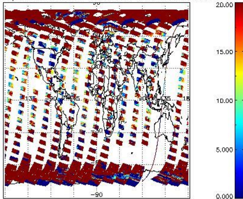
cL_opt_depth for 05APR2004 00:00:00 to 06APR2004 00:00:00
