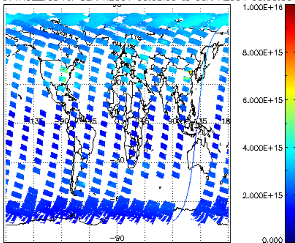
SCIOL2P_NADUV1NO2_vcd for 05APR2004 00:00:00 to 06APR2004 00:00:00
