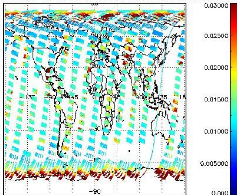
SCIOL2P_NADUV003_vcd_err for 05APR2004 00:00:00 to 06APR2004 00:00:00
