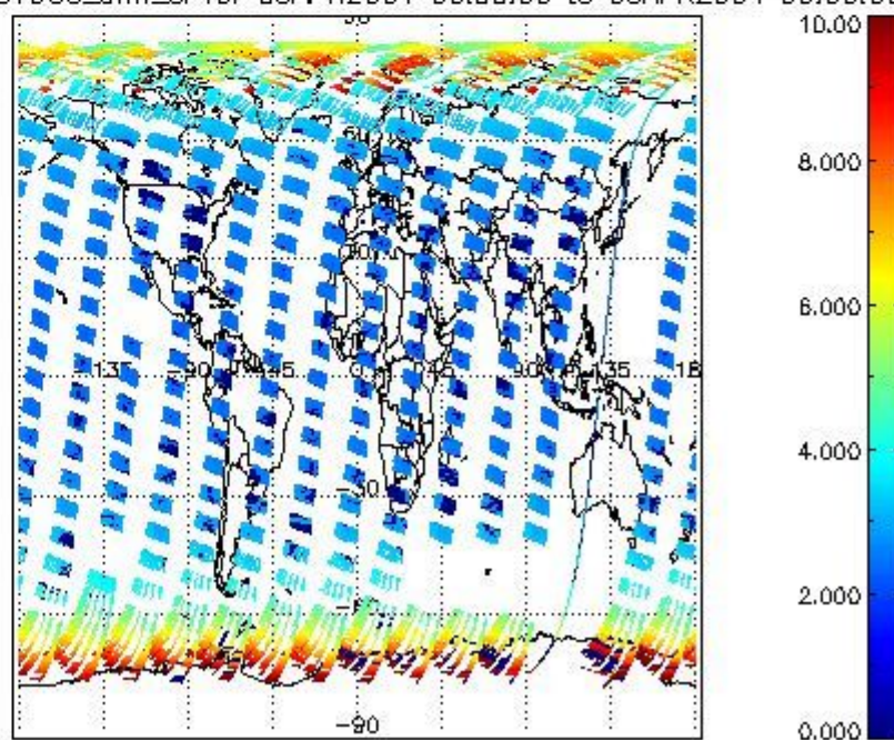
SCIOL2P_NADUV003_amf_cl for 05APR2004 00:00:00 to 06APR2004 00:00:00
