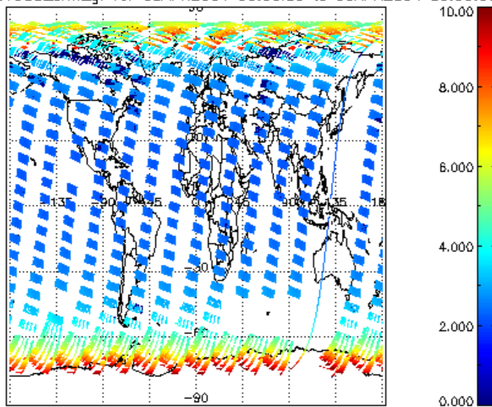
SCIOL2P_NADUV003_amf_gr for 05APR2004 00:00:00 to 06APR2004 00:00:00
