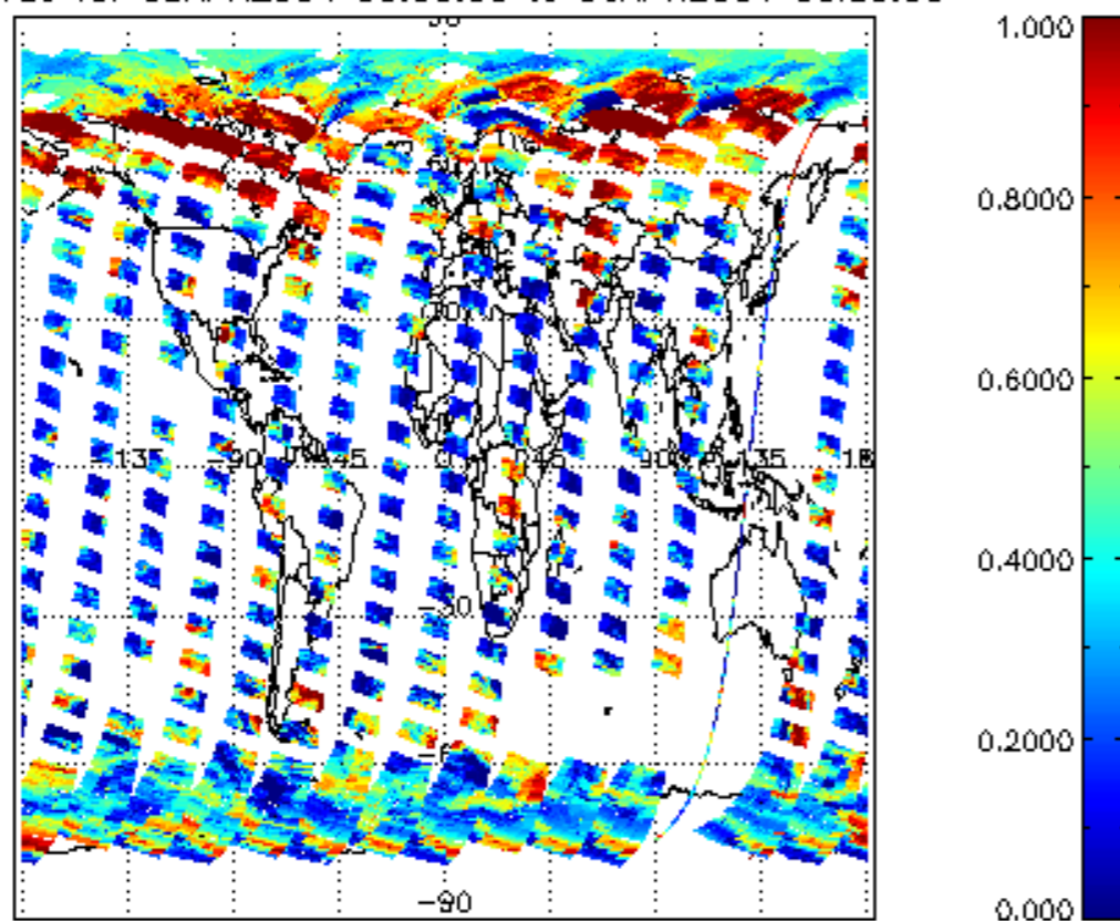
cl_frac for 05APR2004 00:00:00 to 06APR2004 00:00:00
