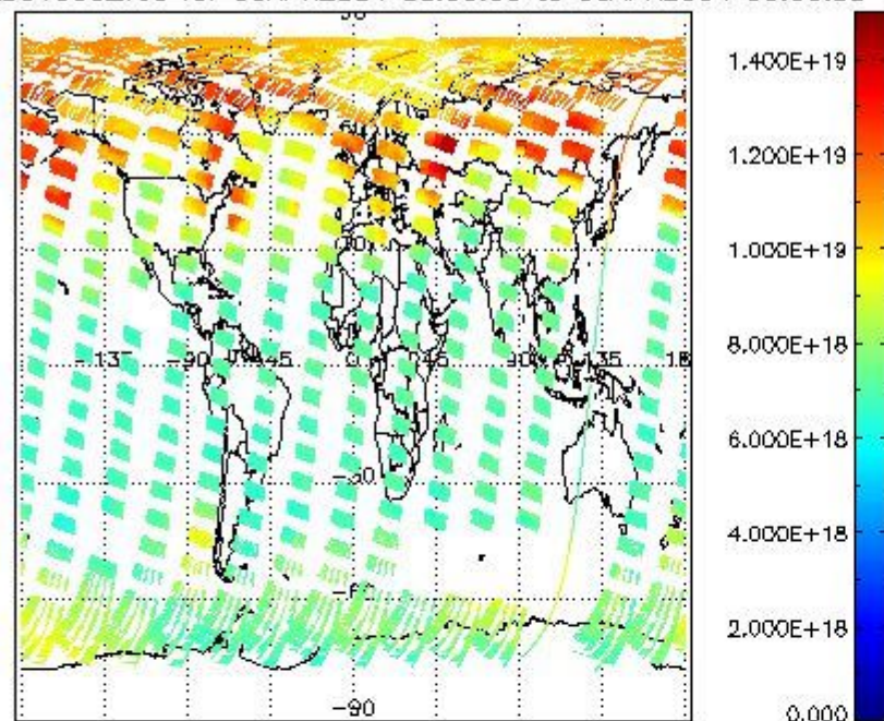
SCIOL2P_NADUV003_vcd for 05APR2004 00:00:00 to 06APR2004 00:00:00
