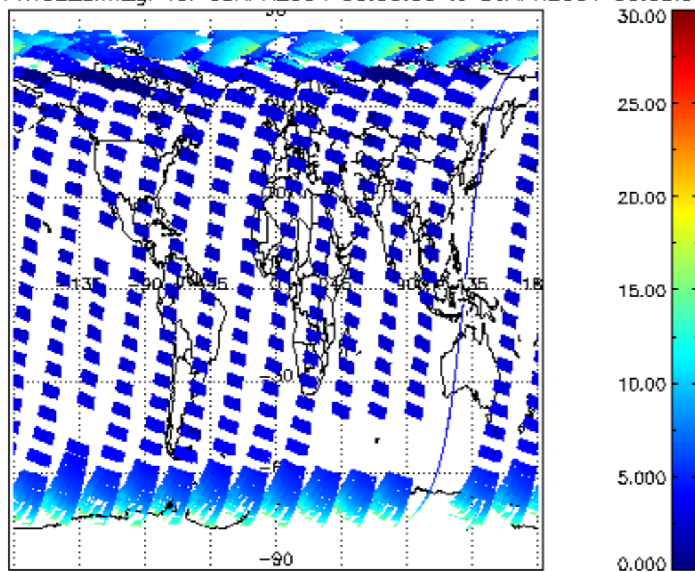
iCIOL2P_NADUV1NO2_amf_gr for 05APR2004 00:00:00 to 06APR2004 00:00:00
