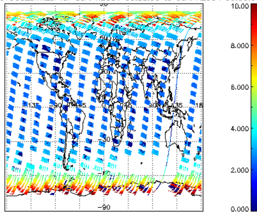
SCIOL2P_NADUV003_amf_cl for 05APR2004 00:00:00 to 06APR2004 00:00:00
