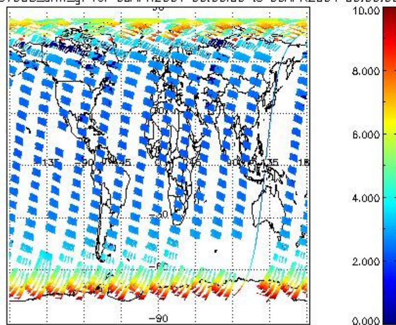
SCIOL2P_NADUV003_amf_gr for 05APR2004 00:00:00 to 06APR2004 00:00:00
