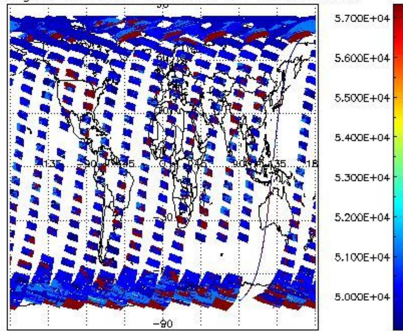
cloud_flags for 05APR2004 00:00:00 to 06APR2004 00:00:00
