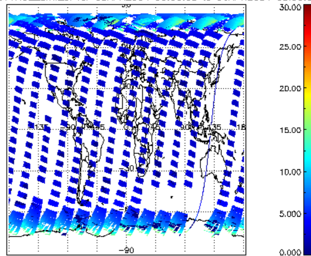
iCIOL2P_NADUV1NO2_amf_cl for 05APR2004 00:00:00 to 06APR2004 00:00:00
