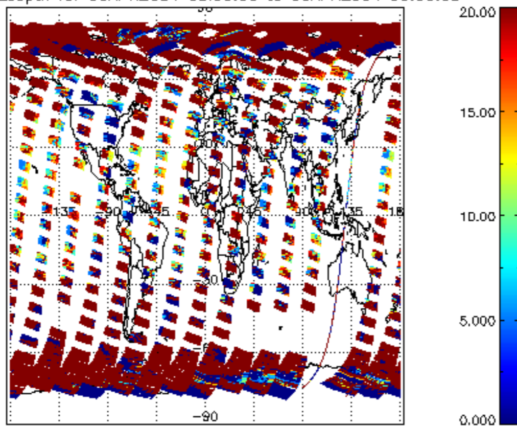
cl_opt_depth for 05APR2004 00:00:00 to 06APR2004 00:00:00
