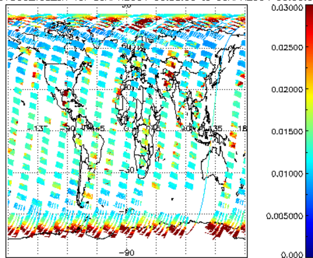
SCIOL2P_NADUV003_vcd_err for 05APR2004 00:00:00 to 06APR2004 00:00:00
