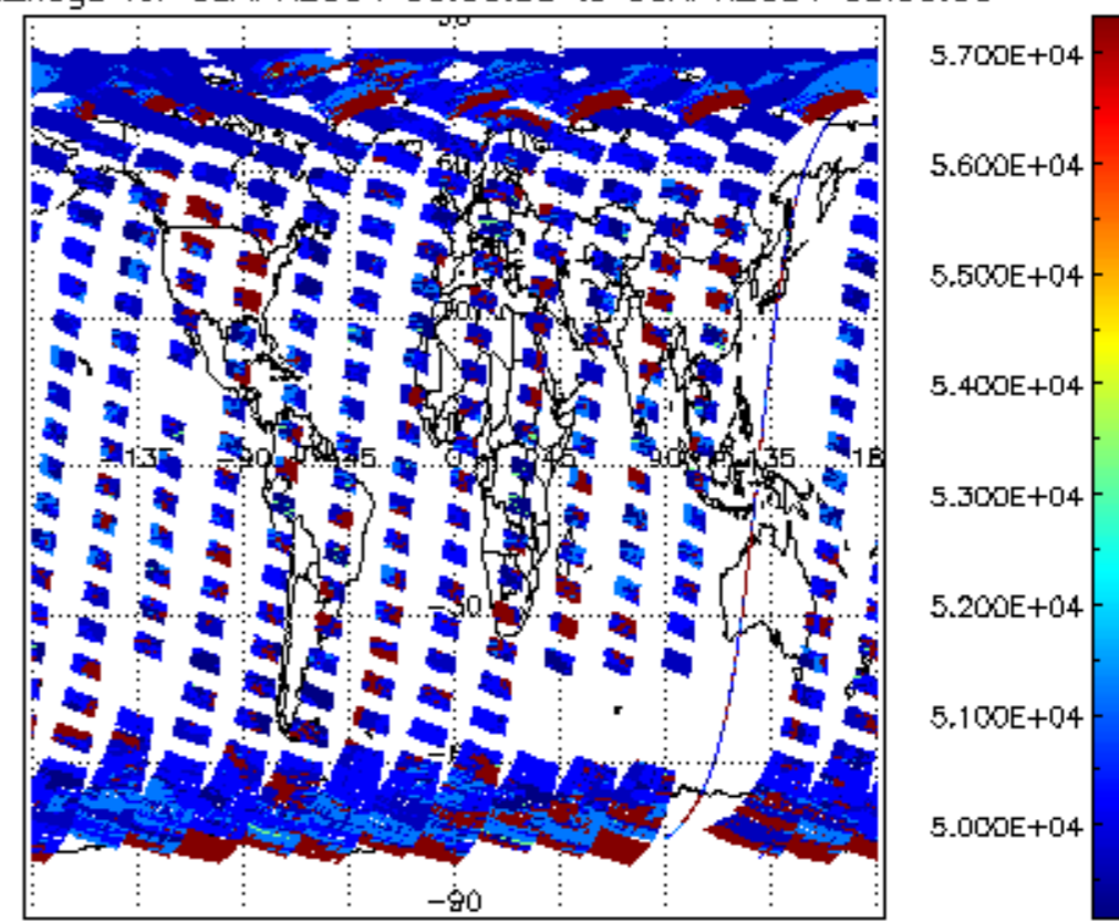
cloud_flags for 05APR2004 00:00:00 to 06APR2004 00:00:00
