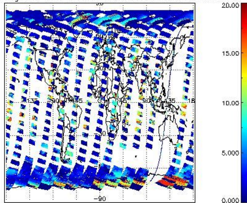
cL_top_height for 05APR2004 00:00:00 to 06APR2004 00:00:00
