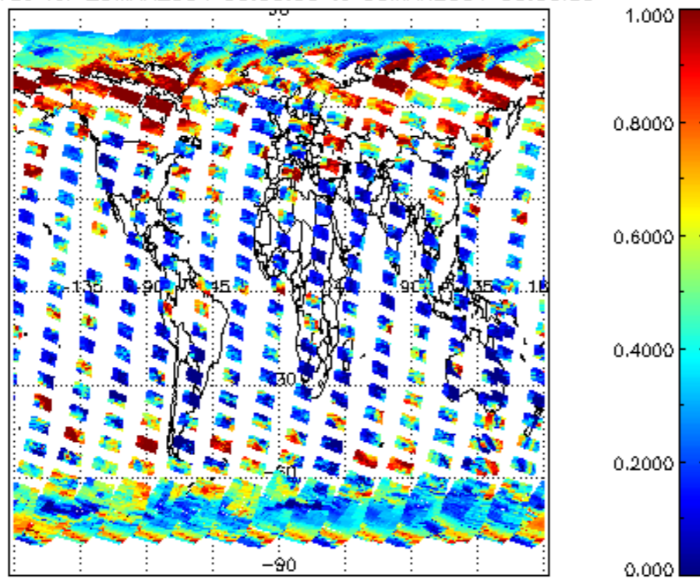
cL_frac for 29MAR2004 00:00:00 to 30MAR2004 00:00:00
