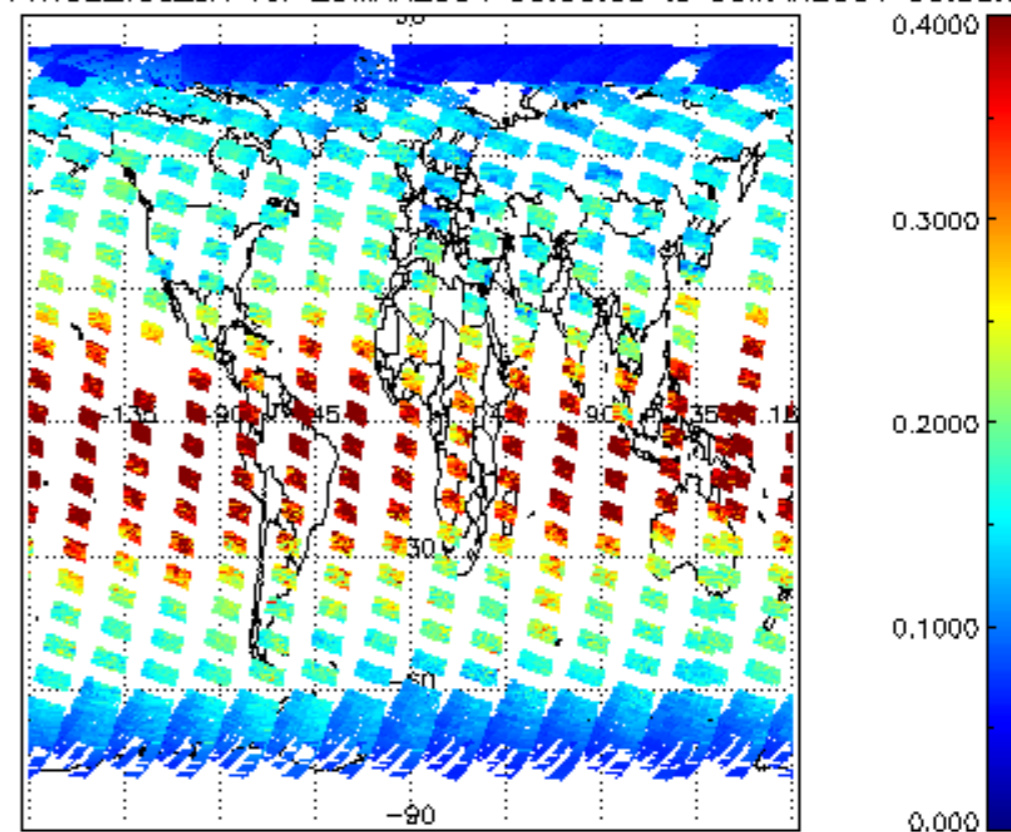
CIOL2P_NADUV1NO2_vcd_err for 29MAR2004 00:00:00 to 30MAR2004 00:00:00
