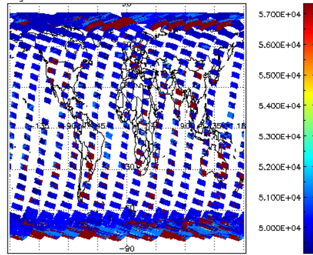
cloud_flags for 29MAR2004 00:00:00 to 30MAR2004 00:00:00
