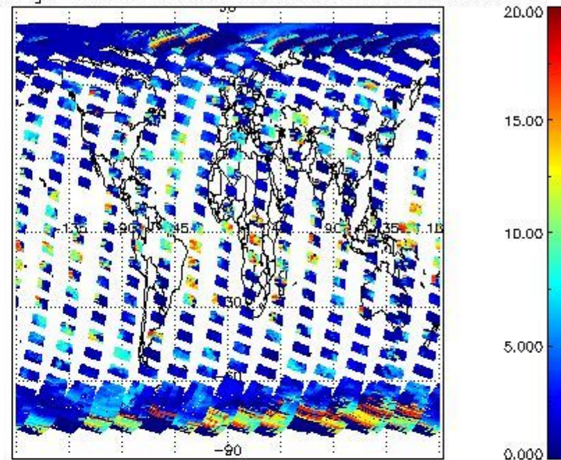
cL_top_height for 29MAR2004 00:00:00 to 30MAR2004 00:00:00
