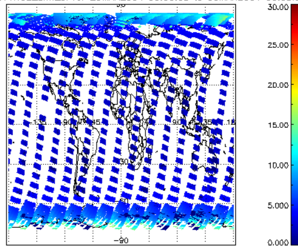
CIOL2P_NADUV1NO2_amf_cl for 29MAR2004 00:00:00 to 30MAR2004 00:00:00
