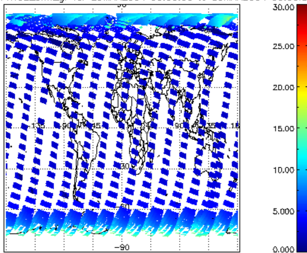
CIOL2P_NADUV1NO2_amf_gr for 29MAR2004 00:00:00 to 30MAR2004 00:00:00
