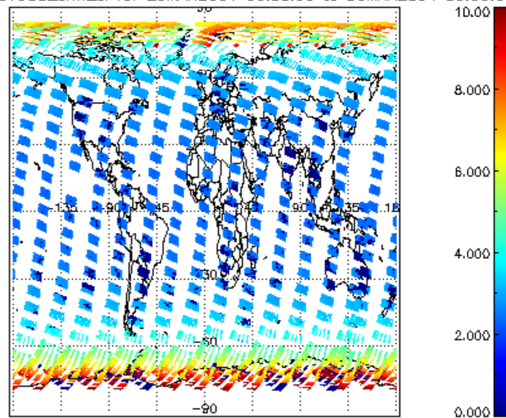
SCIOL2P_NADUV003_amf_cl for 29MAR2004 00:00:00 to 30MAR2004 00:00:00
