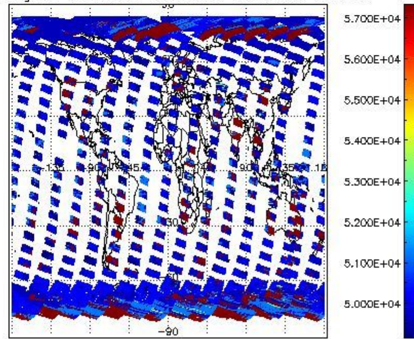
cloud_flags for 29MAR2004 00:00:00 to 30MAR2004 00:00:00
