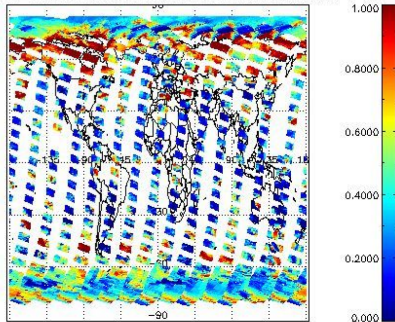
cL_frac for 29MAR2004 00:00:00 to 30MAR2004 00:00:00
