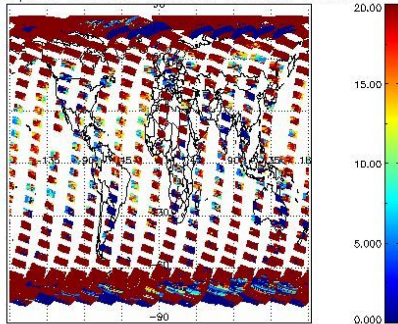
cL_opt_depth for 29MAR2004 00:00:00 to 30MAR2004 00:00:00
