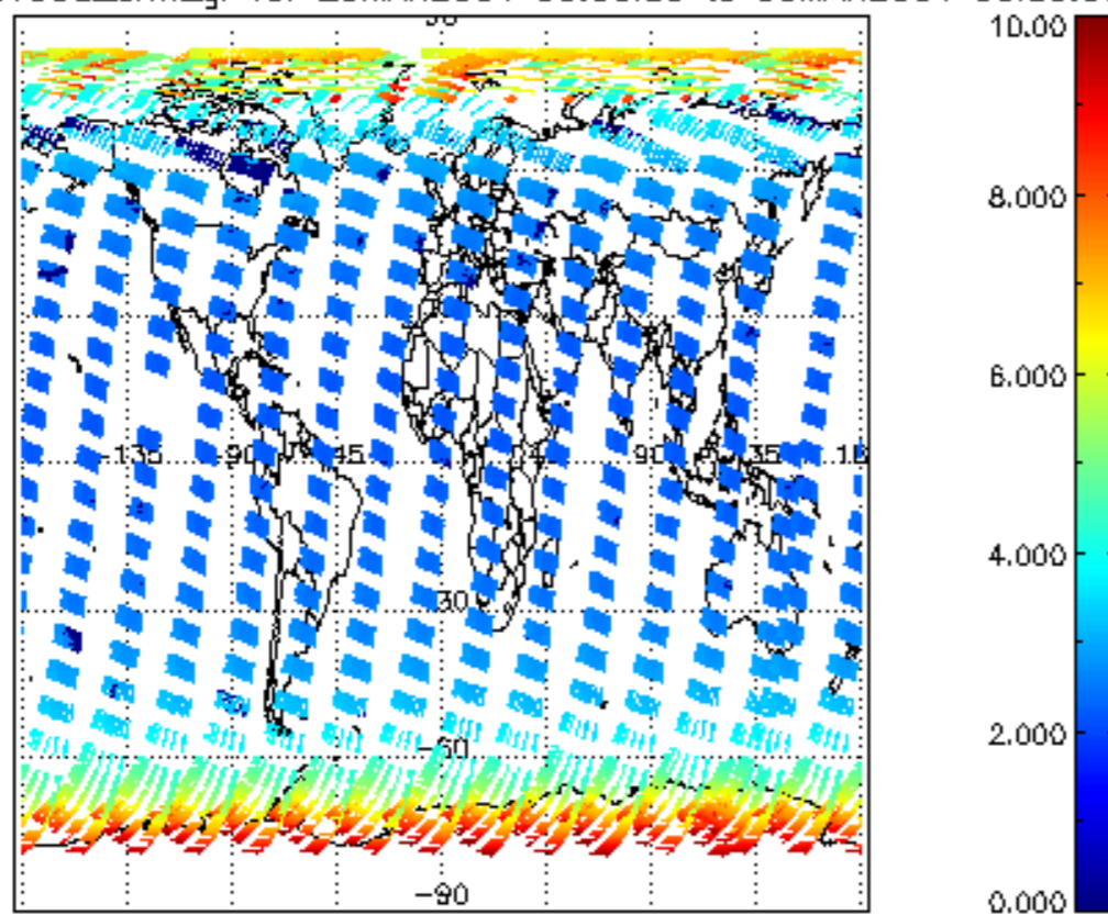
SCIOL2P_NADUV003_amf_gr for 29MAR2004 00:00:00 to 30MAR2004 00:00:00
