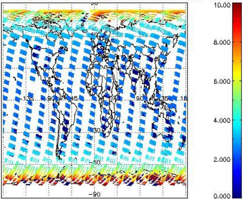
SCIOL2P_NADUV003_amf_cl for 29MAR2004 00:00:00 to 30MAR2004 00:00:00
