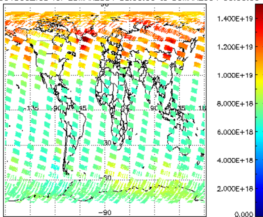
SCIOL2P_NADUV003_vcd for 29MAR2004 00:00:00 to 30MAR2004 00:00:00
