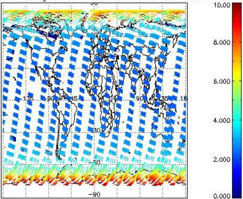
SCIOL2P_NADUV003_amf_gr for 29MAR2004 00:00:00 to 30MAR2004 00:00:00
