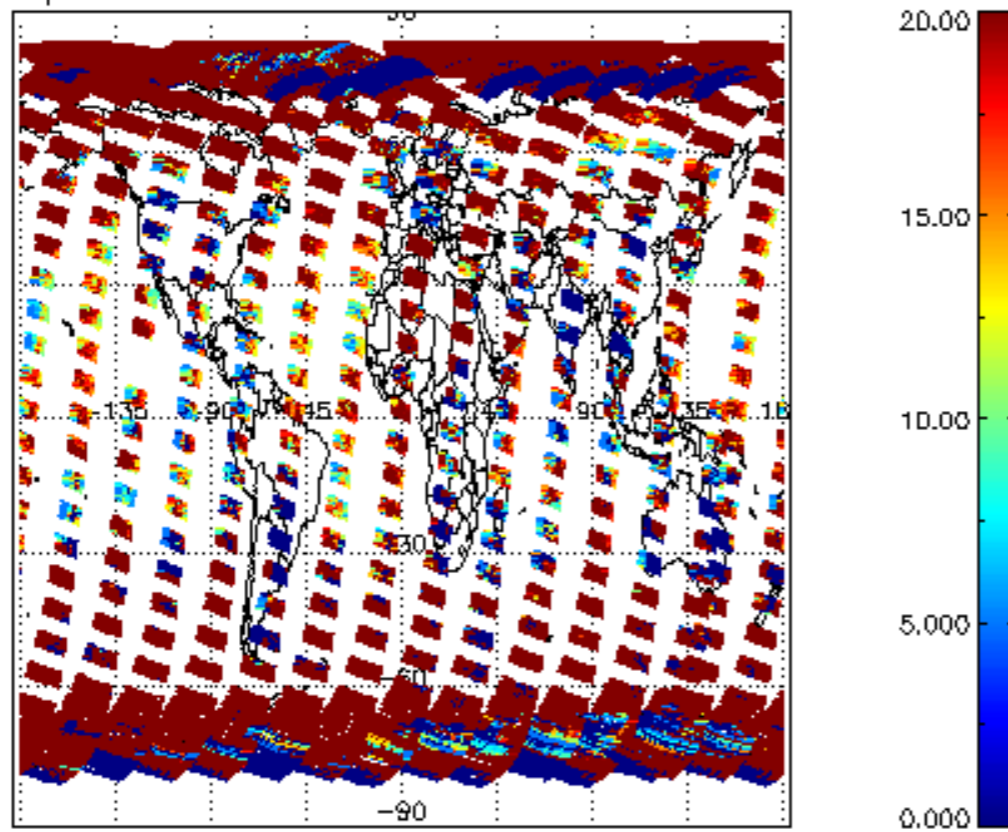
cL_opt_depth for 29MAR2004 00:00:00 to 30MAR2004 00:00:00
