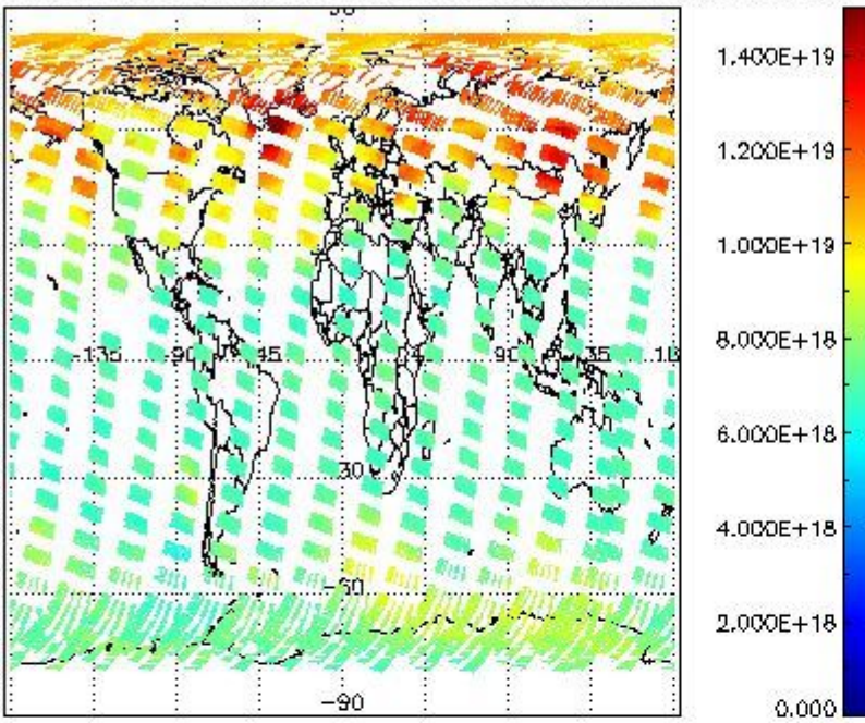
SCIOL2P_NADUV003_vcd for 29MAR2004 00:00:00 to 30MAR2004 00:00:00
