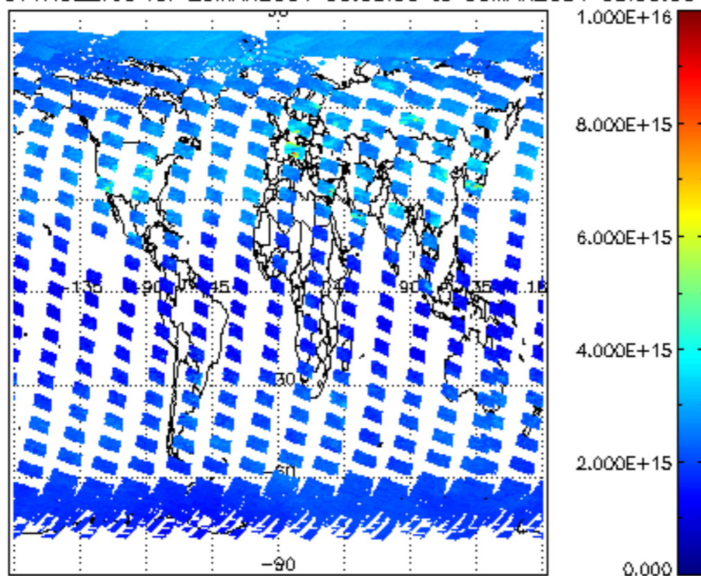
SCIOL2P_NADUV1NO2_vcd for 29MAR2004 00:00:00 to 30MAR2004 00:00:00
