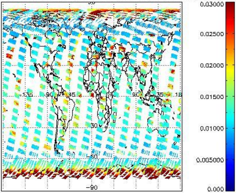
SCIOL2P_NADUV003_vcd_err for 29MAR2004 00:00:00 to 30MAR2004 00:00:00
