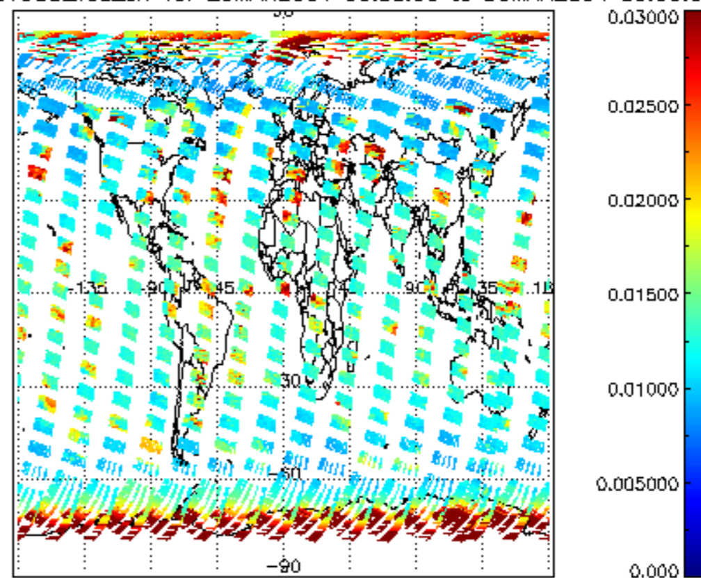
SCIOL2P_NADUV003_vcd_err for 29MAR2004 00:00:00 to 30MAR2004 00:00:00
