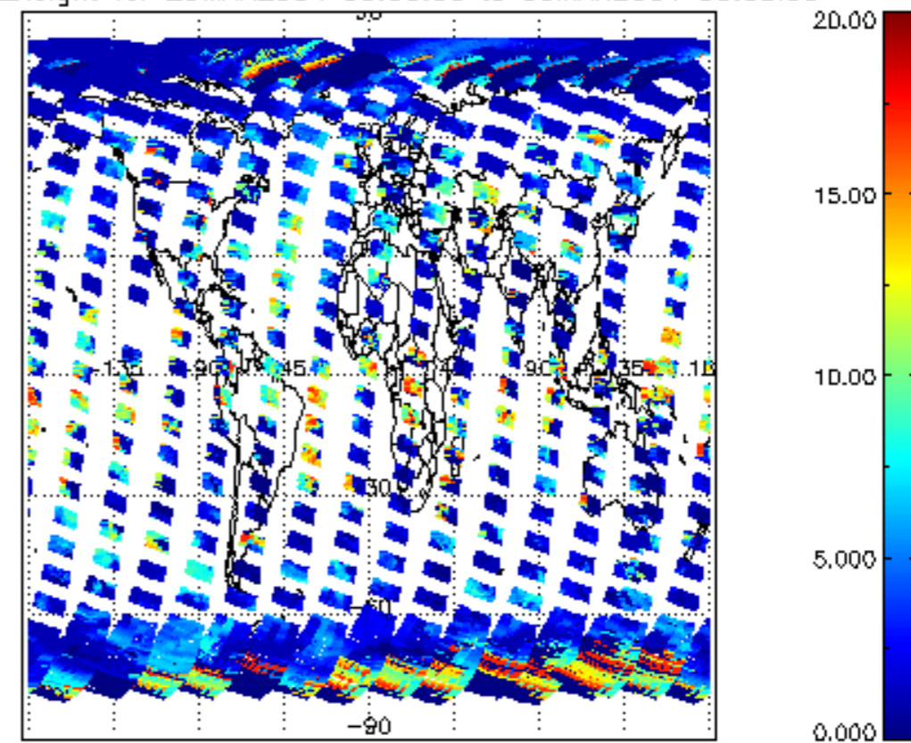
cL_top_height for 29MAR2004 00:00:00 to 30MAR2004 00:00:00
