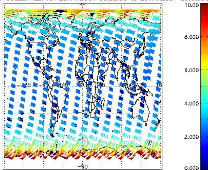
SCIOL2P_NADUV003_amf_cl for 28MAR2004 00:00:00 to 29MAR2004 00:00:00
