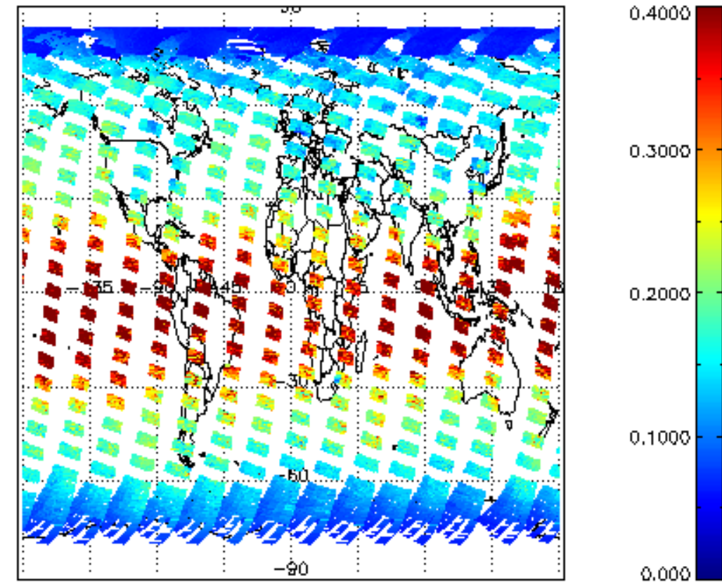
SCIOL2P_NADUV1NO2_vcd_err for 28MAR2004 00:00:00 to 29MAR2004 00:00:00
