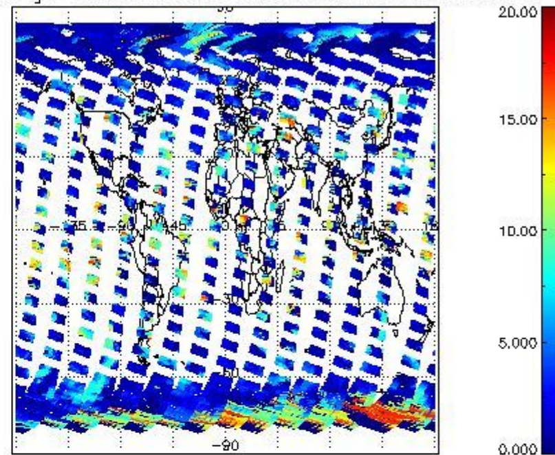
cL_top_height for 28MAR2004 00:00:00 to 29MAR2004 00:00:00
