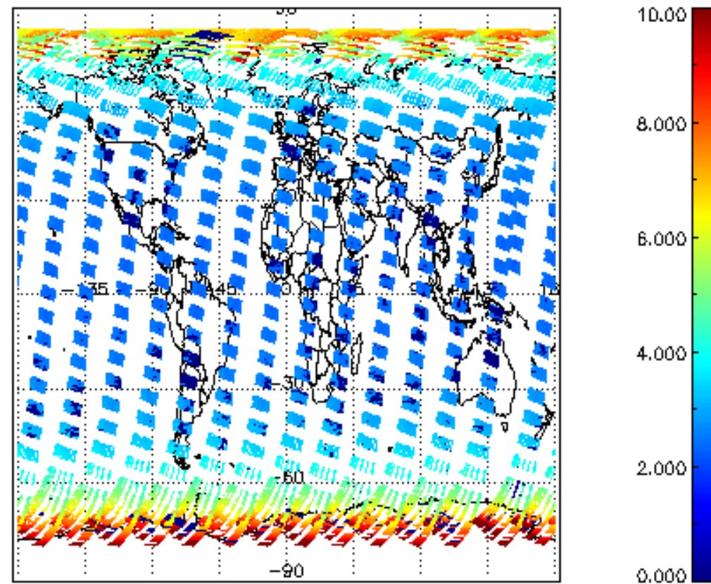
SCIOL2P_NADUV003_amf_cl for 28MAR2004 00:00:00 to 29MAR2004 00:00:00
