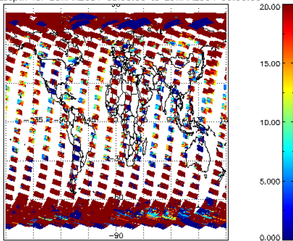
cL_opt_depth for 28MAR2004 00:00:00 to 29MAR2004 00:00:00
