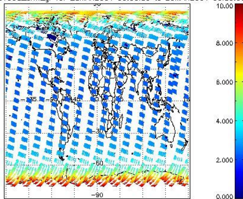
SCIOL2P_NADUV003_amf_gr for 28MAR2004 00:00:00 to 29MAR2004 00:00:00
