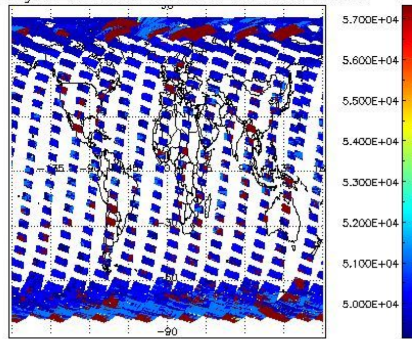
cloud_flags for 28MAR2004 00:00:00 to 29MAR2004 00:00:00
