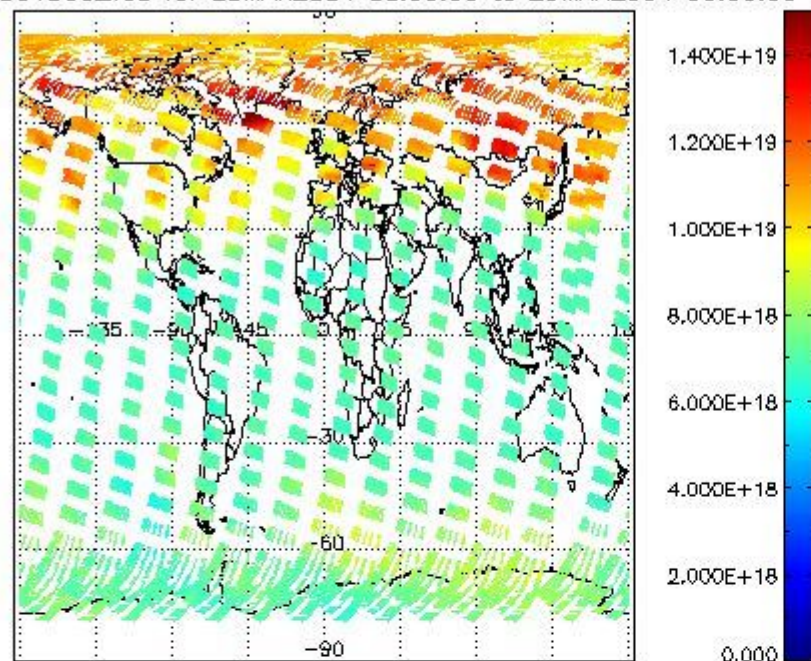
SCIOL2P_NADUV003_vcd for 28MAR2004 00:00:00 to 29MAR2004 00:00:00
