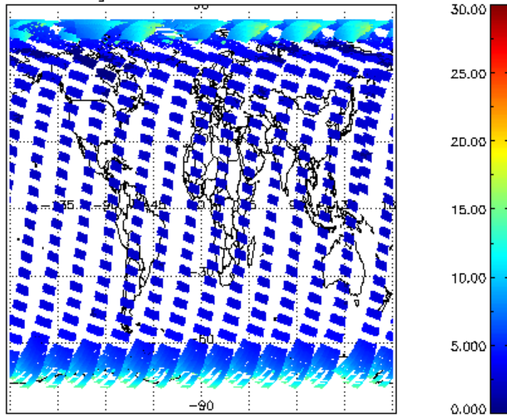
SCIOL2P_NADUV1NO2_amf_gr for 28MAR2004 00:00:00 to 29MAR2004 00:00:00
