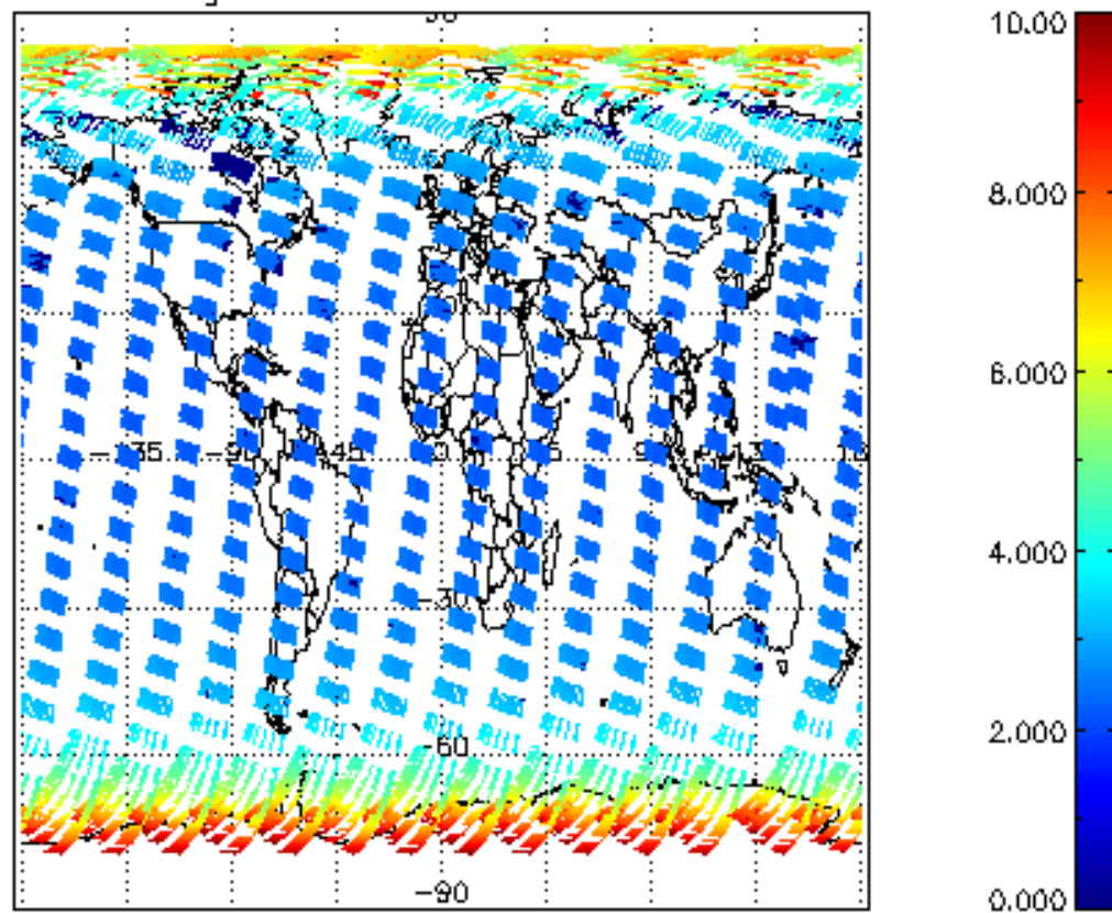
SCIOL2P_NADUV003_amf_gr for 28MAR2004 00:00:00 to 29MAR2004 00:00:00
