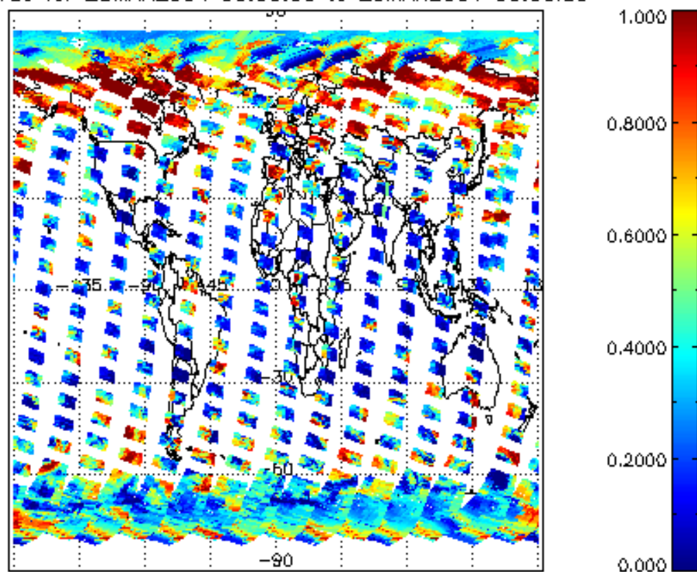
cL_frac for 28MAR2004 00:00:00 to 29MAR2004 00:00:00
