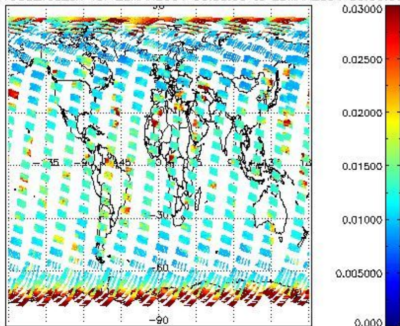
SCIOL2P_NADUV003_vcd_err for 28MAR2004 00:00:00 to 29MAR2004 00:00:00
