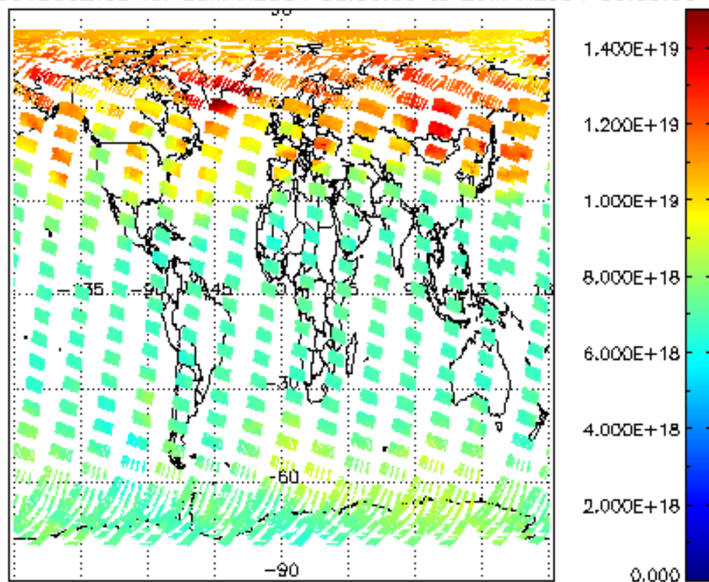
SCIOL2P_NADUV003_vcd for 28MAR2004 00:00:00 to 29MAR2004 00:00:00
