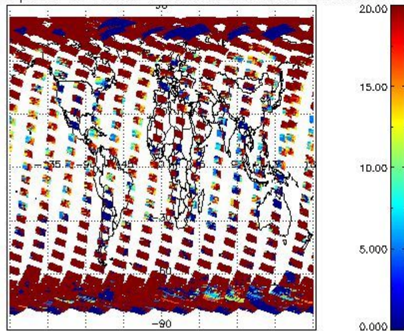
cL_opt_depth for 28MAR2004 00:00:00 to 29MAR2004 00:00:00
