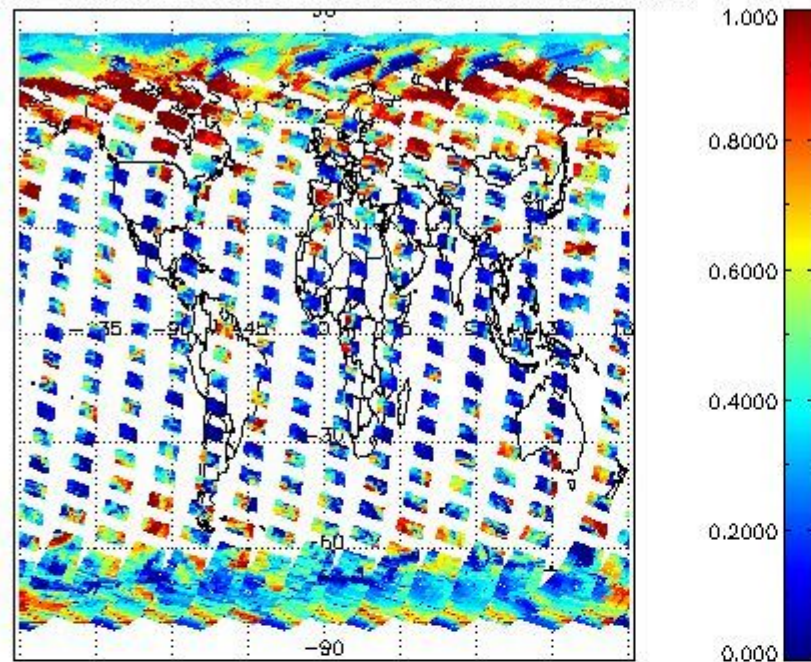
cL_frac for 28MAR2004 00:00:00 to 29MAR2004 00:00:00
