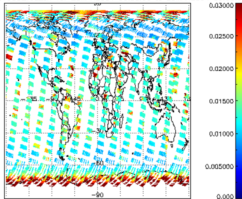
SCIOL2P_NADUV003_vcd_err for 28MAR2004 00:00:00 to 29MAR2004 00:00:00
