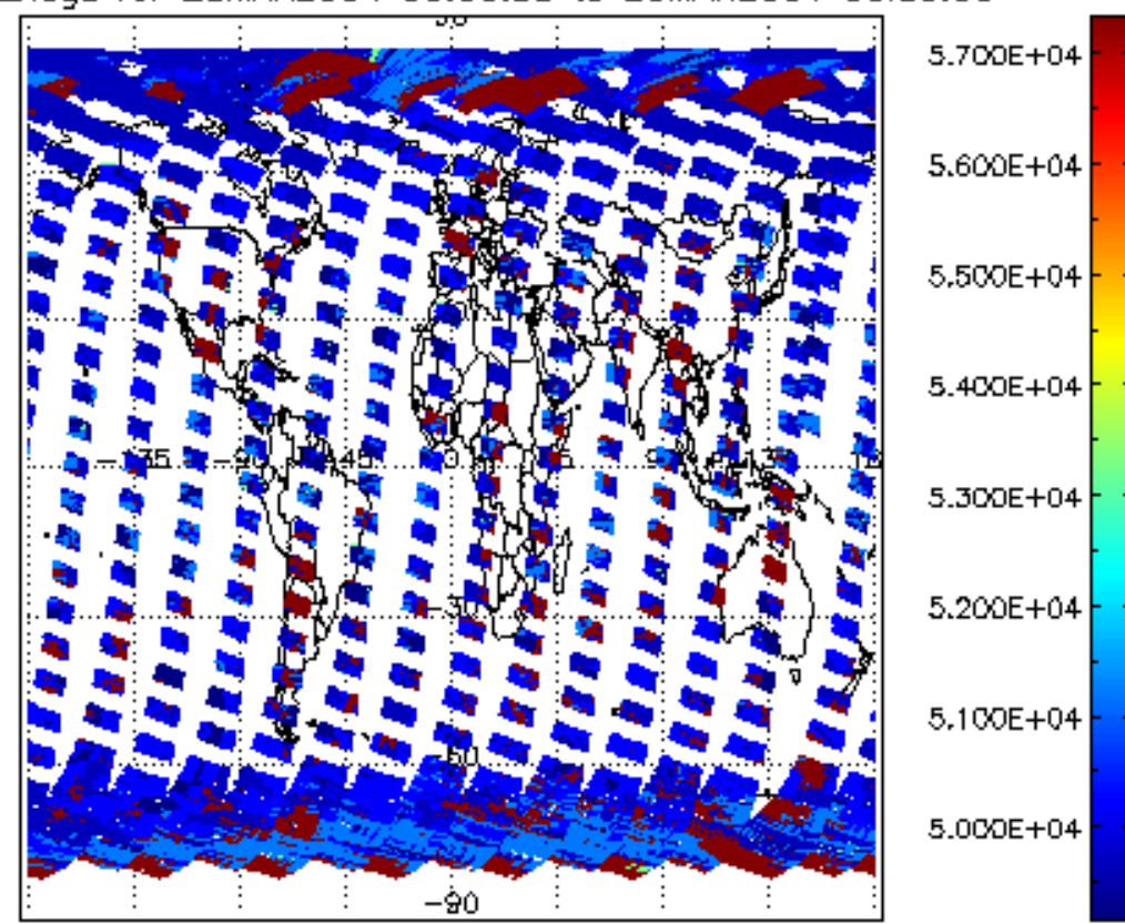
cloud_flags for 28MAR2004 00:00:00 to 29MAR2004 00:00:00
