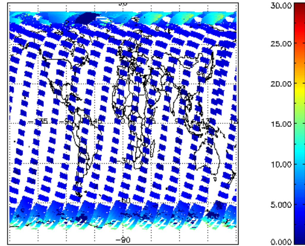
SCIOL2P_NADUV1NO2_amf_cl for 28MAR2004 00:00:00 to 29MAR2004 00:00:00
