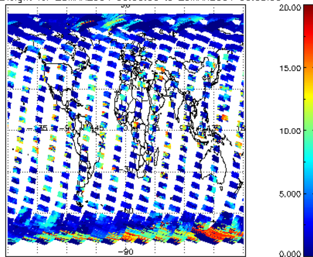
cL_top_height for 28MAR2004 00:00:00 to 29MAR2004 00:00:00
