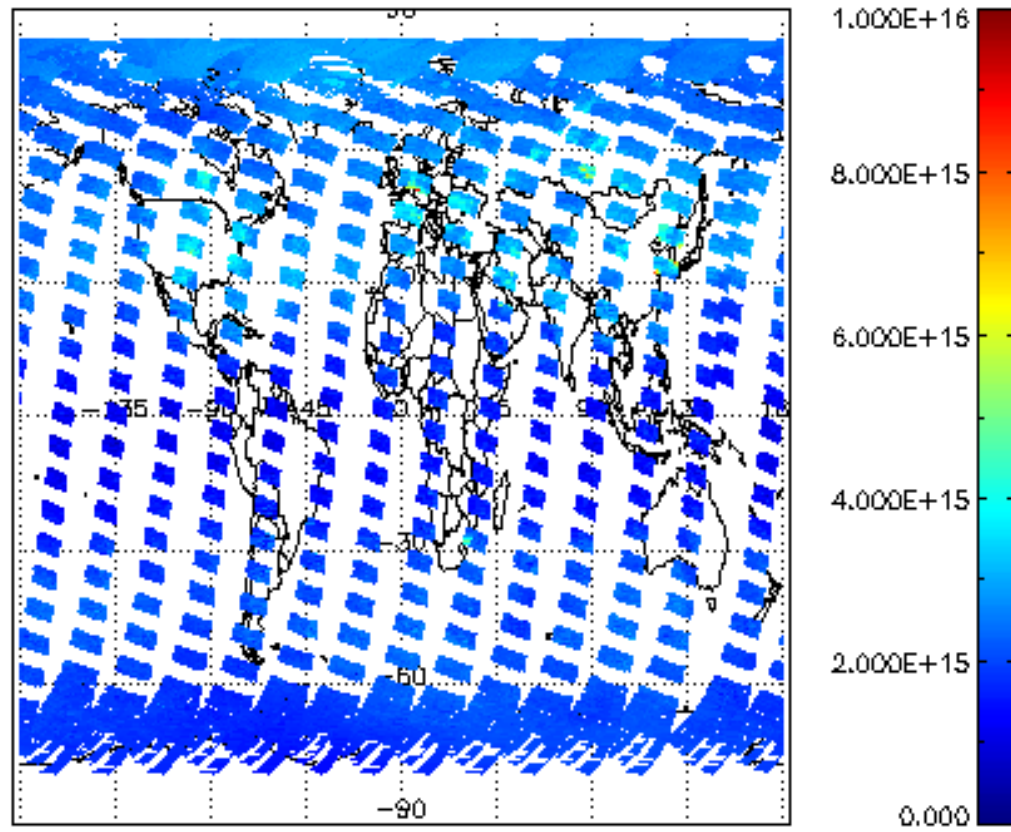
SCIOL2P_NADUV1NO2_vcd for 28MAR2004 00:00:00 to 29MAR2004 00:00:00
