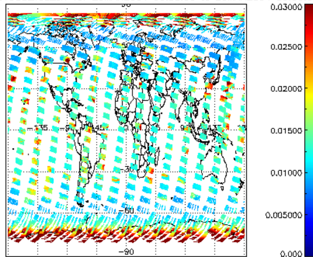
SCIOL2P_NADUV003_vcd_err for 25MAR2004 00:00:00 to 26MAR2004 00:00:00
