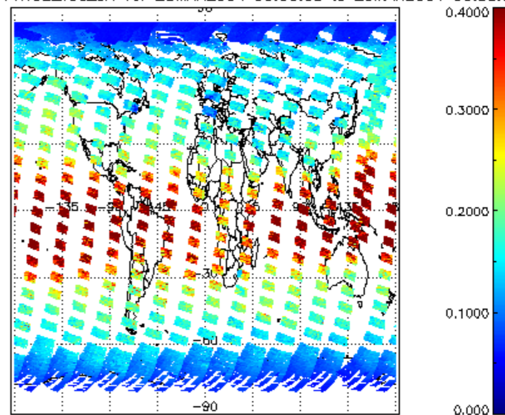
SCIOL2P_NADUV1NO2_vcd_err for 25MAR2004 00:00:00 to 26MAR2004 00:00:00
