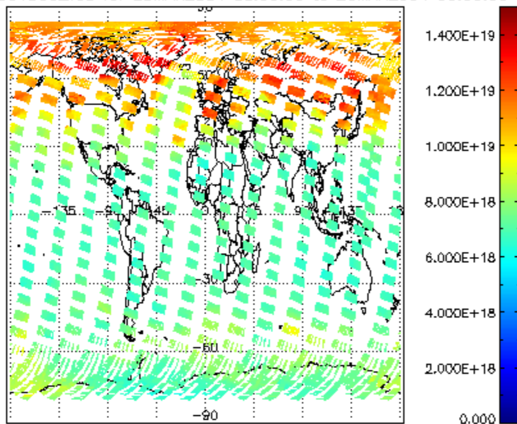
SCIOL2P_NADUV003_vcd for 25MAR2004 00:00:00 to 26MAR2004 00:00:00
