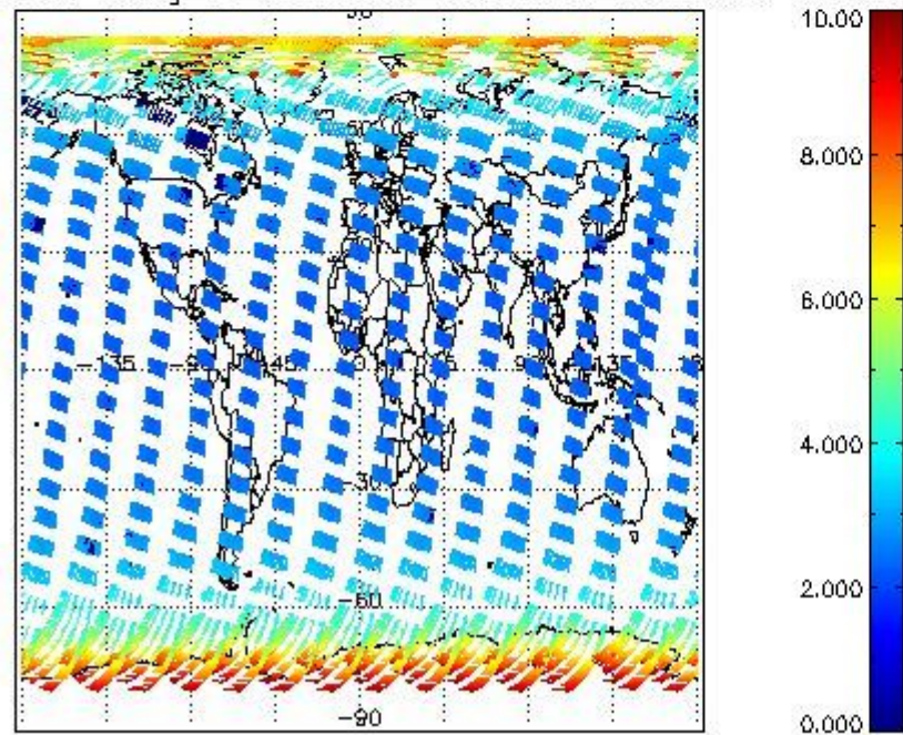
SCIOL2P_NADUV003_amf_gr for 25MAR2004 00:00:00 to 26MAR2004 00:00:00 SCIOL2P_NADUV003_amf_cl for 25MAR2004 00:00:00 to 26MAR2004 00:00:00
