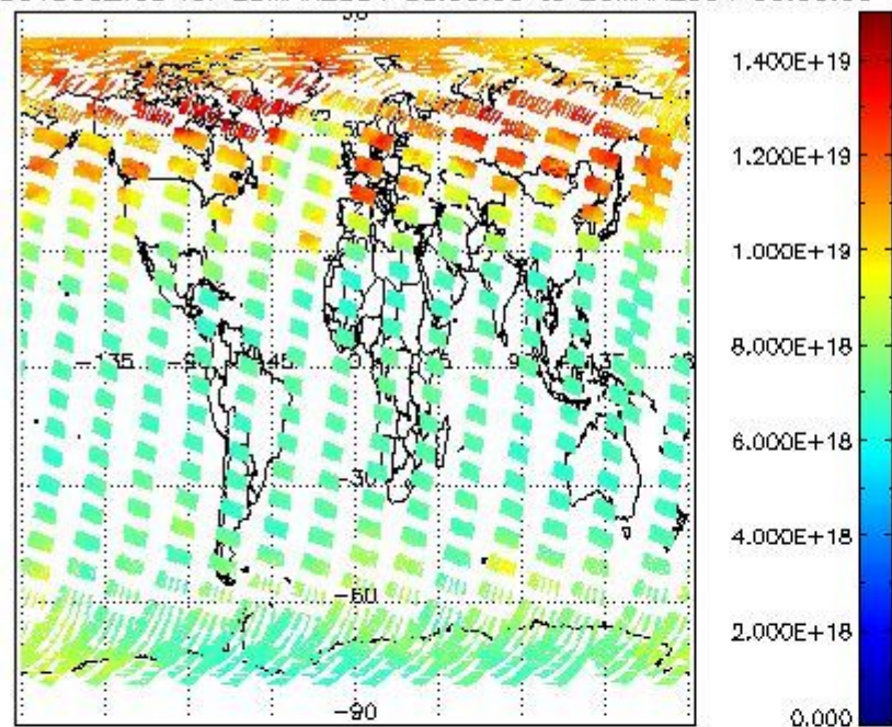
SCIOL2P_NADUV003_vcd for 25MAR2004 00:00:00 to 26MAR2004 00:00:00 SCIOL2P_NADUV003_vcd_err for 25MAR2004 00:00:00 to 26MAR2004 00:00:00
