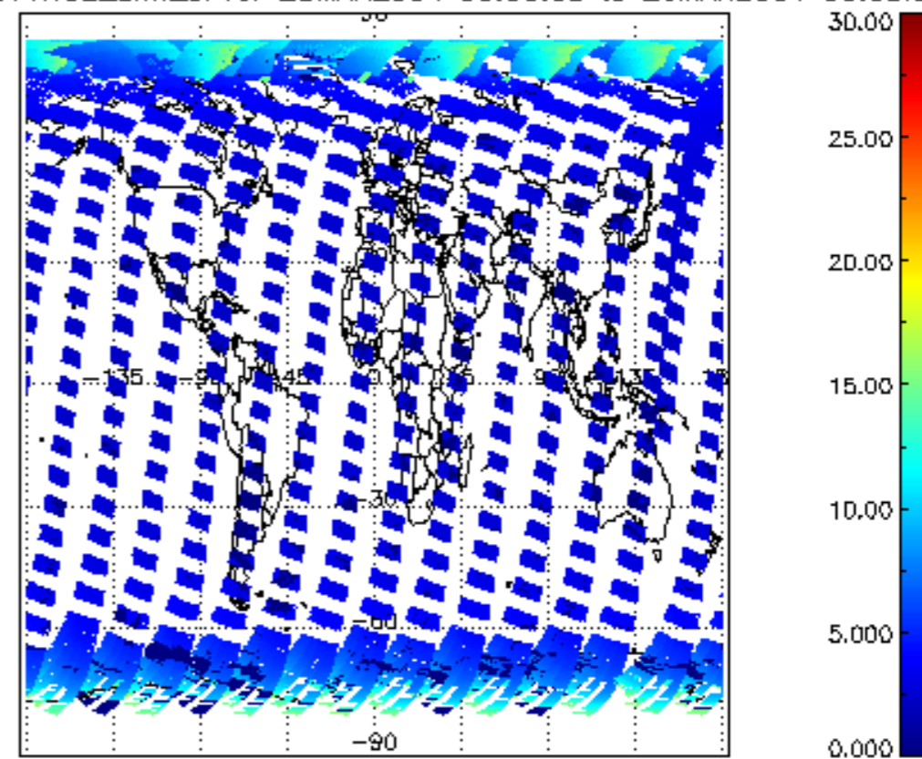
SCIOL2P_NADUV1NO2_amf_cl for 25MAR2004 00:00:00 to 26MAR2004 00:00:00
