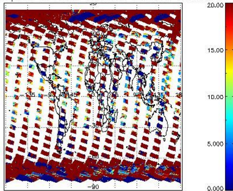
cL_opt_depth for 25MAR2004 00:00:00 to 26MAR2004 00:00:00
