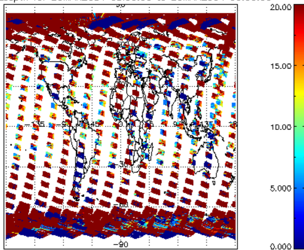
cL_opt_depth for 25MAR2004 00:00:00 to 26MAR2004 00:00:00
