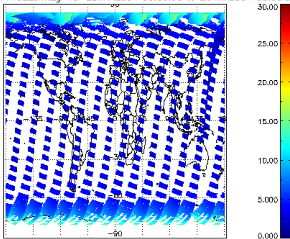
SCIOL2P_NADUV1NO2_amf_gr for 25MAR2004 00:00:00 to 26MAR2004 00:00:00
