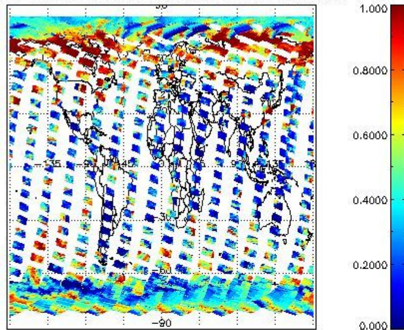
cL_frac for 25MAR2004 00:00:00 to 26MAR2004 00:00:00
