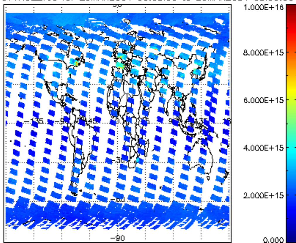
SCIOL2P_NADUV1NO2_vcd for 25MAR2004 00:00:00 to 26MAR2004 00:00:00
