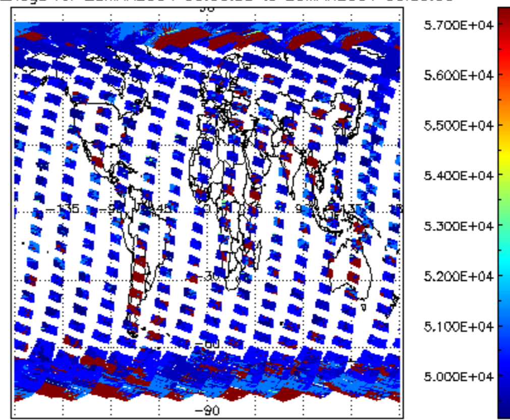
cloud_flags for 25MAR2004 00:00:00 to 26MAR2004 00:00:00
