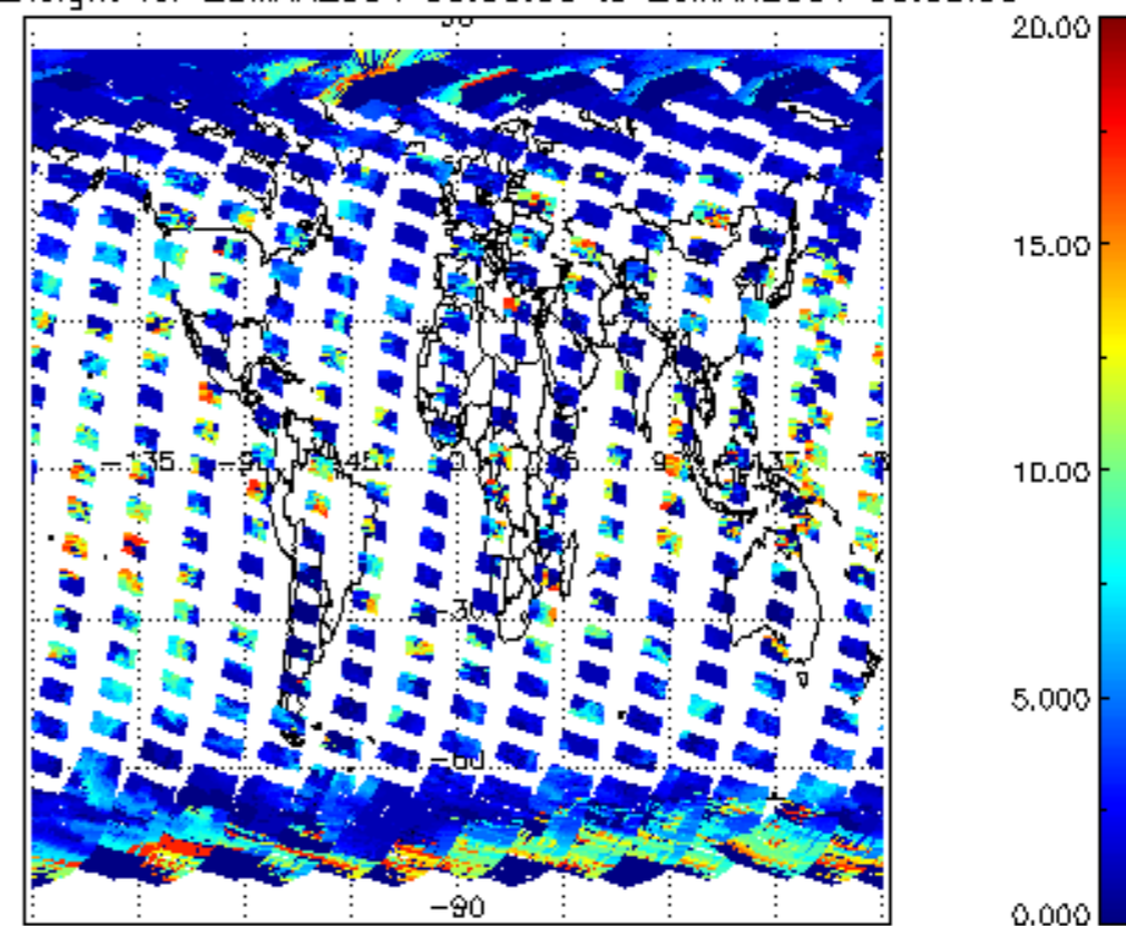
cL_top_height for 25MAR2004 00:00:00 to 26MAR2004 00:00:00
