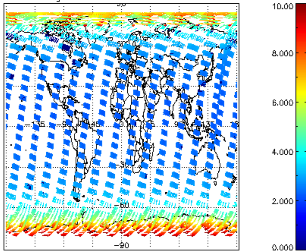
SCIOL2P_NADUV003_amf_gr for 25MAR2004 00:00:00 to 26MAR2004 00:00:00
