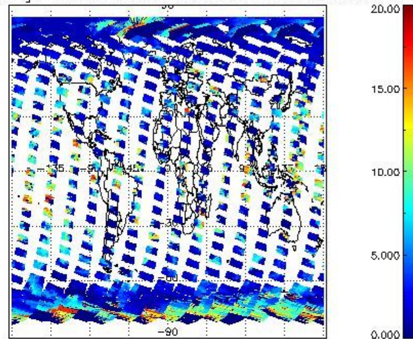
cL_top_height for 25MAR2004 00:00:00 to 26MAR2004 00:00:00
