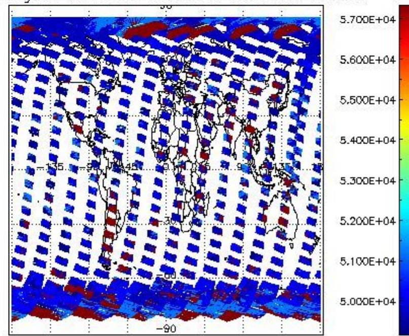
cloud_flags for 25MAR2004 00:00:00 to 26MAR2004 00:00:00
