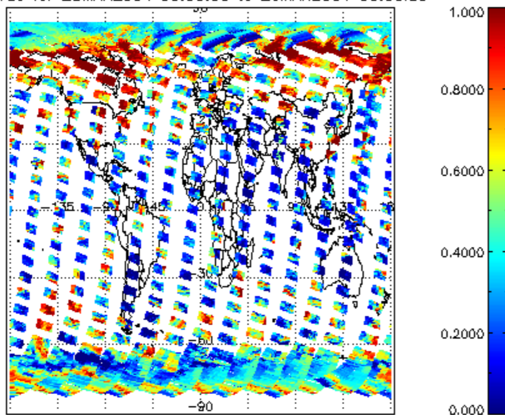
cL_frac for 25MAR2004 00:00:00 to 26MAR2004 00:00:00
