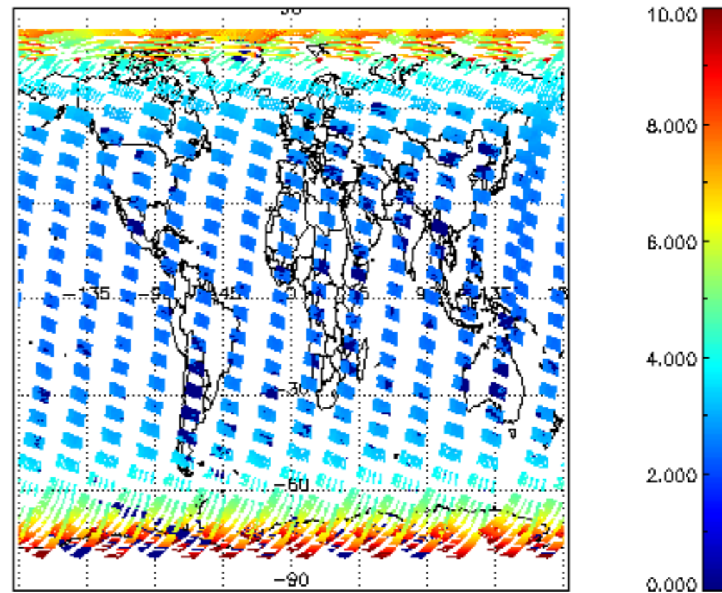
SCIOL2P_NADUV003_amf_cl for 25MAR2004 00:00:00 to 26MAR2004 00:00:00
