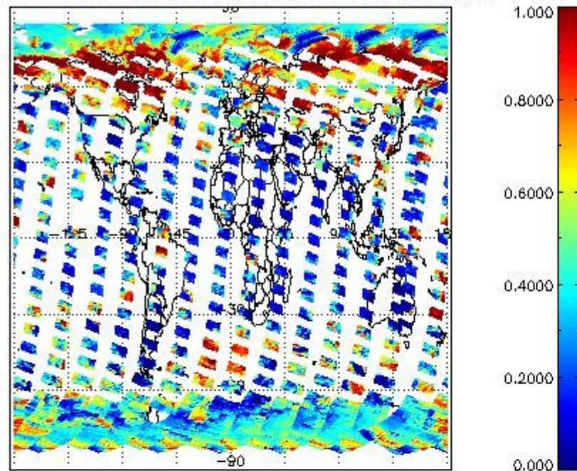
cL_frac for 22MAR2004 00:00:00 to 23MAR2004 00:00:00
