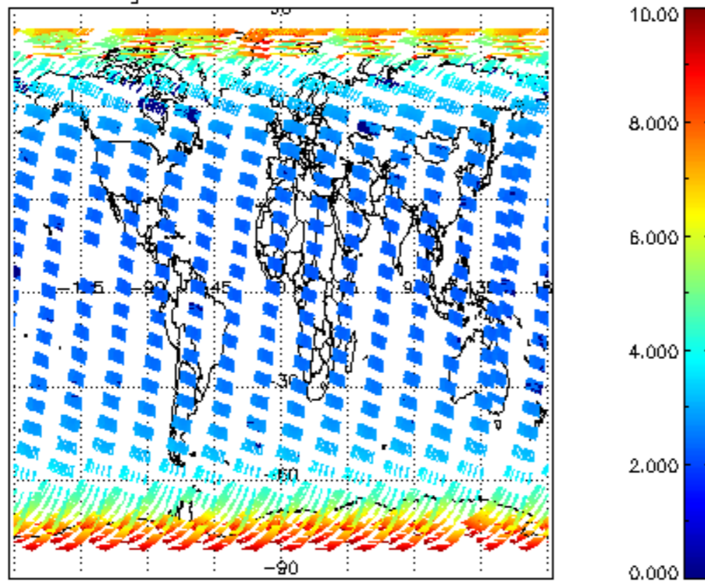
SCIOL2P_NADUV003_amf_gr for 22MAR2004 00:00:00 to 23MAR2004 00:00:00
