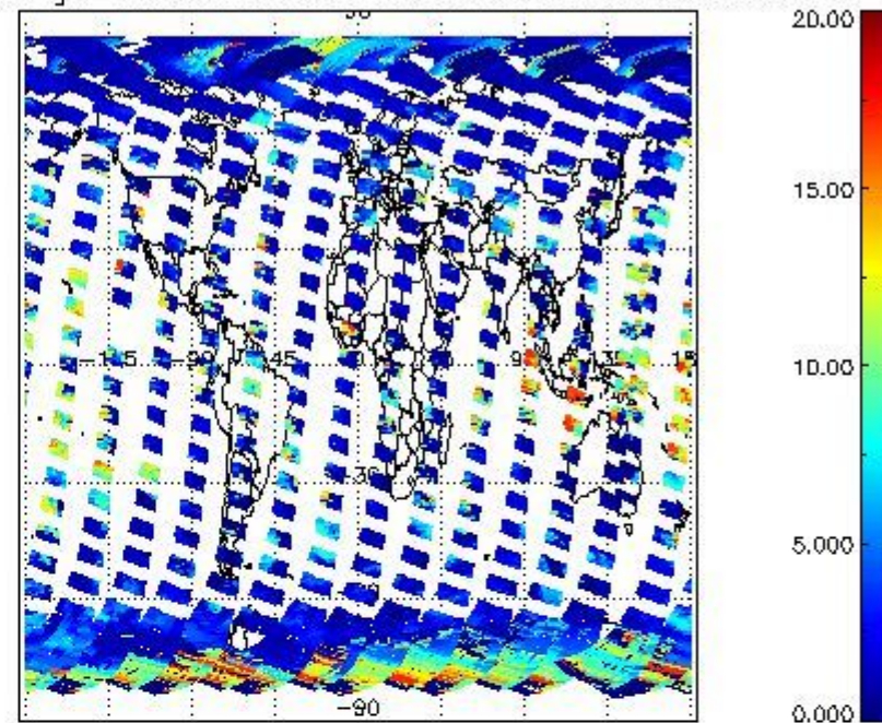
cL_top_height for 22MAR2004 00:00:00 to 23MAR2004 00:00:00
