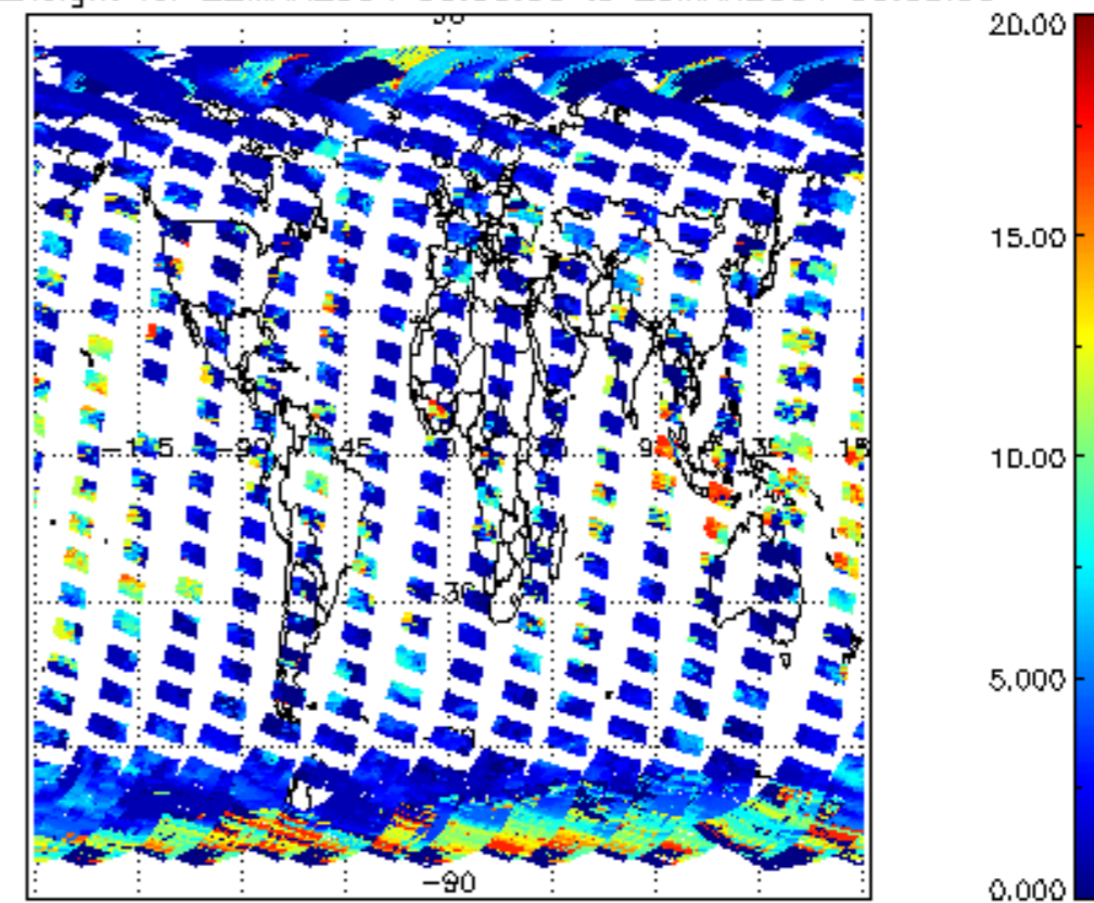
cL_top_height for 22MAR2004 00:00:00 to 23MAR2004 00:00:00
