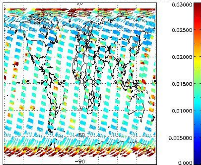
SCIOL2P_NADUV003_vcd_err for 22MAR2004 00:00:00 to 23MAR2004 00:00:00
