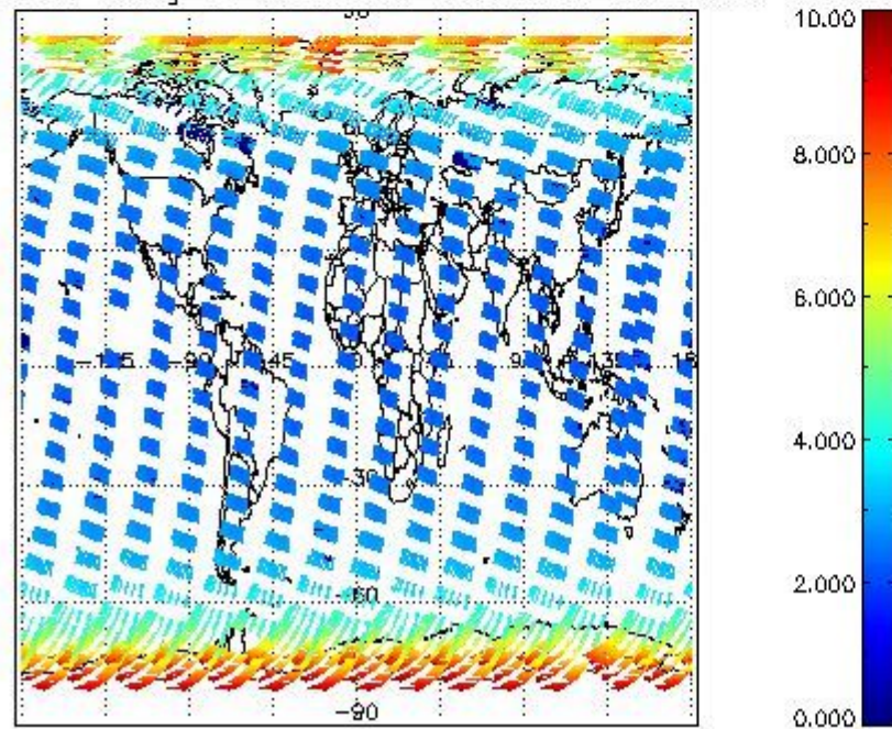
SCIOL2P_NADUV003_amf_gr for 22MAR2004 00:00:00 to 23MAR2004 00:00:00
