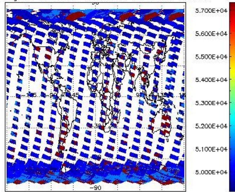
cloud_flags for 22MAR2004 00:00:00 to 23MAR2004 00:00:00
