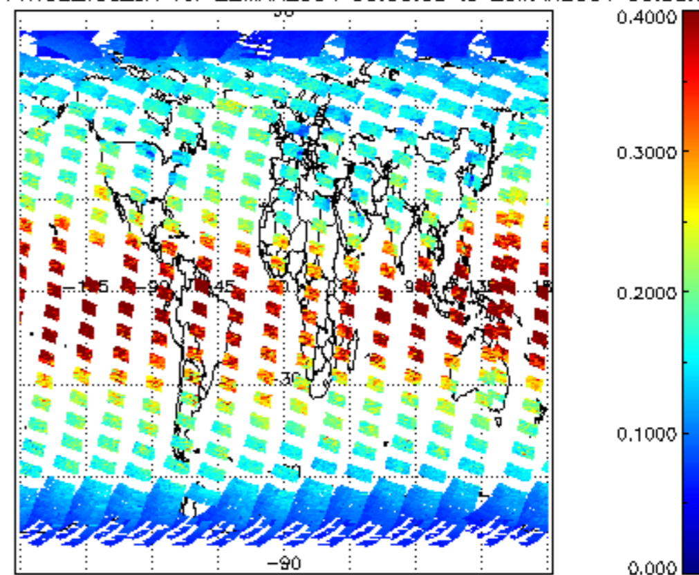
SCIOL2P_NADUV1NO2_vcd_err for 22MAR2004 00:00:00 to 23MAR2004 00:00:00
