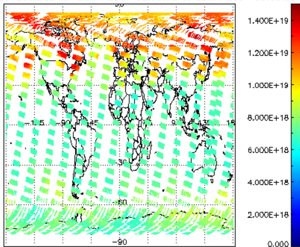
SCIOL2P_NADUV003_vcd for 22MAR2004 00:00:00 to 23MAR2004 00:00:00
