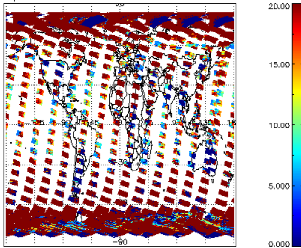
cL_opt_depth for 22MAR2004 00:00:00 to 23MAR2004 00:00:00
