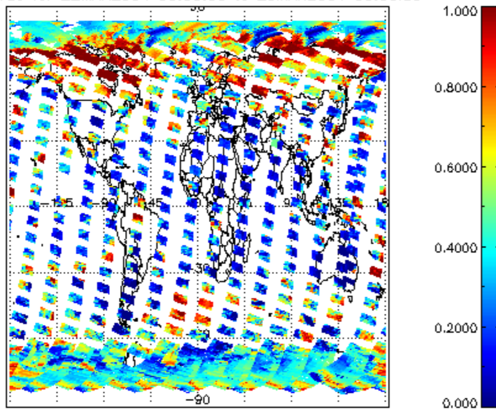
cL_frac for 22MAR2004 00:00:00 to 23MAR2004 00:00:00
