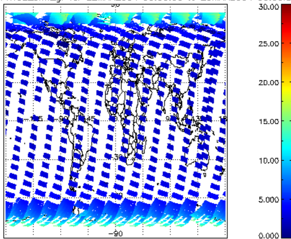
SCIOL2P_NADUV1NO2_amf_gr for 22MAR2004 00:00:00 to 23MAR2004 00:00:00
