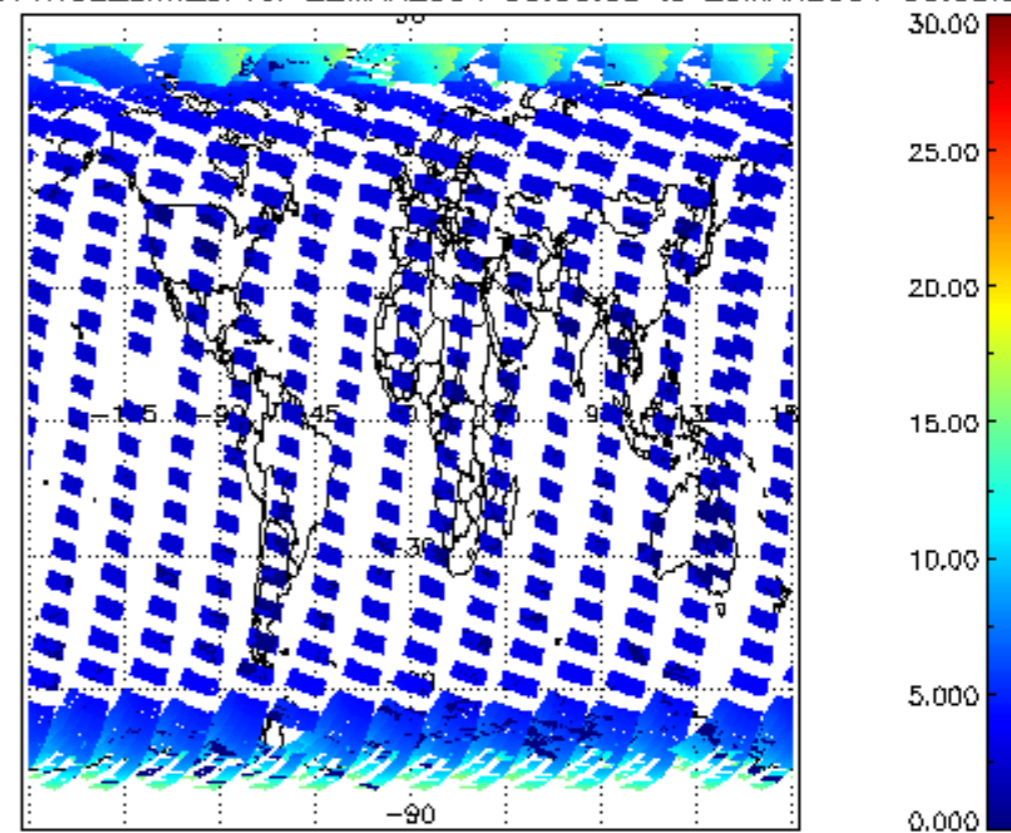
SCIOL2P_NADUV1NO2_amf_cl for 22MAR2004 00:00:00 to 23MAR2004 00:00:00
