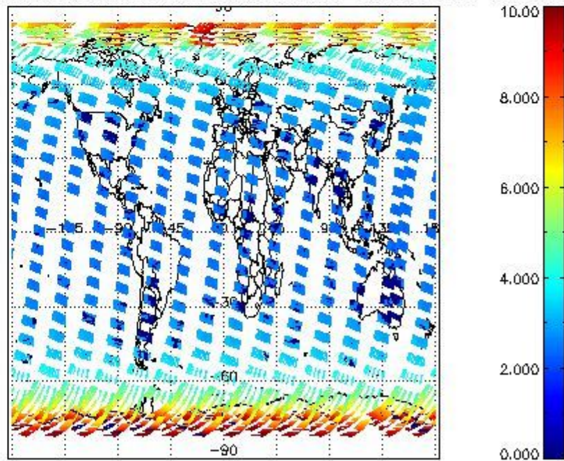
SCIOL2P_NADUV003_amf_cl for 22MAR2004 00:00:00 to 23MAR2004 00:00:00
