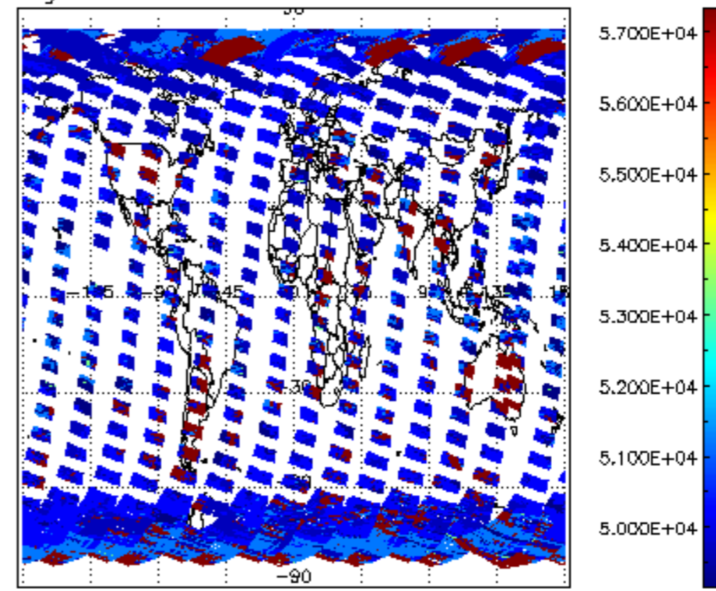
cloud_flags for 22MAR2004 00:00:00 to 23MAR2004 00:00:00
