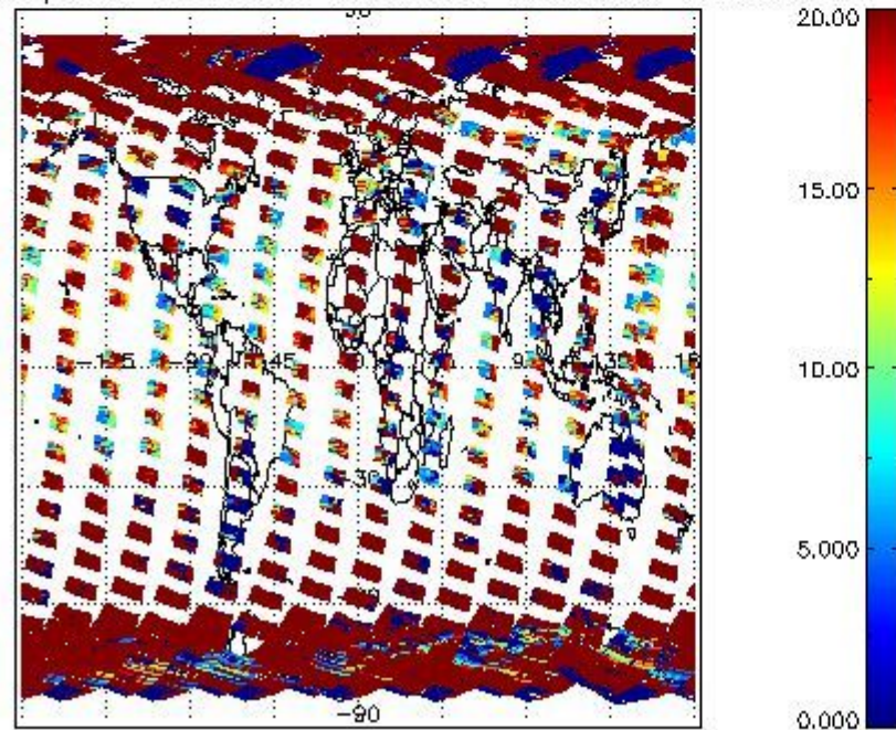
cL_opt_depth for 22MAR2004 00:00:00 to 23MAR2004 00:00:00
