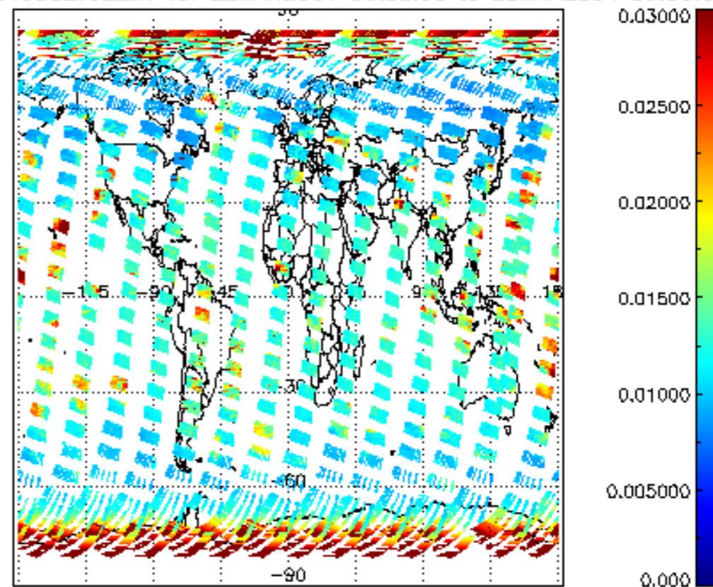
SCIOL2P_NADUV003_vcd_err for 22MAR2004 00:00:00 to 23MAR2004 00:00:00
