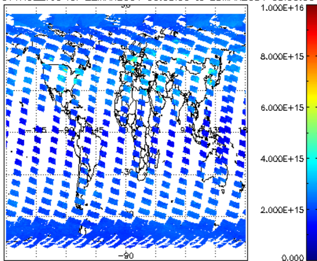
SCIOL2P_NADUV1NO2_vcd for 22MAR2004 00:00:00 to 23MAR2004 00:00:00
