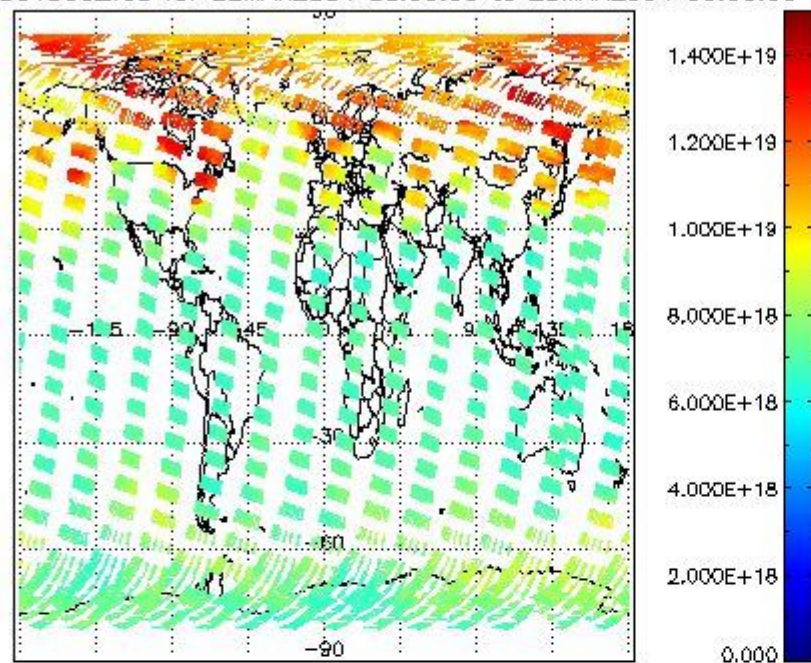
SCIOL2P_NADUV003_vcd for 22MAR2004 00:00:00 to 23MAR2004 00:00:00
