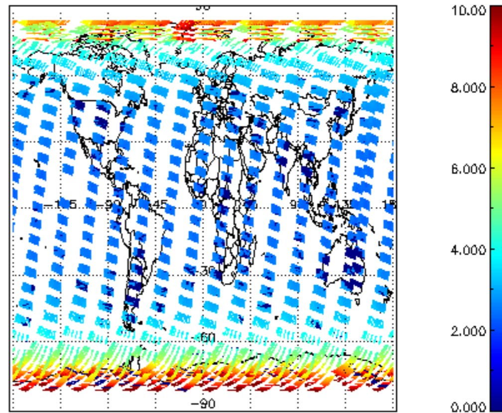
SCIOL2P_NADUV003_amf_cl for 22MAR2004 00:00:00 to 23MAR2004 00:00:00
