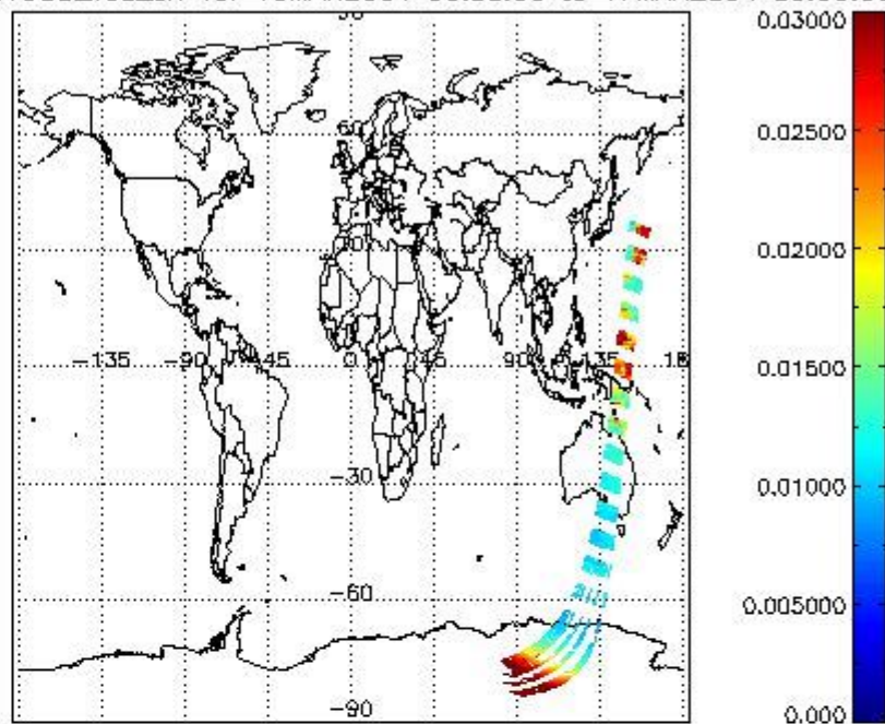
SCIOL2P_NADUV003_vcd_err for 16MAR2004 00:00:00 to 17MAR2004 00:00:00
