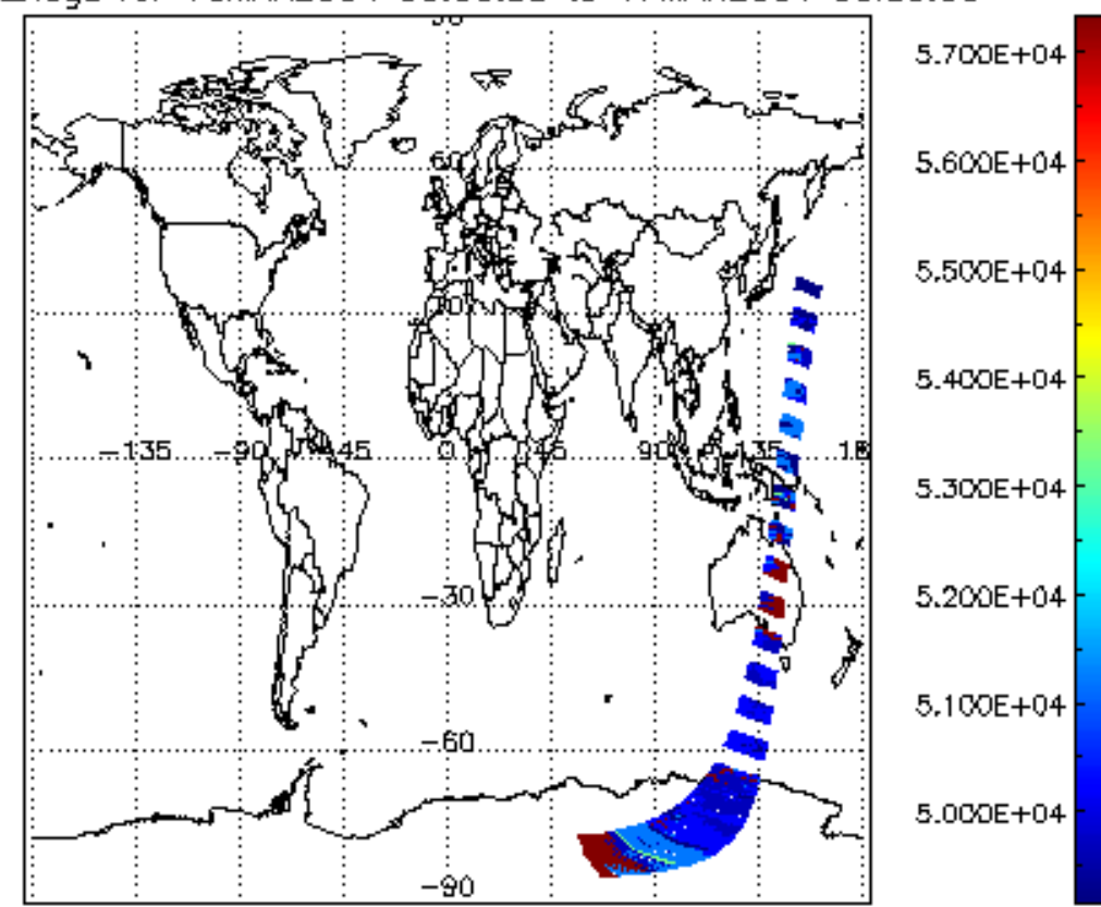
cloud_flags for 16MAR2004 00:00:00 to 17MAR2004 00:00:00
