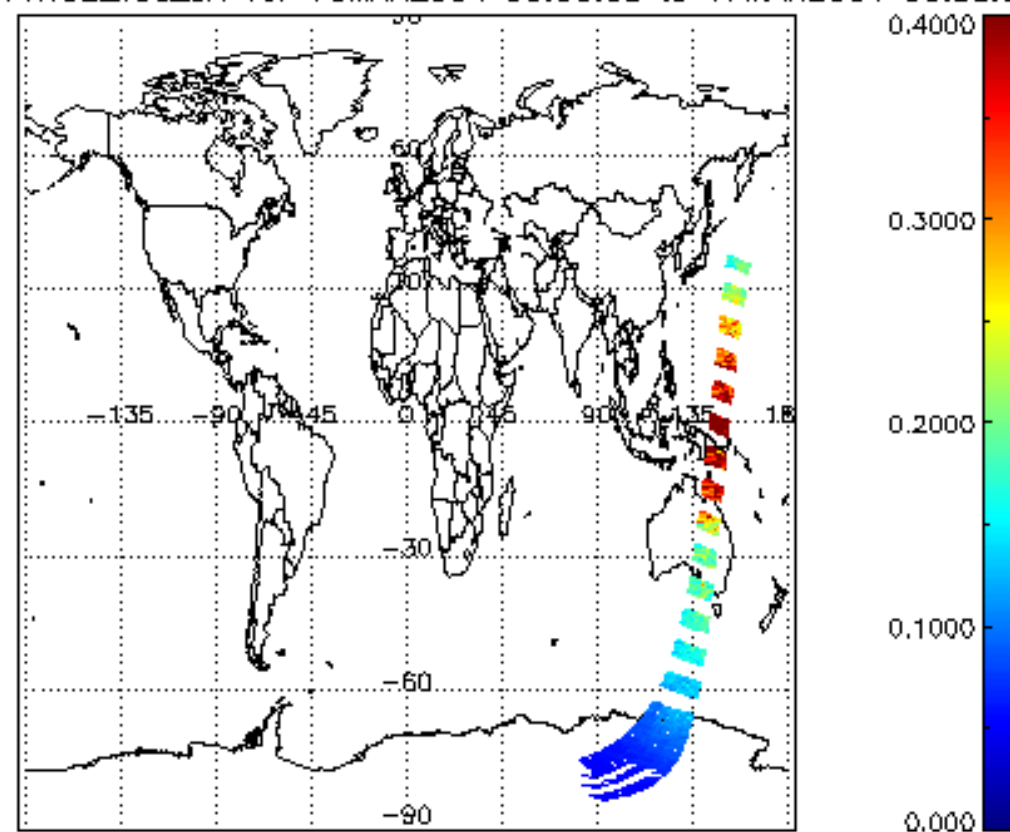
SCIOL2P_NADUV1NO2_vcd_err for 16MAR2004 00:00:00 to 17MAR2004 00:00:00
