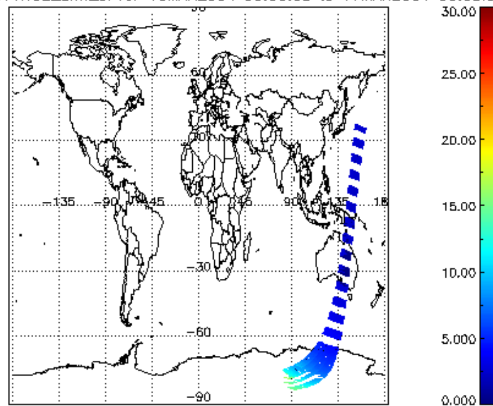
SCIOL2P_NADUV1NO2_amf_cl for 16MAR2004 00:00:00 to 17MAR2004 00:00:00
