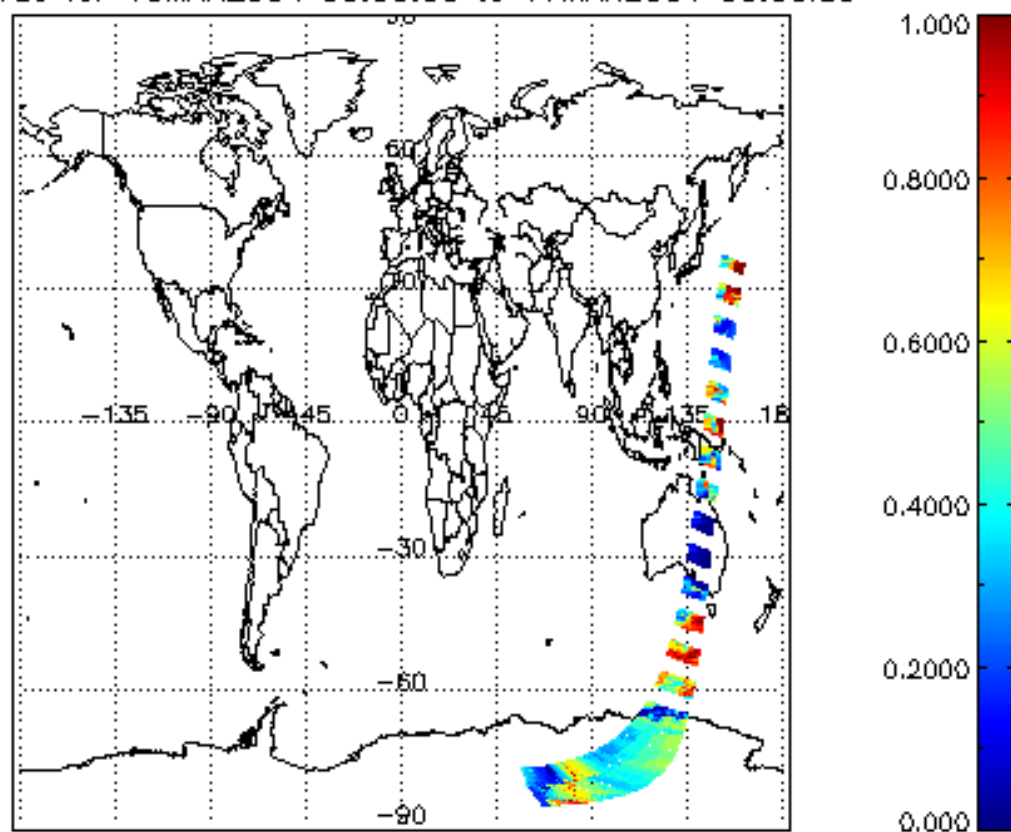
cL_frac for 16MAR2004 00:00:00 to 17MAR2004 00:00:00
