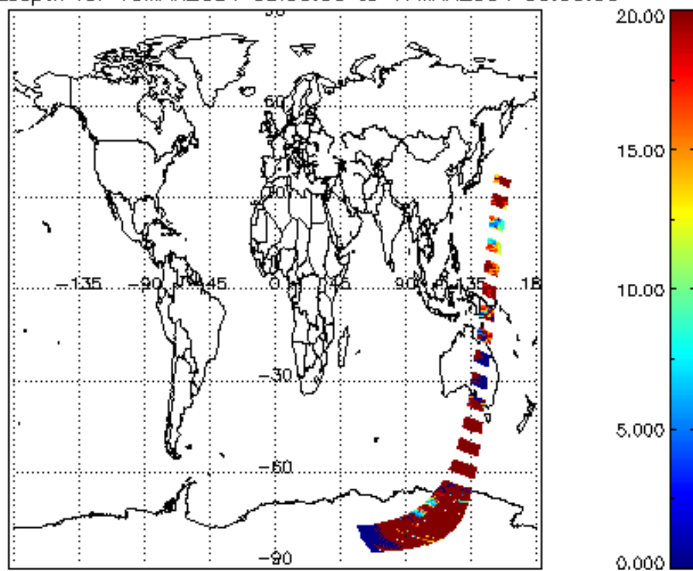
cL_opt_depth for 16MAR2004 00:00:00 to 17MAR2004 00:00:00
