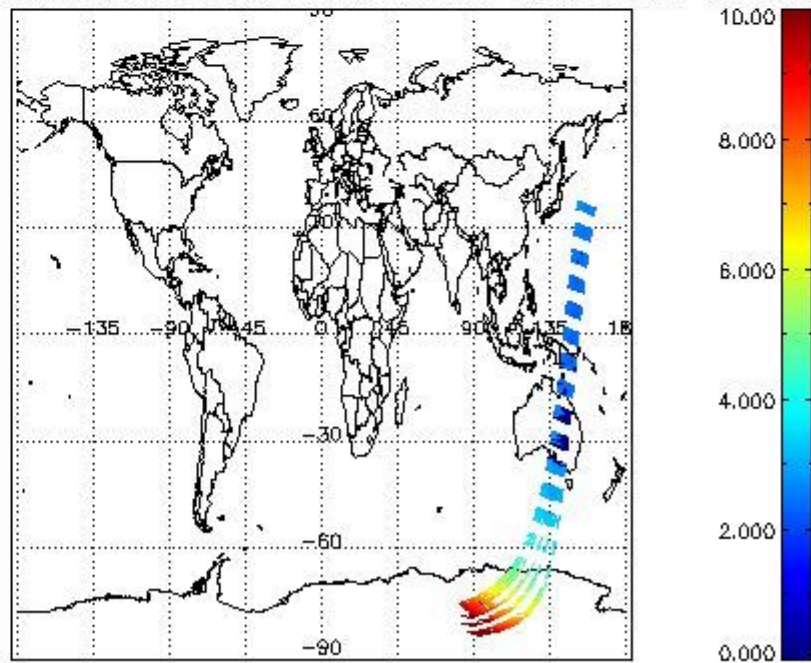
SCIOL2P_NADUV003_amf_cl for 16MAR2004 00:00:00 to 17MAR2004 00:00:00
