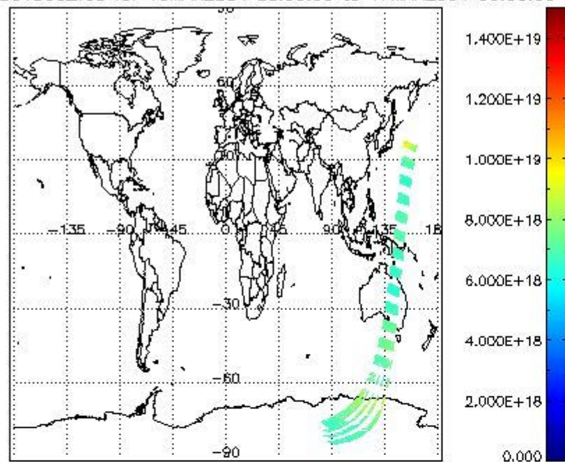
SCIOL2P_NADUV003_vcd for 16MAR2004 00:00:00 to 17MAR2004 00:00:00
