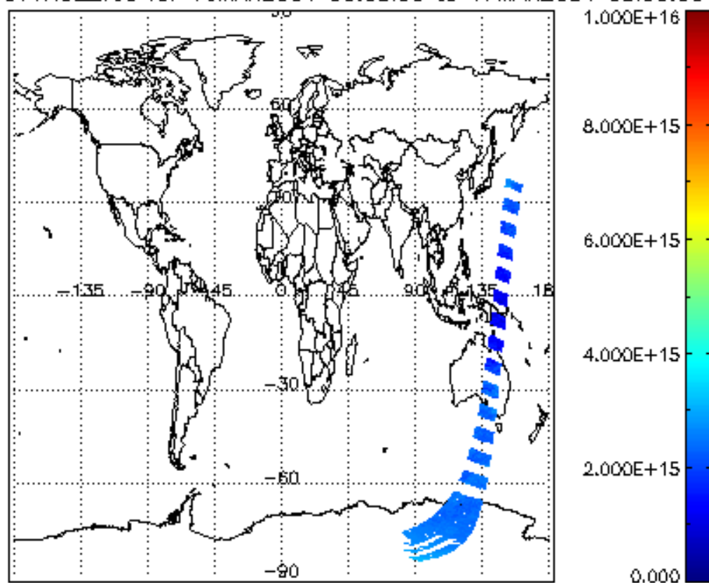
SCIOL2P_NADUV1NO2_vcd for 16MAR2004 00:00:00 to 17MAR2004 00:00:00
