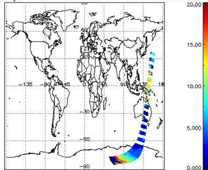
cL_top_height for 16MAR2004 00:00:00 to 17MAR2004 00:00:00
