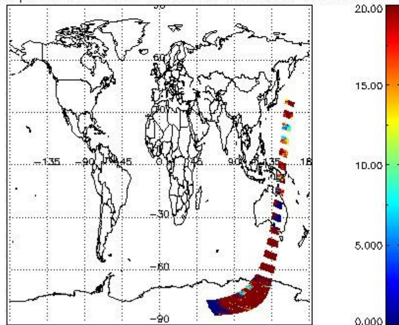
cL_opt_depth for 16MAR2004 00:00:00 to 17MAR2004 00:00:00
