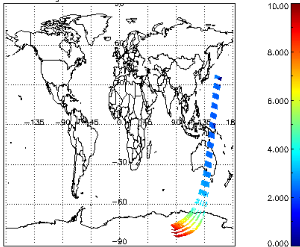
SCIOL2P_NADUV003_amf_gr for 16MAR2004 00:00:00 to 17MAR2004 00:00:00
