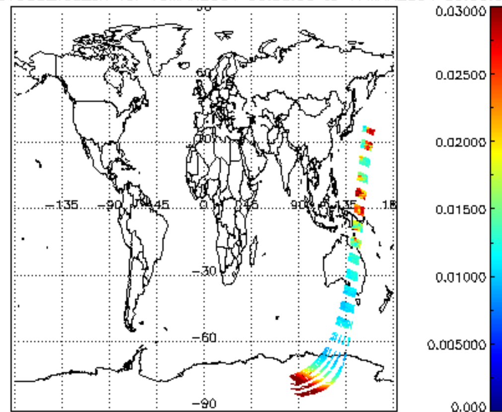
SCIOL2P_NADUV003_vcd_err for 16MAR2004 00:00:00 to 17MAR2004 00:00:00
