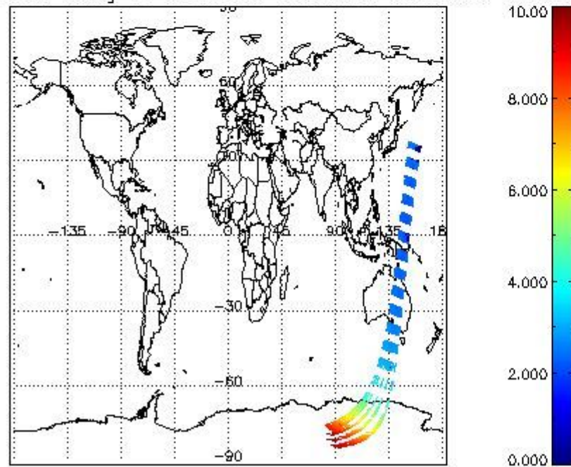
SCIOL2P_NADUV003_amf_gr for 16MAR2004 00:00:00 to 17MAR2004 00:00:00
