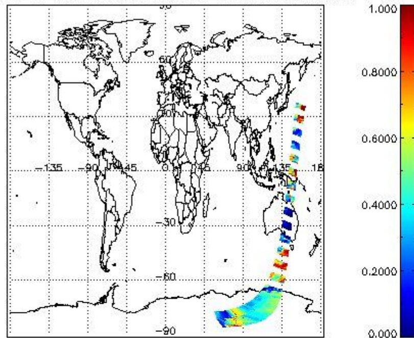
cL_frac for 16MAR2004 00:00:00 to 17MAR2004 00:00:00
