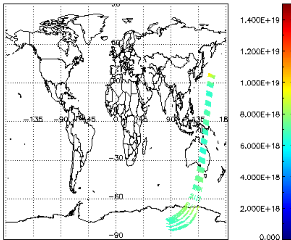
SCIOL2P_NADUV003_vcd for 16MAR2004 00:00:00 to 17MAR2004 00:00:00
