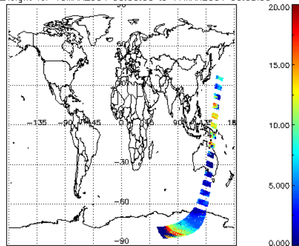
cL_top_height for 16MAR2004 00:00:00 to 17MAR2004 00:00:00
