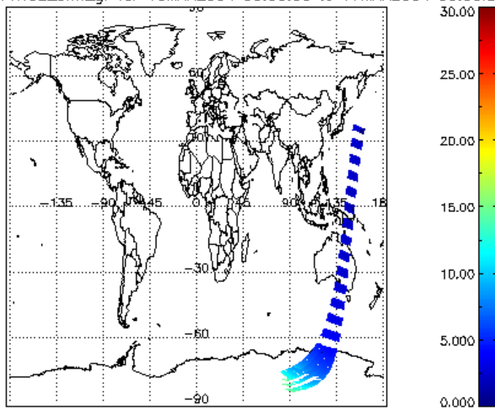
SCIOL2P_NADUV1NO2_amf_gr for 16MAR2004 00:00:00 to 17MAR2004 00:00:00
