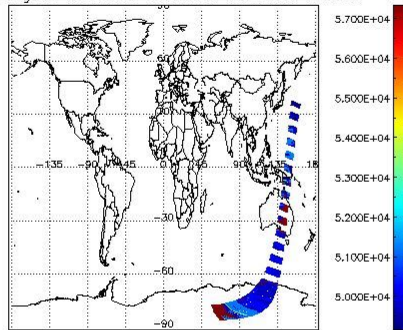
cloud_flags for 16MAR2004 00:00:00 to 17MAR2004 00:00:00
