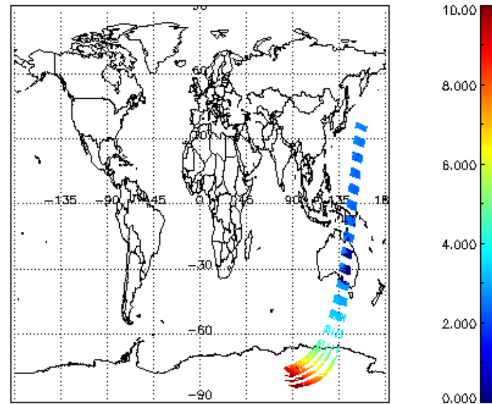
SCIOL2P_NADUV003_amf_cl for 16MAR2004 00:00:00 to 17MAR2004 00:00:00
