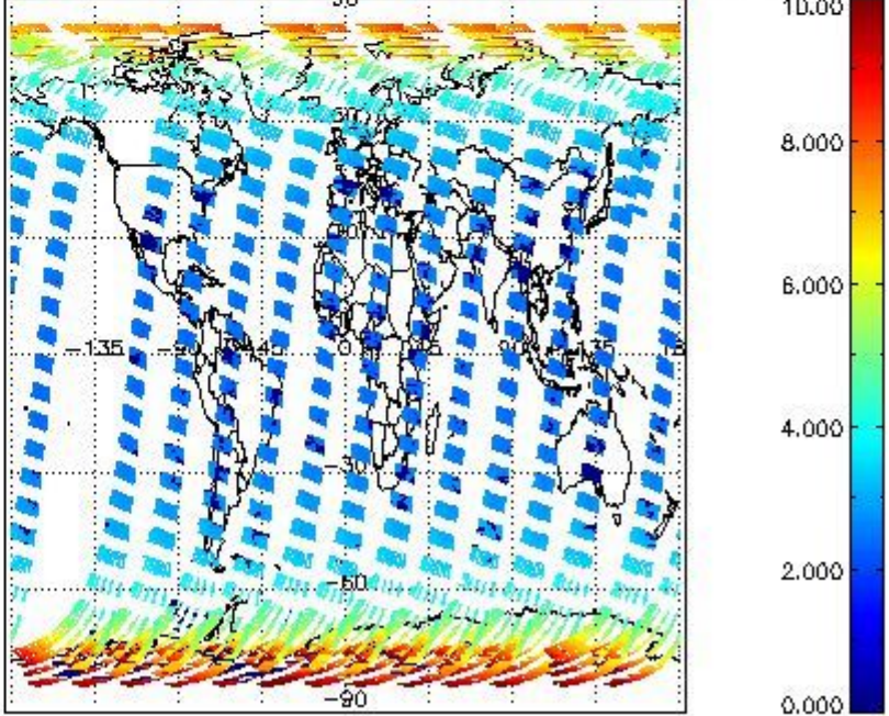
SCIOL2P_NADUV003_amf_cl for 15MAR2004 00:00:00 to 16MAR2004 00:00:00
