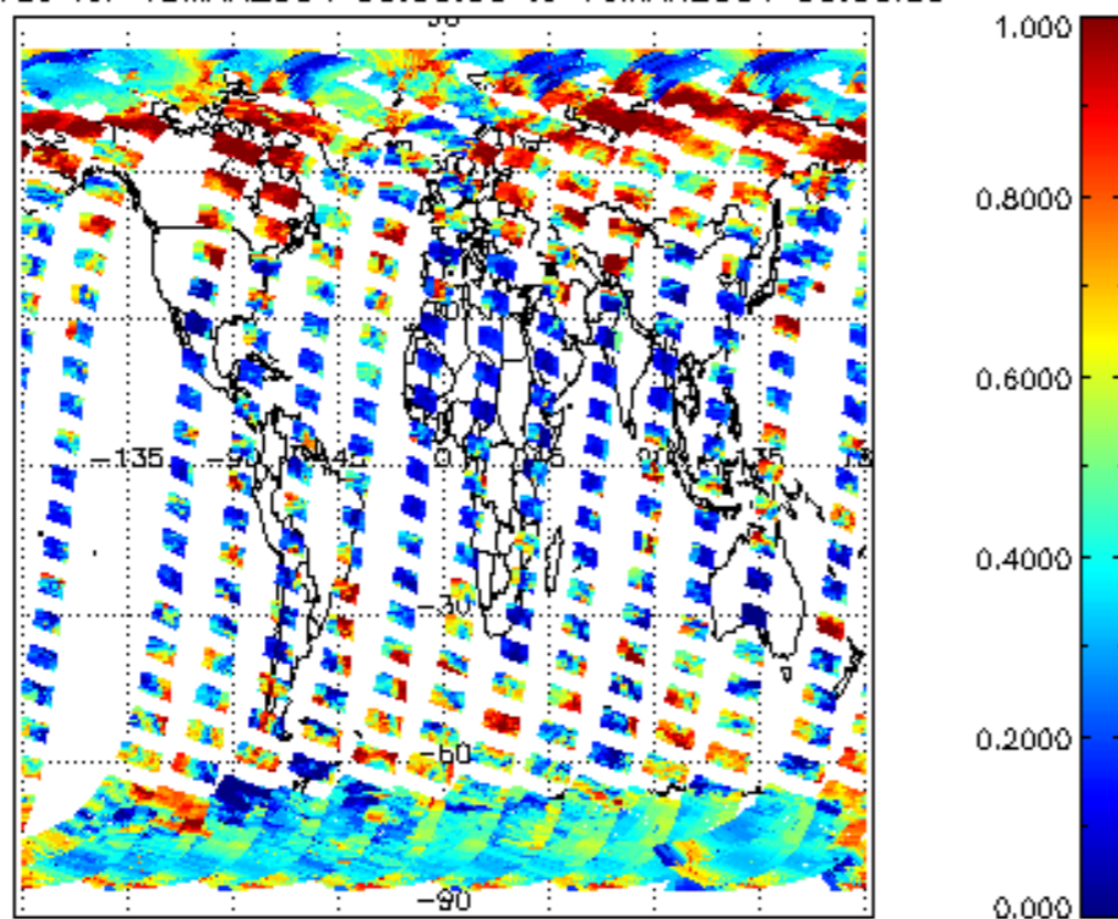
cL_frac for 15MAR2004 00:00:00 to 16MAR2004 00:00:00
