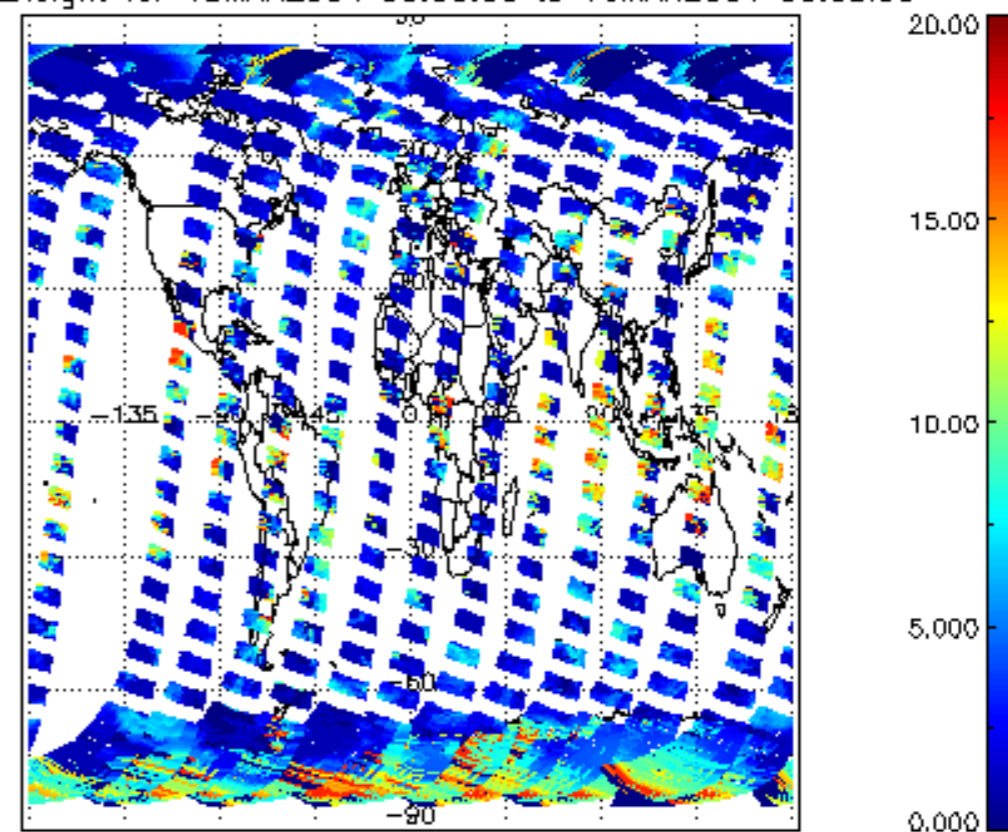
cL_top_height for 15MAR2004 00:00:00 to 16MAR2004 00:00:00
