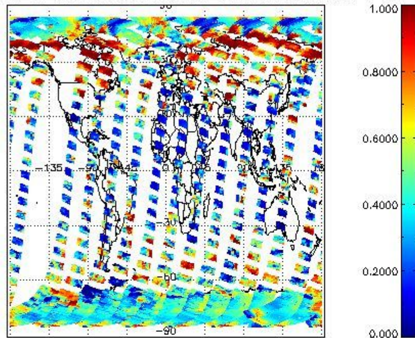
cL_frac for 15MAR2004 00:00:00 to 16MAR2004 00:00:00
