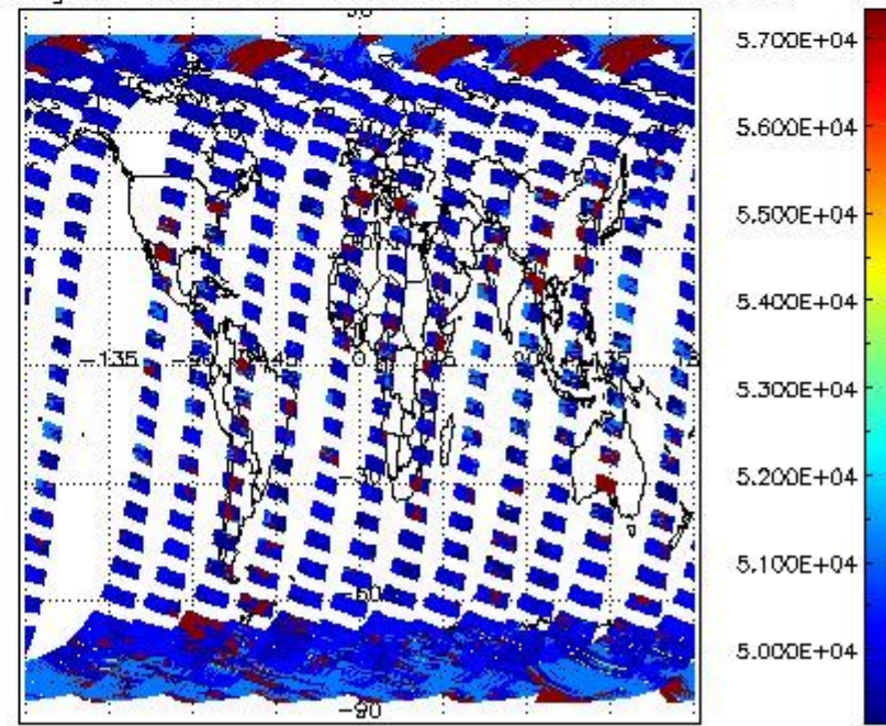
cloud_flags for 15MAR2004 00:00:00 to 16MAR2004 00:00:00
