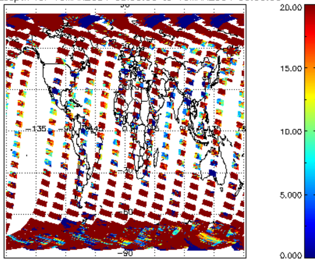
cL_opt_depth for 15MAR2004 00:00:00 to 16MAR2004 00:00:00
