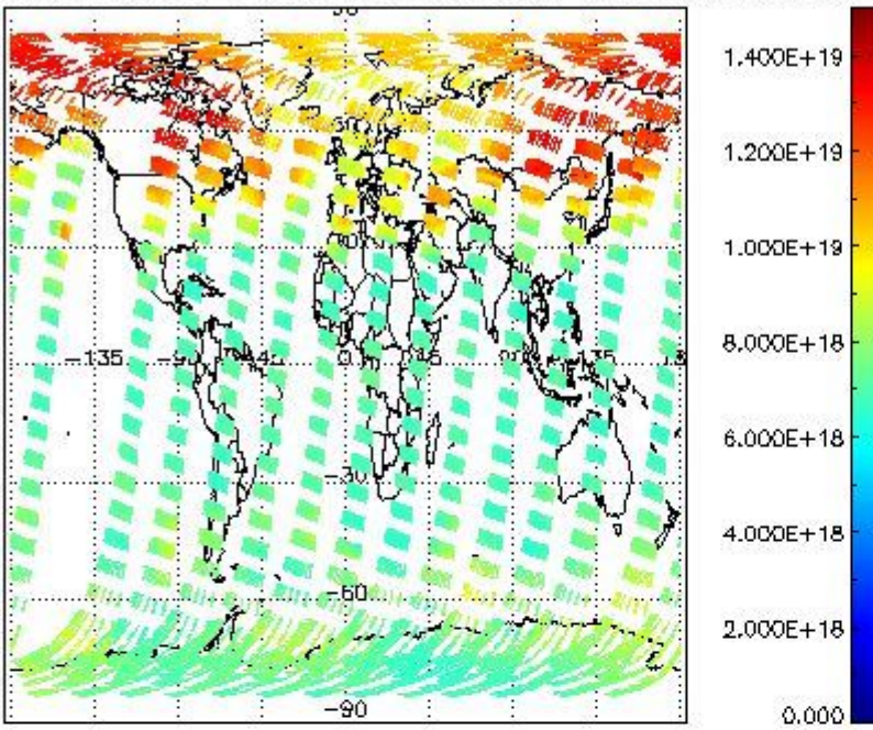
SCIOL2P_NADUV003_vcd for 15MAR2004 00:00:00 to 16MAR2004 00:00:00
