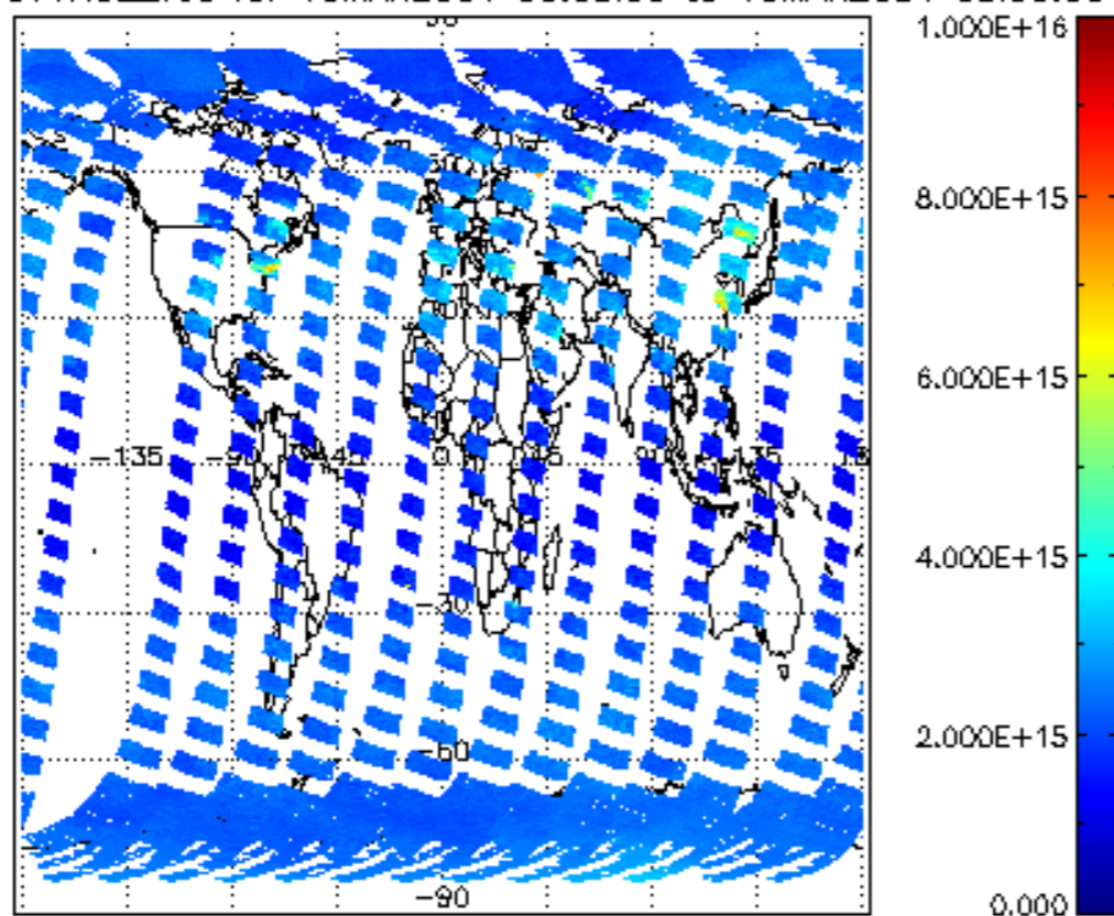
SCIOL2P_NADUV1NO2_vcd for 15MAR2004 00:00:00 to 16MAR2004 00:00:00
