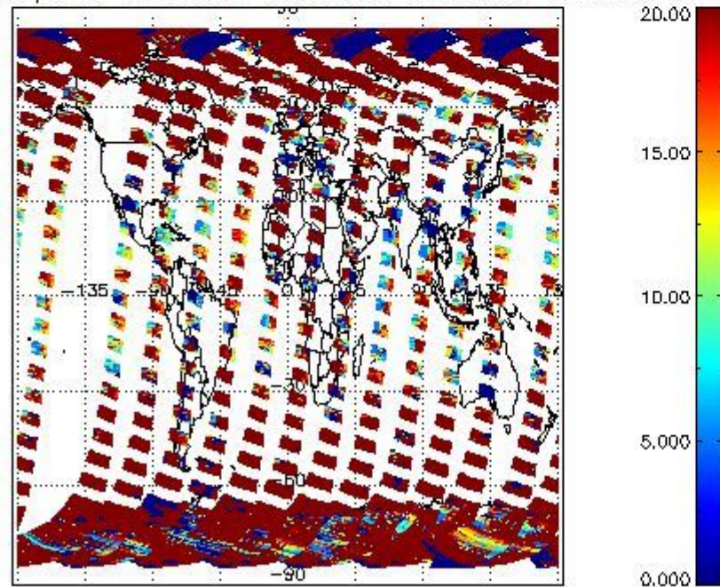
cL_opt_depth for 15MAR2004 00:00:00 to 16MAR2004 00:00:00
