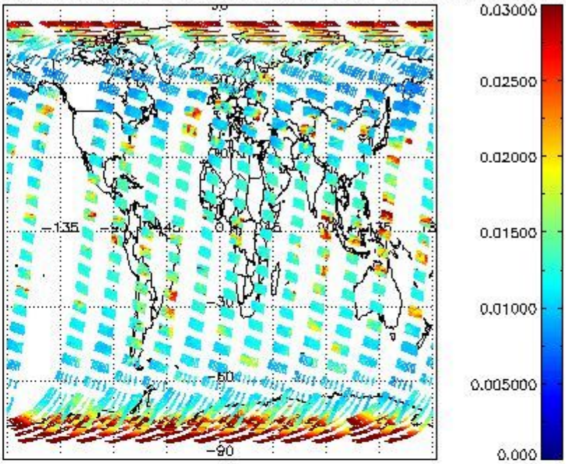
SCIOL2P_NADUV003_vcd_err for 15MAR2004 00:00:00 to 16MAR2004 00:00:00
