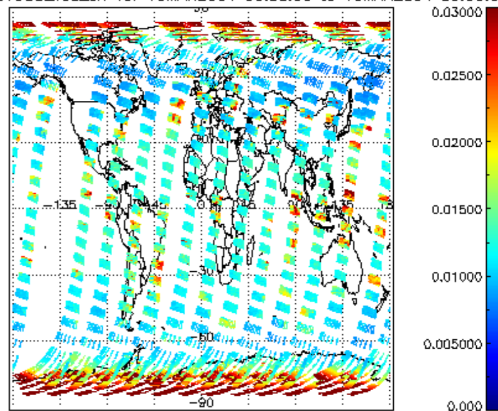
SCIOL2P_NADUV003_vcd_err for 15MAR2004 00:00:00 to 16MAR2004 00:00:00
