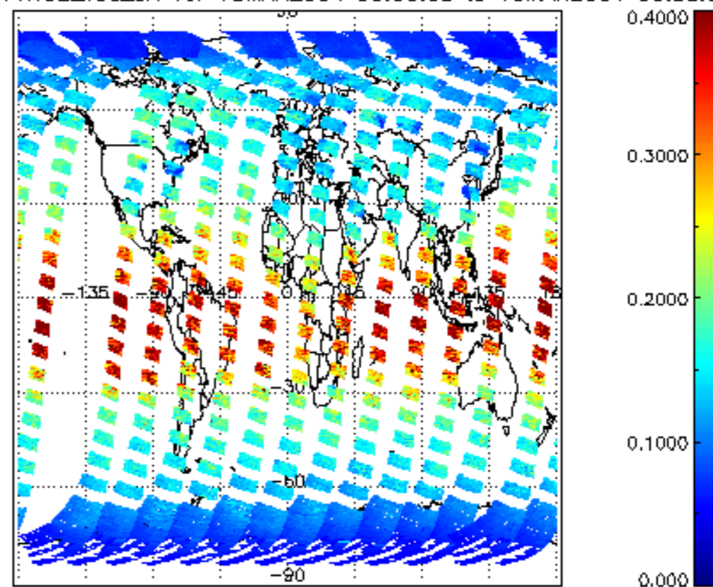
SCIOL2P_NADUV1NO2_vcd_err for 15MAR2004 00:00:00 to 16MAR2004 00:00:00
