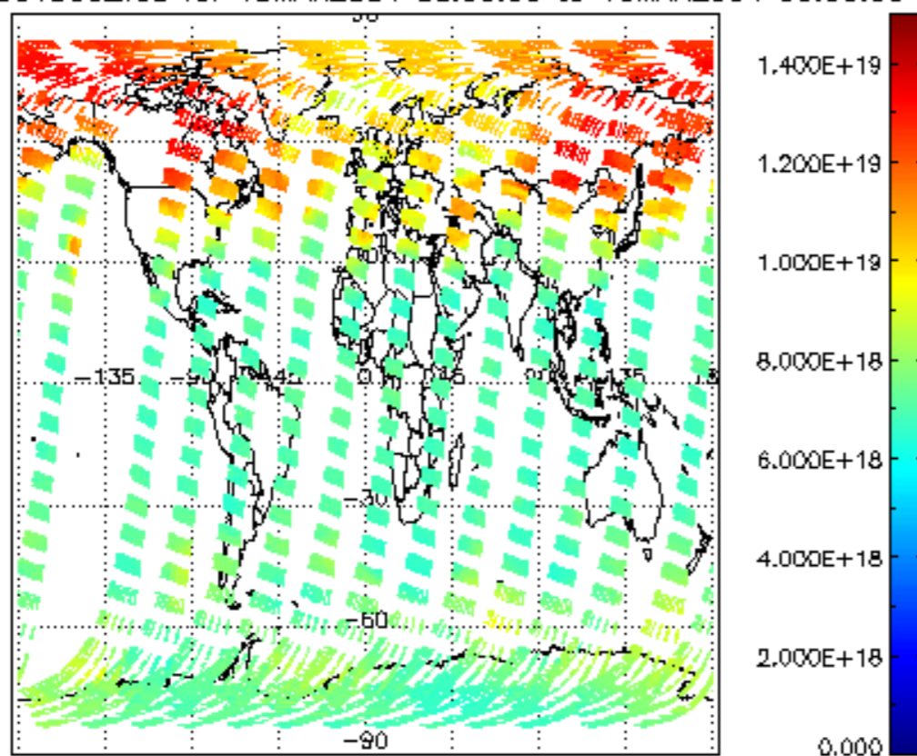
SCIOL2P_NADUV003_vcd for 15MAR2004 00:00:00 to 16MAR2004 00:00:00
