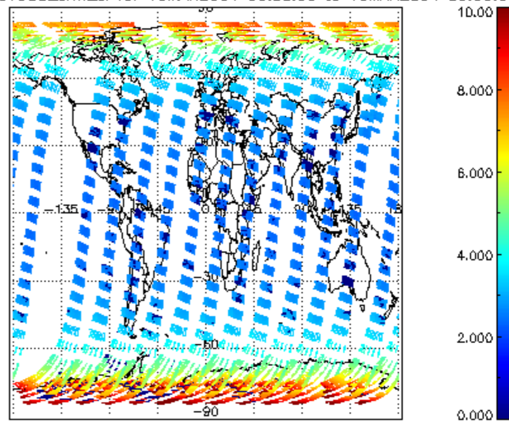
SCIOL2P_NADUV003_amf_cl for 15MAR2004 00:00:00 to 16MAR2004 00:00:00
