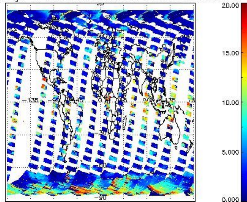
cL_top_height for 15MAR2004 00:00:00 to 16MAR2004 00:00:00
