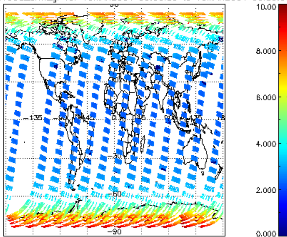
SCIOL2P_NADUV003_amf_gr for 15MAR2004 00:00:00 to 16MAR2004 00:00:00
