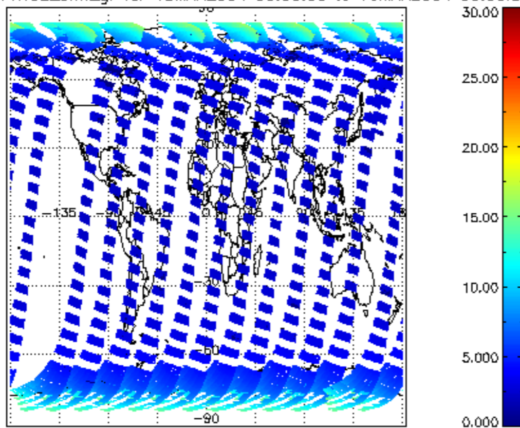
SCIOL2P_NADUV1NO2_amf_gr for 15MAR2004 00:00:00 to 16MAR2004 00:00:00
