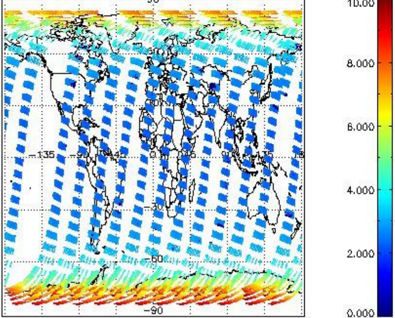
SCIOL2P_NADUV003_amf_gr for 15MAR2004 00:00:00 to 16MAR2004 00:00:00
