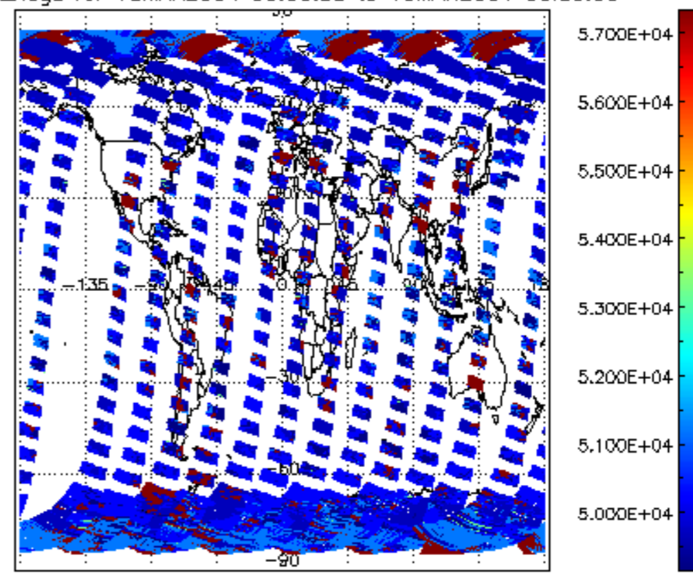
cloud_flags for 15MAR2004 00:00:00 to 16MAR2004 00:00:00
