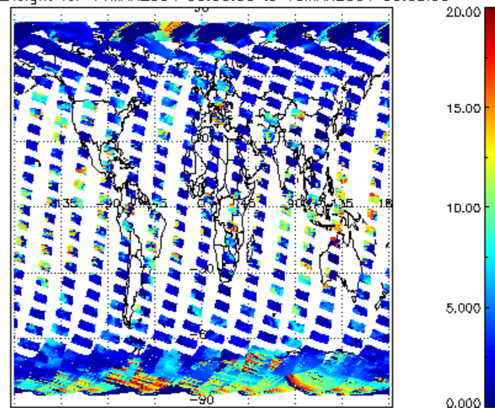
cL_top_height for 14MAR2004 00:00:00 to 15MAR2004 00:00:00
