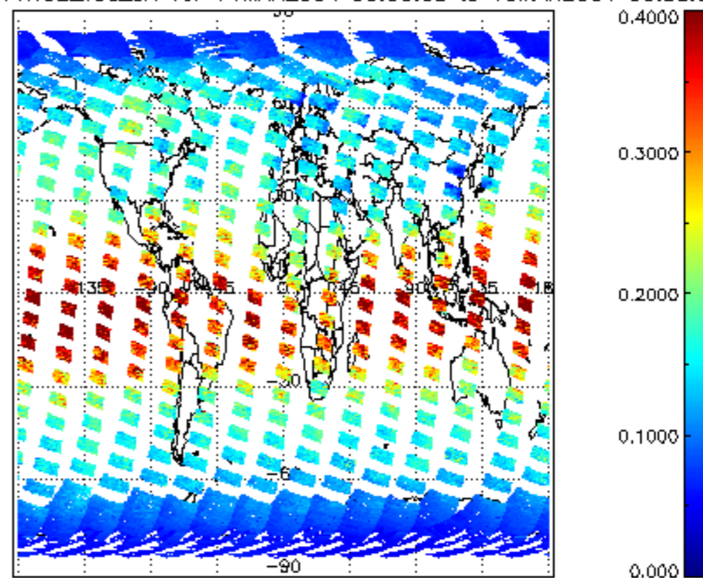
SCIOL2P_NADUV1NO2_vcd_err for 14MAR2004 00:00:00 to 15MAR2004 00:00:00
