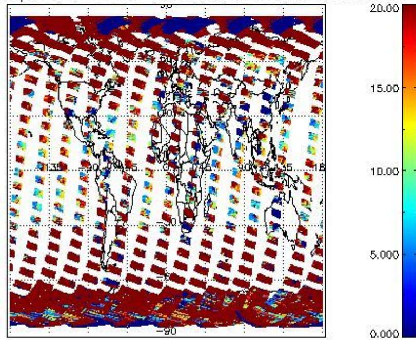
cL_opt_depth for 14MAR2004 00:00:00 to 15MAR2004 00:00:00
