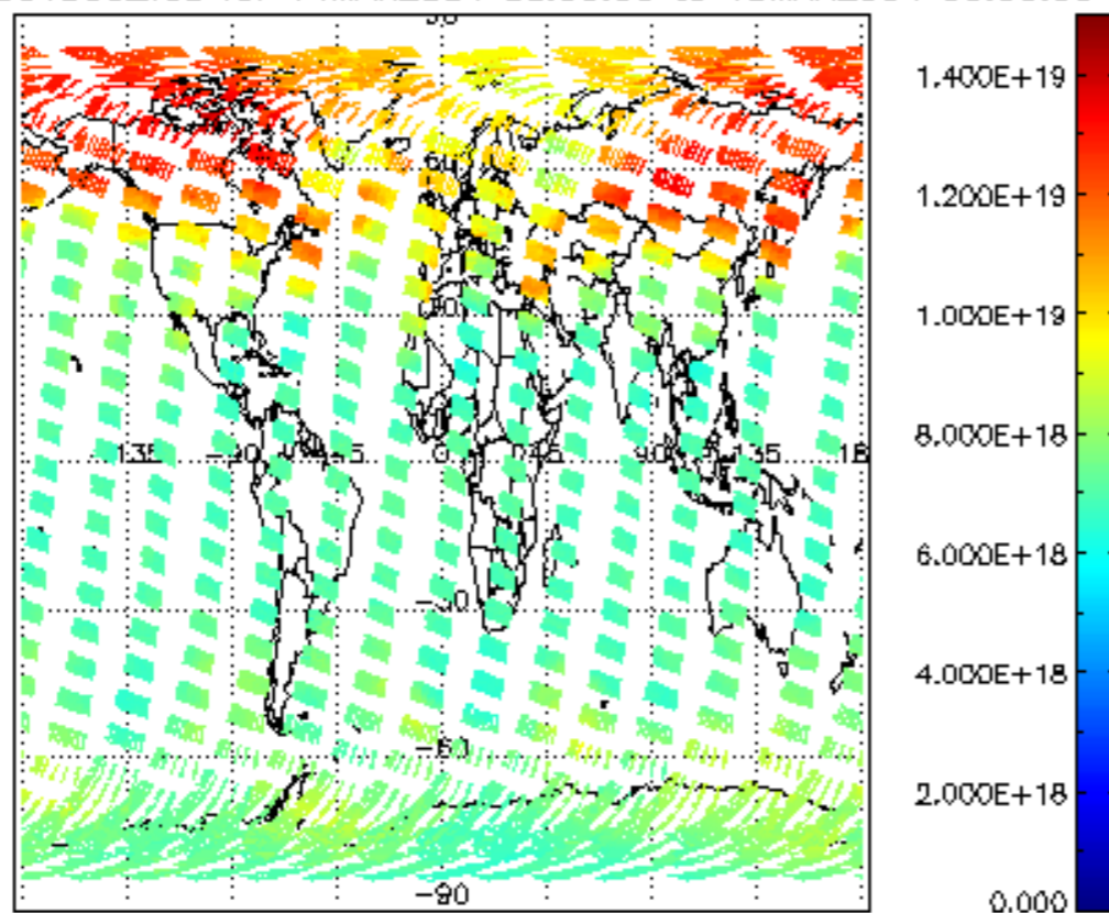
SCIOL2P_NADUV003_vcd for 14MAR2004 00:00:00 to 15MAR2004 00:00:00
