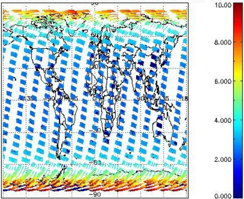
SCIOL2P_NADUV003_amf_cl for 14MAR2004 00:00:00 to 15MAR2004 00:00:00
