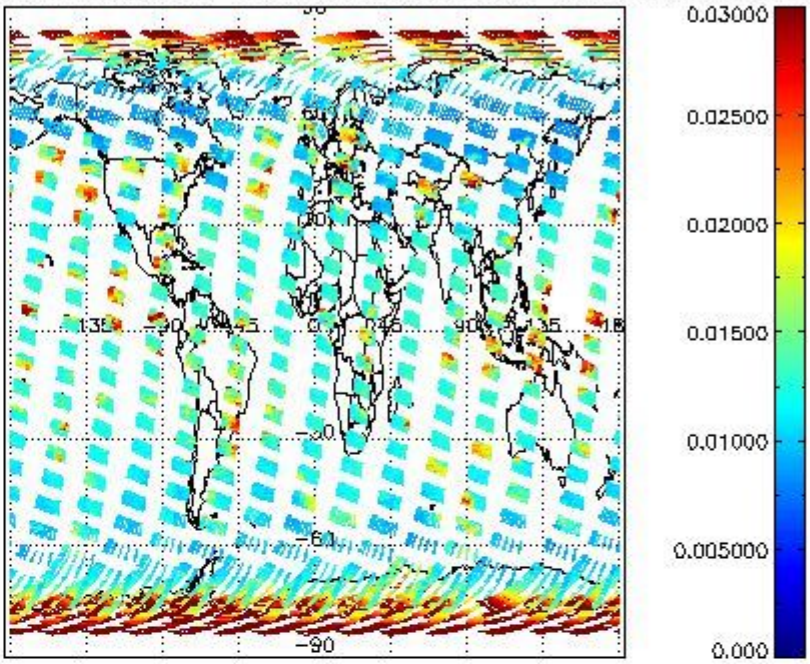
SCIOL2P_NADUV003_vcd_err for 14MAR2004 00:00:00 to 15MAR2004 00:00:00
