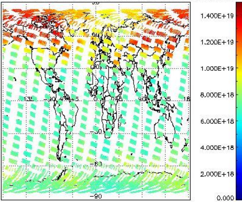
SCIOL2P_NADUV003_vcd for 14MAR2004 00:00:00 to 15MAR2004 00:00:00
