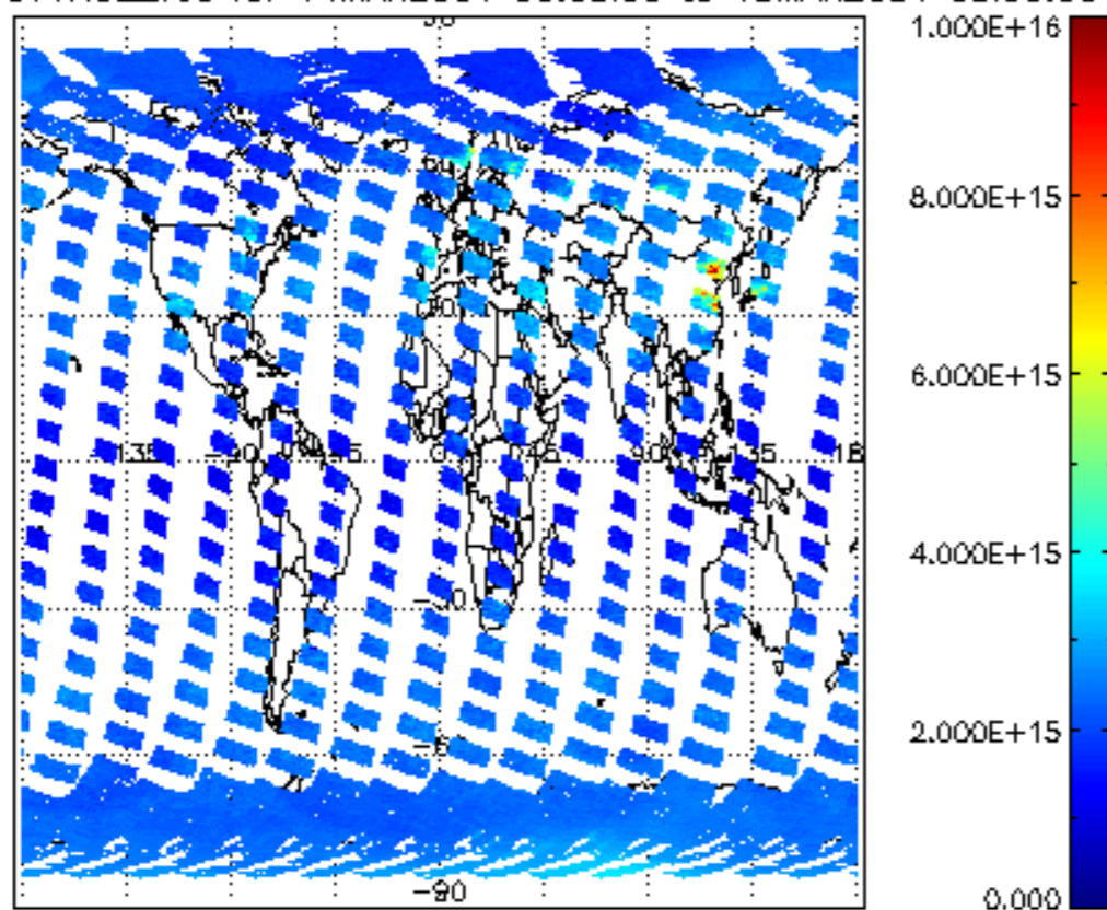
SCIOL2P_NADUV1NO2_vcd for 14MAR2004 00:00:00 to 15MAR2004 00:00:00
