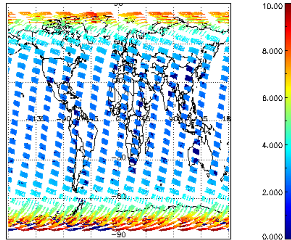
SCIOL2P_NADUV003_amf_cl for 14MAR2004 00:00:00 to 15MAR2004 00:00:00
