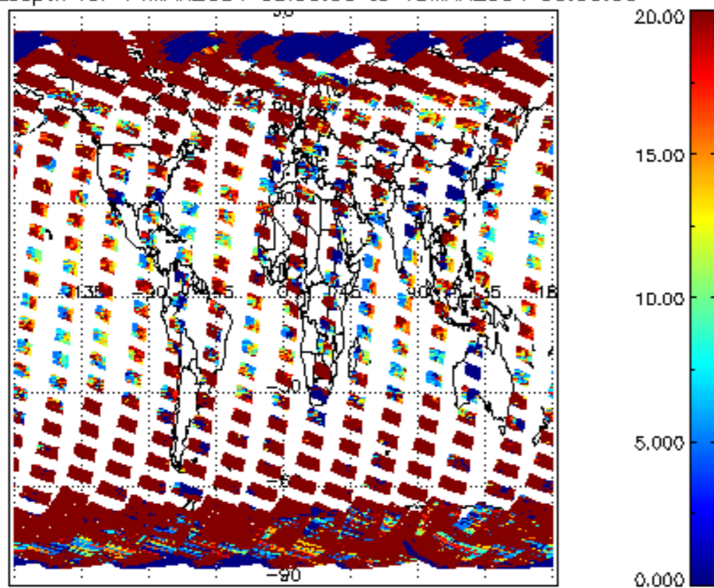
cL_opt_depth for 14MAR2004 00:00:00 to 15MAR2004 00:00:00
