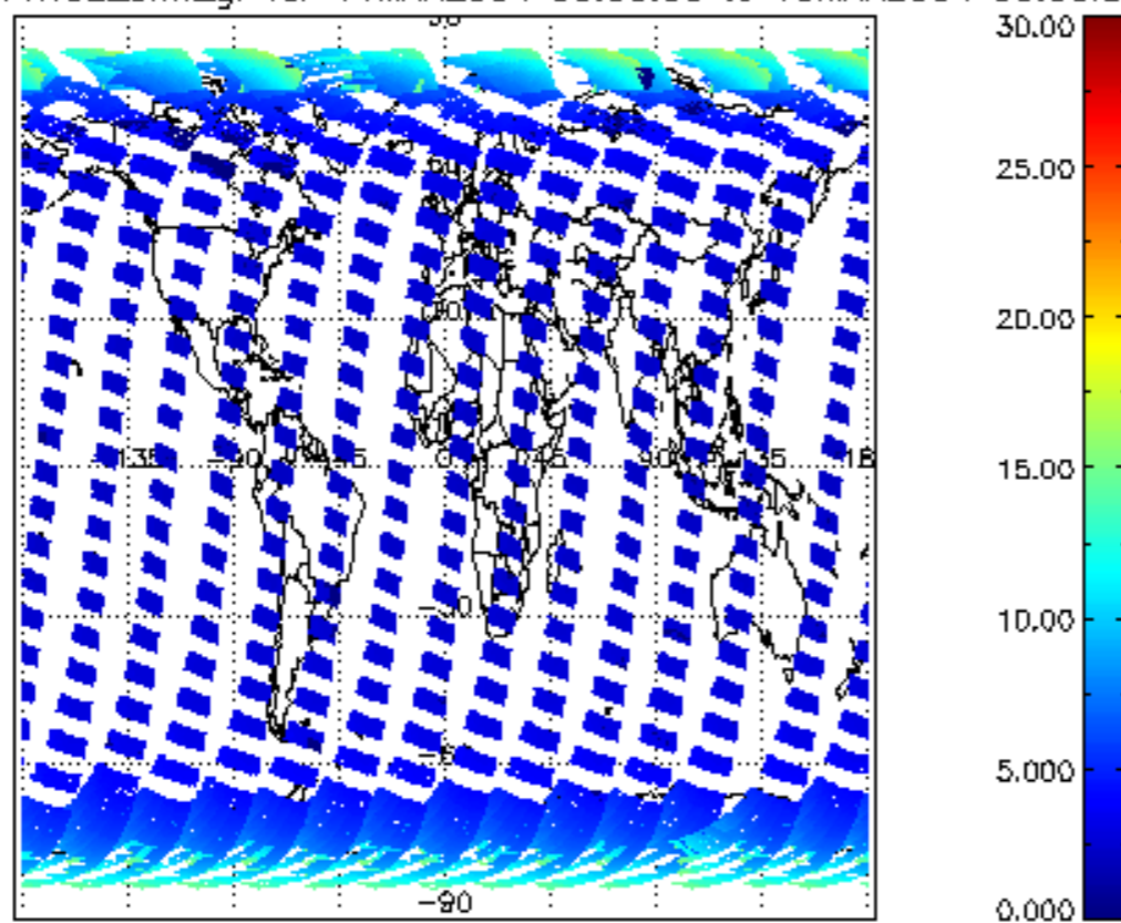
SCIOL2P_NADUV1NO2_amf_gr for 14MAR2004 00:00:00 to 15MAR2004 00:00:00
