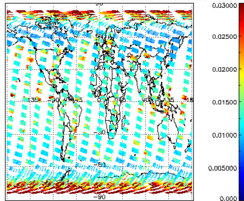
SCIOL2P_NADUV003_vcd_err for 14MAR2004 00:00:00 to 15MAR2004 00:00:00
