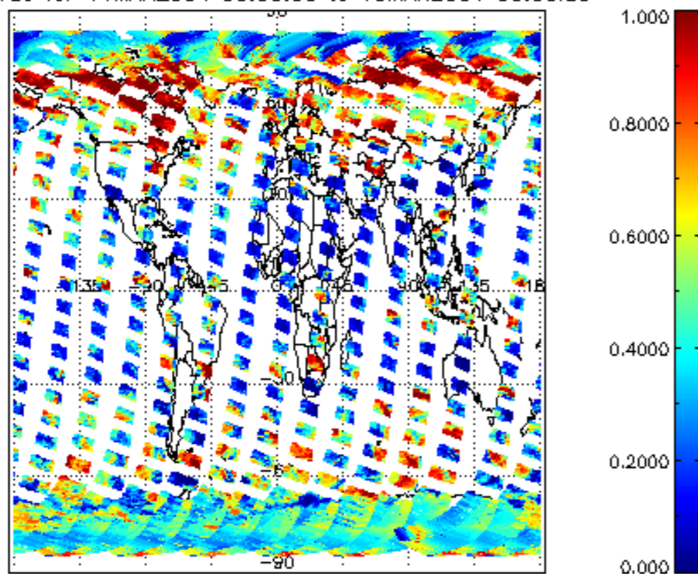
cL_frac for 14MAR2004 00:00:00 to 15MAR2004 00:00:00
