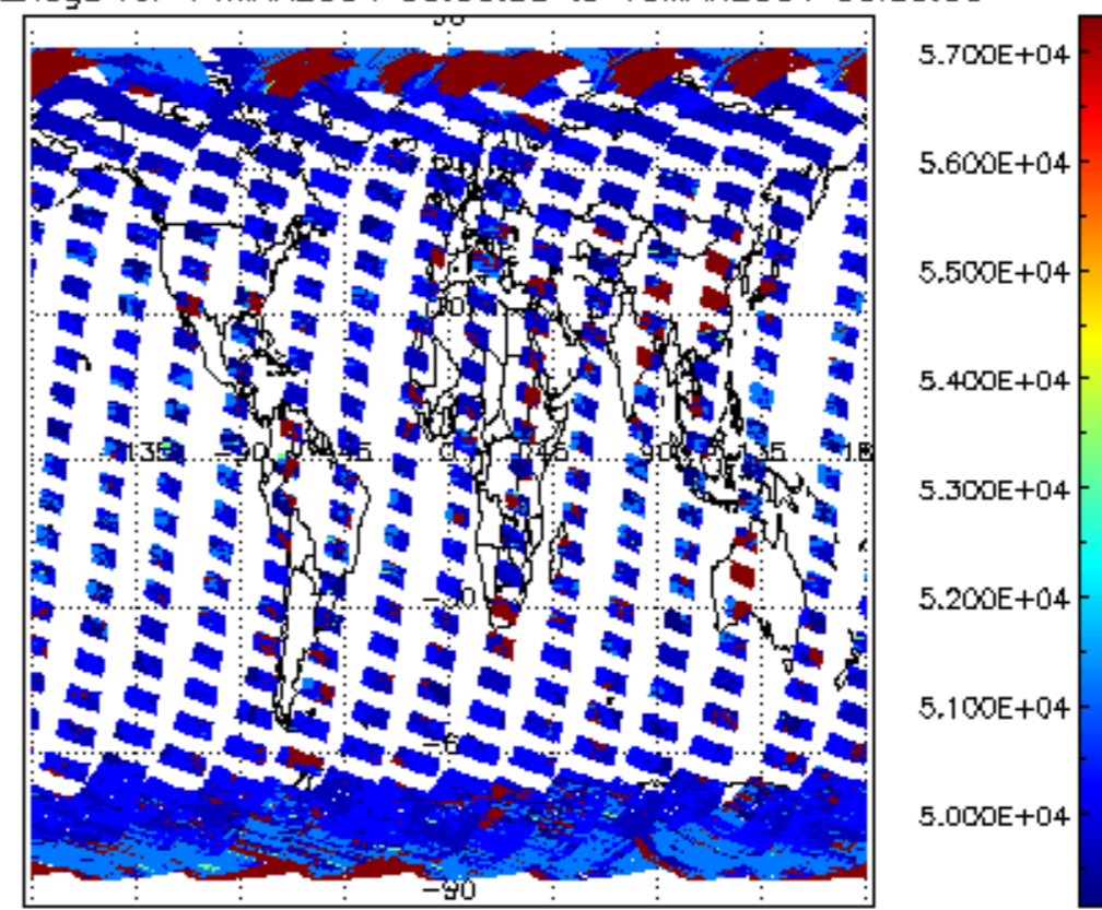
cloud_flags for 14MAR2004 00:00:00 to 15MAR2004 00:00:00
