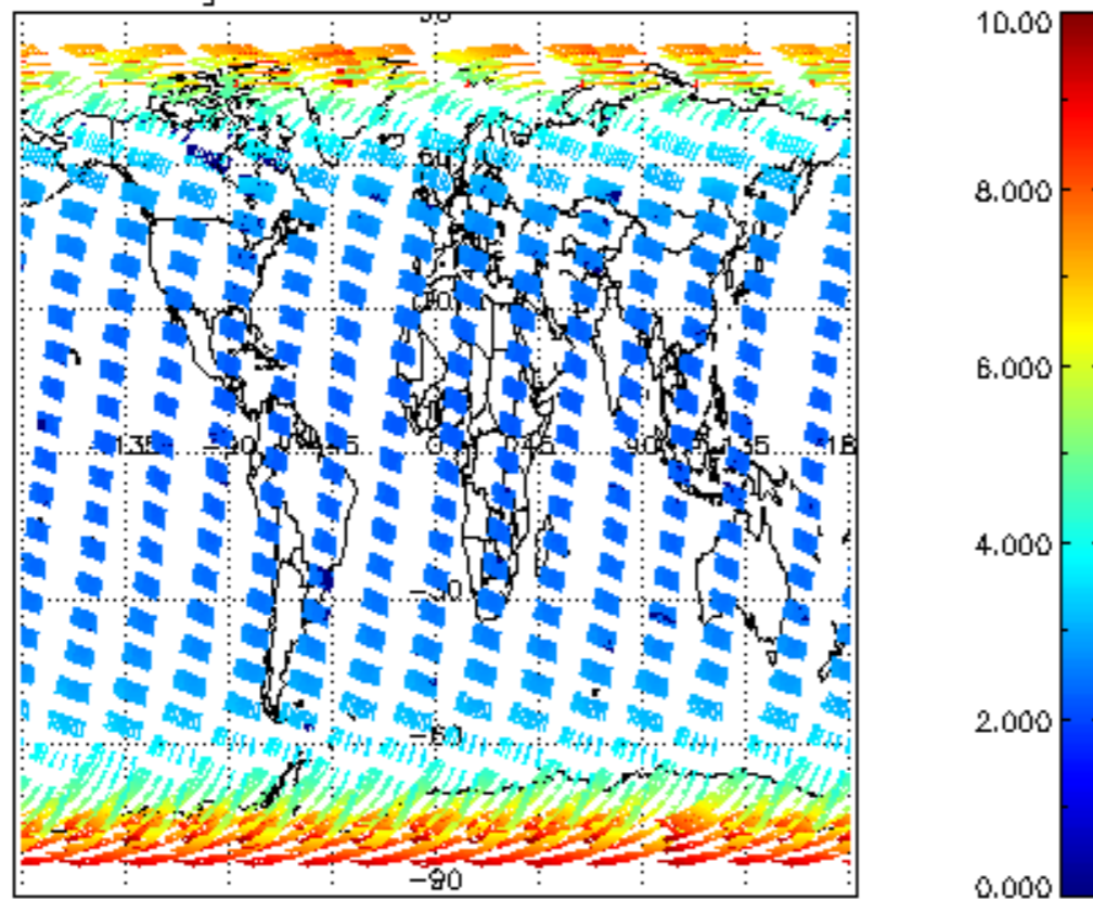
SCIOL2P_NADUV003_amf_gr for 14MAR2004 00:00:00 to 15MAR2004 00:00:00
