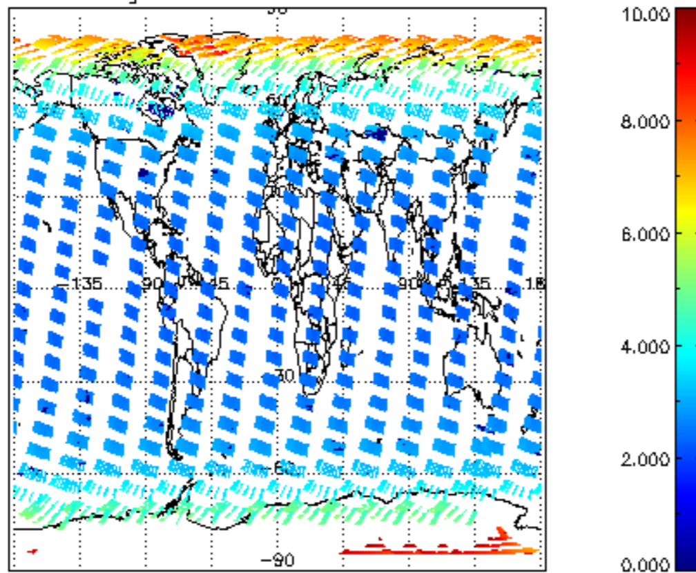
SCIOL2P_NADUV003_amf_gr for 04MAR2004 00:00:00 to 05MAR2004 00:00:00
