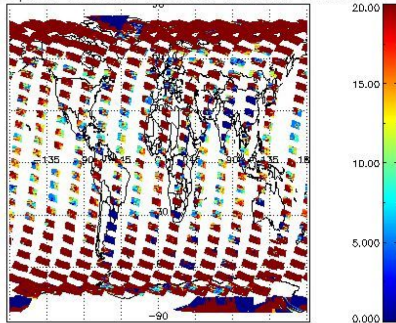
cL_opt_depth for 04MAR2004 00:00:00 to 05MAR2004 00:00:00
