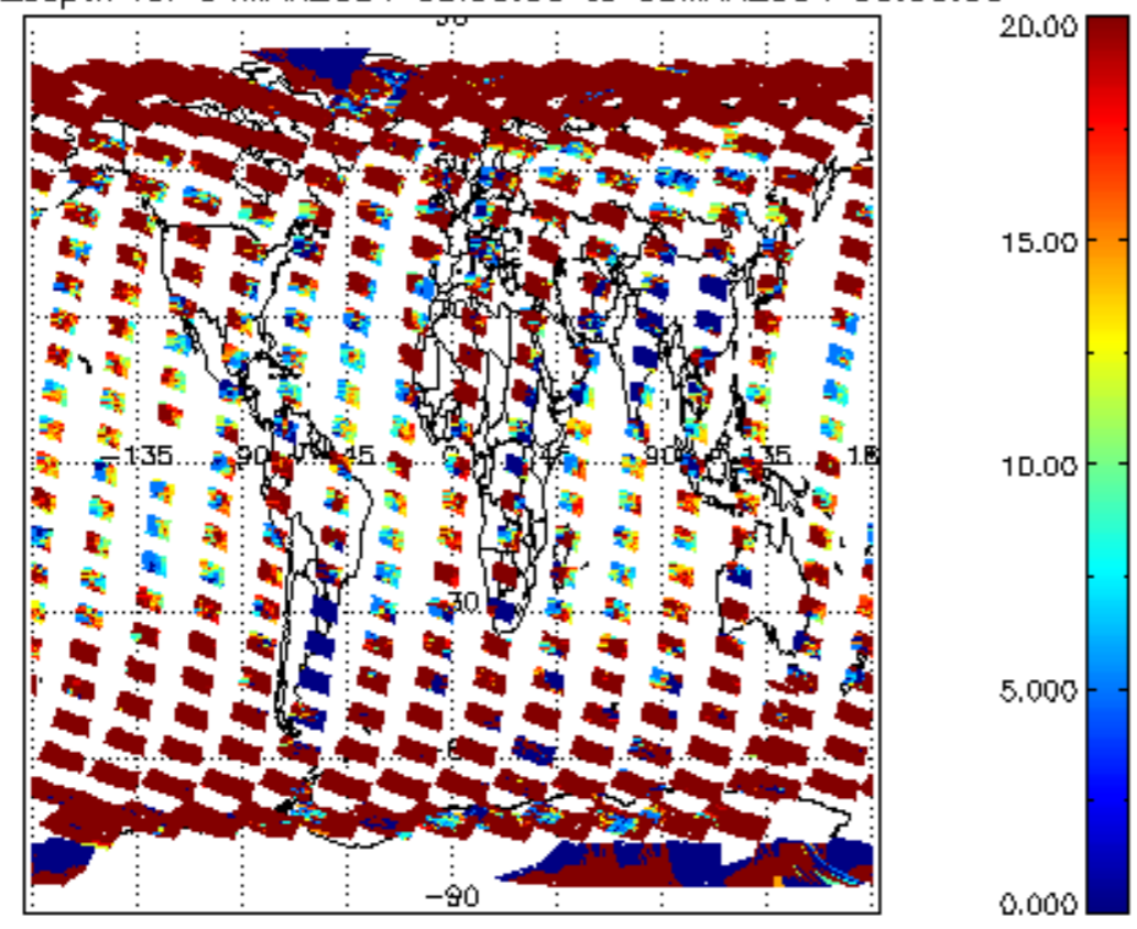
cL_opt_depth for 04MAR2004 00:00:00 to 05MAR2004 00:00:00
