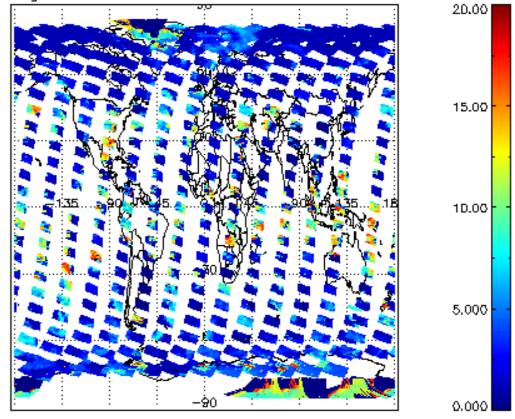
cL_top_height for 04MAR2004 00:00:00 to 05MAR2004 00:00:00
