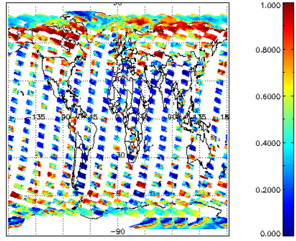
cL_frac for 04MAR2004 00:00:00 to 05MAR2004 00:00:00
