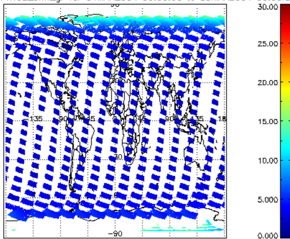
SCIOL2P_NADUV1NO2_amf_gr for 04MAR2004 00:00:00 to 05MAR2004 00:00:00
