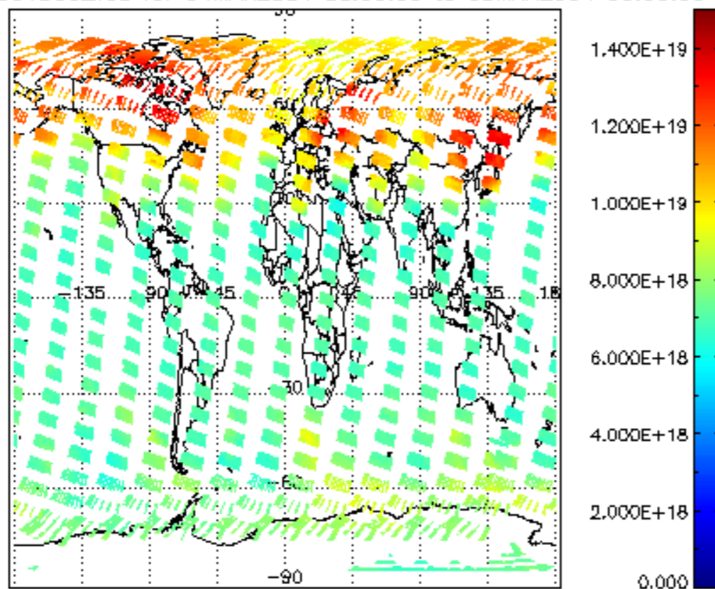
SCIOL2P_NADUV003_vcd for 04MAR2004 00:00:00 to 05MAR2004 00:00:00
