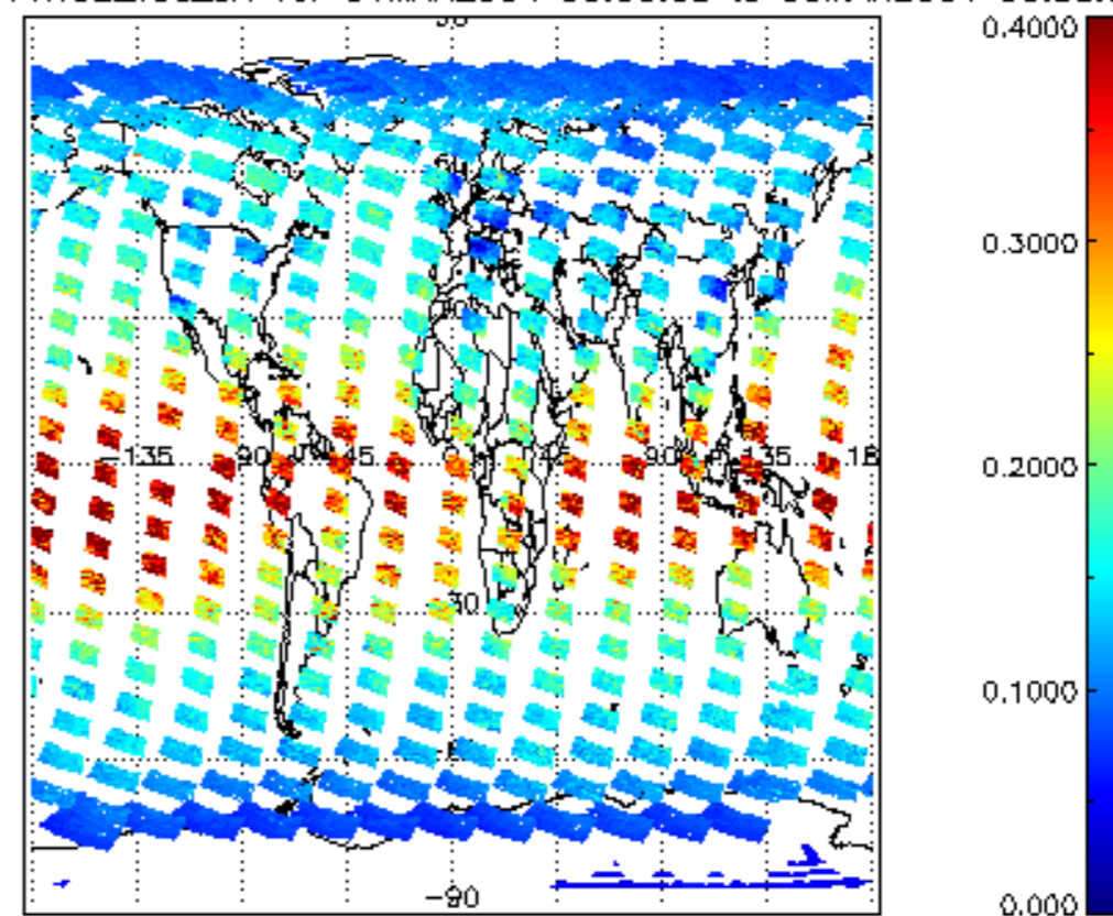
SCIOL2P_NADUV1NO2_vcd_err for 04MAR2004 00:00:00 to 05MAR2004 00:00:00
