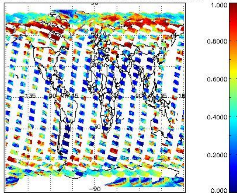
cL_frac for 04MAR2004 00:00:00 to 05MAR2004 00:00:00
