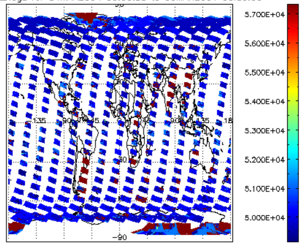
cloud_flags for 04MAR2004 00:00:00 to 05MAR2004 00:00:00
