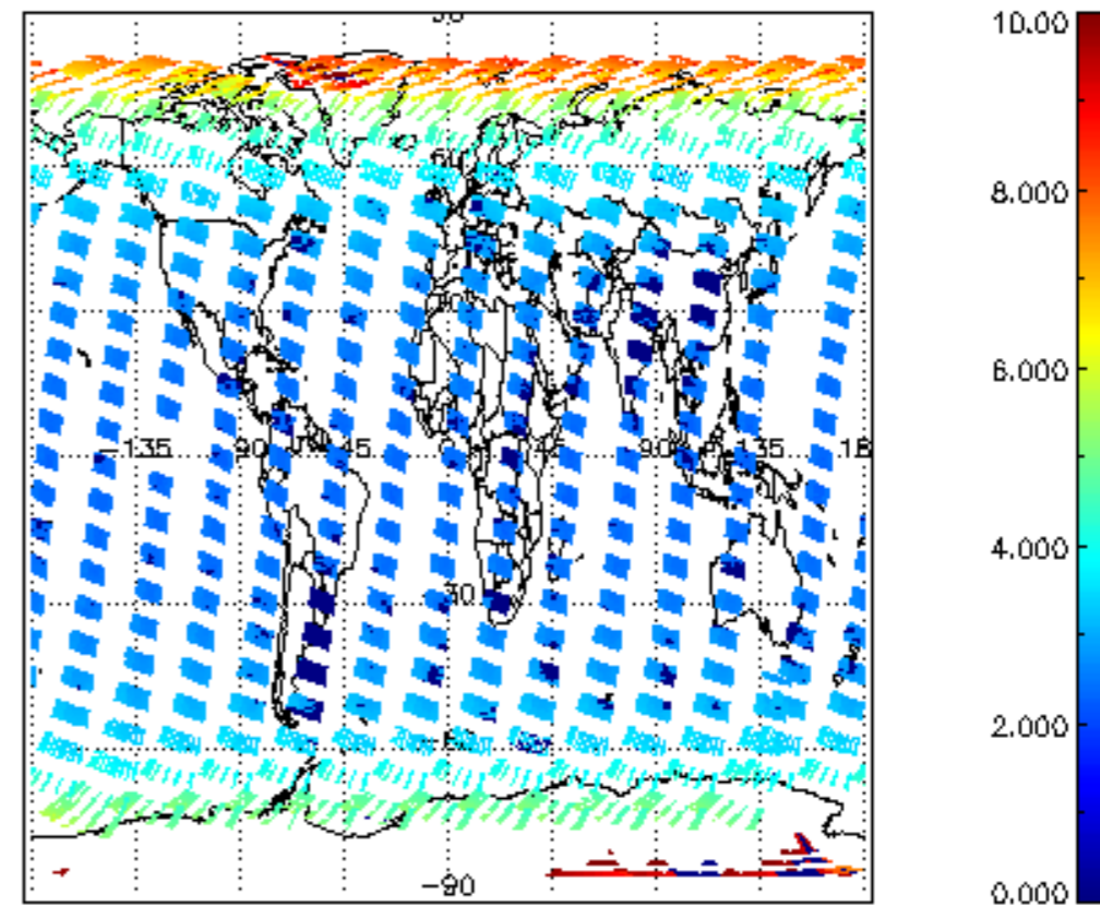
SCIOL2P_NADUV003_amf_cl for 04MAR2004 00:00:00 to 05MAR2004 00:00:00
