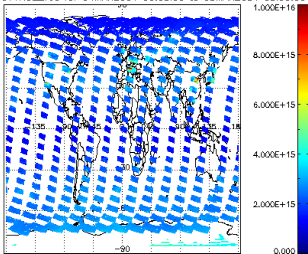
SCIOL2P_NADUV1NO2_vcd for 04MAR2004 00:00:00 to 05MAR2004 00:00:00
