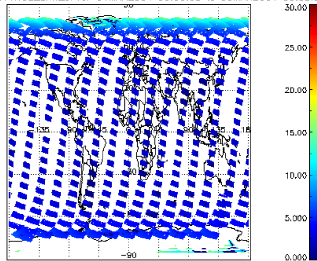
SCIOL2P_NADUV1NO2_amf_cl for 04MAR2004 00:00:00 to 05MAR2004 00:00:00
