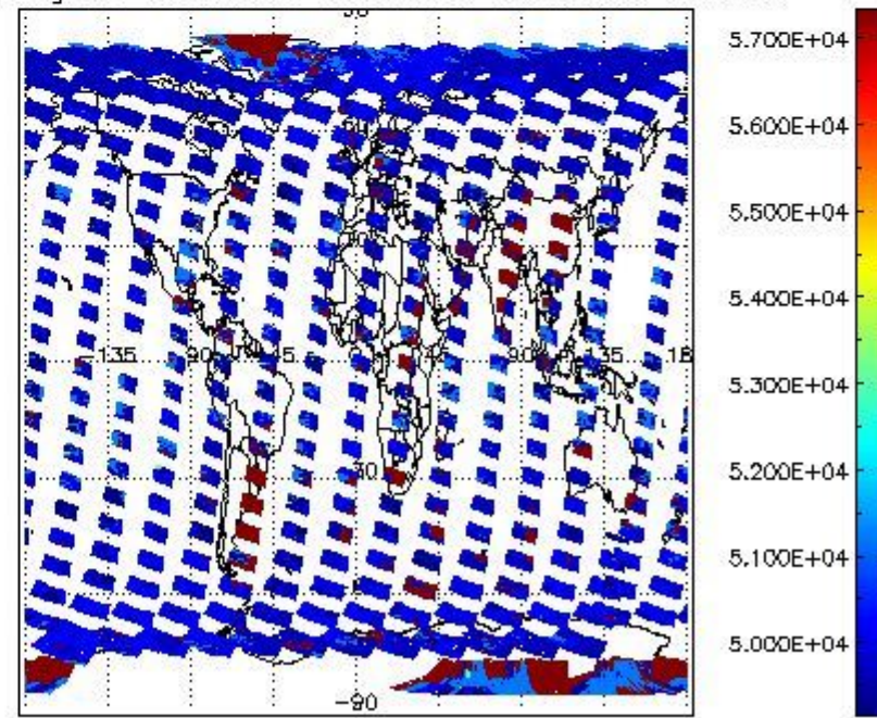
cloud_flags for 04MAR2004 00:00:00 to 05MAR2004 00:00:00
