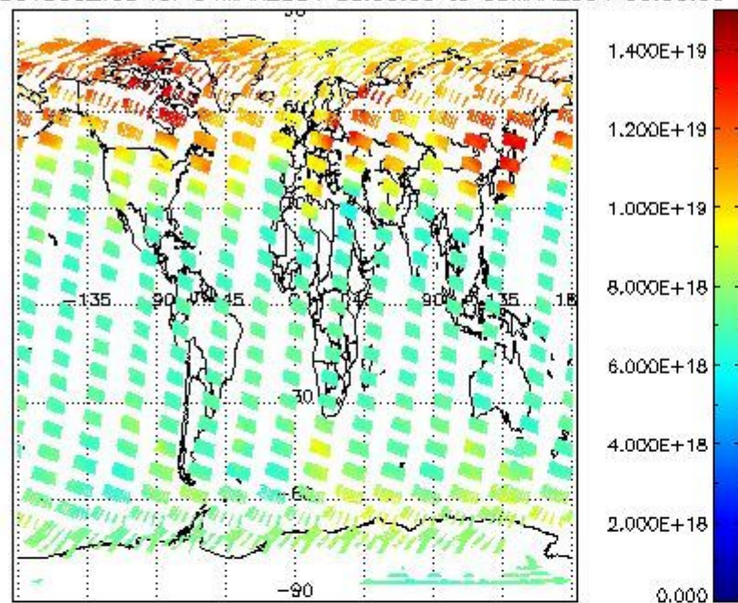
SCIOL2P_NADUV003_vcd for 04MAR2004 00:00:00 to 05MAR2004 00:00:00 SCIOL2P_NADUV003_vcd_err for 04MAR2004 00:00:00 to 05MAR2004 00:00:00
