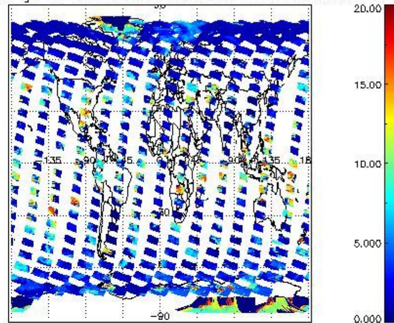
cL_top_height for 04MAR2004 00:00:00 to 05MAR2004 00:00:00
