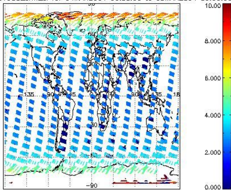
SCIOL2P_NADUV003_amf_gr for 04MAR2004 00:00:00 to 05MAR2004 00:00:00 SCIOL2P_NADUV003_amf_cl for 04MAR2004 00:00:00 to 05MAR2004 00:00:00
