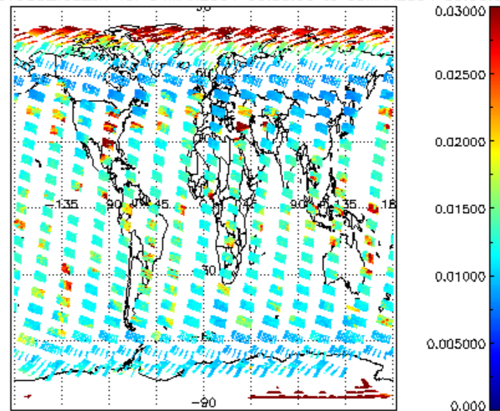
SCIOL2P_NADUV003_vcd_err for 04MAR2004 00:00:00 to 05MAR2004 00:00:00
