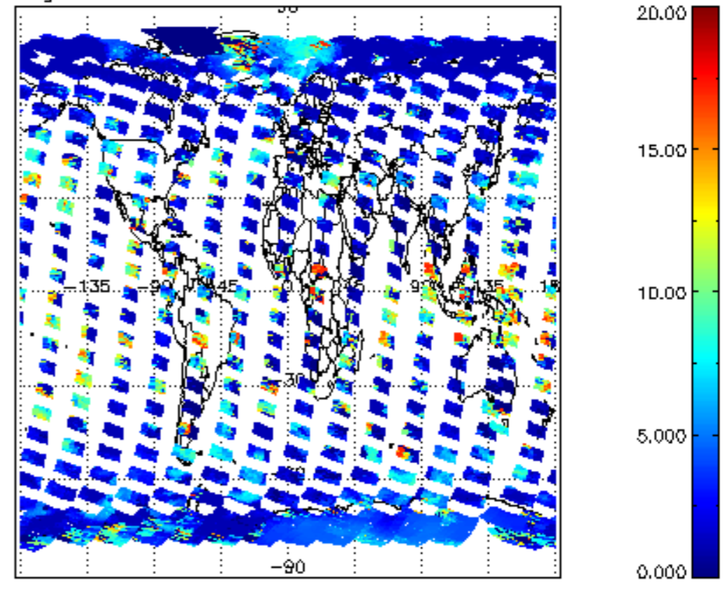
cL_top_height for 03MAR2004 00:00:00 to 04MAR2004 00:00:00
