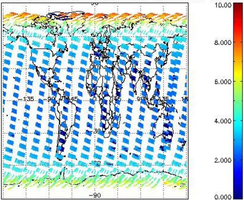
SCIOL2P_NADUV003_amf_cl for 03MAR2004 00:00:00 to 04MAR2004 00:00:00
