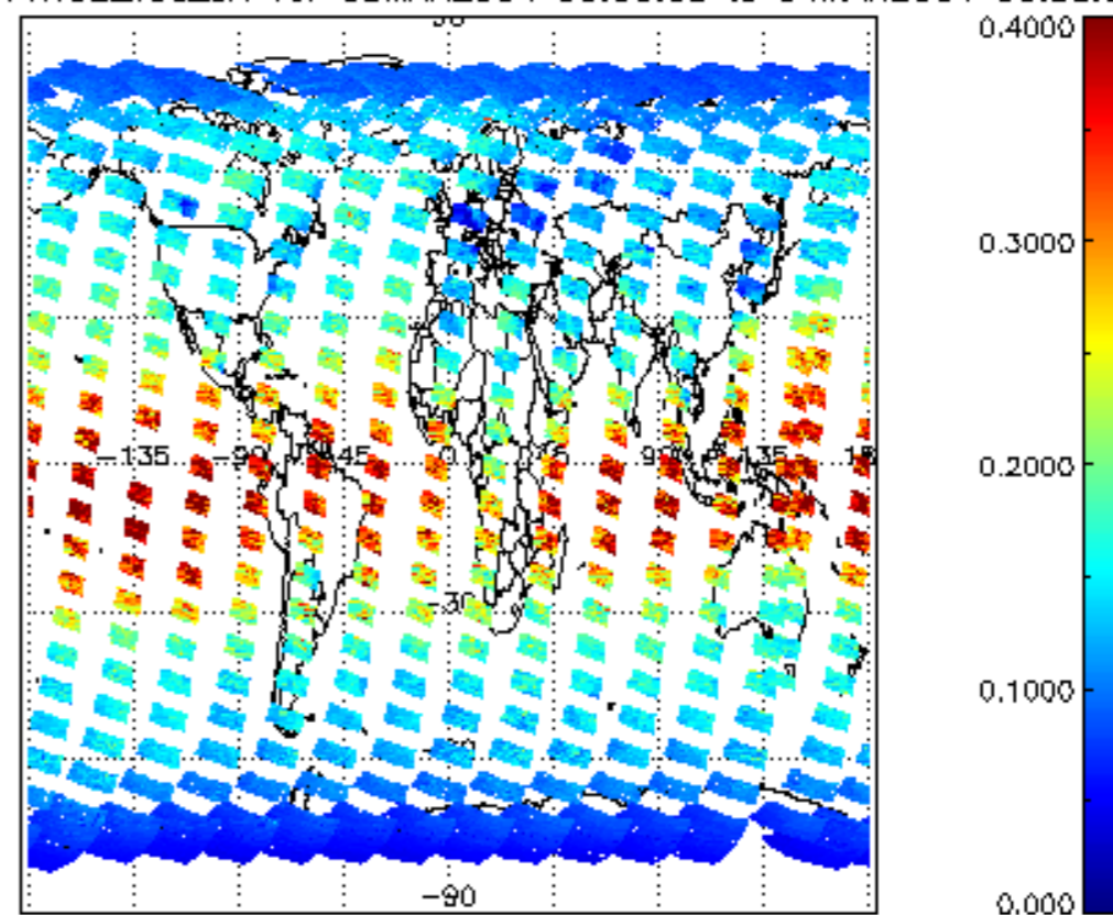
SCIOL2P_NADUV1NO2_vcd_err for 03MAR2004 00:00:00 to 04MAR2004 00:00:00
