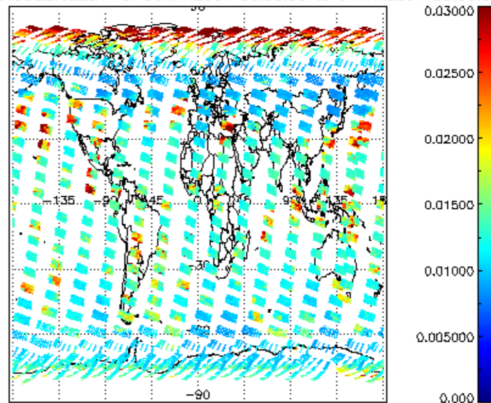
SCIOL2P_NADUV003_vcd_err for 03MAR2004 00:00:00 to 04MAR2004 00:00:00
