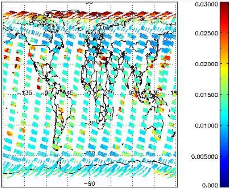
SCIOL2P_NADUV003_vcd_err for 03MAR2004 00:00:00 to 04MAR2004 00:00:00
