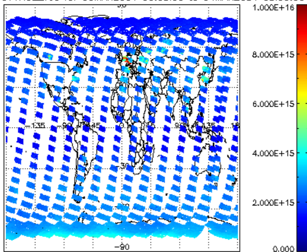
SCIOL2P_NADUV1NO2_vcd for 03MAR2004 00:00:00 to 04MAR2004 00:00:00
