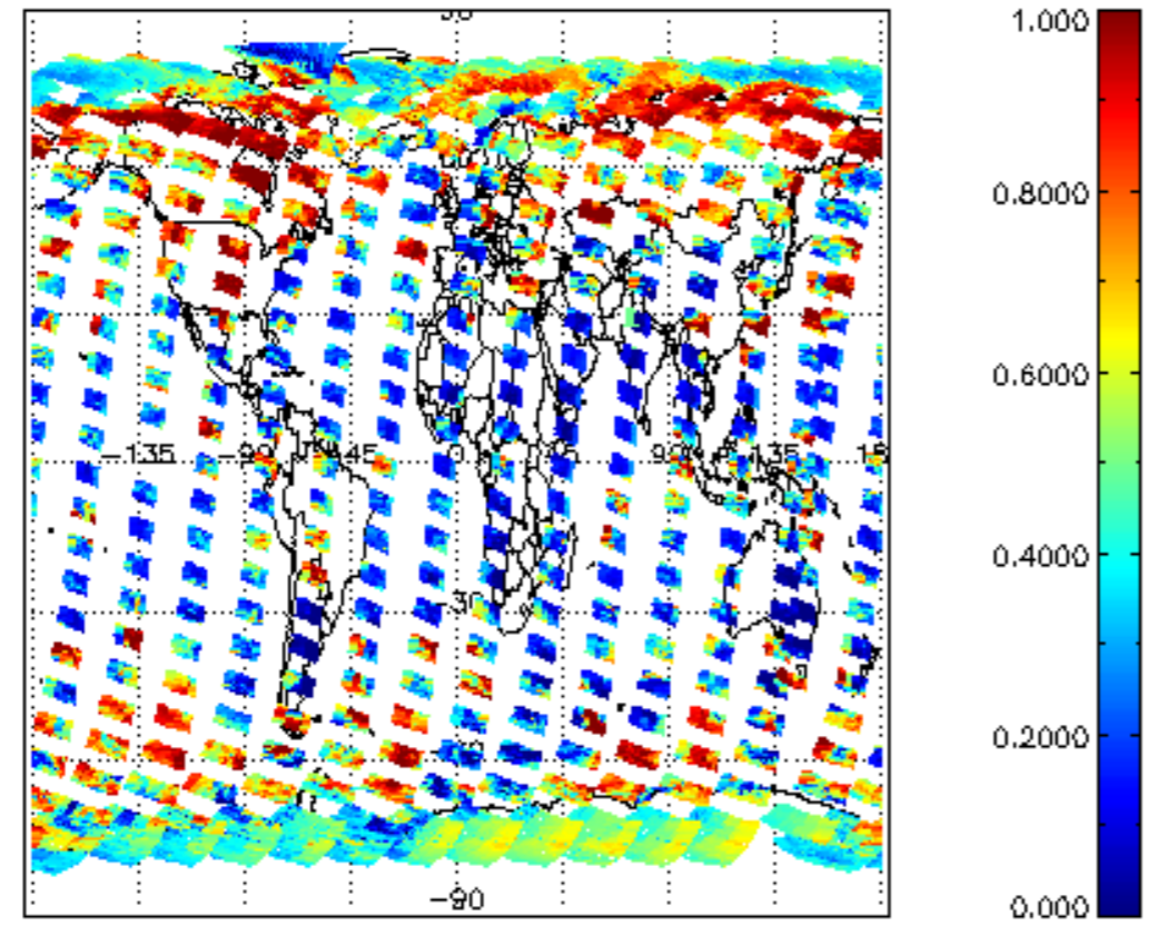
cLfrac for 03MAR2004 00:00:00 to 04MAR2004 00:00:00
