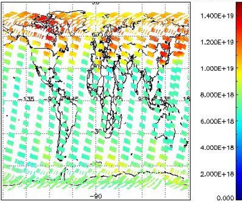
SCIOL2P_NADUV003_vcd for 03MAR2004 00:00:00 to 04MAR2004 00:00:00
