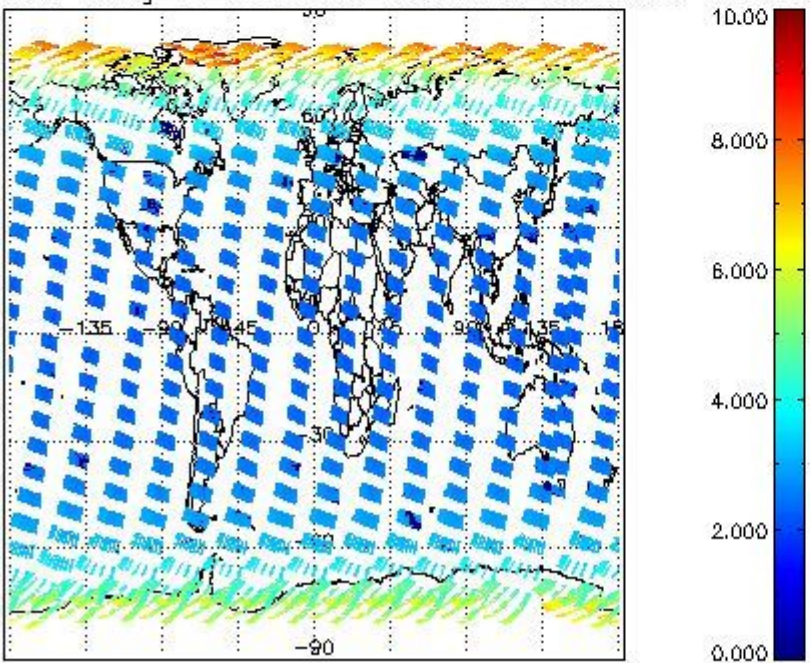
SCIOL2P_NADUV003_amf_gr for 03MAR2004 00:00:00 to 04MAR2004 00:00:00
