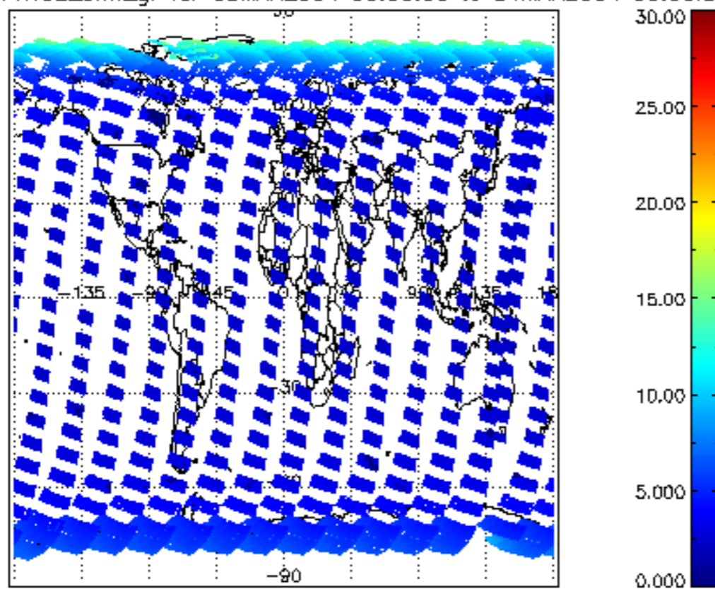
SCIOL2P_NADUV1NO2_amf_gr for 03MAR2004 00:00:00 to 04MAR2004 00:00:00
