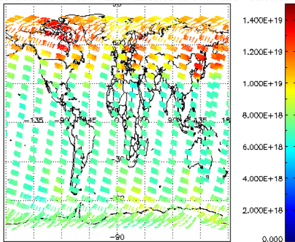
SCIOL2P_NADUV003_vcd for 03MAR2004 00:00:00 to 04MAR2004 00:00:00
