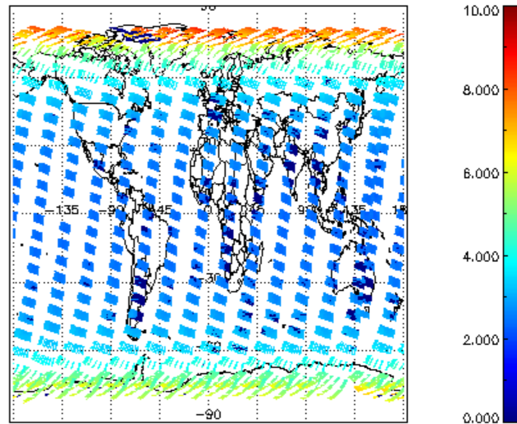
SCIOL2P_NADUV003_amf_cl for 03MAR2004 00:00:00 to 04MAR2004 00:00:00
