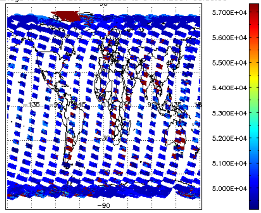
cloud_flags for 03MAR2004 00:00:00 to 04MAR2004 00:00:00
