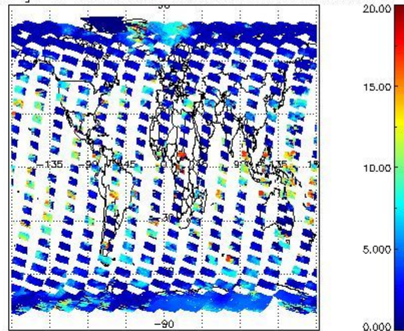
cL_top_height for 03MAR2004 00:00:00 to 04MAR2004 00:00:00
