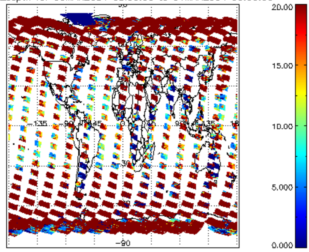
cL_opt_depth for 03MAR2004 00:00:00 to 04MAR2004 00:00:00
