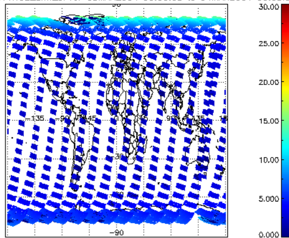
SCIOL2P_NADUV1NO2_amf_cl for 03MAR2004 00:00:00 to 04MAR2004 00:00:00
