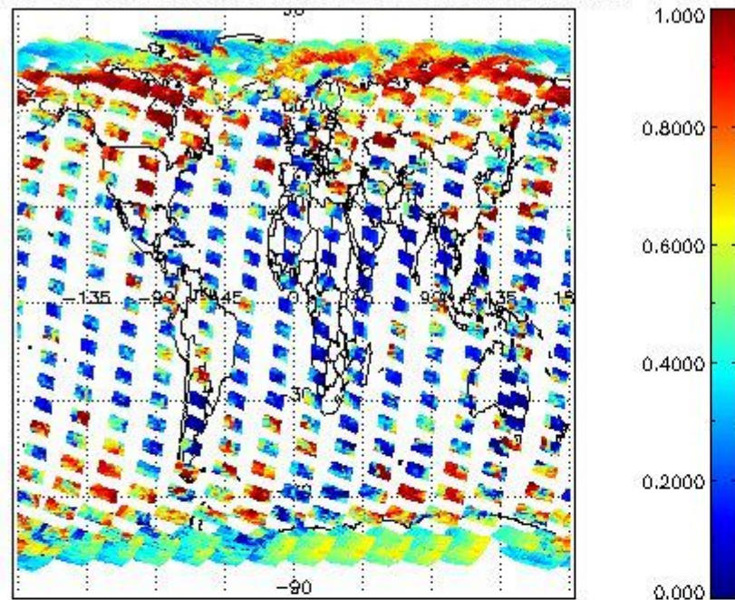
cL_frac for 03MAR2004 00:00:00 to 04MAR2004 00:00:00
