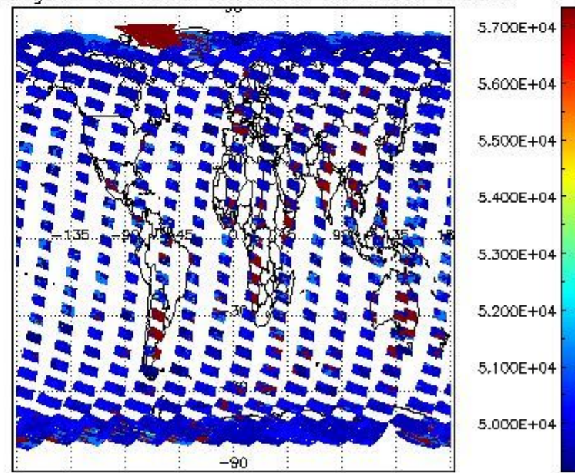
cloud_flags for 03MAR2004 00:00:00 to 04MAR2004 00:00:00
