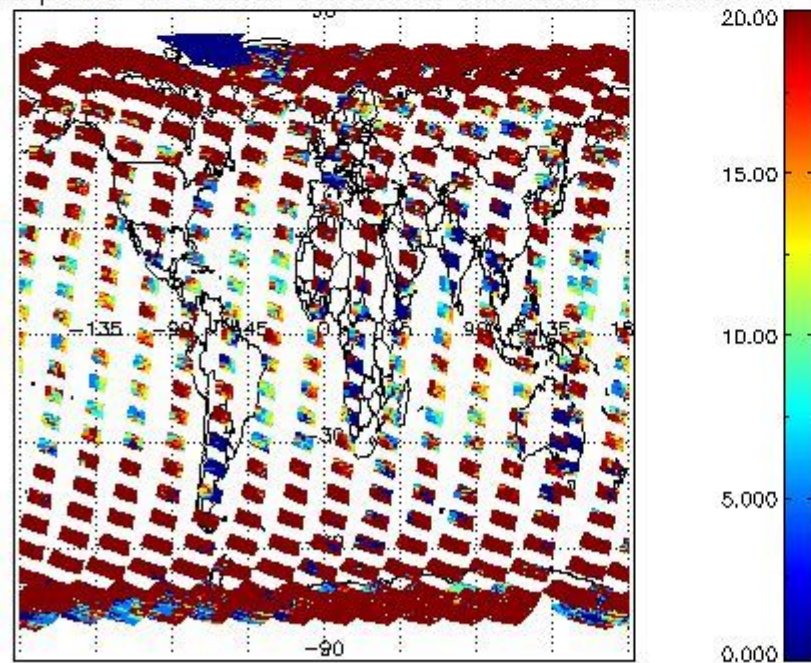
cL_opt_depth for 03MAR2004 00:00:00 to 04MAR2004 00:00:00
