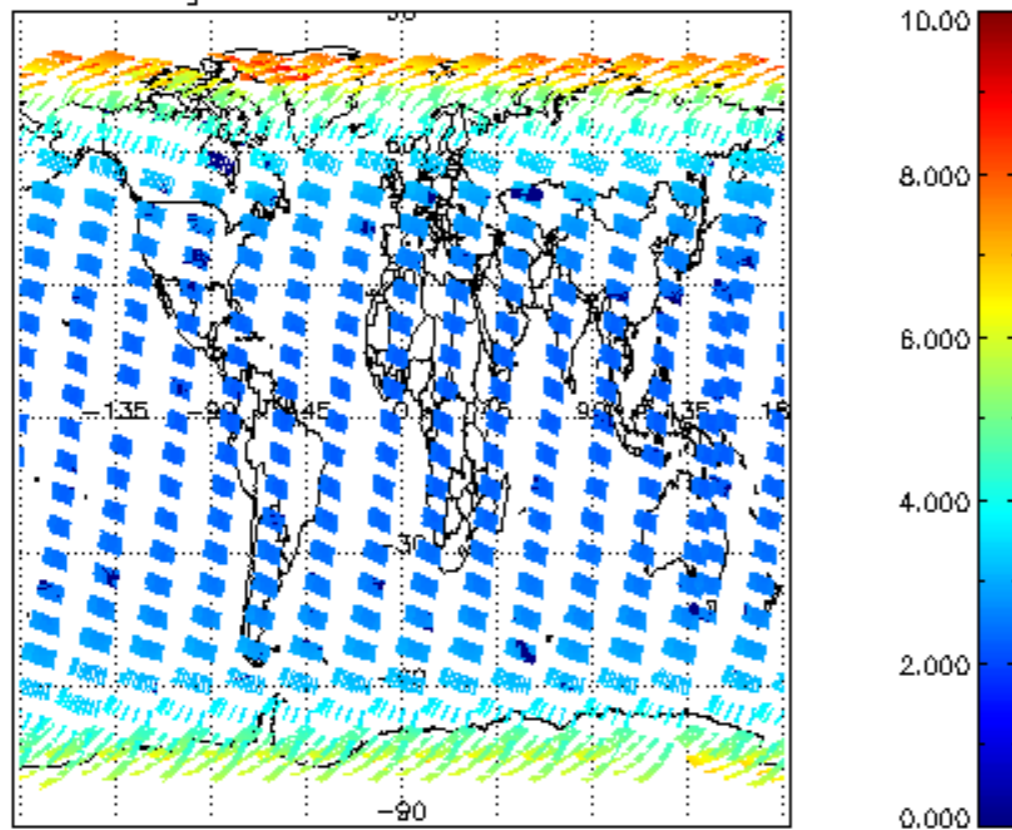
SCIOL2P_NADUV003_amf_gr for 03MAR2004 00:00:00 to 04MAR2004 00:00:00
