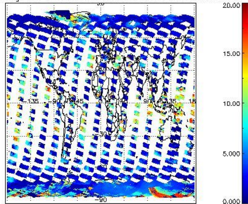
cL_top_height for 29FEB2004 00:00:00 to 01MAR2004 00:00:00
