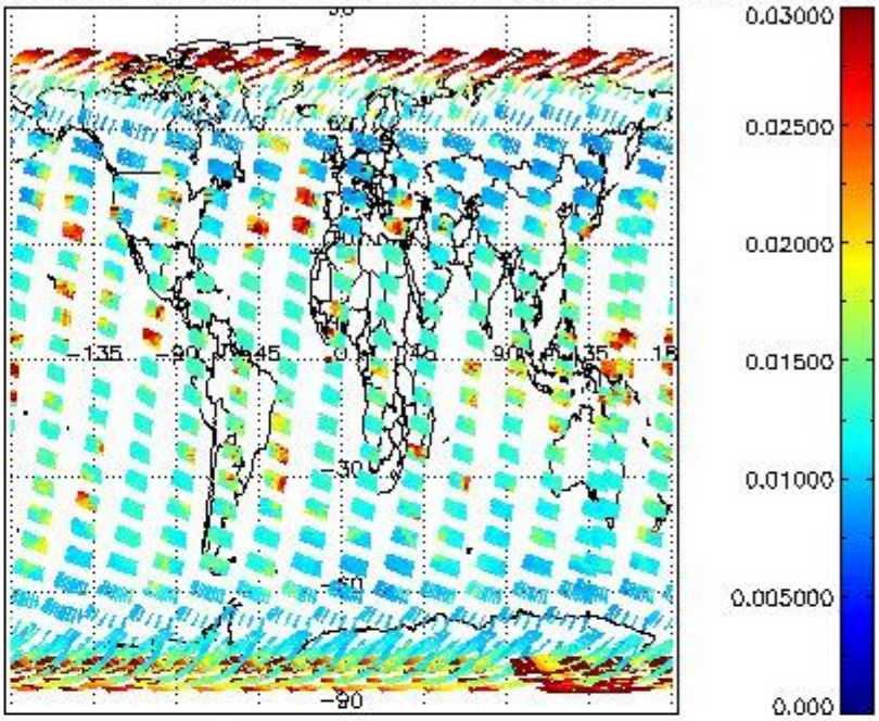
SCIOL2P_NADUV003_vcd_err for 29FEB2004 00:00:00 to 01MAR2004 00:00:00
