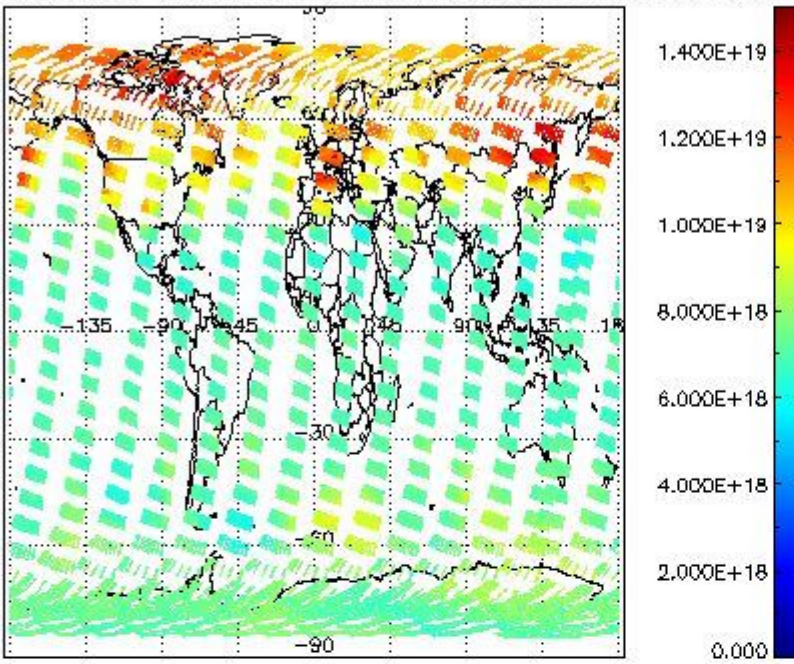
SCIOL2P_NADUV003_vcd for 29FEB2004 00:00:00 to 01MAR2004 00:00:00
