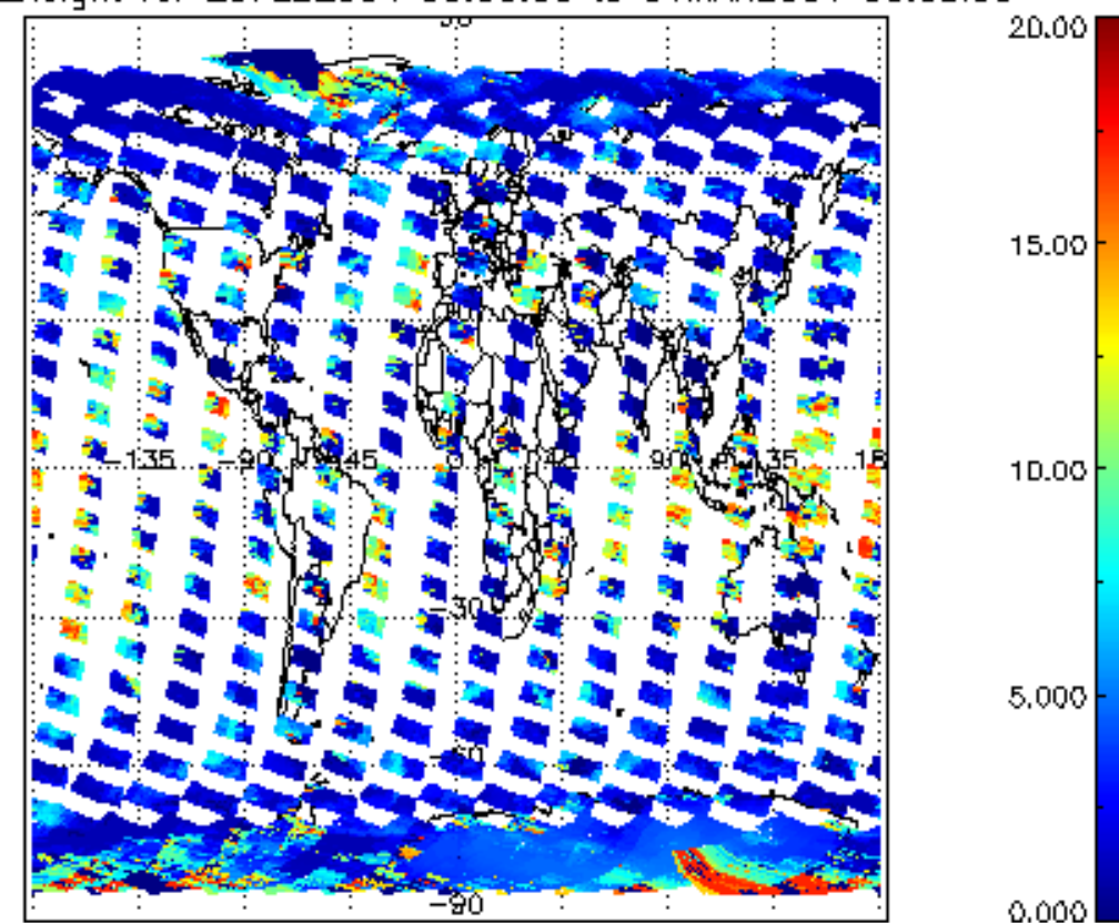
cL_top_height for 29FEB2004 00:00:00 to 01MAR2004 00:00:00
