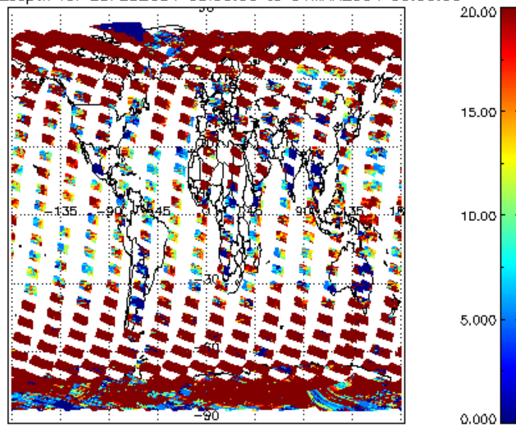
cL_opt_depth for 29FEB2004 00:00:00 to 01MAR2004 00:00:00
