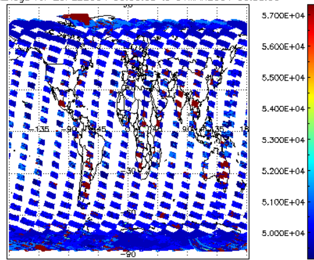
cloud_flags for 29FEB2004 00:00:00 to 01MAR2004 00:00:00
