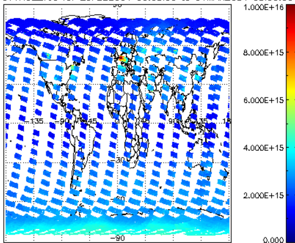
SCIOL2P_NADUV1NO2_vcd for 29FEB2004 00:00:00 to 01MAR2004 00:00:00 ; ICIOL2P_NADUV1NO2_vcd_err for 29FEB2004 00:00:00 to 01MAR2004 00:00:00
