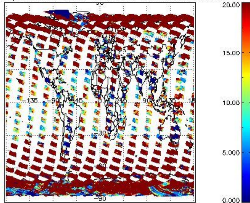
cL_opt_depth for 29FEB2004 00:00:00 to 01MAR2004 00:00:00
