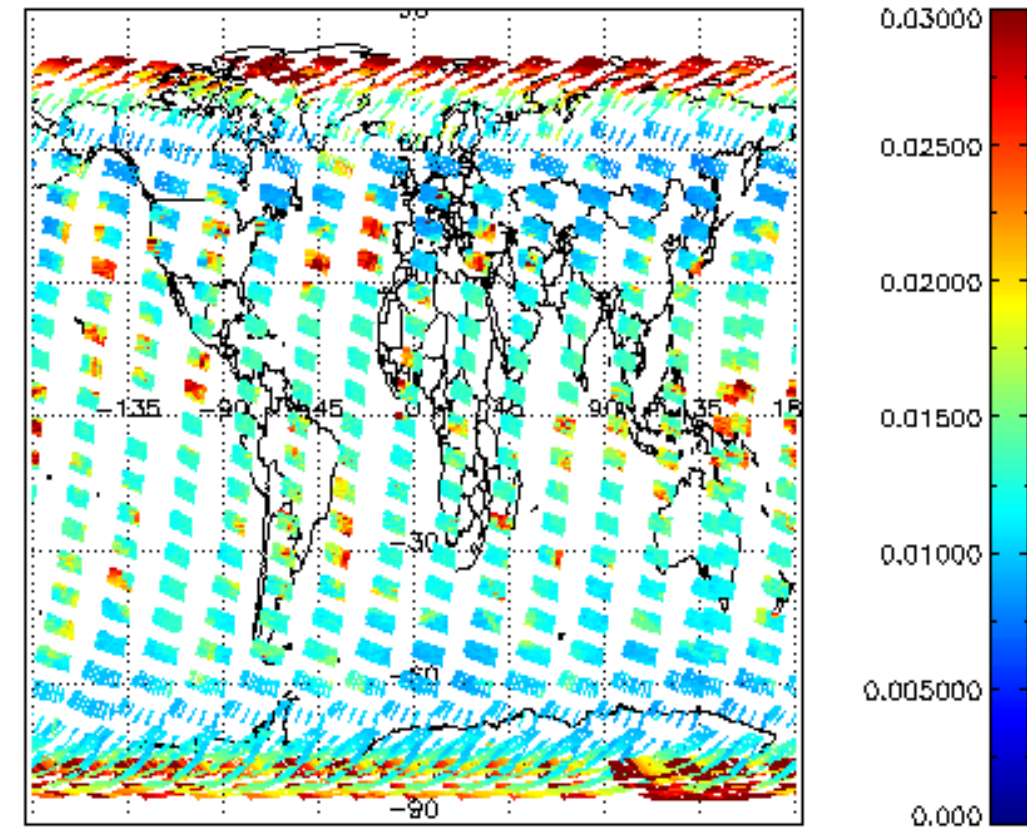
SCIOL2P_NADUV003_vcd_err for 29FEB2004 00:00:00 to 01MAR2004 00:00:00
