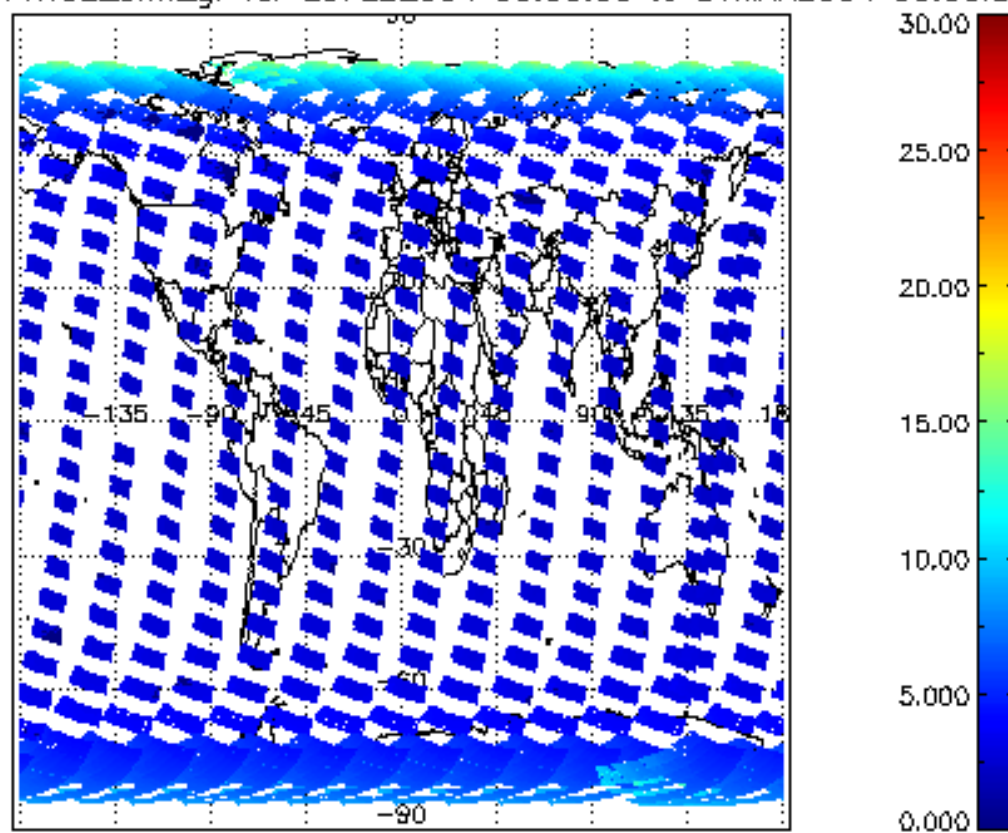
ICIOL2P_NADUV1NO2_amf_gr for 29FEB2004 00:00:00 to 01MAR2004 00:00:00 ; ICIOL2P_NADUV1NO2_amf_cl for 29FEB2004 00:00:00 to 01MAR2004 00:00:00
