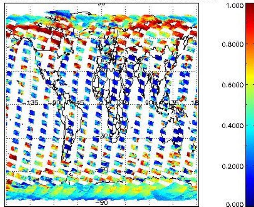
cL_frac for 29FEB2004 00:00:00 to 01MAR2004 00:00:00
