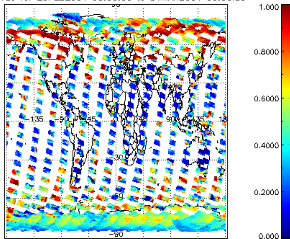
cL_frac for 29FEB2004 00:00:00 to 01MAR2004 00:00:00
