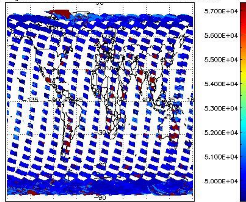
cloud_flags for 29FEB2004 00:00:00 to 01MAR2004 00:00:00
