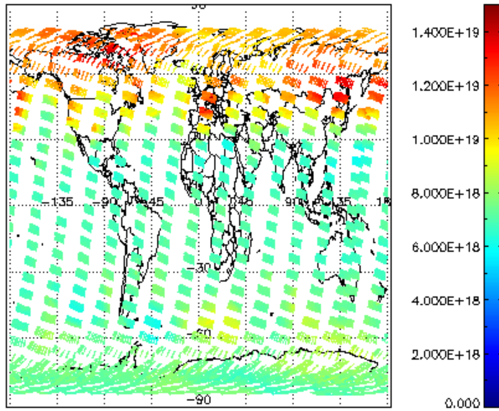
SCIOL2P_NADUV003_vcd for 29FEB2004 00:00:00 to 01MAR2004 00:00:00
