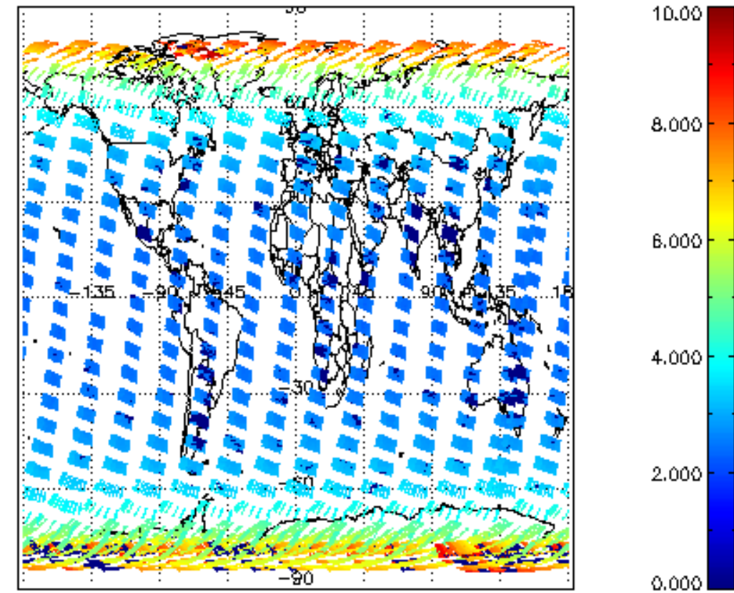
SCIOL2P_NADUV003_amf_cl for 29FEB2004 00:00:00 to 01MAR2004 00:00:00
