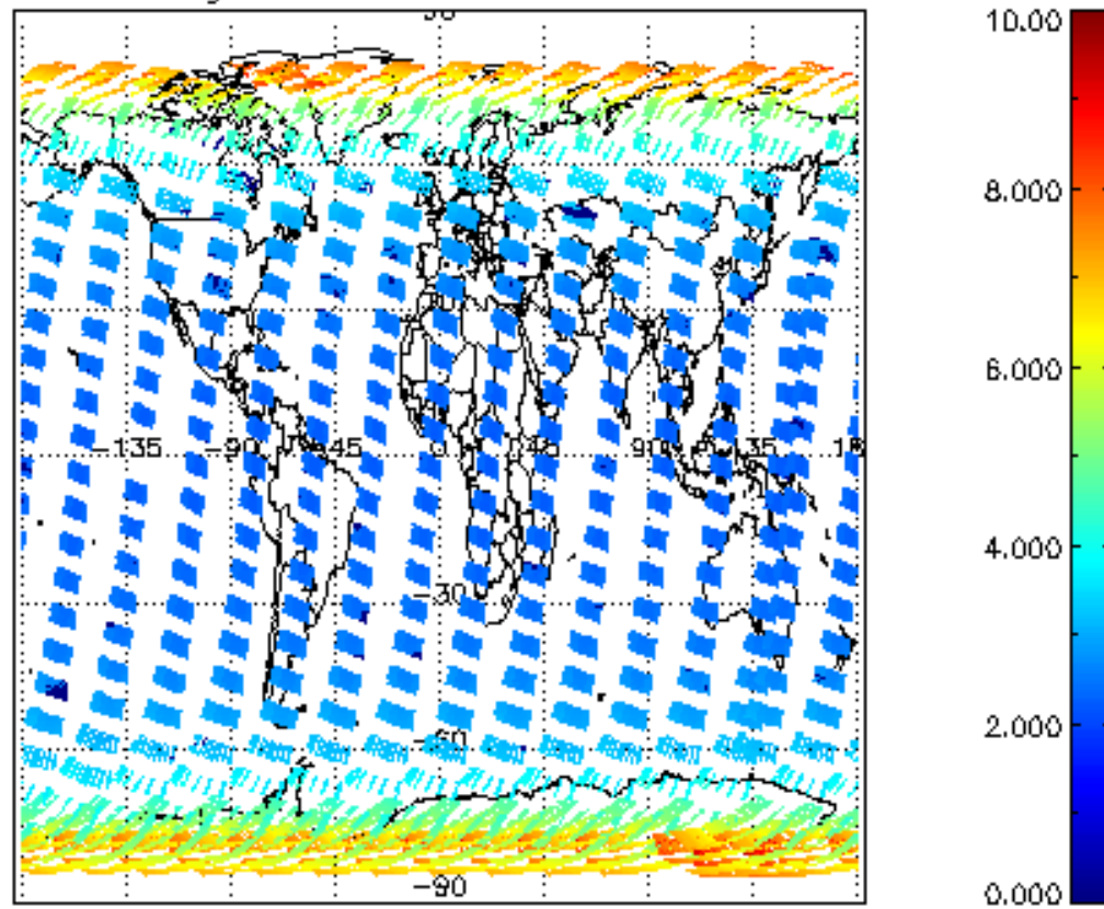
SCIOL2P_NADUV003_amf_gr for 29FEB2004 00:00:00 to 01MAR2004 00:00:00
