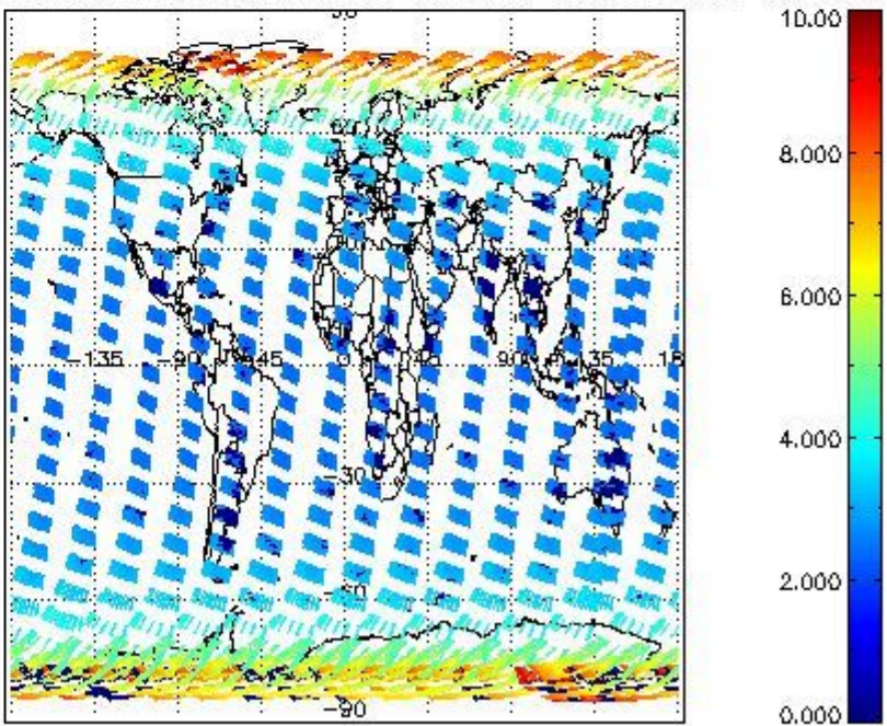
SCIOL2P_NADUV003_amf_cl for 29FEB2004 00:00:00 to 01MAR2004 00:00:00
