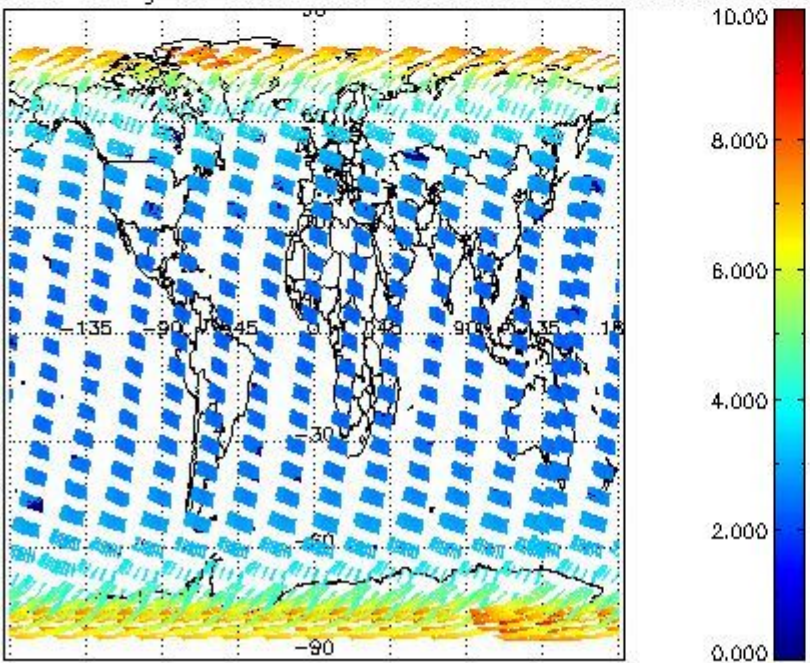
SCIOL2P_NADUV003_amf_gr for 29FEB2004 00:00:00 to 01MAR2004 00:00:00
