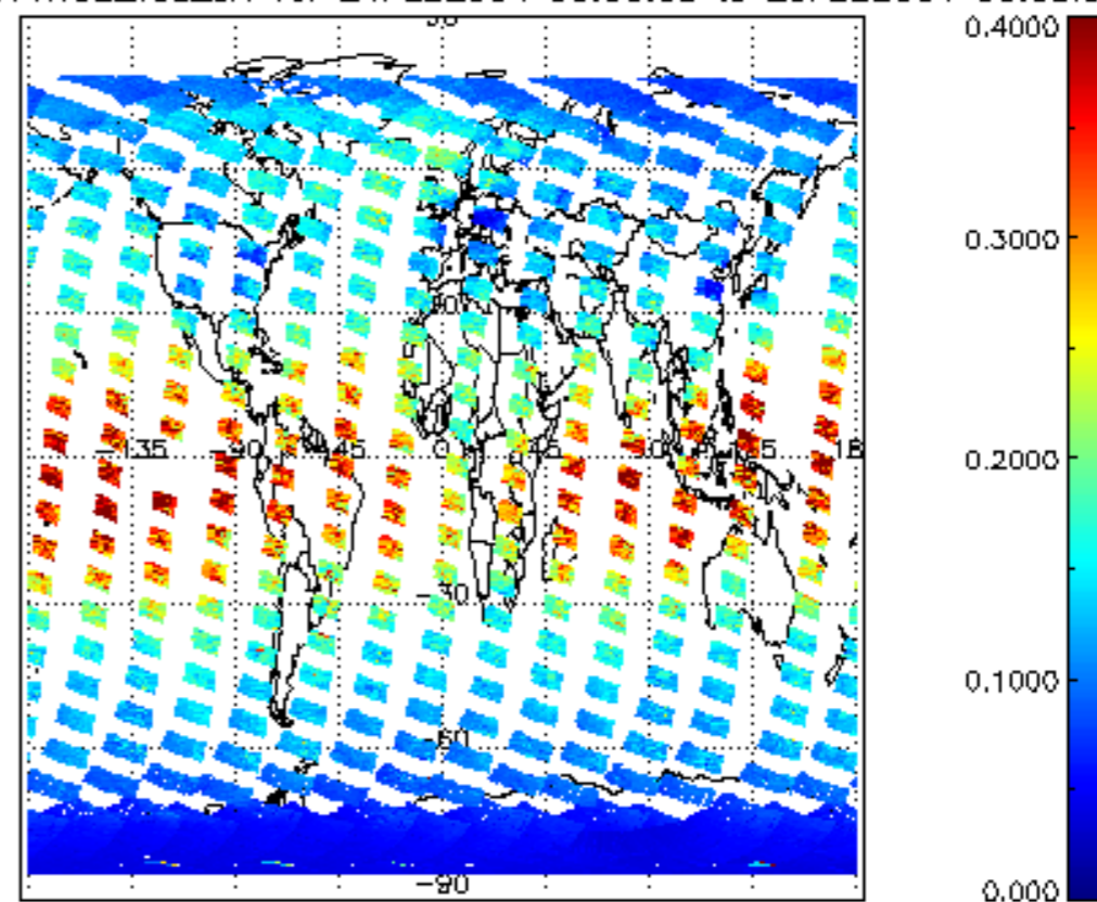
SCIOL2P_NADUV1NO2_vcd_err for 24FEB2004 00:00:00 to 25FEB2004 00:00:00
