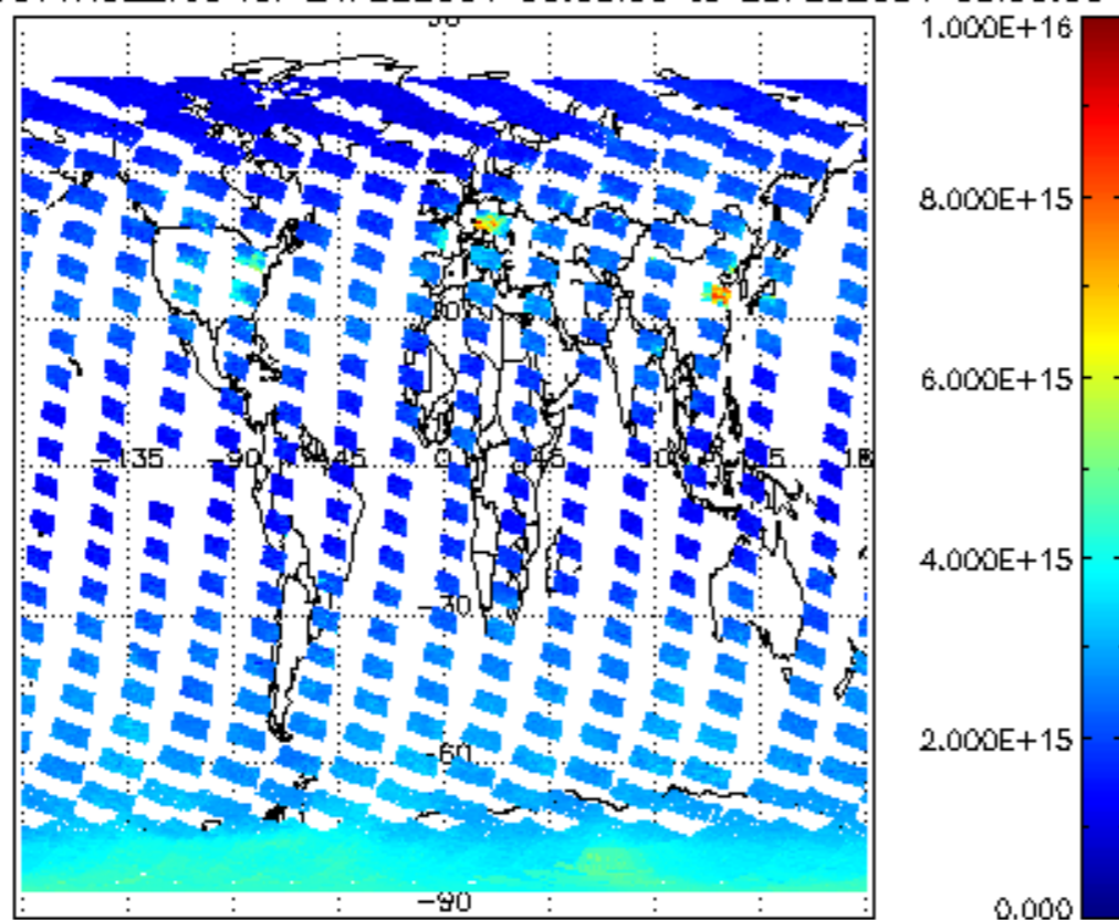
SCIOL2P_NADUV1NO2_vcd for 24FEB2004 00:00:00 to 25FEB2004 00:00:00
