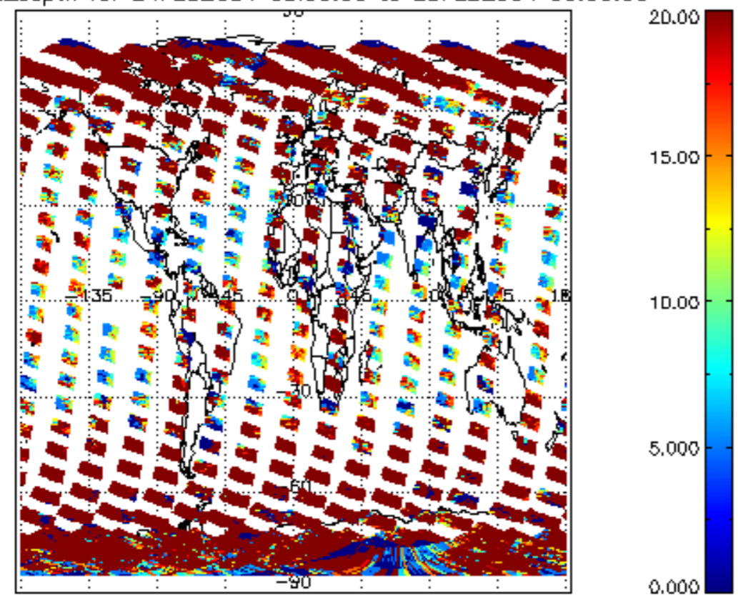
cl_opt_depth for 24FEB2004 00:00:00 to 25FEB2004 00:00:00
