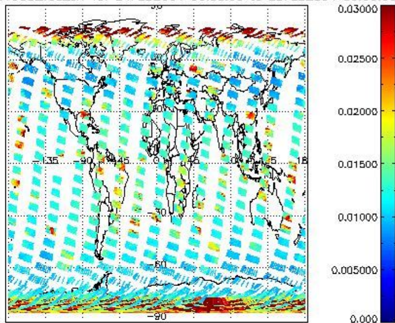
SCIOL2P_NADUV003_vcd_err for 24FEB2004 00:00:00 to 25FEB2004 00:00:00
