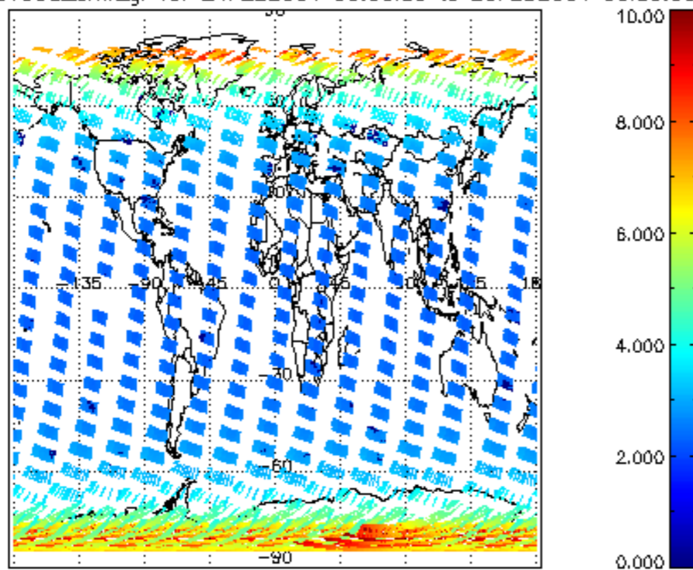
SCIOL2P_NADUV003_amf_gr for 24FEB2004 00:00:00 to 25FEB2004 00:00:00
