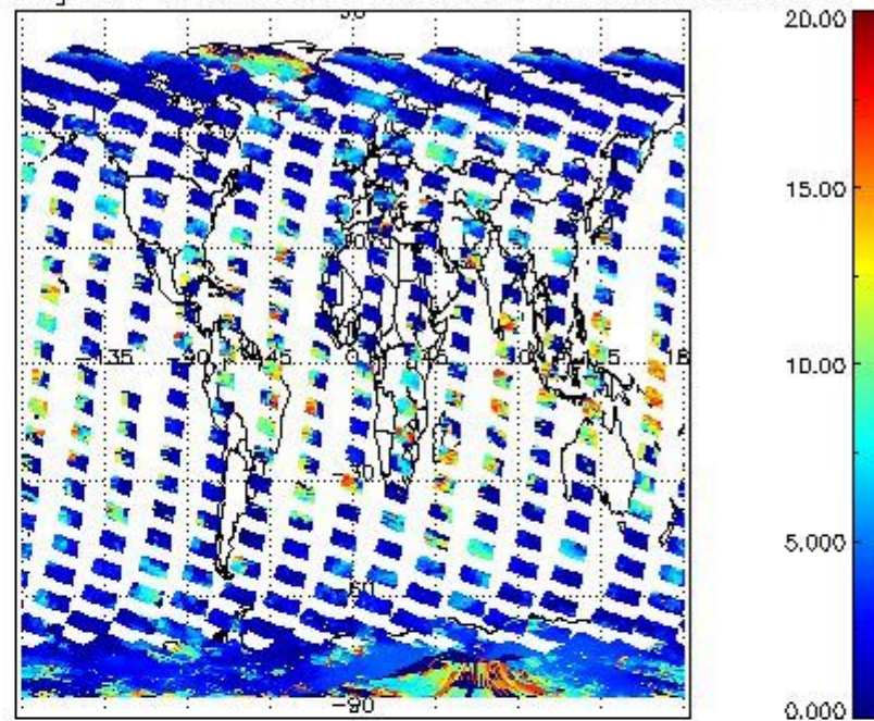
cL_top_height for 24FEB2004 00:00:00 to 25FEB2004 00:00:00
