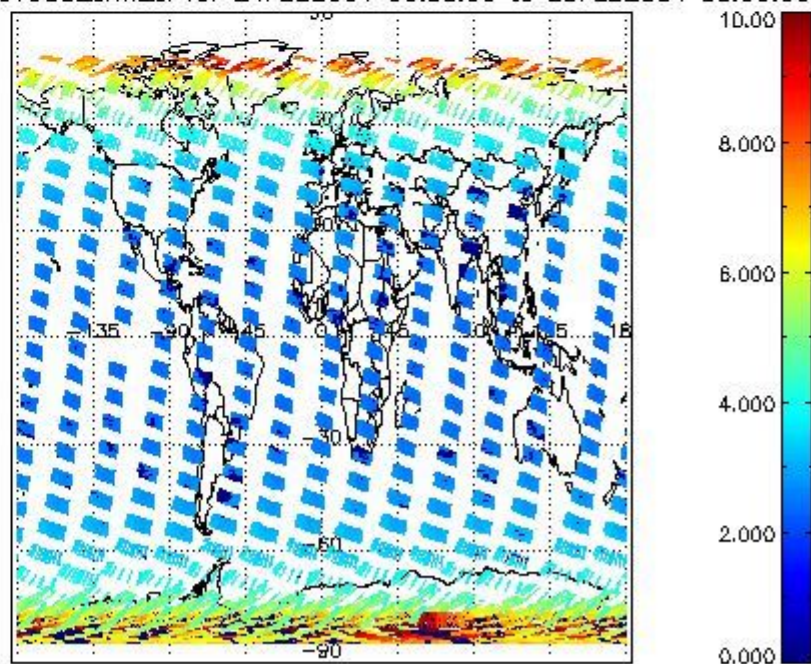
SCIOL2P_NADUV003_amf_cl for 24FEB2004 00:00:00 to 25FEB2004 00:00:00
