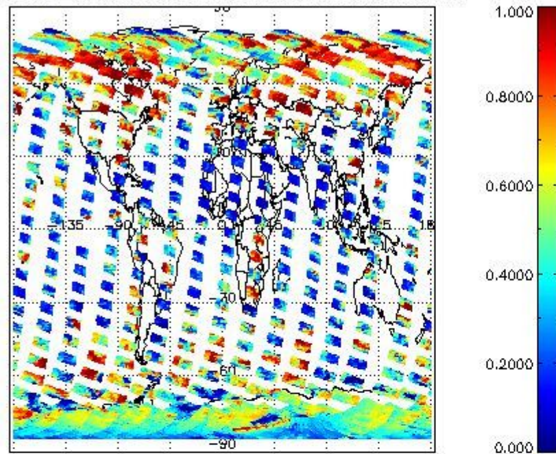
cLfrac for 24FEB2004 00:00:00 to 25FEB2004 00:00:00
