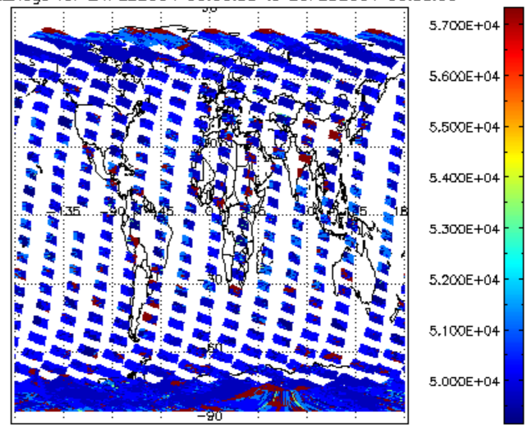
cloud_flags for 24FEB2004 00:00:00 to 25FEB2004 00:00:00
