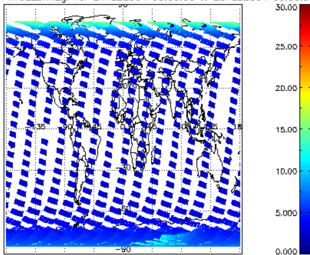
SCIOL2P_NADUV1NO2_amf_gr for 24FEB2004 00:00:00 to 25FEB2004 00:00:00
