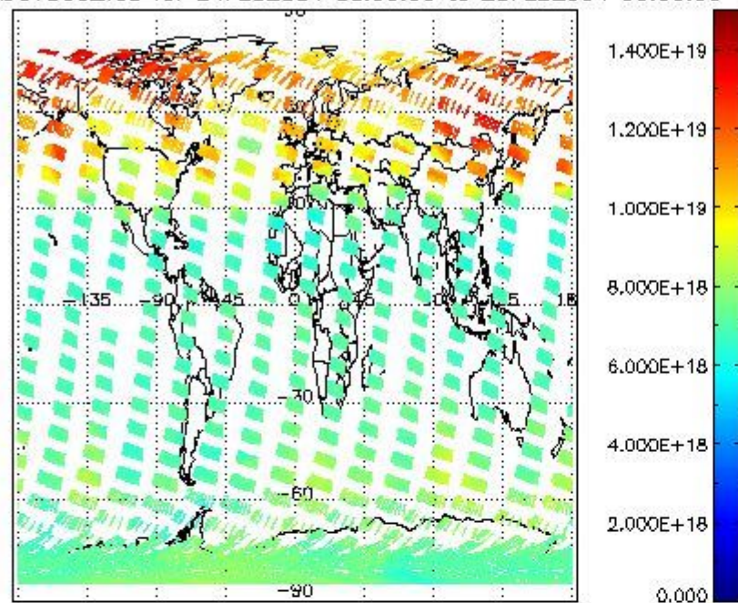
SCIOL2P_NADUV003_vcd for 24FEB2004 00:00:00 to 25FEB2004 00:00:00
