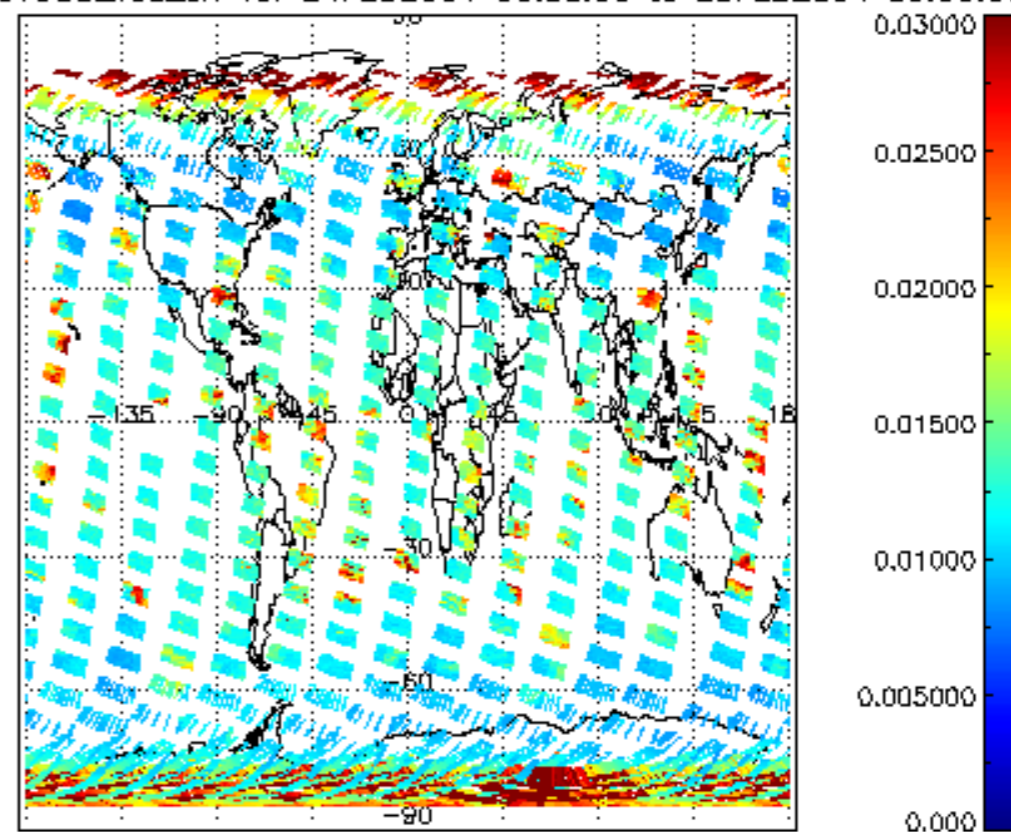
SCIOL2P_NADUV003_vcd_err for 24FEB2004 00:00:00 to 25FEB2004 00:00:00
