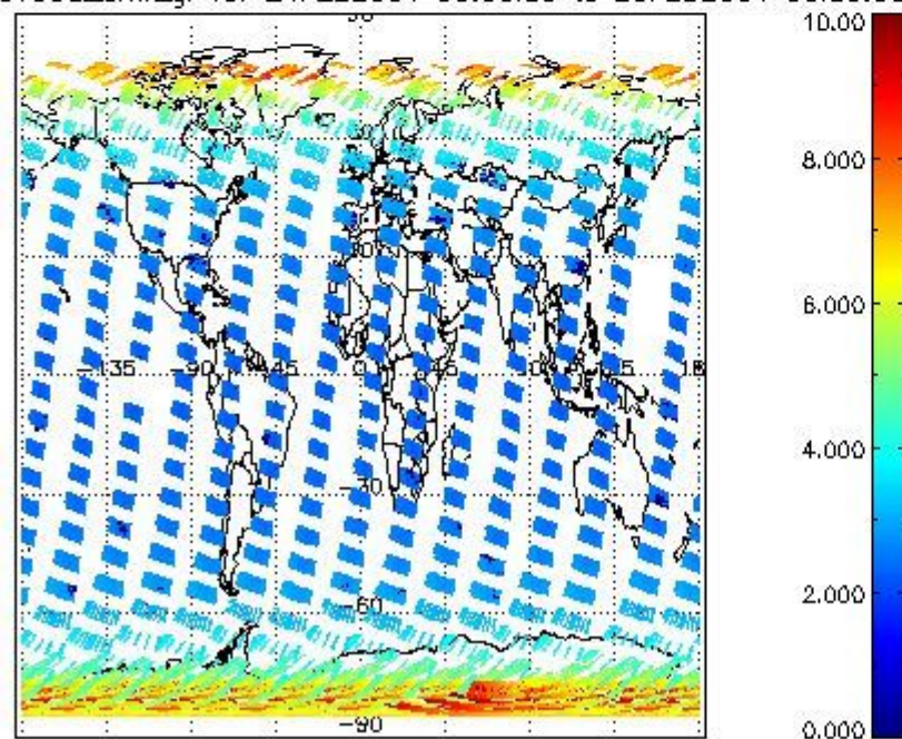
SCIOL2P_NADUV003_amf_gr for 24FEB2004 00:00:00 to 25FEB2004 00:00:00
