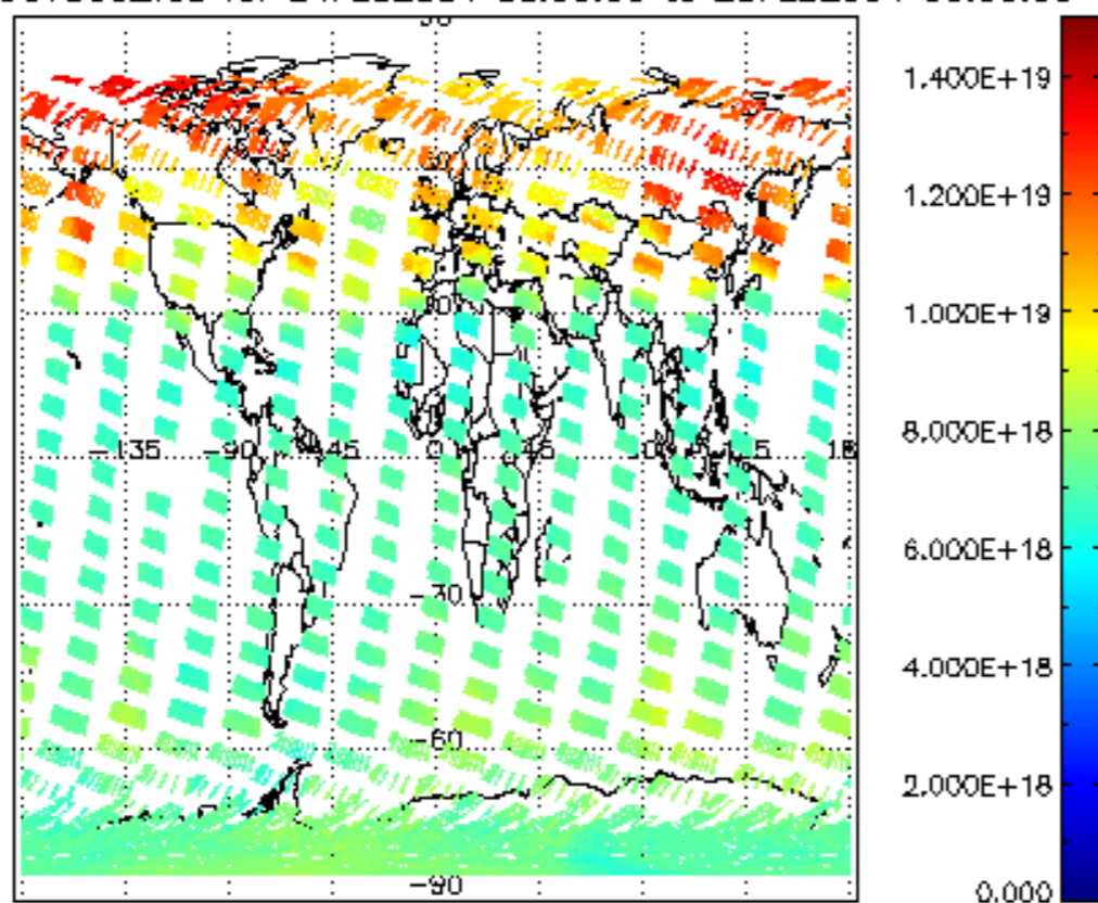
SCIOL2P_NADUV003_vcd for 24FEB2004 00:00:00 to 25FEB2004 00:00:00
