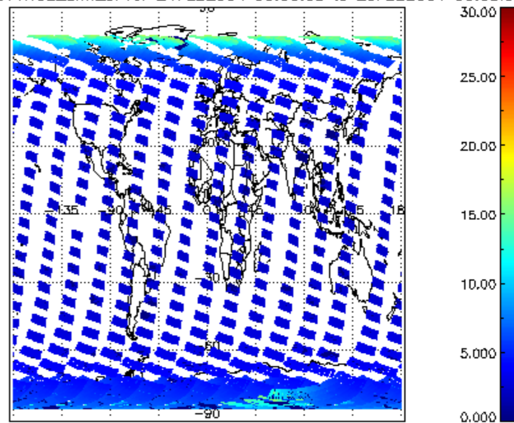
SCIOL2P_NADUV1NO2_amf_cl for 24FEB2004 00:00:00 to 25FEB2004 00:00:00
