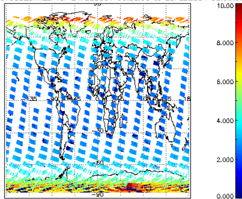
SCIOL2P_NADUV003_amf_cl for 24FEB2004 00:00:00 to 25FEB2004 00:00:00
