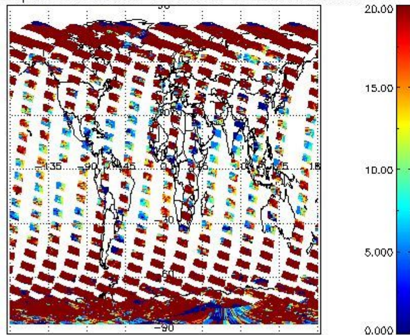
cLopt_depth for 24FEB2004 00:00:00 to 25FEB2004 00:00:00
