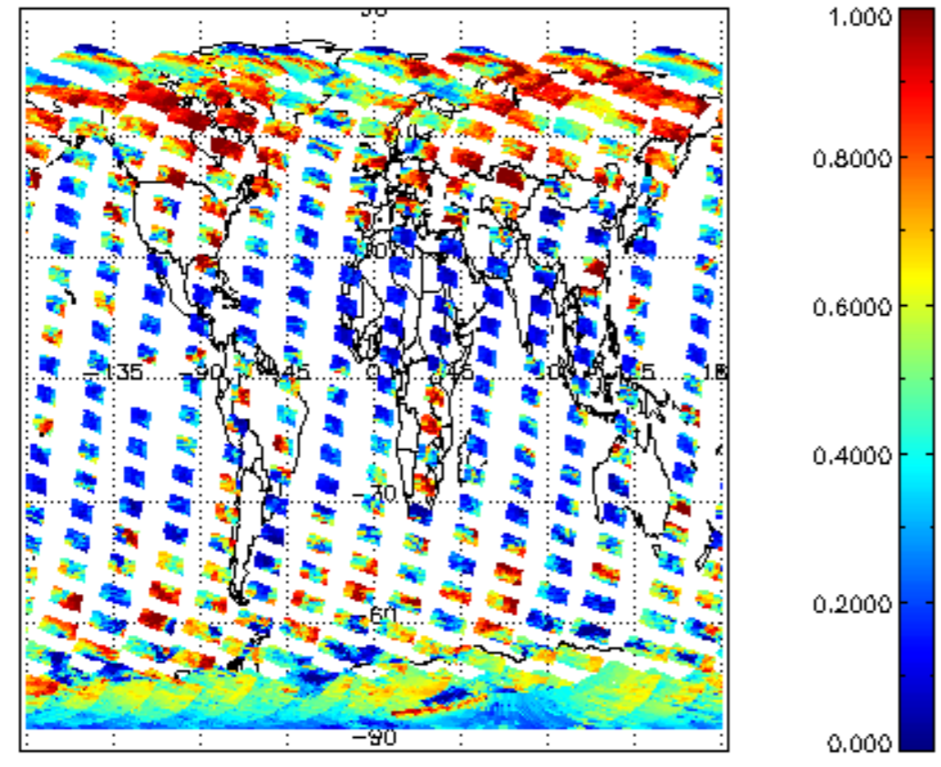
cl_frac for 24FEB2004 00:00:00 to 25FEB2004 00:00:00
