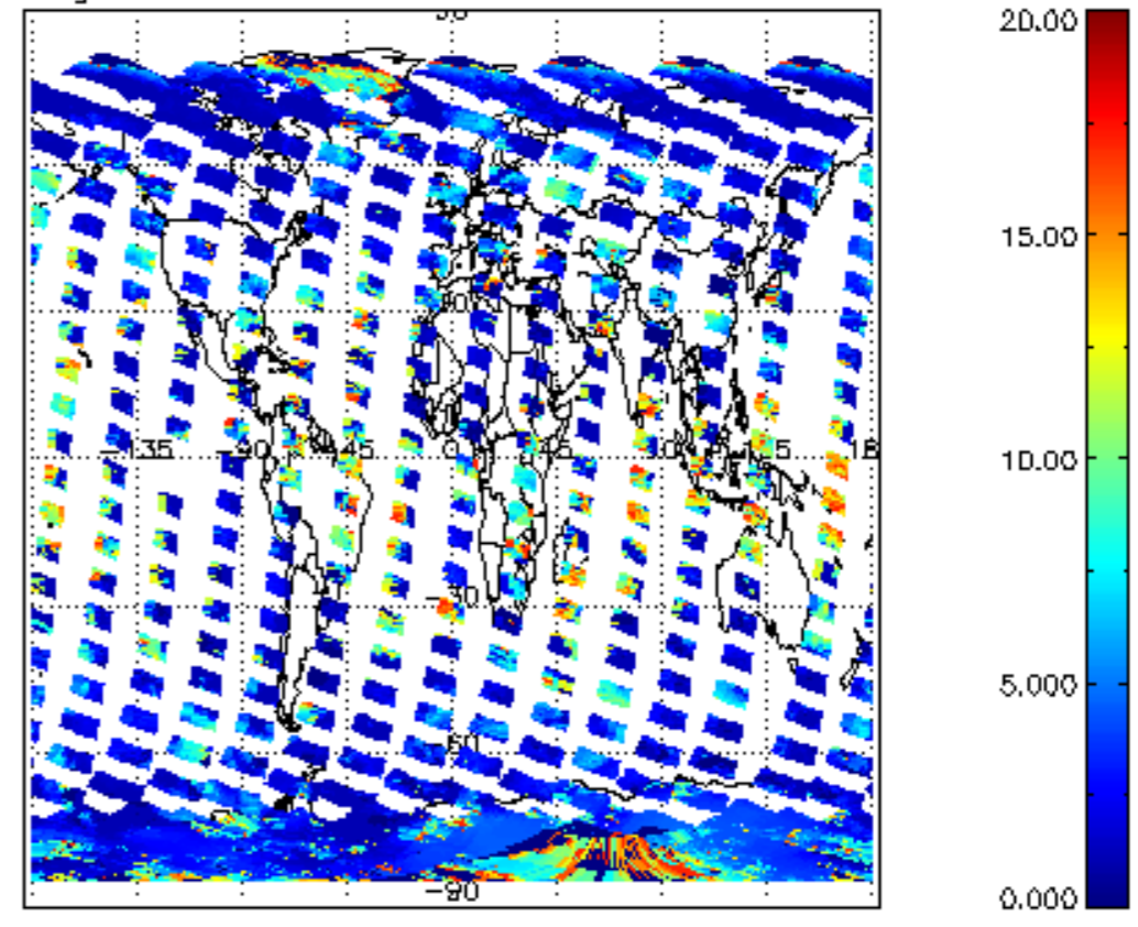
cl_top_height for 24FEB2004 00:00:00 to 25FEB2004 00:00:00
