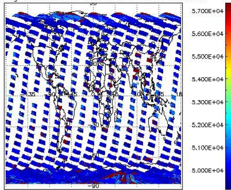
cloud_flags for 24FEB2004 00:00:00 to 25FEB2004 00:00:00
