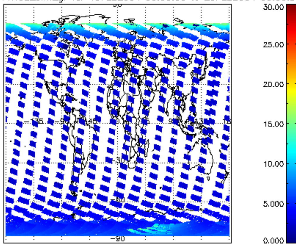
SCIOL2P_NADUV1NO2_amf_gr for 19FEB2004 00:00:00 to 20FEB2004 00:00:00
