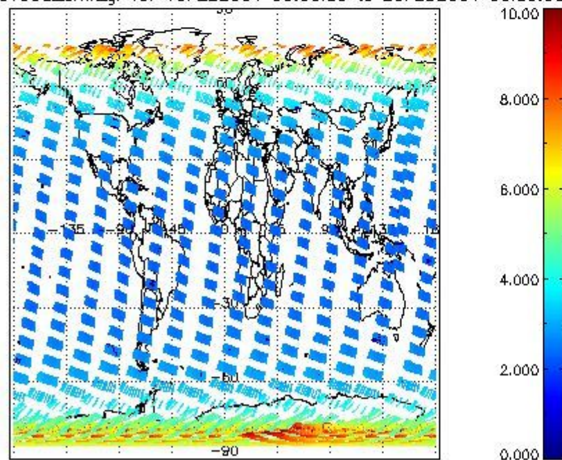
SCIOL2P_NADUV003_amf_gr for 19FEB2004 00:00:00 to 20FEB2004 00:00:00
