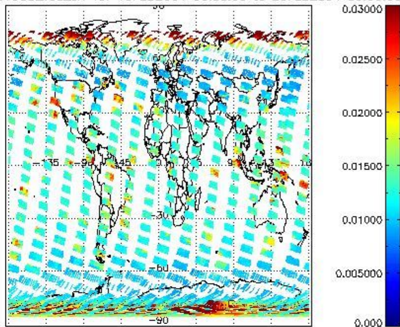
SCIOL2P_NADUV003_vcd_err for 19FEB2004 00:00:00 to 20FEB2004 00:00:00
