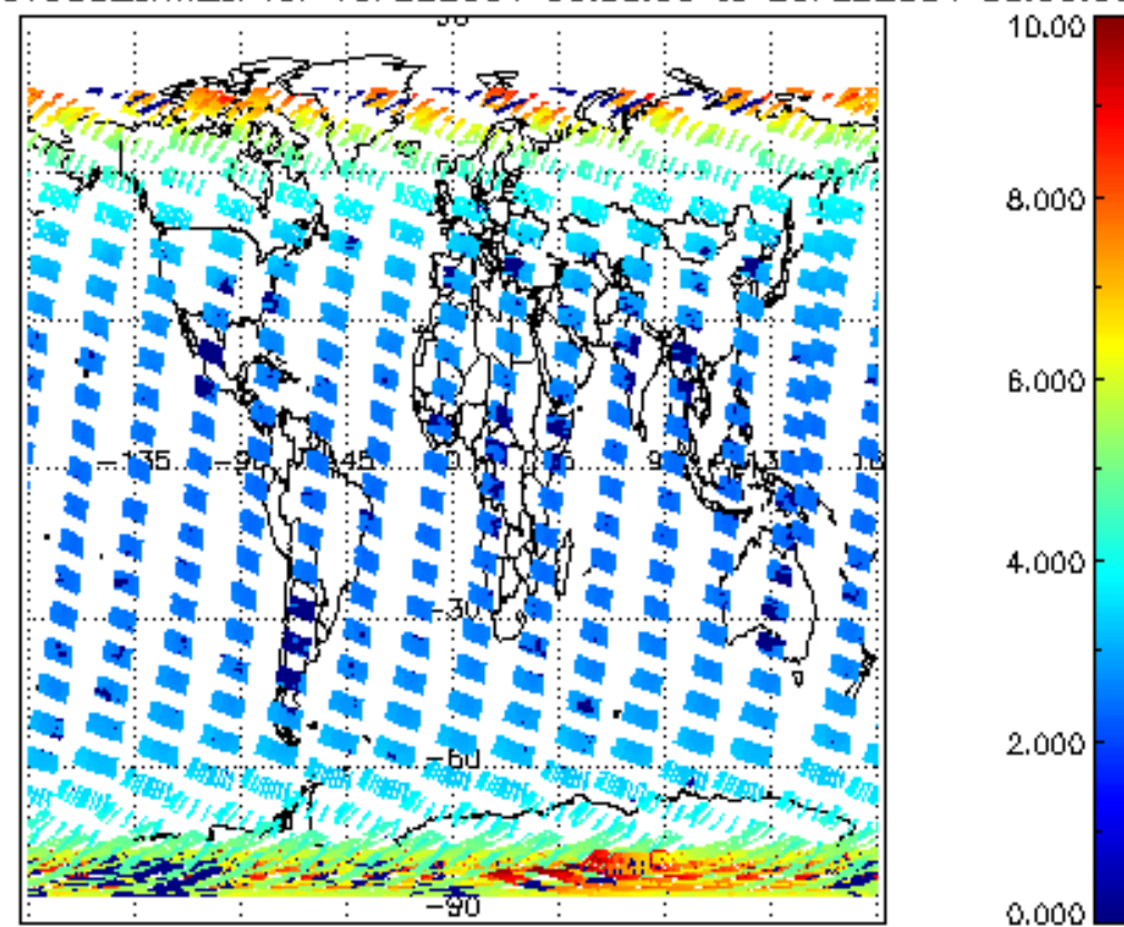
SCIOL2P_NADUV003_amf_cl for 19FEB2004 00:00:00 to 20FEB2004 00:00:00
