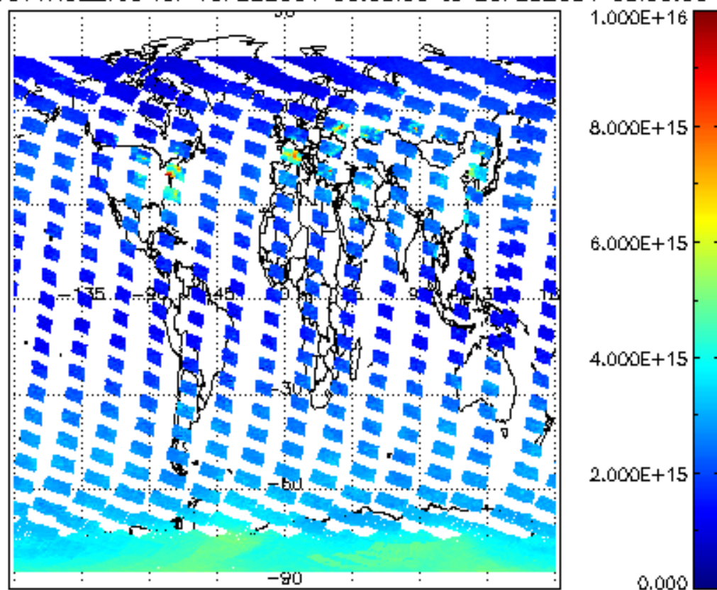
SCIOL2P_NADUV1NO2_vcd for 19FEB2004 00:00:00 to 20FEB2004 00:00:00
