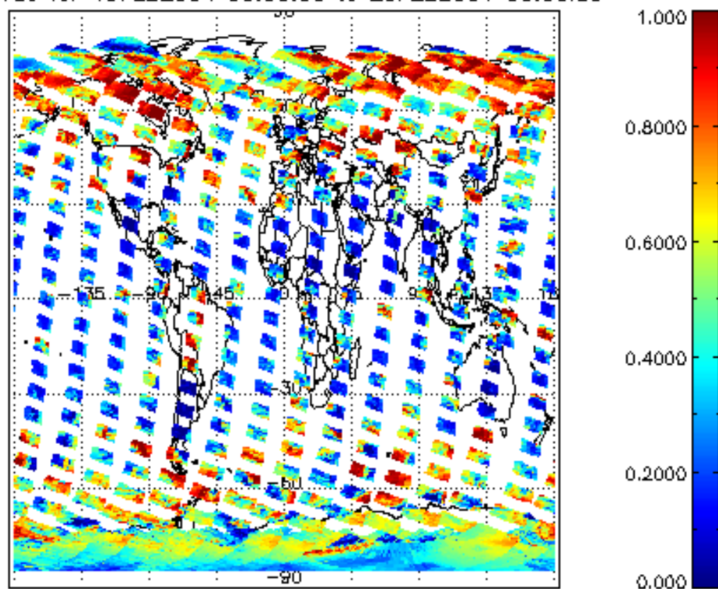
cl_frac for 19FEB2004 00:00:00 to 20FEB2004 00:00:00
