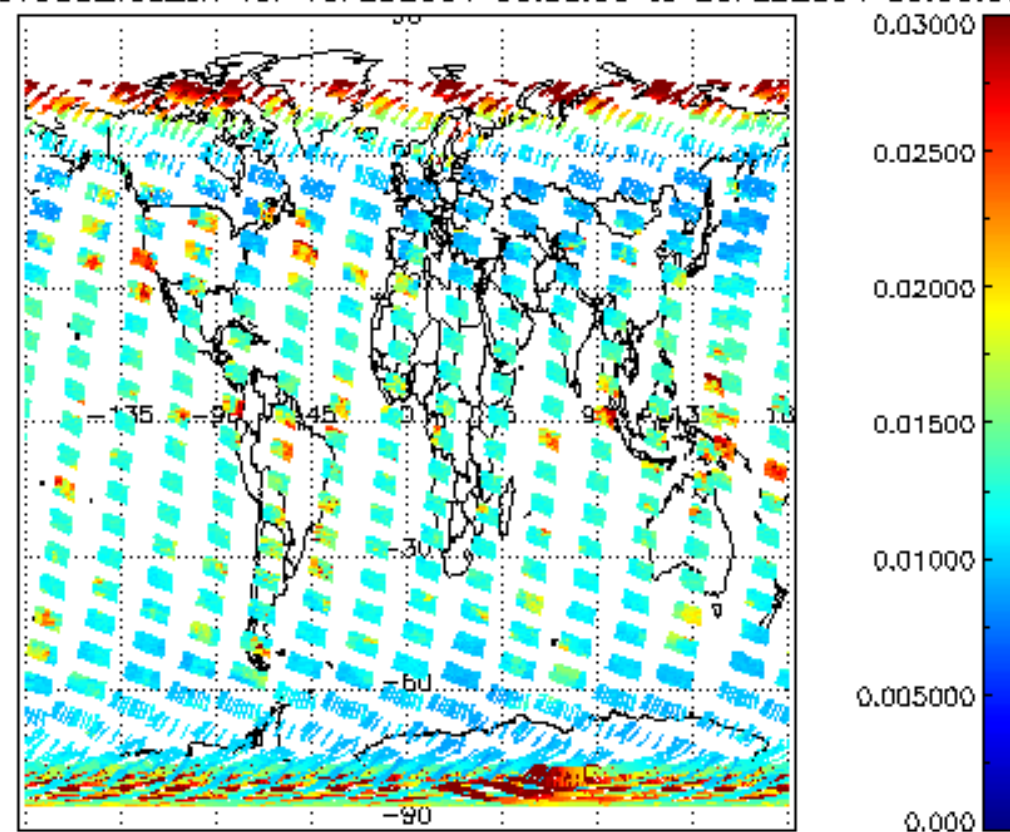
SCIOL2P_NADUV003_vcd_err for 19FEB2004 00:00:00 to 20FEB2004 00:00:00
