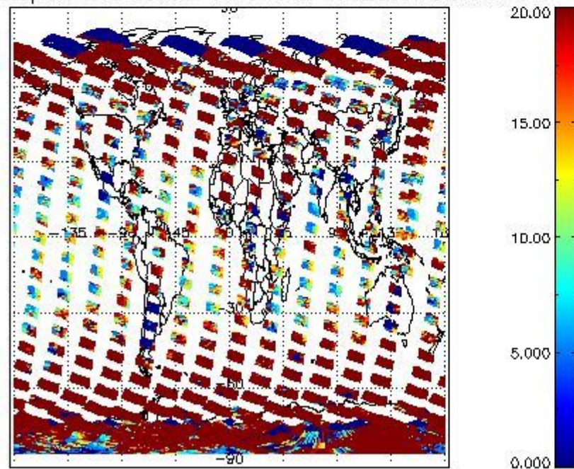
cLopt_depth for 19FEB2004 00:00:00 to 20FEB2004 00:00:00
