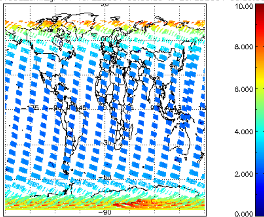
SCIOL2P_NADUV003_amf_gr for 19FEB2004 00:00:00 to 20FEB2004 00:00:00
