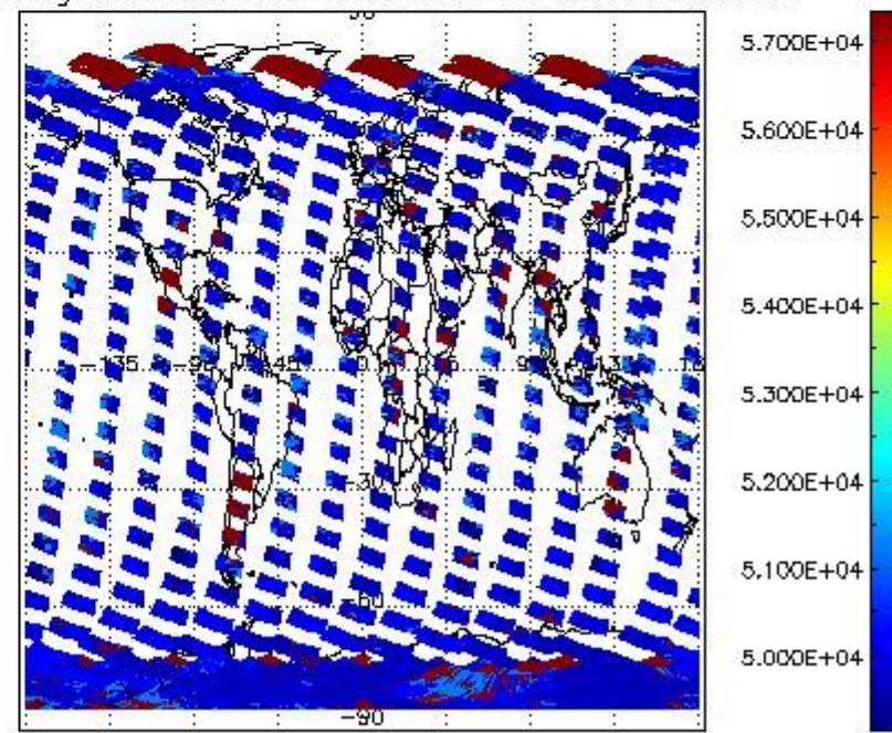
cloud_flags for 19FEB2004 00:00:00 to 20FEB2004 00:00:00
