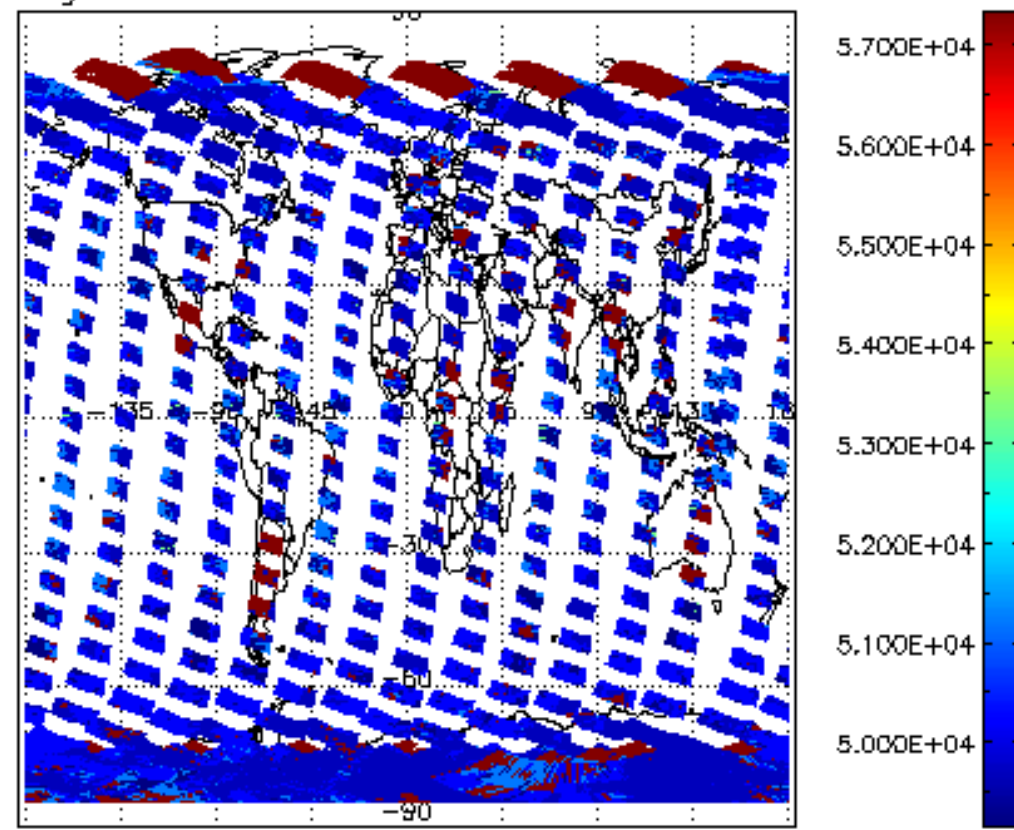
cloud_flags for 19FEB2004 00:00:00 to 20FEB2004 00:00:00
