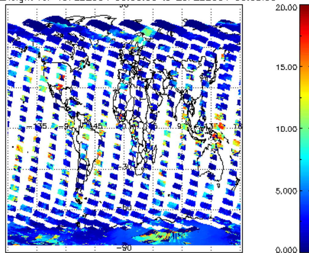
cl_top_height for 19FEB2004 00:00:00 to 20FEB2004 00:00:00
