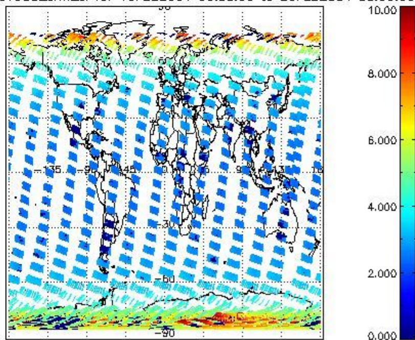
SCIOL2P_NADUV003_amf_cl for 19FEB2004 00:00:00 to 20FEB2004 00:00:00
