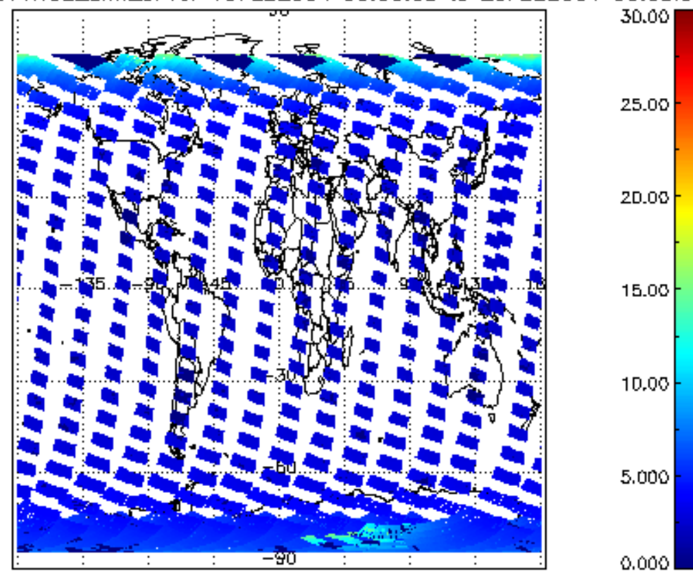
SCIOL2P_NADUV1NO2_amf_cl for 19FEB2004 00:00:00 to 20FEB2004 00:00:00
