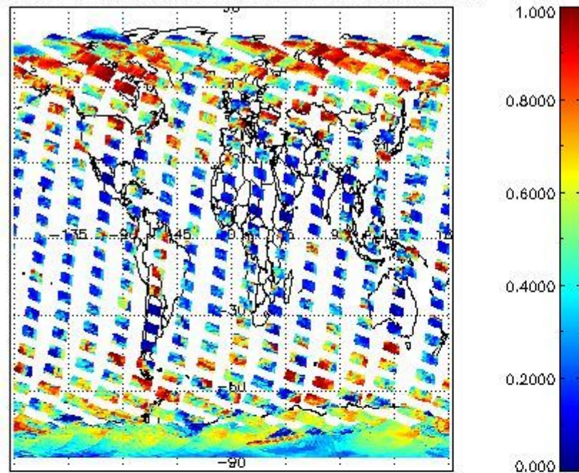
cLfrac for 19FEB2004 00:00:00 to 20FEB2004 00:00:00
