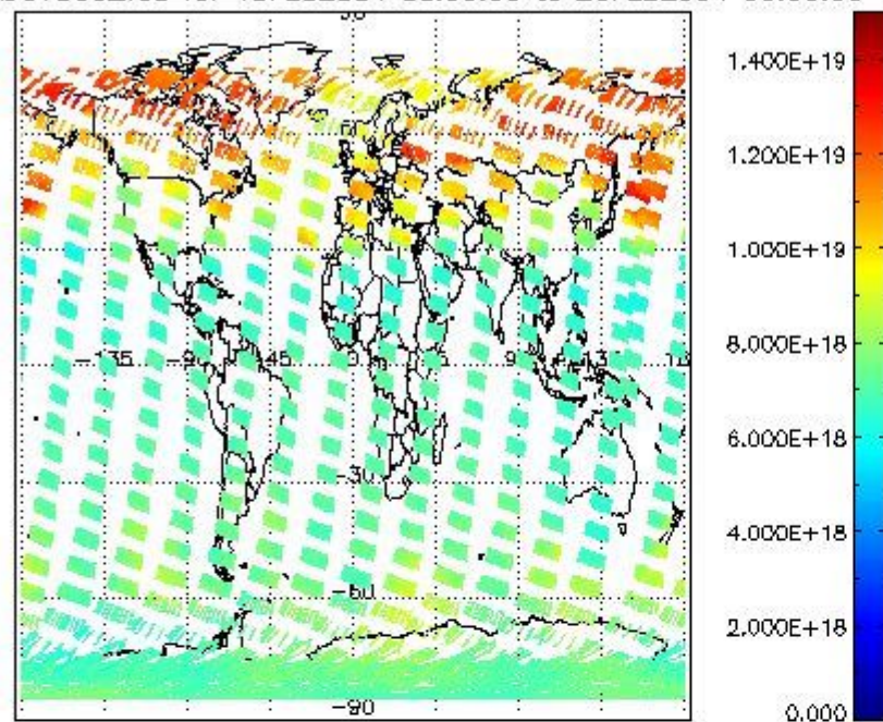
SCIOL2P_NADUV003_vcd for 19FEB2004 00:00:00 to 20FEB2004 00:00:00
