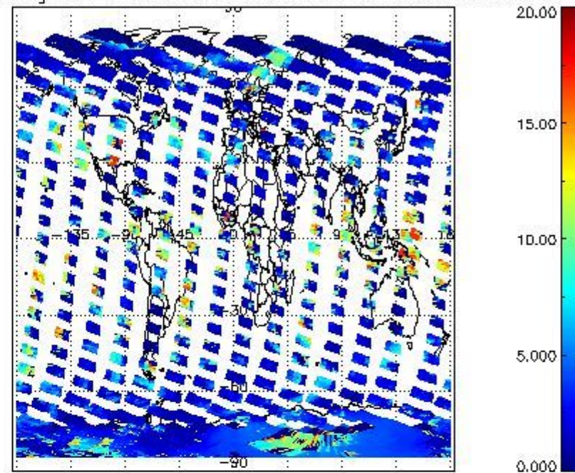
cL_top_height for 19FEB2004 00:00:00 to 20FEB2004 00:00:00
