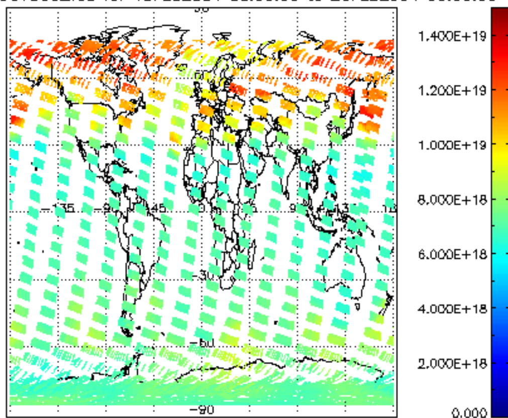
SCIOL2P_NADUV003_vcd for 19FEB2004 00:00:00 to 20FEB2004 00:00:00
