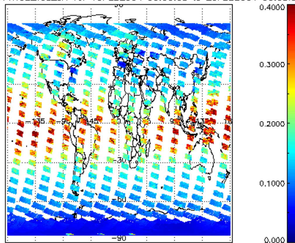
SCIOL2P_NADUV1NO2_vcd_err for 19FEB2004 00:00:00 to 20FEB2004 00:00:00
