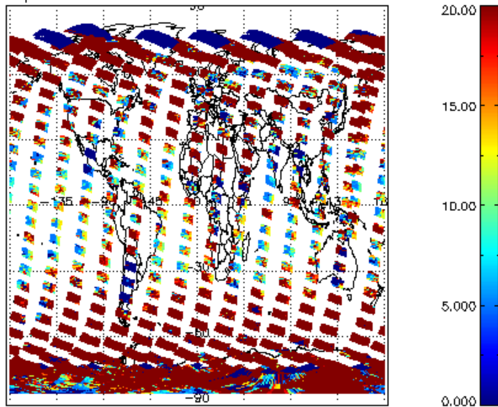
cl_lopt_depth for 19FEB2004 00:00:00 to 20FEB2004 00:00:00
