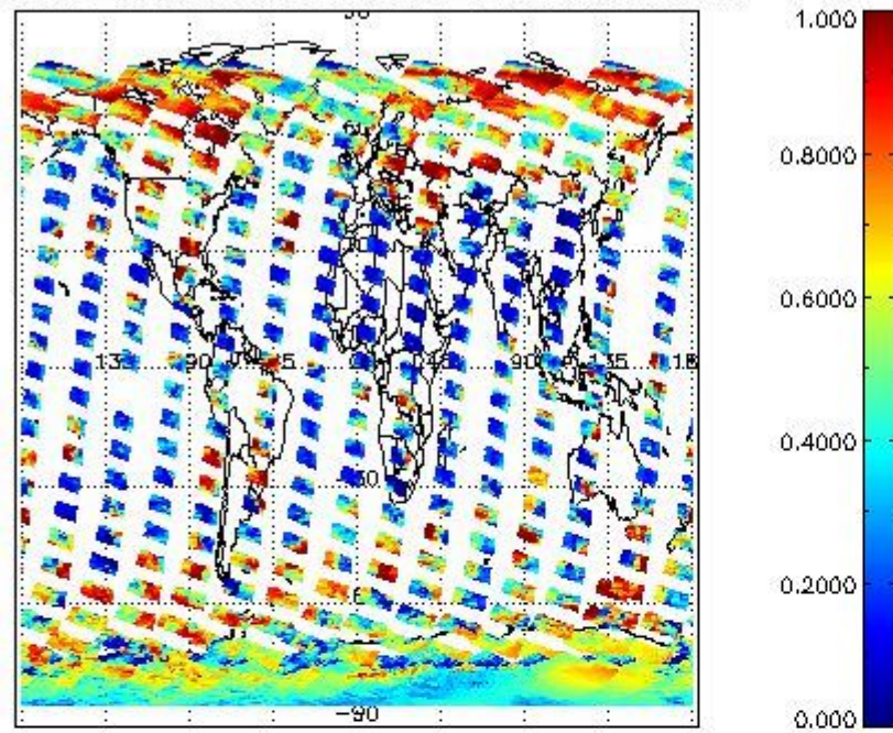
cLfrac for 14FEB2004 00:00:00 to 15FEB2004 00:00:00
