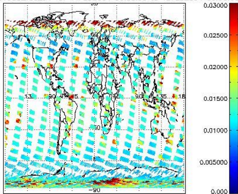
SCIOL2P_NADUV003_vcd_err for 14FEB2004 00:00:00 to 15FEB2004 00:00:00
