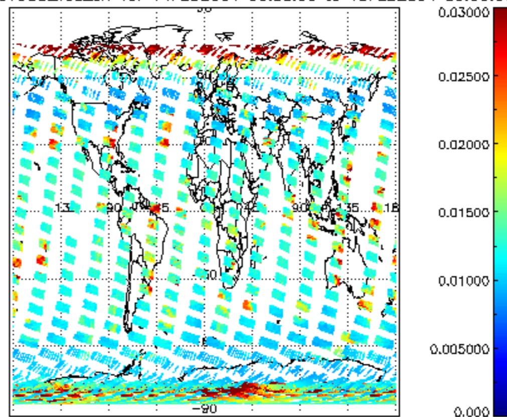
SCIOL2P_NADUV003_vcd_err for 14FEB2004 00:00:00 to 15FEB2004 00:00:00
