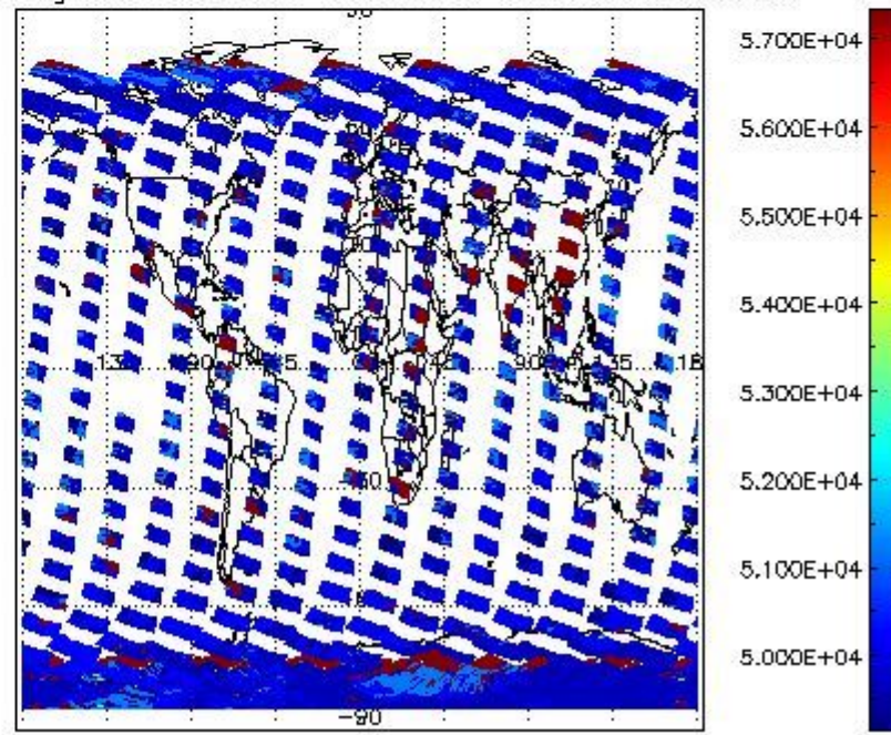
cloud_flags for 14FEB2004 00:00:00 to 15FEB2004 00:00:00
