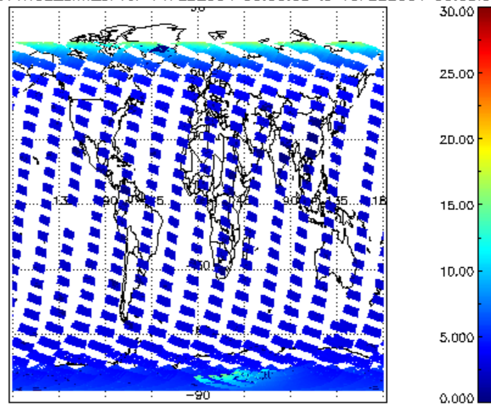
SCIOL2P_NADUV1NO2_amf_cl for 14FEB2004 00:00:00 to 15FEB2004 00:00:00
