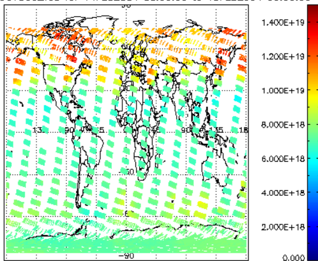
SCIOL2P_NADUV003_vcd for 14FEB2004 00:00:00 to 15FEB2004 00:00:00
