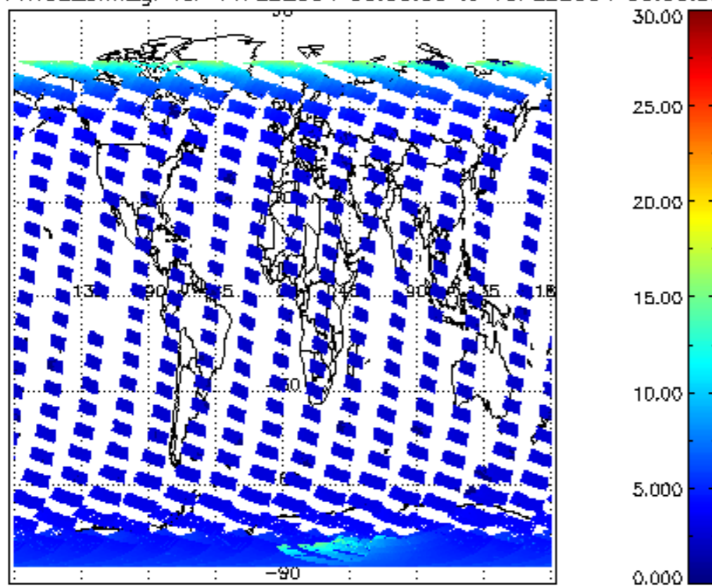
SCIOL2P_NADUV1NO2_amf_gr for 14FEB2004 00:00:00 to 15FEB2004 00:00:00
