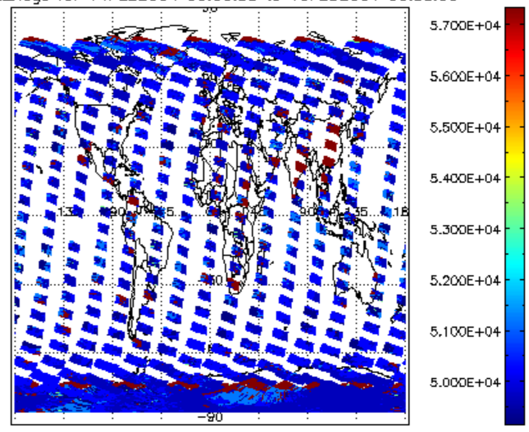
cloud_flags for 14FEB2004 00:00:00 to 15FEB2004 00:00:00
