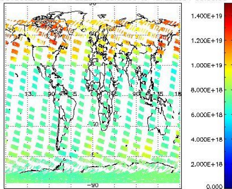
SCIOL2P_NADUV003_vcd for 14FEB2004 00:00:00 to 15FEB2004 00:00:00
