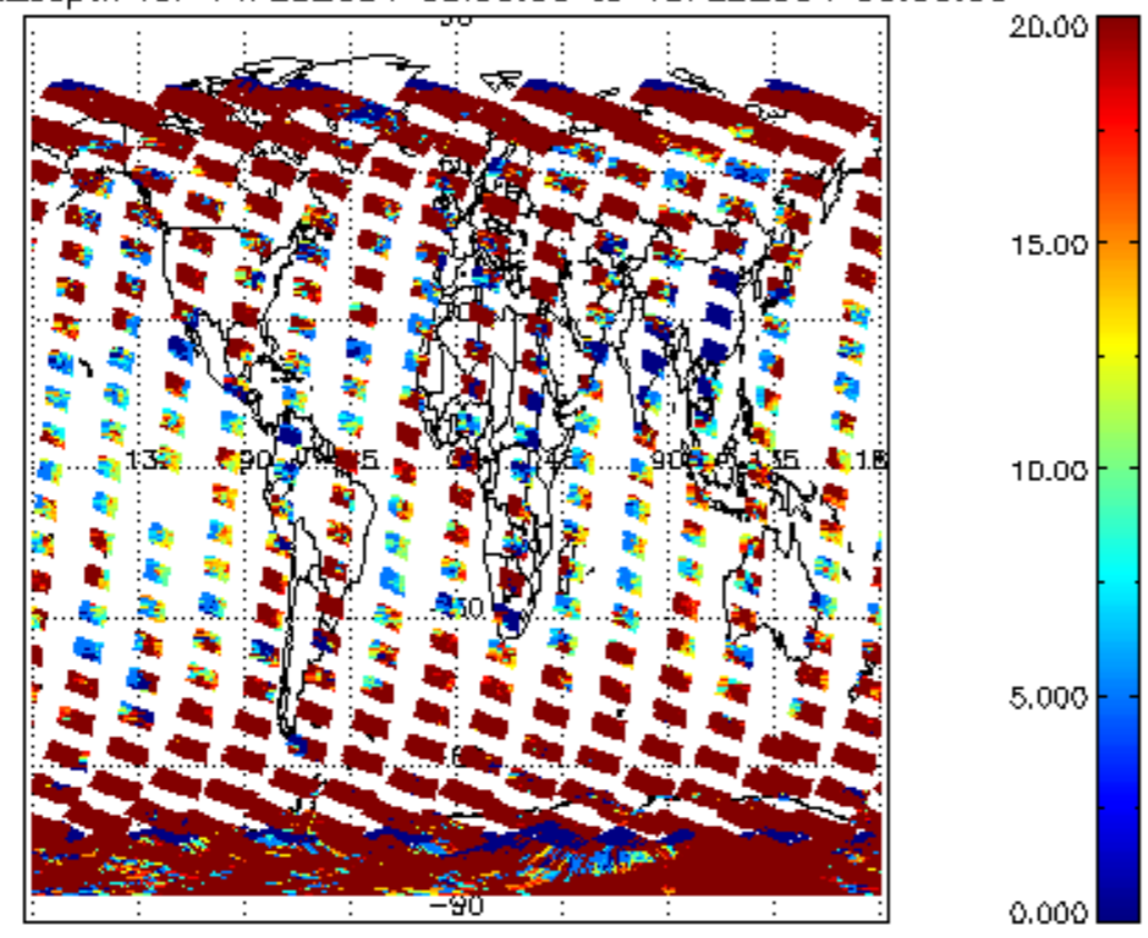
cl_lopt_depth for 14FEB2004 00:00:00 to 15FEB2004 00:00:00
