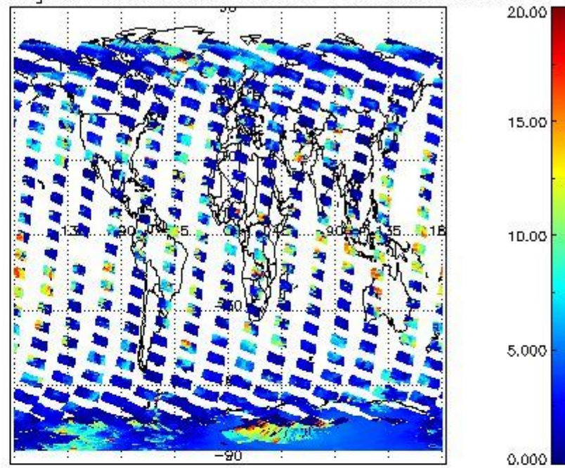
cL_top_height for 14FEB2004 00:00:00 to 15FEB2004 00:00:00
