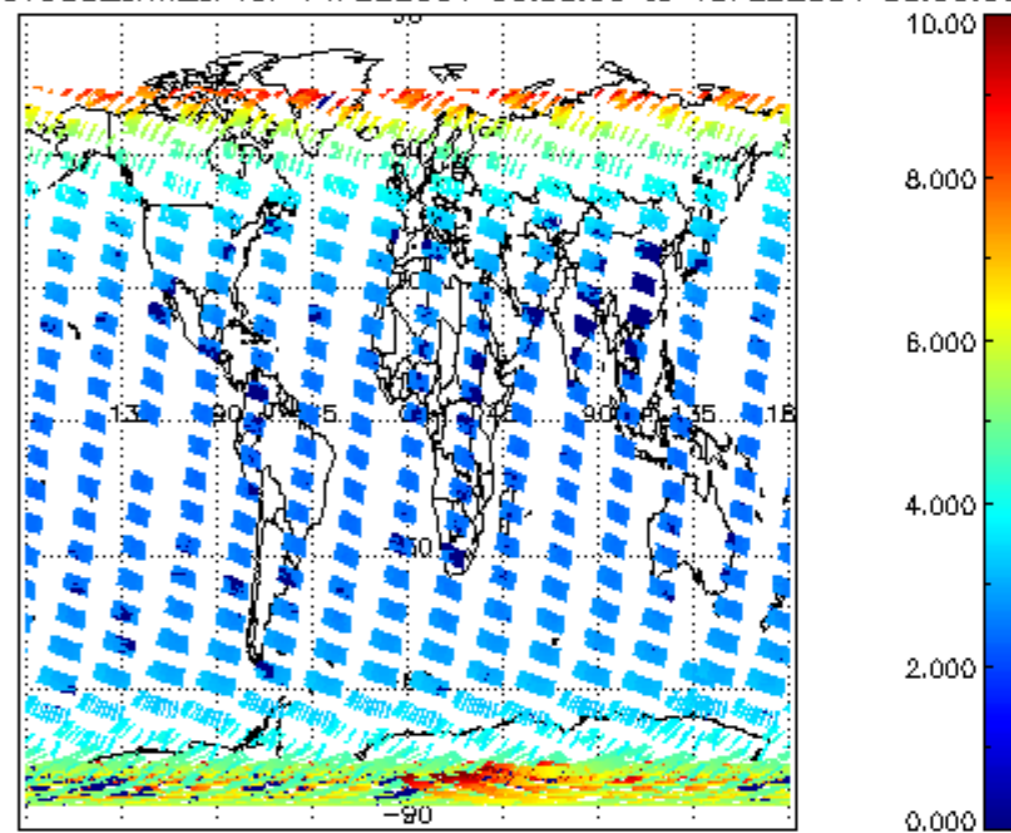
SCIOL2P_NADUV003_amf_cl for 14FEB2004 00:00:00 to 15FEB2004 00:00:00
