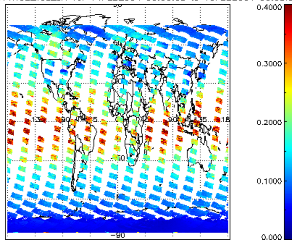
SCIOL2P_NADUV1NO2_vcd_err for 14FEB2004 00:00:00 to 15FEB2004 00:00:00
