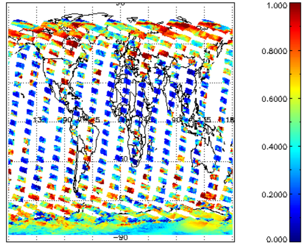
cl_frac for 14FEB2004 00:00:00 to 15FEB2004 00:00:00
