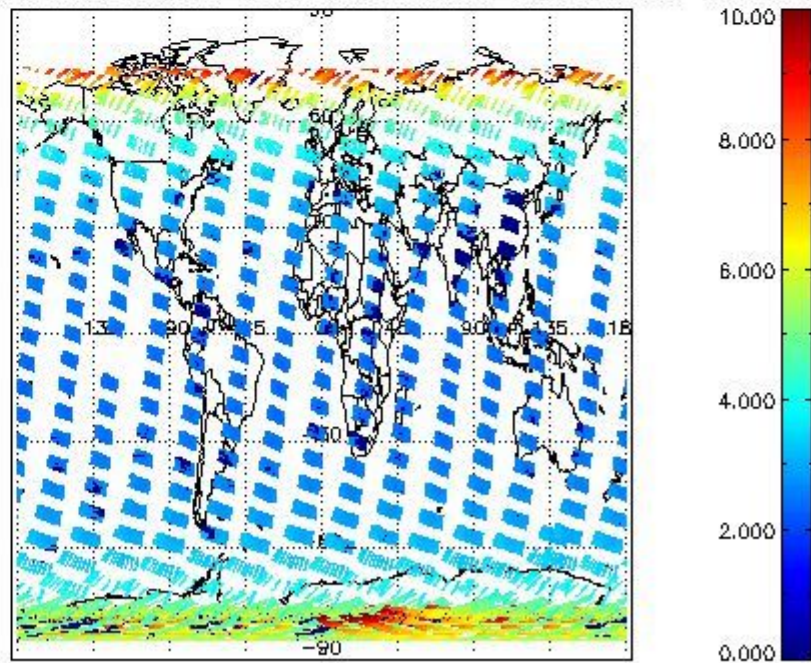
SCIOL2P_NADUV003_amf_cl for 14FEB2004 00:00:00 to 15FEB2004 00:00:00
