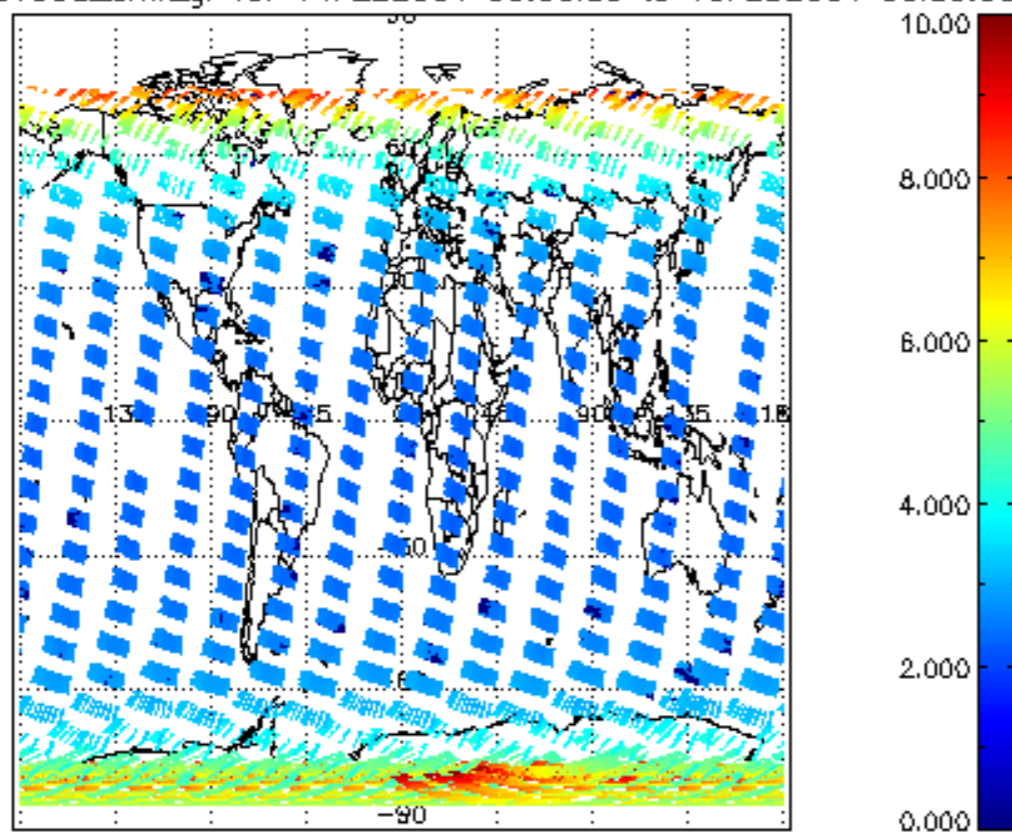
SCIOL2P_NADUV003_amf_gr for 14FEB2004 00:00:00 to 15FEB2004 00:00:00
