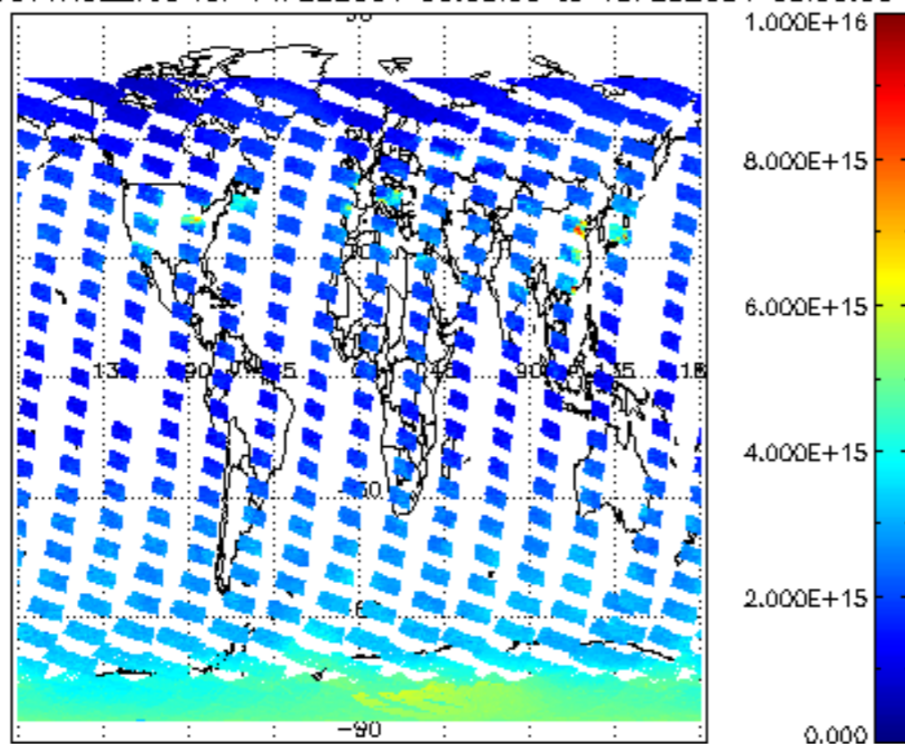
SCIOL2P_NADUV1NO2_vcd for 14FEB2004 00:00:00 to 15FEB2004 00:00:00
