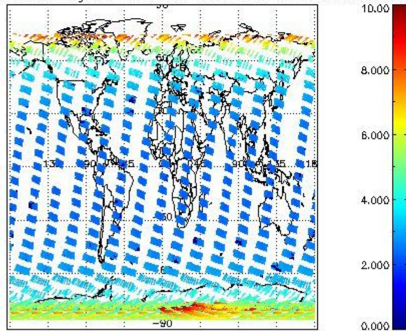
SCIOL2P_NADUV003_amf_gr for 14FEB2004 00:00:00 to 15FEB2004 00:00:00
