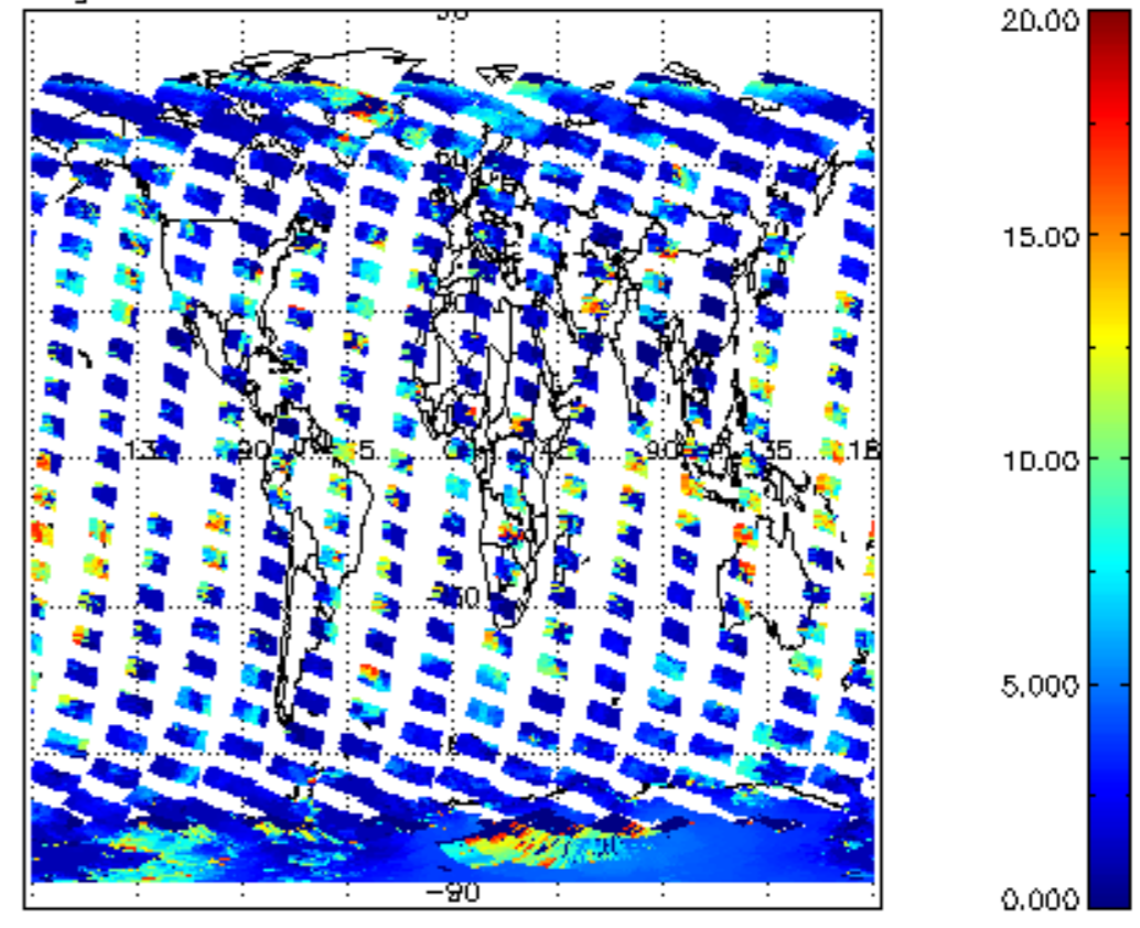
cl_top_height for 14FEB2004 00:00:00 to 15FEB2004 00:00:00
