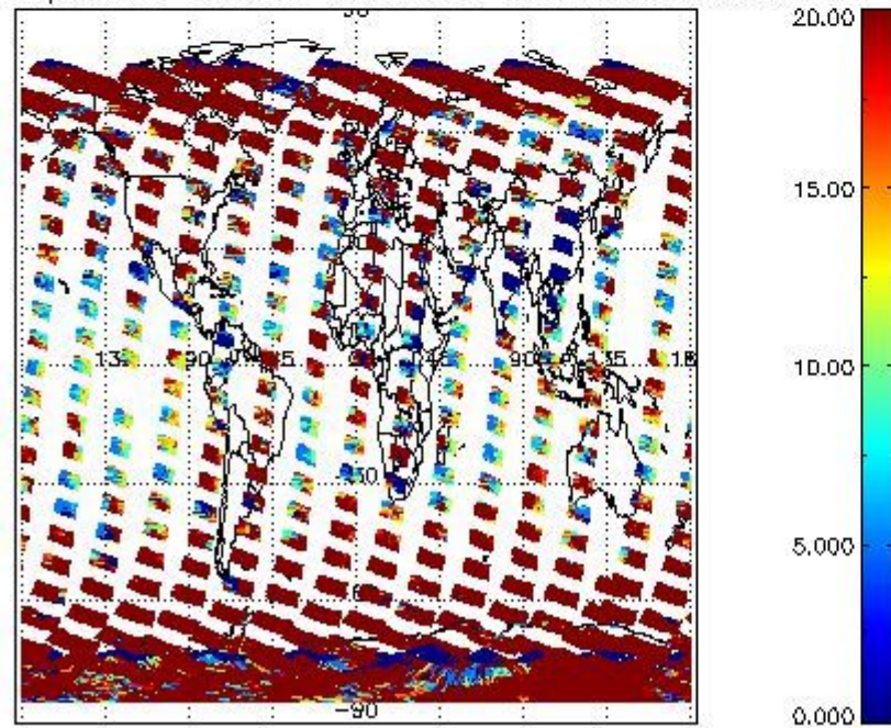
cLopt_depth for 14FEB2004 00:00:00 to 15FEB2004 00:00:00
