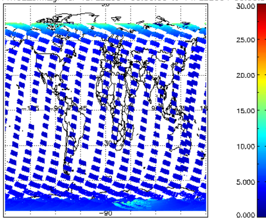
SCIOL2P_NADUV1NO2_amf_gr for 13FEB2004 00:00:00 to 14FEB2004 00:00:00
