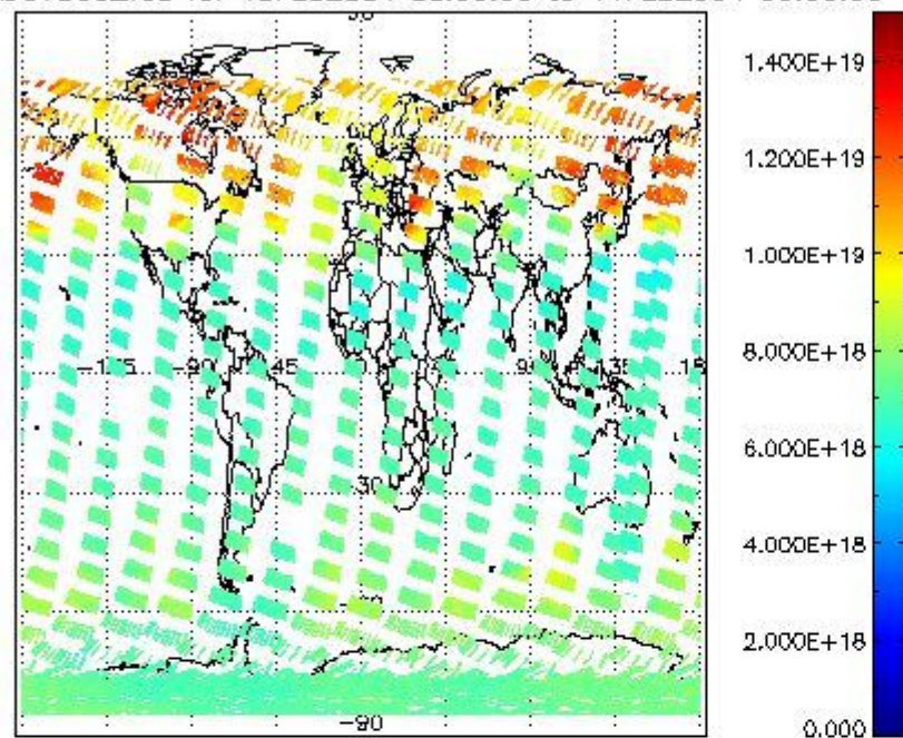
SCIOL2P_NADUV003_vcd for 13FEB2004 00:00:00 to 14FEB2004 00:00:00
