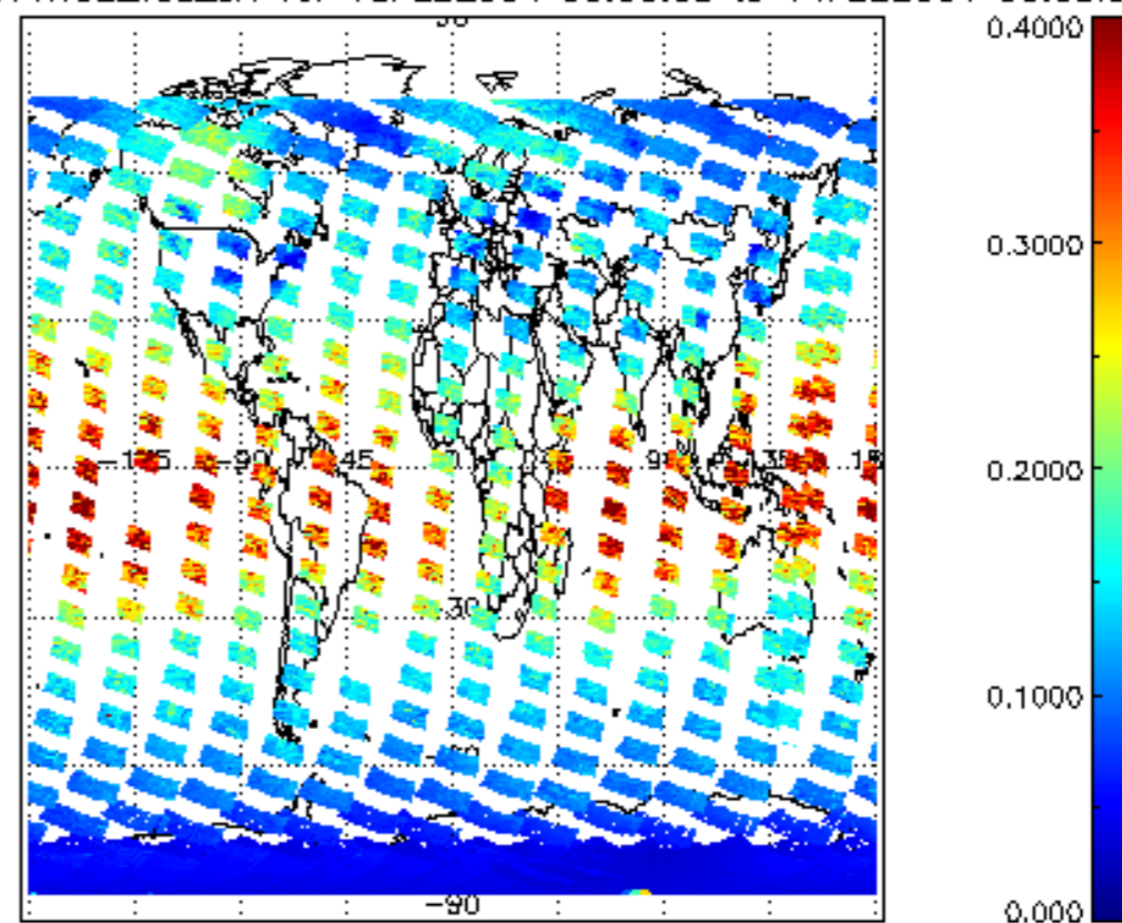
SCIOL2P_NADUV1NO2_vcd_err for 13FEB2004 00:00:00 to 14FEB2004 00:00:00
