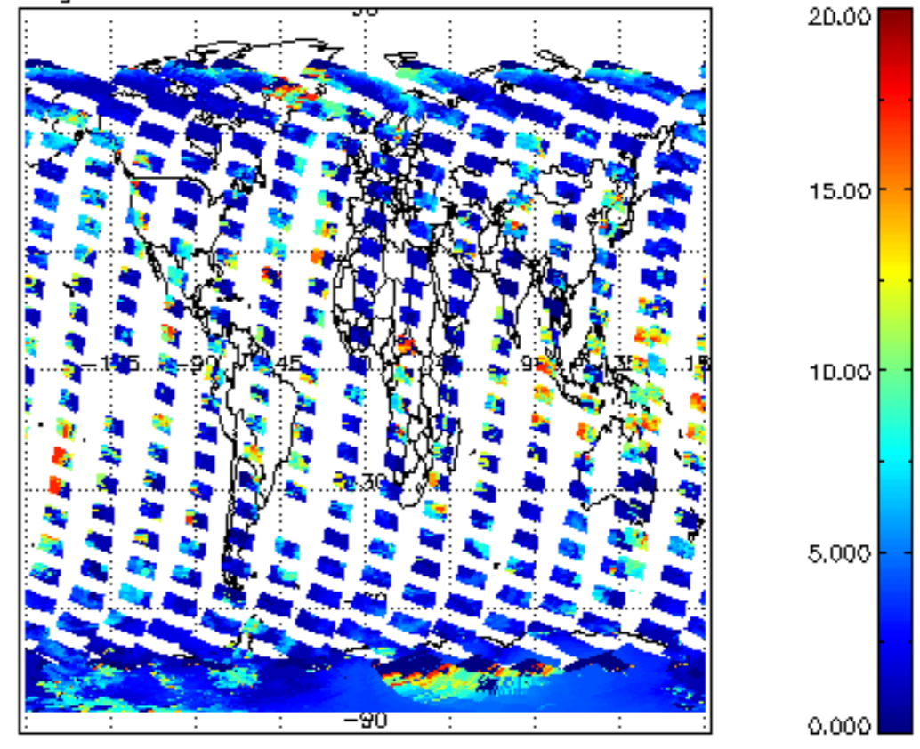
cI_top_height for 13FEB2004 00:00:00 to 14FEB2004 00:00:00
