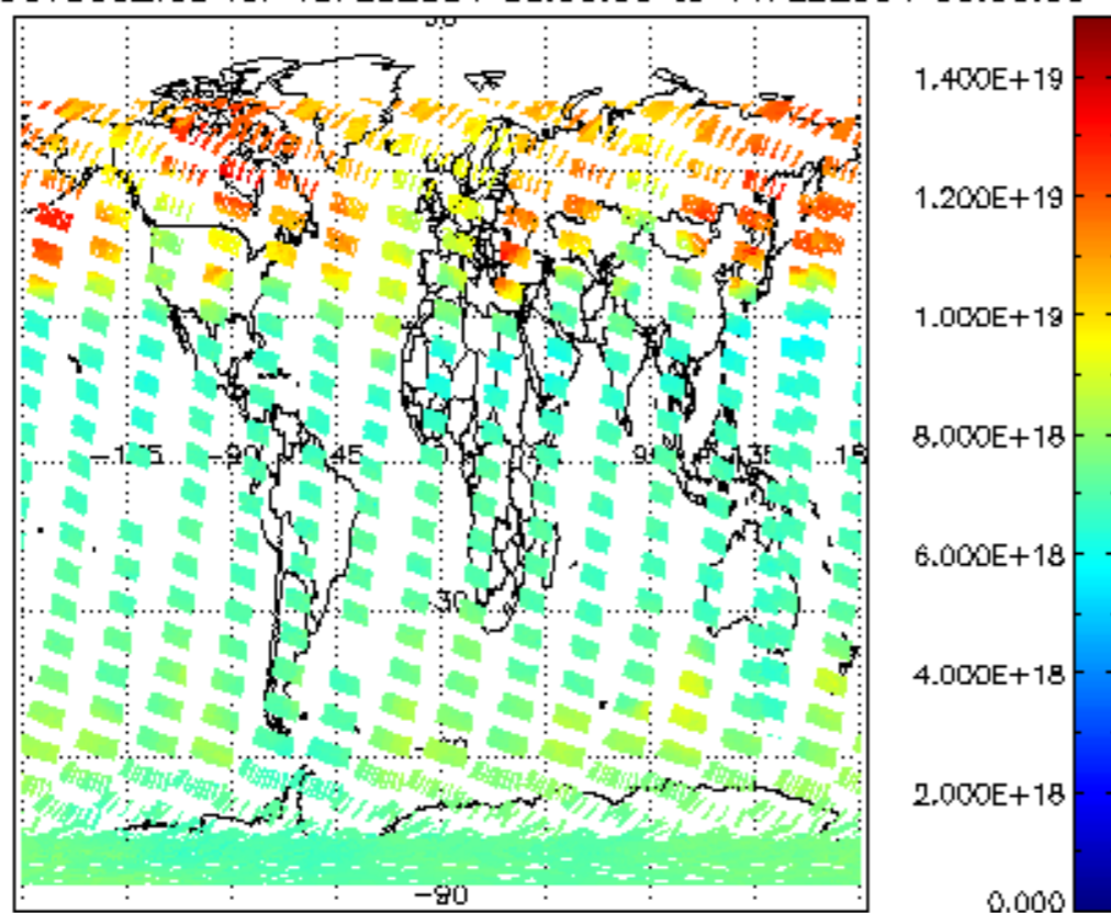
SCIOL2P_NADUV003_vcd for 13FEB2004 00:00:00 to 14FEB2004 00:00:00
