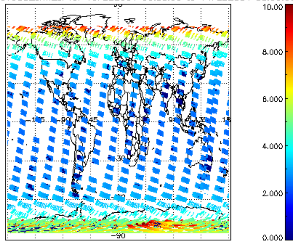
SCIOL2P_NADUV003_amf_cl for 13FEB2004 00:00:00 to 14FEB2004 00:00:00
