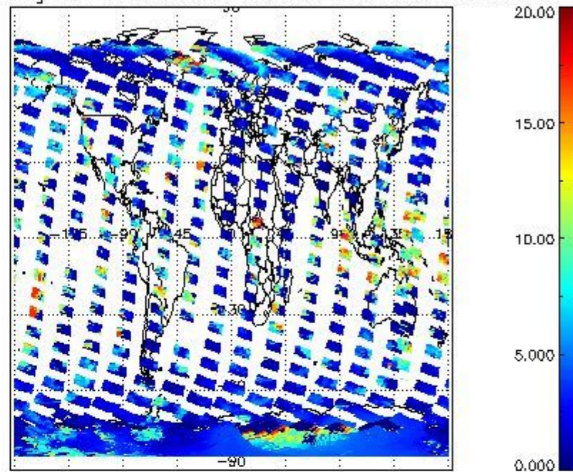
cL_top_height for 13FEB2004 00:00:00 to 14FEB2004 00:00:00
