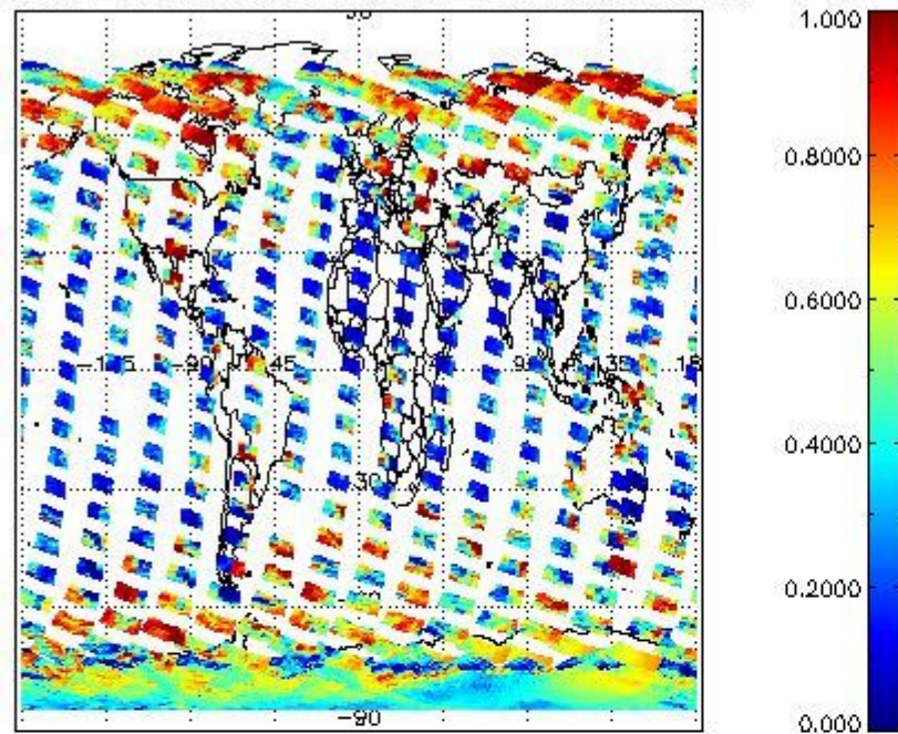
cL_frac for 13FEB2004 00:00:00 to 14FEB2004 00:00:00
