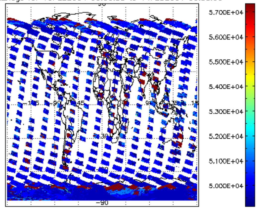
cloud_flags for 13FEB2004 00:00:00 to 14FEB2004 00:00:00
