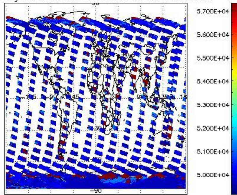
cloud_flags for 13FEB2004 00:00:00 to 14FEB2004 00:00:00
