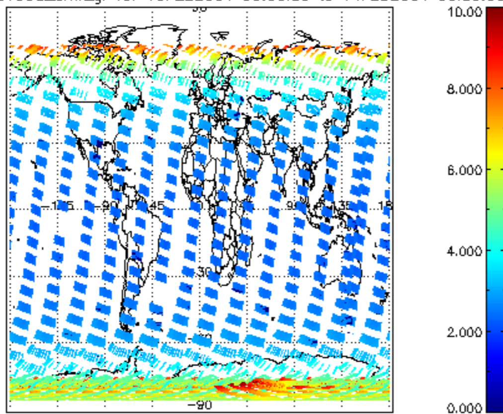
SCIOL2P_NADUV003_amf_gr for 13FEB2004 00:00:00 to 14FEB2004 00:00:00
