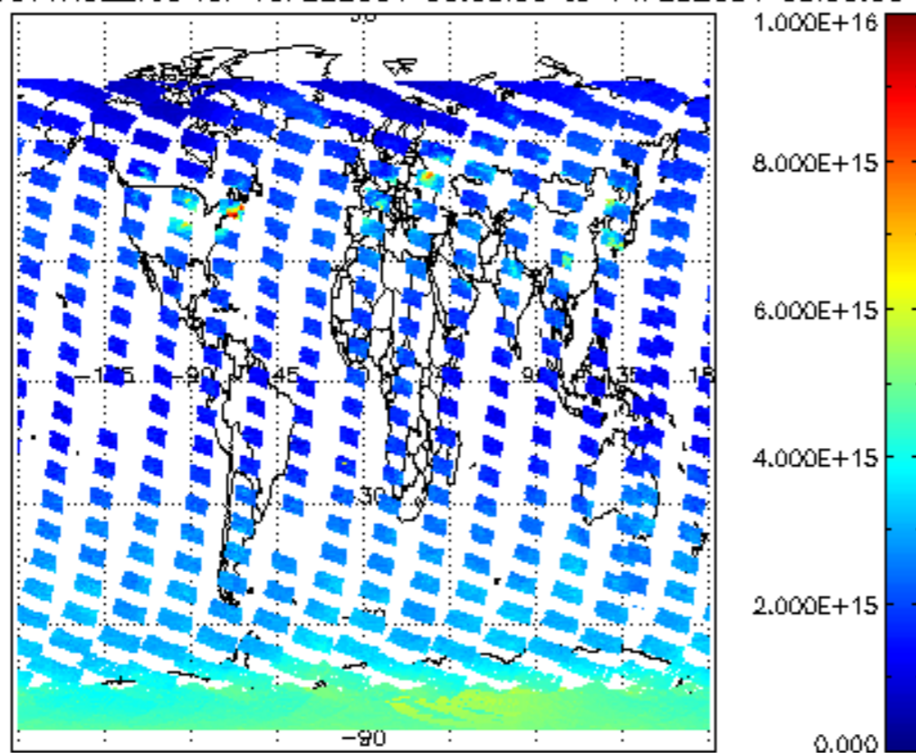
SCIOL2P_NADUV1NO2_vcd for 13FEB2004 00:00:00 to 14FEB2004 00:00:00
