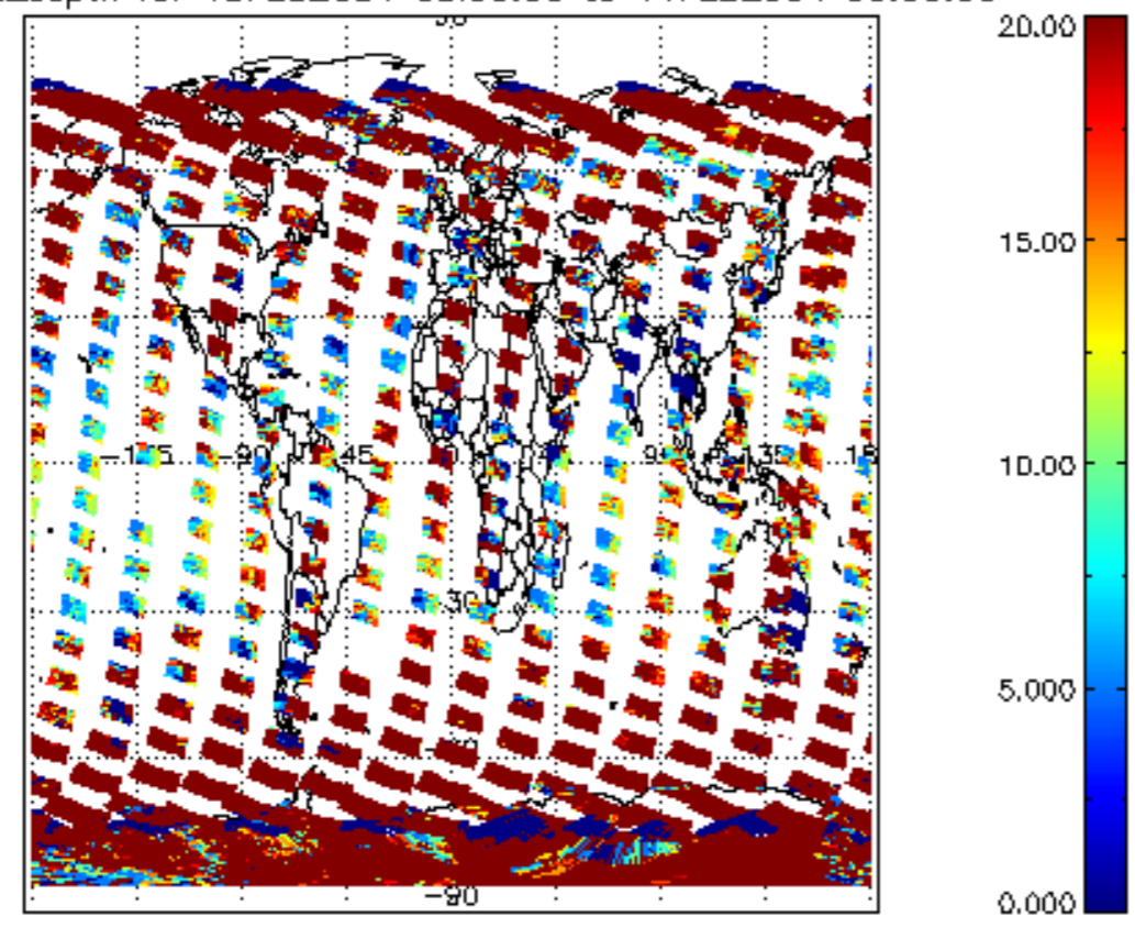
cI_opt_depth for 13FEB2004 00:00:00 to 14FEB2004 00:00:00
