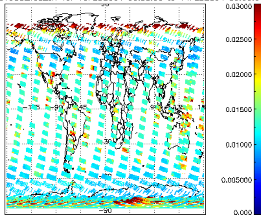
SCIOL2P_NADUV003_vcd_err for 13FEB2004 00:00:00 to 14FEB2004 00:00:00
