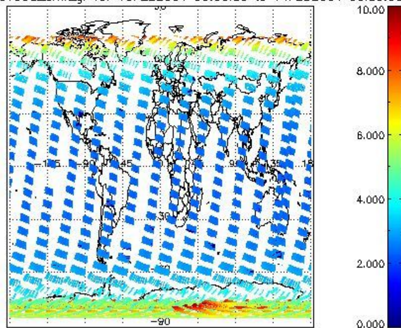
SCIOL2P_NADUV003_amf_gr for 13FEB2004 00:00:00 to 14FEB2004 00:00:00
