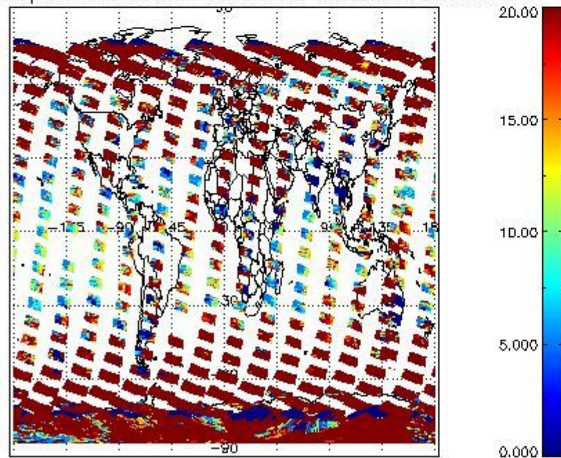
cL_opt_depth for 13FEB2004 00:00:00 to 14FEB2004 00:00:00
