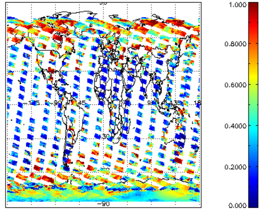
cI_frac for 13FEB2004 00:00:00 to 14FEB2004 00:00:00
