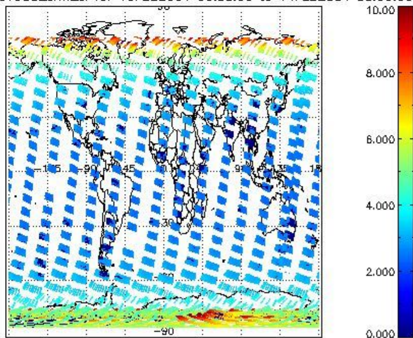
SCIOL2P_NADUV003_amf_cl for 13FEB2004 00:00:00 to 14FEB2004 00:00:00
