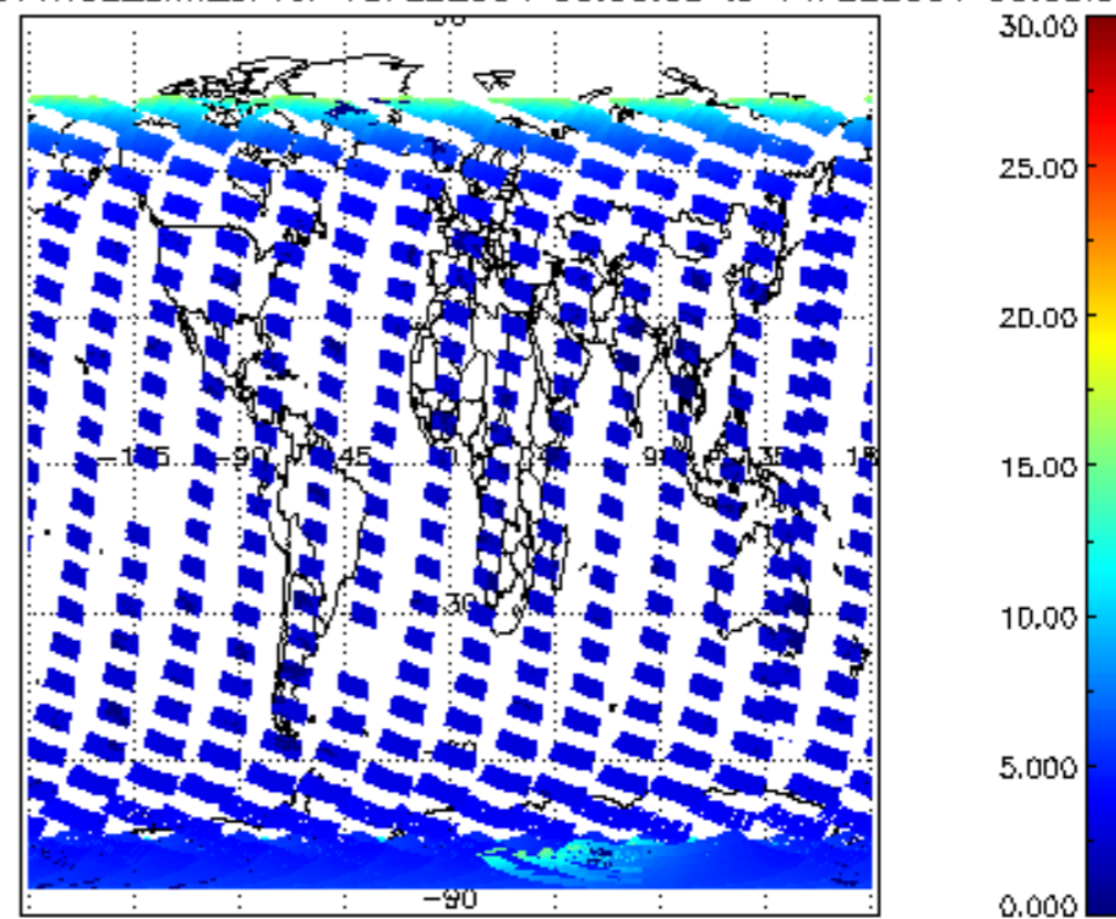
SCIOL2P_NADUV1NO2_amf_cl for 13FEB2004 00:00:00 to 14FEB2004 00:00:00
