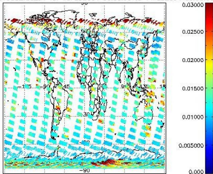
SCIOL2P_NADUV003_vcd_err for 13FEB2004 00:00:00 to 14FEB2004 00:00:00
