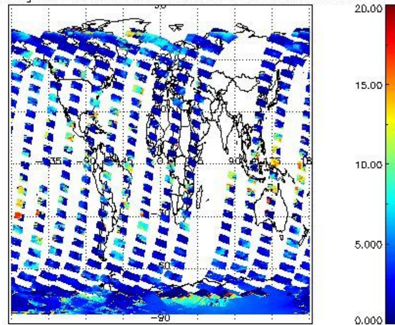
cL_top_height for 12FEB2004 00:00:00 to 13FEB2004 00:00:00
