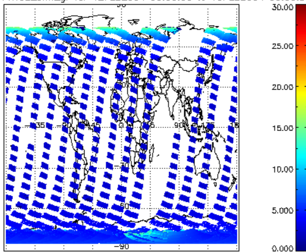
SCIOL2P_NADUV1NO2_amf_gr for 12FEB2004 00:00:00 to 13FEB2004 00:00:00
