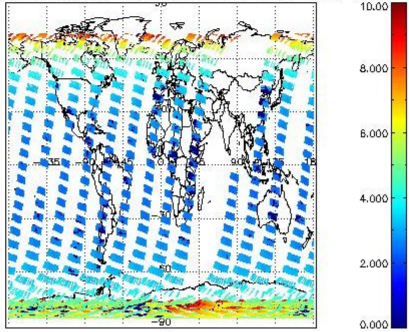
SCIOL2P_NADUV003_amf_cl for 12FEB2004 00:00:00 to 13FEB2004 00:00:00
