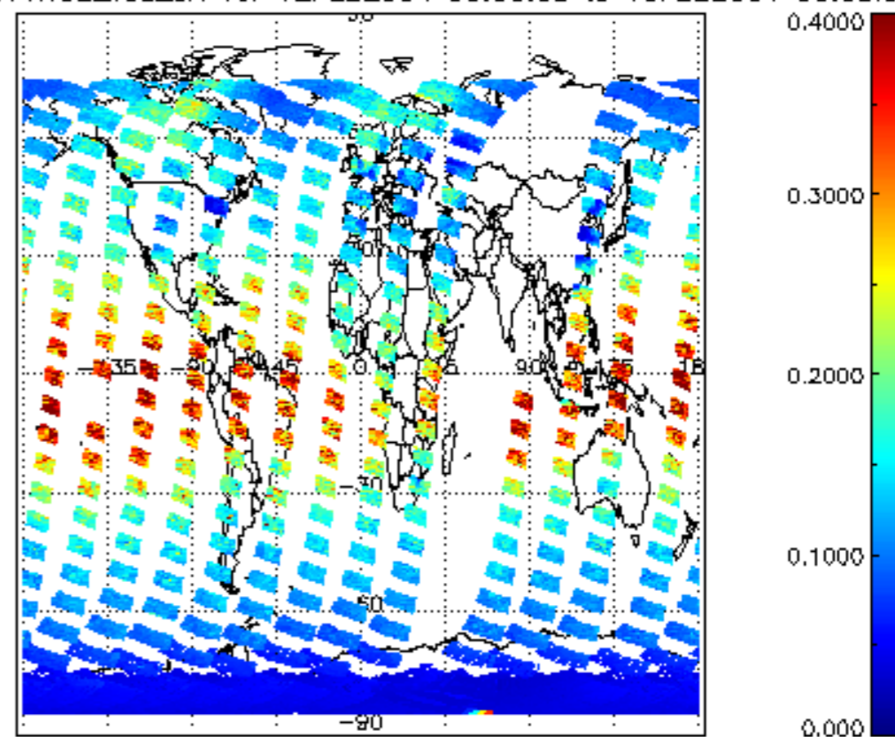
SCIOL2P_NADUV1NO2_vcd_err for 12FEB2004 00:00:00 to 13FEB2004 00:00:00
