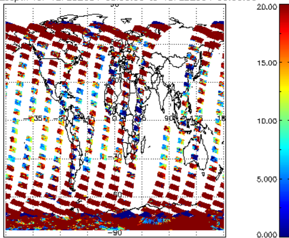
cl_lopt_depth for 12FEB2004 00:00:00 to 13FEB2004 00:00:00
