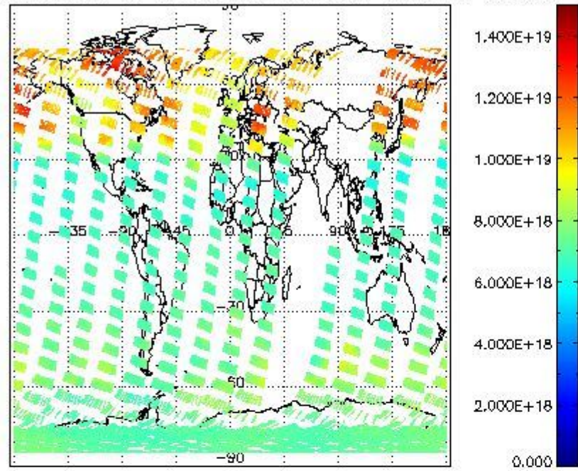
SCIOL2P_NADUV003_vcd for 12FEB2004 00:00:00 to 13FEB2004 00:00:00
