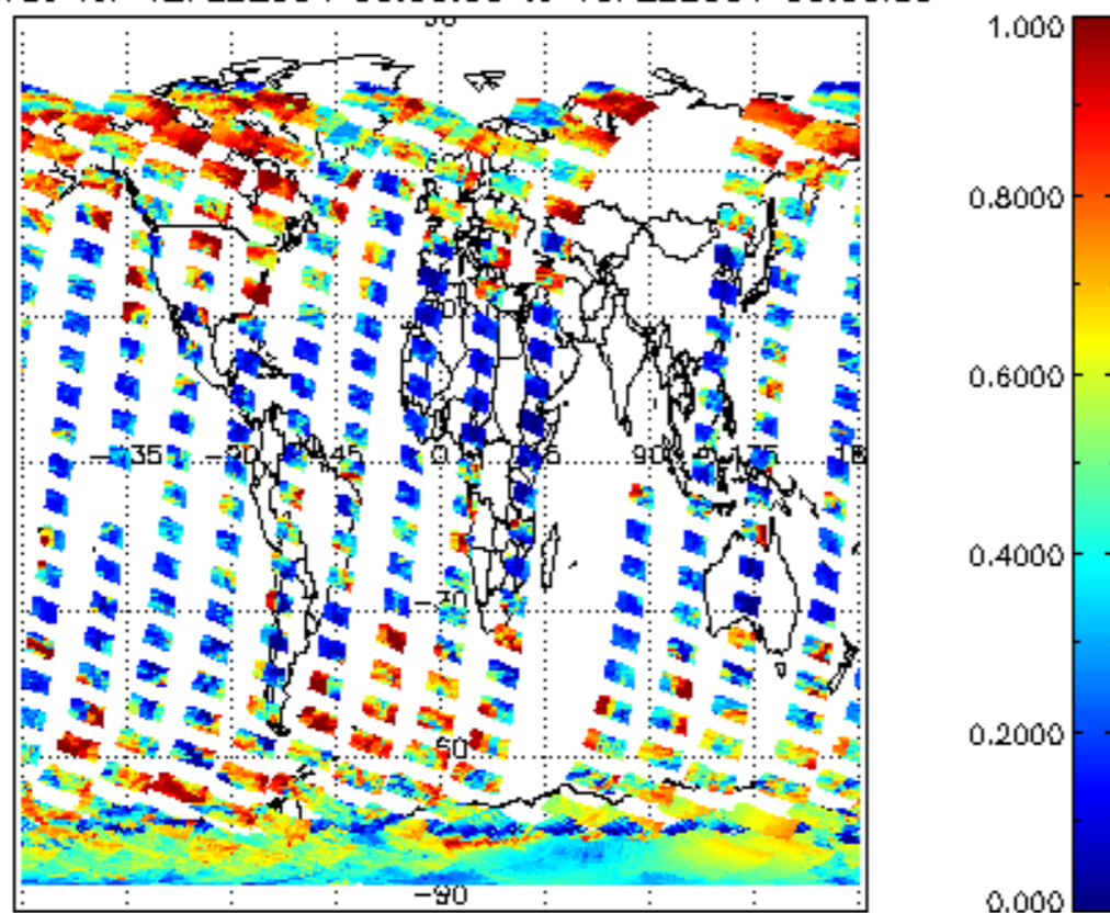
cl_frac for 12FEB2004 00:00:00 to 13FEB2004 00:00:00
