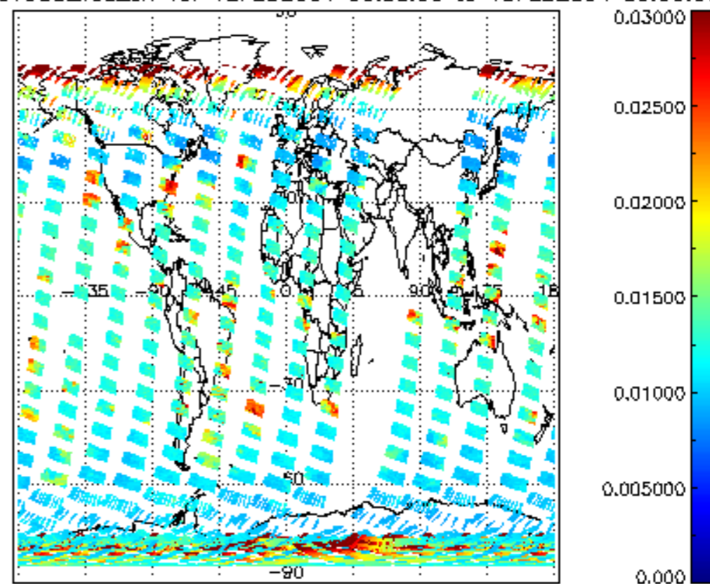
SCIOL2P_NADUV003_vcd_err for 12FEB2004 00:00:00 to 13FEB2004 00:00:00
