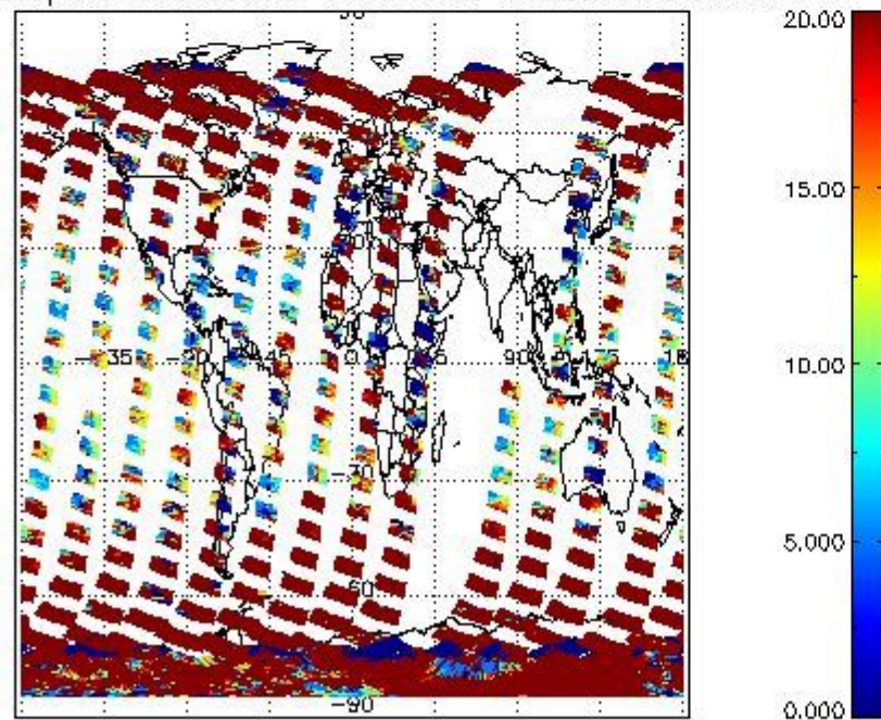
cLopt_depth for 12FEB2004 00:00:00 to 13FEB2004 00:00:00
