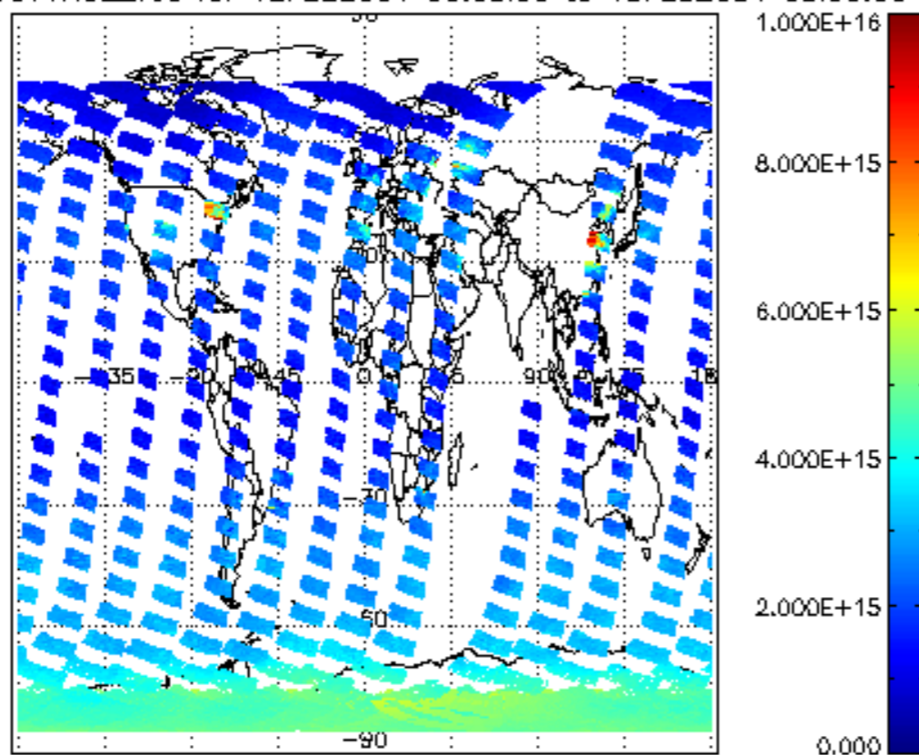
SCIOL2P_NADUV1NO2_vcd for 12FEB2004 00:00:00 to 13FEB2004 00:00:00
