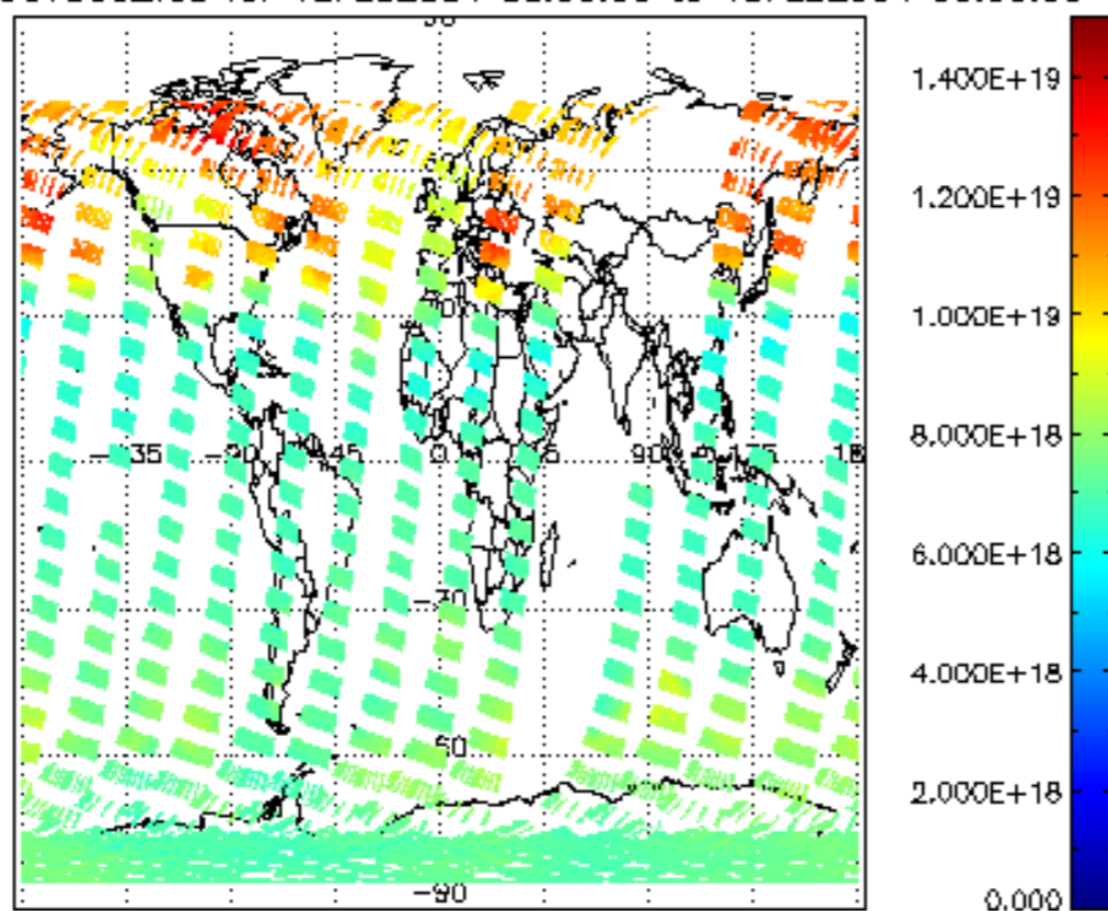
SCIOL2P_NADUV003_vcd for 12FEB2004 00:00:00 to 13FEB2004 00:00:00
