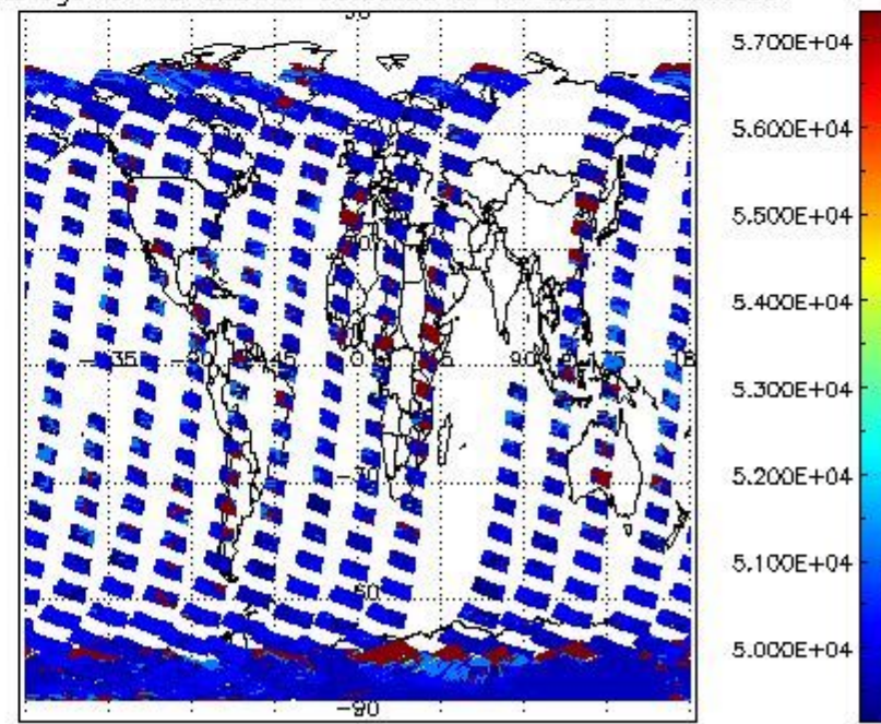
cloud_flags for 12FEB2004 00:00:00 to 13FEB2004 00:00:00
