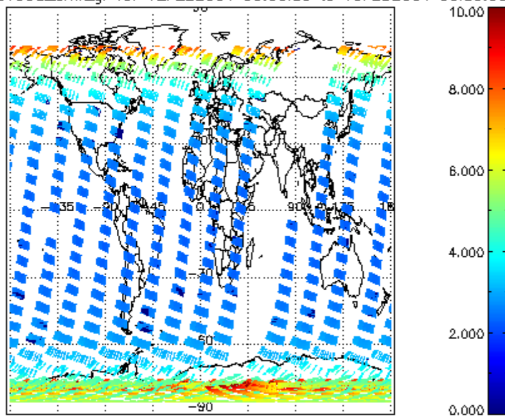
SCIOL2P_NADUV003_amf_gr for 12FEB2004 00:00:00 to 13FEB2004 00:00:00
