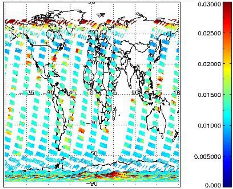
SCIOL2P_NADUV003_vcd_err for 12FEB2004 00:00:00 to 13FEB2004 00:00:00
