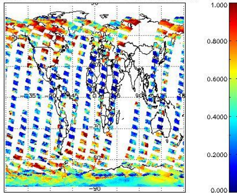
cLfrac for 12FEB2004 00:00:00 to 13FEB2004 00:00:00
