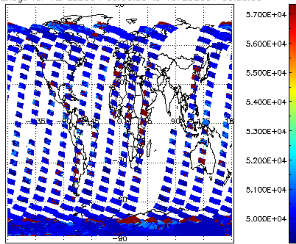
cloud_flags for 12FEB2004 00:00:00 to 13FEB2004 00:00:00
