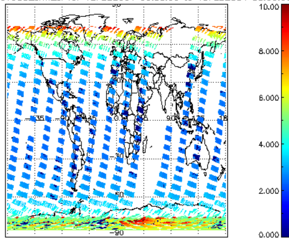
SCIOL2P_NADUV003_amf_cl for 12FEB2004 00:00:00 to 13FEB2004 00:00:00
