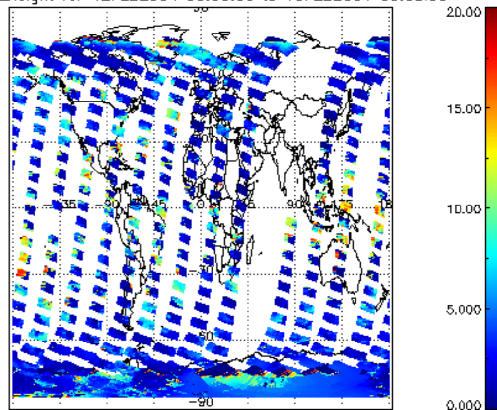
cl_top_height for 12FEB2004 00:00:00 to 13FEB2004 00:00:00
