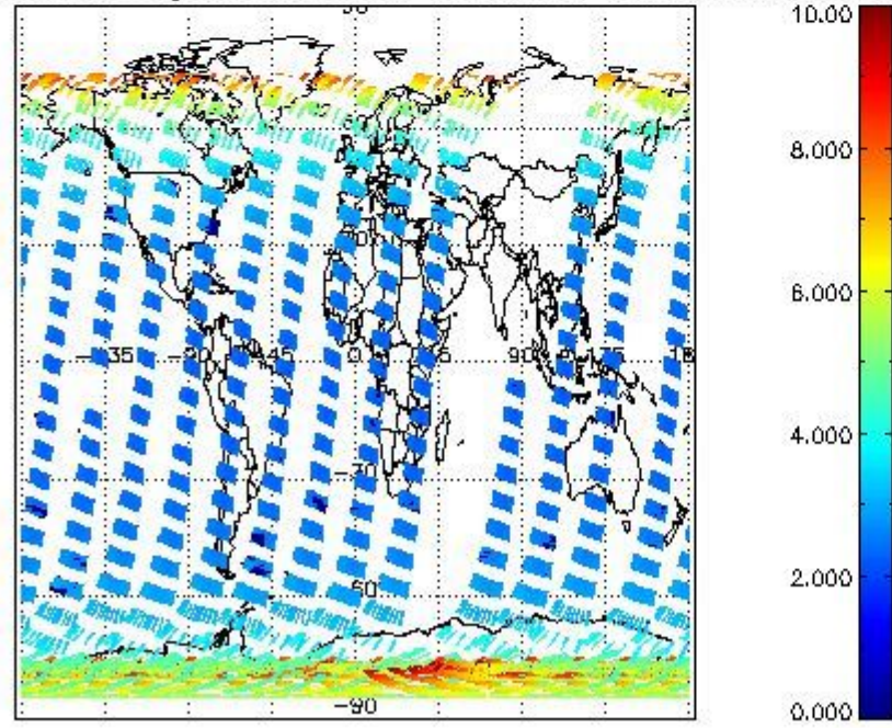
SCIOL2P_NADUV003_amf_gr for 12FEB2004 00:00:00 to 13FEB2004 00:00:00
