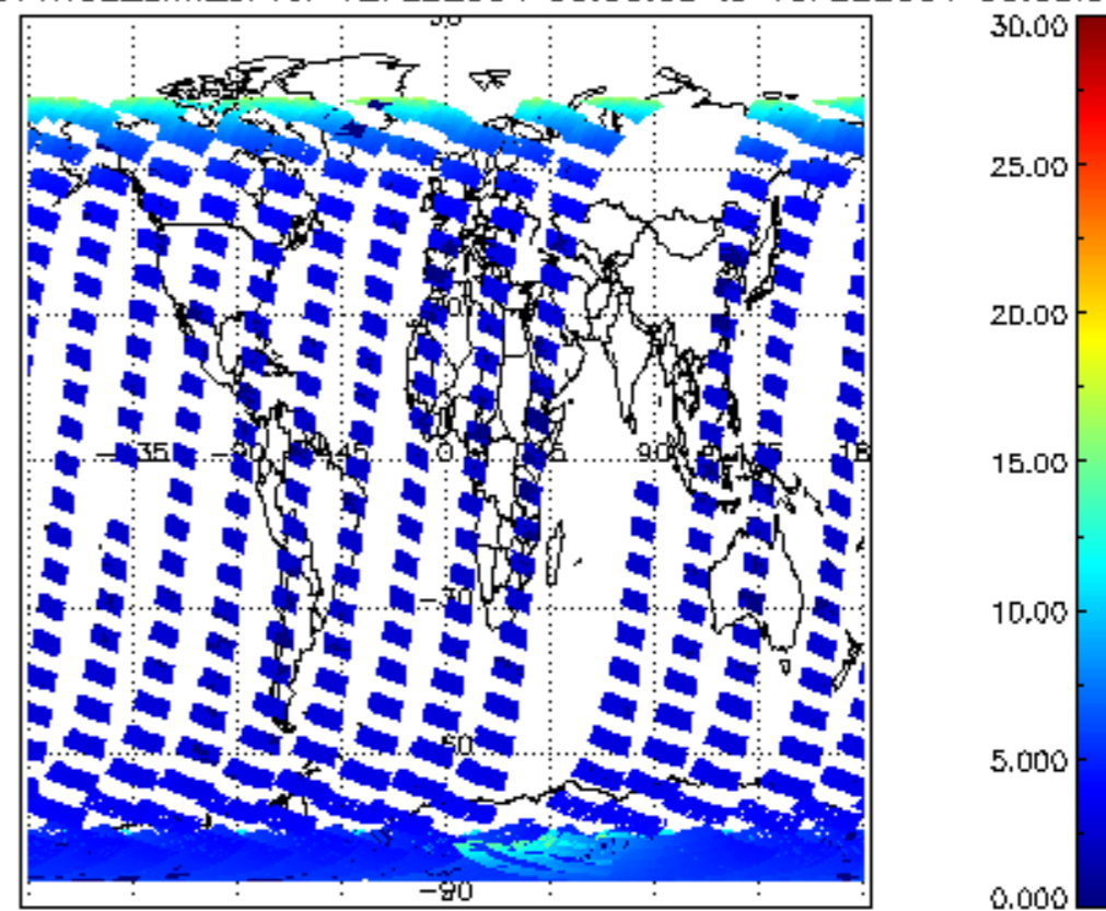
SCIOL2P_NADUV1NO2_amf_cl for 12FEB2004 00:00:00 to 13FEB2004 00:00:00
