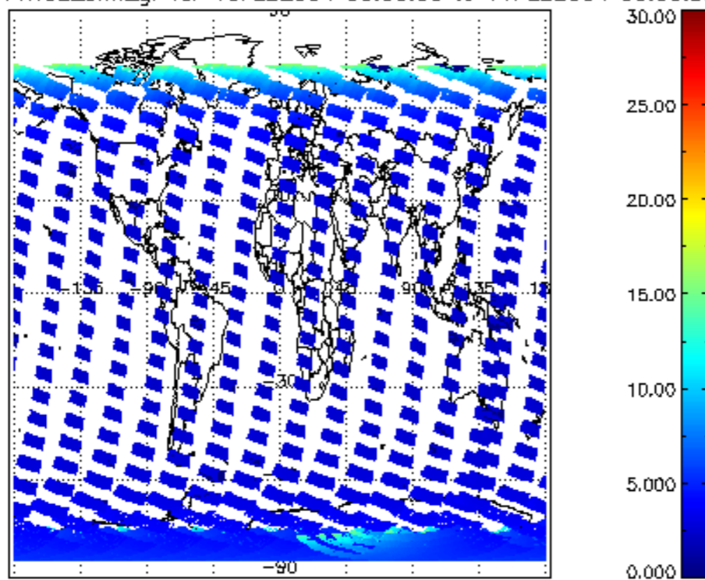
SCIOL2P_NADUV1NO2_amf_gr for 10FEB2004 00:00:00 to 11FEB2004 00:00:00
