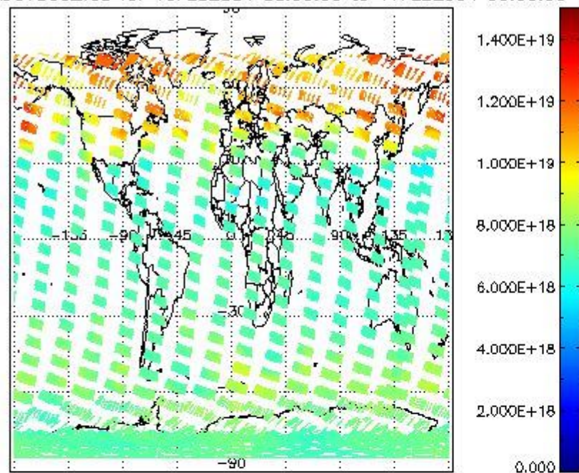
SCIOL2P_NADUV003_vcd for 10FEB2004 00:00:00 to 11FEB2004 00:00:00
