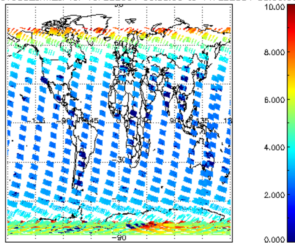
SCIOL2P_NADUV003_amf_cl for 10FEB2004 00:00:00 to 11FEB2004 00:00:00
