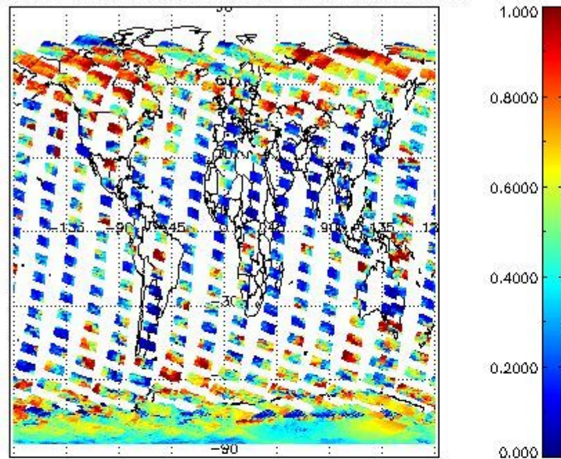
cLfrac for 10FEB2004 00:00:00 to 11FEB2004 00:00:00
