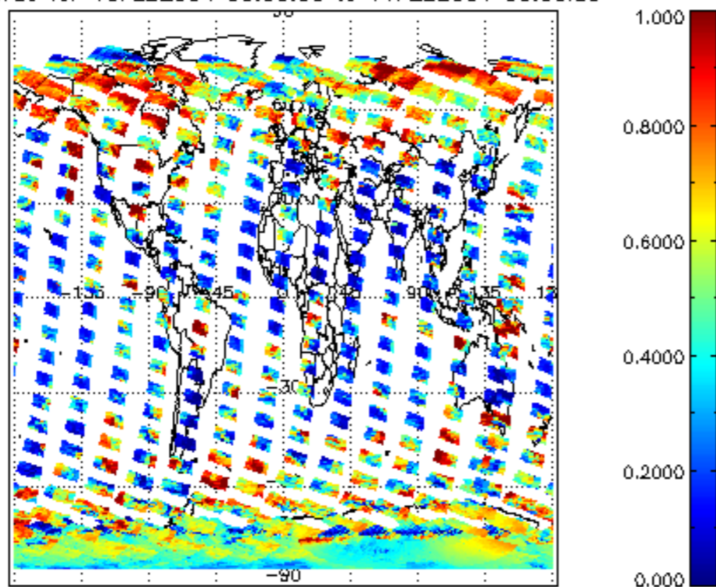
cl_frac for 10FEB2004 00:00:00 to 11FEB2004 00:00:00
