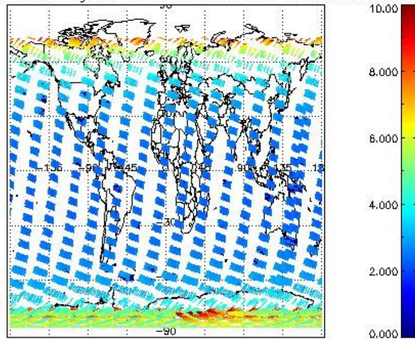
SCIOL2P_NADUV003_amf_gr for 10FEB2004 00:00:00 to 11FEB2004 00:00:00
