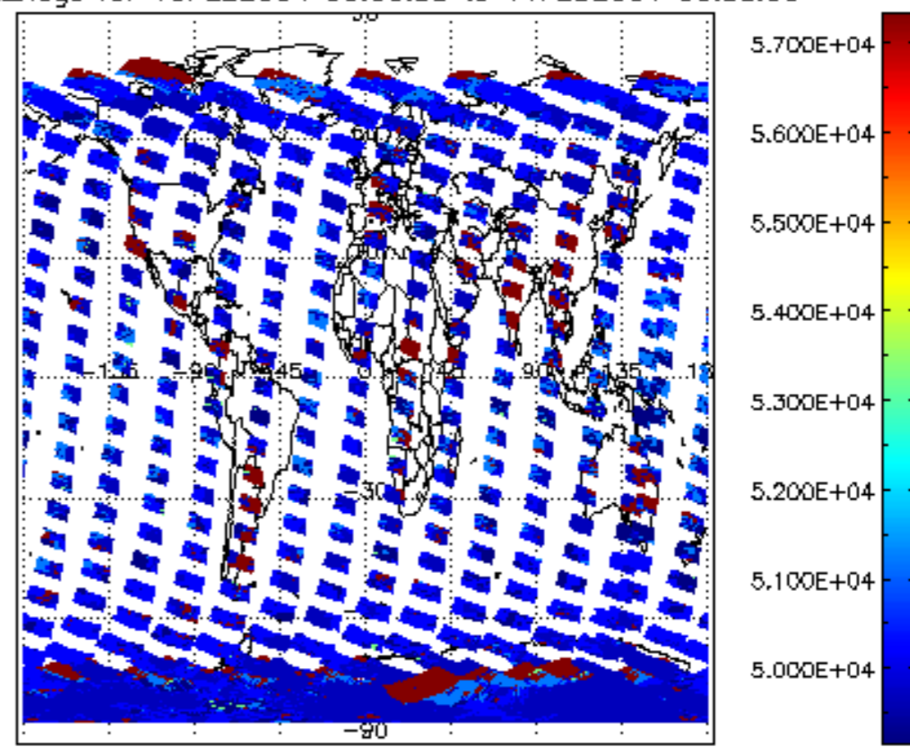
cloud_flags for 10FEB2004 00:00:00 to 11FEB2004 00:00:00
