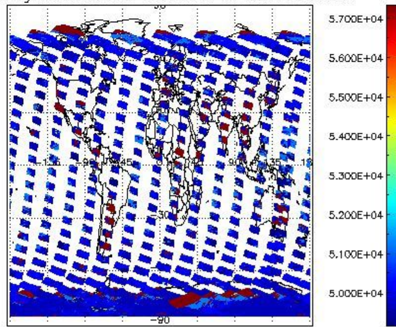
cloud_flags for 10FEB2004 00:00:00 to 11FEB2004 00:00:00
