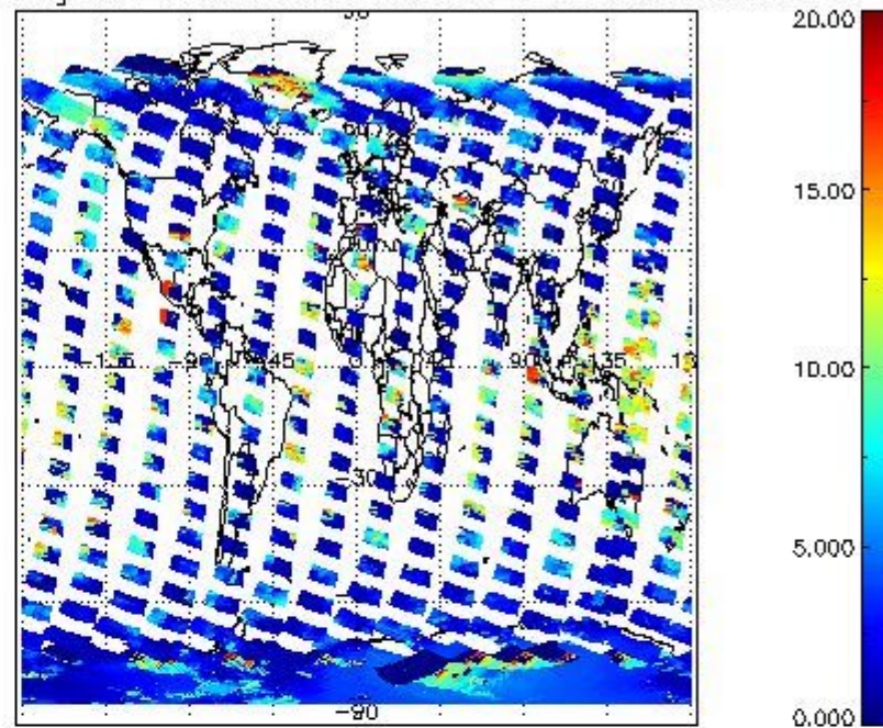
cL_top_height for 10FEB2004 00:00:00 to 11FEB2004 00:00:00
