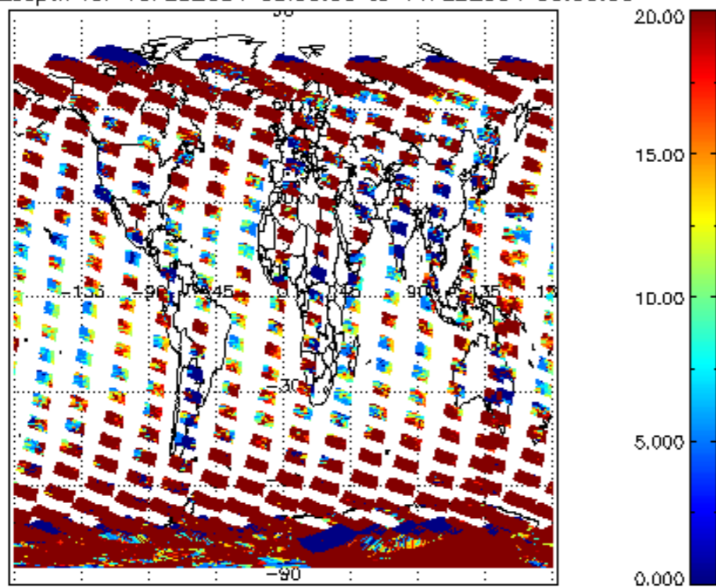
cl_opt_depth for 10FEB2004 00:00:00 to 11FEB2004 00:00:00
