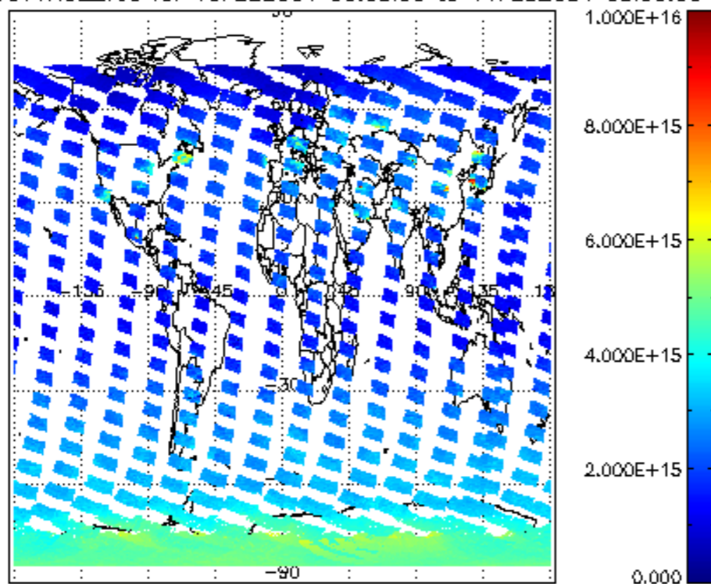
SCIOL2P_NADUV1NO2_vcd for 10FEB2004 00:00:00 to 11FEB2004 00:00:00
