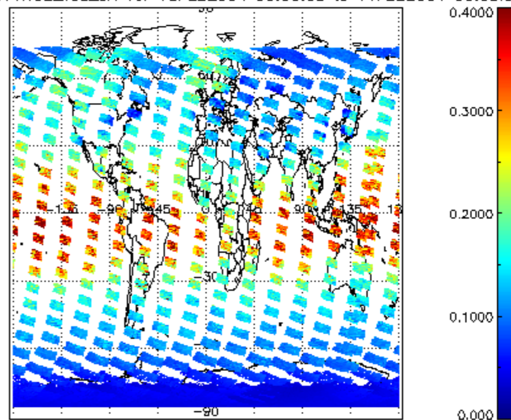
SCIOL2P_NADUV1NO2_vcd_err for 10FEB2004 00:00:00 to 11FEB2004 00:00:00
