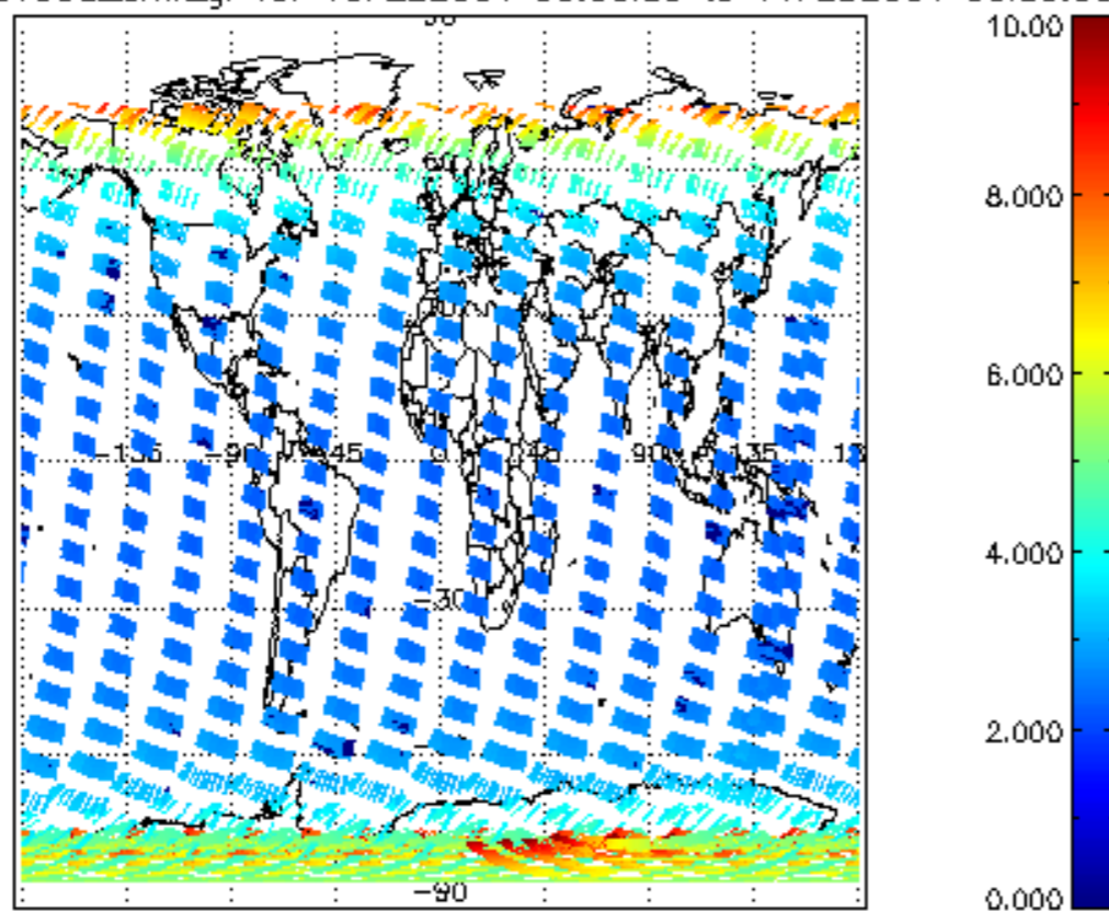
SCIOL2P_NADUV003_amf_gr for 10FEB2004 00:00:00 to 11FEB2004 00:00:00
