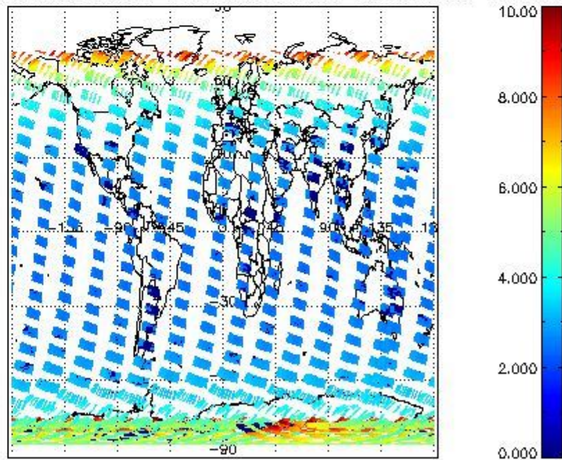
SCIOL2P_NADUV003_amf_cl for 10FEB2004 00:00:00 to 11FEB2004 00:00:00
