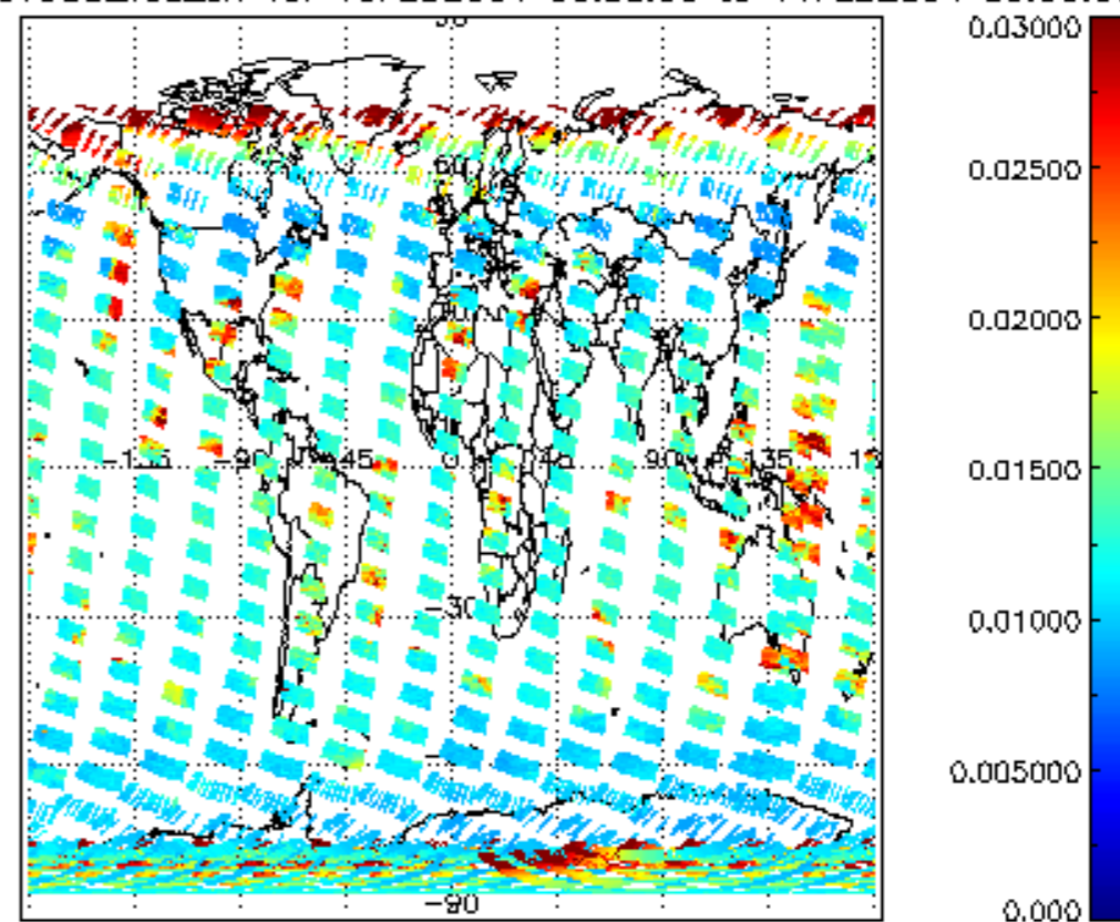
SCIOL2P_NADUV003_vcd_err for 10FEB2004 00:00:00 to 11FEB2004 00:00:00
