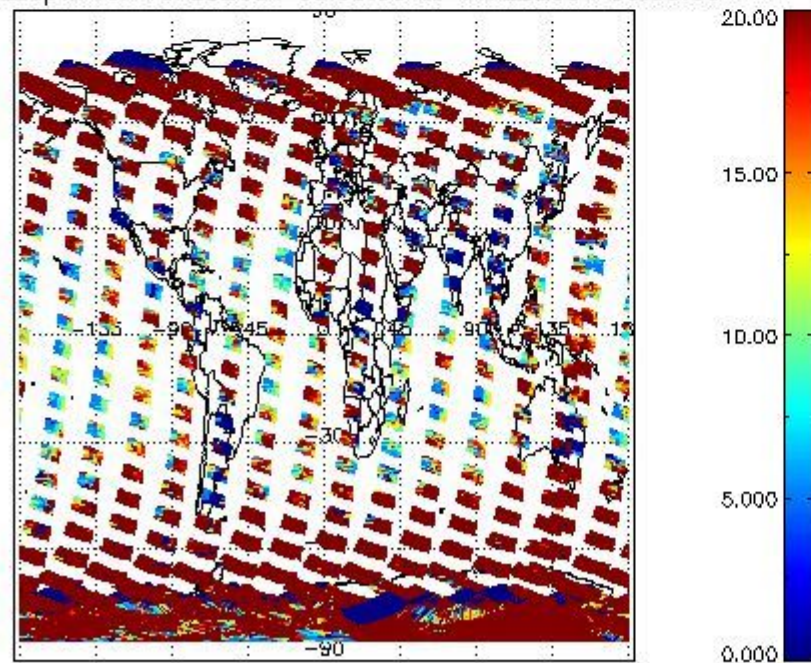
cLopt_depth for 10FEB2004 00:00:00 to 11FEB2004 00:00:00
