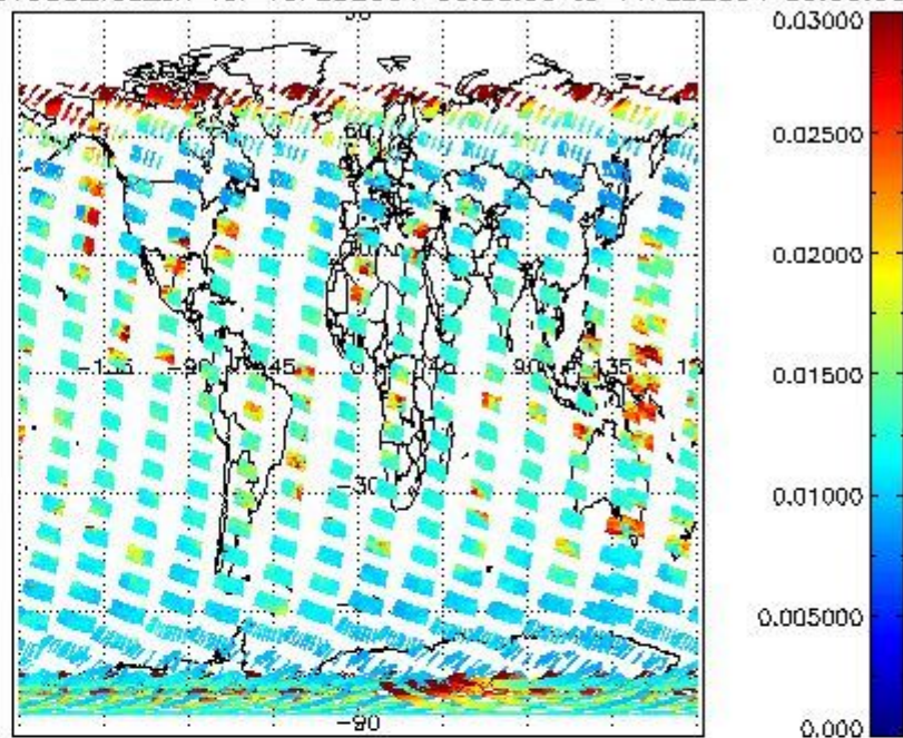
SCIOL2P_NADUV003_vcd_err for 10FEB2004 00:00:00 to 11FEB2004 00:00:00
