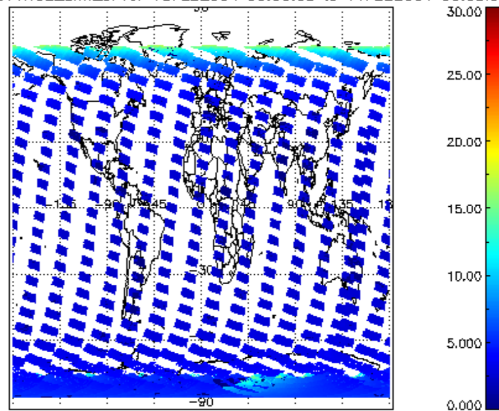
SCIOL2P_NADUV1NO2_amf_cl for 10FEB2004 00:00:00 to 11FEB2004 00:00:00
