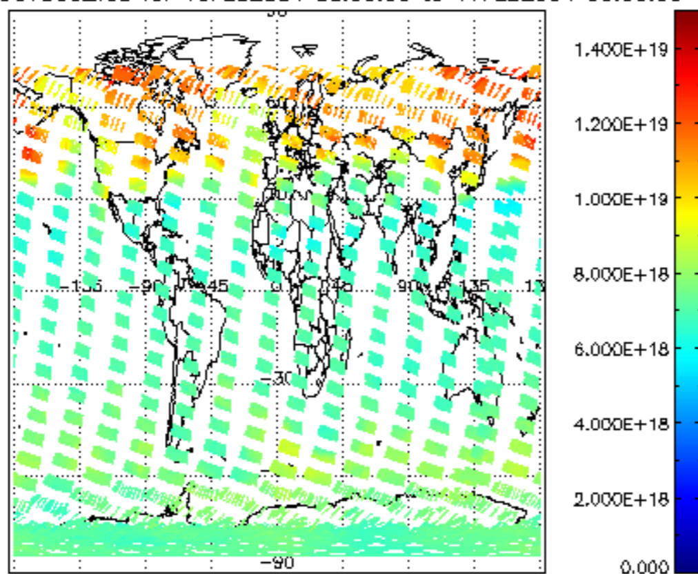
SCIOL2P_NADUV003_vcd for 10FEB2004 00:00:00 to 11FEB2004 00:00:00
