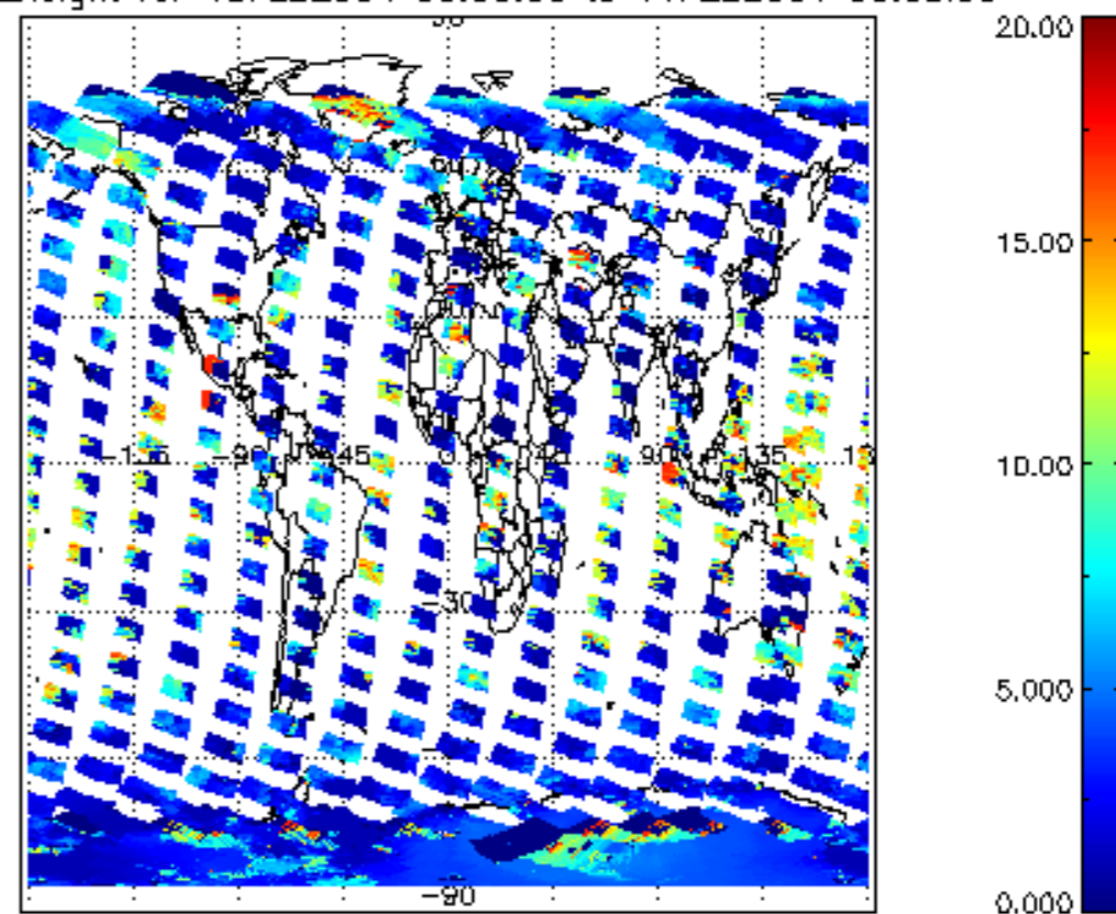
cl_top_height for 10FEB2004 00:00:00 to 11FEB2004 00:00:00
