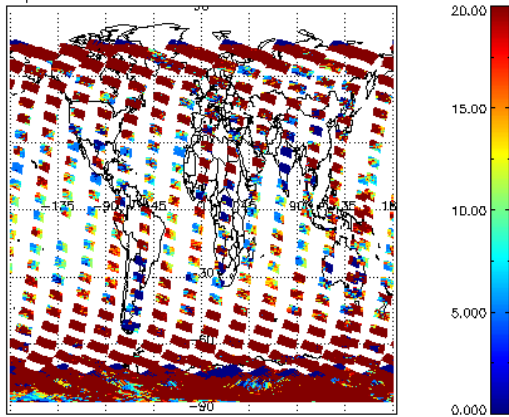
cl_opt_depth for 07FEB2004 00:00:00 to 08FEB2004 00:00:00
