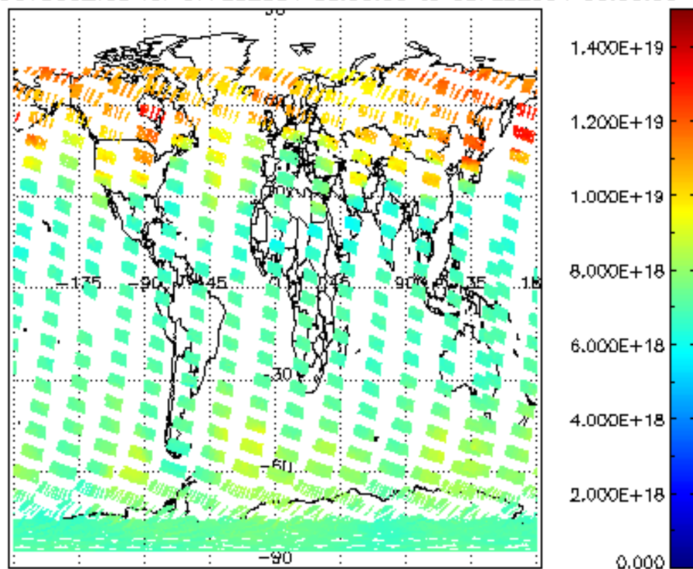
SCIOL2P_NADUV003_vcd for 07FEB2004 00:00:00 to 08FEB2004 00:00:00
