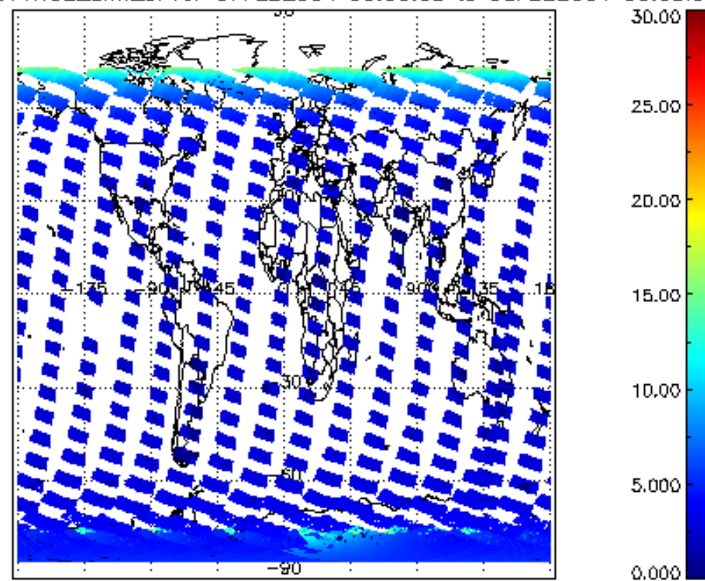
SCIOL2P_NADUV1NO2_amf_cl for 07FEB2004 00:00:00 to 08FEB2004 00:00:00
