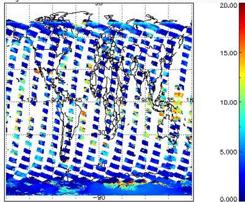
cL_top_height for 07FEB2004 00:00:00 to 08FEB2004 00:00:00
