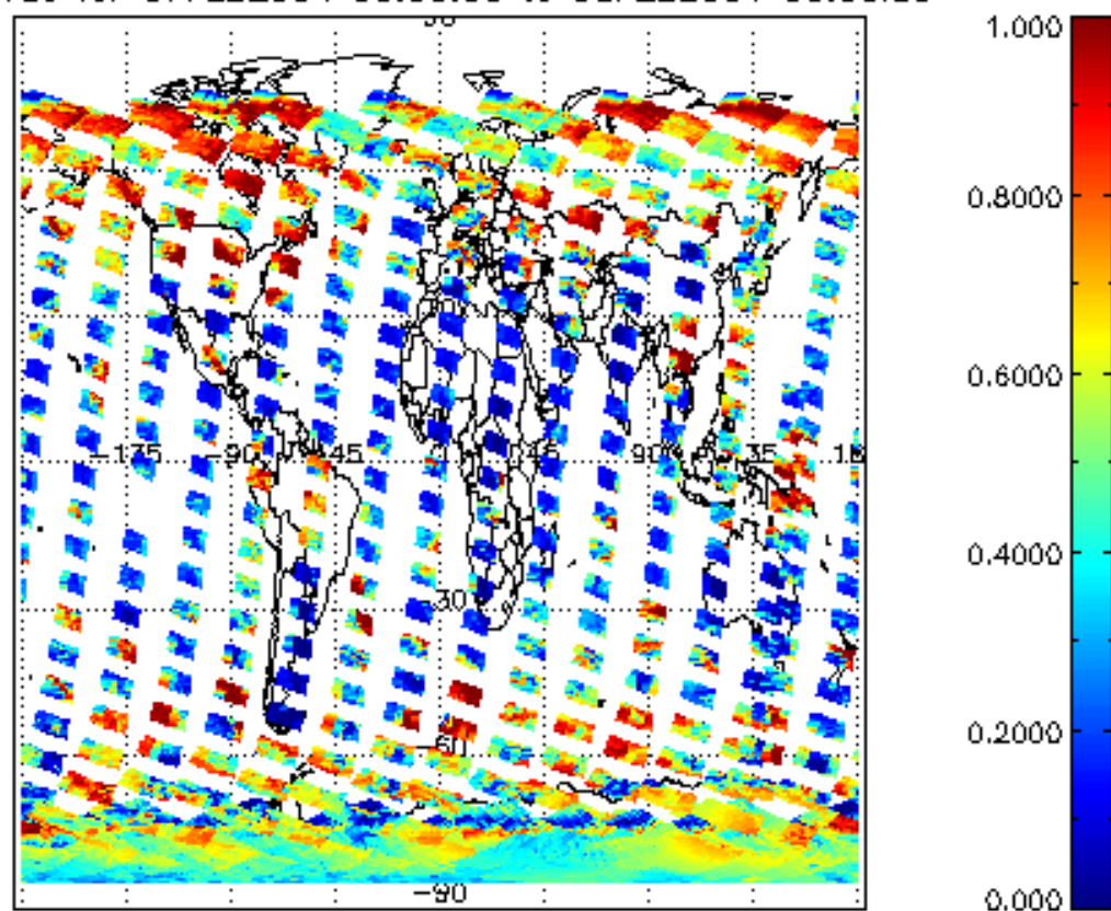
cl_frac for 07FEB2004 00:00:00 to 08FEB2004 00:00:00
