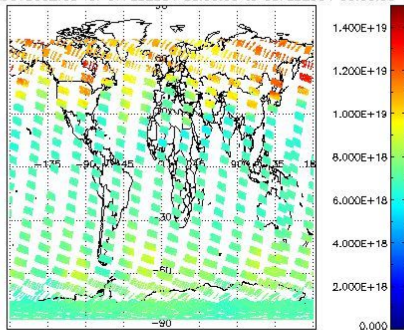
SCIOL2P_NADUV003_vcd for 07FEB2004 00:00:00 to 08FEB2004 00:00:00
