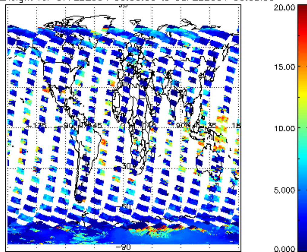
cl_top_height for 07FEB2004 00:00:00 to 08FEB2004 00:00:00
