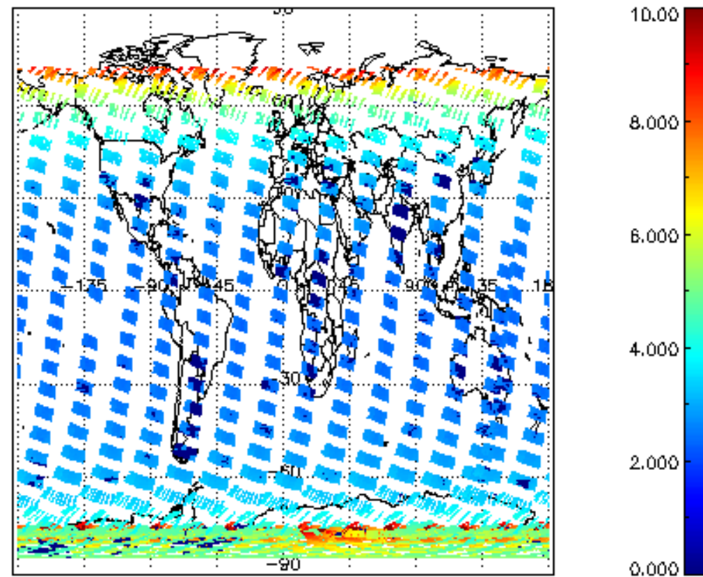
SCIOL2P_NADUV003_amf_cl for 07FEB2004 00:00:00 to 08FEB2004 00:00:00
