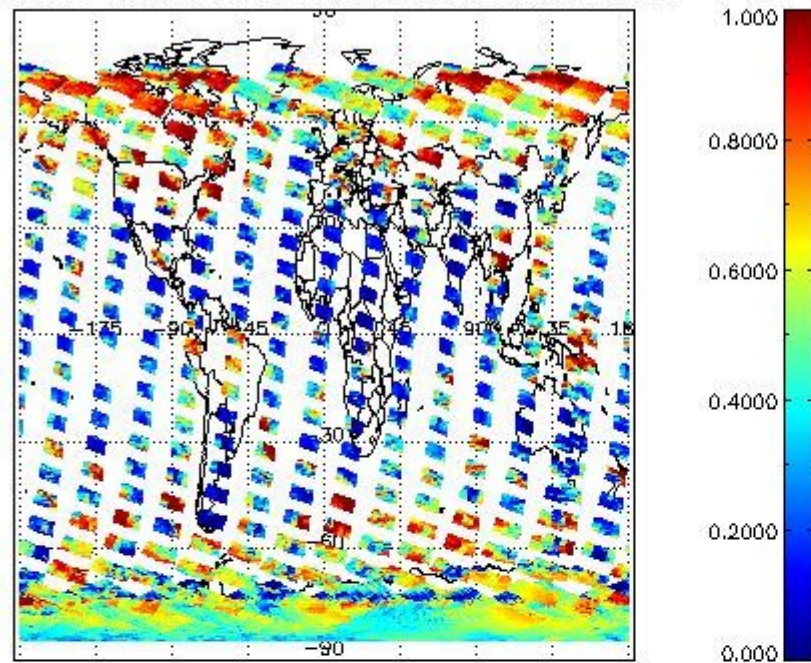
cLfrac for 07FEB2004 00:00:00 to 08FEB2004 00:00:00
