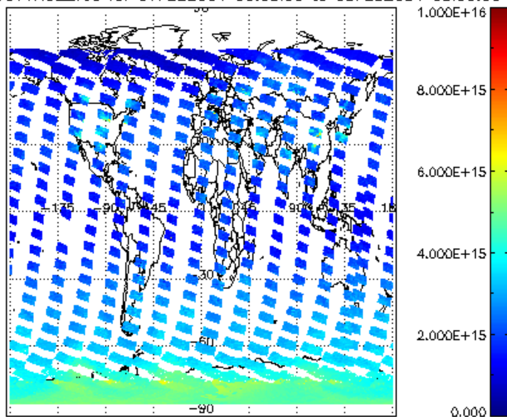
SCIOL2P_NADUV1NO2_vcd for 07FEB2004 00:00:00 to 08FEB2004 00:00:00
