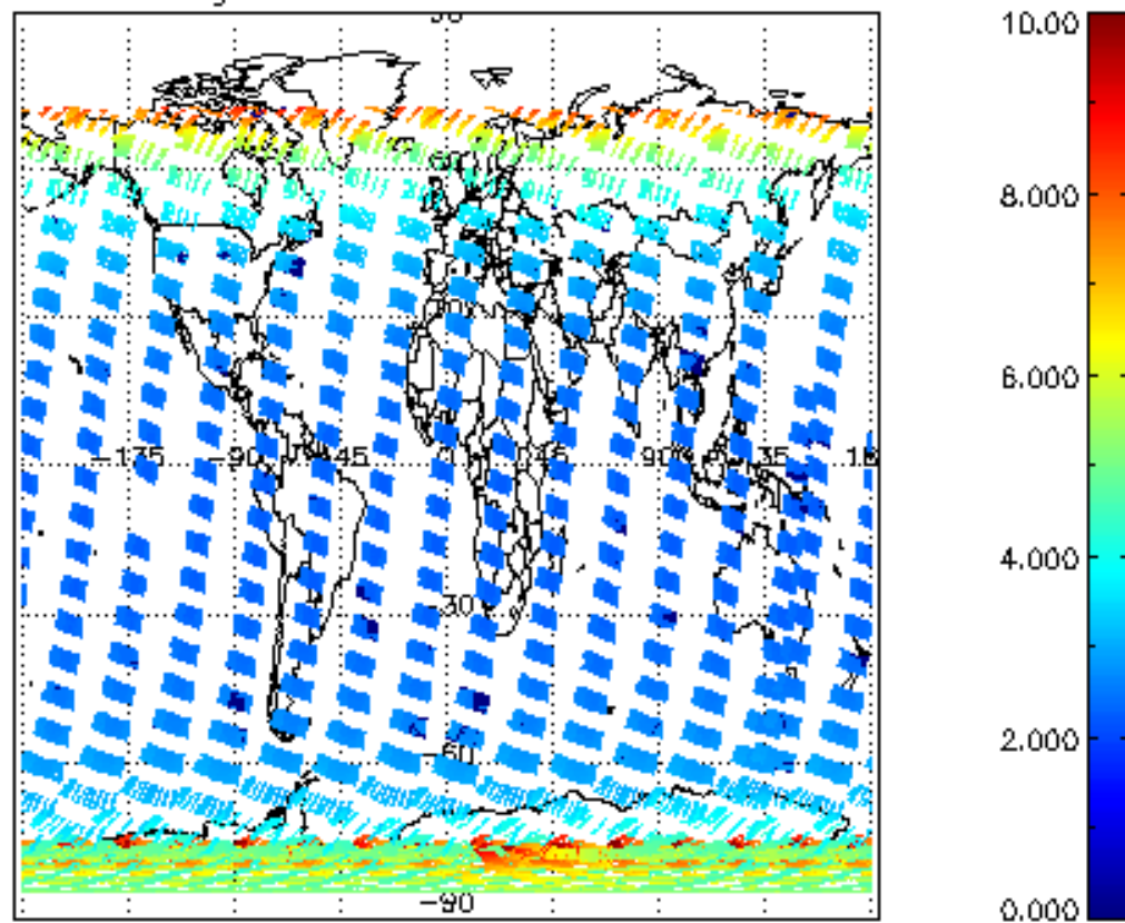
SCIOL2P_NADUV003_amf_gr for 07FEB2004 00:00:00 to 08FEB2004 00:00:00
