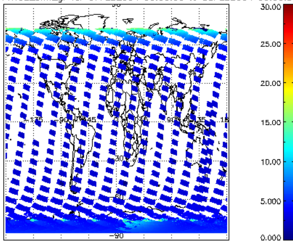
SCIOL2P_NADUV1NO2_amf_gr for 07FEB2004 00:00:00 to 08FEB2004 00:00:00
