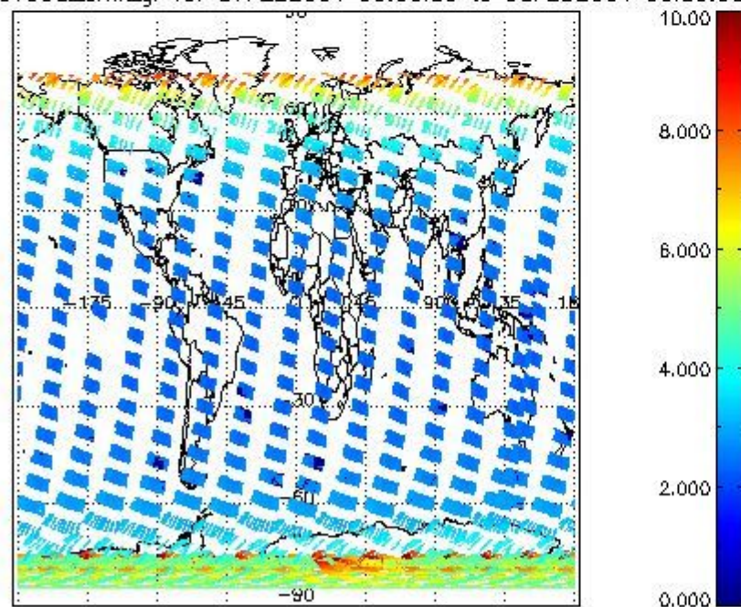
SCIOL2P_NADUV003_amf_gr for 07FEB2004 00:00:00 to 08FEB2004 00:00:00
