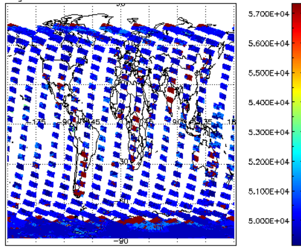
cloud_flags for 07FEB2004 00:00:00 to 08FEB2004 00:00:00
