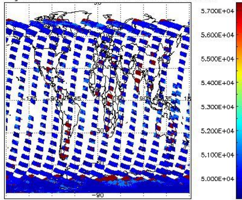
cloud_flags for 07FEB2004 00:00:00 to 08FEB2004 00:00:00
