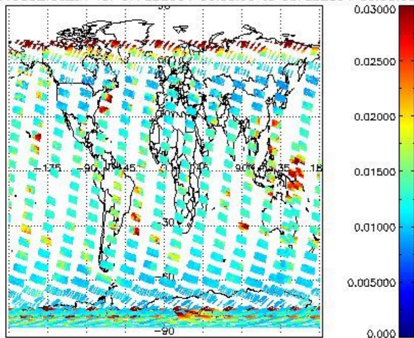
SCIOL2P_NADUV003_vcd_err for 07FEB2004 00:00:00 to 08FEB2004 00:00:00
