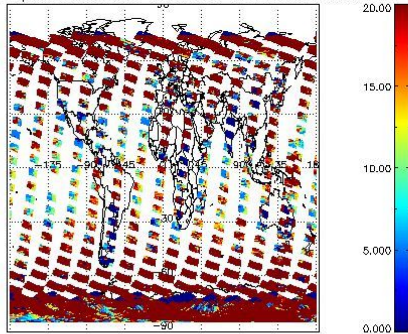
cLopt_depth for 07FEB2004 00:00:00 to 08FEB2004 00:00:00
