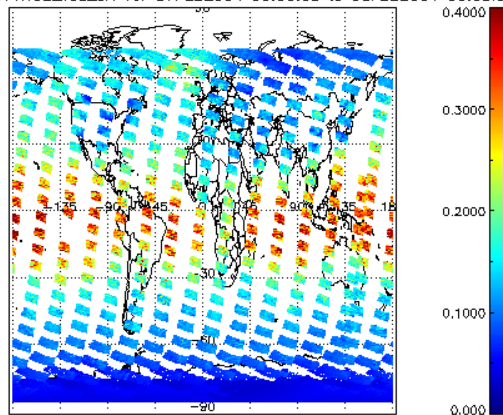
SCIOL2P_NADUV1NO2_vcd_err for 07FEB2004 00:00:00 to 08FEB2004 00:00:00
