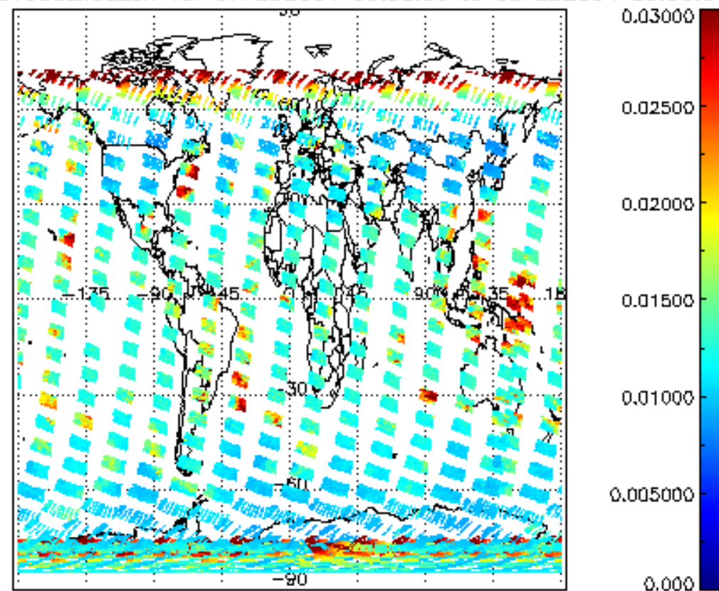
SCIOL2P_NADUV003_vcd_err for 07FEB2004 00:00:00 to 08FEB2004 00:00:00
