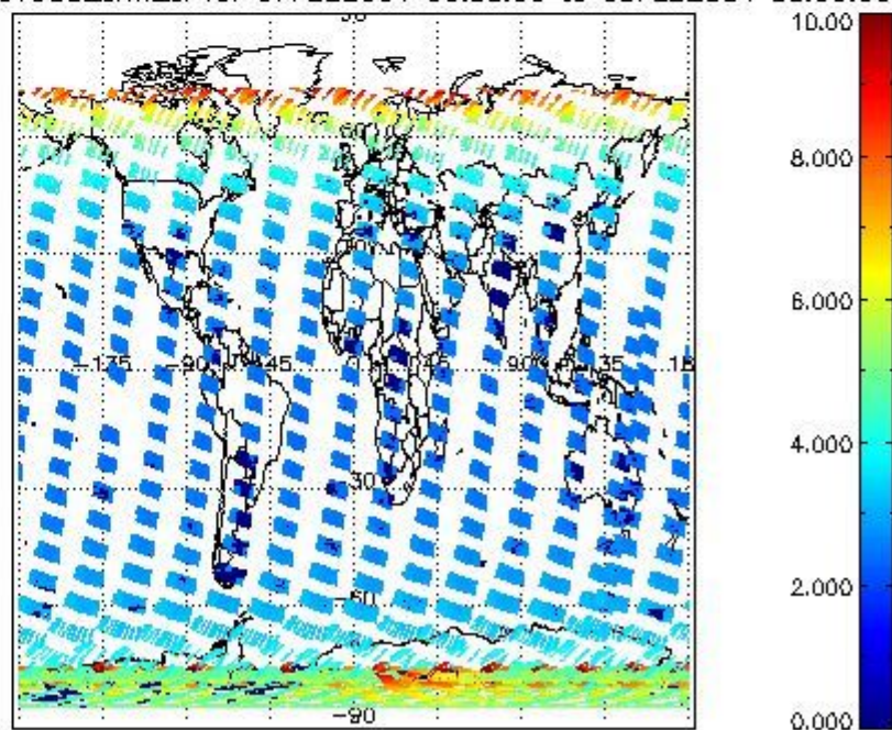
SCIOL2P_NADUV003_amf_cl for 07FEB2004 00:00:00 to 08FEB2004 00:00:00
