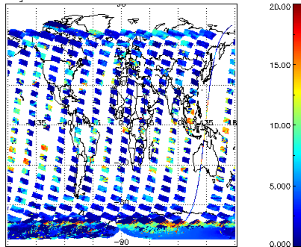
cl_top_height for 05FEB2004 00:00:00 to 06FEB2004 00:00:00
