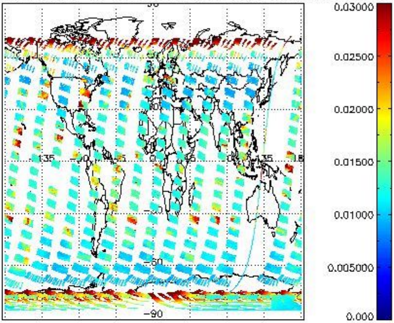
SCIOL2P_NADUV003_vcd_err for 05FEB2004 00:00:00 to 06FEB2004 00:00:00
