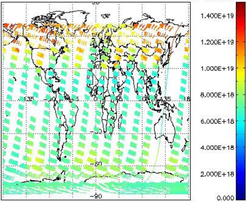
SCIOL2P_NADUV003_vcd for 05FEB2004 00:00:00 to 06FEB2004 00:00:00
