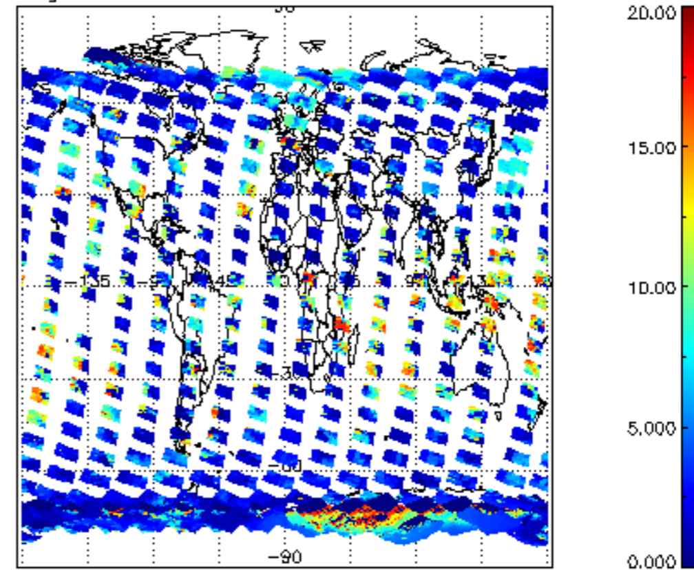
cl_top_height for 03FEB2004 00:00:00 to 04FEB2004 00:00:00
