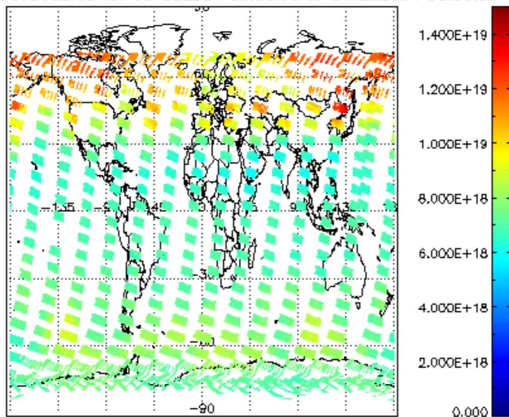
SCIOL2P_NADUV003_vcd for 03FEB2004 00:00:00 to 04FEB2004 00:00:00
