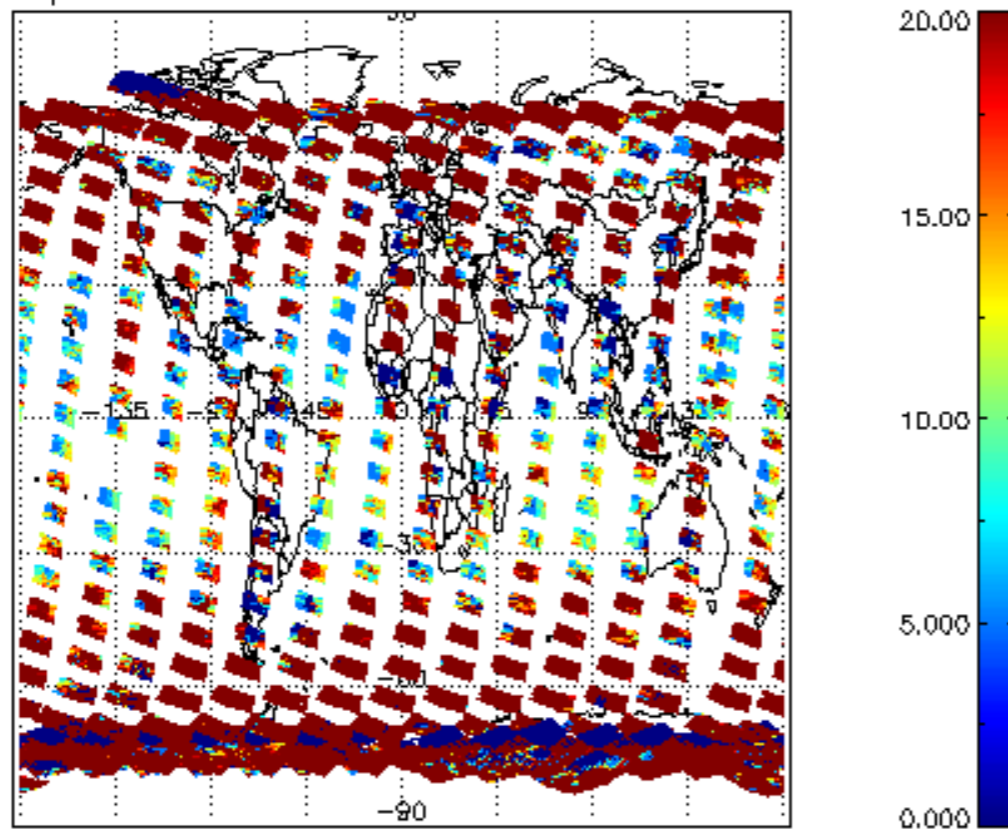
cl_lopt_depth for 03FEB2004 00:00:00 to 04FEB2004 00:00:00
