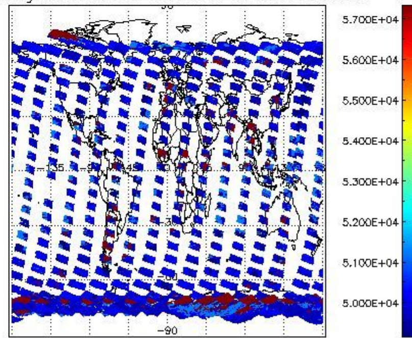
cloud_flags for 03FEB2004 00:00:00 to 04FEB2004 00:00:00
