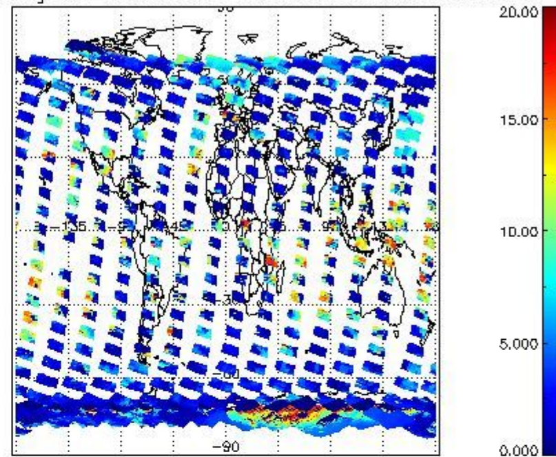
cL_top_height for 03FEB2004 00:00:00 to 04FEB2004 00:00:00
