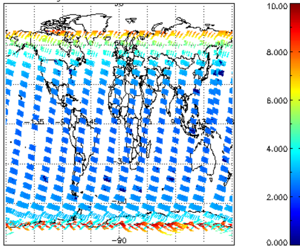
SCIOL2P_NADUV003_amf_gr for 03FEB2004 00:00:00 to 04FEB2004 00:00:00
