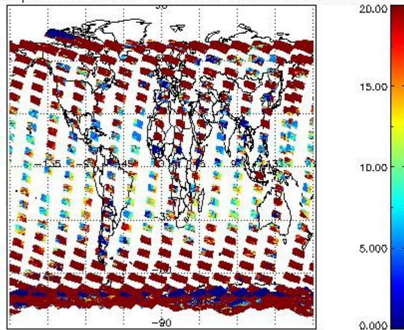
cLopt_depth for 03FEB2004 00:00:00 to 04FEB2004 00:00:00
