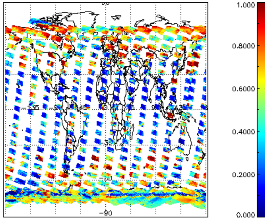
cl_frac for 03FEB2004 00:00:00 to 04FEB2004 00:00:00
