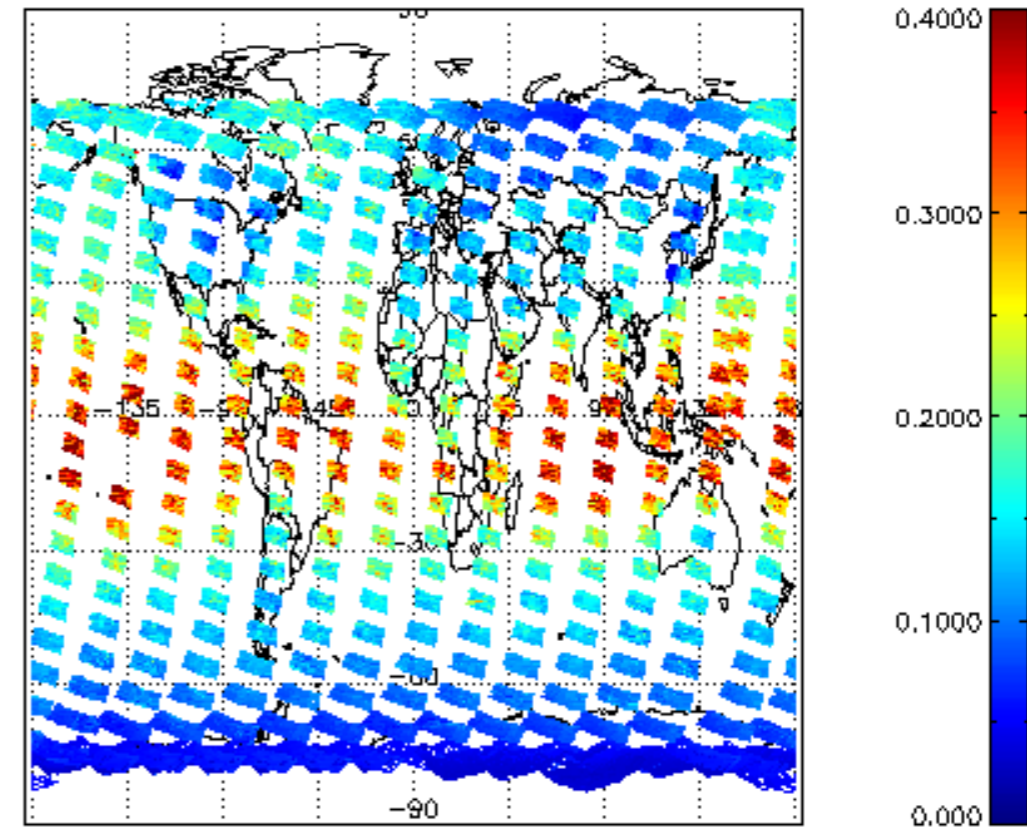
SCIOL2P_NADUV1NO2_vcd_err for 03FEB2004 00:00:00 to 04FEB2004 00:00:00
