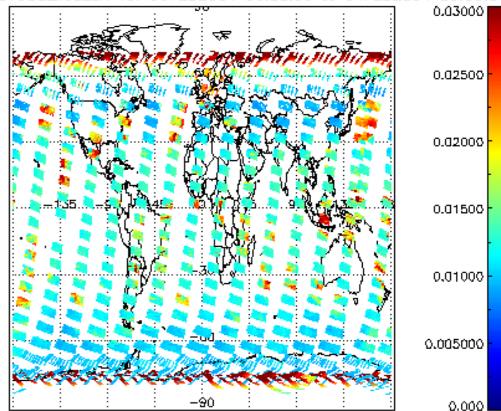
SCIOL2P_NADUV003_vcd_err for 03FEB2004 00:00:00 to 04FEB2004 00:00:00
