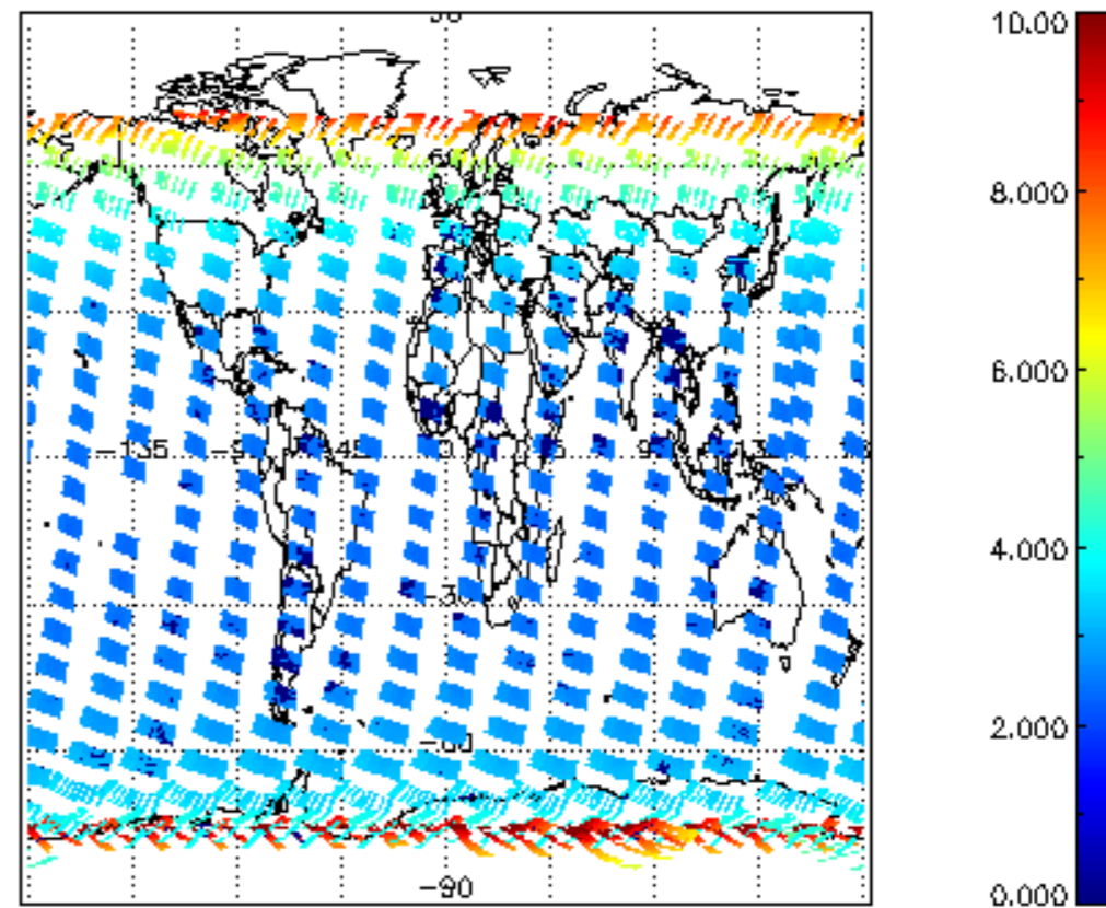
SCIOL2P_NADUV003_amf_cl for 03FEB2004 00:00:00 to 04FEB2004 00:00:00
