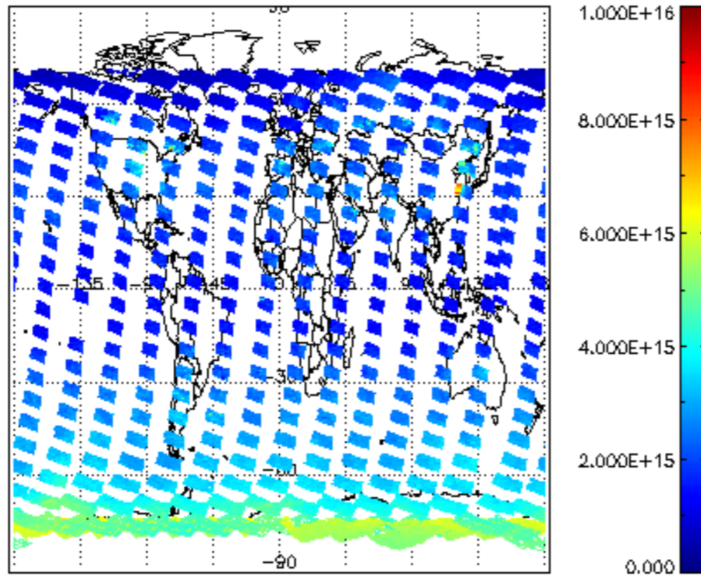
SCIOL2P_NADUV1NO2_vcd for 03FEB2004 00:00:00 to 04FEB2004 00:00:00
