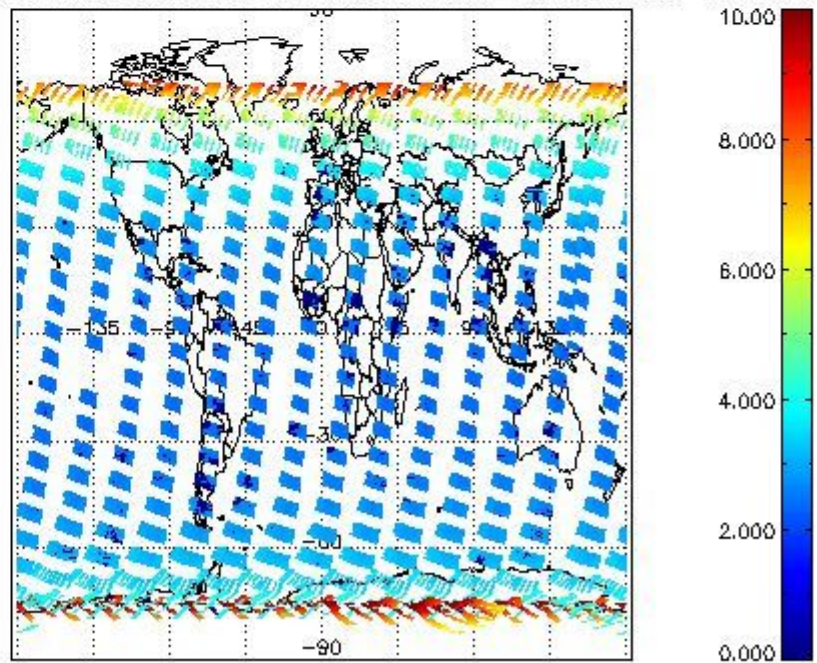
SCIOL2P_NADUV003_amf_cl for 03FEB2004 00:00:00 to 04FEB2004 00:00:00
