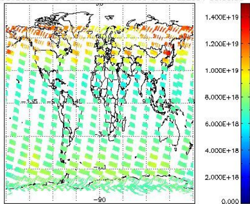
SCIOL2P_NADUV003_vcd for 03FEB2004 00:00:00 to 04FEB2004 00:00:00
