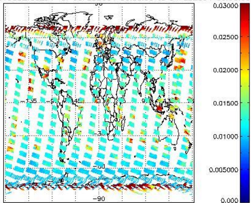
SCIOL2P_NADUV003_vcd_err for 03FEB2004 00:00:00 to 04FEB2004 00:00:00
