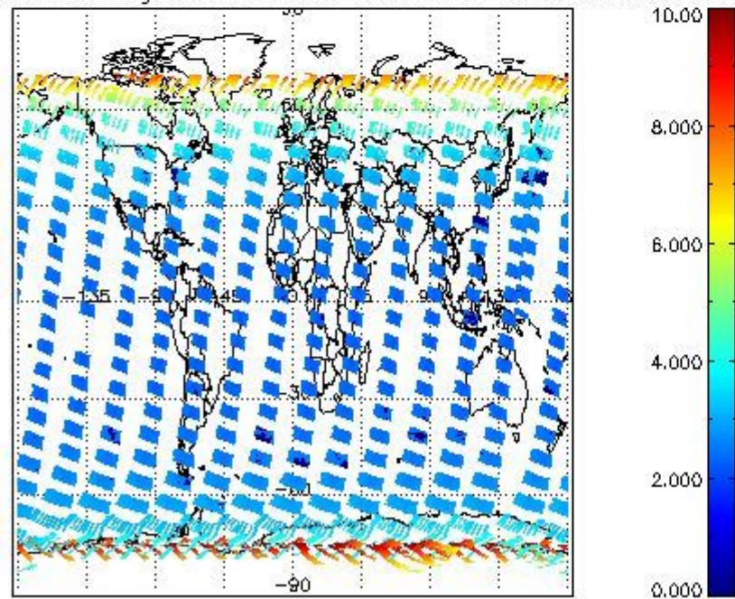
SCIOL2P_NADUV003_amf_gr for 03FEB2004 00:00:00 to 04FEB2004 00:00:00
