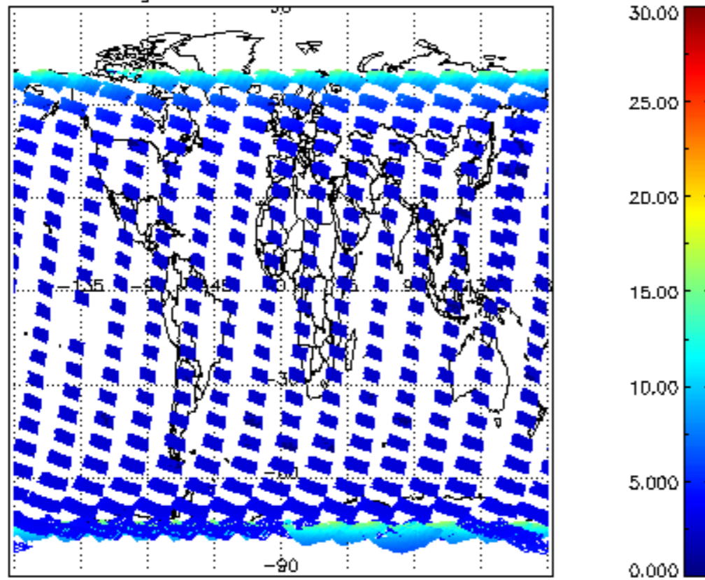
SCIOL2P_NADUV1NO2_amf_gr for 03FEB2004 00:00:00 to 04FEB2004 00:00:00
