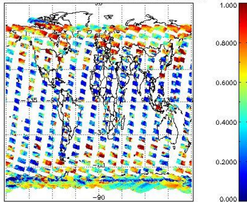
cLfrac for 03FEB2004 00:00:00 to 04FEB2004 00:00:00
