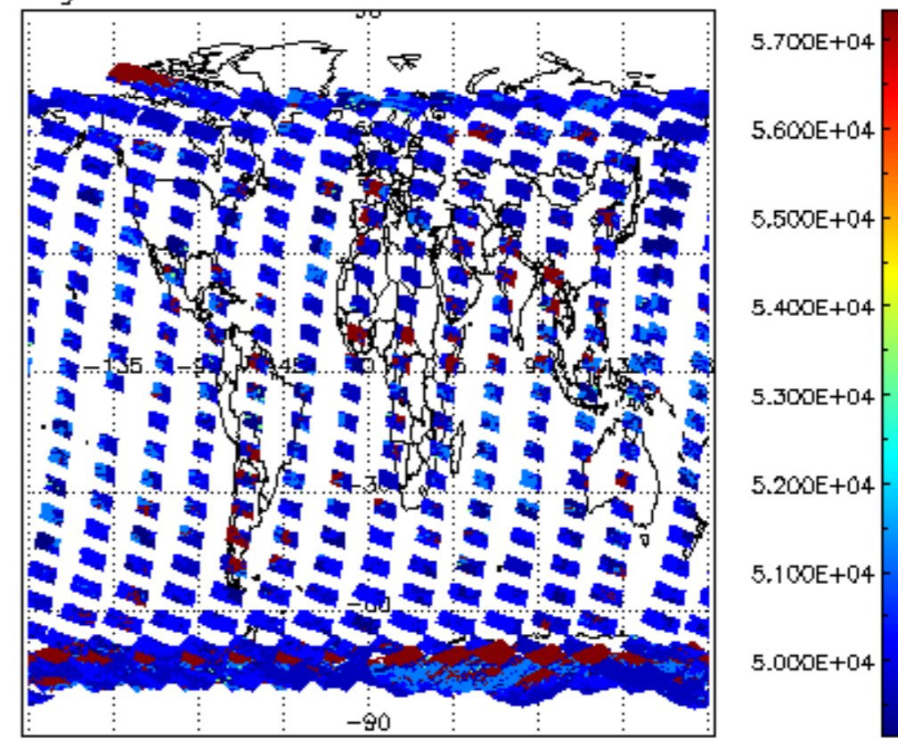
cloud_flags for 03FEB2004 00:00:00 to 04FEB2004 00:00:00
