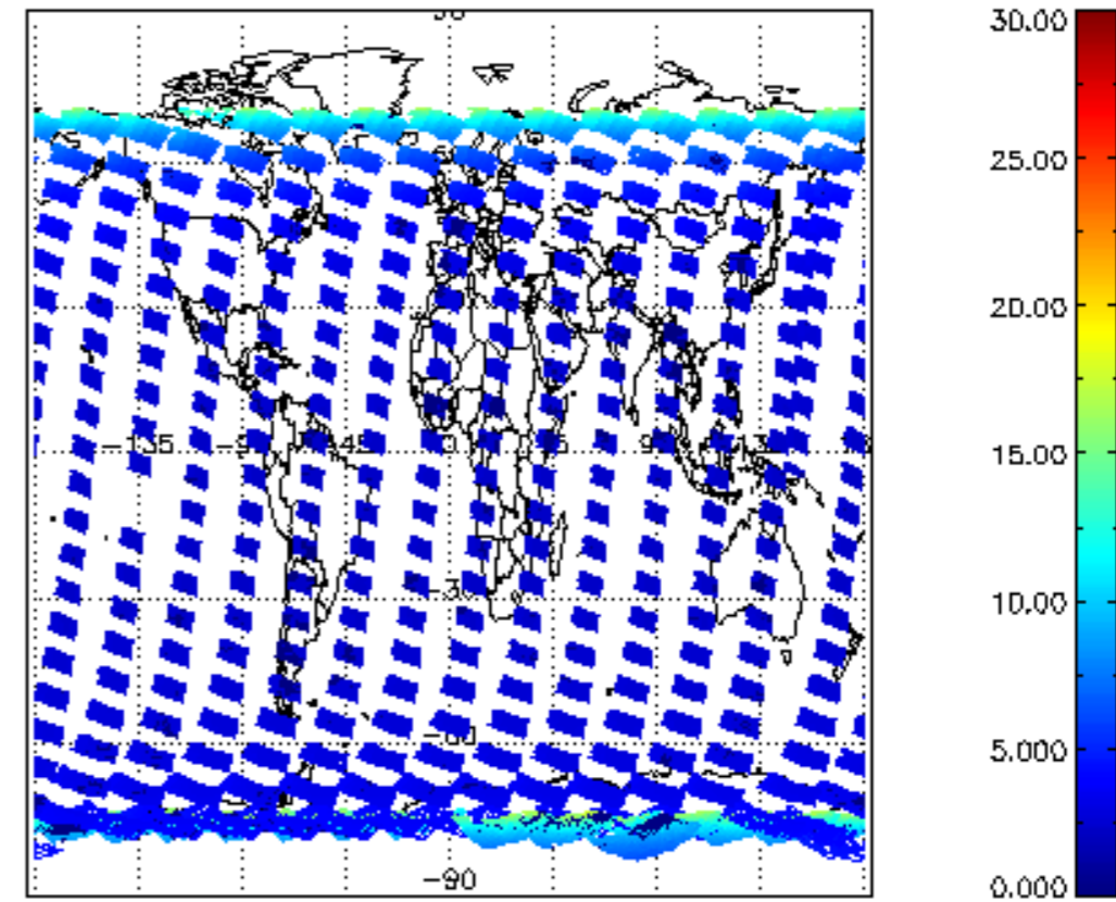
SCIOL2P_NADUV1NO2_amf_cl for 03FEB2004 00:00:00 to 04FEB2004 00:00:00
