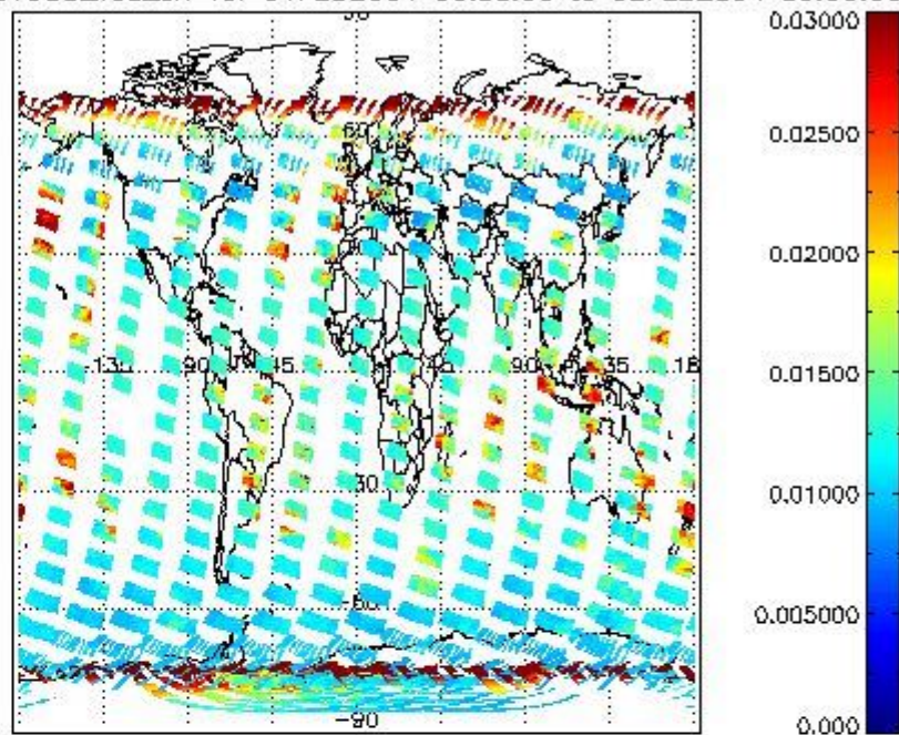
SCIOL2P_NADUV003_vcd_err for 01FEB2004 00:00:00 to 02FEB2004 00:00:00
