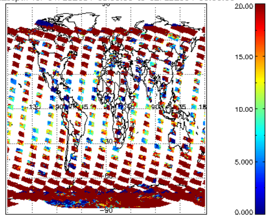
cl_lopt_depth for 01FEB2004 00:00:00 to 02FEB2004 00:00:00
