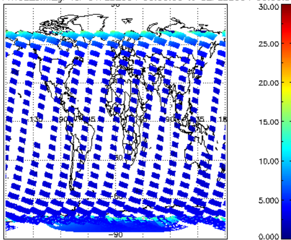
SCIOL2P_NADUV1NO2_amf_gr for 01FEB2004 00:00:00 to 02FEB2004 00:00:00
