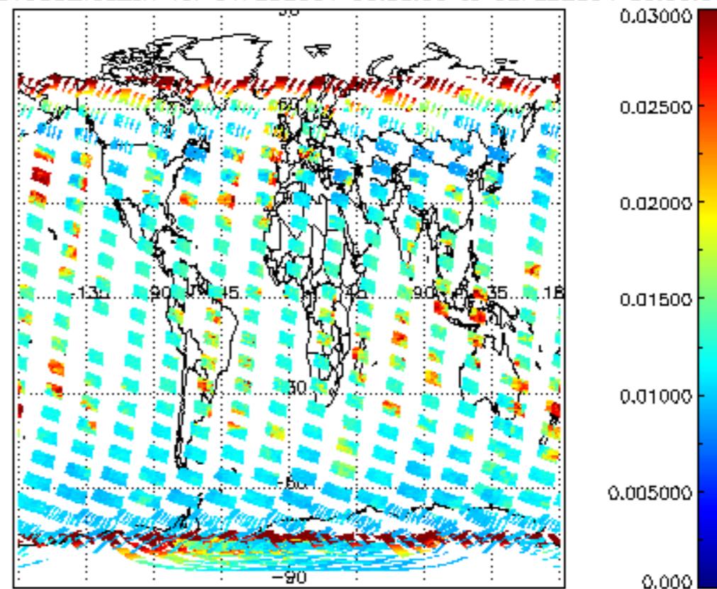
SCIOL2P_NADUV003_vcd_err for 01FEB2004 00:00:00 to 02FEB2004 00:00:00
