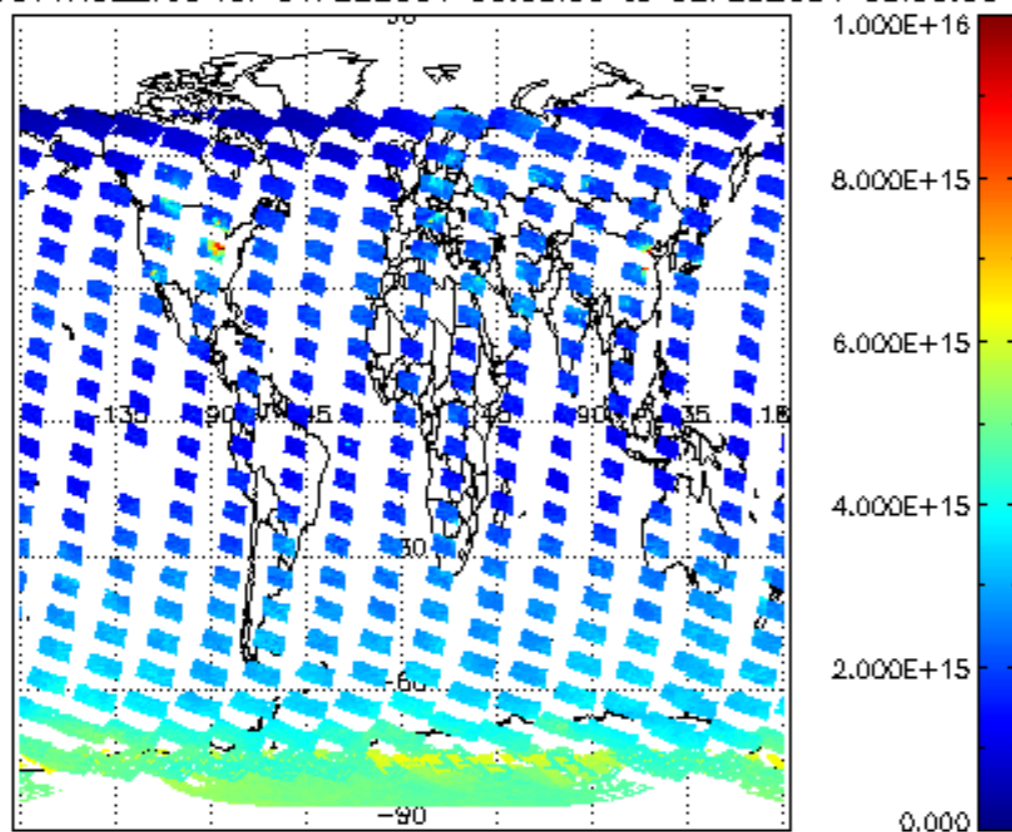
SCIOL2P_NADUV1NO2_vcd for 01FEB2004 00:00:00 to 02FEB2004 00:00:00
