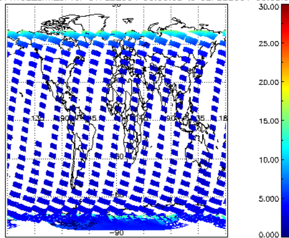
SCIOL2P_NADUV1NO2_amf_cl for 01FEB2004 00:00:00 to 02FEB2004 00:00:00
