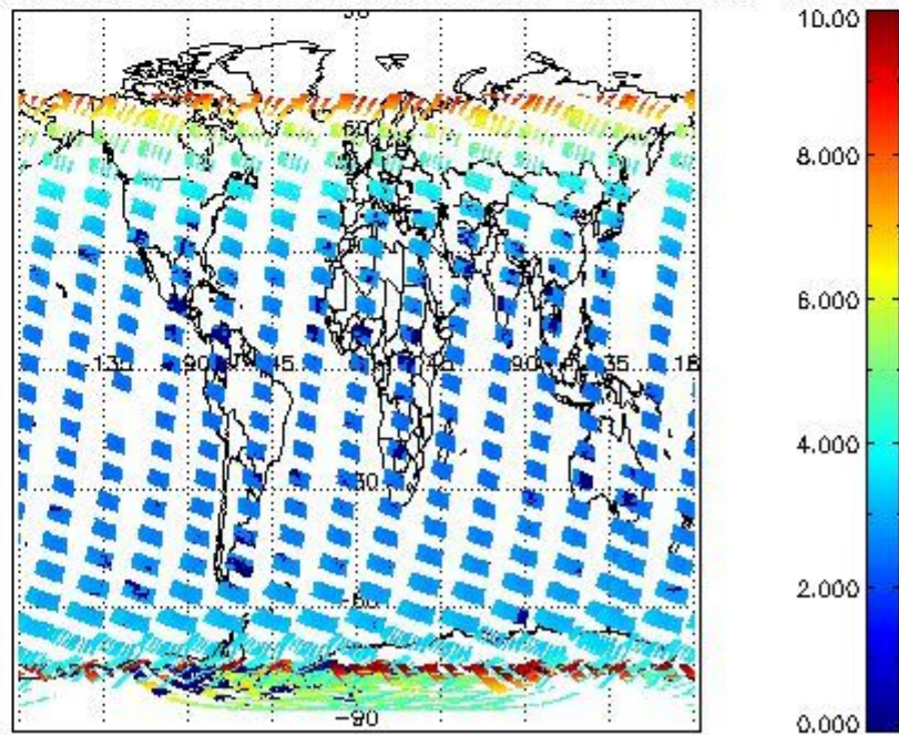
SCIOL2P_NADUV003_amf_cl for 01FEB2004 00:00:00 to 02FEB2004 00:00:00
