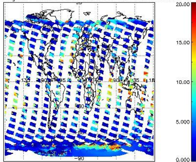
cL_top_height for 01FEB2004 00:00:00 to 02FEB2004 00:00:00
