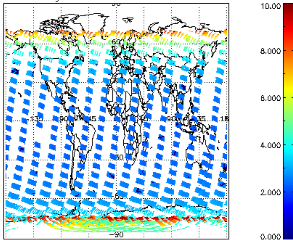
SCIOL2P_NADUV003_amf_gr for 01FEB2004 00:00:00 to 02FEB2004 00:00:00
