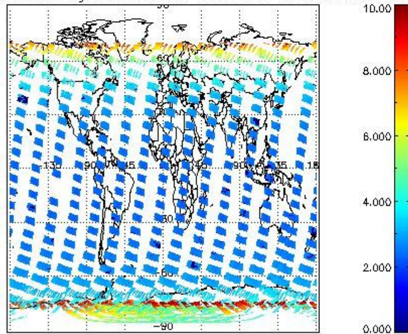
SCIOL2P_NADUV003_amf_gr for 01FEB2004 00:00:00 to 02FEB2004 00:00:00
