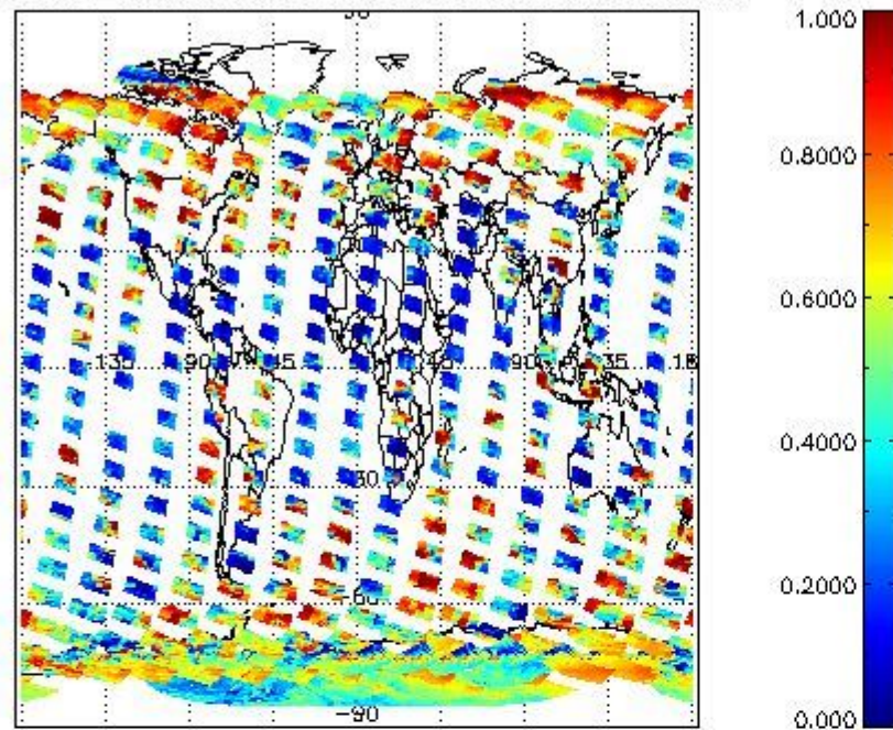
cLfrac for 01FEB2004 00:00:00 to 02FEB2004 00:00:00
