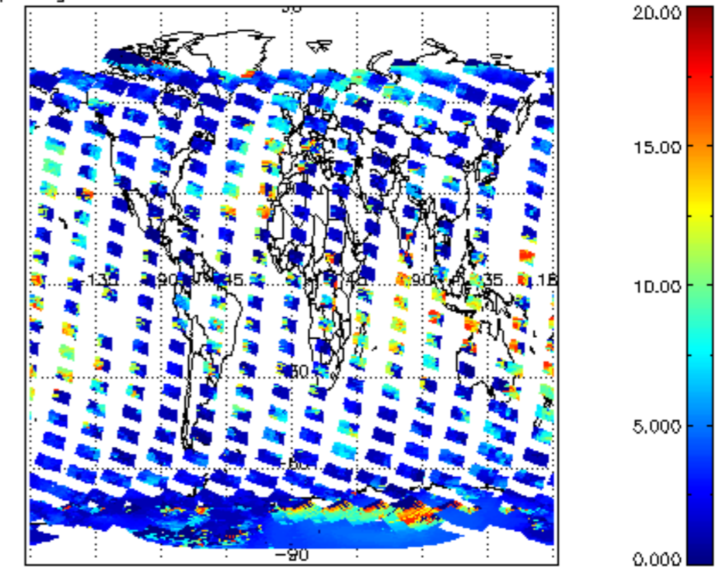
cl_top_height for 01FEB2004 00:00:00 to 02FEB2004 00:00:00
