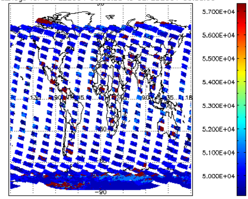
cloud_flags for 01FEB2004 00:00:00 to 02FEB2004 00:00:00
