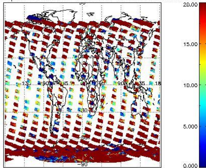
cLopt_depth for 01FEB2004 00:00:00 to 02FEB2004 00:00:00
