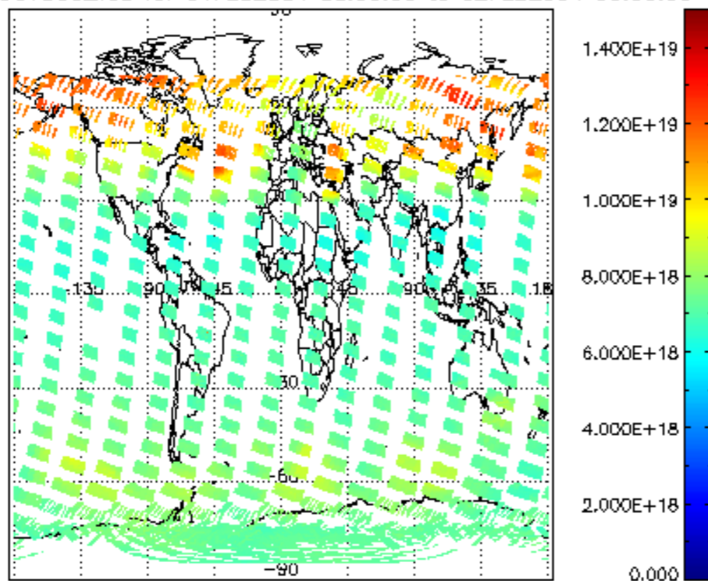
SCIOL2P_NADUV003_vcd for 01FEB2004 00:00:00 to 02FEB2004 00:00:00
