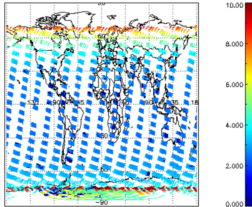
SCIOL2P_NADUV003_amf_cl for 01FEB2004 00:00:00 to 02FEB2004 00:00:00
