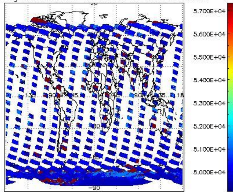
cloud_flags for 01FEB2004 00:00:00 to 02FEB2004 00:00:00
