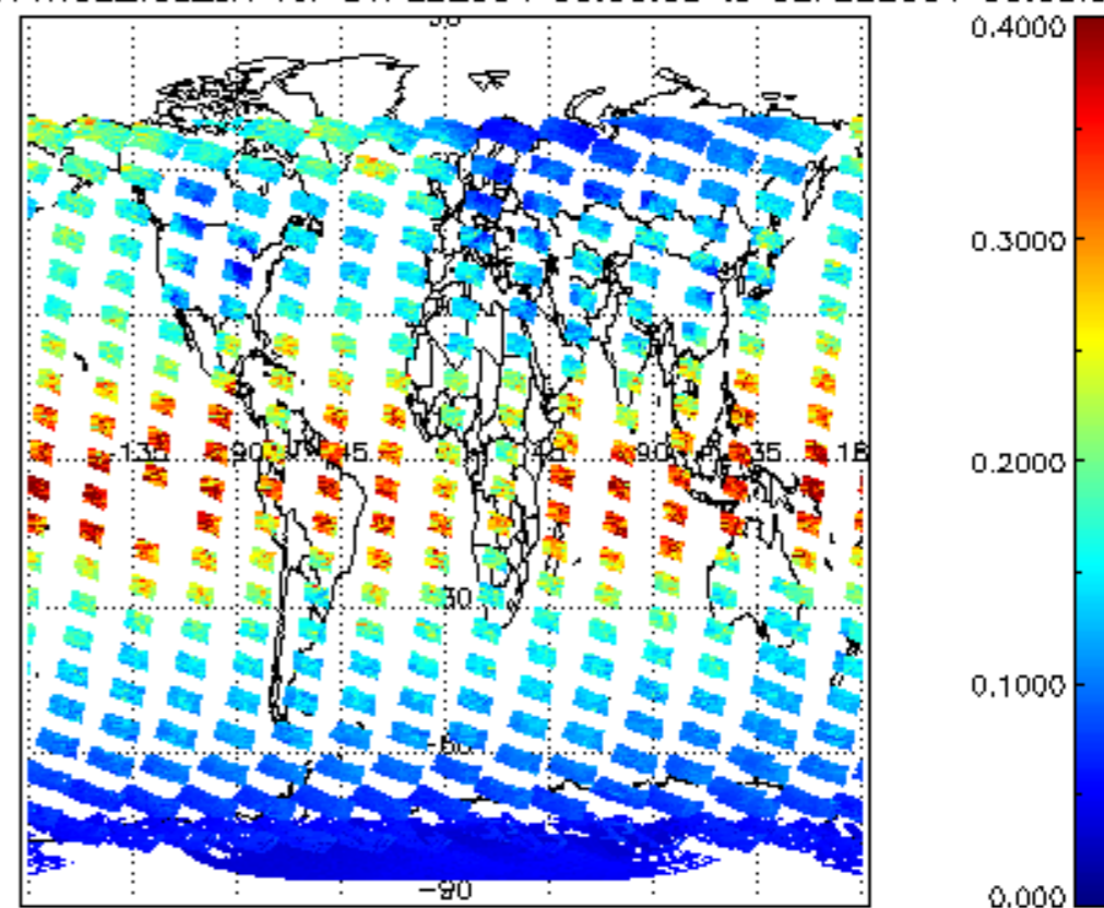
SCIOL2P_NADUV1NO2_vcd_err for 01FEB2004 00:00:00 to 02FEB2004 00:00:00
