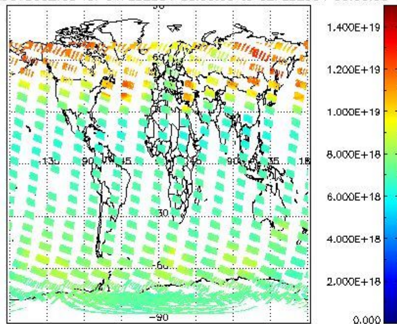
SCIOL2P_NADUV003_vcd for 01FEB2004 00:00:00 to 02FEB2004 00:00:00
