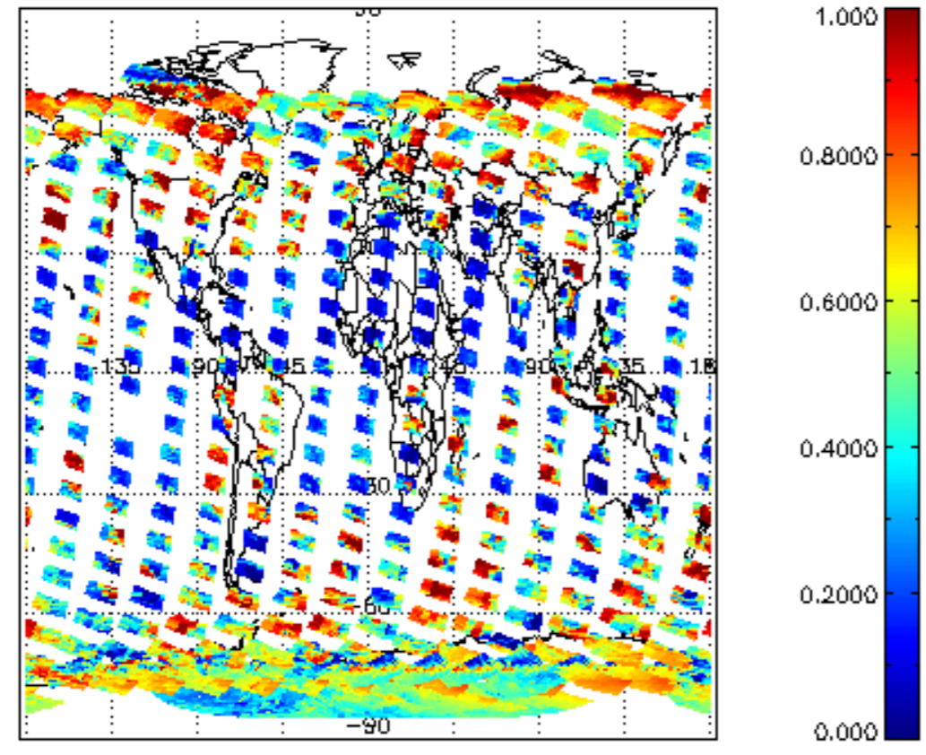
cl_frac for 01FEB2004 00:00:00 to 02FEB2004 00:00:00
