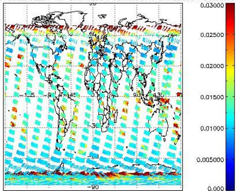
SCIOL2P_NADUV003_vcd_err for 31JAN2004 00:00:00 to 01FEB2004 00:00:00
