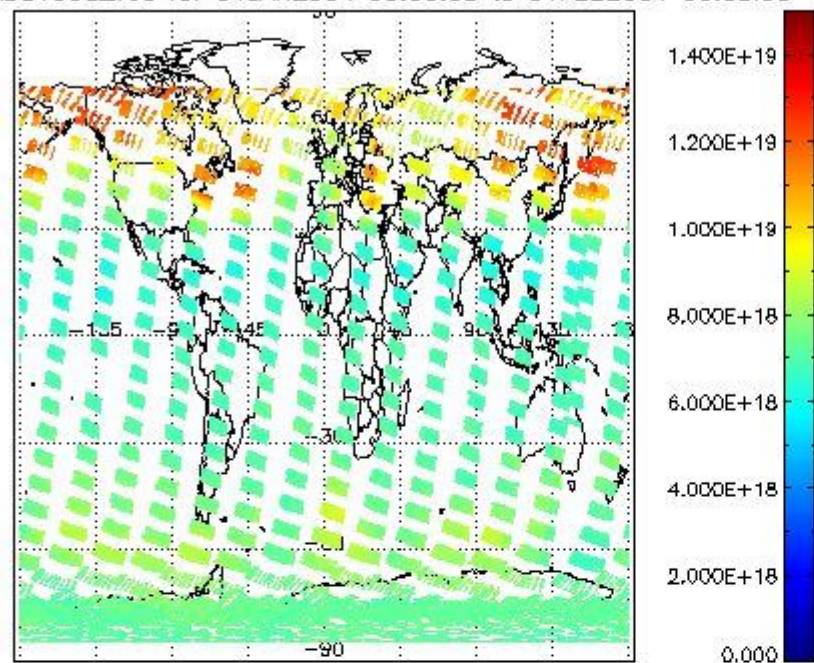
SCIOL2P_NADUV003_vcd for 31JAN2004 00:00:00 to 01FEB2004 00:00:00
