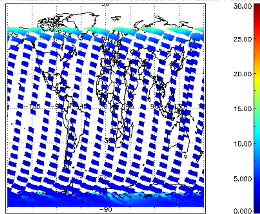
SCIOL2P_NADUV1NO2_amf_cl for 31JAN2004 00:00:00 to 01FEB2004 00:00:00
