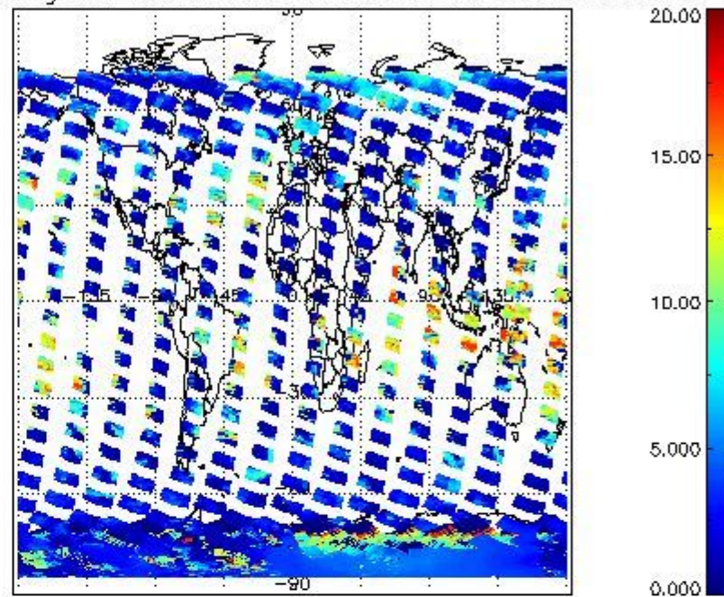
cL_top_height for 31JAN2004 00:00:00 to 01FEB2004 00:00:00
