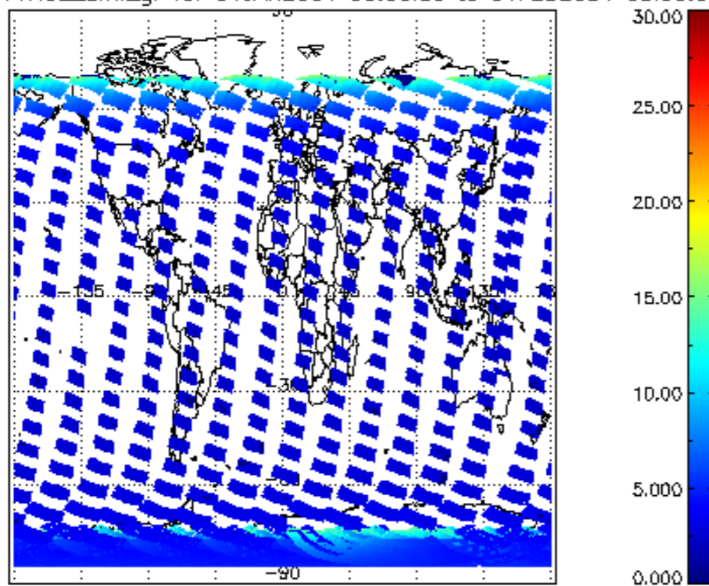
SCIOL2P_NADUV1NO2_amf_gr for 31JAN2004 00:00:00 to 01FEB2004 00:00:00
