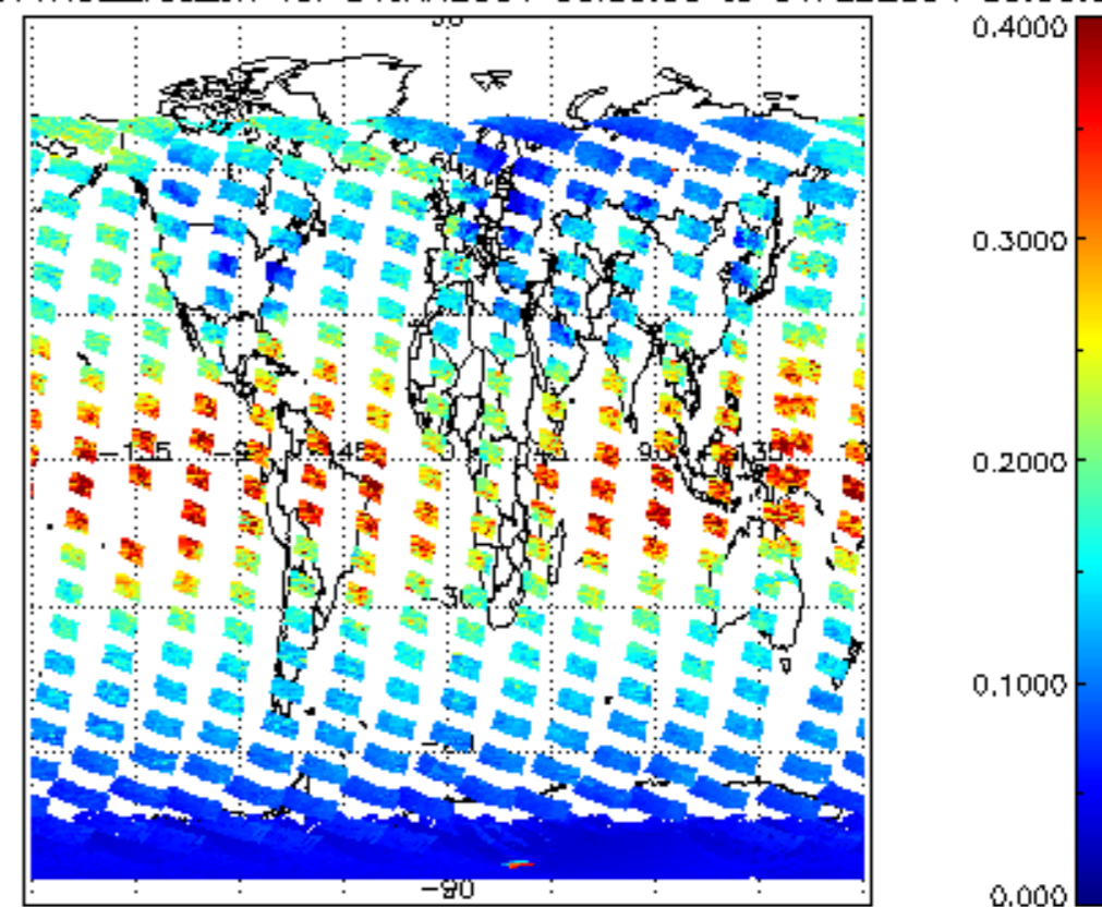
SCIOL2P_NADUV1NO2_vcd_err for 31JAN2004 00:00:00 to 01FEB2004 00:00:00
