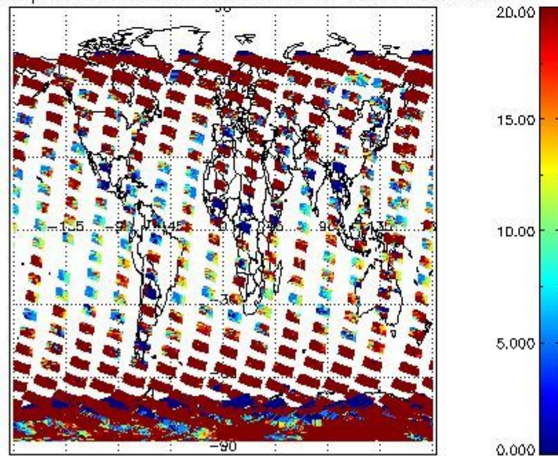
cLopt_depth for 31JAN2004 00:00:00 to 01FEB2004 00:00:00
