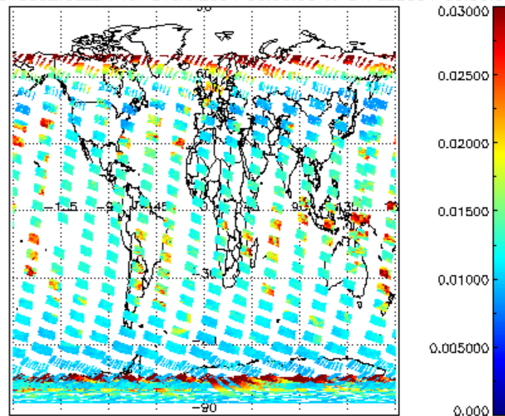
SCIOL2P_NADUV003_vcd_err for 31JAN2004 00:00:00 to 01FEB2004 00:00:00
