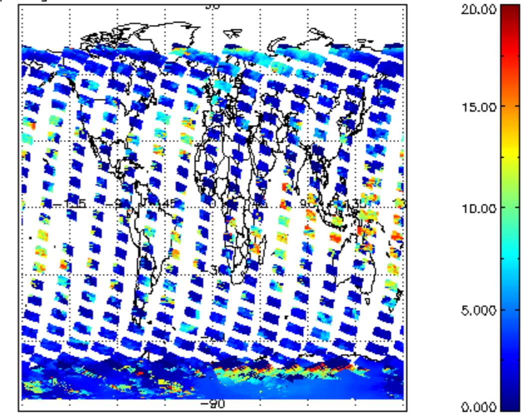
cl_top_height for 31JAN2004 00:00:00 to 01FEB2004 00:00:00
