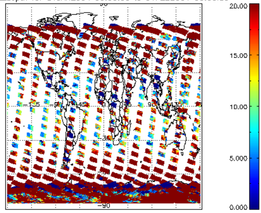
cl_opt_depth for 31JAN2004 00:00:00 to 01FEB2004 00:00:00
