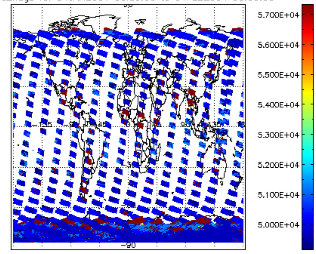
cloud_flags for 31JAN2004 00:00:00 to 01FEB2004 00:00:00
