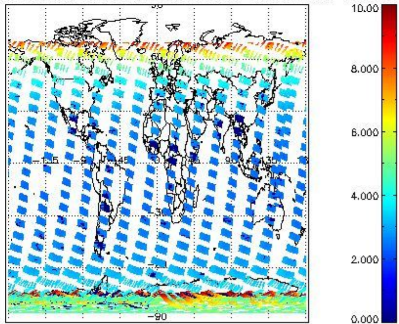
SCIOL2P_NADUV003_amf_cl for 31JAN2004 00:00:00 to 01FEB2004 00:00:00
