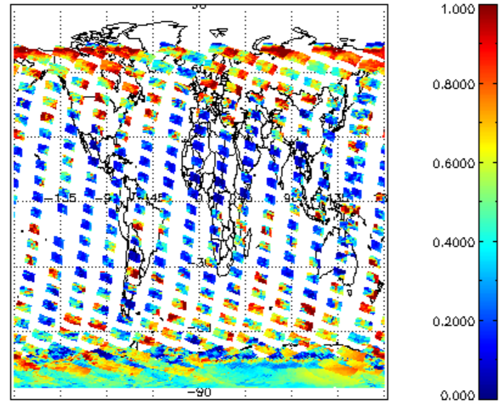
cl_frac for 31JAN2004 00:00:00 to 01FEB2004 00:00:00
