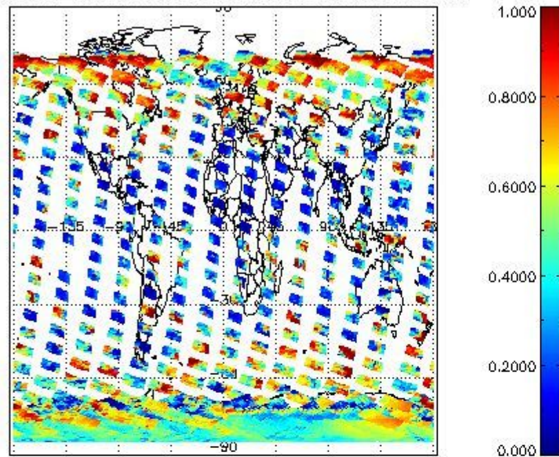
cLfrac for 31JAN2004 00:00:00 to 01FEB2004 00:00:00
