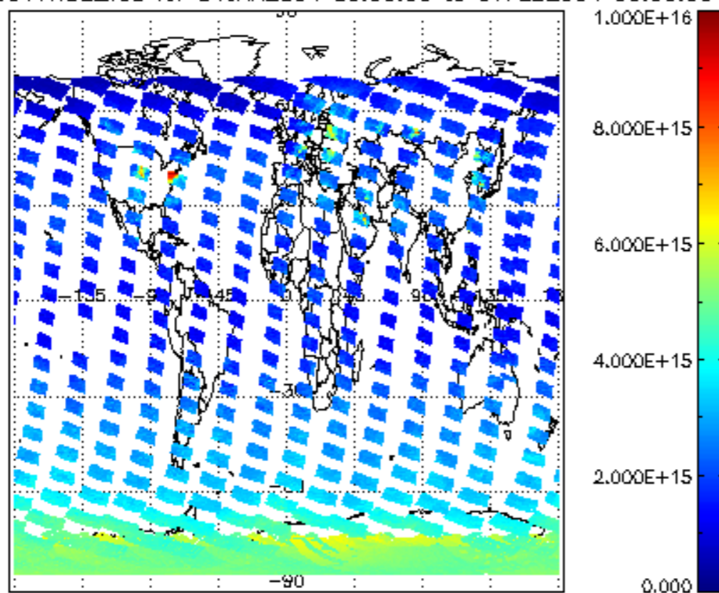
SCIOL2P_NADUV1NO2_vcd for 31JAN2004 00:00:00 to 01FEB2004 00:00:00
