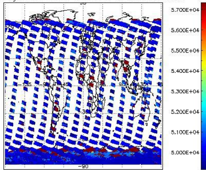
cloud_flags for 31JAN2004 00:00:00 to 01FEB2004 00:00:00
