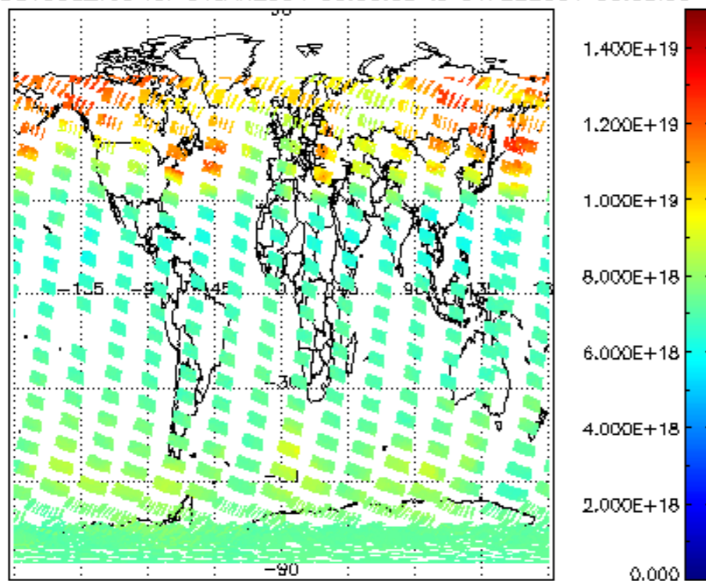
SCIOL2P_NADUV003_vcd for 31JAN2004 00:00:00 to 01FEB2004 00:00:00
