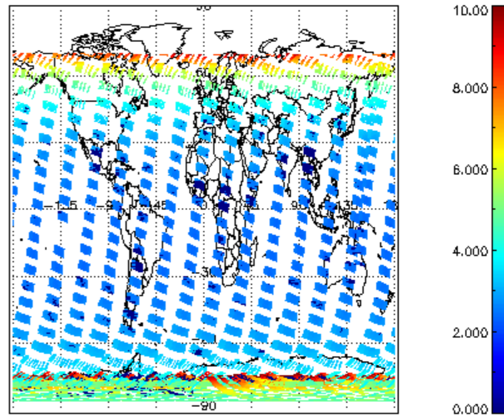
SCIOL2P_NADUV003_amf_cl for 31JAN2004 00:00:00 to 01FEB2004 00:00:00
