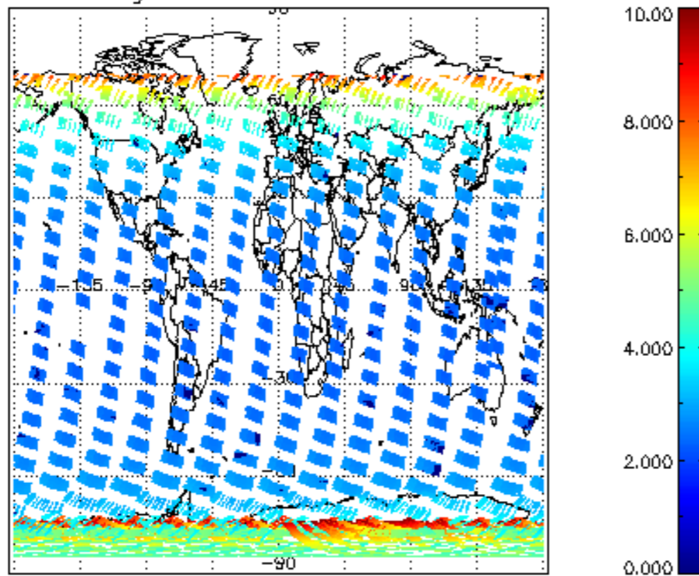
SCIOL2P_NADUV003_amf_gr for 31JAN2004 00:00:00 to 01FEB2004 00:00:00
