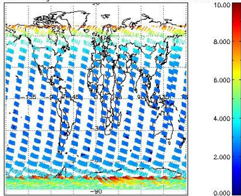
SCIOL2P_NADUV003_amf_gr for 31JAN2004 00:00:00 to 01FEB2004 00:00:00
