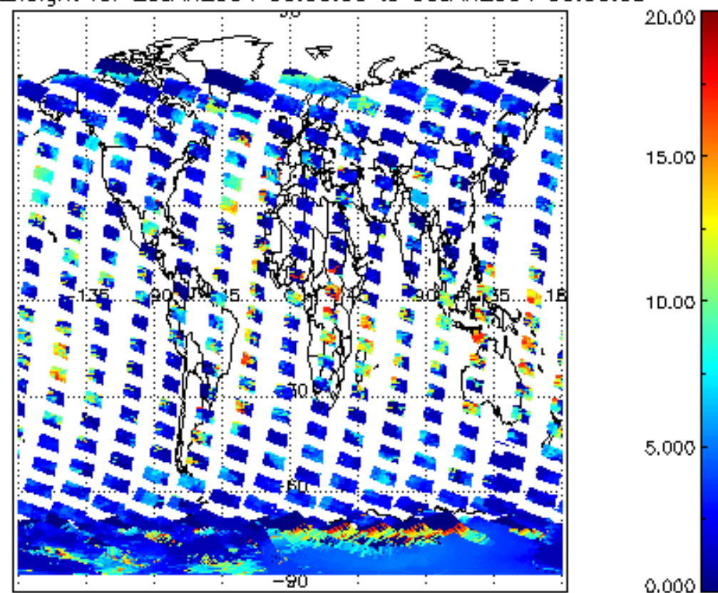
cL_top_height for 29JAN2004 00:00:00 to 30JAN2004 00:00:00
