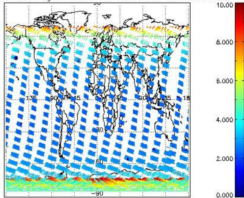
SCIOL2P_NADUV003_amf_gr for 29JAN2004 00:00:00 to 30JAN2004 00:00:00
