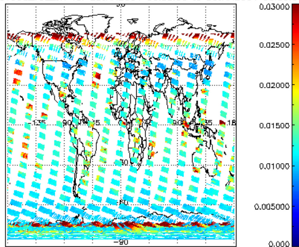
SCIOL2P_NADUV003_vcd_err for 29JAN2004 00:00:00 to 30JAN2004 00:00:00
