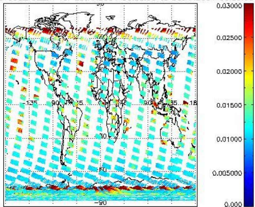
SCIOL2P_NADUV003_vcd_err for 29JAN2004 00:00:00 to 30JAN2004 00:00:00
