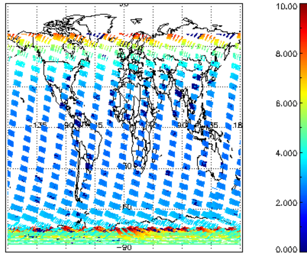
SCIOL2P_NADUV003_amf_cl for 29JAN2004 00:00:00 to 30JAN2004 00:00:00
