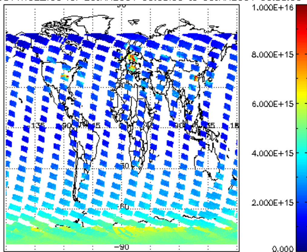
SCIOL2P_NADUV1NO2_vcd for 29JAN2004 00:00:00 to 30JAN2004 00:00:00
