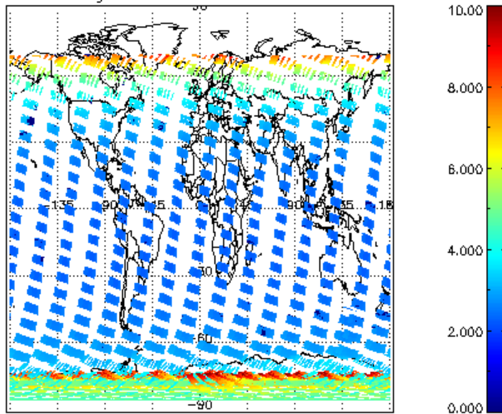
SCIOL2P_NADUV003_amf_gr for 29JAN2004 00:00:00 to 30JAN2004 00:00:00
