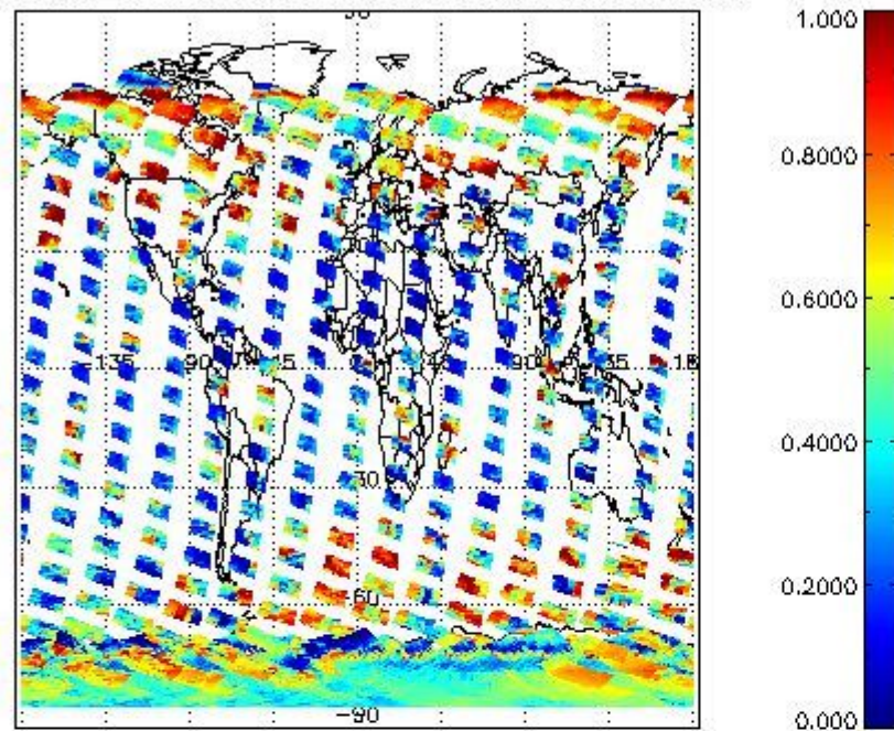
cL_frac for 29JAN2004 00:00:00 to 30JAN2004 00:00:00
