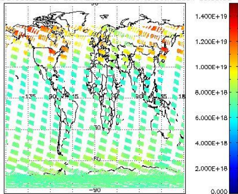
SCIOL2P_NADUV003_vcd for 29JAN2004 00:00:00 to 30JAN2004 00:00:00
