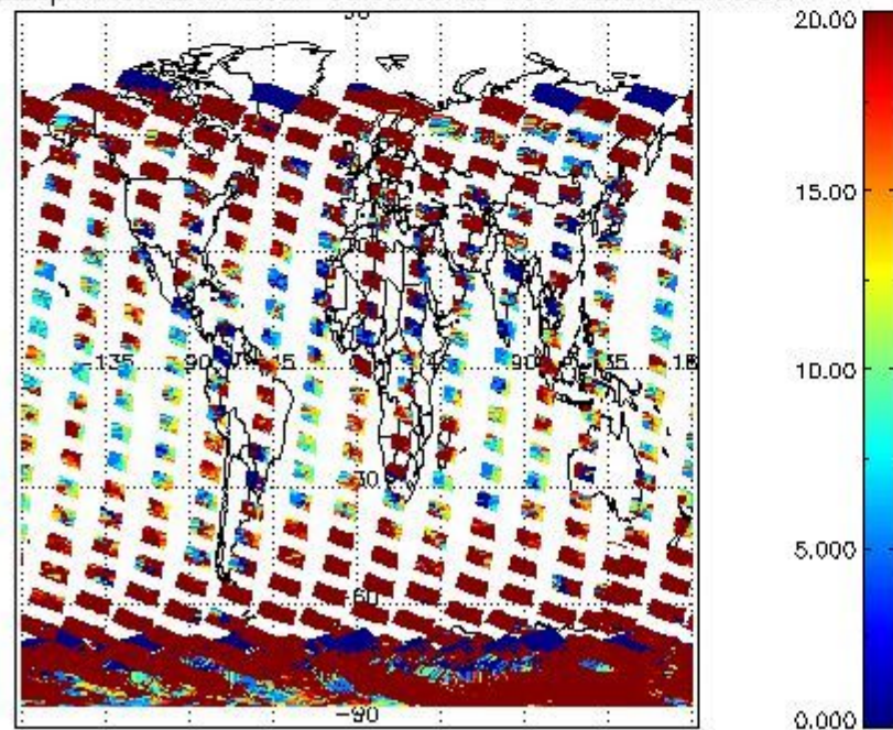
cLopt_depth for 29JAN2004 00:00:00 to 30JAN2004 00:00:00
