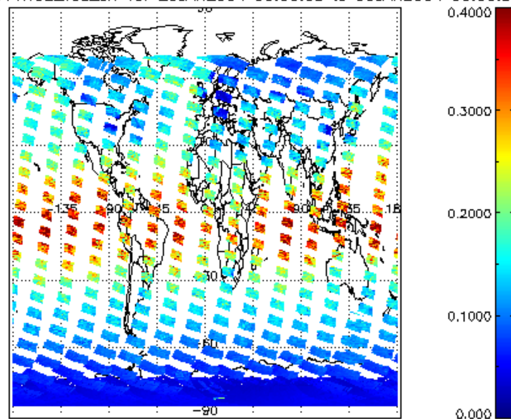
SCIOL2P_NADUV1NO2_vcd_err for 29JAN2004 00:00:00 to 30JAN2004 00:00:00
