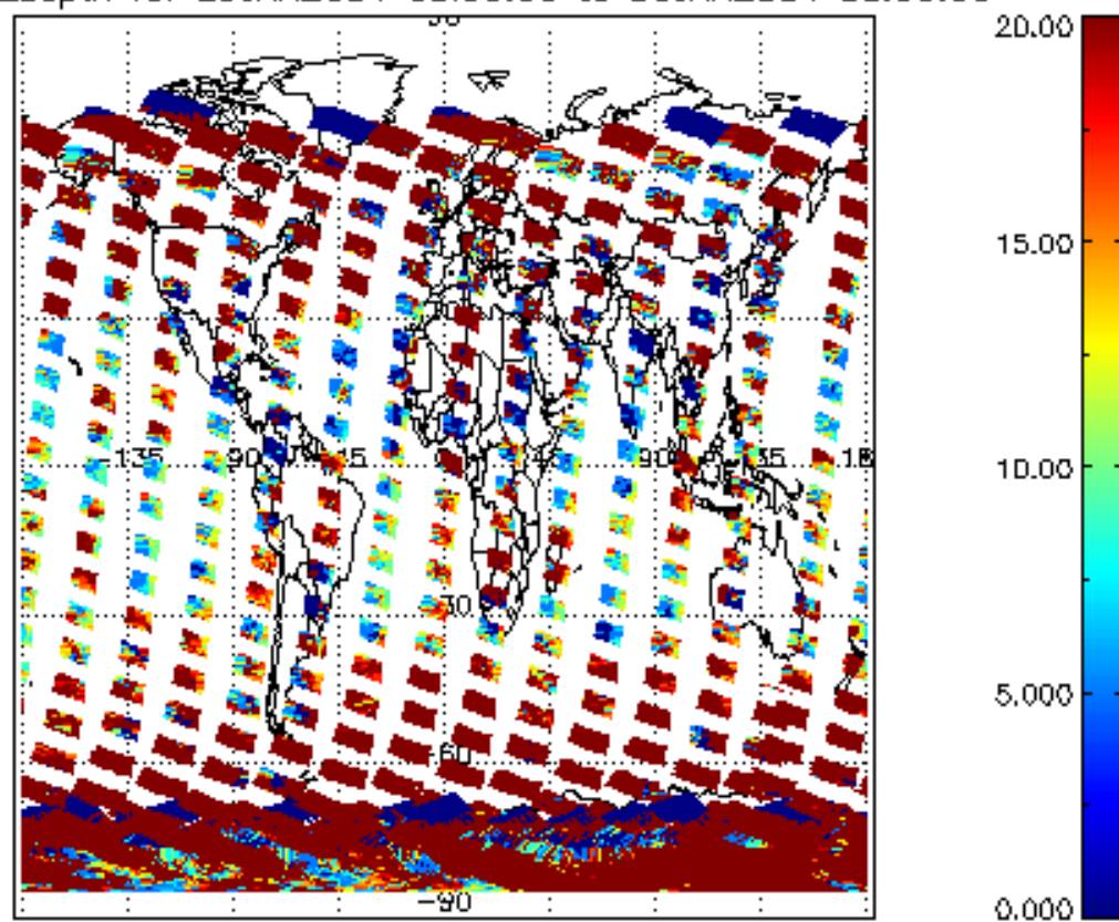
cLopt_depth for 29JAN2004 00:00:00 to 30JAN2004 00:00:00
