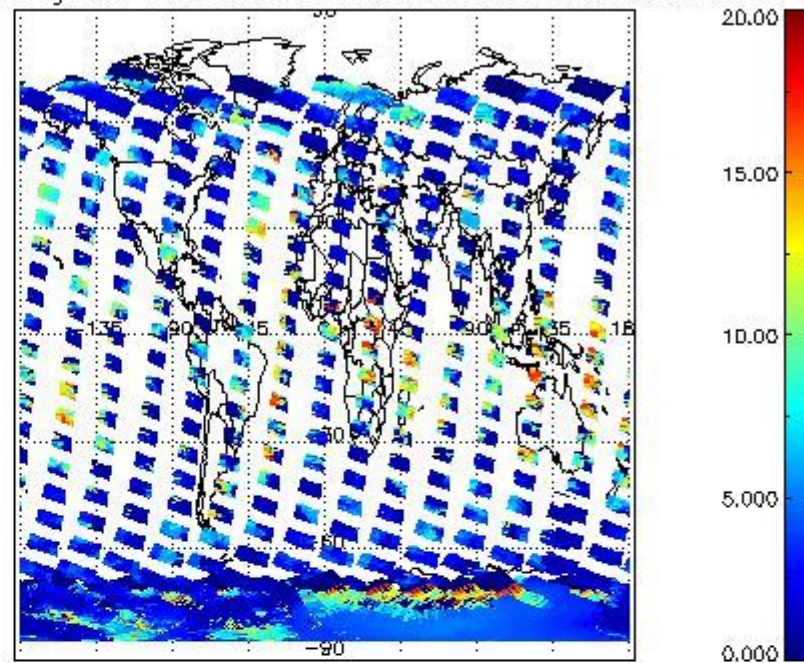
cL_top_height for 29JAN2004 00:00:00 to 30JAN2004 00:00:00
