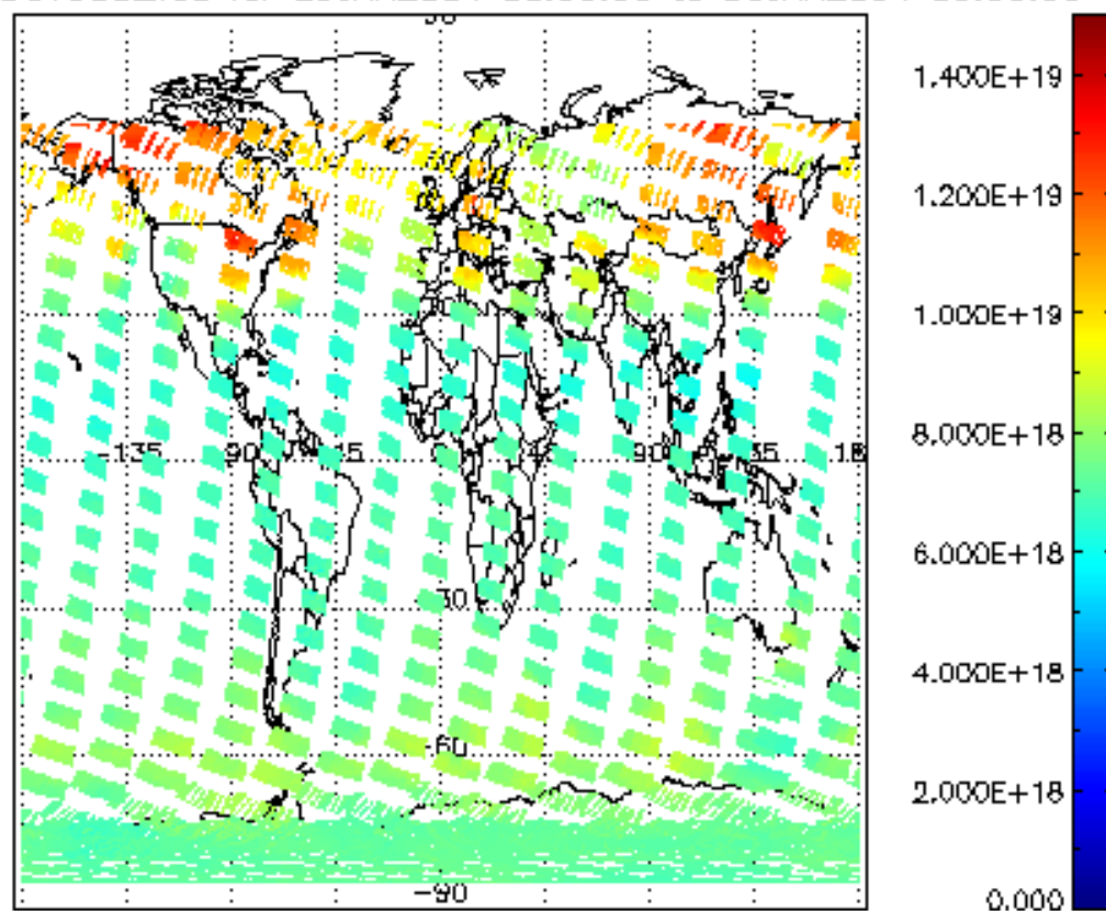
SCIOL2P_NADUV003_vcd for 29JAN2004 00:00:00 to 30JAN2004 00:00:00
