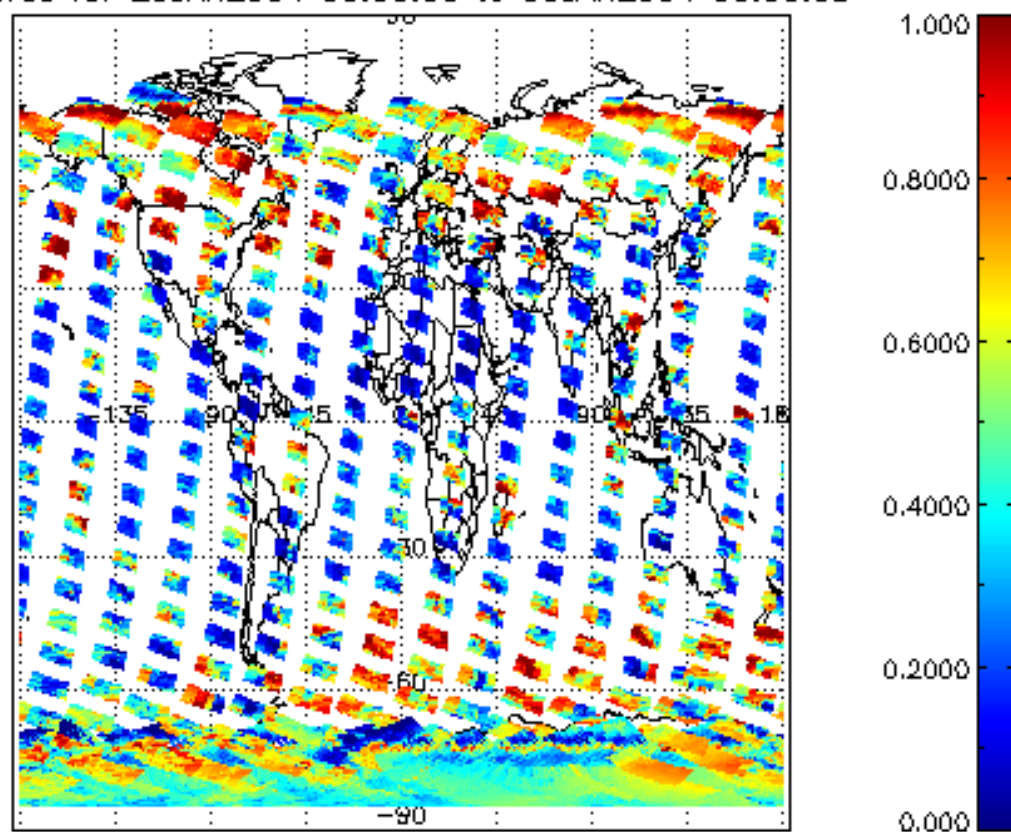
cL_frac for 29JAN2004 00:00:00 to 30JAN2004 00:00:00
