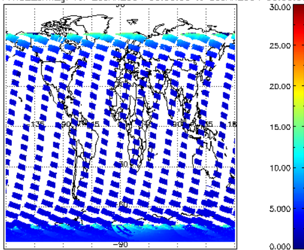
SCIOL2P_NADUV1NO2_amf_gr for 29JAN2004 00:00:00 to 30JAN2004 00:00:00
