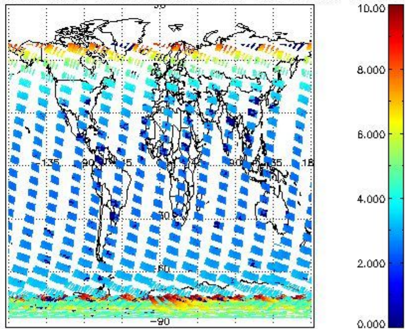
SCIOL2P_NADUV003_amf_cl for 29JAN2004 00:00:00 to 30JAN2004 00:00:00
