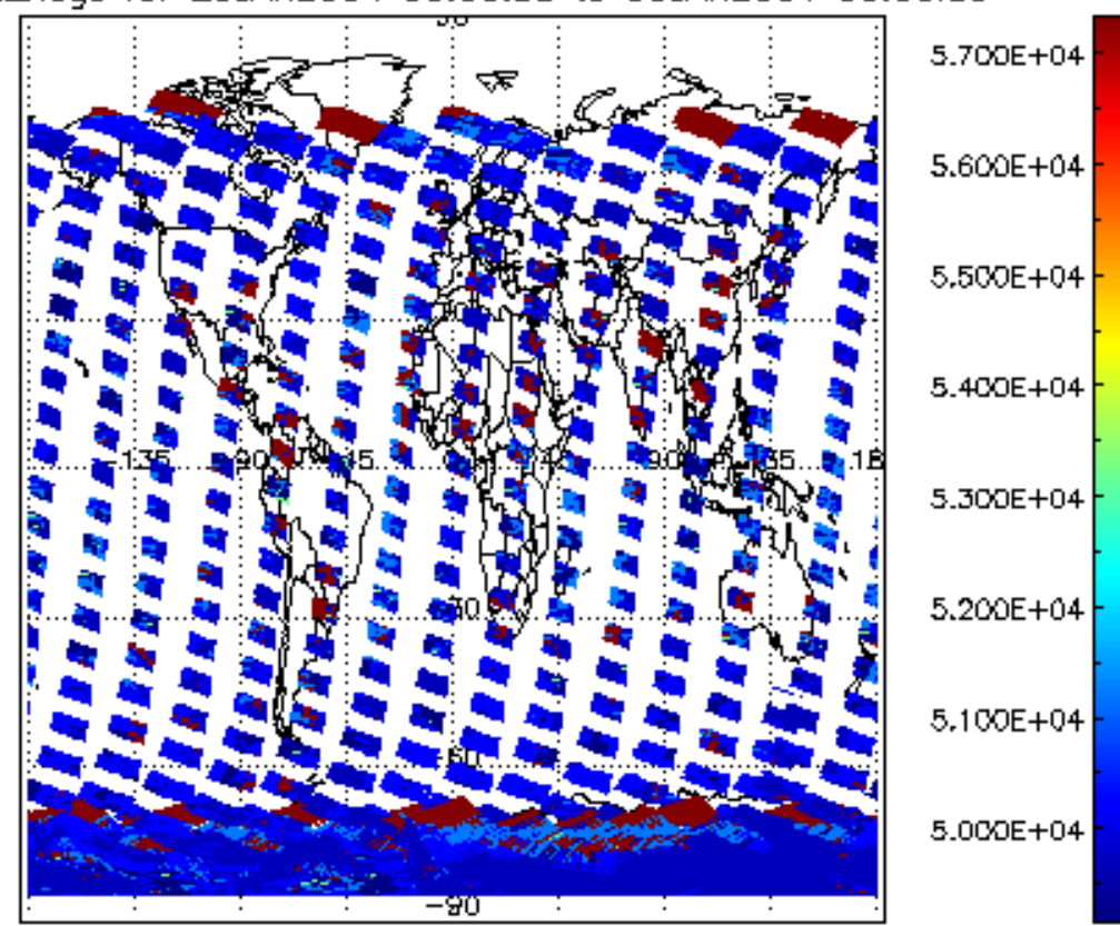
cloud_flags for 29JAN2004 00:00:00 to 30JAN2004 00:00:00
