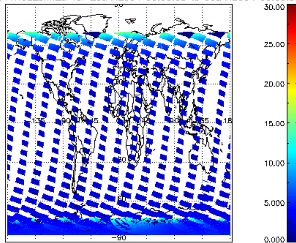
SCIOL2P_NADUV1NO2_amf_cl for 29JAN2004 00:00:00 to 30JAN2004 00:00:00
