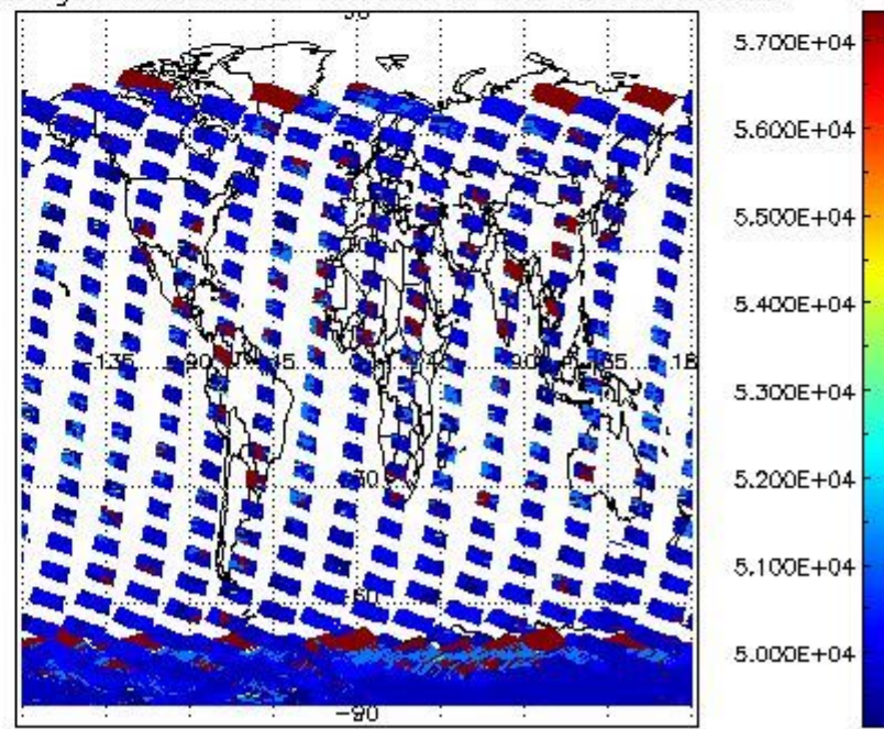
cloud_flags for 29JAN2004 00:00:00 to 30JAN2004 00:00:00
