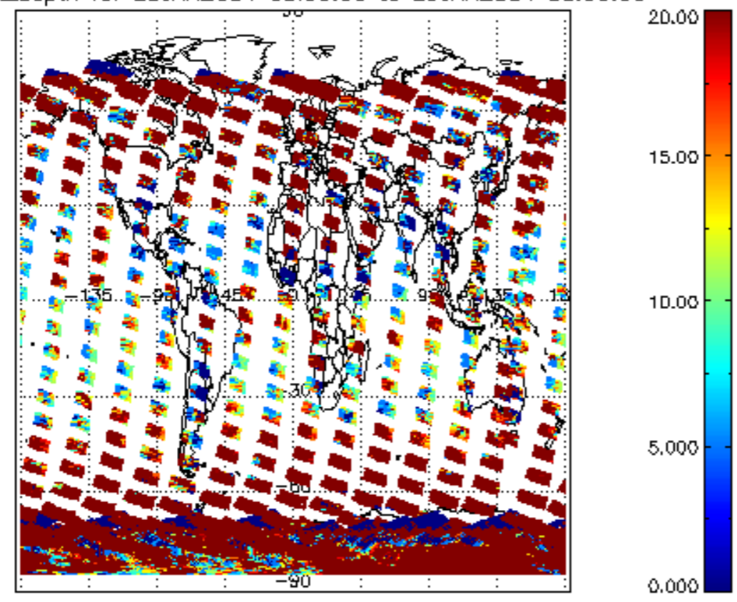
cL_opt_depth for 28JAN2004 00:00:00 to 29JAN2004 00:00:00
