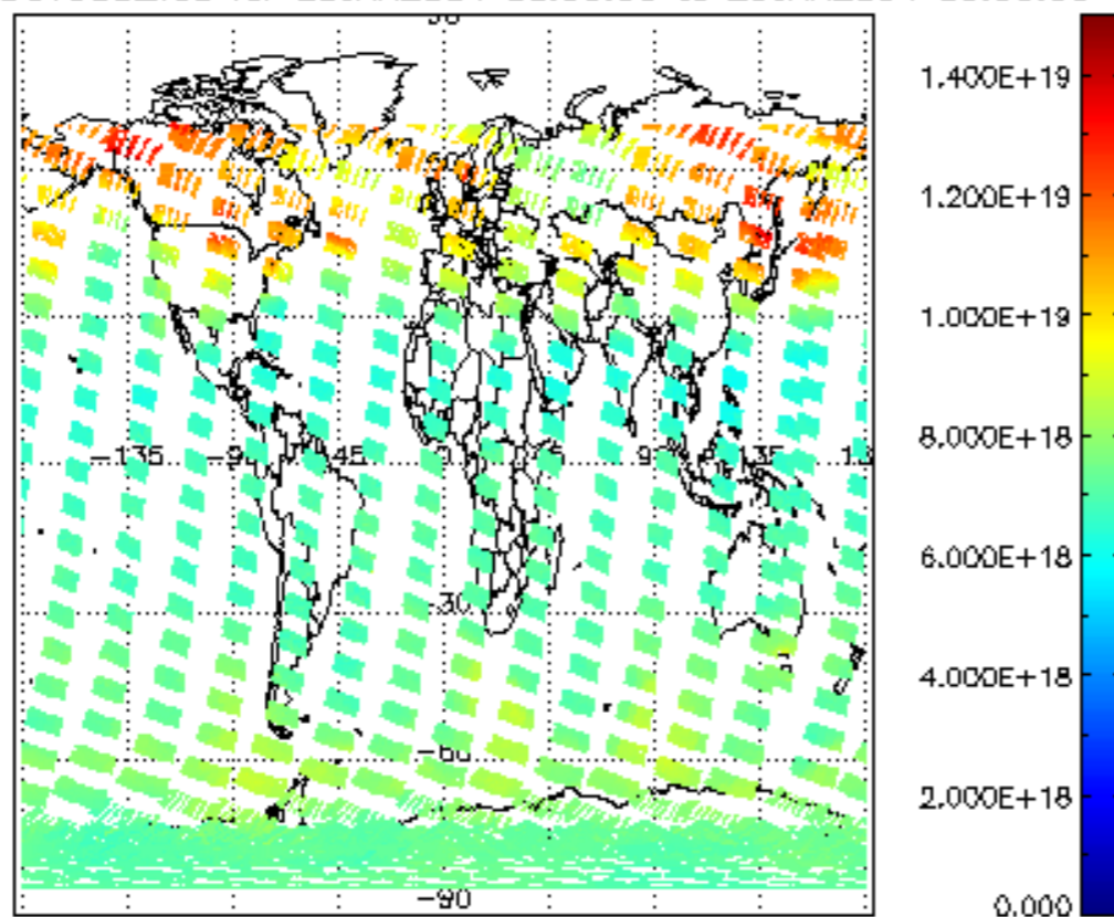
SCIOL2P_NADUV003_vcd for 28JAN2004 00:00:00 to 29JAN2004 00:00:00
