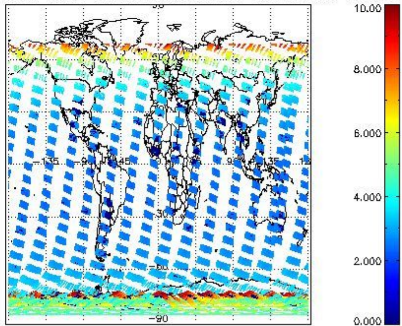
SCIOL2P_NADUV003_amf_cl for 28JAN2004 00:00:00 to 29JAN2004 00:00:00
