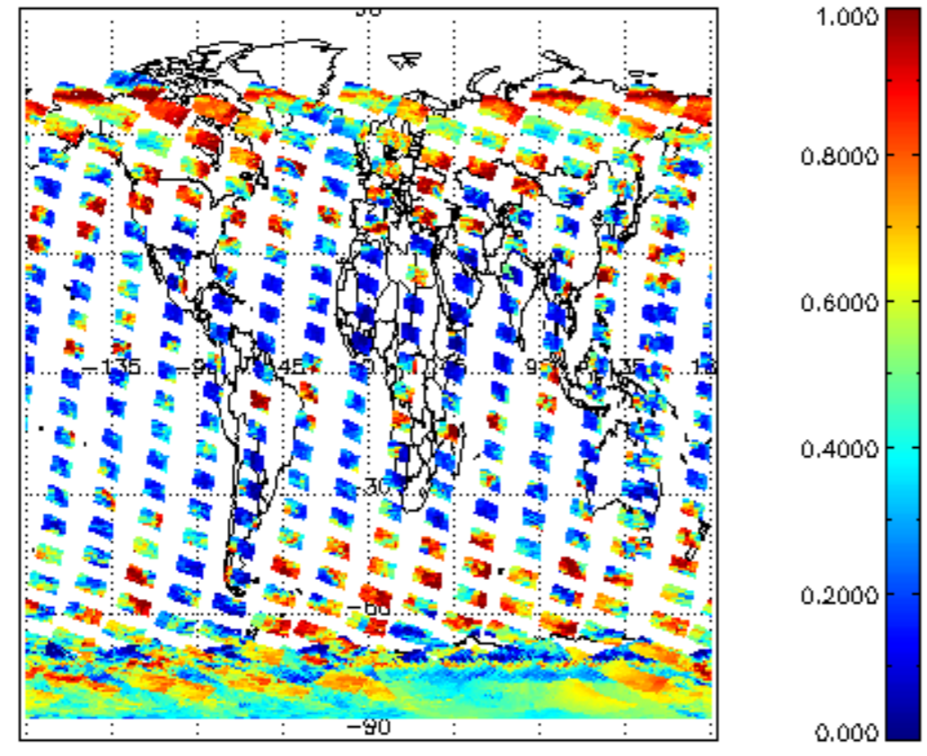
cL_frac for 28JAN2004 00:00:00 to 29JAN2004 00:00:00
