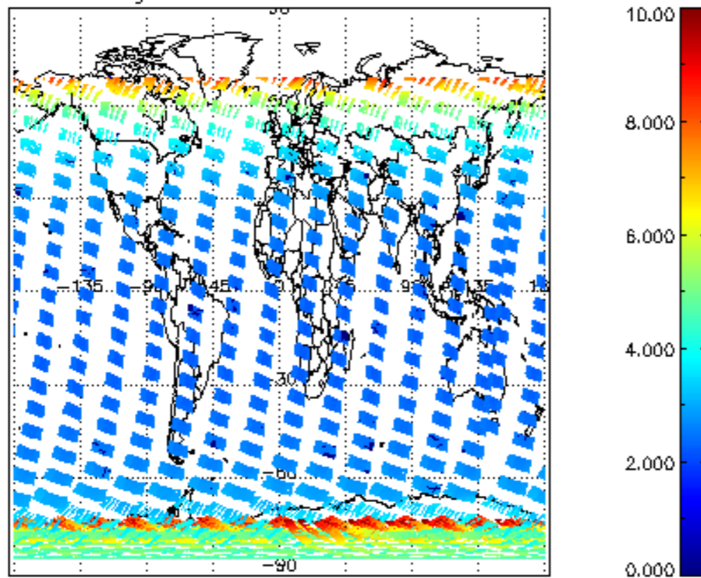
SCIOL2P_NADUV003_amf_gr for 28JAN2004 00:00:00 to 29JAN2004 00:00:00
