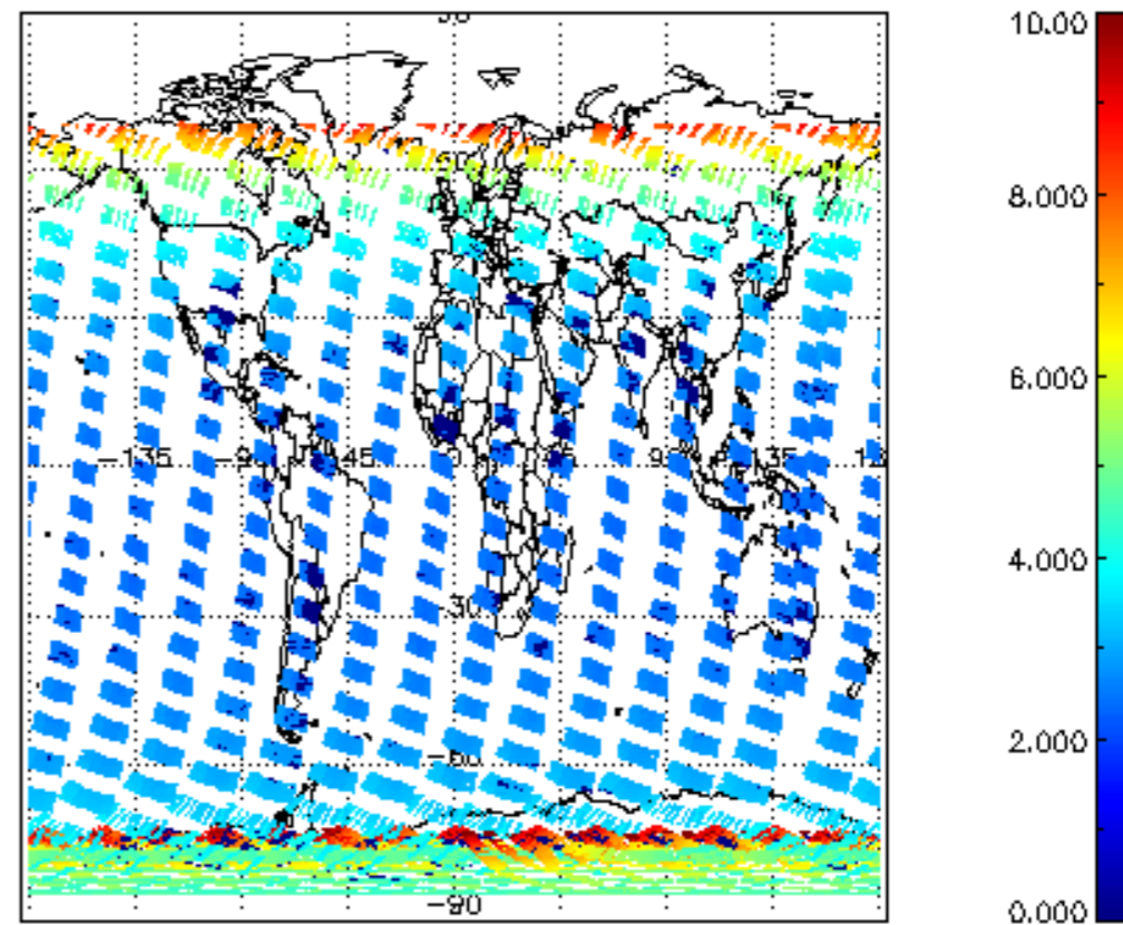
SCIOL2P_NADUV003_amf_cl for 28JAN2004 00:00:00 to 29JAN2004 00:00:00
