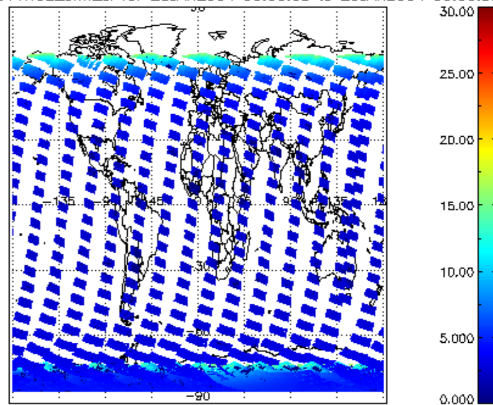
SCIOL2P_NADUV1NO2_amf_cl for 28JAN2004 00:00:00 to 29JAN2004 00:00:00
