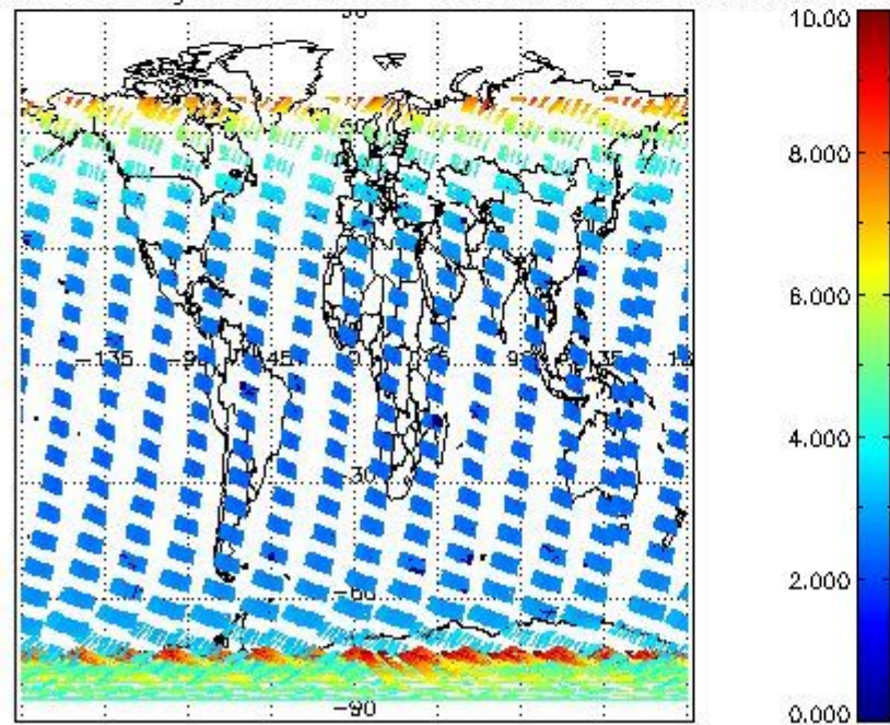
SCIOL2P_NADUV003_amf_gr for 28JAN2004 00:00:00 to 29JAN2004 00:00:00
