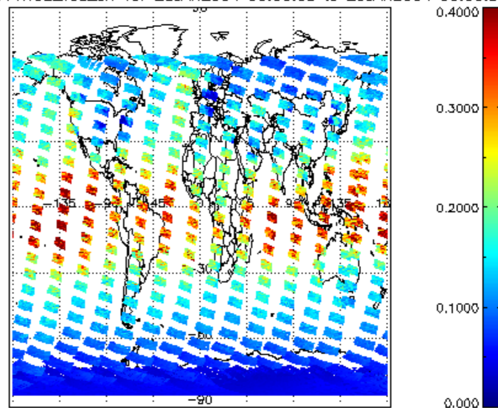
SCIOL2P_NADUV1NO2_vcd_err for 28JAN2004 00:00:00 to 29JAN2004 00:00:00
