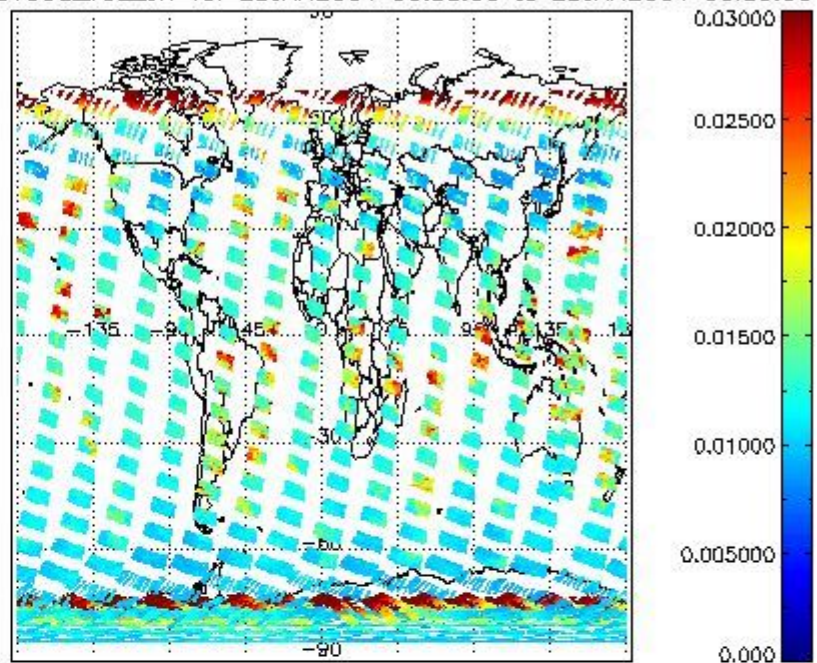
SCIOL2P_NADUV003_vcd_err for 28JAN2004 00:00:00 to 29JAN2004 00:00:00
