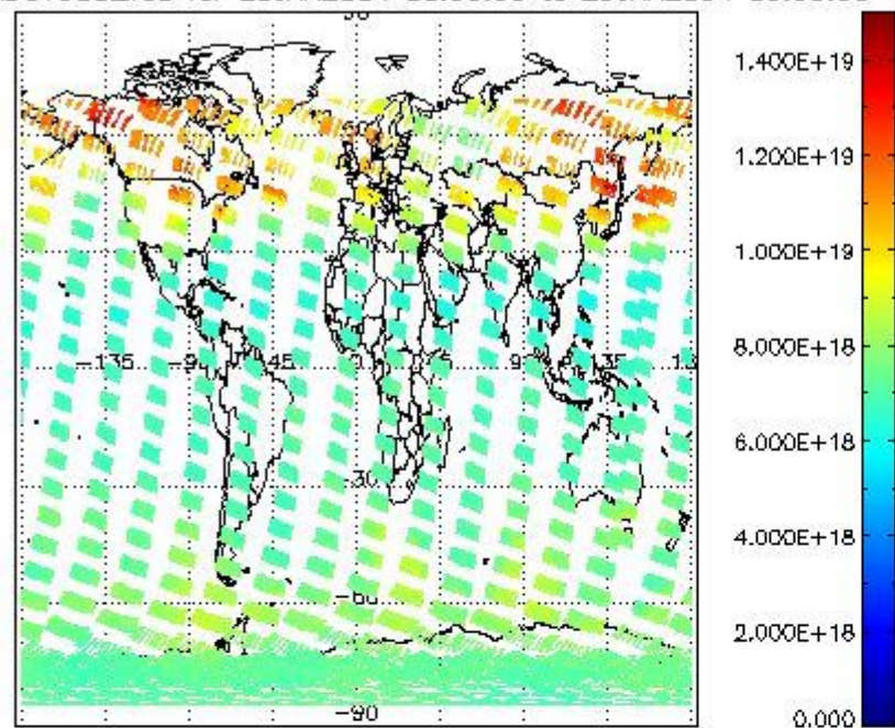
SCIOL2P_NADUV003_vcd for 28JAN2004 00:00:00 to 29JAN2004 00:00:00
