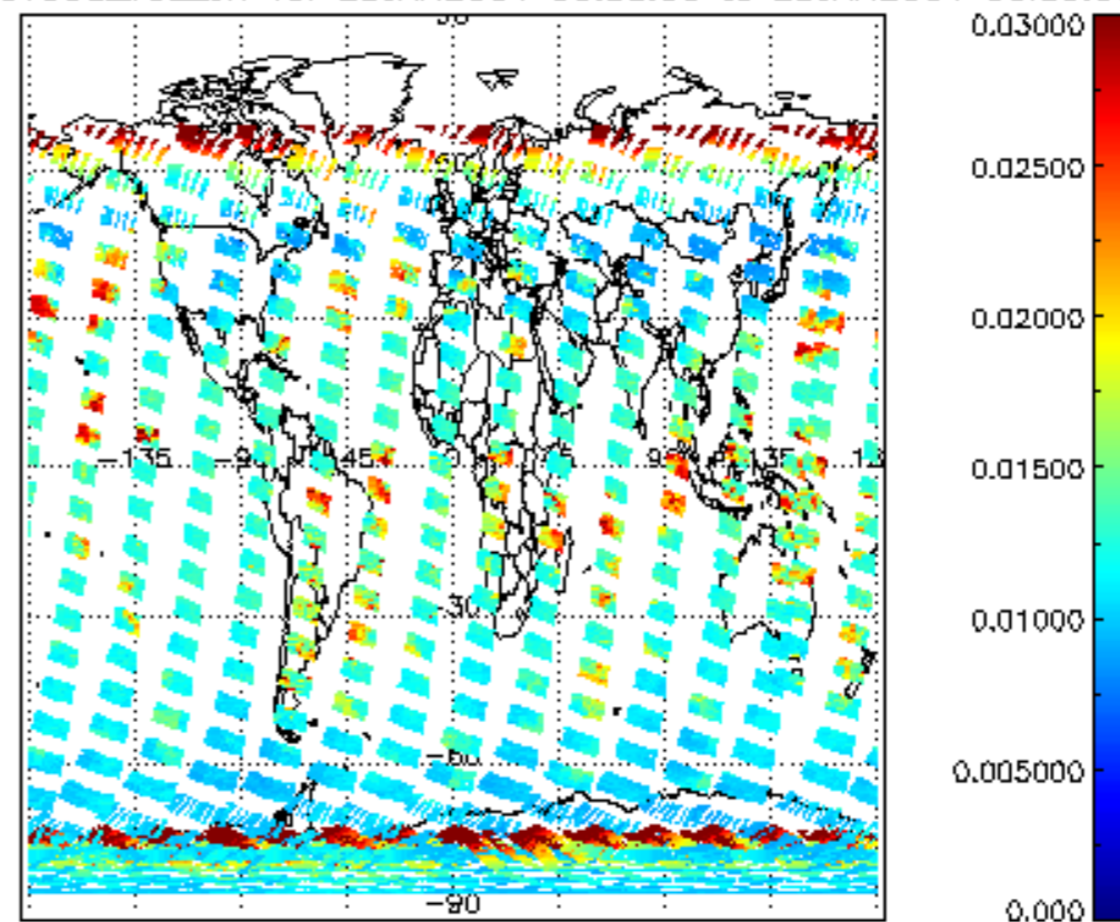
SCIOL2P_NADUV003_vcd_err for 28JAN2004 00:00:00 to 29JAN2004 00:00:00
