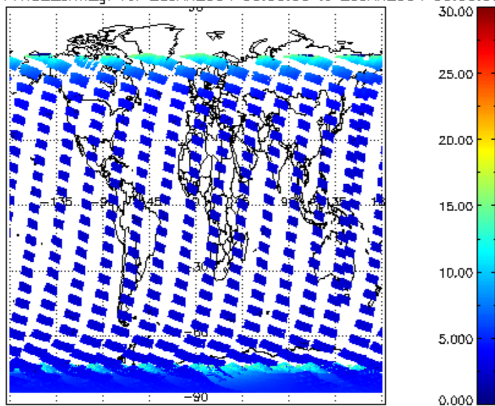
SCIOL2P_NADUV1NO2_amf_gr for 28JAN2004 00:00:00 to 29JAN2004 00:00:00
