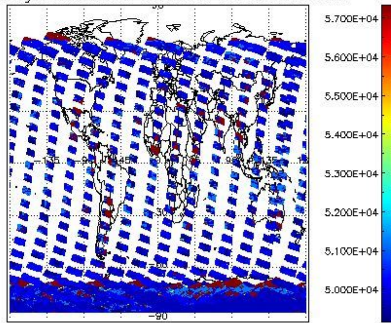
cloud_flags for 28JAN2004 00:00:00 to 29JAN2004 00:00:00
