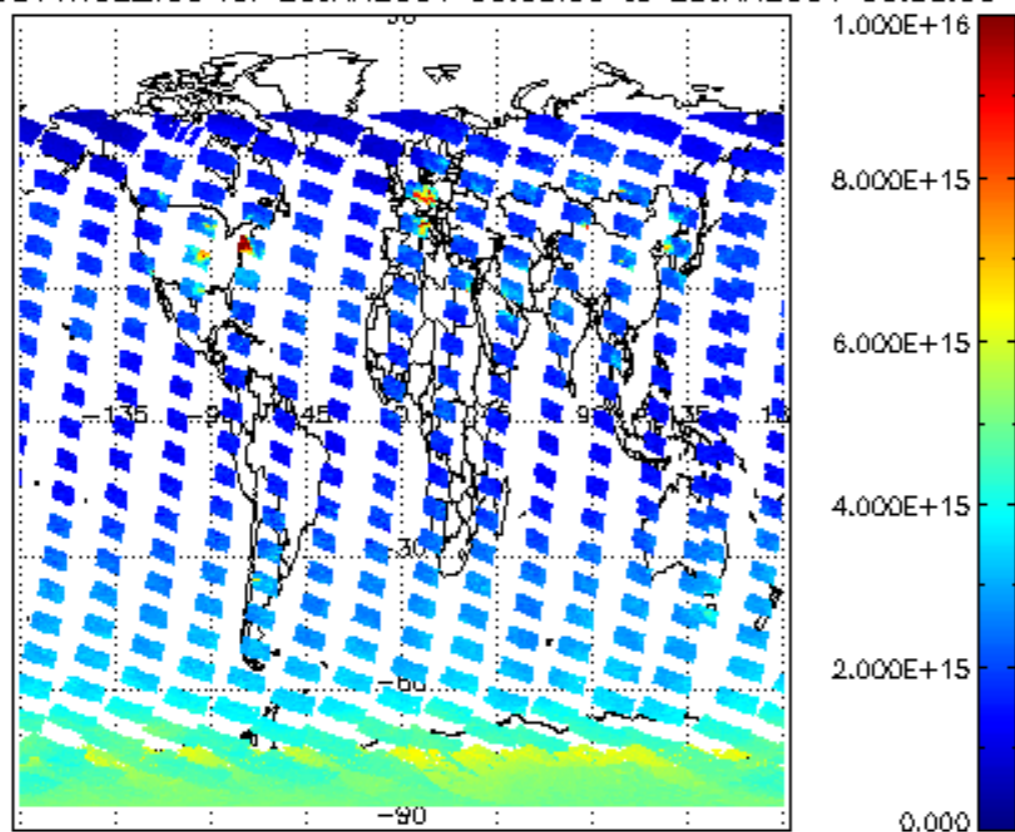
SCIOL2P_NADUV1NO2_vcd for 28JAN2004 00:00:00 to 29JAN2004 00:00:00
