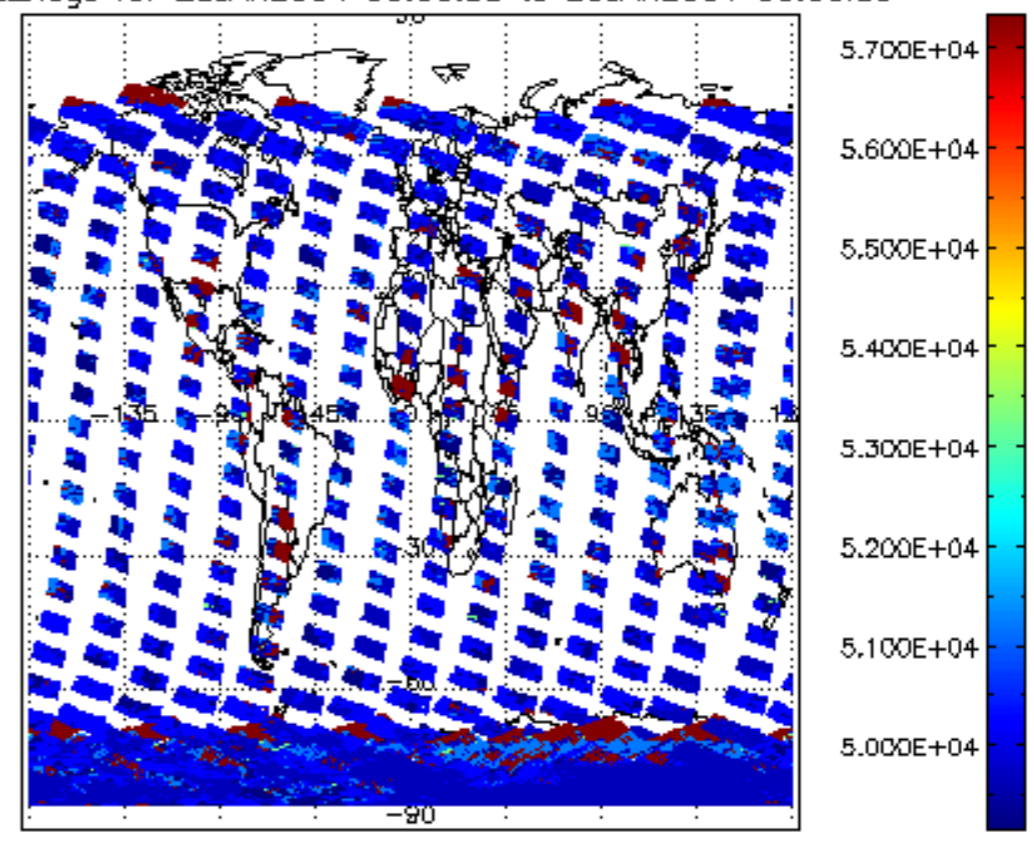
cloud_flags for 28JAN2004 00:00:00 to 29JAN2004 00:00:00
