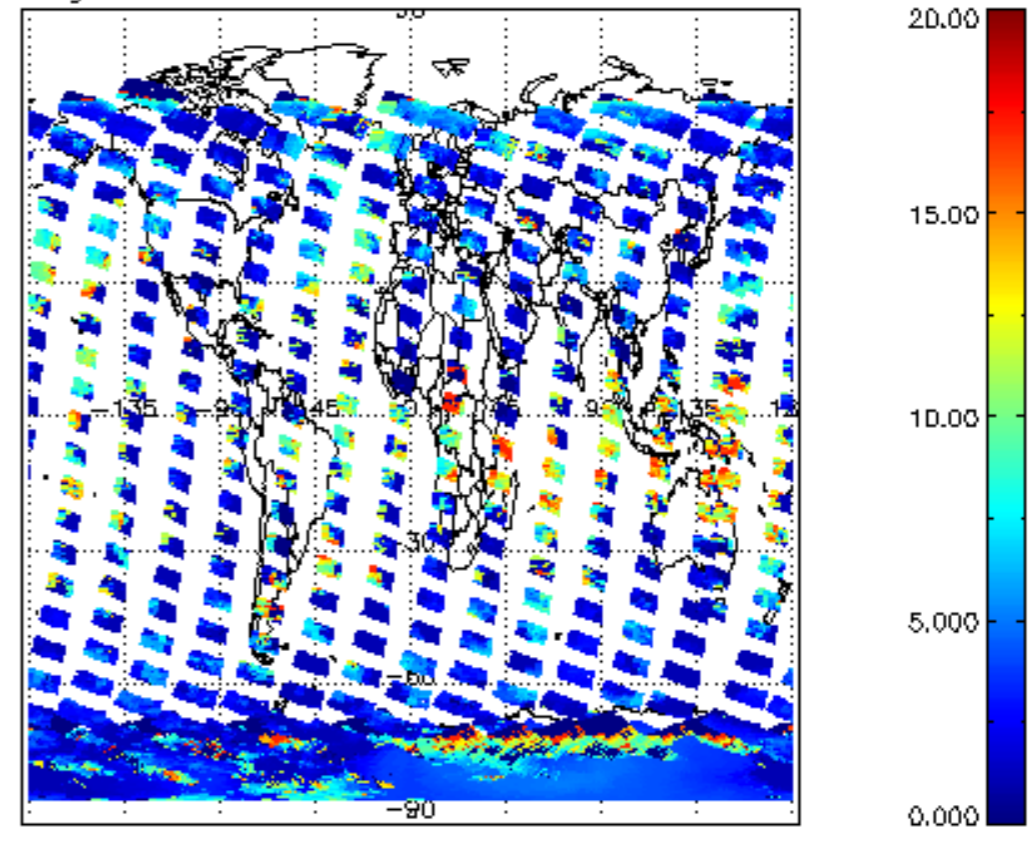
cL_top_height for 28JAN2004 00:00:00 to 29JAN2004 00:00:00
