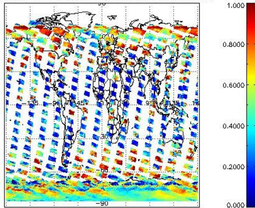
cL_frac for 28JAN2004 00:00:00 to 29JAN2004 00:00:00
