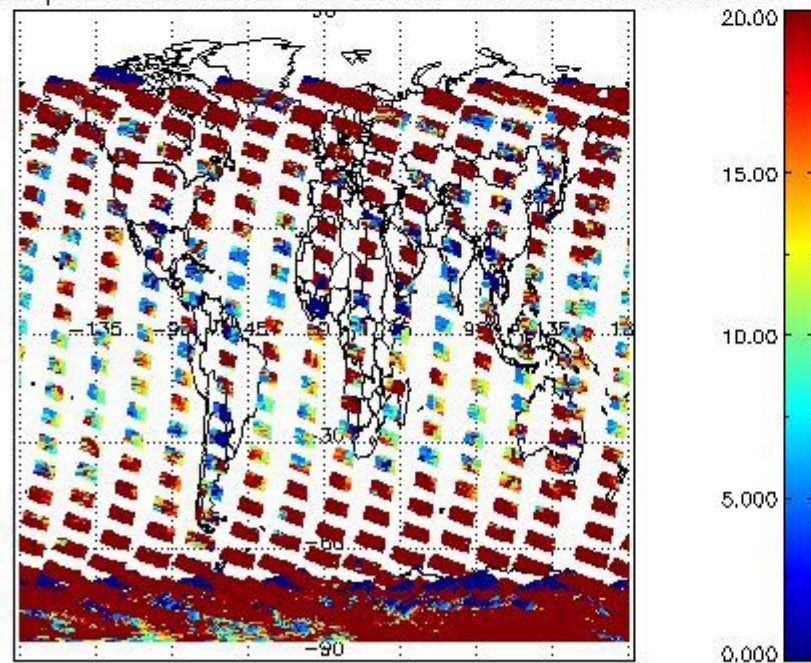
cLopt_depth for 28JAN2004 00:00:00 to 29JAN2004 00:00:00
