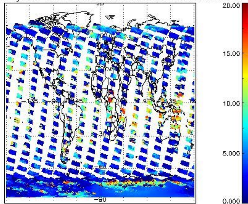
cL_top_height for 28JAN2004 00:00:00 to 29JAN2004 00:00:00
