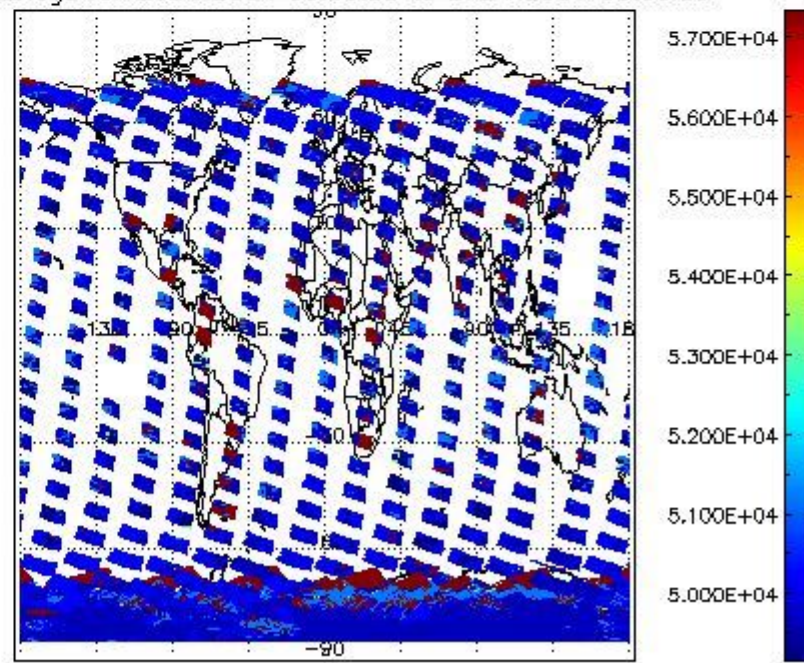
cloud_flags for 26JAN2004 00:00:00 to 27JAN2004 00:00:00
