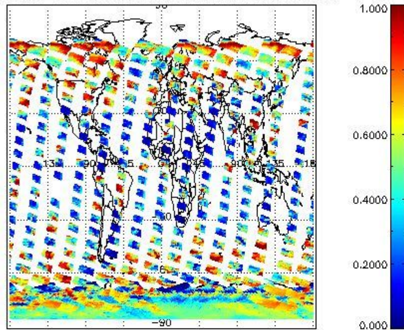
cL_frac for 26JAN2004 00:00:00 to 27JAN2004 00:00:00
