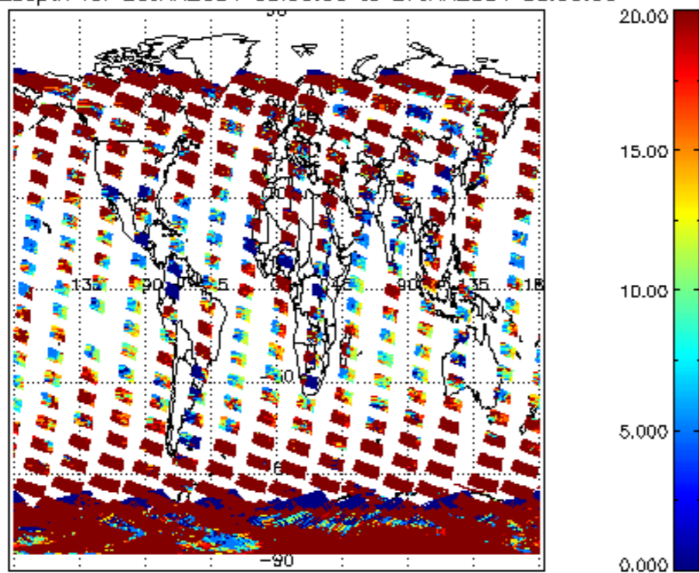
cLopt_depth for 26JAN2004 00:00:00 to 27JAN2004 00:00:00
