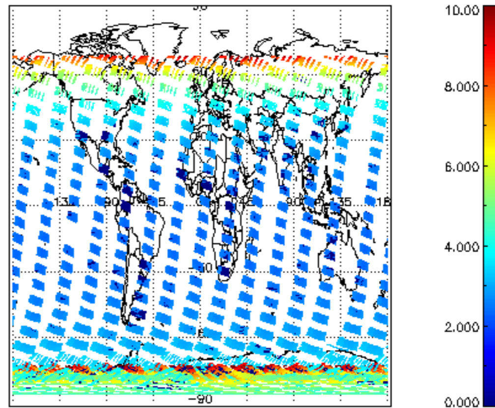
SCIOL2P_NADUV003_amf_cl for 26JAN2004 00:00:00 to 27JAN2004 00:00:00
