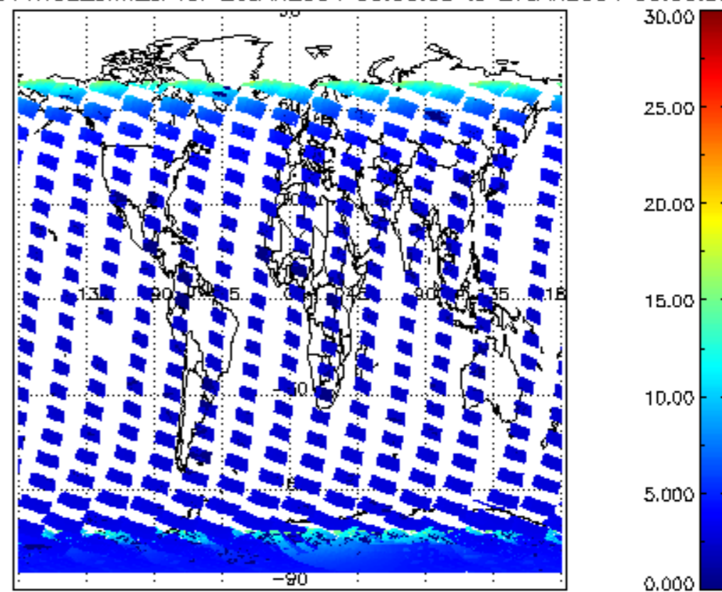
SCIOL2P_NADUV1NO2_amf_cl for 26JAN2004 00:00:00 to 27JAN2004 00:00:00
