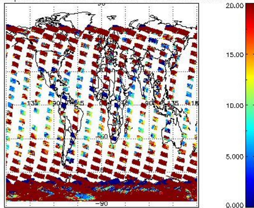
cLopt_depth for 26JAN2004 00:00:00 to 27JAN2004 00:00:00
