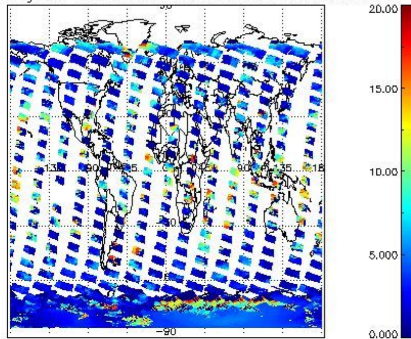
cL_top_height for 26JAN2004 00:00:00 to 27JAN2004 00:00:00
