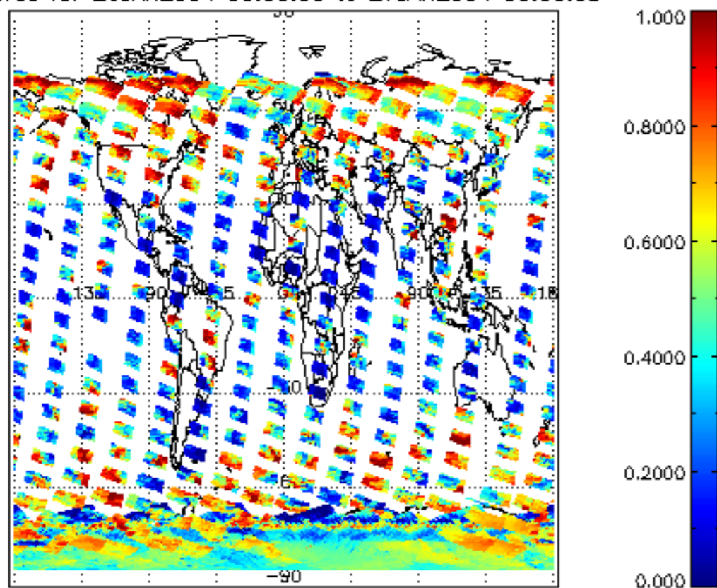
cL_frac for 26JAN2004 00:00:00 to 27JAN2004 00:00:00
