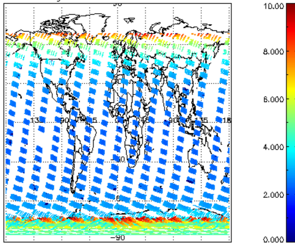
SCIOL2P_NADUV003_amf_gr for 26JAN2004 00:00:00 to 27JAN2004 00:00:00
