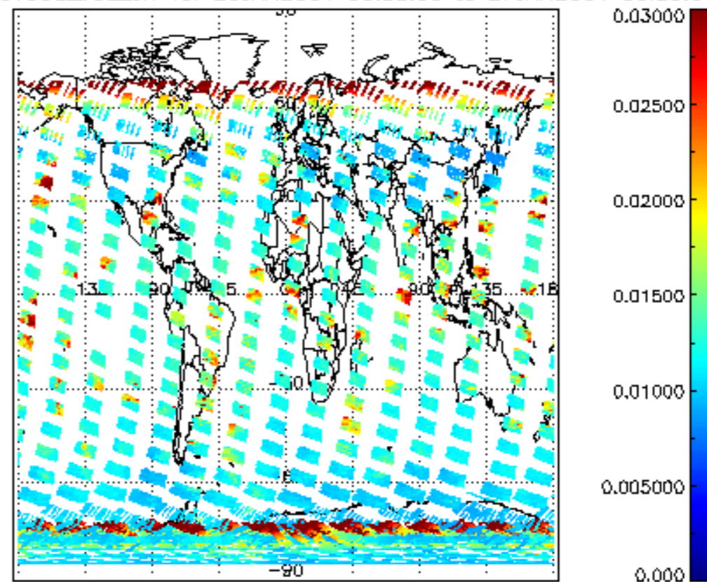
SCIOL2P_NADUV003_vcd_err for 26JAN2004 00:00:00 to 27JAN2004 00:00:00
