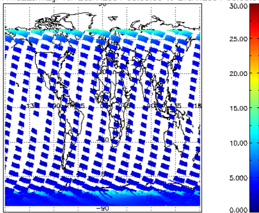
SCIOL2P_NADUV1NO2_amf_gr for 26JAN2004 00:00:00 to 27JAN2004 00:00:00
