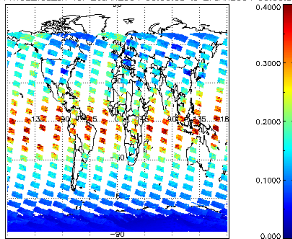
SCIOL2P_NADUV1NO2_vcd_err for 26JAN2004 00:00:00 to 27JAN2004 00:00:00
