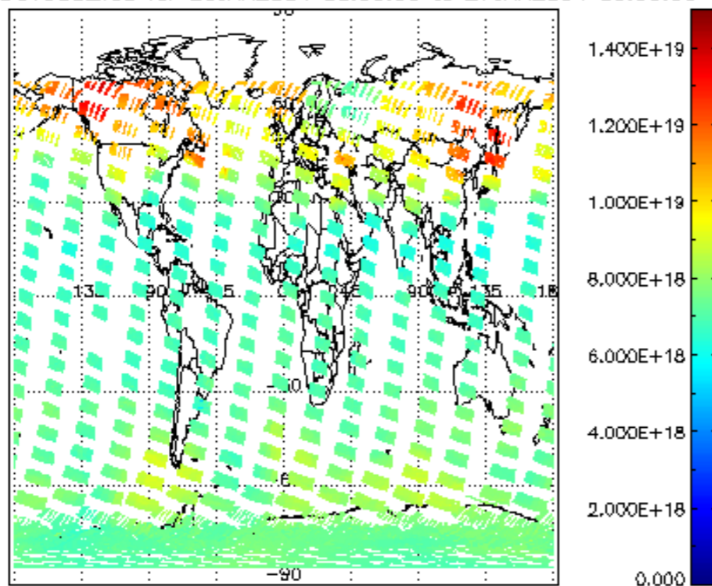
SCIOL2P_NADUV003_vcd for 26JAN2004 00:00:00 to 27JAN2004 00:00:00
