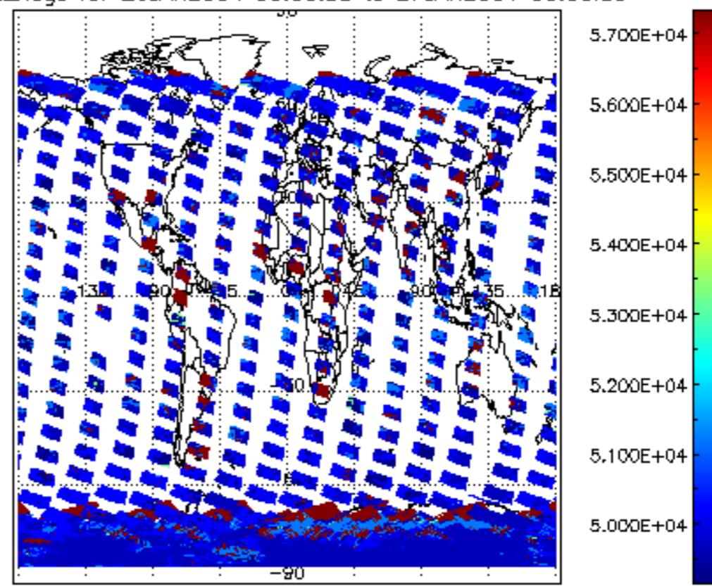
cloud_flags for 26JAN2004 00:00:00 to 27JAN2004 00:00:00
