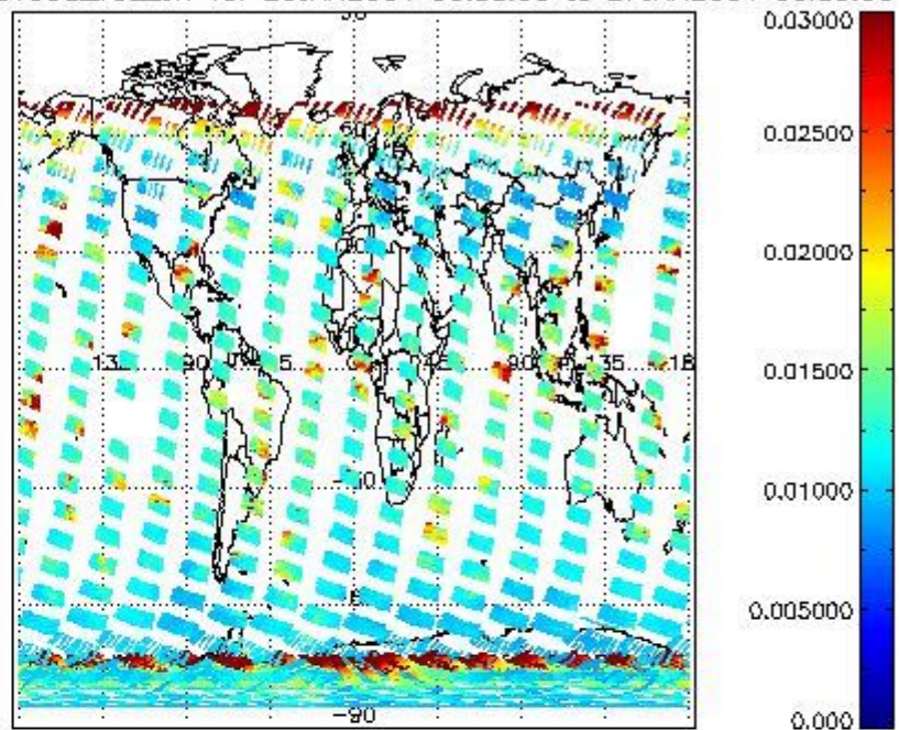
SCIOL2P_NADUV003_vcd_err for 26JAN2004 00:00:00 to 27JAN2004 00:00:00
