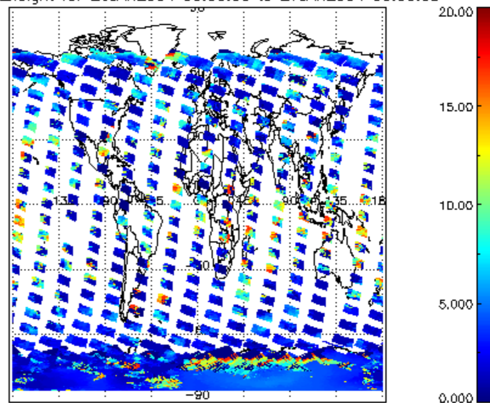
cL_top_height for 26JAN2004 00:00:00 to 27JAN2004 00:00:00
