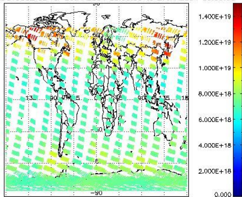
SCIOL2P_NADUV003_vcd for 26JAN2004 00:00:00 to 27JAN2004 00:00:00
