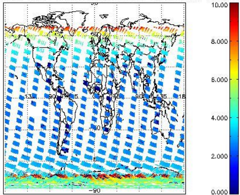
SCIOL2P_NADUV003_amf_cl for 26JAN2004 00:00:00 to 27JAN2004 00:00:00
