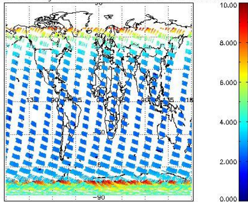
SCIOL2P_NADUV003_amf_gr for 26JAN2004 00:00:00 to 27JAN2004 00:00:00
