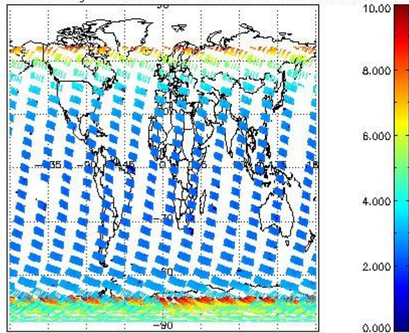
SCIOL2P_NADUV003_amf_gr for 24JAN2004 00:00:00 to 25JAN2004 00:00:00
