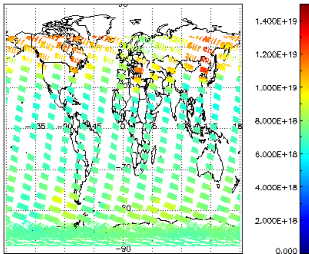
SCIOL2P_NADUV003_vcd for 24JAN2004 00:00:00 to 25JAN2004 00:00:00
