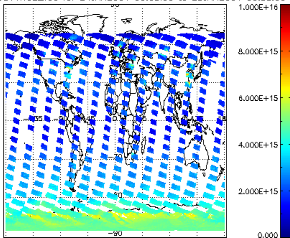
SCIOL2P_NADUV1NO2_vcd for 24JAN2004 00:00:00 to 25JAN2004 00:00:00
