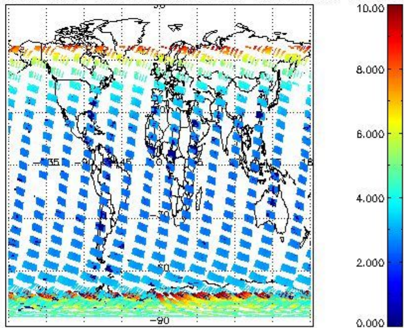
SCIOL2P_NADUV003_amf_cl for 24JAN2004 00:00:00 to 25JAN2004 00:00:00
