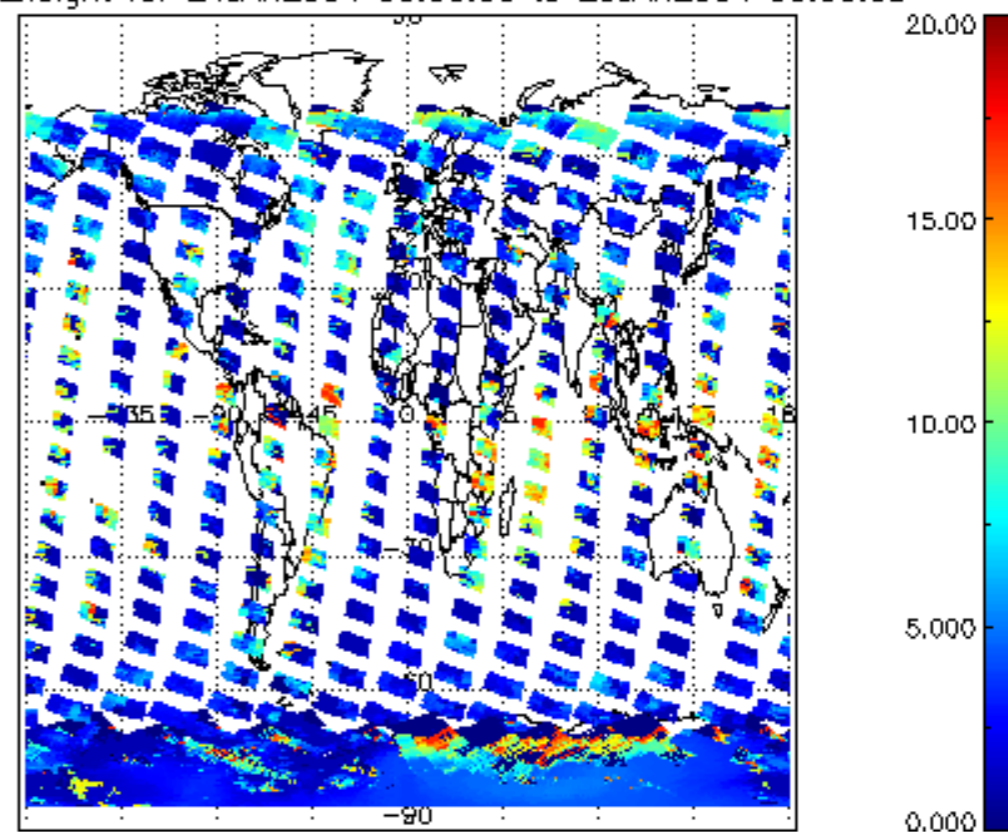
cL_top_height for 24JAN2004 00:00:00 to 25JAN2004 00:00:00
