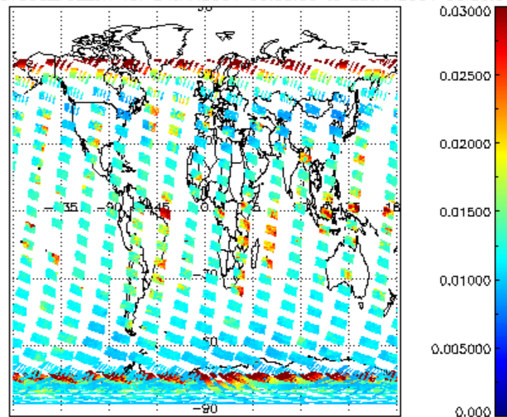
SCIOL2P_NADUV003_vcd_err for 24JAN2004 00:00:00 to 25JAN2004 00:00:00
