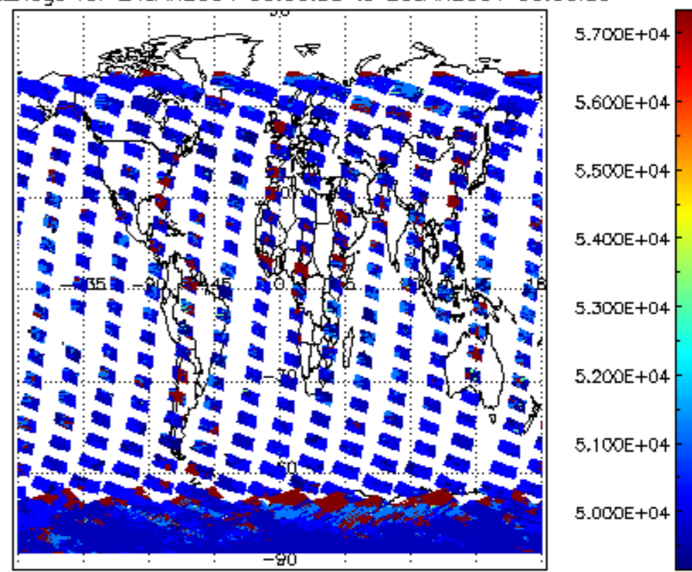
cloud_flags for 24JAN2004 00:00:00 to 25JAN2004 00:00:00
