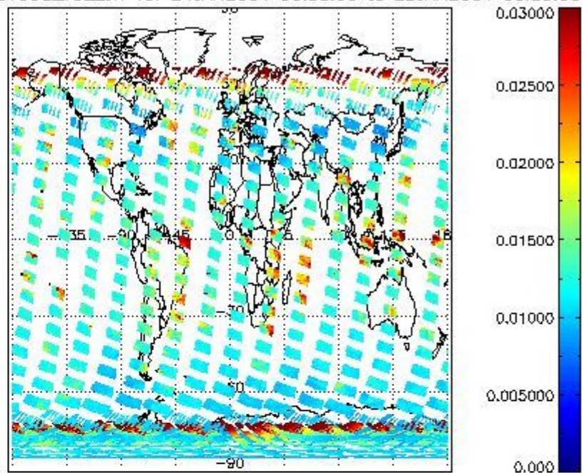
SCIOL2P_NADUV003_vcd_err for 24JAN2004 00:00:00 to 25JAN2004 00:00:00
