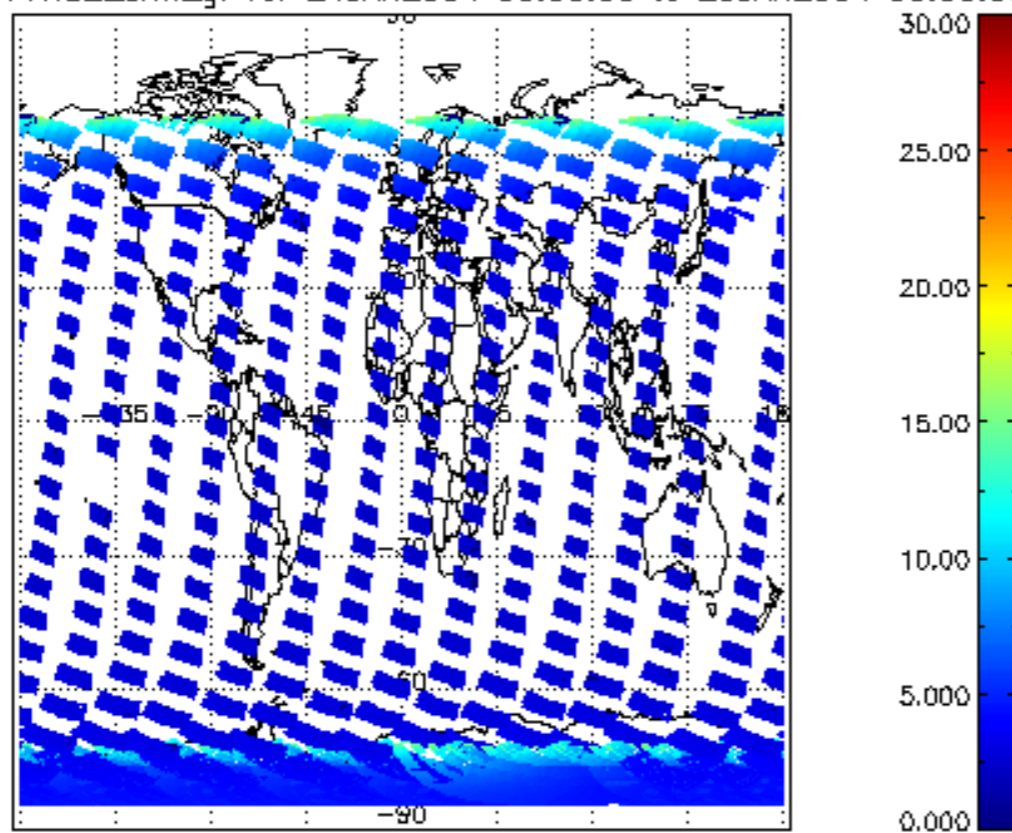
SCIOL2P_NADUV1NO2_amf_gr for 24JAN2004 00:00:00 to 25JAN2004 00:00:00
