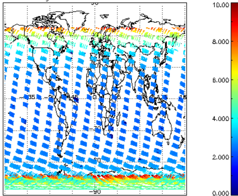
SCIOL2P_NADUV003_amf_gr for 24JAN2004 00:00:00 to 25JAN2004 00:00:00
