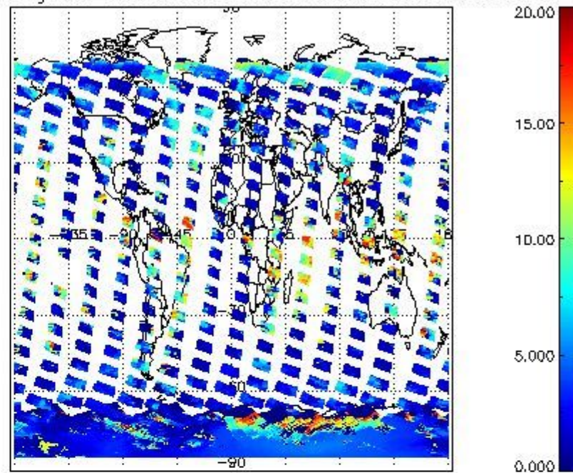
cL_top_height for 24JAN2004 00:00:00 to 25JAN2004 00:00:00
