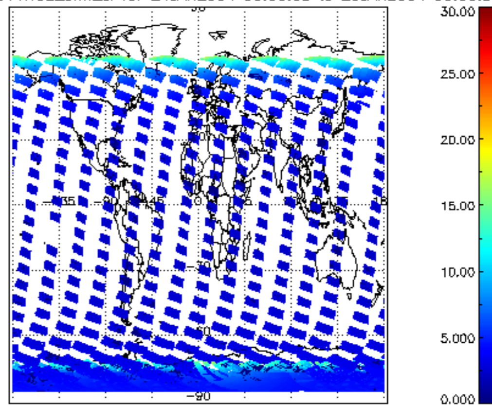
SCIOL2P_NADUV1NO2_amf_cl for 24JAN2004 00:00:00 to 25JAN2004 00:00:00
