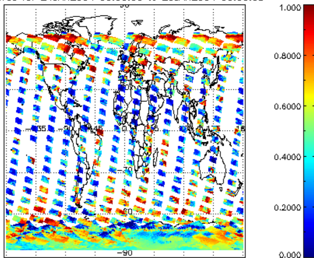
cL_frac for 24JAN2004 00:00:00 to 25JAN2004 00:00:00
