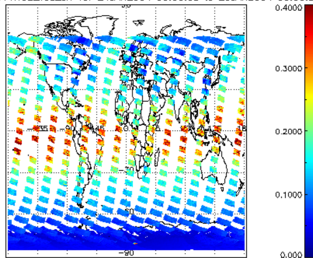
SCIOL2P_NADUV1NO2_vcd_err for 24JAN2004 00:00:00 to 25JAN2004 00:00:00
