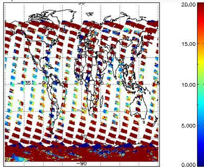
cLopt_depth for 24JAN2004 00:00:00 to 25JAN2004 00:00:00
