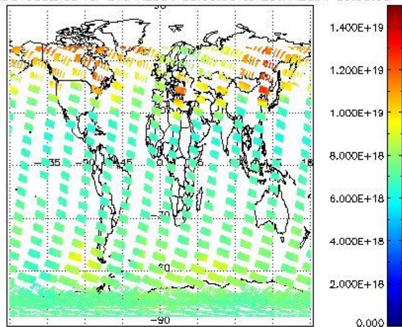
SCIOL2P_NADUV003_vcd for 24JAN2004 00:00:00 to 25JAN2004 00:00:00
