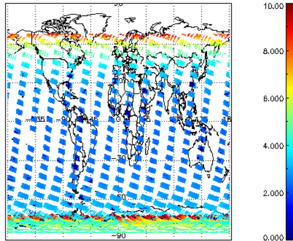
SCIOL2P_NADUV003_amf_cl for 24JAN2004 00:00:00 to 25JAN2004 00:00:00
