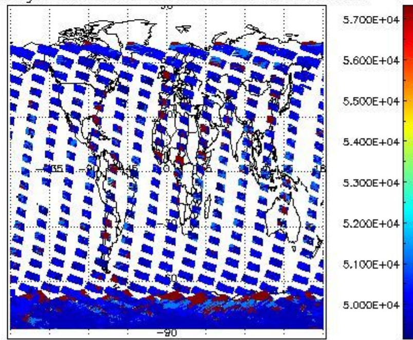
cloud_flags for 24JAN2004 00:00:00 to 25JAN2004 00:00:00
