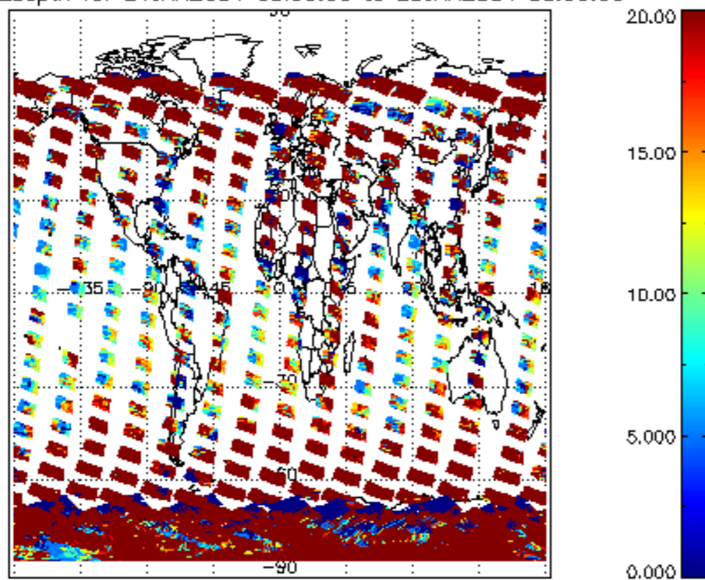
cLopt_depth for 24JAN2004 00:00:00 to 25JAN2004 00:00:00
