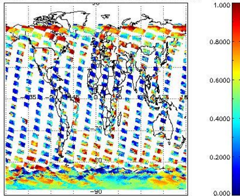
cL_frac for 24JAN2004 00:00:00 to 25JAN2004 00:00:00
