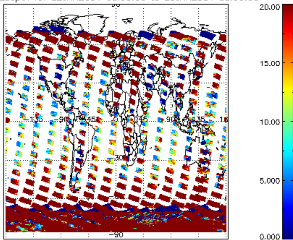
cLopt_depth for 22JAN2004 00:00:00 to 23JAN2004 00:00:00
