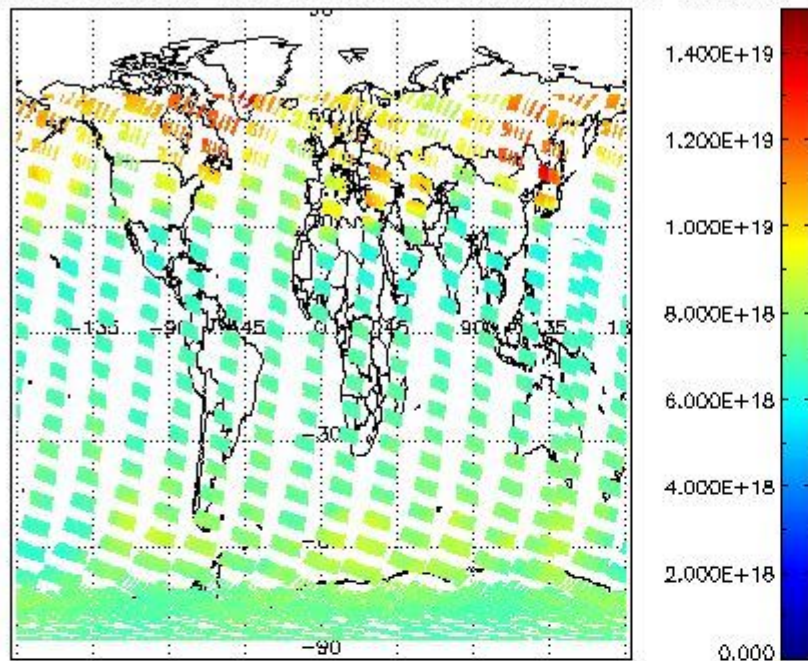
SCIOL2P_NADUV003_vcd for 22JAN2004 00:00:00 to 23JAN2004 00:00:00
