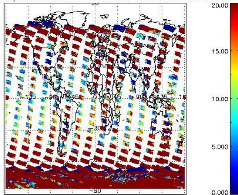
cLopt_depth for 22JAN2004 00:00:00 to 23JAN2004 00:00:00
