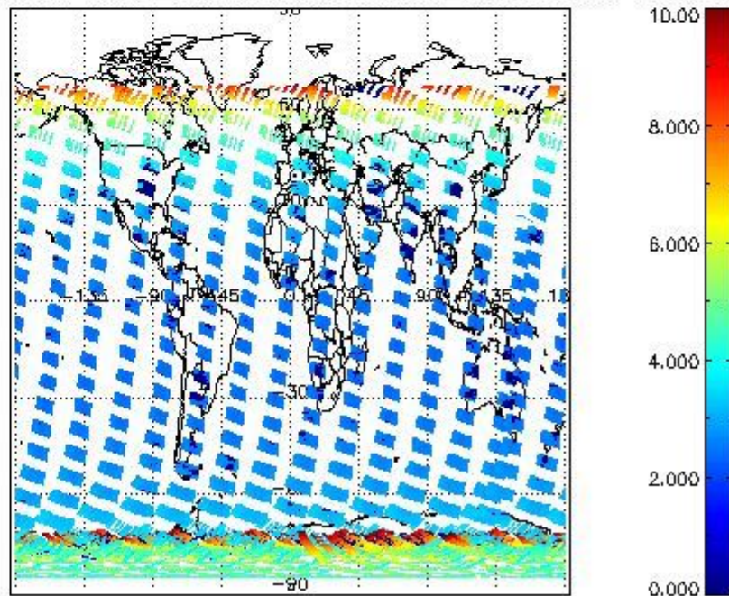
SCIOL2P_NADUV003_amf_cl for 22JAN2004 00:00:00 to 23JAN2004 00:00:00
