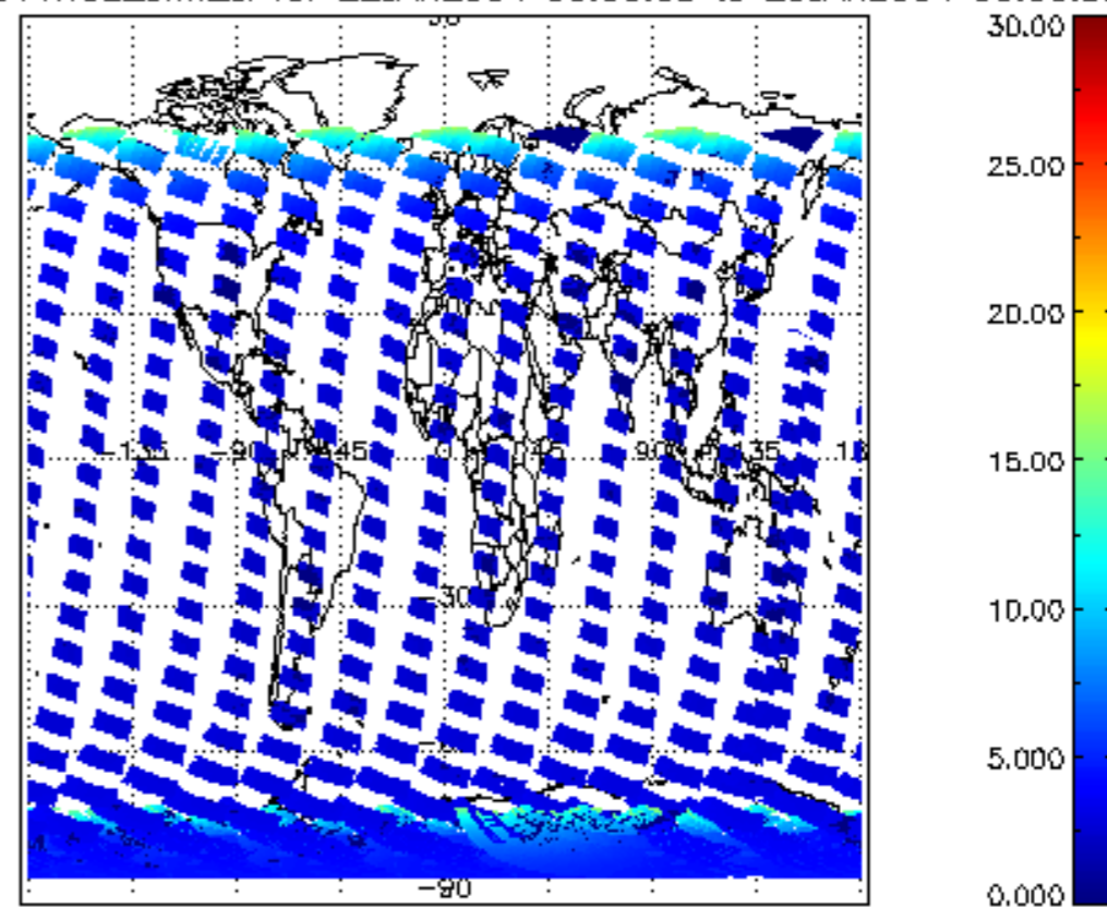
SCIOL2P_NADUV1NO2_amf_cl for 22JAN2004 00:00:00 to 23JAN2004 00:00:00
