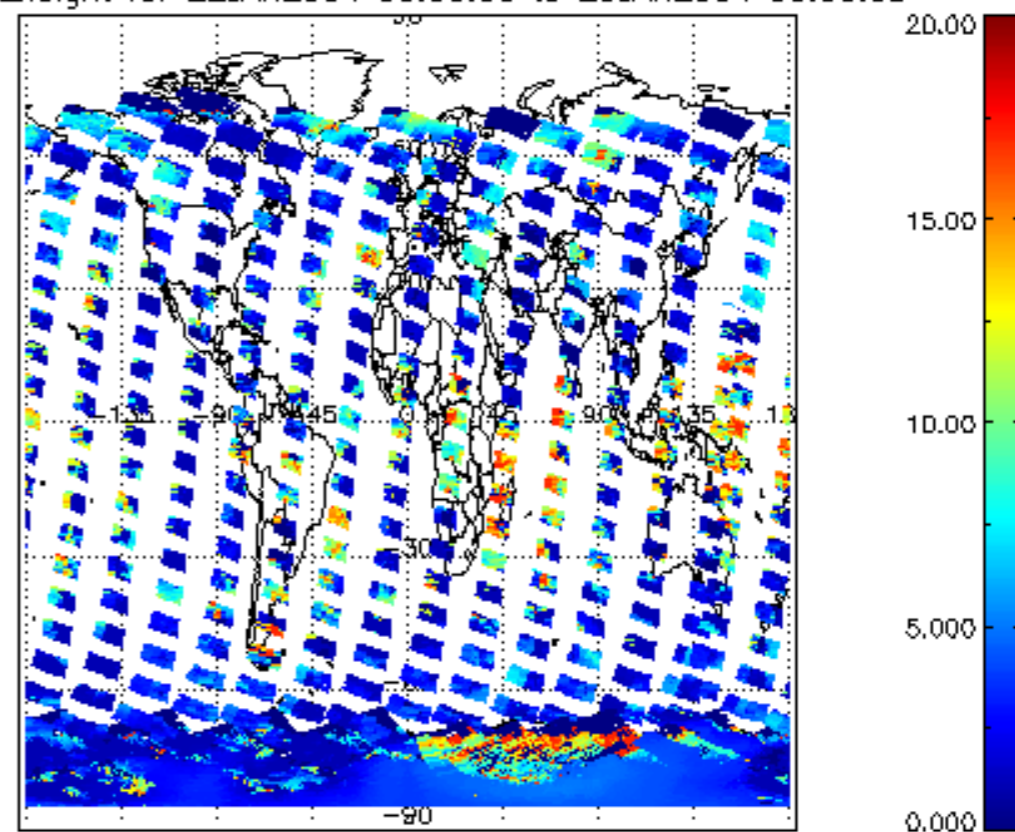
cL_top_height for 22JAN2004 00:00:00 to 23JAN2004 00:00:00
