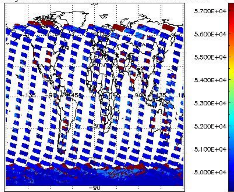
cloud_flags for 22JAN2004 00:00:00 to 23JAN2004 00:00:00
