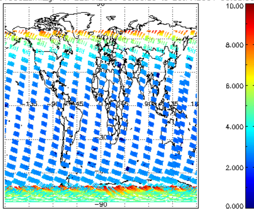
SCIOL2P_NADUV003_amf_gr for 22JAN2004 00:00:00 to 23JAN2004 00:00:00
