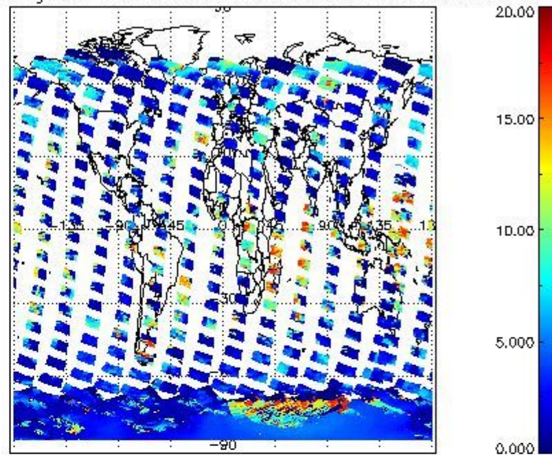
cL_top_height for 22JAN2004 00:00:00 to 23JAN2004 00:00:00
