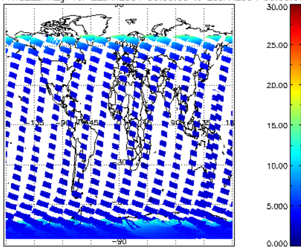
SCIOL2P_NADUV1NO2_amf_gr for 22JAN2004 00:00:00 to 23JAN2004 00:00:00
