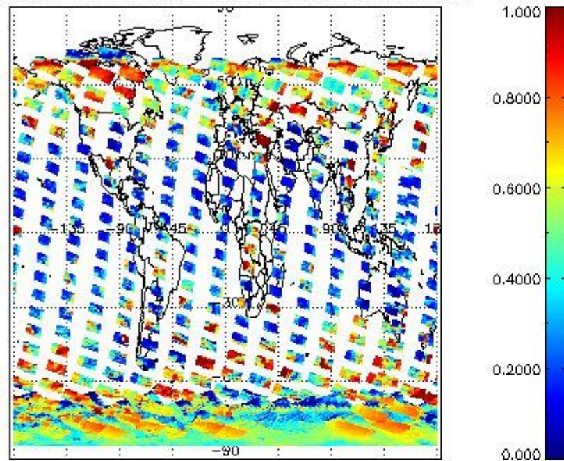
cL_frac for 22JAN2004 00:00:00 to 23JAN2004 00:00:00
