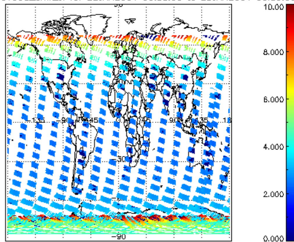
SCIOL2P_NADUV003_amf_cl for 22JAN2004 00:00:00 to 23JAN2004 00:00:00
