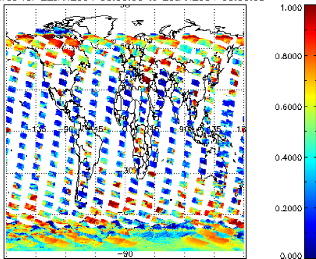
cL_frac for 22JAN2004 00:00:00 to 23JAN2004 00:00:00
