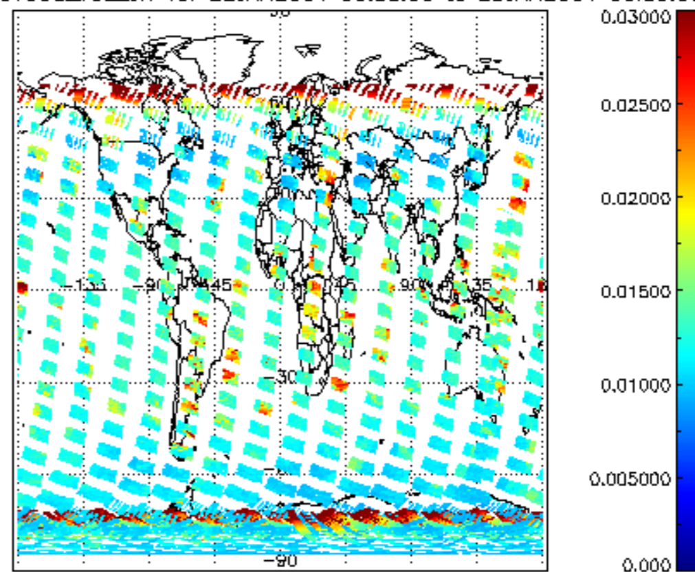
SCIOL2P_NADUV003_vcd_err for 22JAN2004 00:00:00 to 23JAN2004 00:00:00
