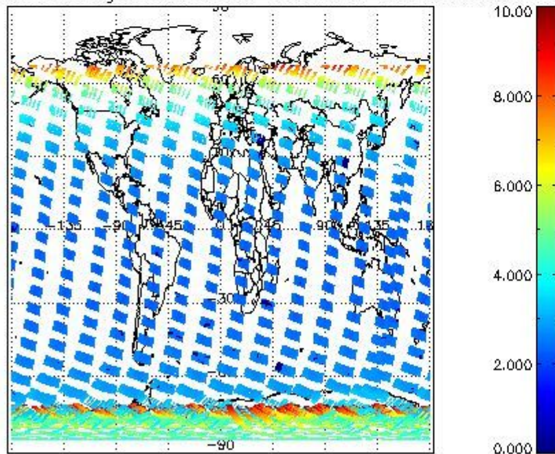
SCIOL2P_NADUV003_amf_gr for 22JAN2004 00:00:00 to 23JAN2004 00:00:00
