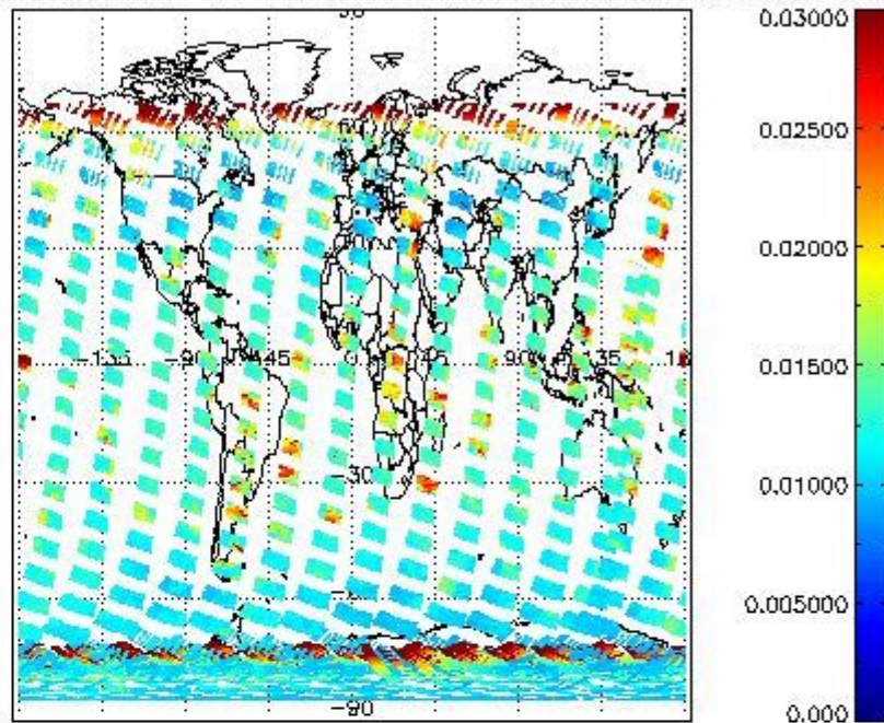
SCIOL2P_NADUV003_vcd_err for 22JAN2004 00:00:00 to 23JAN2004 00:00:00
