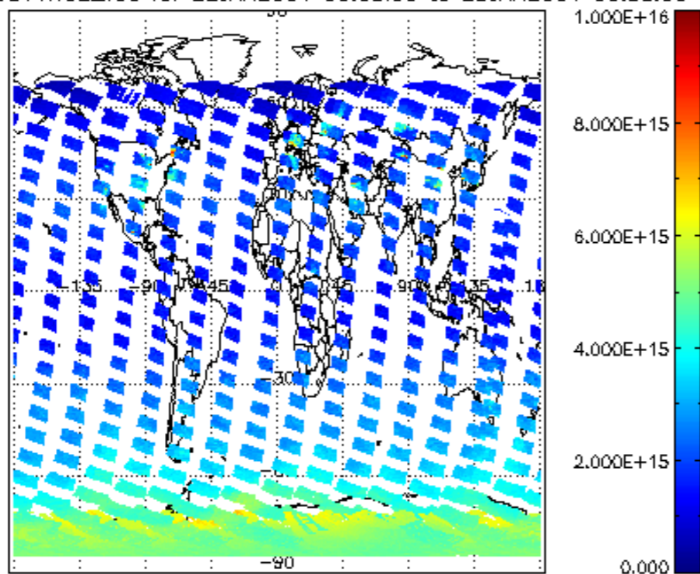
SCIOL2P_NADUV1NO2_vcd for 22JAN2004 00:00:00 to 23JAN2004 00:00:00
