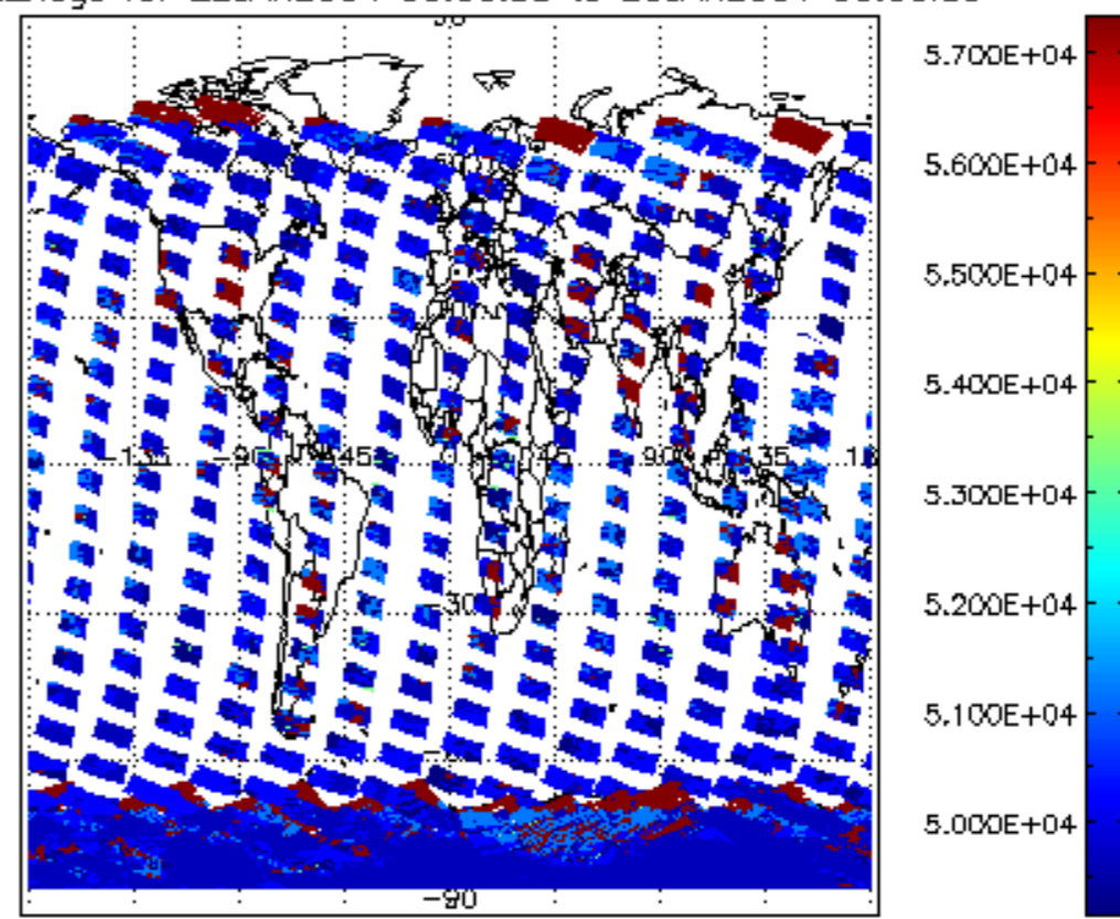
cloud_flags for 22JAN2004 00:00:00 to 23JAN2004 00:00:00
