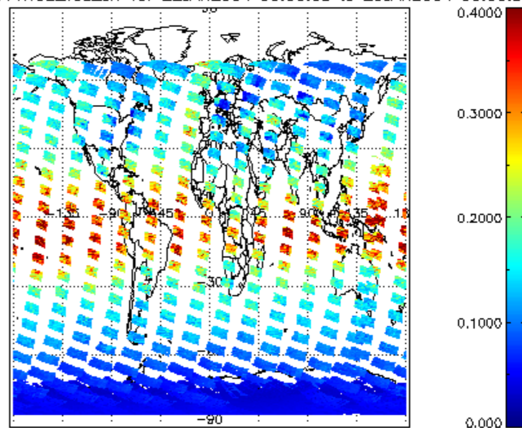
SCIOL2P_NADUV1NO2_vcd_err for 22JAN2004 00:00:00 to 23JAN2004 00:00:00
