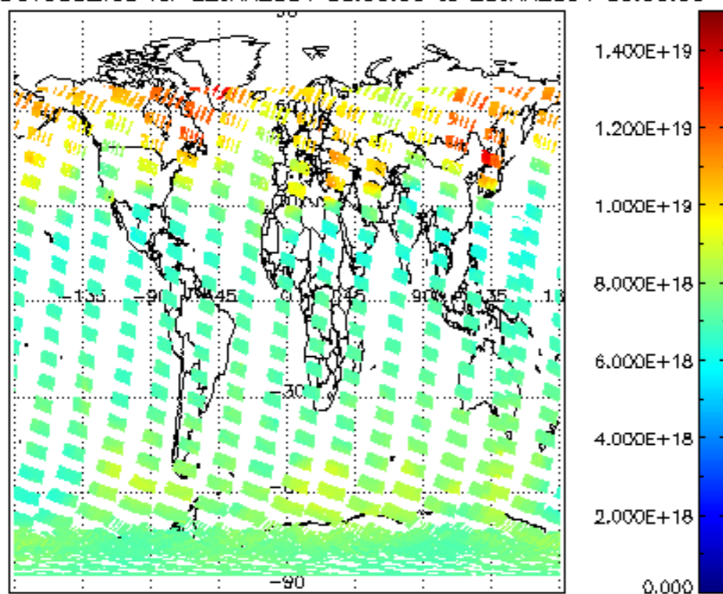
SCIOL2P_NADUV003_vcd for 22JAN2004 00:00:00 to 23JAN2004 00:00:00
