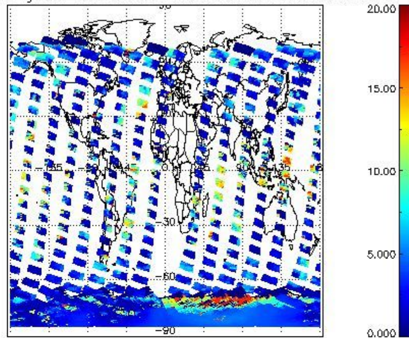
cL_top_height for 21JAN2004 00:00:00 to 22JAN2004 00:00:00
