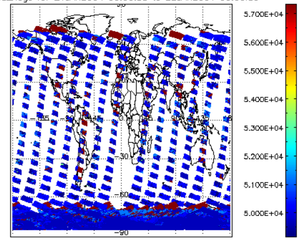
cloud_flags for 21JAN2004 00:00:00 to 22JAN2004 00:00:00
