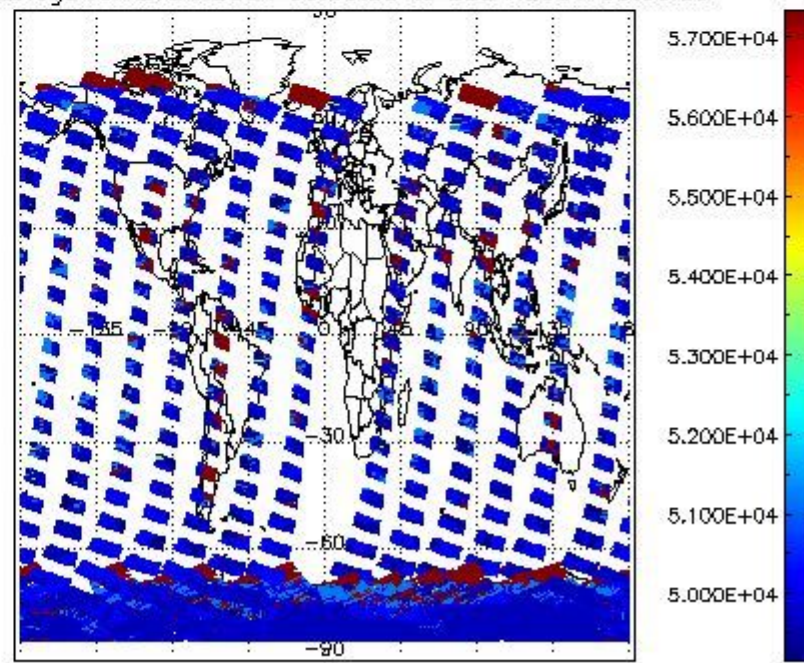
cloud_flags for 21JAN2004 00:00:00 to 22JAN2004 00:00:00
