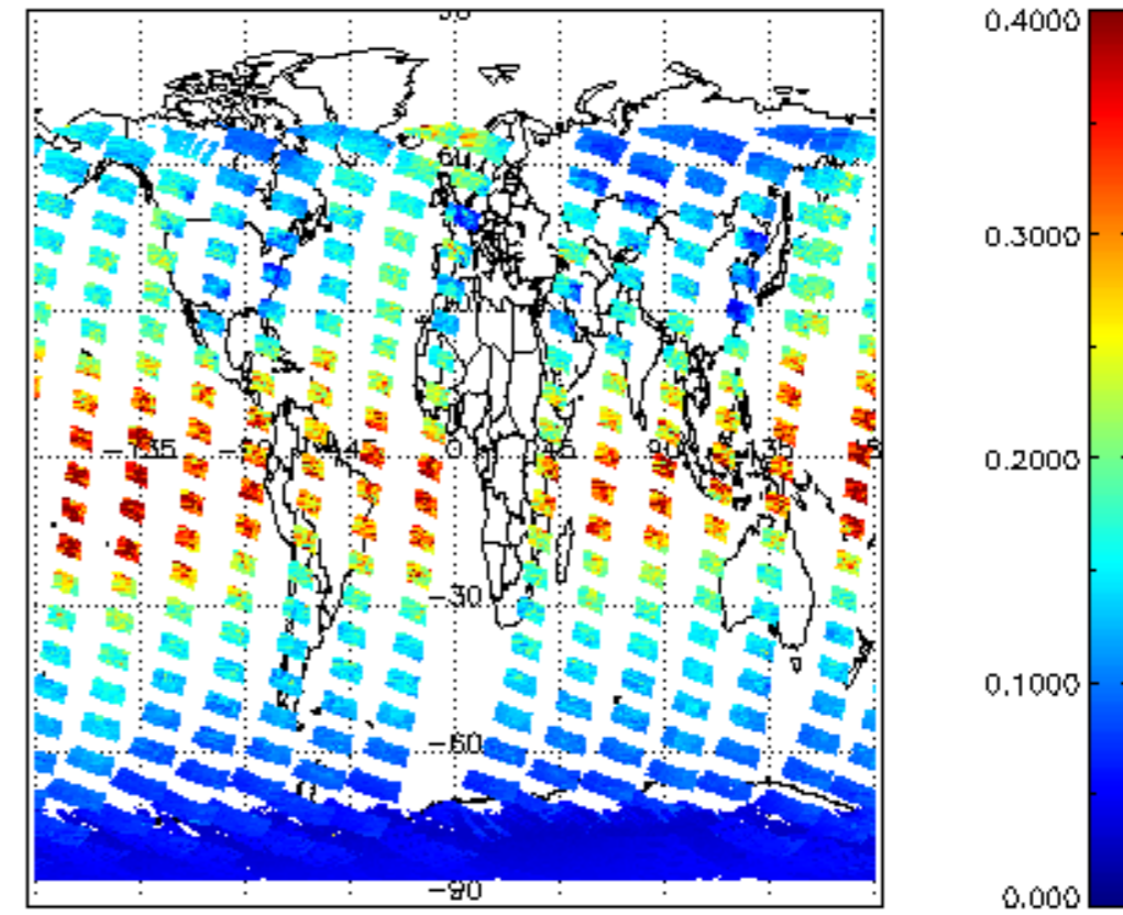
SCIOL2P_NADUV1NO2_vcd_err for 21JAN2004 00:00:00 to 22JAN2004 00:00:00
