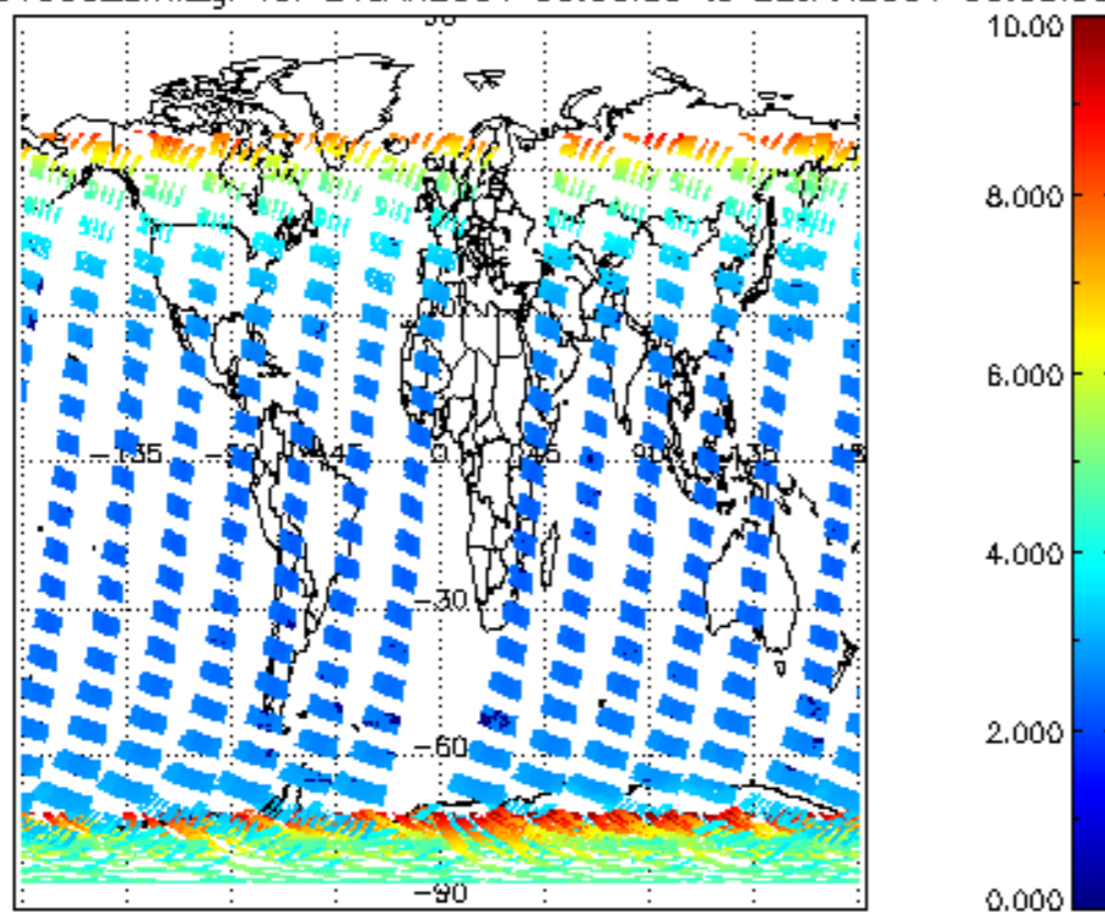
SCIOL2P_NADUV003_amf_gr for 21JAN2004 00:00:00 to 22JAN2004 00:00:00
