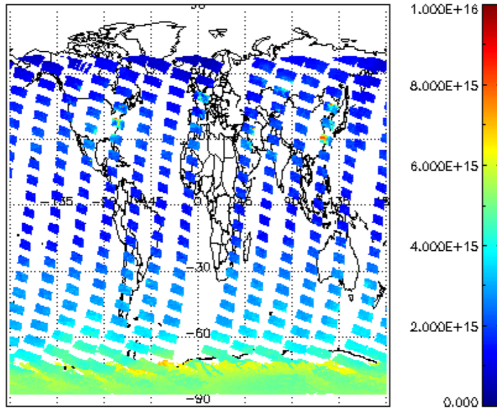
SCIOL2P_NADUV1NO2_vcd for 21JAN2004 00:00:00 to 22JAN2004 00:00:00
