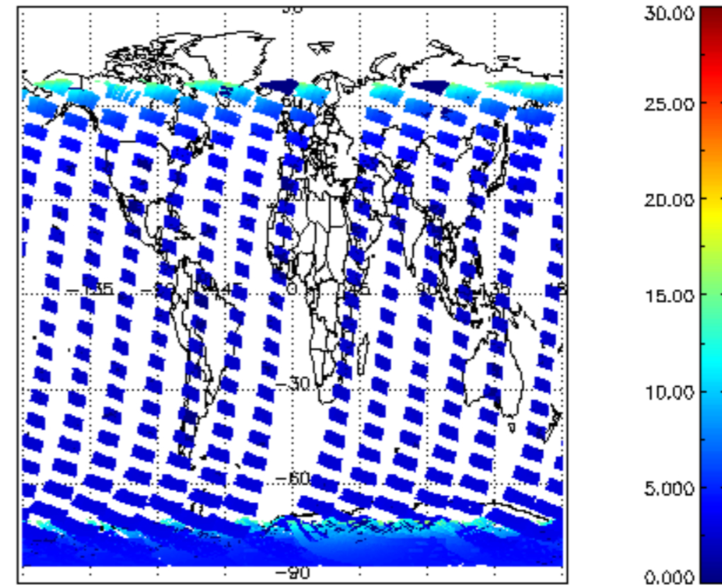
SCIOL2P_NADUV1NO2_amf_cl for 21JAN2004 00:00:00 to 22JAN2004 00:00:00
