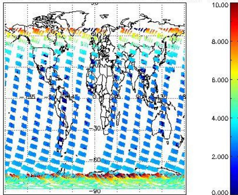
SCIOL2P_NADUV003_amf_cl for 21JAN2004 00:00:00 to 22JAN2004 00:00:00
