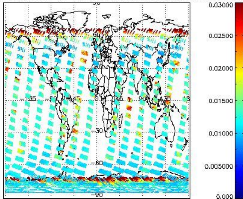
SCIOL2P_NADUV003_vcd_err for 21JAN2004 00:00:00 to 22JAN2004 00:00:00
