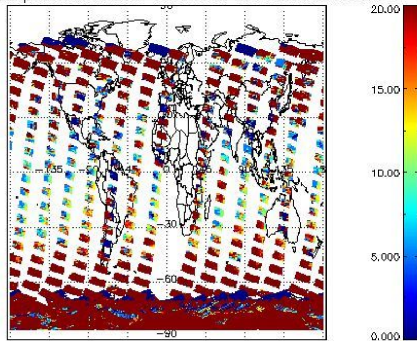
cLopt_depth for 21JAN2004 00:00:00 to 22JAN2004 00:00:00
