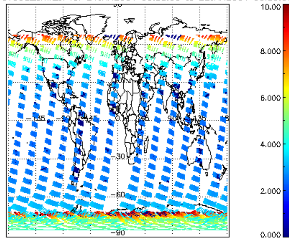
SCIOL2P_NADUV003_amf_cl for 21JAN2004 00:00:00 to 22JAN2004 00:00:00
