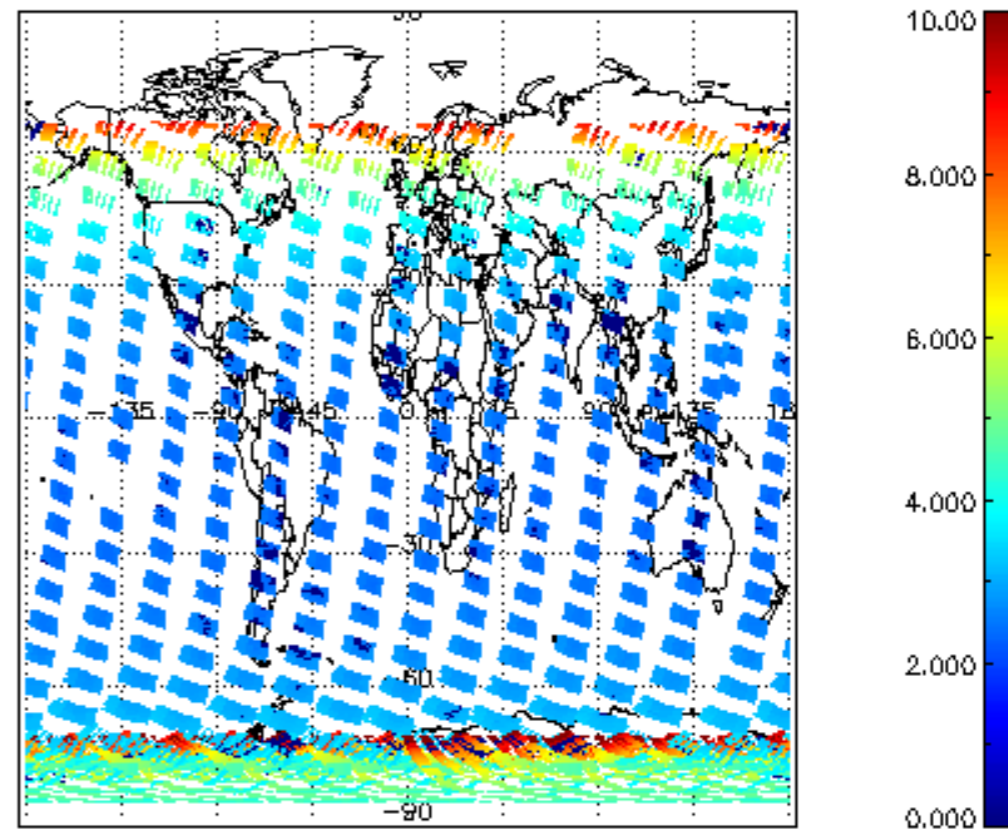
SCIOL2P_NADUV003_amf_cl for 18JAN2004 00:00:00 to 19JAN2004 00:00:00
