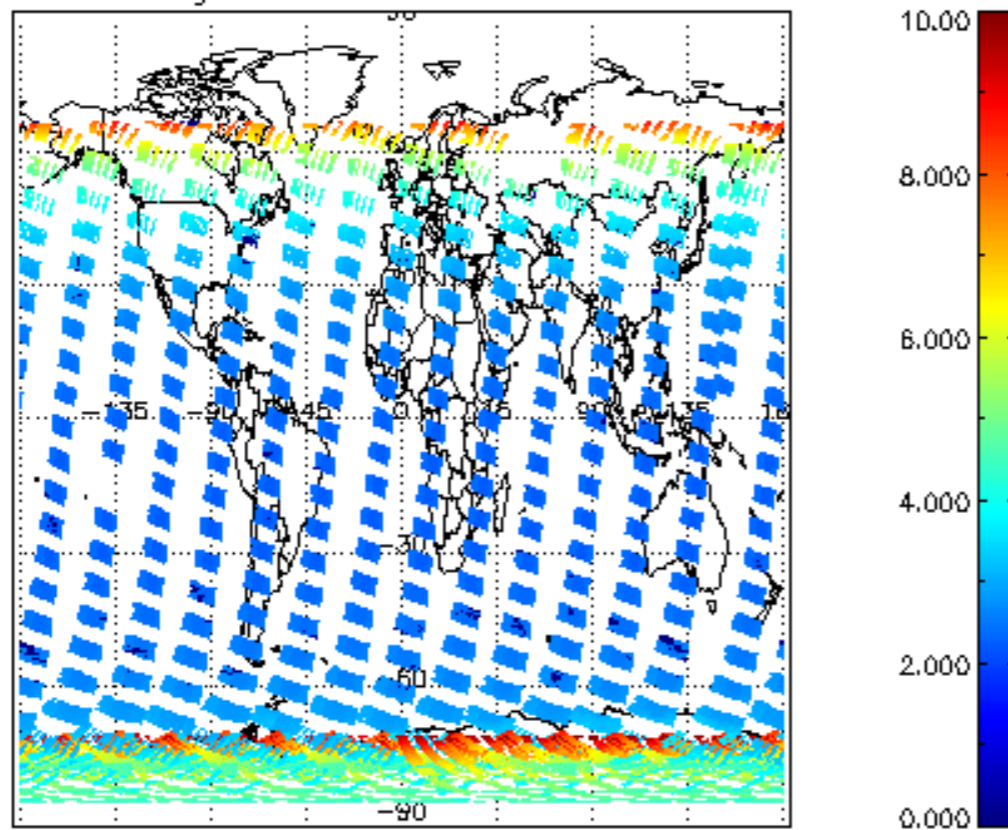
SCIOL2P_NADUV003_amf_gr for 18JAN2004 00:00:00 to 19JAN2004 00:00:00
