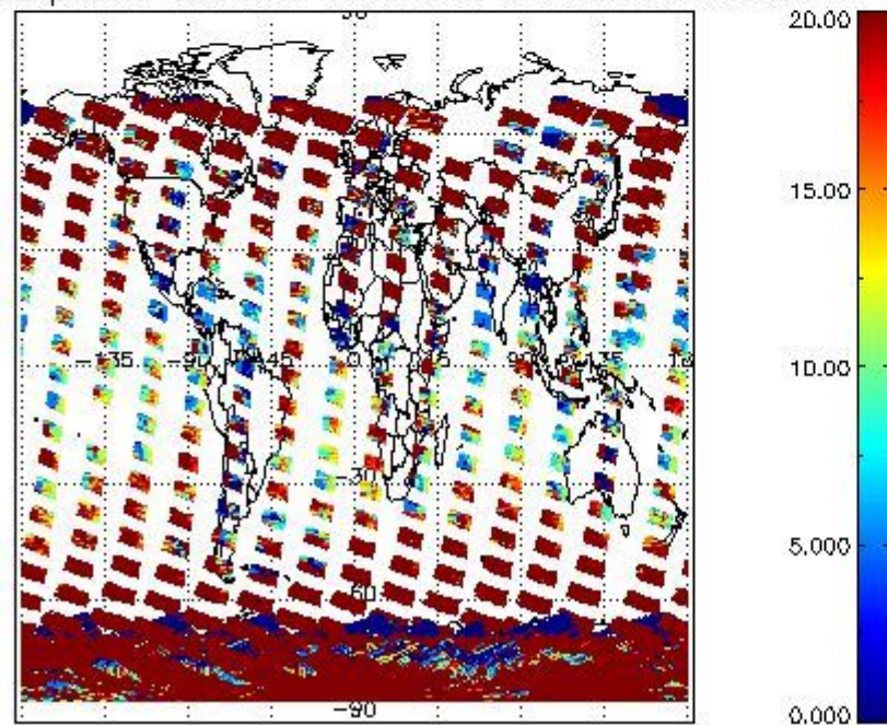
cLopt_depth for 18JAN2004 00:00:00 to 19JAN2004 00:00:00
