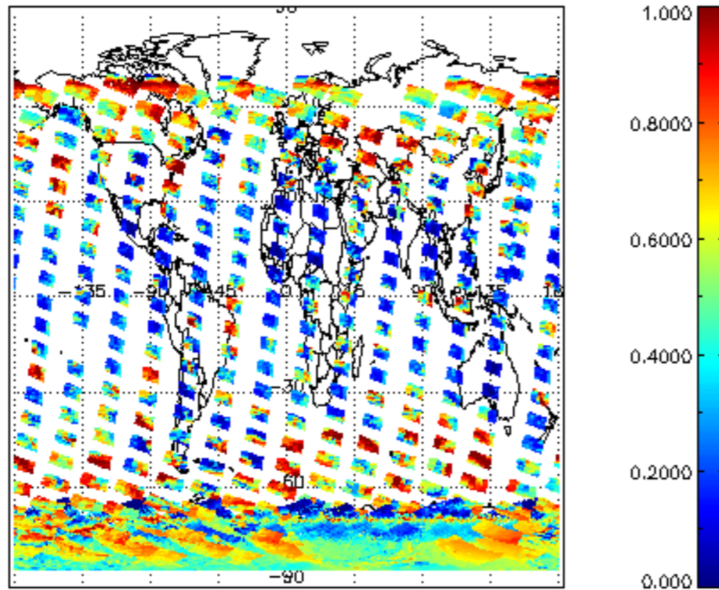
cL_frac for 18JAN2004 00:00:00 to 19JAN2004 00:00:00
