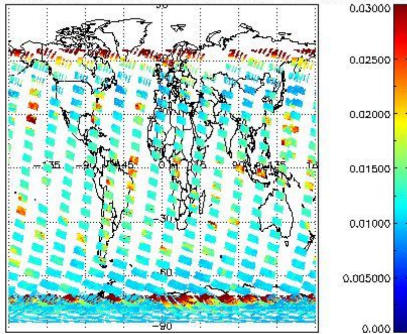
SCIOL2P_NADUV003_vcd_err for 18JAN2004 00:00:00 to 19JAN2004 00:00:00
