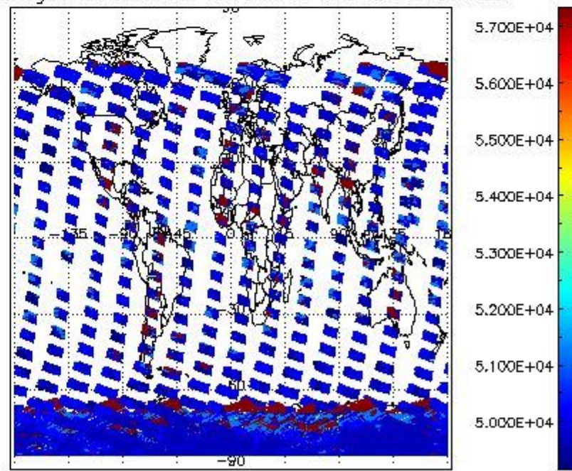
cloud_flags for 18JAN2004 00:00:00 to 19JAN2004 00:00:00
