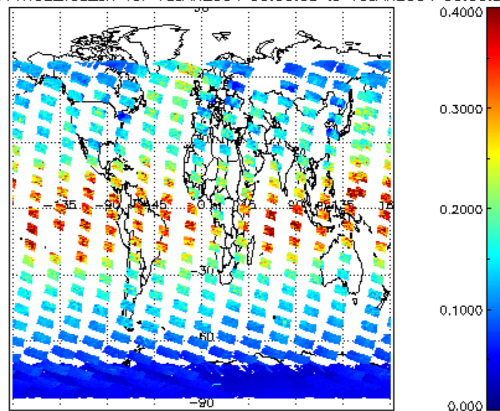
SCIOL2P_NADUV1NO2_vcd_err for 18JAN2004 00:00:00 to 19JAN2004 00:00:00
