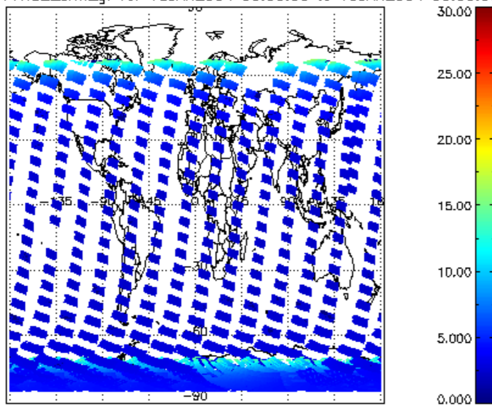
SCIOL2P_NADUV1NO2_amf_gr for 18JAN2004 00:00:00 to 19JAN2004 00:00:00
