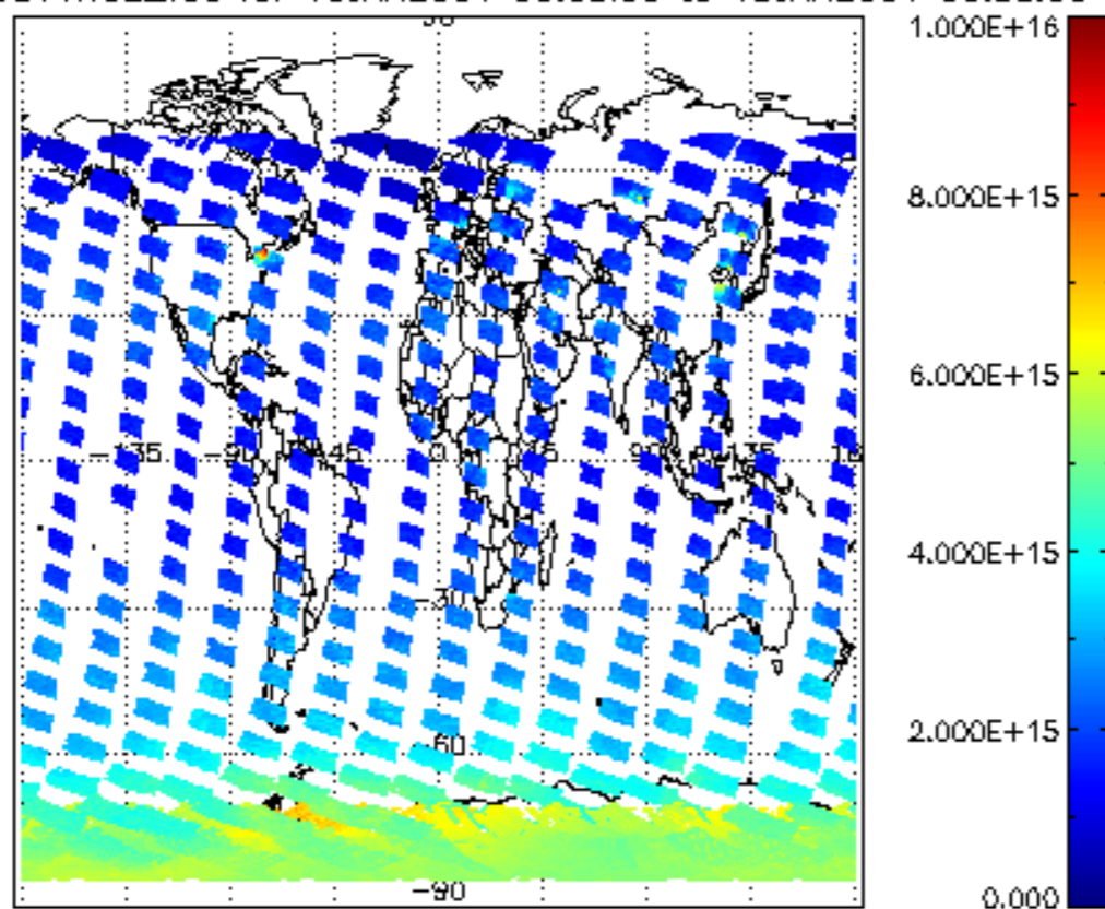
SCIOL2P_NADUV1NO2_vcd for 18JAN2004 00:00:00 to 19JAN2004 00:00:00
