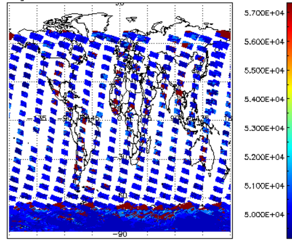
cloud_flags for 18JAN2004 00:00:00 to 19JAN2004 00:00:00
