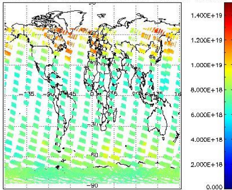
SCIOL2P_NADUV003_vcd for 18JAN2004 00:00:00 to 19JAN2004 00:00:00
