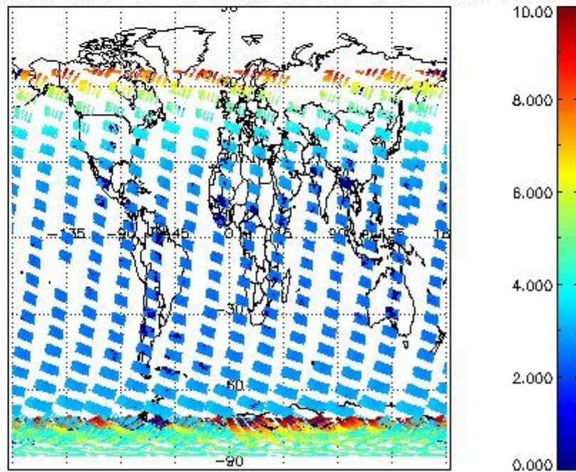
SCIOL2P_NADUV003_amf_cl for 18JAN2004 00:00:00 to 19JAN2004 00:00:00
