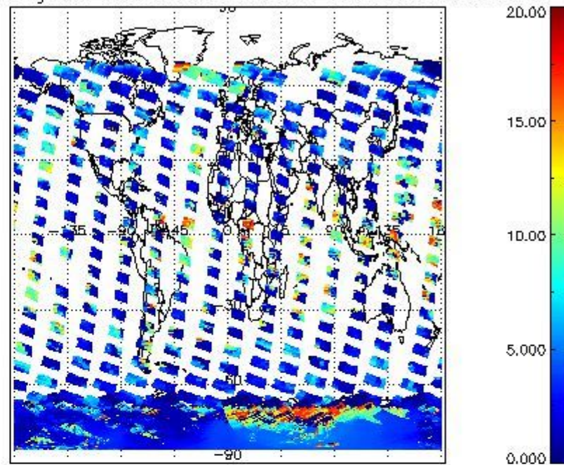
cL_top_height for 18JAN2004 00:00:00 to 19JAN2004 00:00:00
