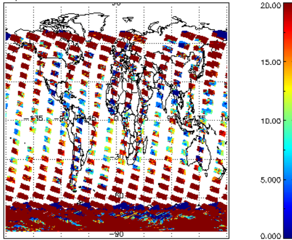
cL_opt_depth for 18JAN2004 00:00:00 to 19JAN2004 00:00:00
