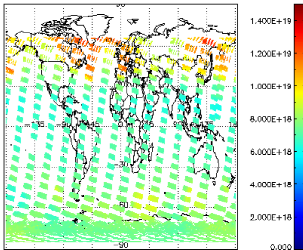
SCIOL2P_NADUV003_vcd for 18JAN2004 00:00:00 to 19JAN2004 00:00:00
