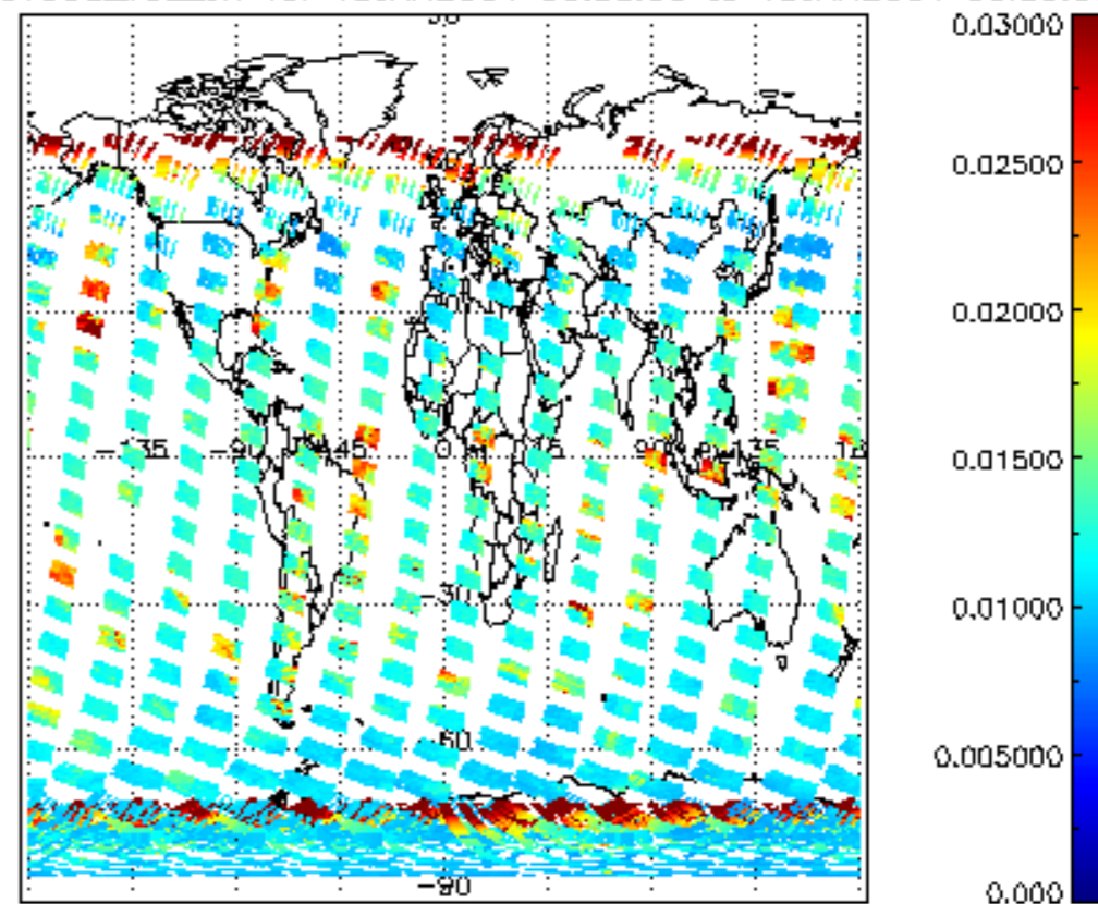
SCIOL2P_NADUV003_vcd_err for 18JAN2004 00:00:00 to 19JAN2004 00:00:00
