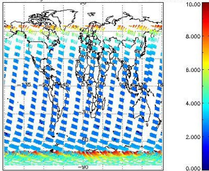
SCIOL2P_NADUV003_amf_gr for 18JAN2004 00:00:00 to 19JAN2004 00:00:00
