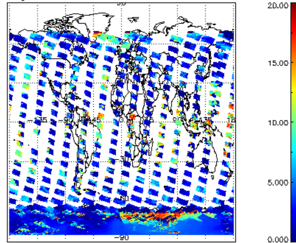
cL_top_height for 18JAN2004 00:00:00 to 19JAN2004 00:00:00
