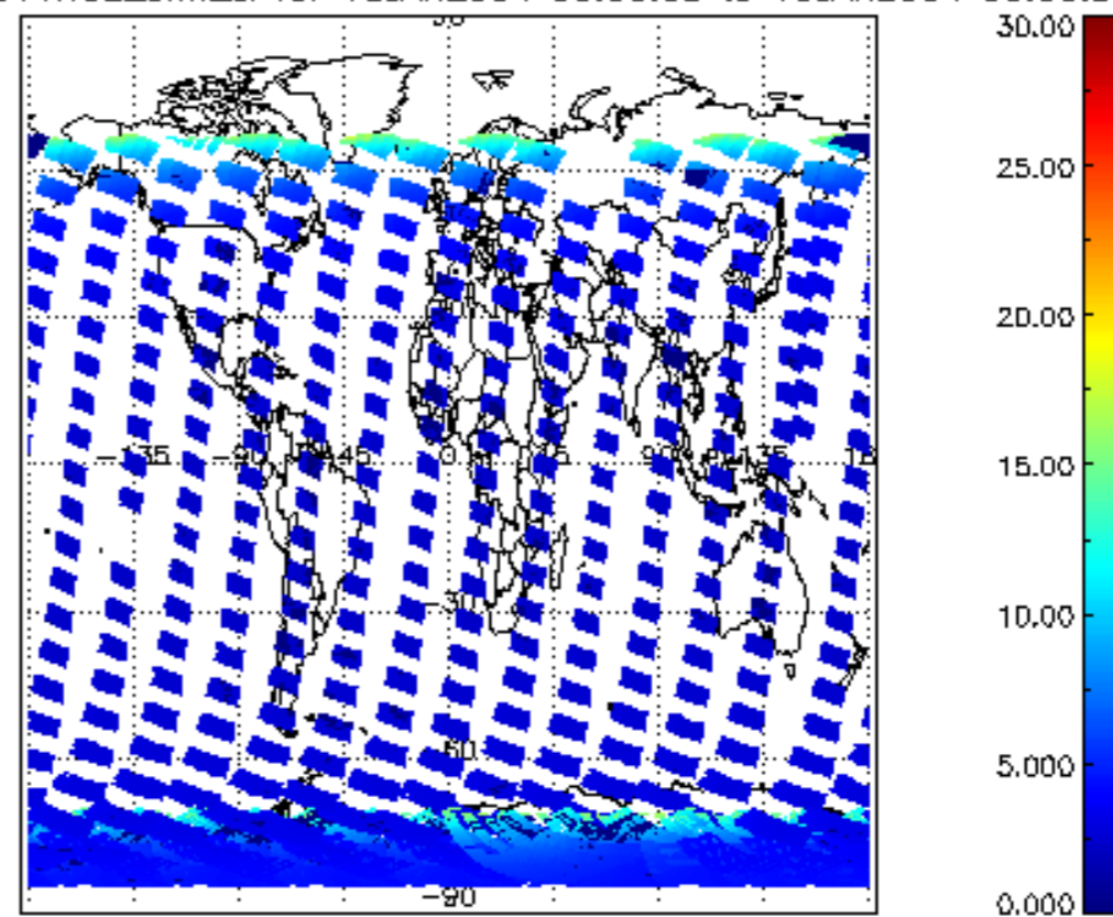
SCIOL2P_NADUV1NO2_amf_cl for 18JAN2004 00:00:00 to 19JAN2004 00:00:00
