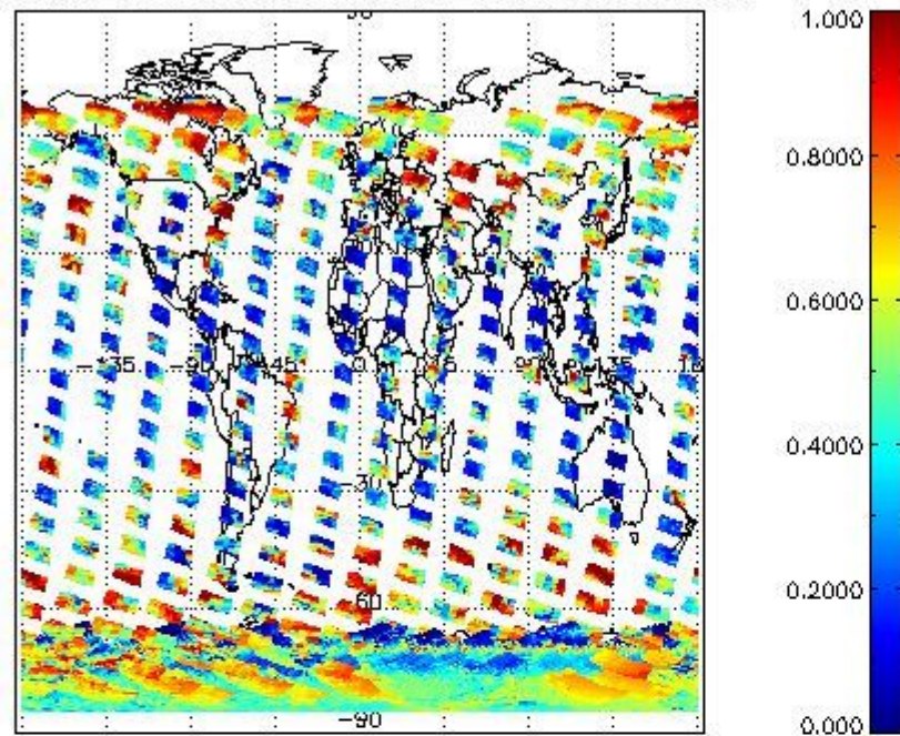
cL_frac for 18JAN2004 00:00:00 to 19JAN2004 00:00:00
