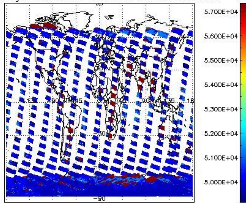
cloud_flags for 16JAN2004 00:00:00 to 17JAN2004 00:00:00
