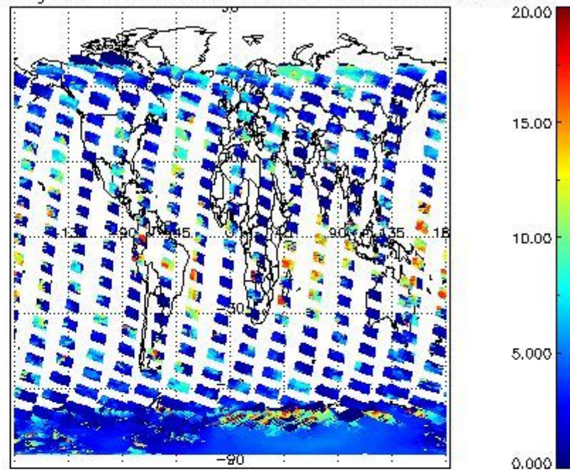
cL_top_height for 16JAN2004 00:00:00 to 17JAN2004 00:00:00
