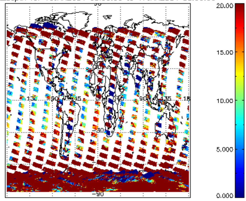
cL_opt_depth for 16JAN2004 00:00:00 to 17JAN2004 00:00:00
