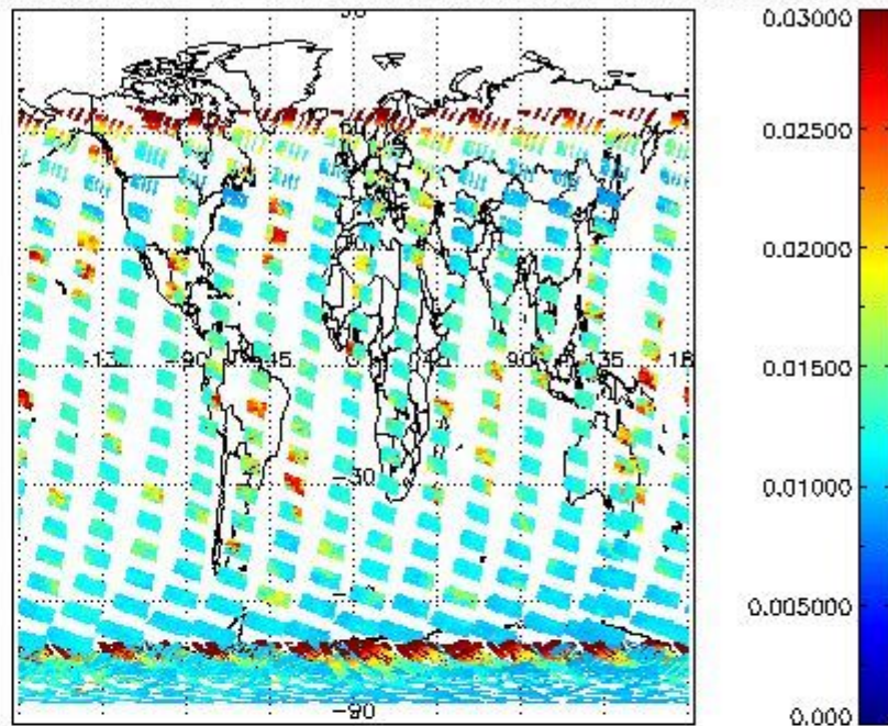
SCIOL2P_NADUV003_vcd_err for 16JAN2004 00:00:00 to 17JAN2004 00:00:00
