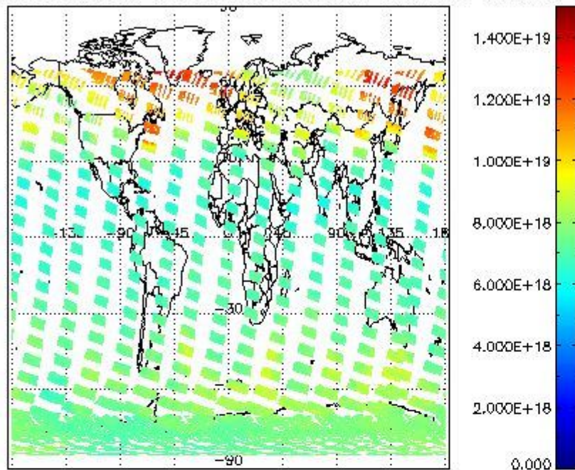
SCIOL2P_NADUV003_vcd for 16JAN2004 00:00:00 to 17JAN2004 00:00:00
