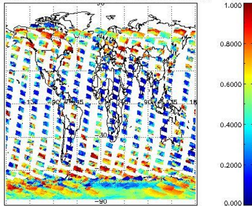
cL_frac for 16JAN2004 00:00:00 to 17JAN2004 00:00:00
