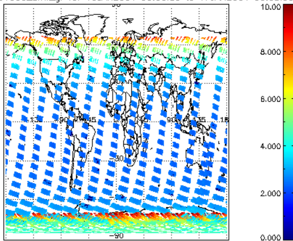
SCIOL2P_NADUV003_amf_gr for 16JAN2004 00:00:00 to 17JAN2004 00:00:00
