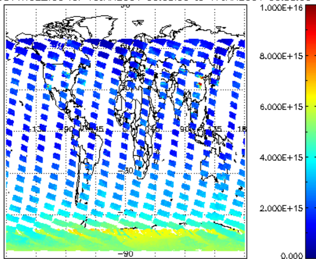
SCIOL2P_NADUV1NO2_vcd for 16JAN2004 00:00:00 to 17JAN2004 00:00:00
