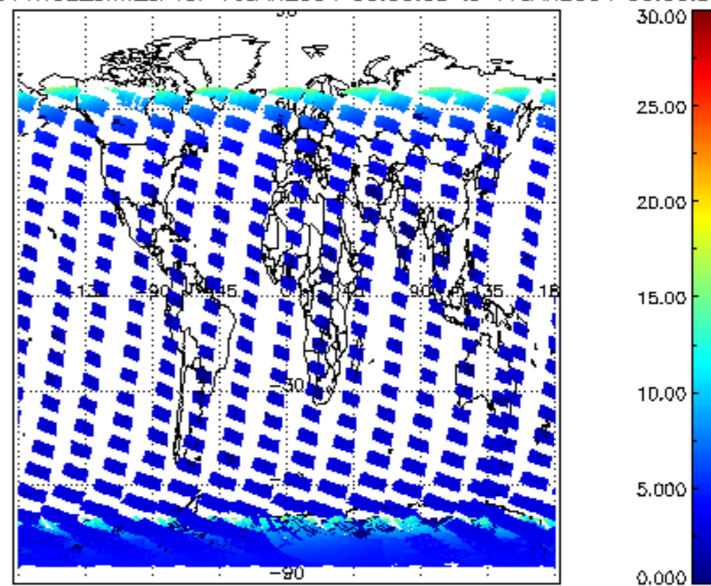
SCIOL2P_NADUV1NO2_amf_cl for 16JAN2004 00:00:00 to 17JAN2004 00:00:00
