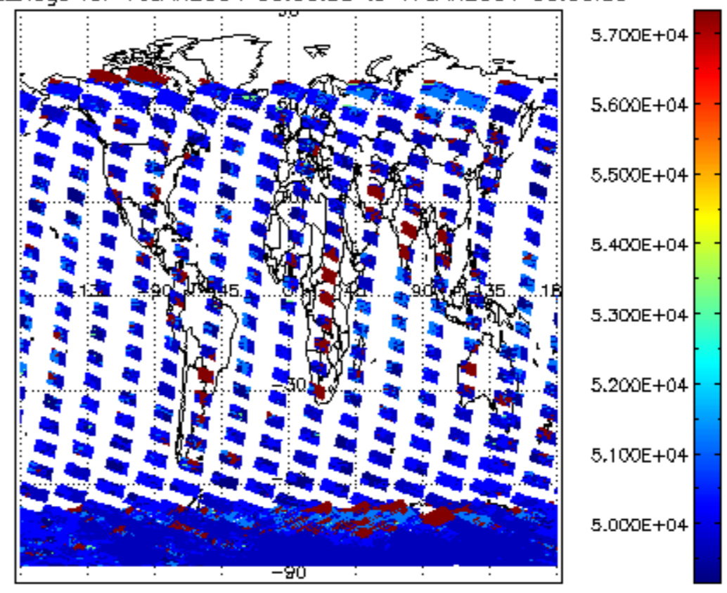
cloud_flags for 16JAN2004 00:00:00 to 17JAN2004 00:00:00
