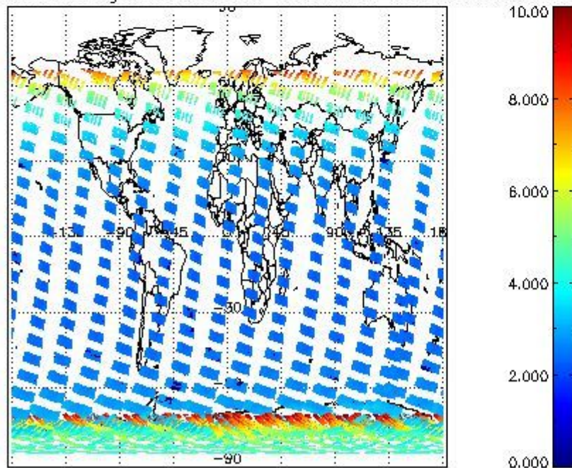
SCIOL2P_NADUV003_amf_gr for 16JAN2004 00:00:00 to 17JAN2004 00:00:00
