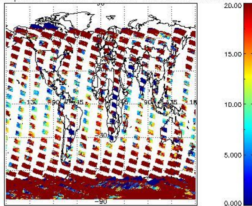
cLopt_depth for 16JAN2004 00:00:00 to 17JAN2004 00:00:00
