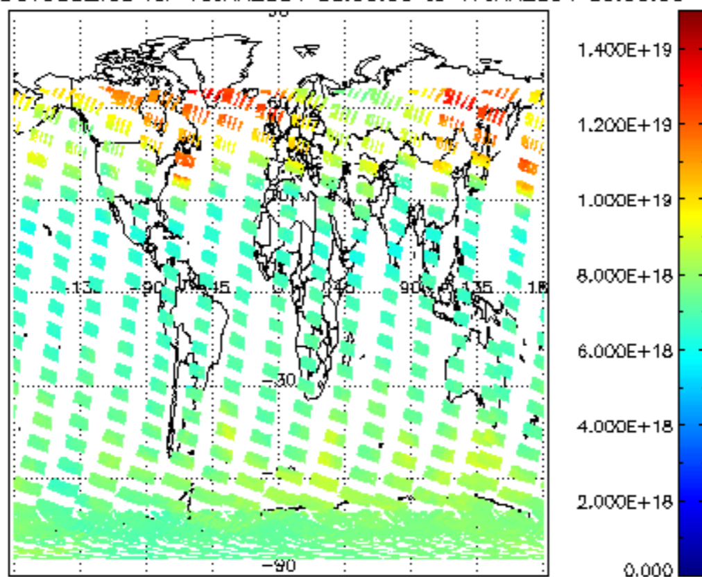
SCIOL2P_NADUV003_vcd for 16JAN2004 00:00:00 to 17JAN2004 00:00:00
