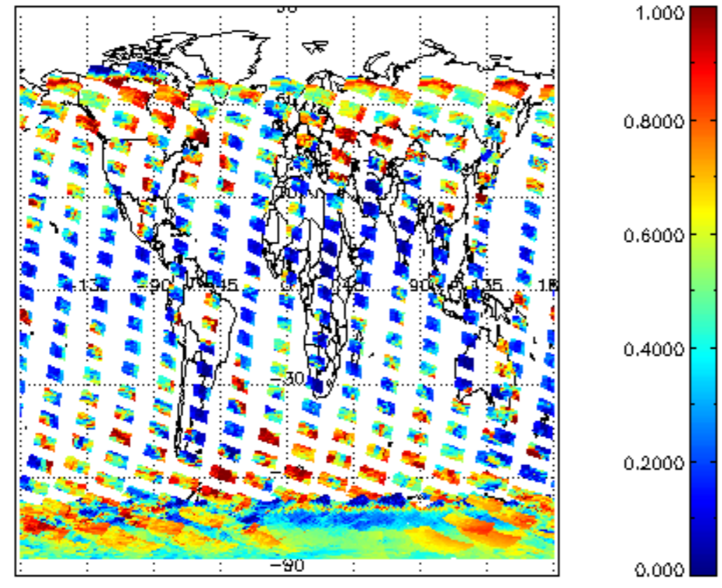
cL_frac for 16JAN2004 00:00:00 to 17JAN2004 00:00:00
