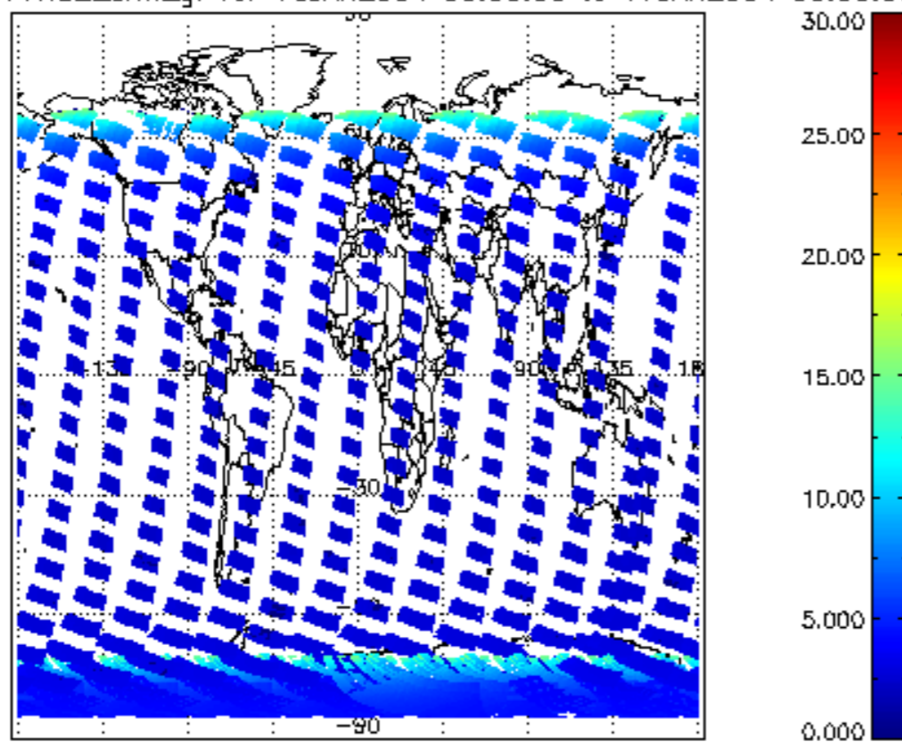
SCIOL2P_NADUV1NO2_amf_gr for 16JAN2004 00:00:00 to 17JAN2004 00:00:00
