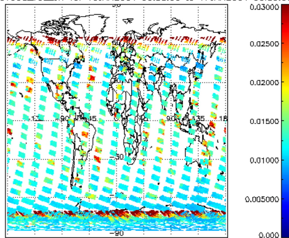
SCIOL2P_NADUV003_vcd_err for 16JAN2004 00:00:00 to 17JAN2004 00:00:00
