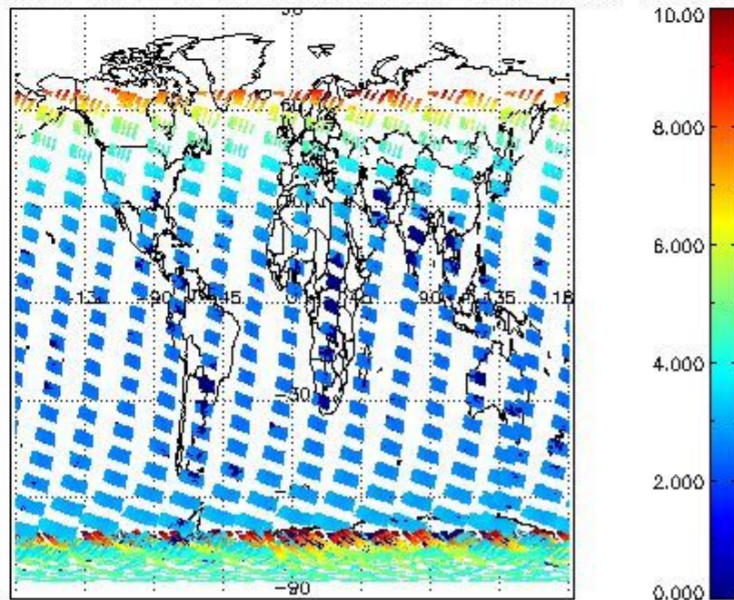
SCIOL2P_NADUV003_amf_cl for 16JAN2004 00:00:00 to 17JAN2004 00:00:00
