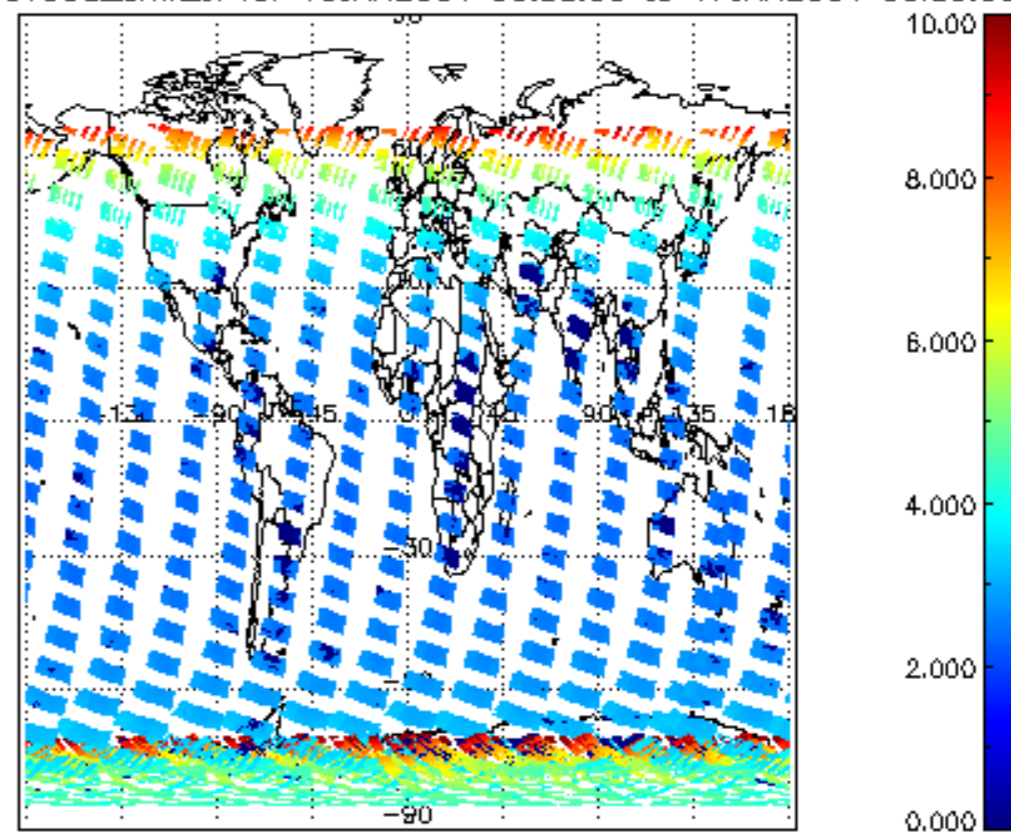
SCIOL2P_NADUV003_amf_cl for 16JAN2004 00:00:00 to 17JAN2004 00:00:00
