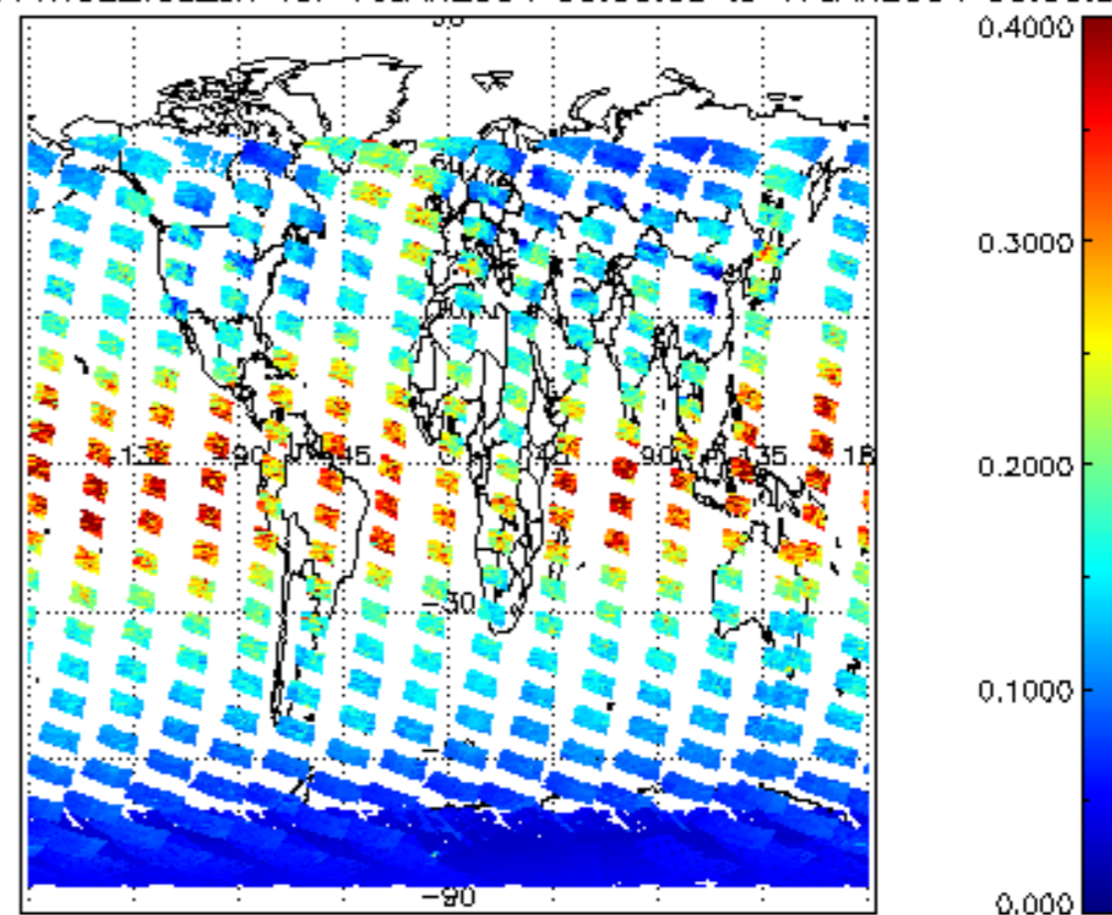
SCIOL2P_NADUV1NO2_vcd_err for 16JAN2004 00:00:00 to 17JAN2004 00:00:00
