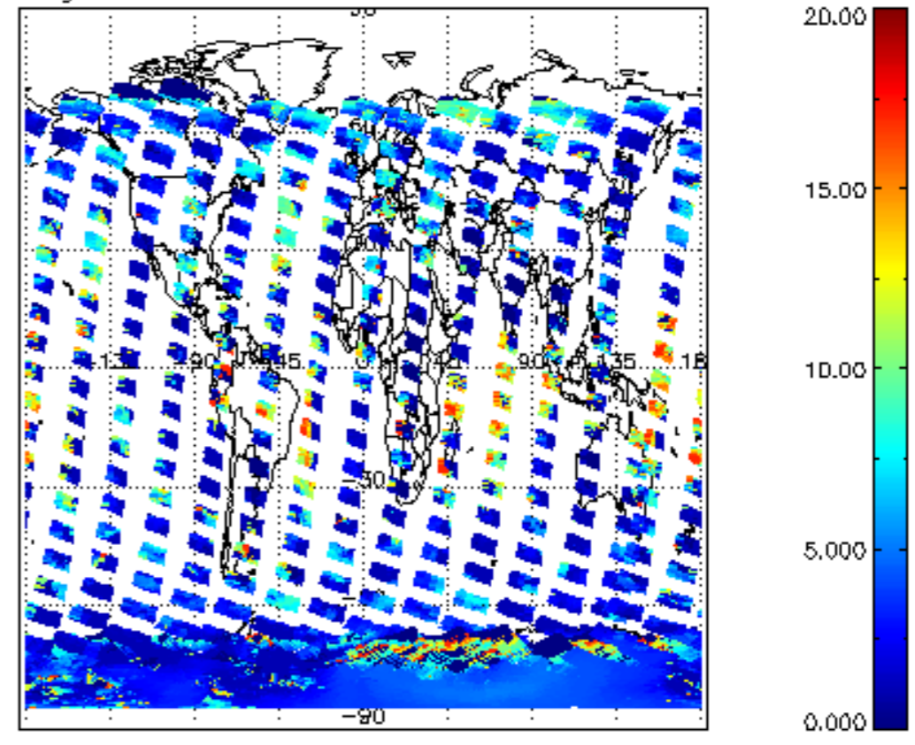
cL_top_height for 16JAN2004 00:00:00 to 17JAN2004 00:00:00
