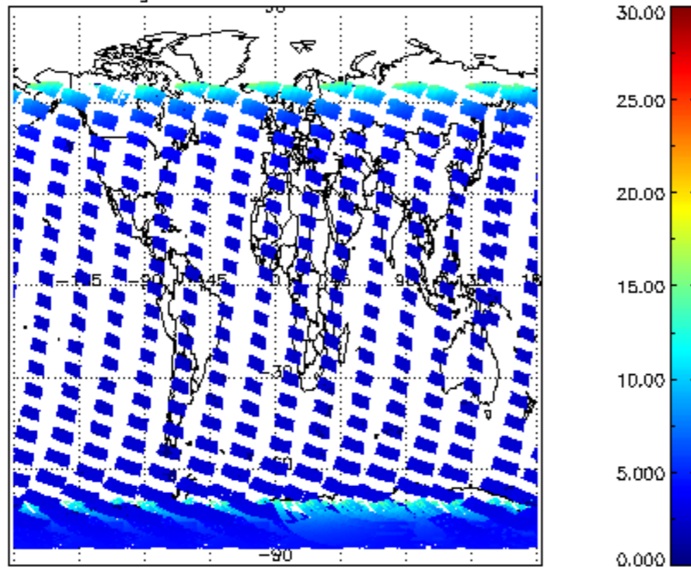
SCIOL2P_NADUV1NO2_amf_gr for 15JAN2004 00:00:00 to 16JAN2004 00:00:00
