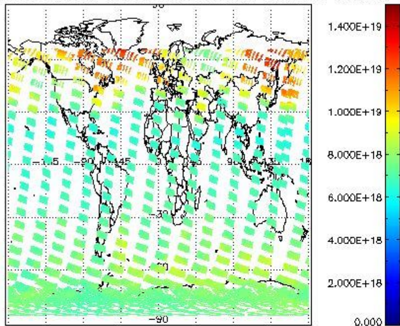
SCIOL2P_NADUV003_vcd for 15JAN2004 00:00:00 to 16JAN2004 00:00:00
