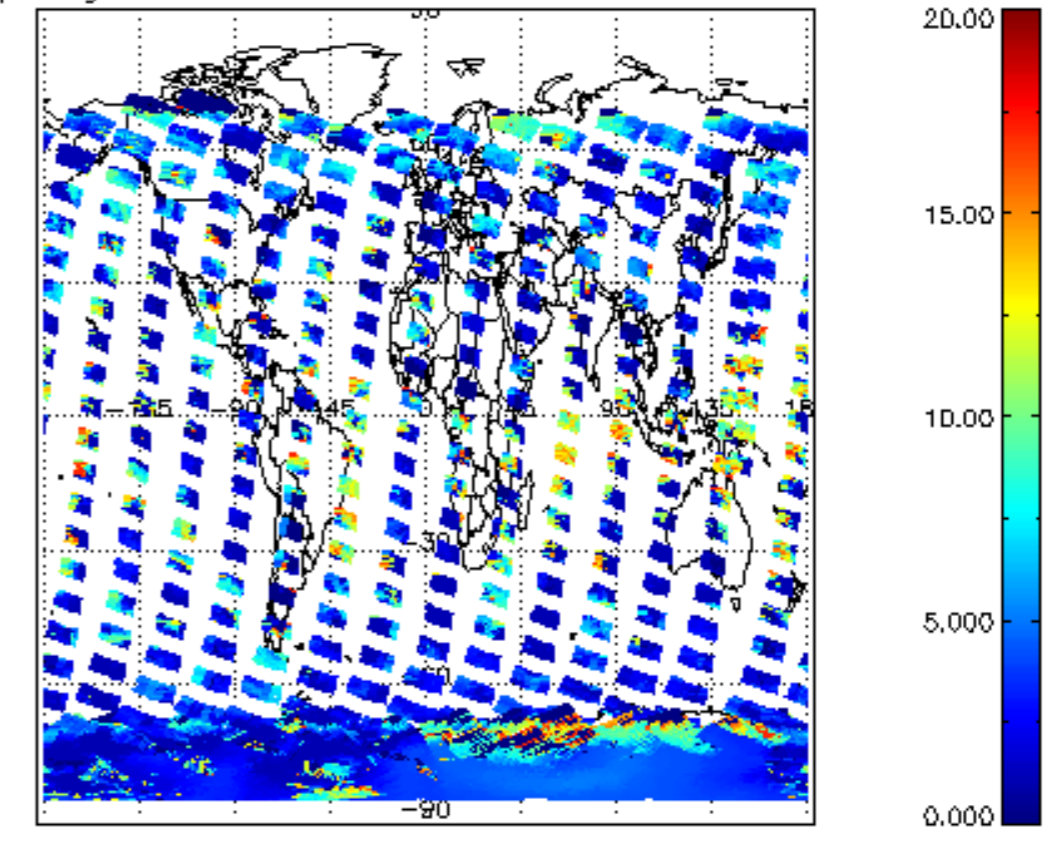
cL_top_height for 15JAN2004 00:00:00 to 16JAN2004 00:00:00
