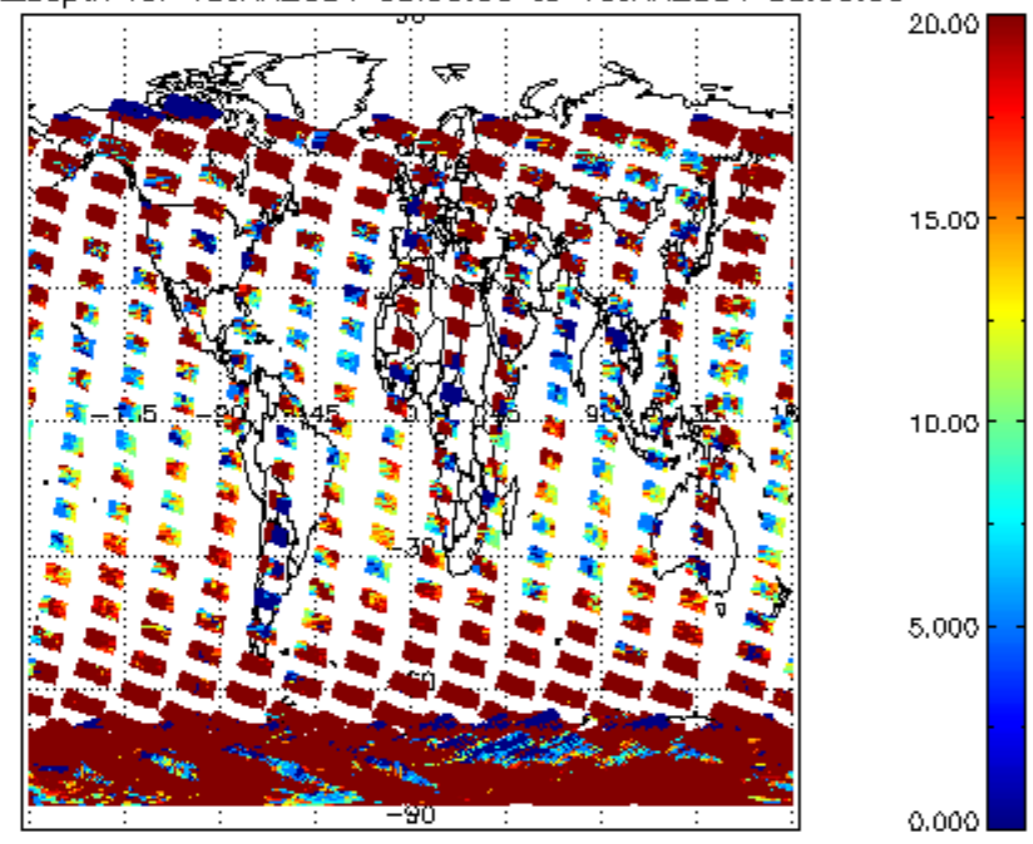
cL_opt_depth for 15JAN2004 00:00:00 to 16JAN2004 00:00:00
