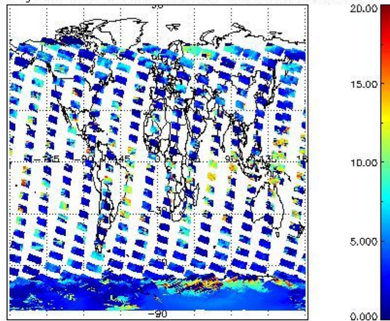
cL_top_height for 15JAN2004 00:00:00 to 16JAN2004 00:00:00
