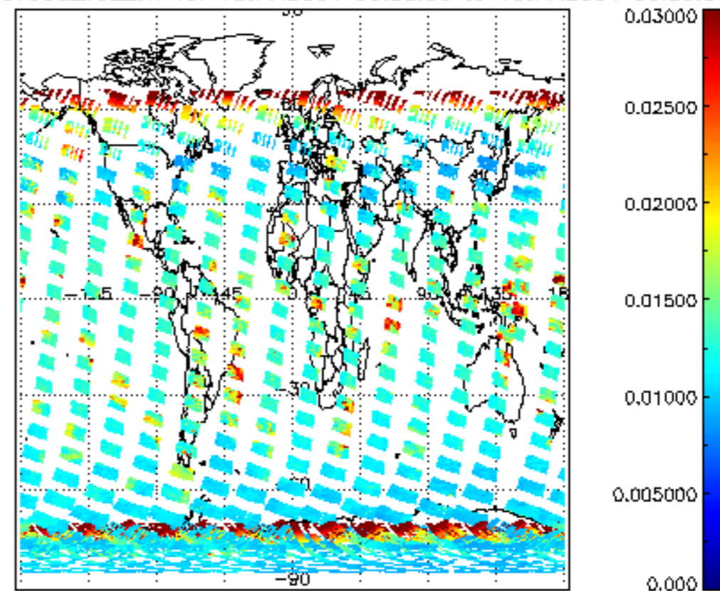
SCIOL2P_NADUV003_vcd_err for 15JAN2004 00:00:00 to 16JAN2004 00:00:00
