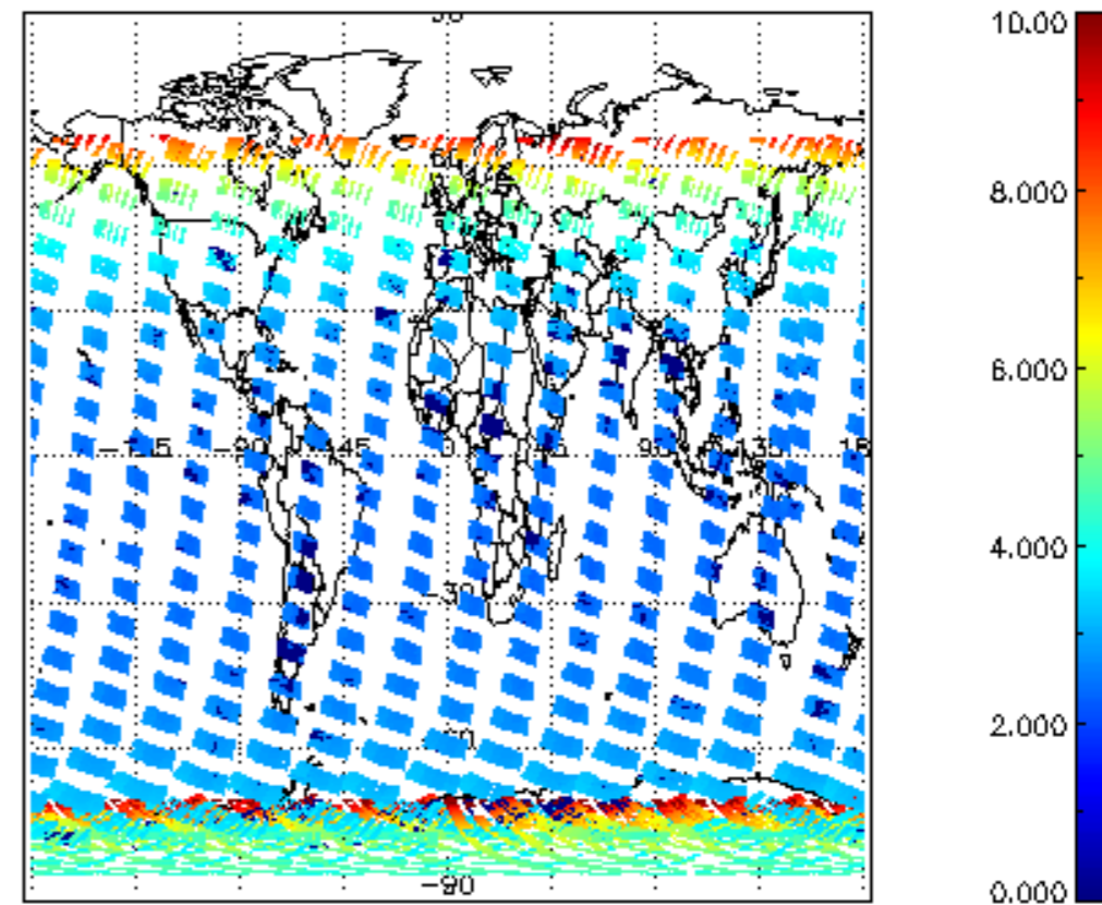
SCIOL2P_NADUV003_amf_cl for 15JAN2004 00:00:00 to 16JAN2004 00:00:00
