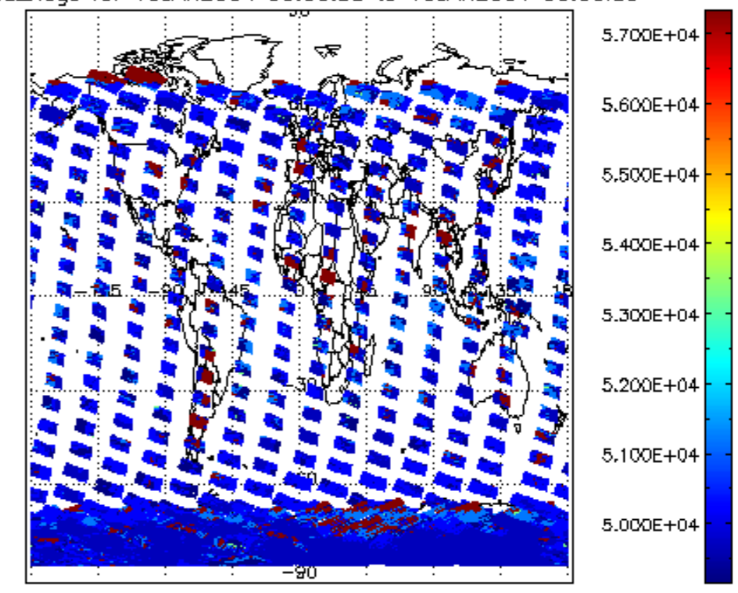
cloud_flags for 15JAN2004 00:00:00 to 16JAN2004 00:00:00
