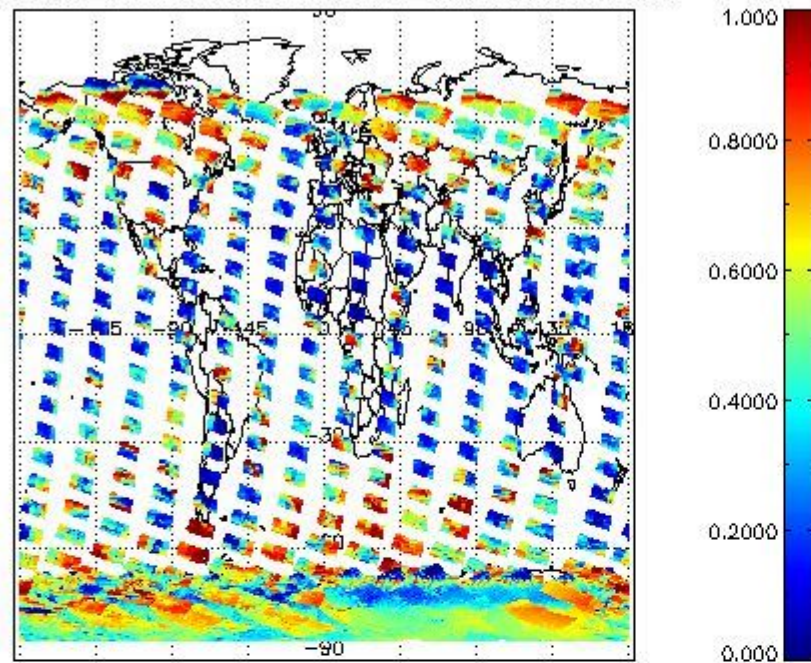
cL_frac for 15JAN2004 00:00:00 to 16JAN2004 00:00:00
