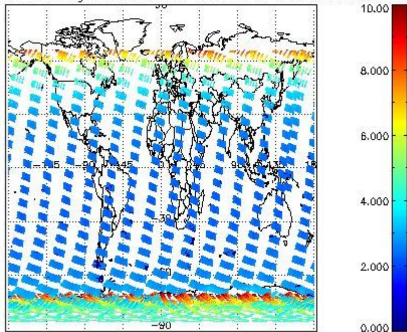
SCIOL2P_NADUV003_amf_gr for 15JAN2004 00:00:00 to 16JAN2004 00:00:00
