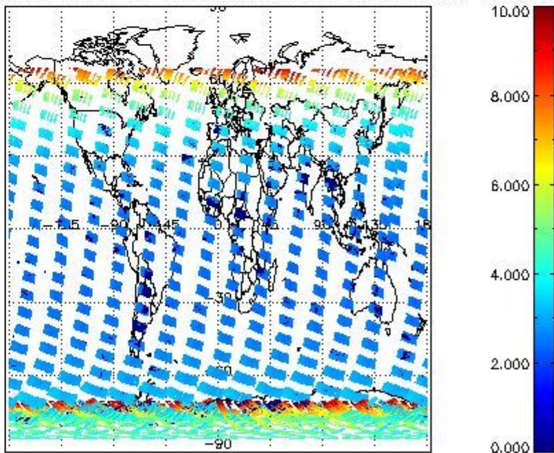
SCIOL2P_NADUV003_amf_cl for 15JAN2004 00:00:00 to 16JAN2004 00:00:00
