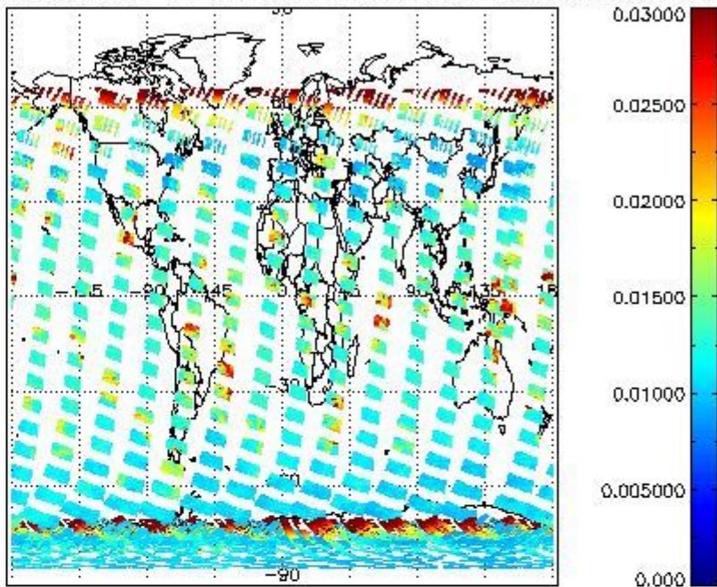
SCIOL2P_NADUV003_vcd_err for 15JAN2004 00:00:00 to 16JAN2004 00:00:00
