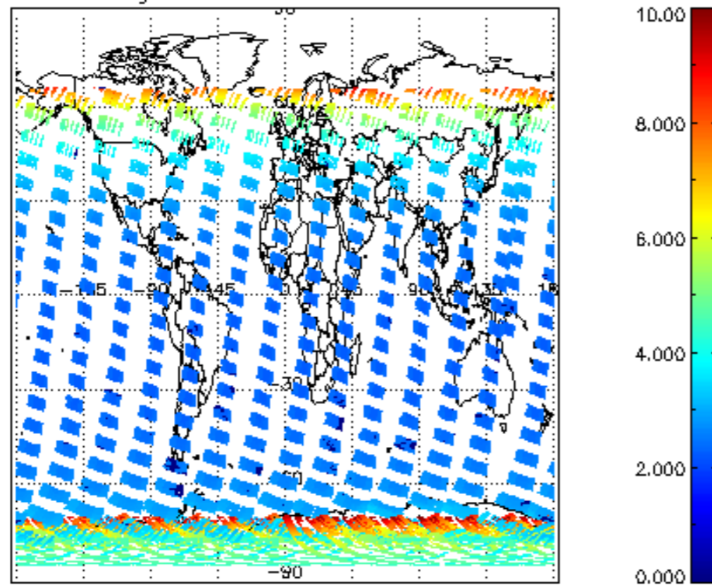
SCIOL2P_NADUV003_amf_gr for 15JAN2004 00:00:00 to 16JAN2004 00:00:00
