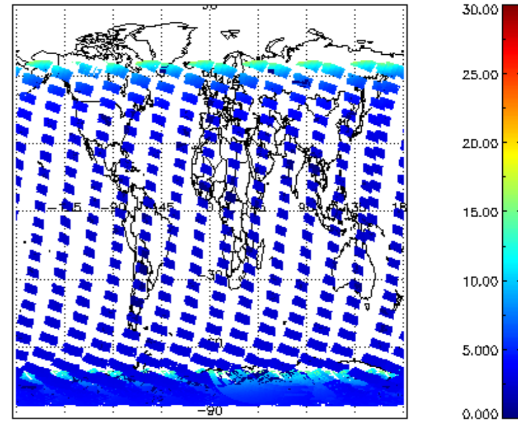
SCIOL2P_NADUV1NO2_amf_cl for 15JAN2004 00:00:00 to 16JAN2004 00:00:00
