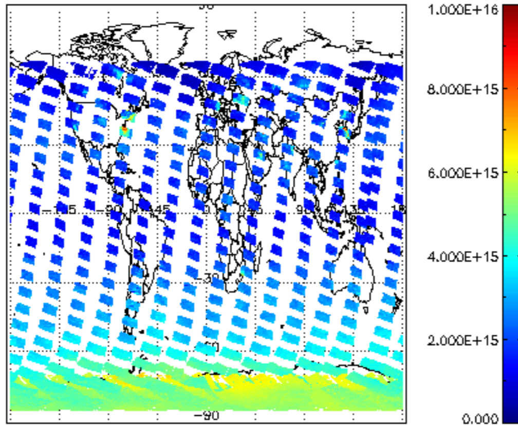
SCIOL2P_NADUV1NO2_vcd for 15JAN2004 00:00:00 to 16JAN2004 00:00:00
