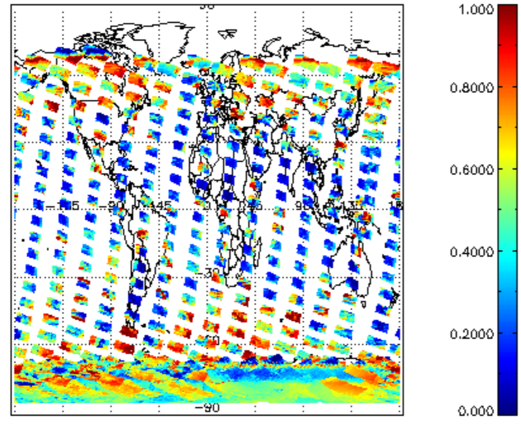
cL_frac for 15JAN2004 00:00:00 to 16JAN2004 00:00:00
