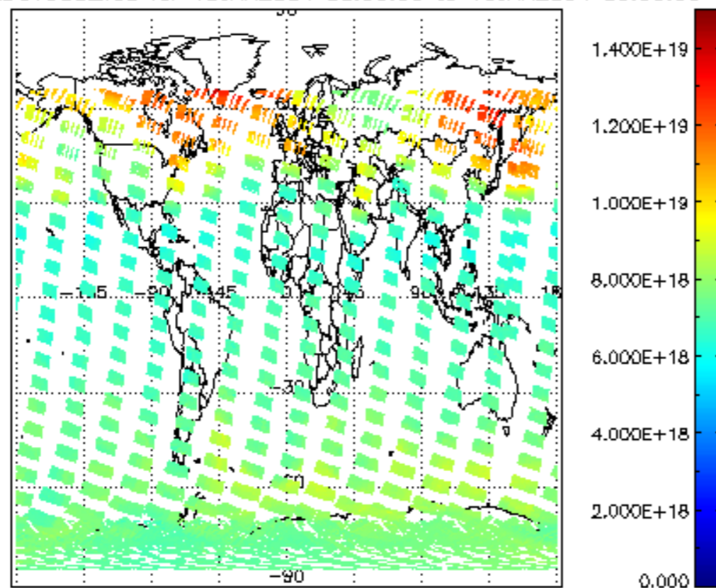
SCIOL2P_NADUV003_vcd for 15JAN2004 00:00:00 to 16JAN2004 00:00:00
