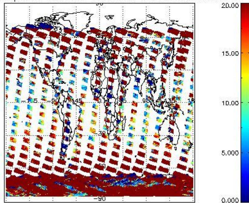
cLopt_depth for 15JAN2004 00:00:00 to 16JAN2004 00:00:00
