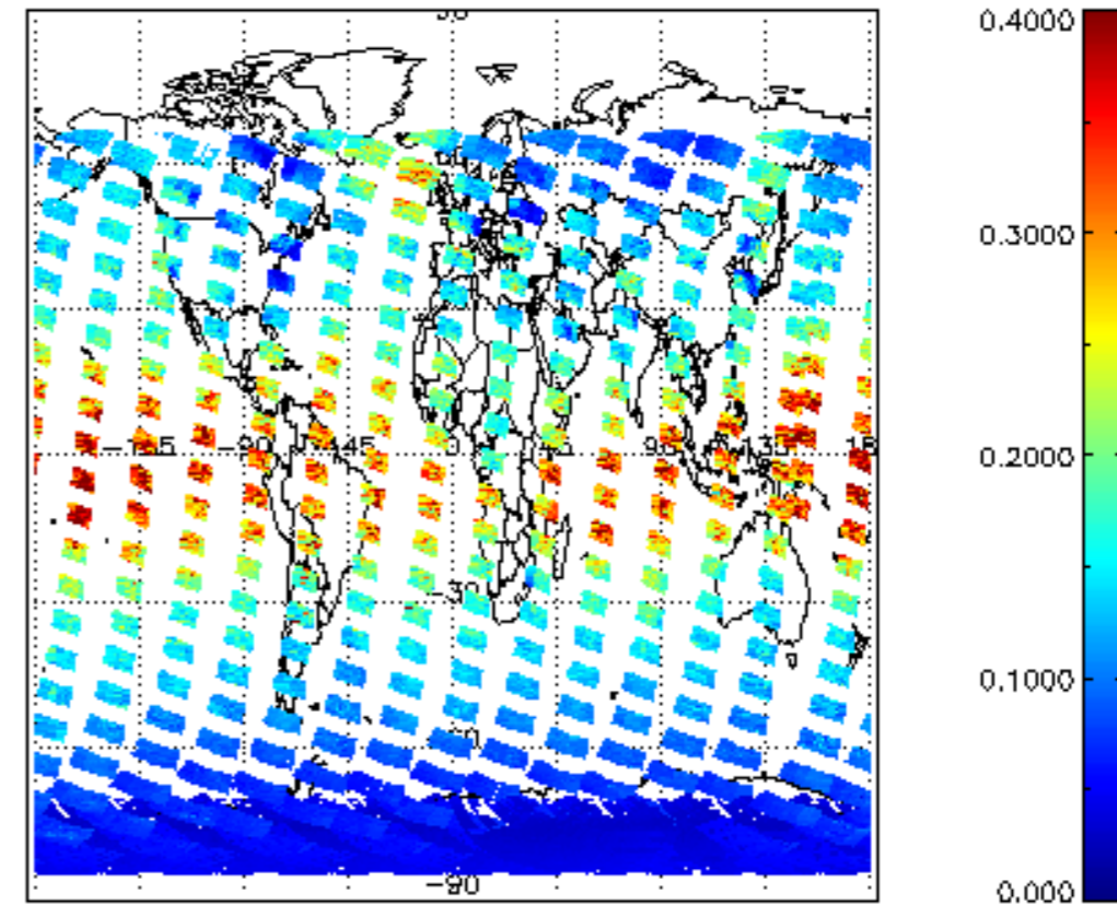
SCIOL2P_NADUV1NO2_vcd_err for 15JAN2004 00:00:00 to 16JAN2004 00:00:00
