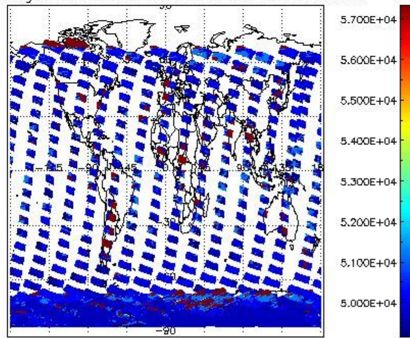
cloud_flags for 15JAN2004 00:00:00 to 16JAN2004 00:00:00
