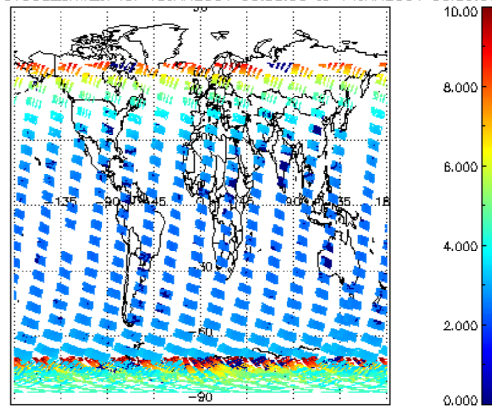
SCIOL2P_NADUV003_amf_cl for 13JAN2004 00:00:00 to 14JAN2004 00:00:00
