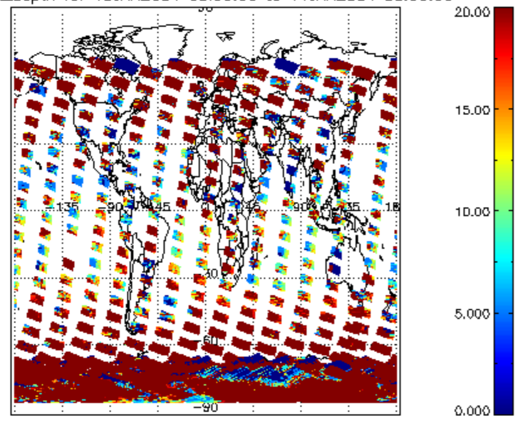
cL_opt_depth for 13JAN2004 00:00:00 to 14JAN2004 00:00:00
