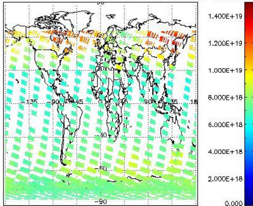
SCIOL2P_NADUV003_vcd for 13JAN2004 00:00:00 to 14JAN2004 00:00:00
