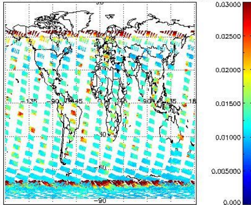
SCIOL2P_NADUV003_vcd_err for 13JAN2004 00:00:00 to 14JAN2004 00:00:00
