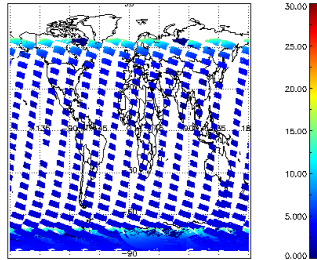
SCIOL2P_NADUV1NO2_amf_cl for 13JAN2004 00:00:00 to 14JAN2004 00:00:00
