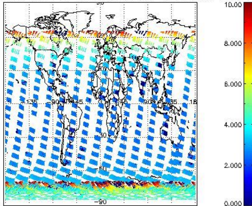
SCIOL2P_NADUV003_amf_cl for 13JAN2004 00:00:00 to 14JAN2004 00:00:00
