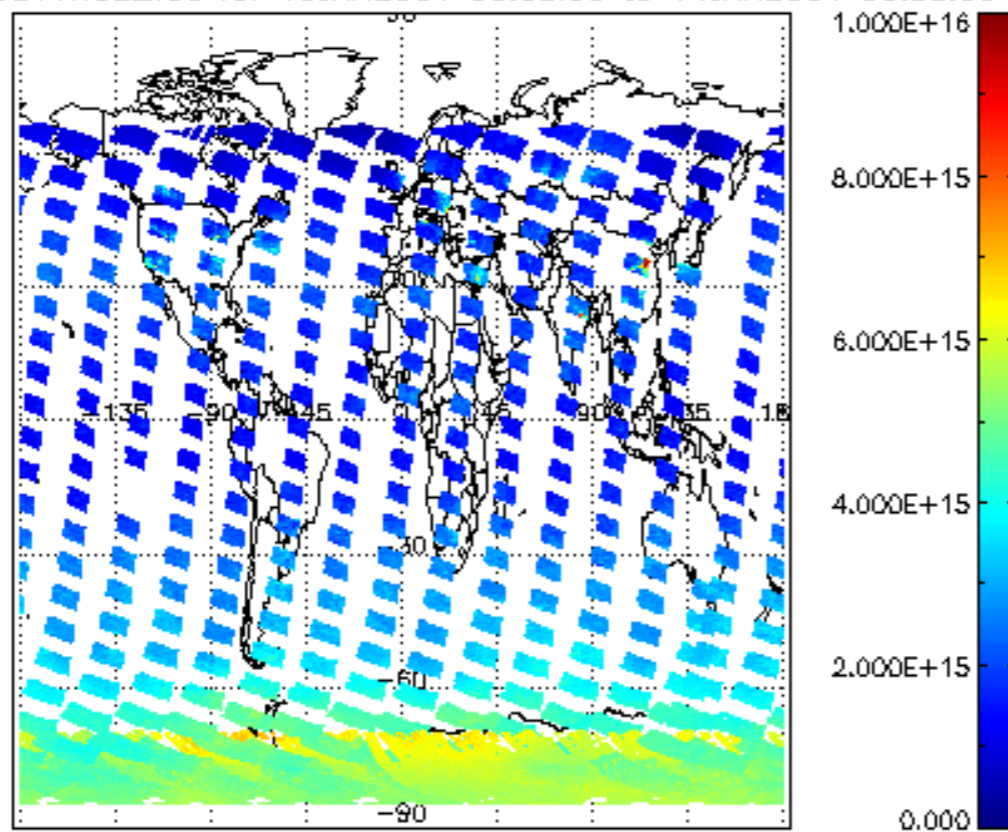
SCIOL2P_NADUV1NO2_vcd for 13JAN2004 00:00:00 to 14JAN2004 00:00:00
