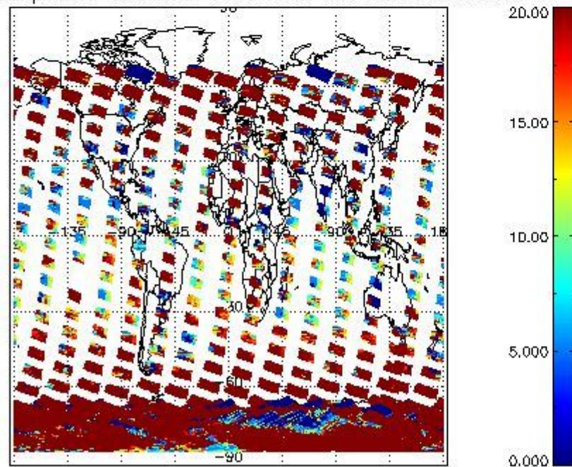
cLopt_depth for 13JAN2004 00:00:00 to 14JAN2004 00:00:00
