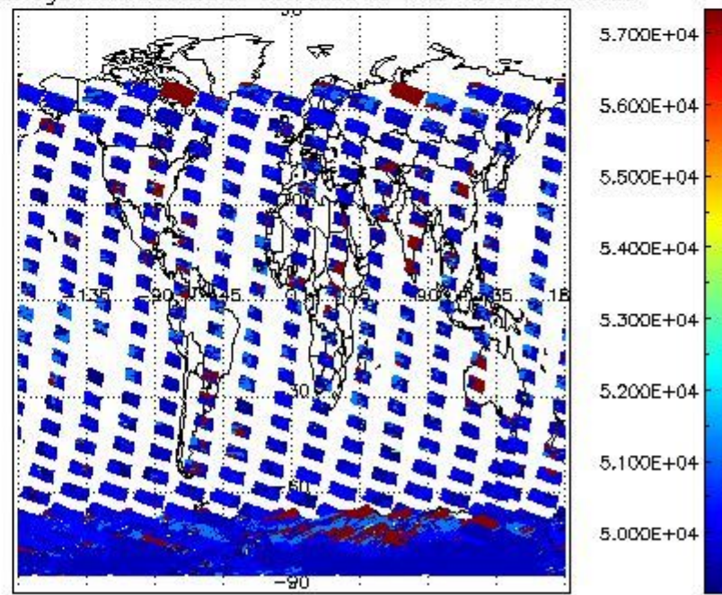
cloud_flags for 13JAN2004 00:00:00 to 14JAN2004 00:00:00
