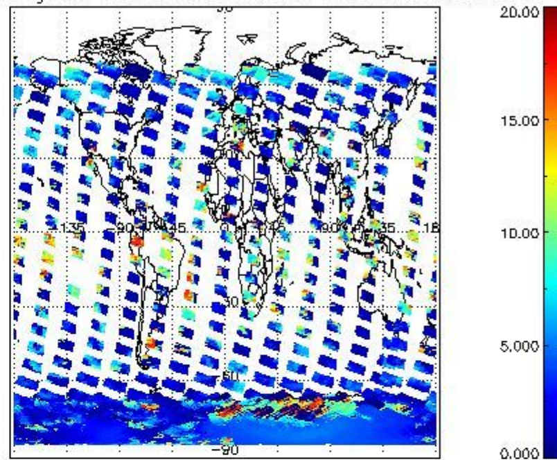
cL_top_height for 13JAN2004 00:00:00 to 14JAN2004 00:00:00
