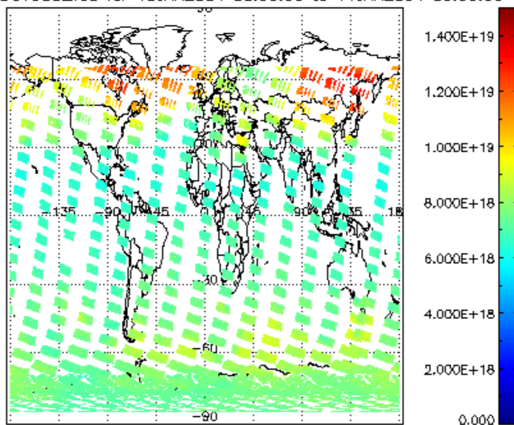
SCIOL2P_NADUV003_vcd for 13JAN2004 00:00:00 to 14JAN2004 00:00:00
