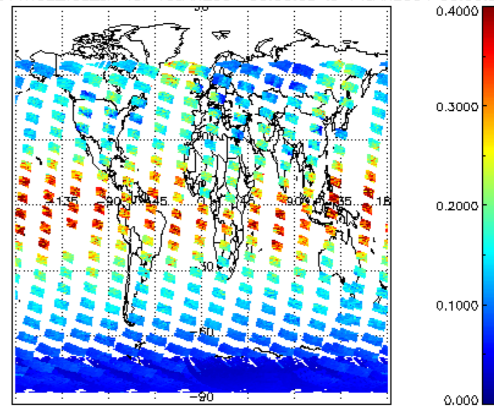
SCIOL2P_NADUV1NO2_vcd_err for 13JAN2004 00:00:00 to 14JAN2004 00:00:00
