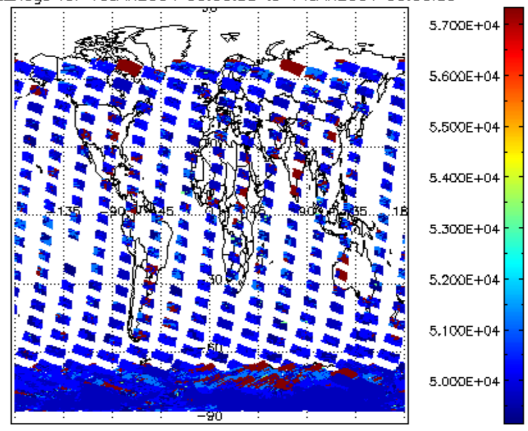
cloud_flags for 13JAN2004 00:00:00 to 14JAN2004 00:00:00
