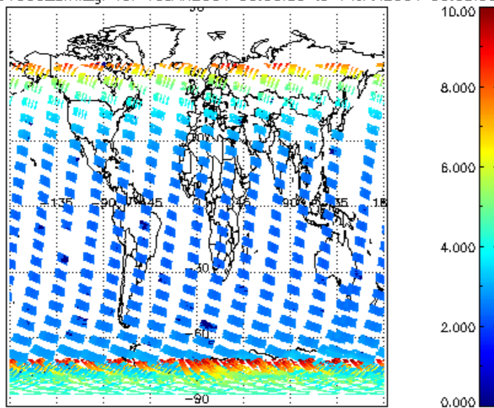
SCIOL2P_NADUV003_amf_gr for 13JAN2004 00:00:00 to 14JAN2004 00:00:00
