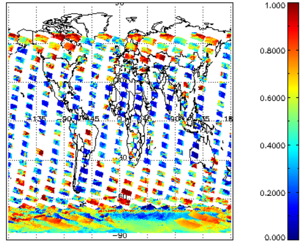
cL_frac for 13JAN2004 00:00:00 to 14JAN2004 00:00:00
