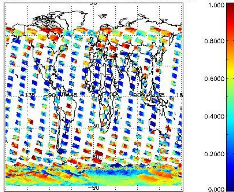
cL_frac for 13JAN2004 00:00:00 to 14JAN2004 00:00:00
