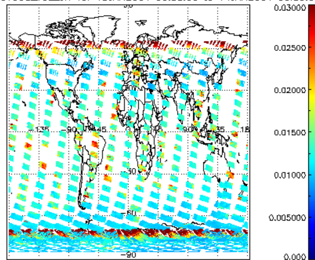
SCIOL2P_NADUV003_vcd_err for 13JAN2004 00:00:00 to 14JAN2004 00:00:00
