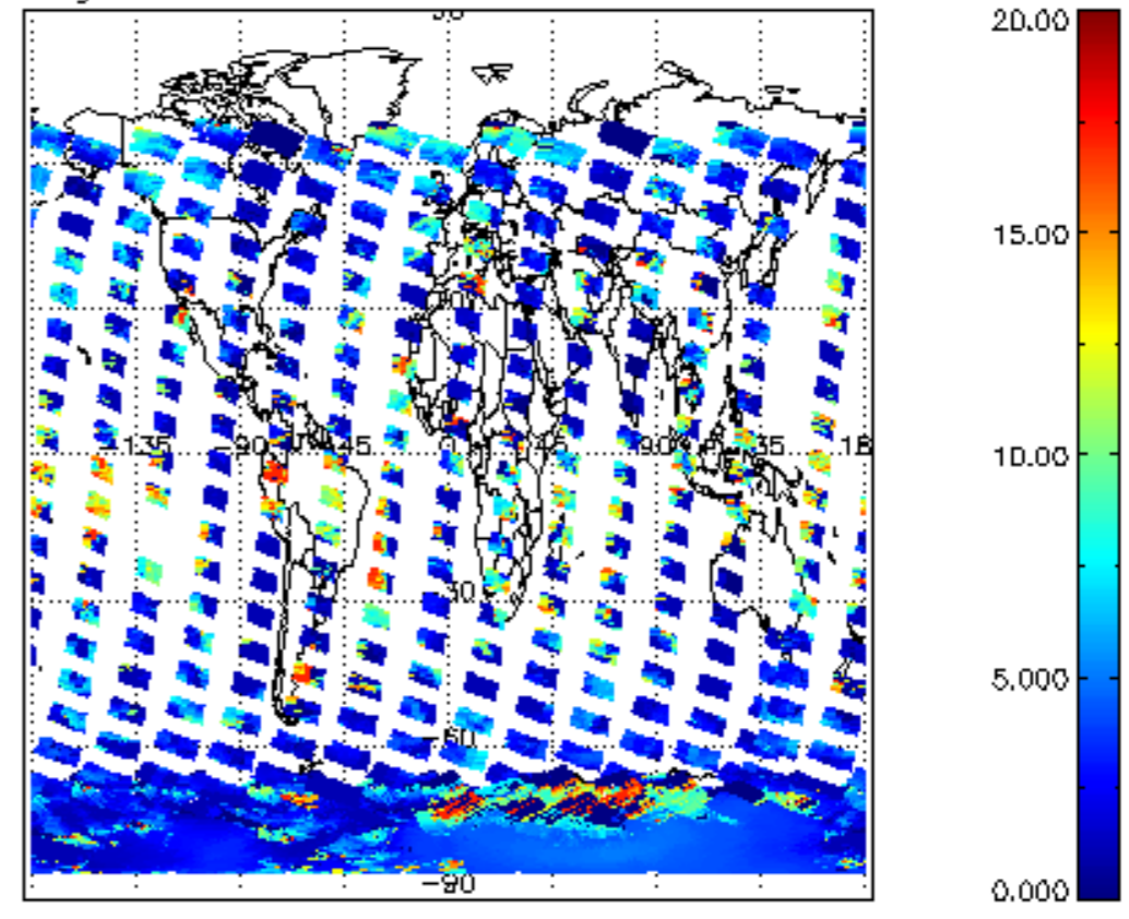
cL_top_height for 13JAN2004 00:00:00 to 14JAN2004 00:00:00
