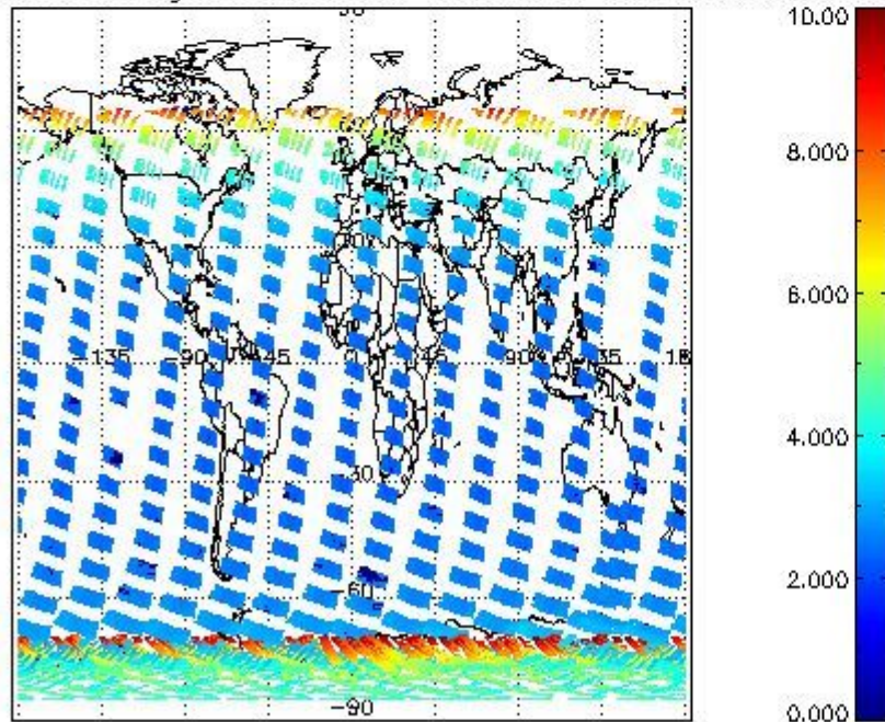
SCIOL2P_NADUV003_amf_gr for 13JAN2004 00:00:00 to 14JAN2004 00:00:00
