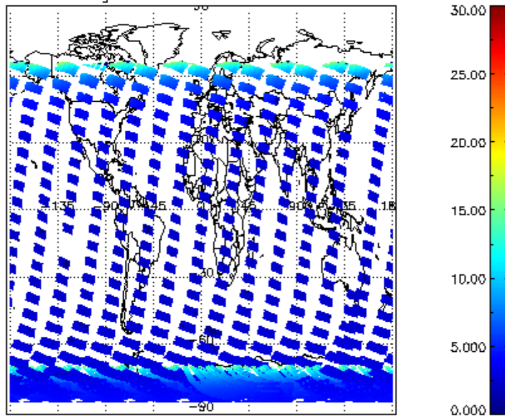
SCIOL2P_NADUV1NO2_amf_gr for 13JAN2004 00:00:00 to 14JAN2004 00:00:00
