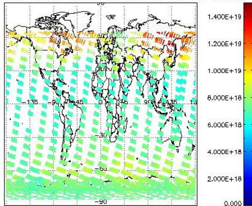
SCIOL2P_NADUV003_vcd for 12JAN2004 00:00:00 to 13JAN2004 00:00:00
