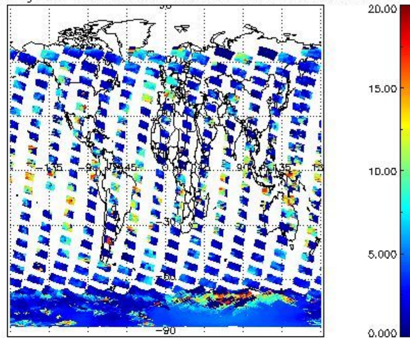
cL_top_height for 12JAN2004 00:00:00 to 13JAN2004 00:00:00
