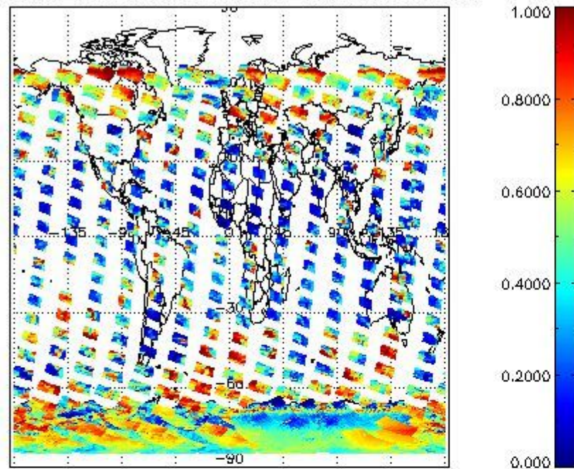
cL_frac for 12JAN2004 00:00:00 to 13JAN2004 00:00:00
