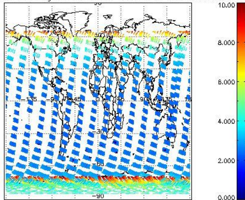
SCIOL2P_NADUV003_amf_gr for 12JAN2004 00:00:00 to 13JAN2004 00:00:00
