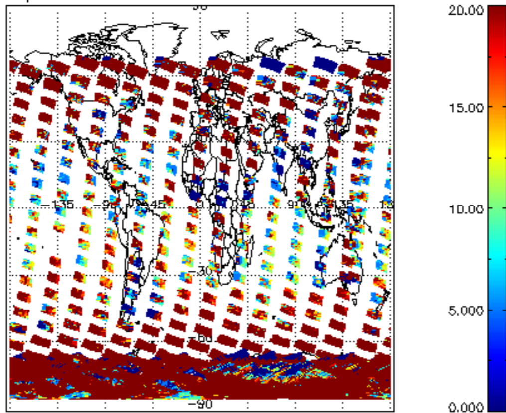
cLopt_depth for 12JAN2004 00:00:00 to 13JAN2004 00:00:00
