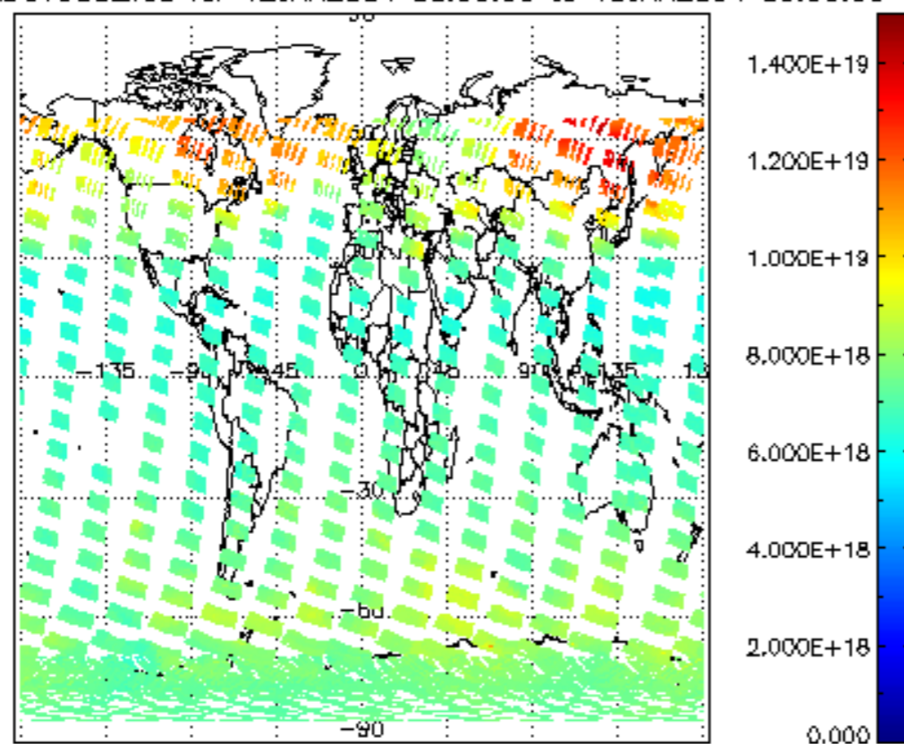
SCIOL2P_NADUV003_vcd for 12JAN2004 00:00:00 to 13JAN2004 00:00:00
