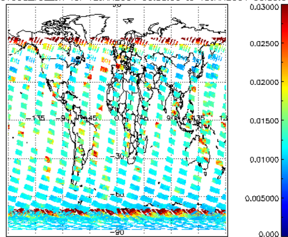
SCIOL2P_NADUV003_vcd_err for 12JAN2004 00:00:00 to 13JAN2004 00:00:00
