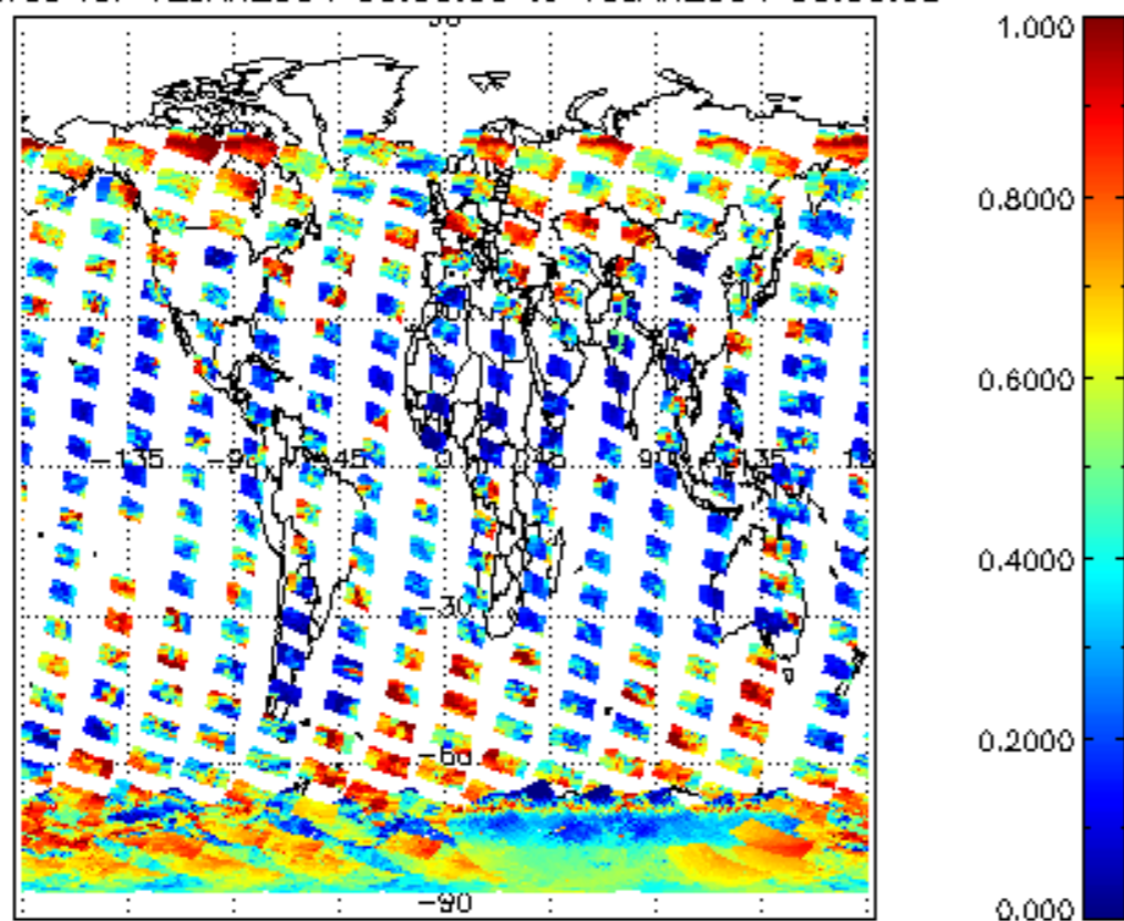
cL_frac for 12JAN2004 00:00:00 to 13JAN2004 00:00:00
