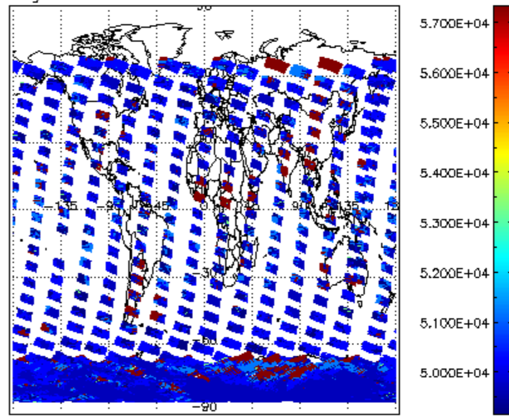
cloud_flags for 12JAN2004 00:00:00 to 13JAN2004 00:00:00
