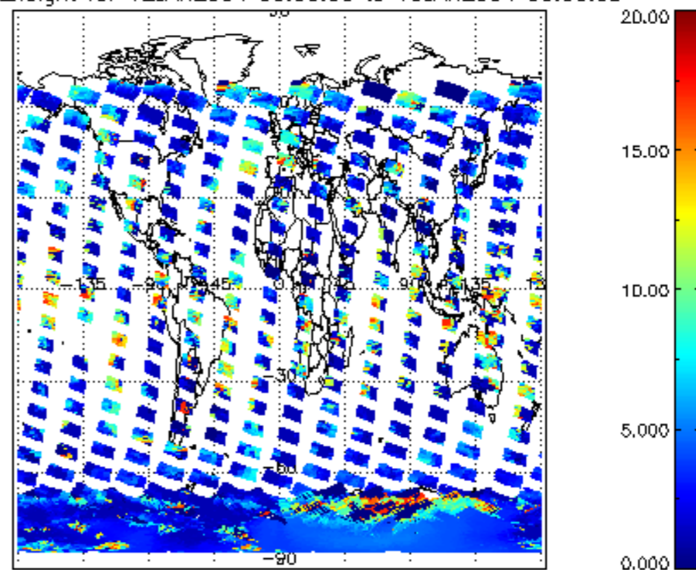
cL_top_height for 12JAN2004 00:00:00 to 13JAN2004 00:00:00
