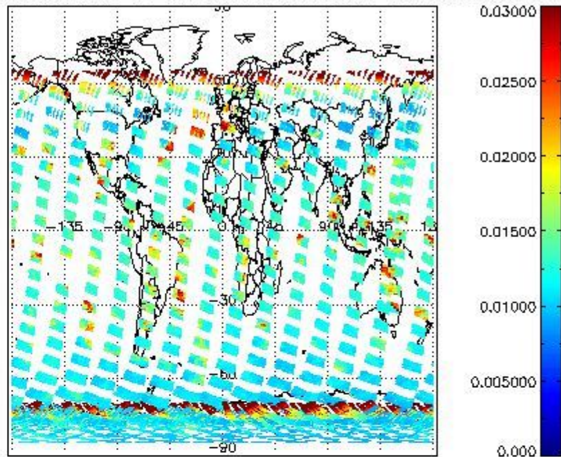
SCIOL2P_NADUV003_vcd_err for 12JAN2004 00:00:00 to 13JAN2004 00:00:00
