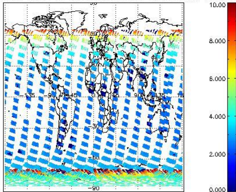
SCIOL2P_NADUV003_amf_cl for 12JAN2004 00:00:00 to 13JAN2004 00:00:00
