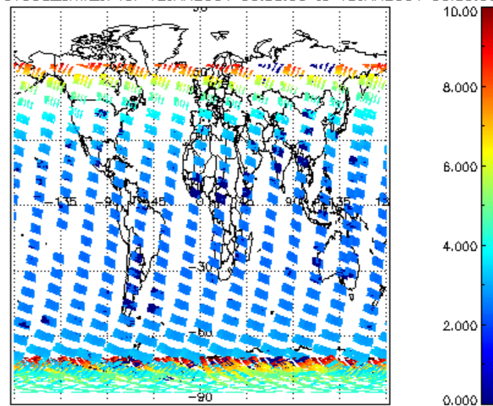
SCIOL2P_NADUV003_amf_cl for 12JAN2004 00:00:00 to 13JAN2004 00:00:00
