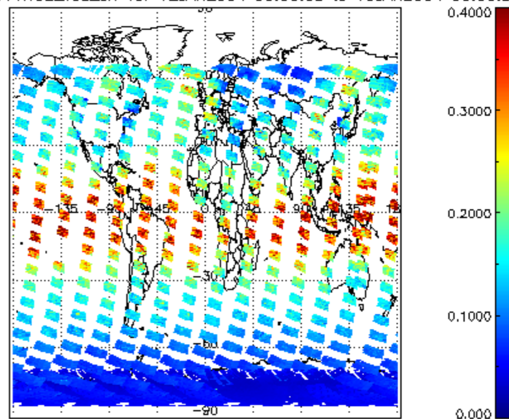
SCIOL2P_NADUV1NO2_vcd_err for 12JAN2004 00:00:00 to 13JAN2004 00:00:00
