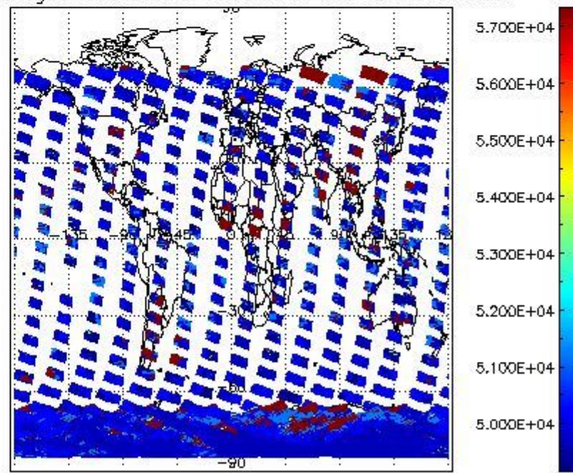
cloud_flags for 12JAN2004 00:00:00 to 13JAN2004 00:00:00
