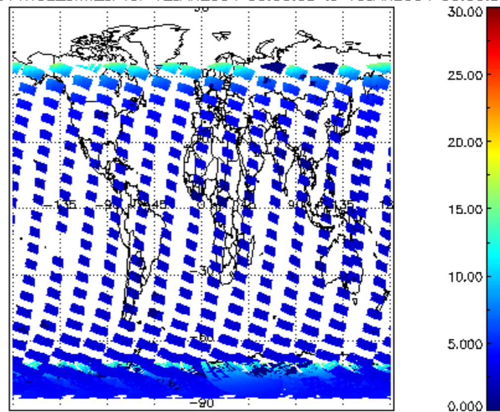
SCIOL2P_NADUV1NO2_amf_cl for 12JAN2004 00:00:00 to 13JAN2004 00:00:00
