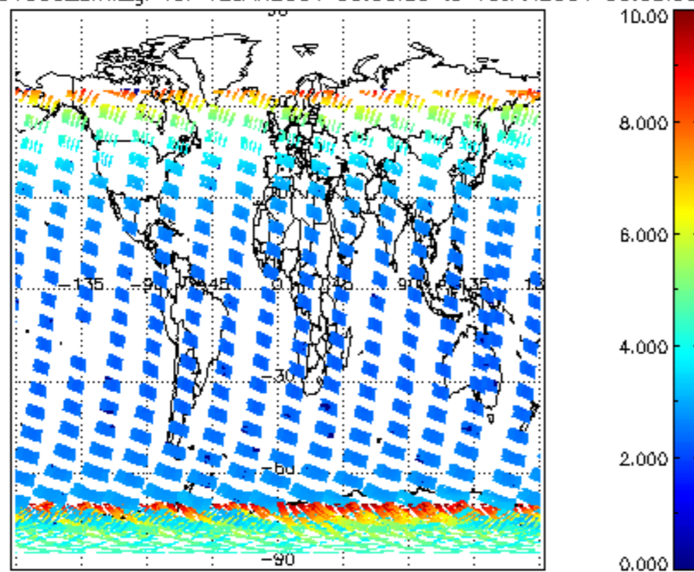
SCIOL2P_NADUV003_amf_gr for 12JAN2004 00:00:00 to 13JAN2004 00:00:00
