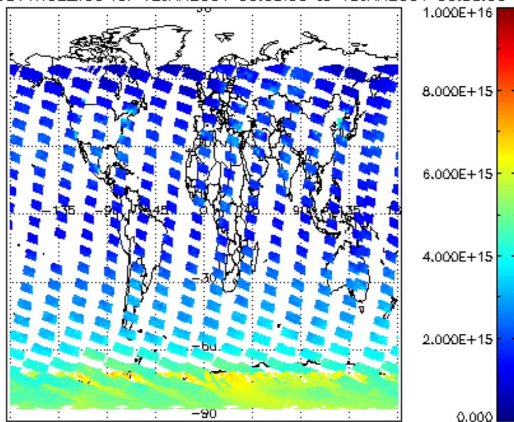
SCIOL2P_NADUV1NO2_vcd for 12JAN2004 00:00:00 to 13JAN2004 00:00:00
