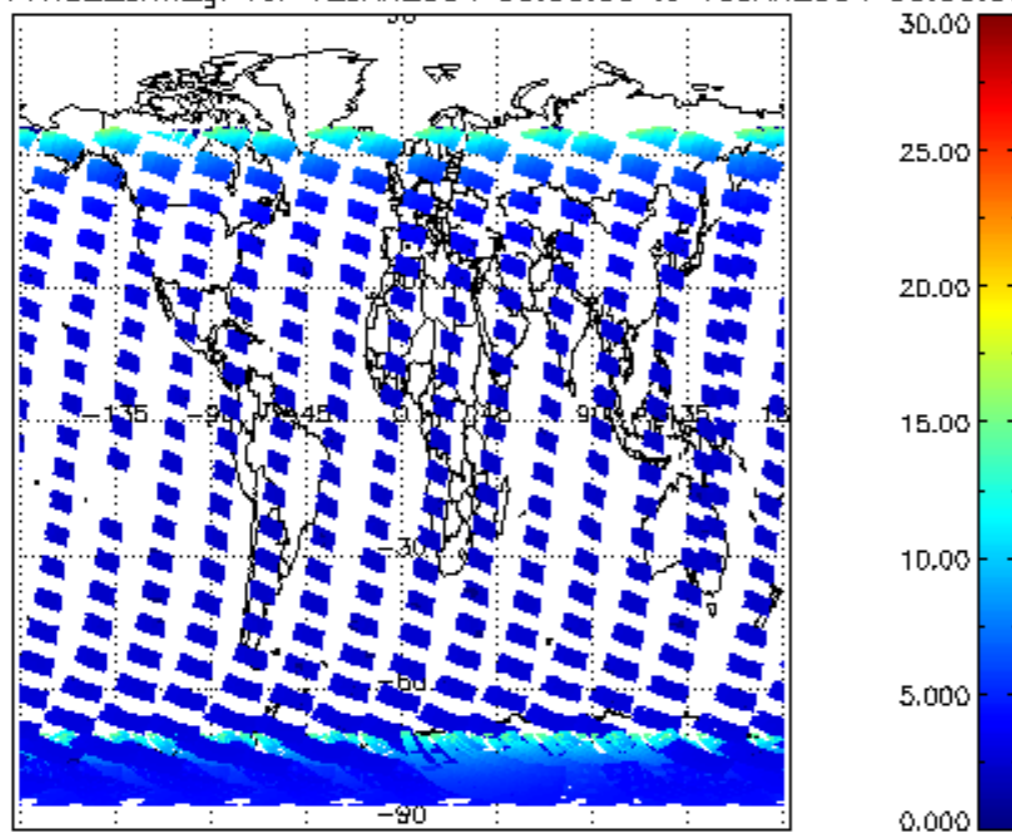
SCIOL2P_NADUV1NO2_amf_gr for 12JAN2004 00:00:00 to 13JAN2004 00:00:00
