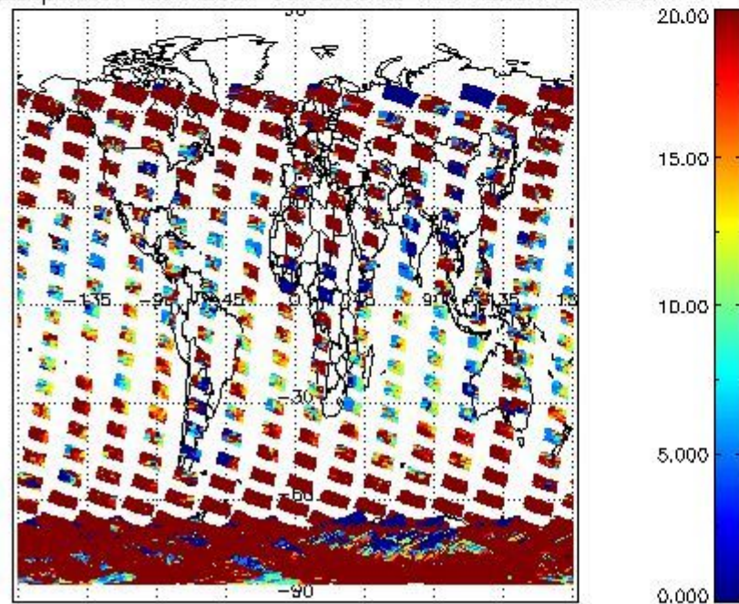
cLopt_depth for 12JAN2004 00:00:00 to 13JAN2004 00:00:00
