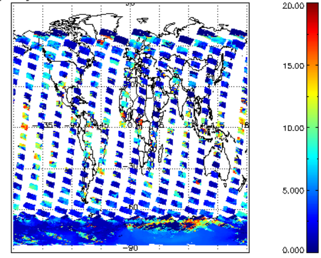
cL_top_height for 08JAN2004 00:00:00 to 09JAN2004 00:00:00
