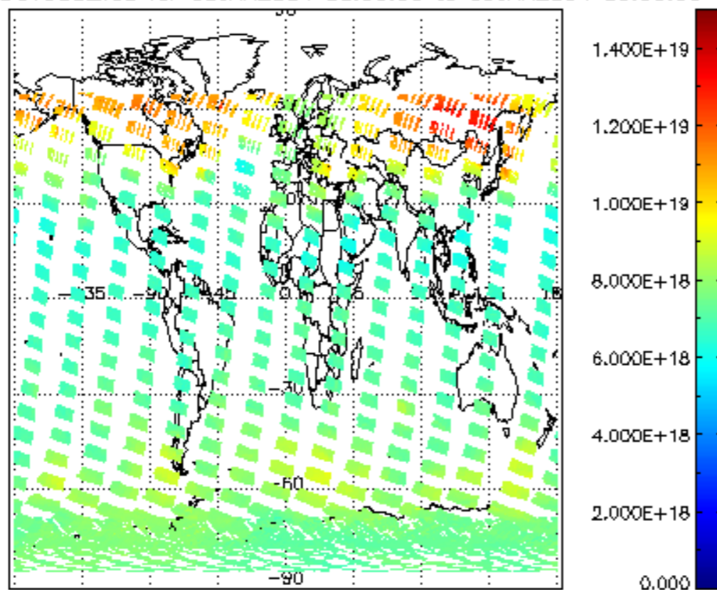
SCIOL2P_NADUV003_vcd for 08JAN2004 00:00:00 to 09JAN2004 00:00:00
