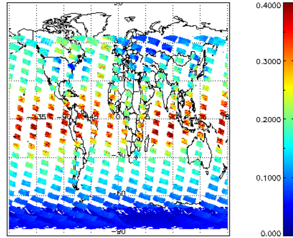
SCIOL2P_NADUV1NO2_vcd_err for 08JAN2004 00:00:00 to 09JAN2004 00:00:00
