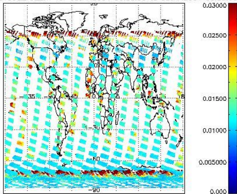
SCIOL2P_NADUV003_vcd_err for 08JAN2004 00:00:00 to 09JAN2004 00:00:00
