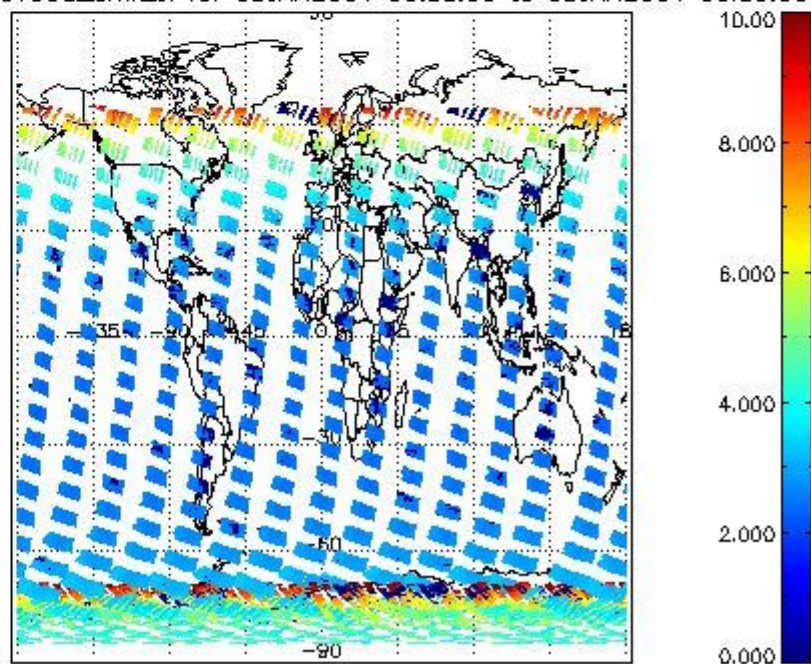
SCIOL2P_NADUV003_amf_cl for 08JAN2004 00:00:00 to 09JAN2004 00:00:00
