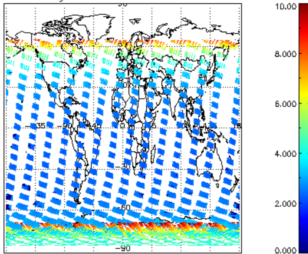
SCIOL2P_NADUV003_amf_gr for 08JAN2004 00:00:00 to 09JAN2004 00:00:00
