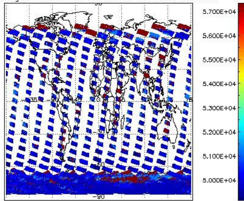
cloud_flags for 08JAN2004 00:00:00 to 09JAN2004 00:00:00
