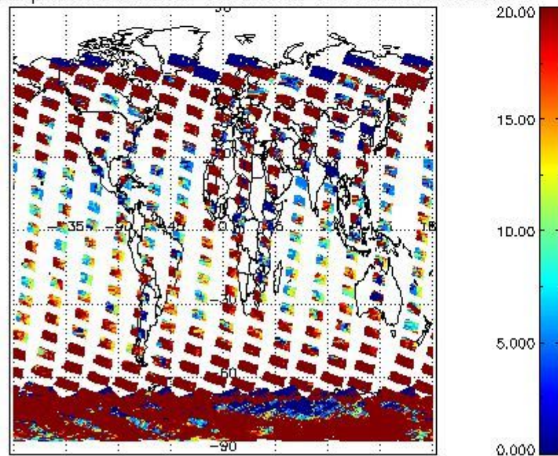
cLopt_depth for 08JAN2004 00:00:00 to 09JAN2004 00:00:00
