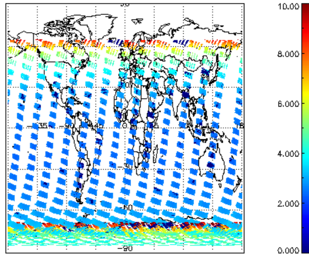
SCIOL2P_NADUV003_amf_cl for 08JAN2004 00:00:00 to 09JAN2004 00:00:00
