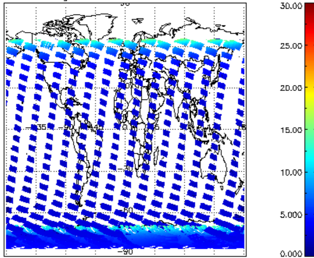
SCIOL2P_NADUV1NO2_amf_gr for 08JAN2004 00:00:00 to 09JAN2004 00:00:00
