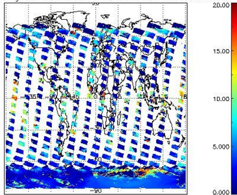
cL_top_height for 08JAN2004 00:00:00 to 09JAN2004 00:00:00
