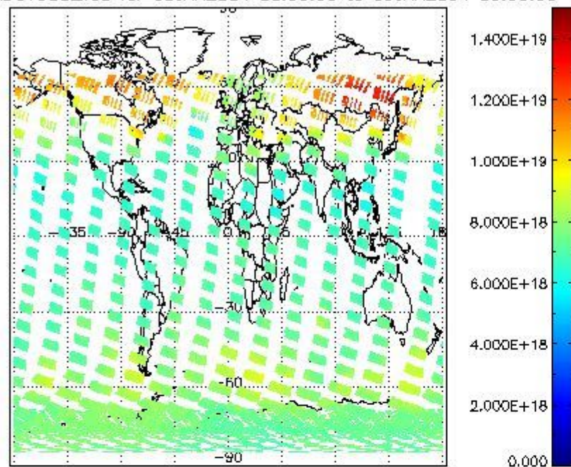
SCIOL2P_NADUV003_vcd for 08JAN2004 00:00:00 to 09JAN2004 00:00:00
