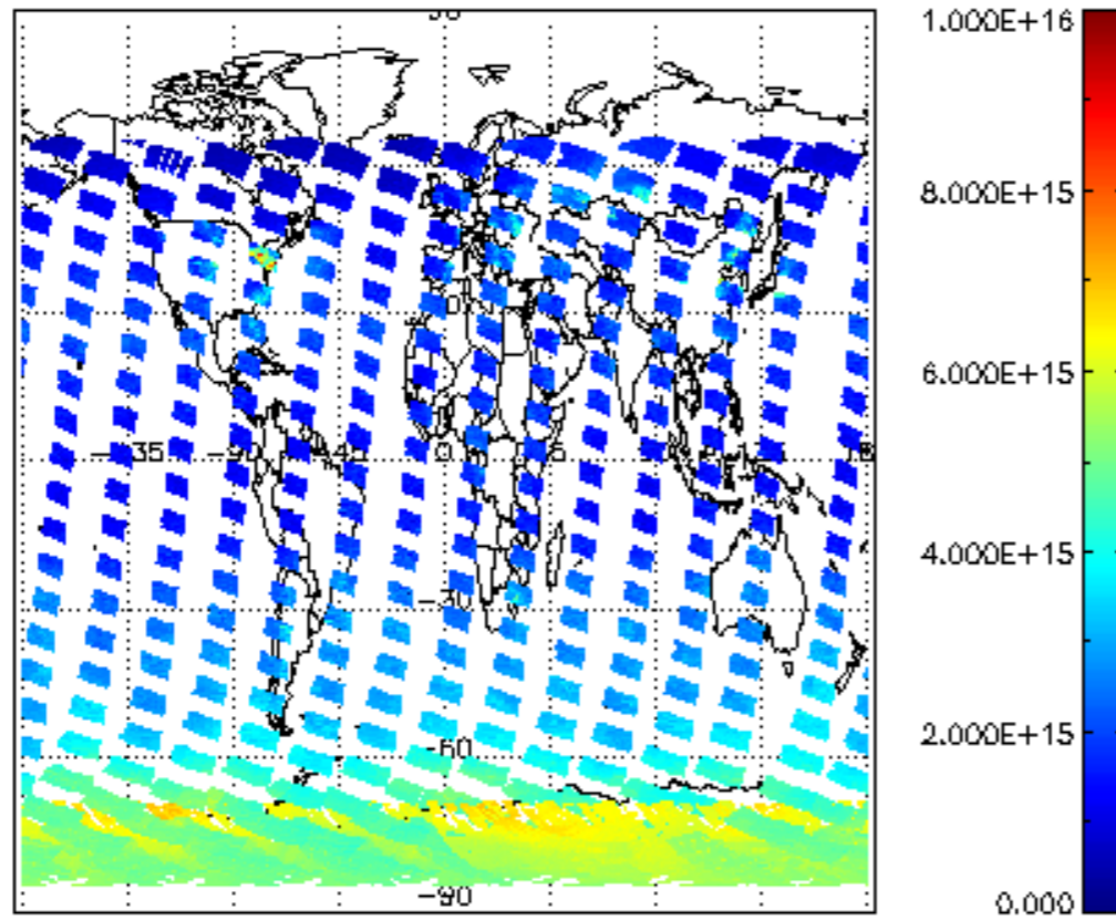
SCIOL2P_NADUV1NO2_vcd for 08JAN2004 00:00:00 to 09JAN2004 00:00:00
