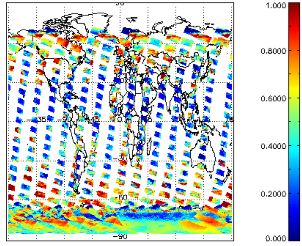
cL_frac for 08JAN2004 00:00:00 to 09JAN2004 00:00:00
