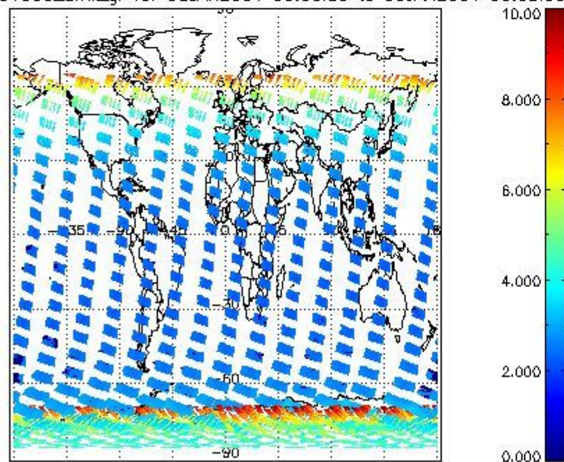
SCIOL2P_NADUV003_amf_gr for 08JAN2004 00:00:00 to 09JAN2004 00:00:00
