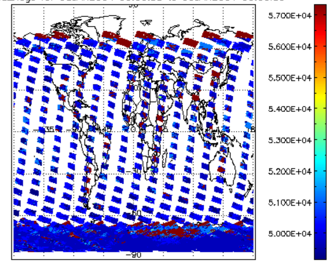
cloud_flags for 08JAN2004 00:00:00 to 09JAN2004 00:00:00
