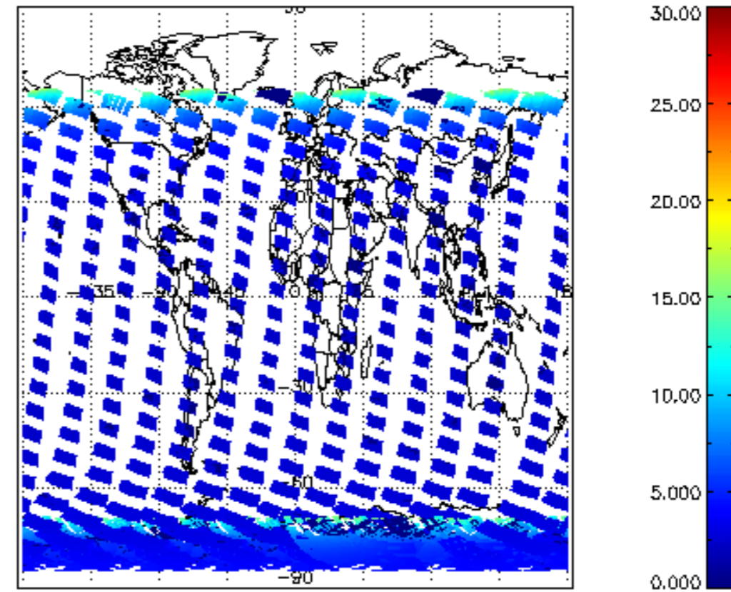
SCIOL2P_NADUV1NO2_amf_cl for 08JAN2004 00:00:00 to 09JAN2004 00:00:00
