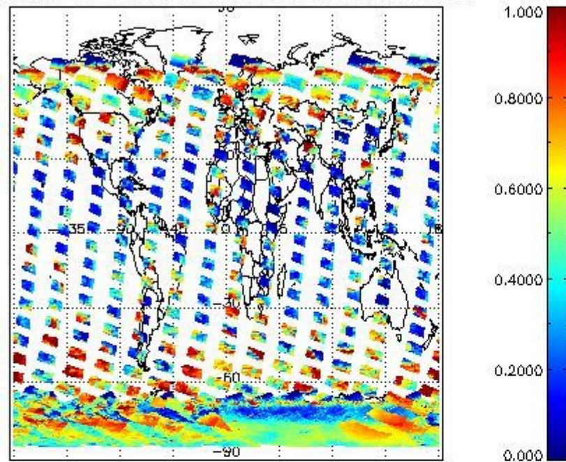
cL_frac for 08JAN2004 00:00:00 to 09JAN2004 00:00:00
