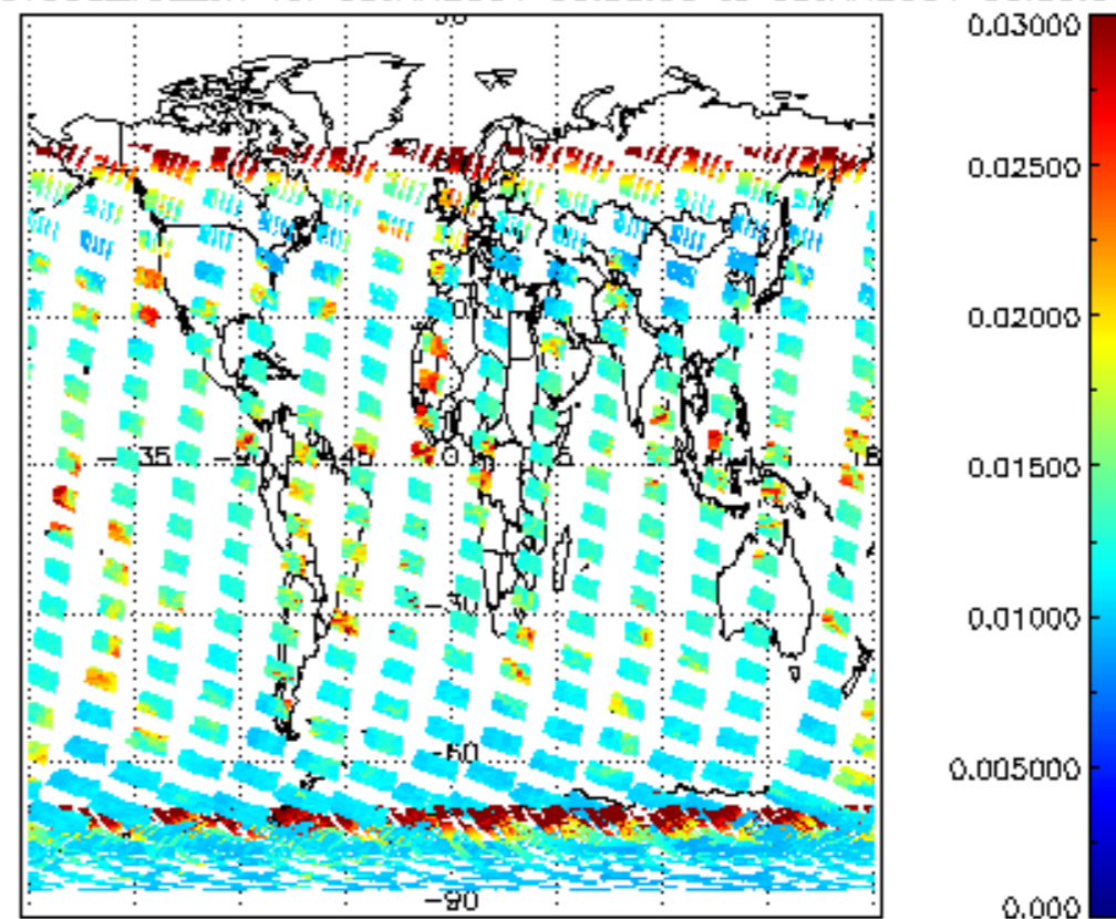
SCIOL2P_NADUV003_vcd_err for 08JAN2004 00:00:00 to 09JAN2004 00:00:00
