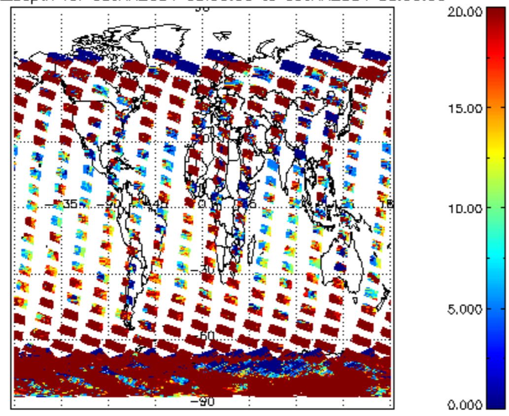
cL_opt_depth for 08JAN2004 00:00:00 to 09JAN2004 00:00:00
