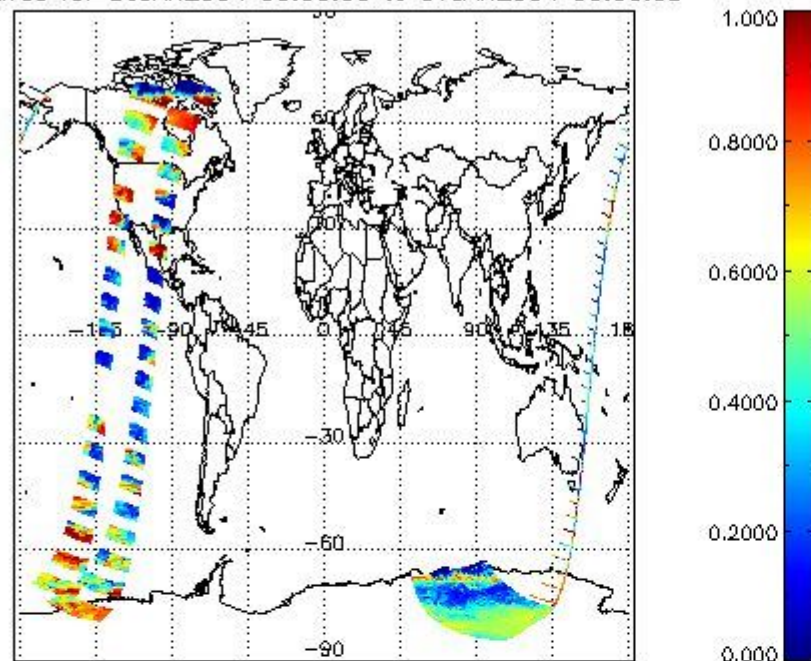
cL_frac for 06JAN2004 00:00:00 to 07JAN2004 00:00:00
