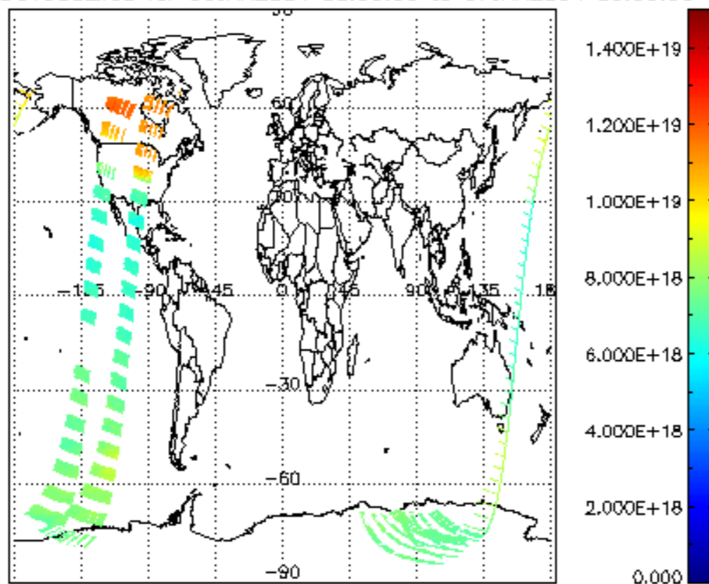
SCIOL2P_NADUV003_vcd for 06JAN2004 00:00:00 to 07JAN2004 00:00:00
