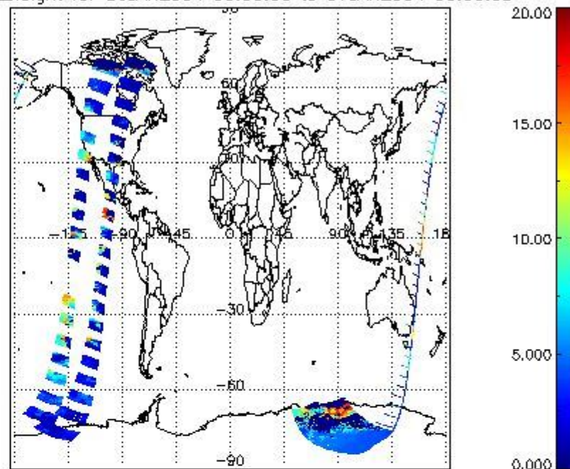
cL_top_height for 06JAN2004 00:00:00 to 07JAN2004 00:00:00
