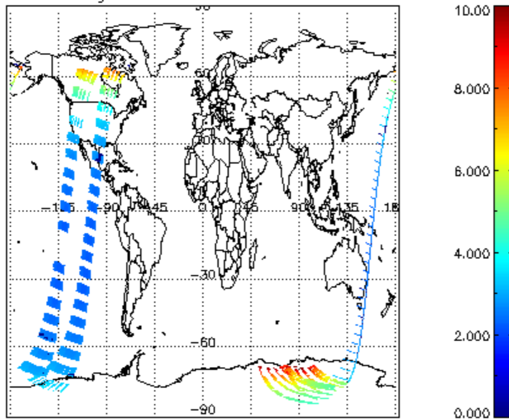
SCIOL2P_NADUV003_amf_gr for 06JAN2004 00:00:00 to 07JAN2004 00:00:00
