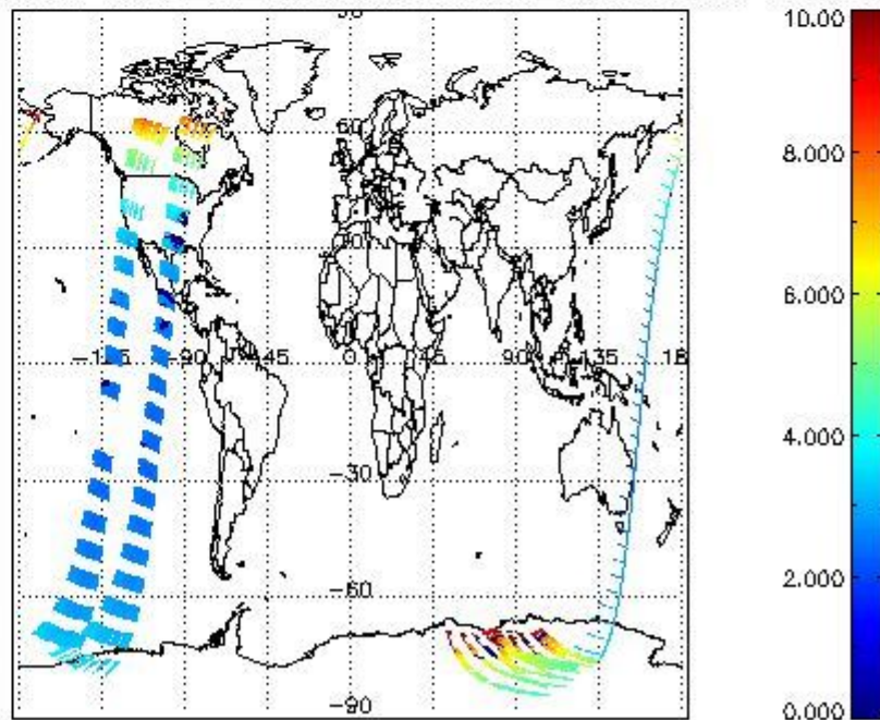
SCIOL2P_NADUV003_amf_cl for 06JAN2004 00:00:00 to 07JAN2004 00:00:00
