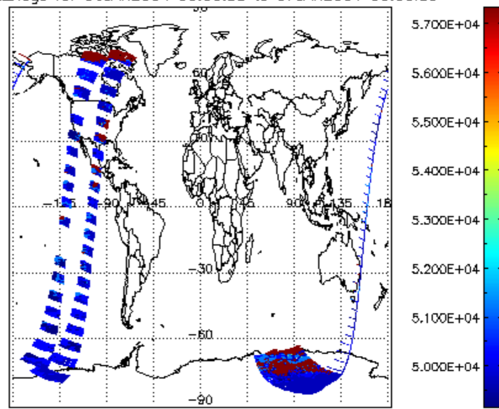
cloud_flags for 06JAN2004 00:00:00 to 07JAN2004 00:00:00
