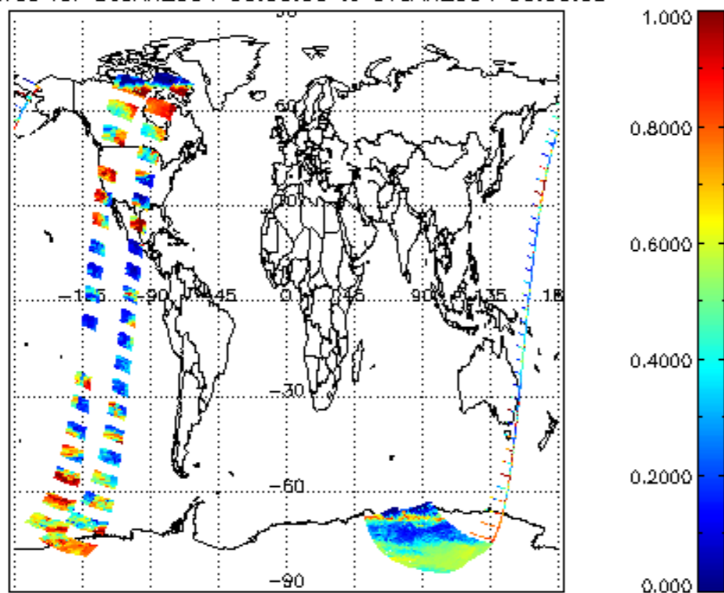
cL_frac for 06JAN2004 00:00:00 to 07JAN2004 00:00:00
