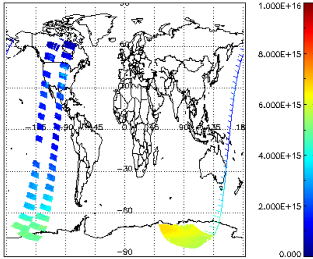
SCIOL2P_NADUV1NO2_vcd for 06JAN2004 00:00:00 to 07JAN2004 00:00:00
