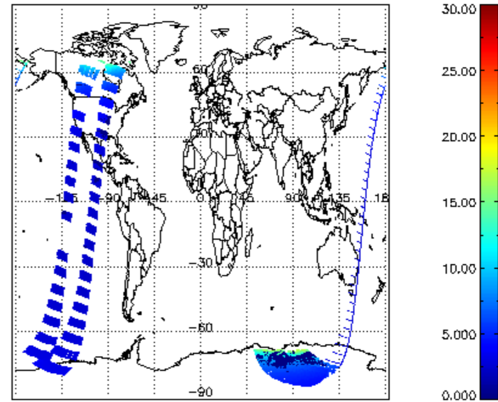
SCIOL2P_NADUV1NO2_amf_cl for 06JAN2004 00:00:00 to 07JAN2004 00:00:00
