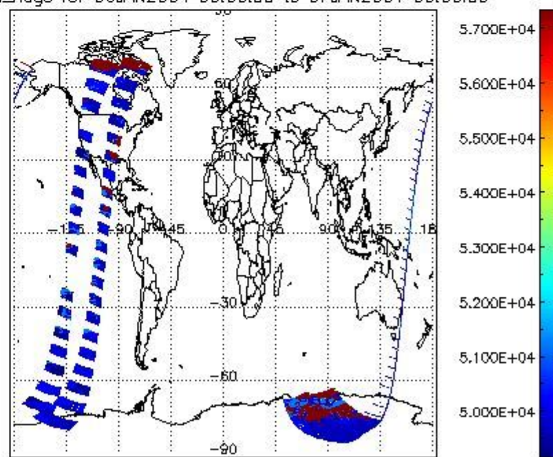
cloud_flags for 06JAN2004 00:00:00 to 07JAN2004 00:00:00
