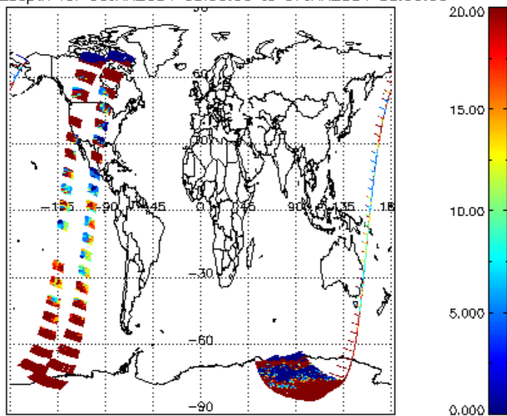
cLopt_depth for 06JAN2004 00:00:00 to 07JAN2004 00:00:00
