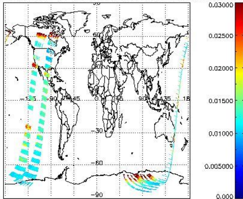
SCIOL2P_NADUV003_vcd_err for 06JAN2004 00:00:00 to 07JAN2004 00:00:00
