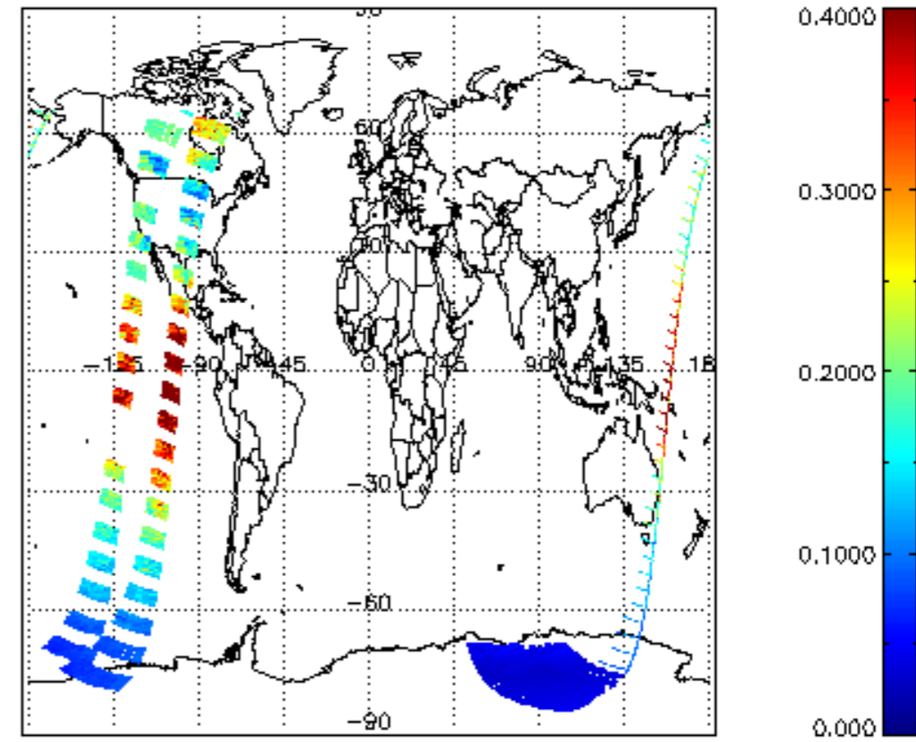
SCIOL2P_NADUV1NO2_vcd_err for 06JAN2004 00:00:00 to 07JAN2004 00:00:00
