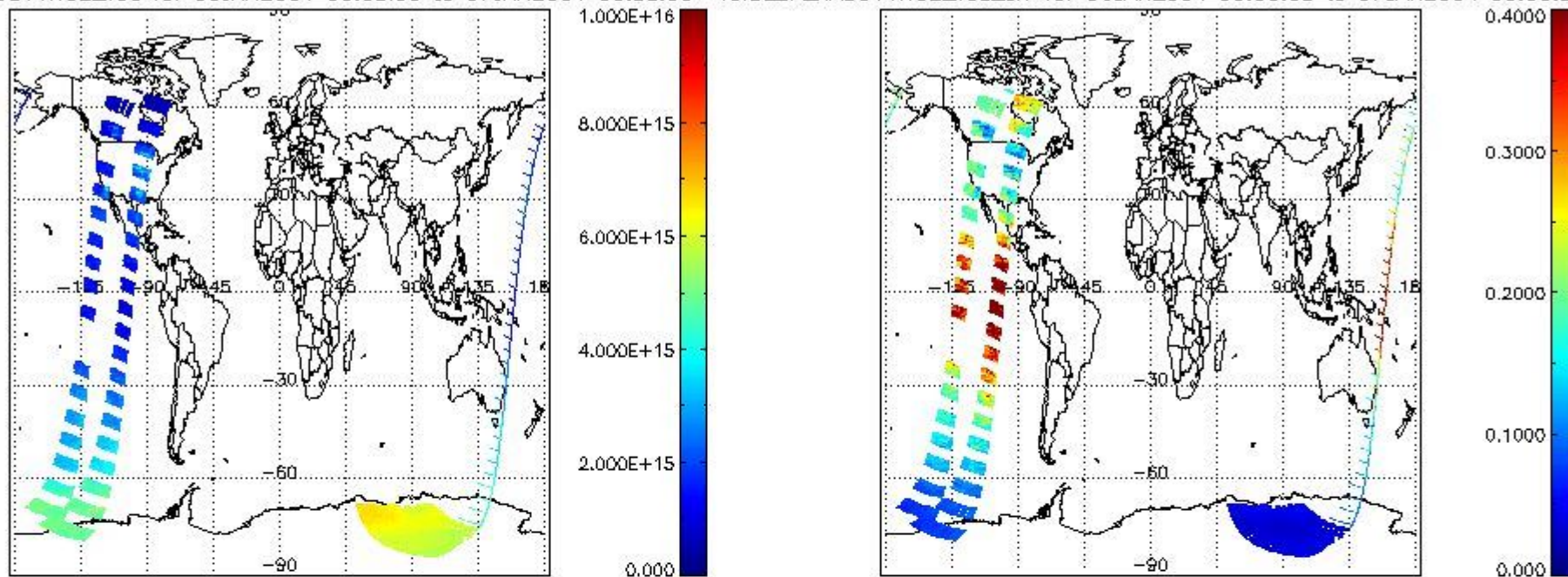
SCIOL2P_NADUV1NO2_vcd for 06JAN2004 00:00:00 to 07JAN2004 00:00:00 SCIOL2P_NADUV1NO2_vcd_err for 06JAN2004 00:00:00 to 07JAN2004 00:00:00
