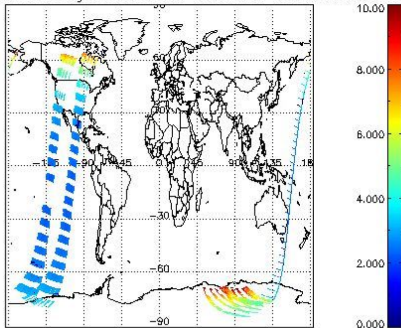
SCIOL2P_NADUV003_amf_gr for 06JAN2004 00:00:00 to 07JAN2004 00:00:00
