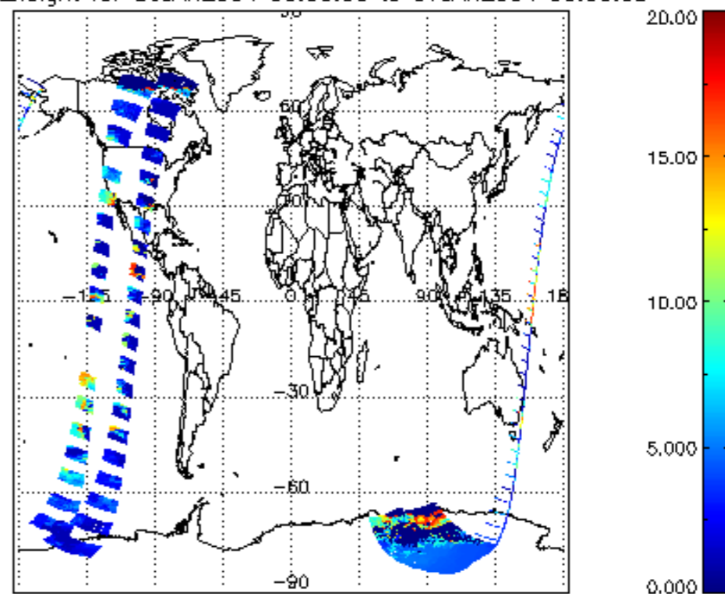
cL_top_height for 06JAN2004 00:00:00 to 07JAN2004 00:00:00
