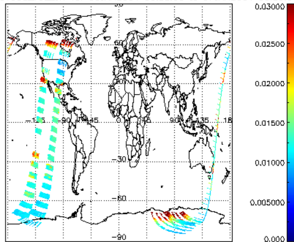
SCIOL2P_NADUV003_vcd_err for 06JAN2004 00:00:00 to 07JAN2004 00:00:00
