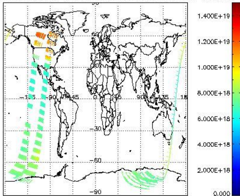
SCIOL2P_NADUV003_vcd for 06JAN2004 00:00:00 to 07JAN2004 00:00:00
