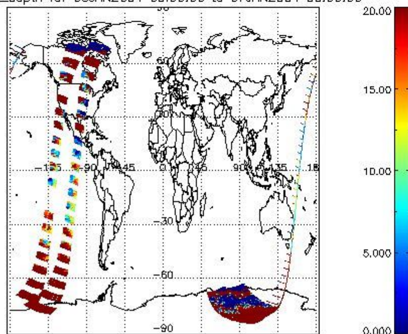
cLopt_depth for 06JAN2004 00:00:00 to 07JAN2004 00:00:00
