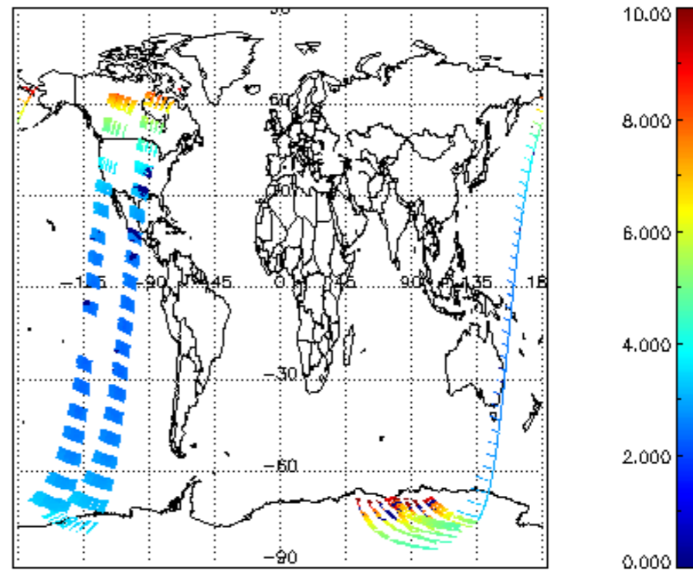
SCIOL2P_NADUV003_amf_cl for 06JAN2004 00:00:00 to 07JAN2004 00:00:00
