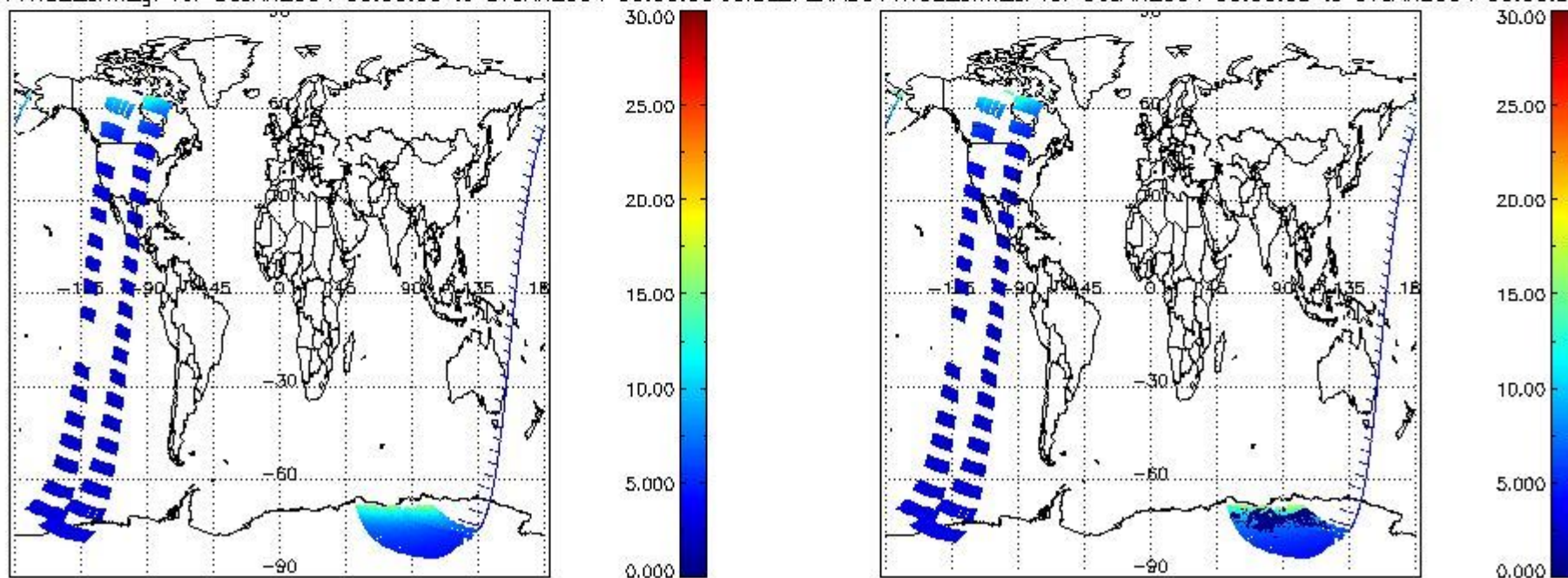
SCIOL2P_NADUV1NO2_amf_gr for 06JAN2004 00:00:00 to 07JAN2004 00:00:00 SCIOL2P_NADUV1NO2_amf_cl for 06JAN2004 00:00:00 to 07JAN2004 00:00:00
