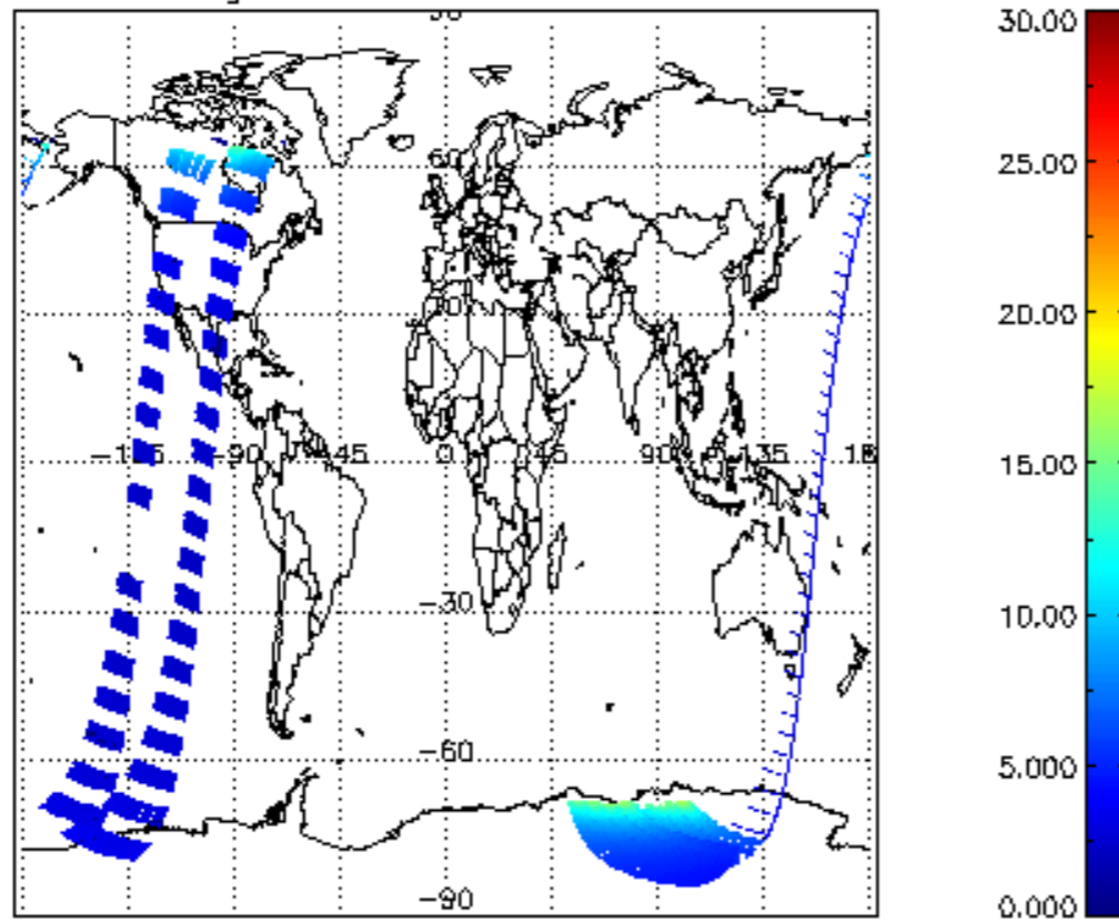
SCIOL2P_NADUV1NO2_amf_gr for 06JAN2004 00:00:00 to 07JAN2004 00:00:00
