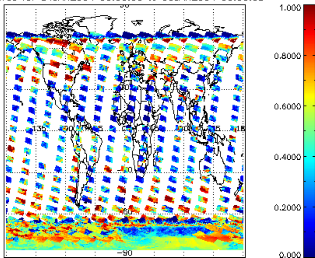
cL_frac for 04JAN2004 00:00:00 to 05JAN2004 00:00:00
