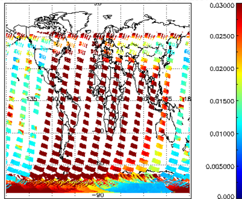
SCIOL2P_NADUV003_vcd_err for 04JAN2004 00:00:00 to 05JAN2004 00:00:00
