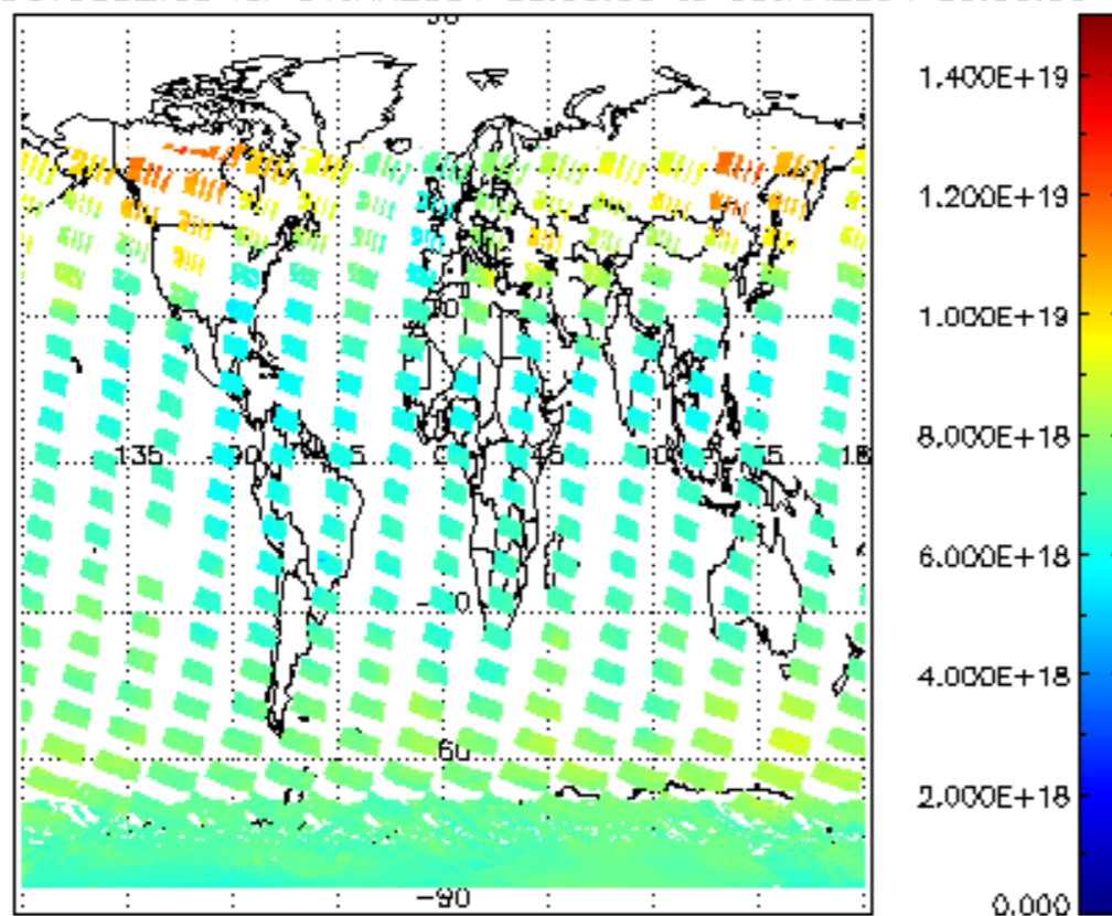
SCIOL2P_NADUV003_vcd for 04JAN2004 00:00:00 to 05JAN2004 00:00:00
