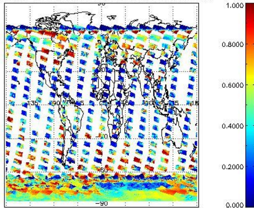
cL_frac for 04JAN2004 00:00:00 to 05JAN2004 00:00:00
