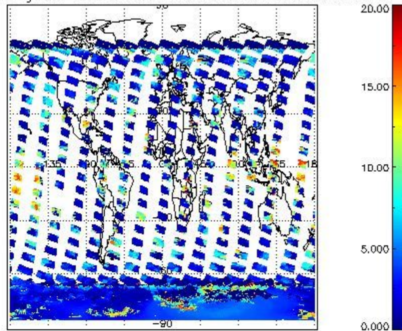
cL_top_height for 04JAN2004 00:00:00 to 05JAN2004 00:00:00
