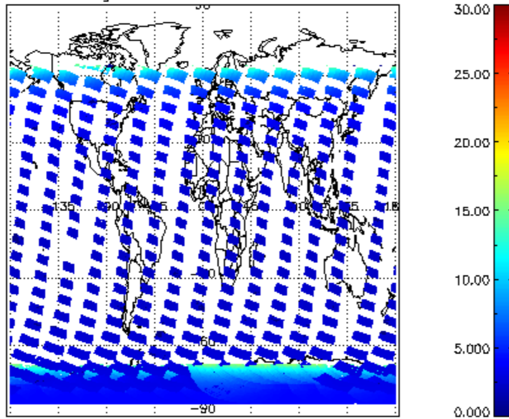
SCIOL2P_NADUV1NO2_amf_gr for 04JAN2004 00:00:00 to 05JAN2004 00:00:00
