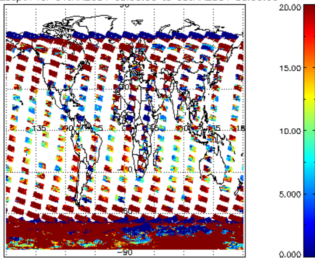
cLopt_depth for 04JAN2004 00:00:00 to 05JAN2004 00:00:00
