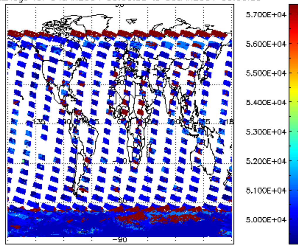
cloud_flags for 04JAN2004 00:00:00 to 05JAN2004 00:00:00
