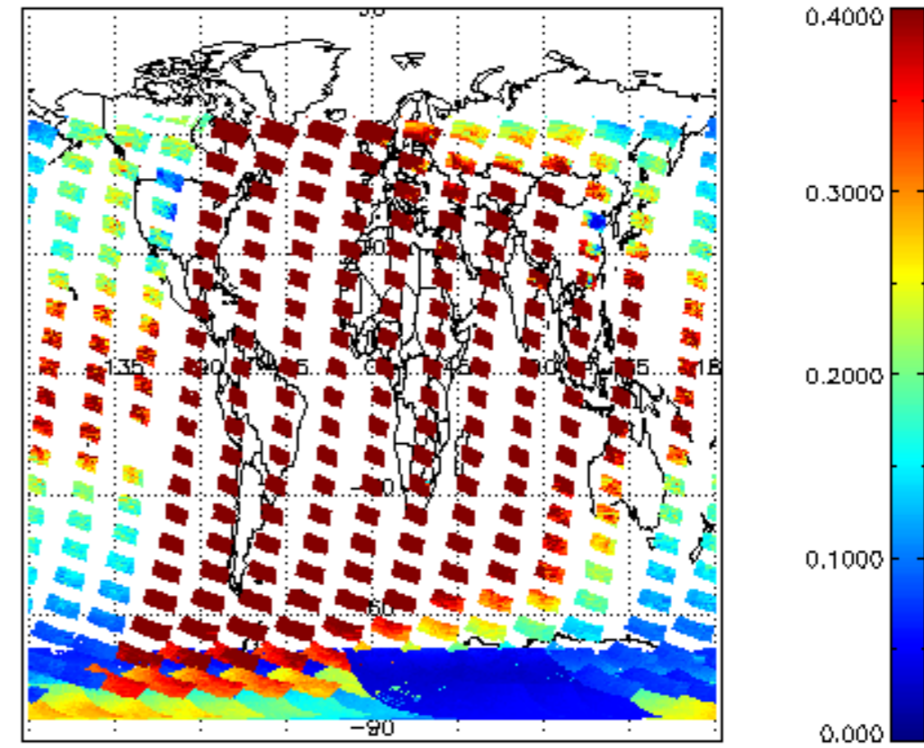
SCIOL2P_NADUV1NO2_vcd_err for 04JAN2004 00:00:00 to 05JAN2004 00:00:00
