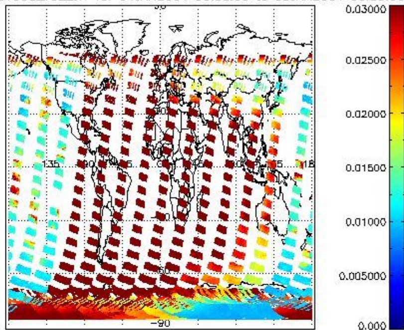
SCIOL2P_NADUV003_vcd_err for 04JAN2004 00:00:00 to 05JAN2004 00:00:00
