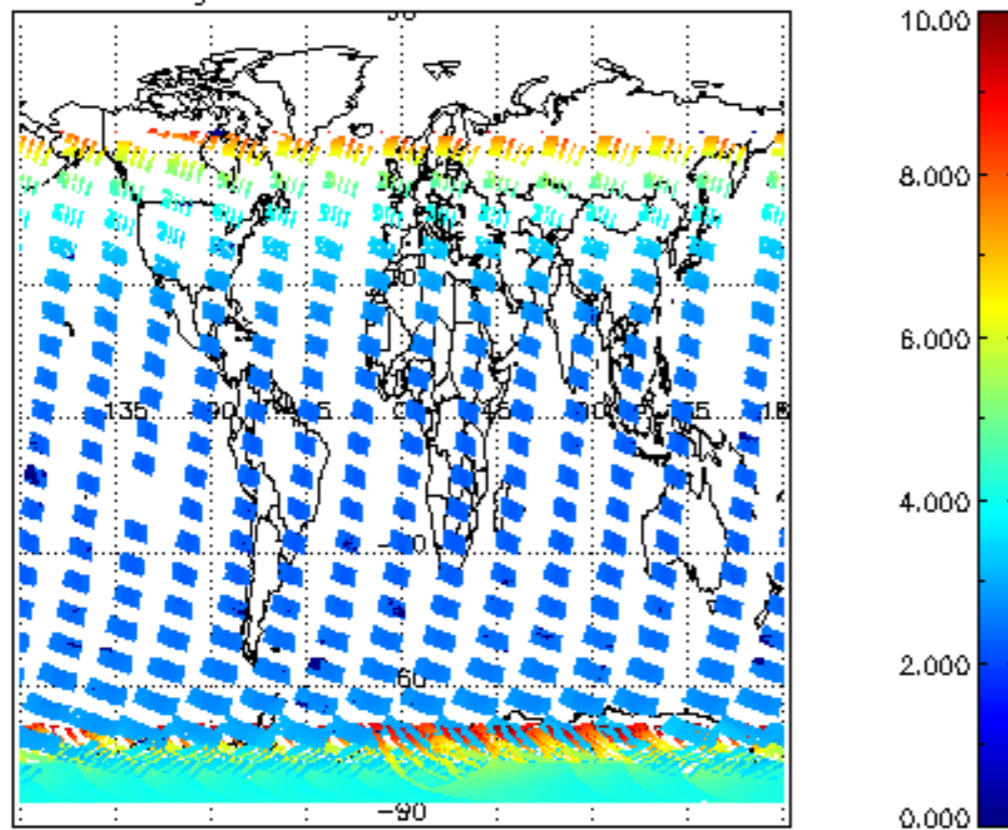
SCIOL2P_NADUV003_amf_gr for 04JAN2004 00:00:00 to 05JAN2004 00:00:00
