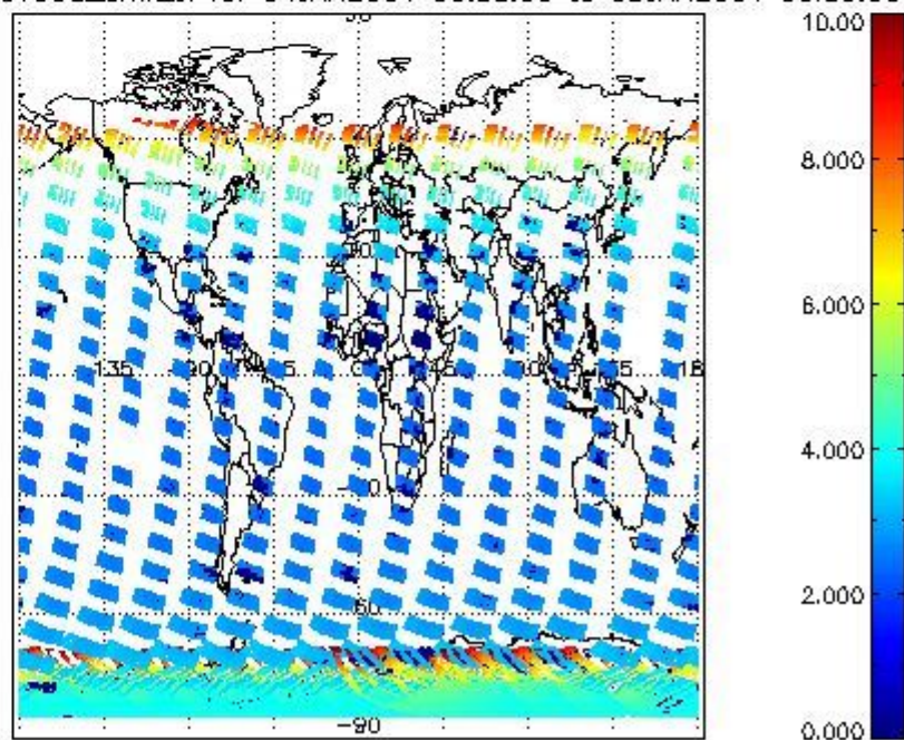
SCIOL2P_NADUV003_amf_cl for 04JAN2004 00:00:00 to 05JAN2004 00:00:00
