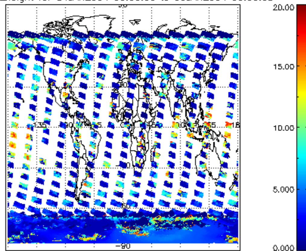
cL_top_height for 04JAN2004 00:00:00 to 05JAN2004 00:00:00
