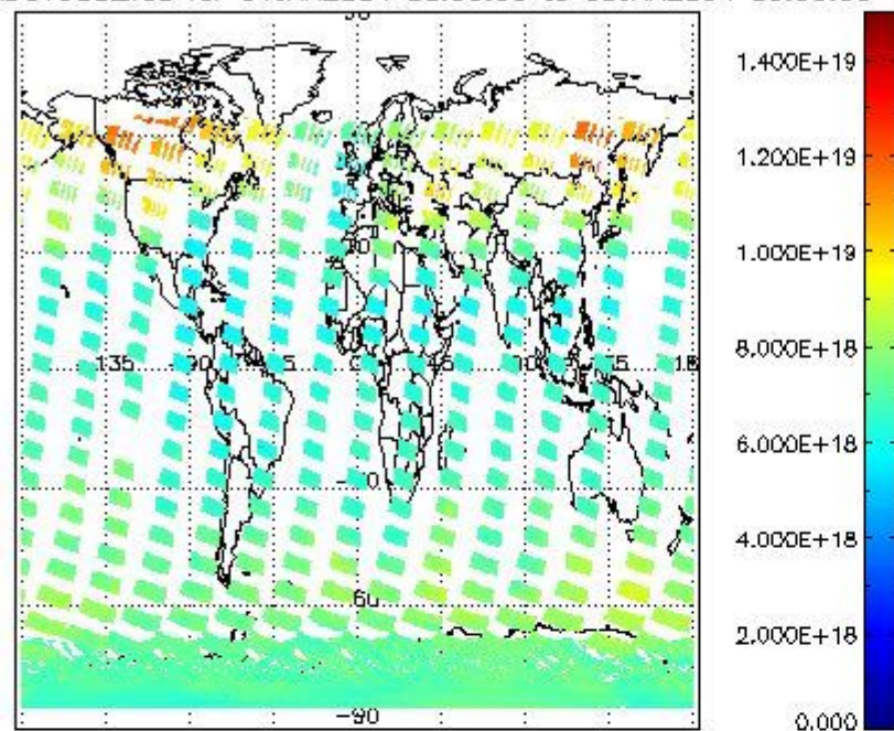
SCIOL2P_NADUV003_vcd for 04JAN2004 00:00:00 to 05JAN2004 00:00:00
