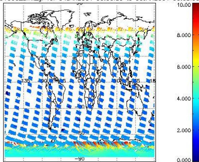
SCIOL2P_NADUV003_amf_gr for 04JAN2004 00:00:00 to 05JAN2004 00:00:00
