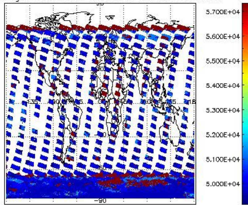
cloud_flags for 04JAN2004 00:00:00 to 05JAN2004 00:00:00
