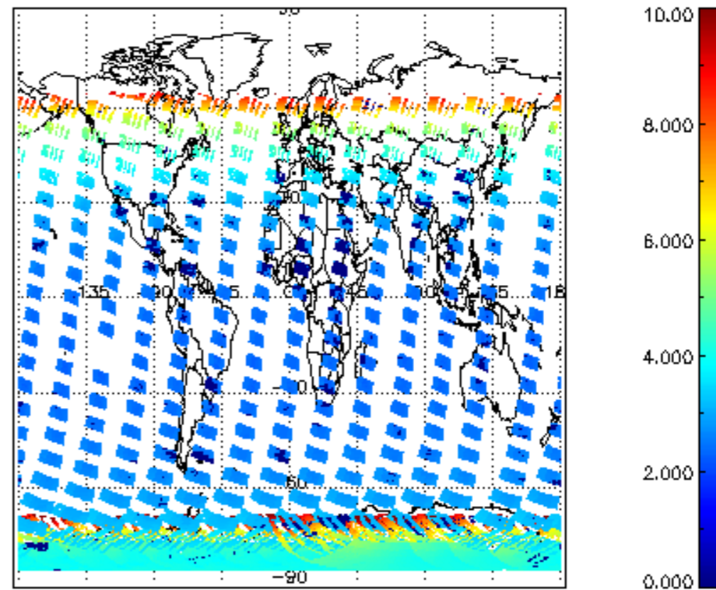
SCIOL2P_NADUV003_amf_cl for 04JAN2004 00:00:00 to 05JAN2004 00:00:00
