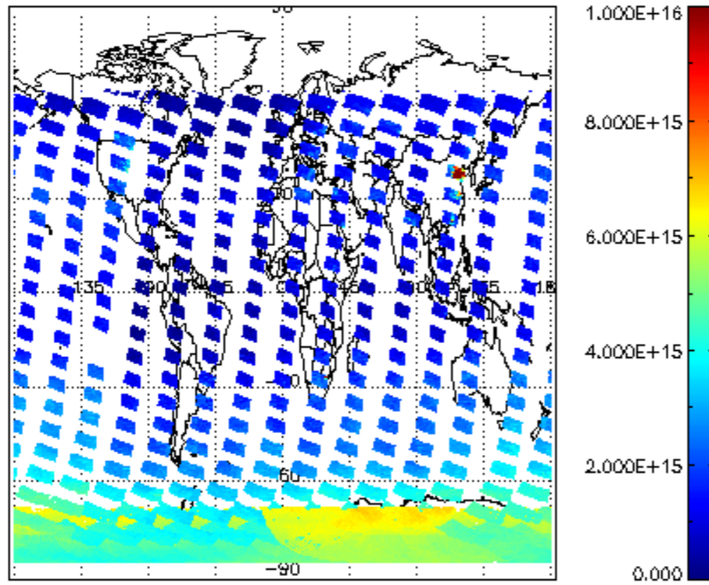
SCIOL2P_NADUV1NO2_vcd for 04JAN2004 00:00:00 to 05JAN2004 00:00:00
