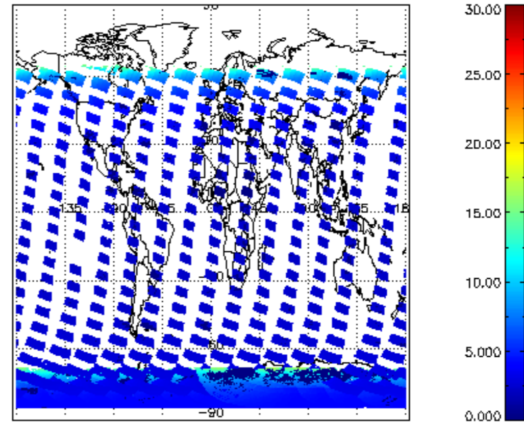
SCIOL2P_NADUV1NO2_amf_cl for 04JAN2004 00:00:00 to 05JAN2004 00:00:00
