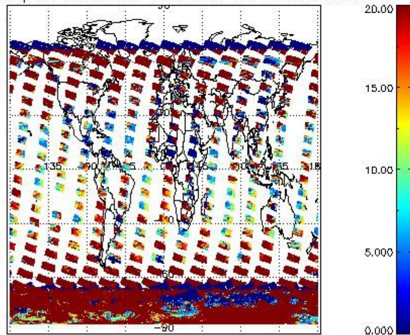
cLopt_depth for 04JAN2004 00:00:00 to 05JAN2004 00:00:00
