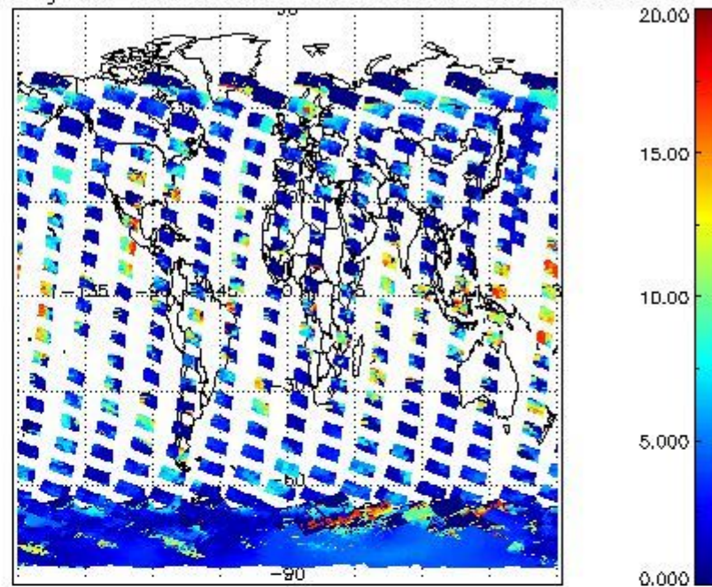
cL_top_height for 02JAN2004 00:00:00 to 03JAN2004 00:00:00
