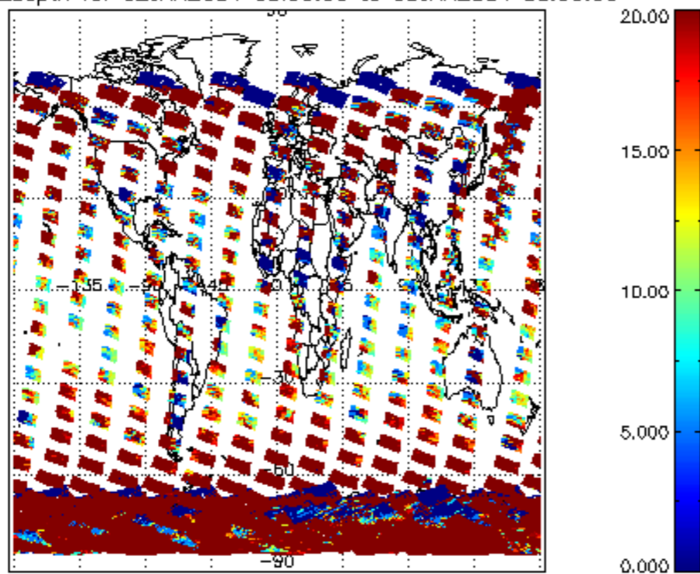
cLopt_depth for 02JAN2004 00:00:00 to 03JAN2004 00:00:00
