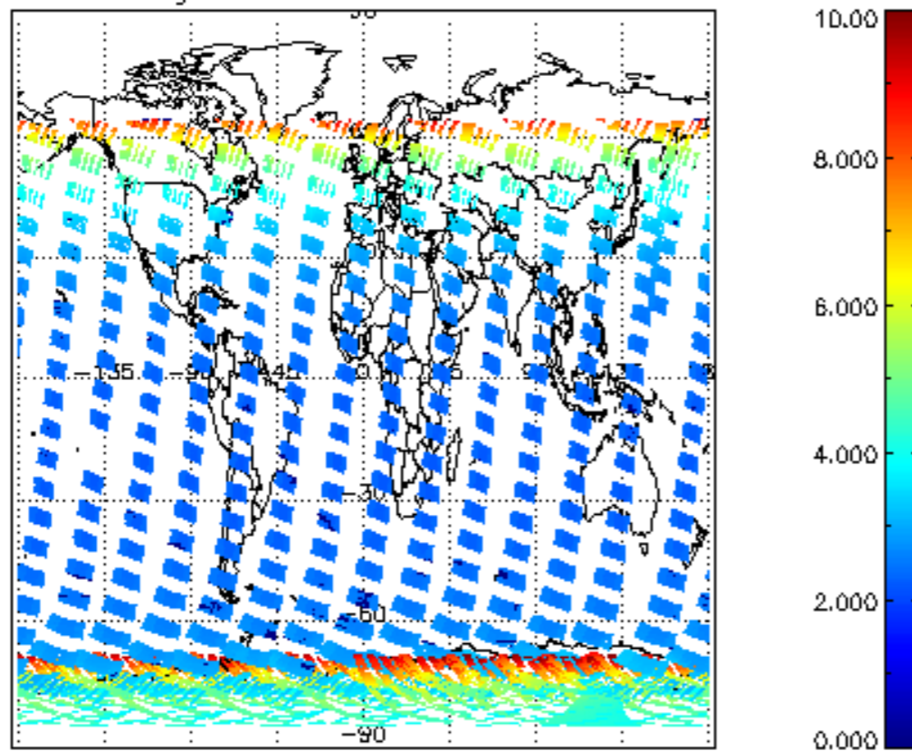
SCIOL2P_NADUV003_amf_gr for 02JAN2004 00:00:00 to 03JAN2004 00:00:00
