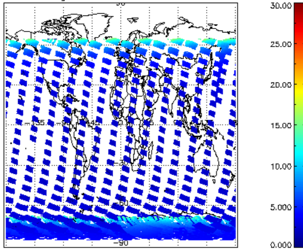
SCIOL2P_NADUV1NO2_amf_gr for 02JAN2004 00:00:00 to 03JAN2004 00:00:00
