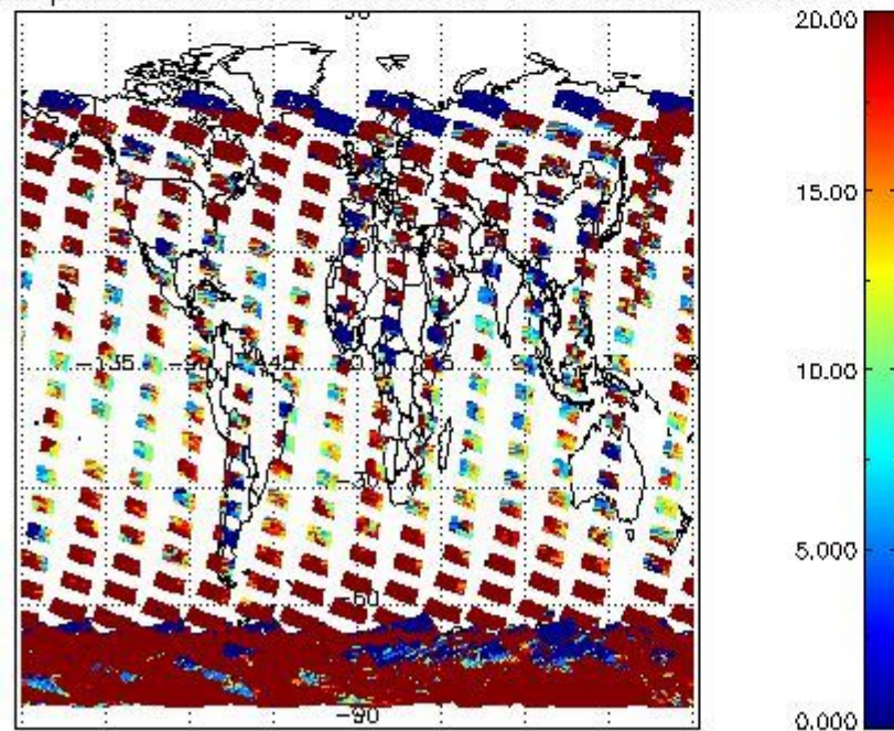
cLopt_depth for 02JAN2004 00:00:00 to 03JAN2004 00:00:00
