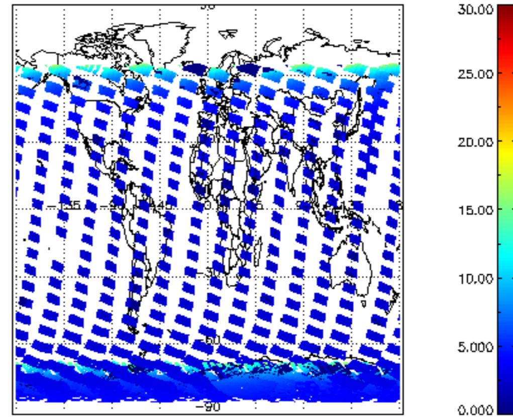
SCIOL2P_NADUV1NO2_amf_cl for 02JAN2004 00:00:00 to 03JAN2004 00:00:00
