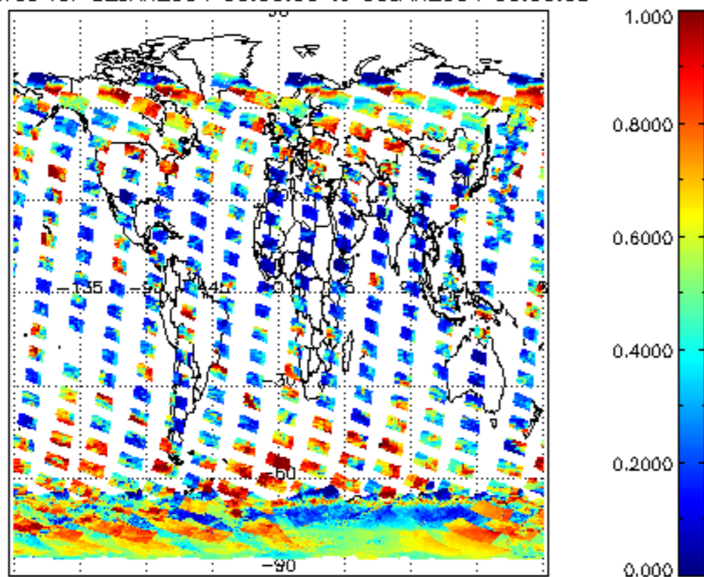
cL_frac for 02JAN2004 00:00:00 to 03JAN2004 00:00:00
