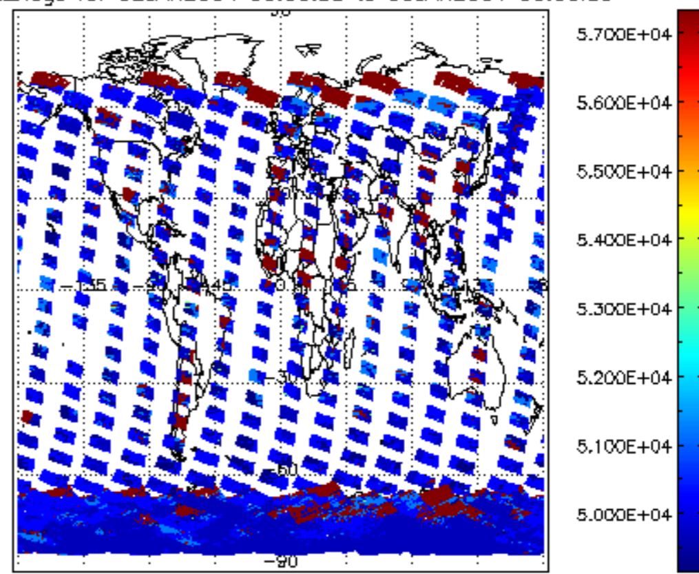
cloud_flags for 02JAN2004 00:00:00 to 03JAN2004 00:00:00
