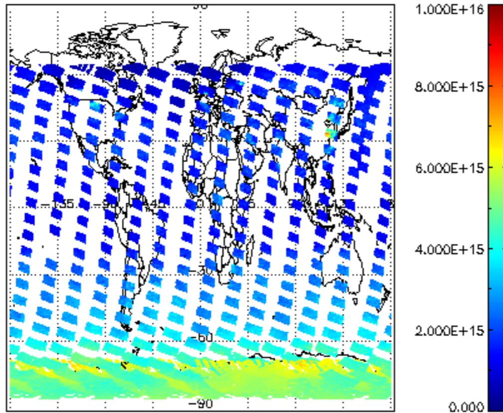
SCIOL2P_NADUV1NO2_vcd for 02JAN2004 00:00:00 to 03JAN2004 00:00:00
