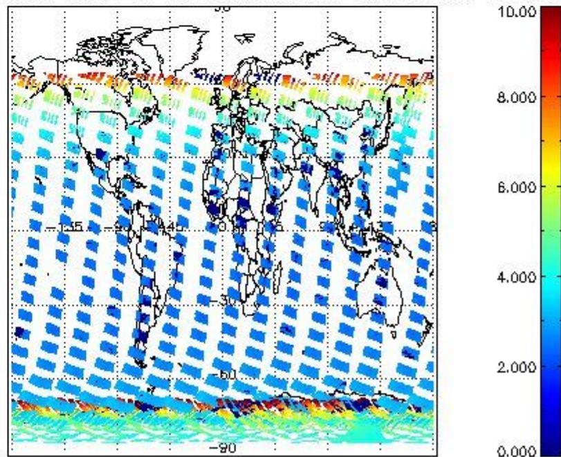
SCIOL2P_NADUV003_amf_cl for 02JAN2004 00:00:00 to 03JAN2004 00:00:00
