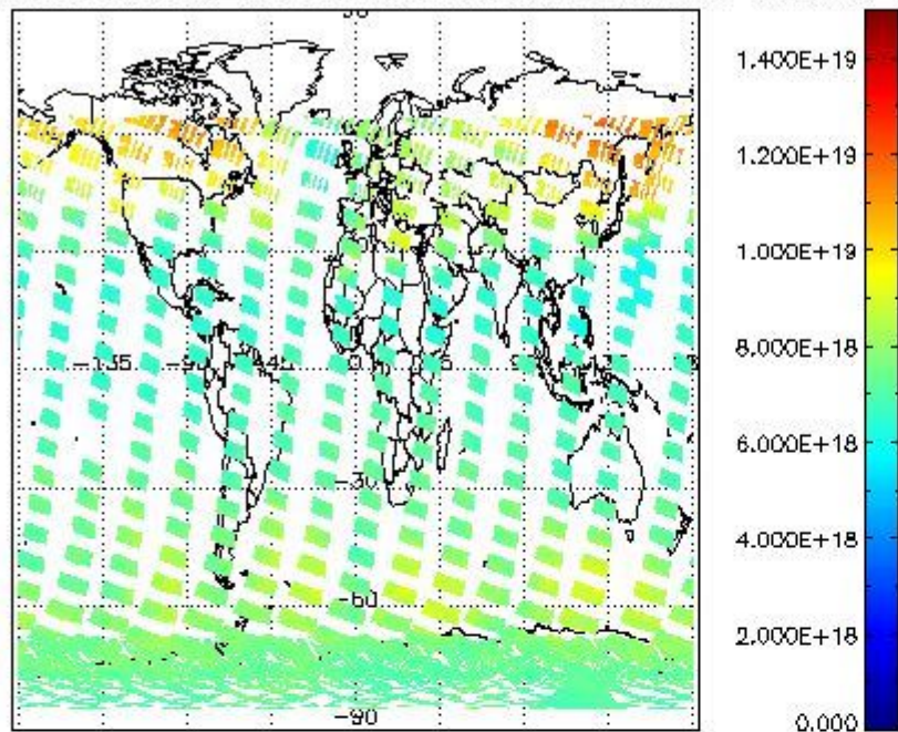
SCIOL2P_NADUV003_vcd for 02JAN2004 00:00:00 to 03JAN2004 00:00:00
