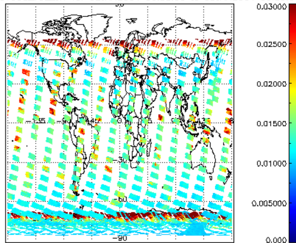
SCIOL2P_NADUV003_vcd_err for 02JAN2004 00:00:00 to 03JAN2004 00:00:00
