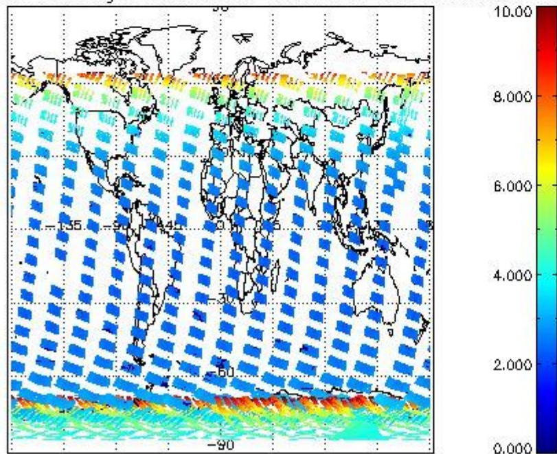
SCIOL2P_NADUV003_amf_gr for 02JAN2004 00:00:00 to 03JAN2004 00:00:00
