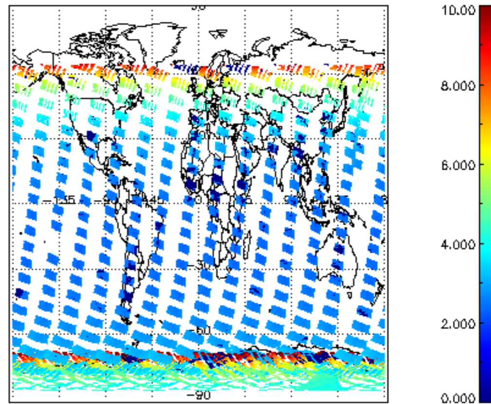
SCIOL2P_NADUV003_amf_cl for 02JAN2004 00:00:00 to 03JAN2004 00:00:00
