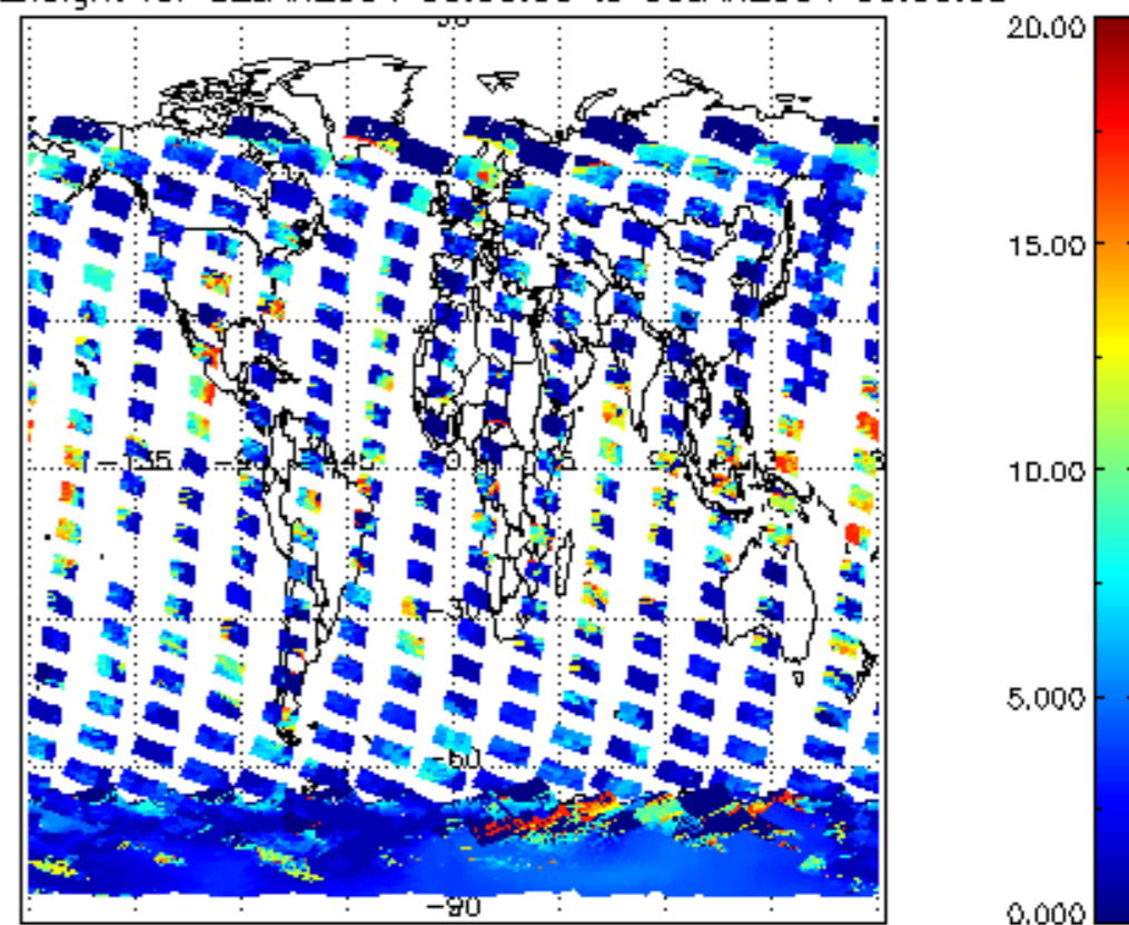
cL_top_height for 02JAN2004 00:00:00 to 03JAN2004 00:00:00
