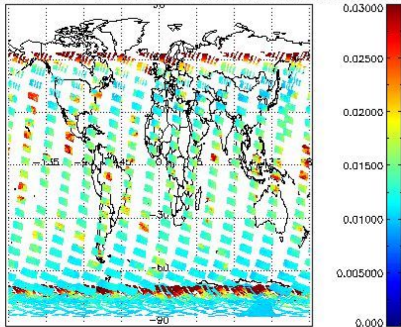
SCIOL2P_NADUV003_vcd_err for 02JAN2004 00:00:00 to 03JAN2004 00:00:00
