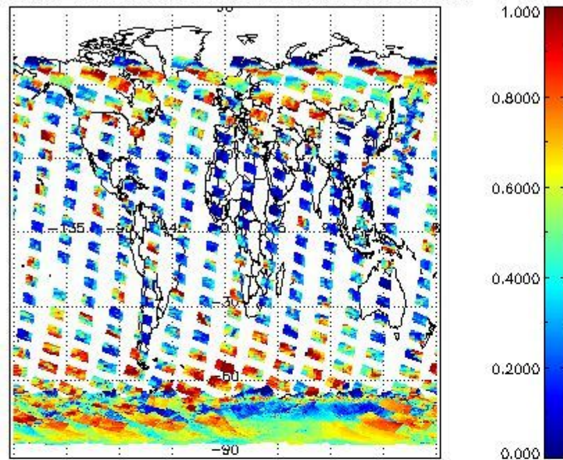
cL_frac for 02JAN2004 00:00:00 to 03JAN2004 00:00:00
