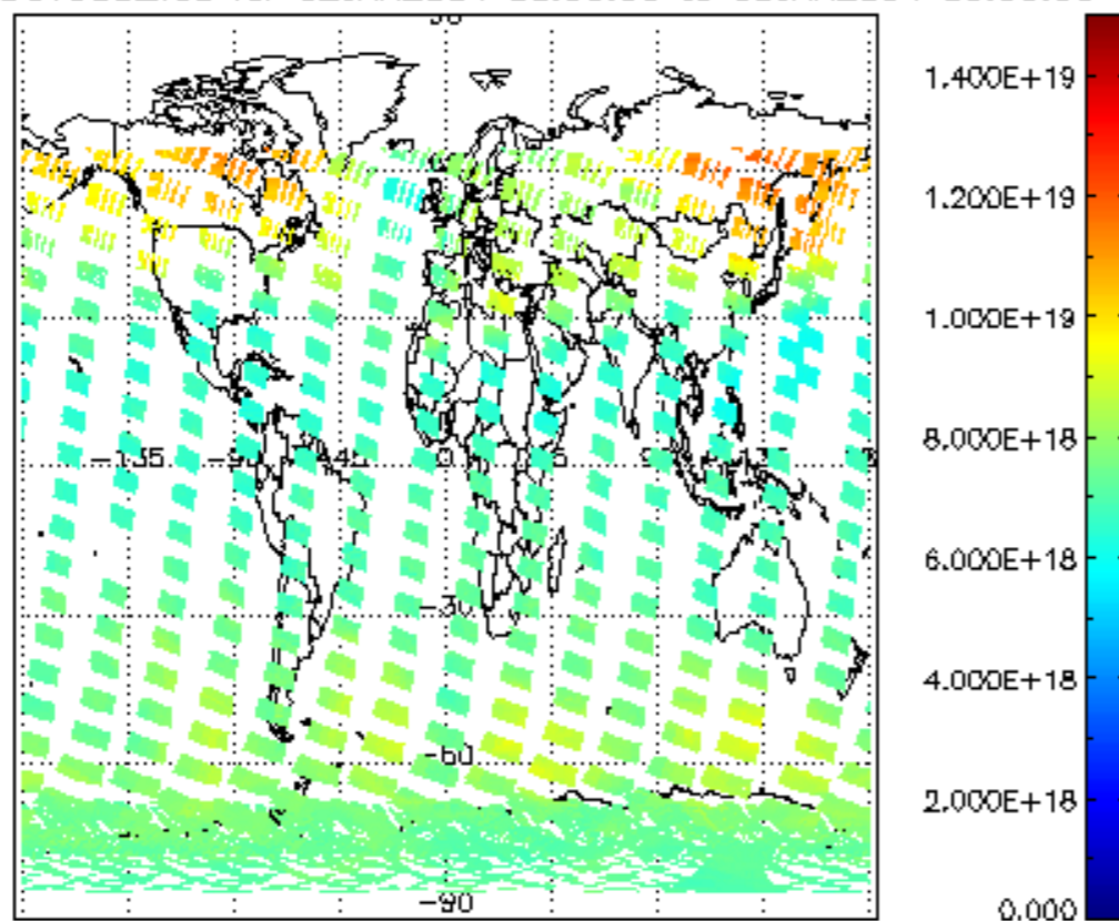
SCIOL2P_NADUV003_vcd for 02JAN2004 00:00:00 to 03JAN2004 00:00:00
