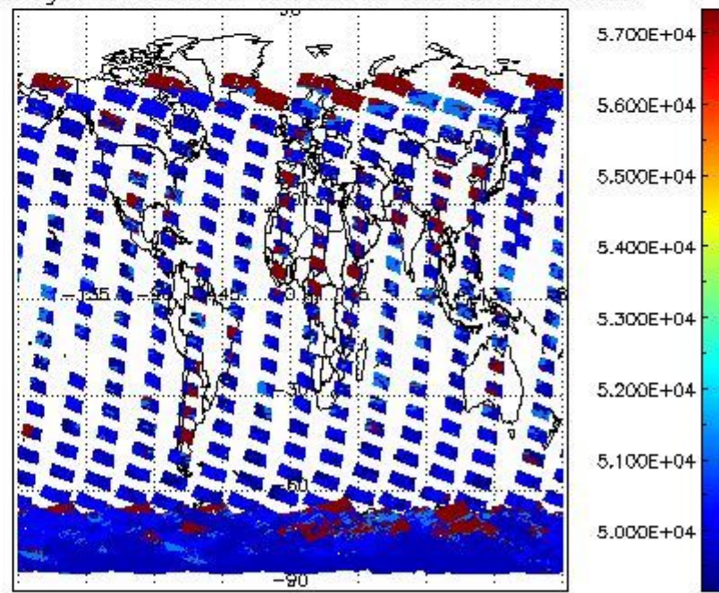
cloud_flags for 02JAN2004 00:00:00 to 03JAN2004 00:00:00
