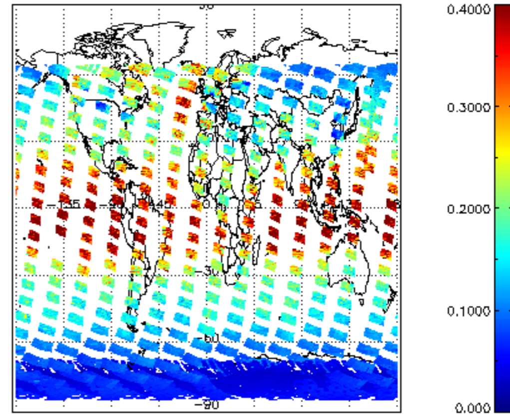
SCIOL2P_NADUV1NO2_vcd_err for 02JAN2004 00:00:00 to 03JAN2004 00:00:00
