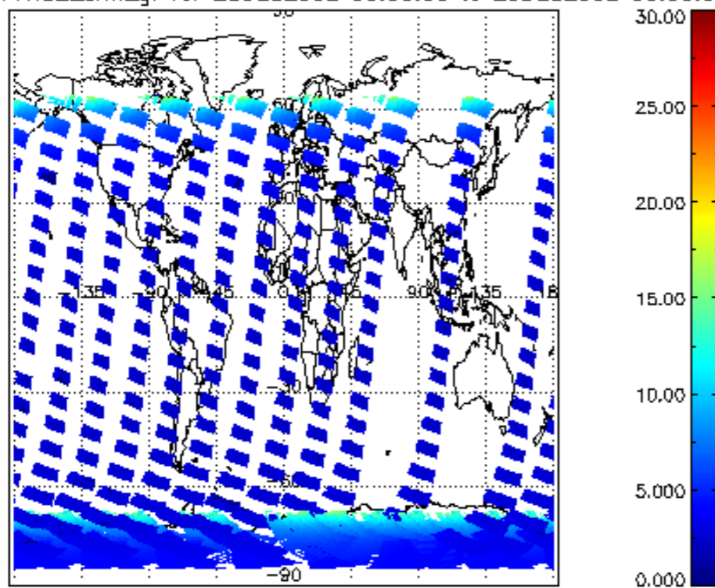
SCIOL2P_NADUV1NO2_amf_gr for 28DEC2002 00:00:00 to 29DEC2002 00:00:00
