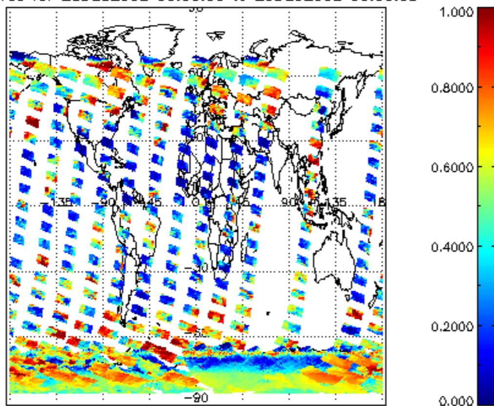
cI_frac for 28DEC2002 00:00:00 to 29DEC2002 00:00:00
