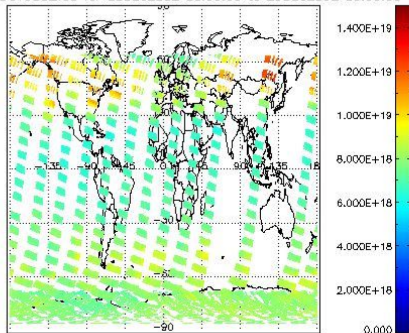
SCIOL2P_NADUV003_vcd for 28DEC2002 00:00:00 to 29DEC2002 00:00:00
