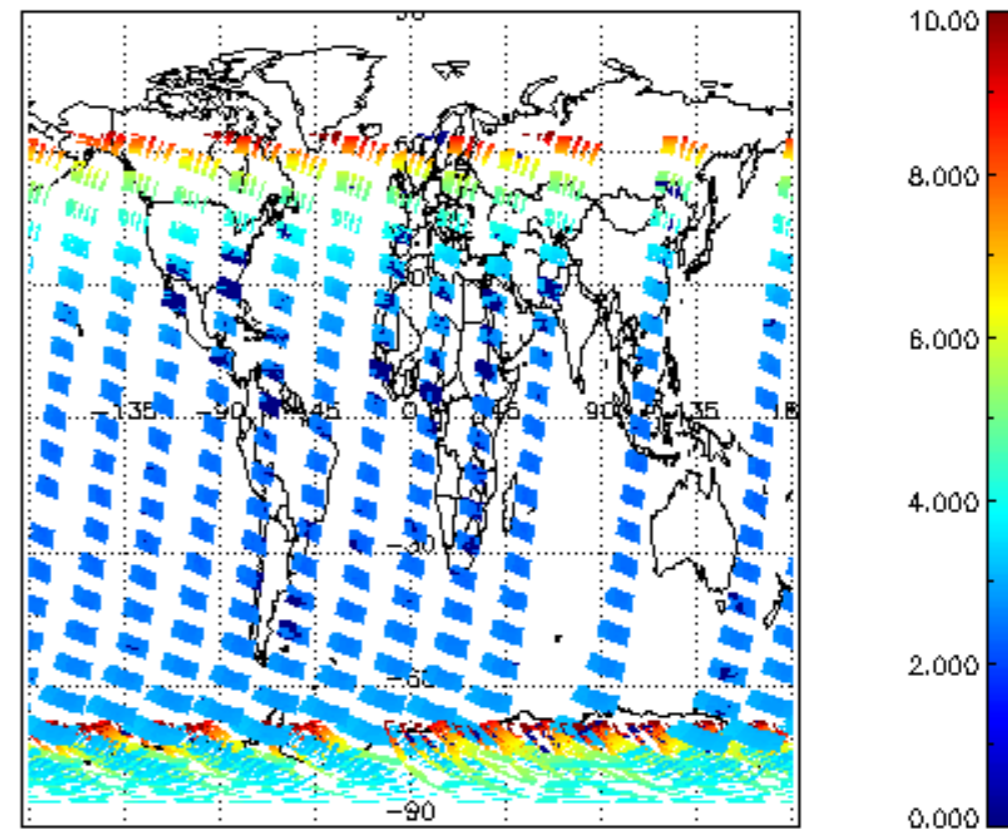
SCIOL2P_NADUV003_amf_cl for 28DEC2002 00:00:00 to 29DEC2002 00:00:00
