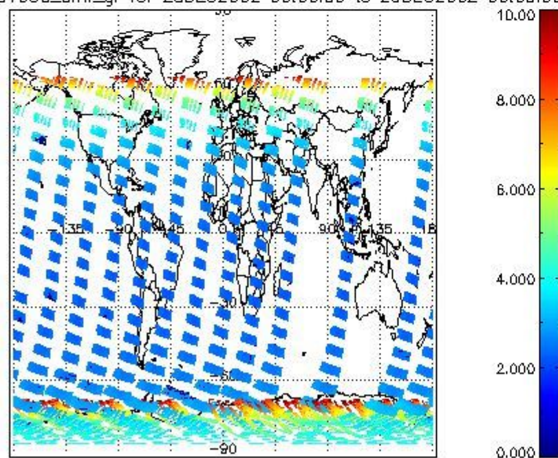
SCIOL2P_NADUV003_amf_gr for 28DEC2002 00:00:00 to 29DEC2002 00:00:00
