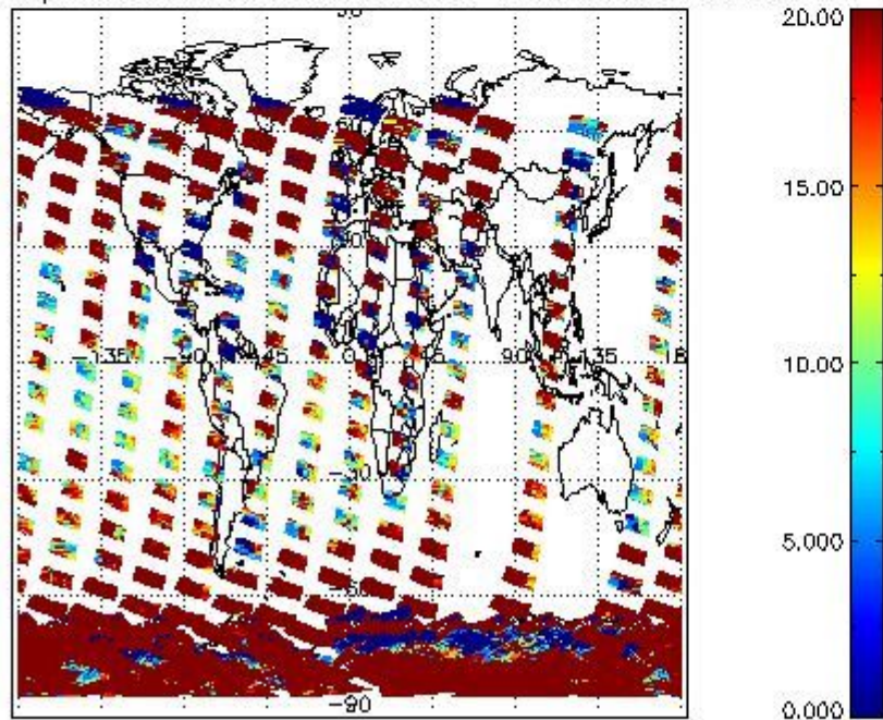
cL_opt_depth for 28DEC2002 00:00:00 to 29DEC2002 00:00:00
