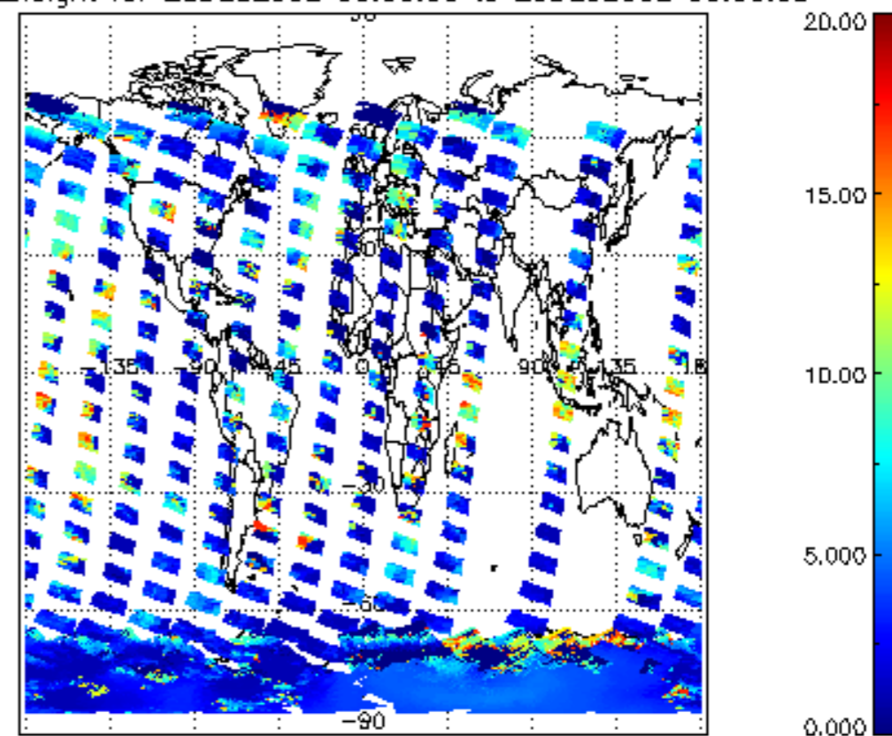
cI_top_height for 28DEC2002 00:00:00 to 29DEC2002 00:00:00
