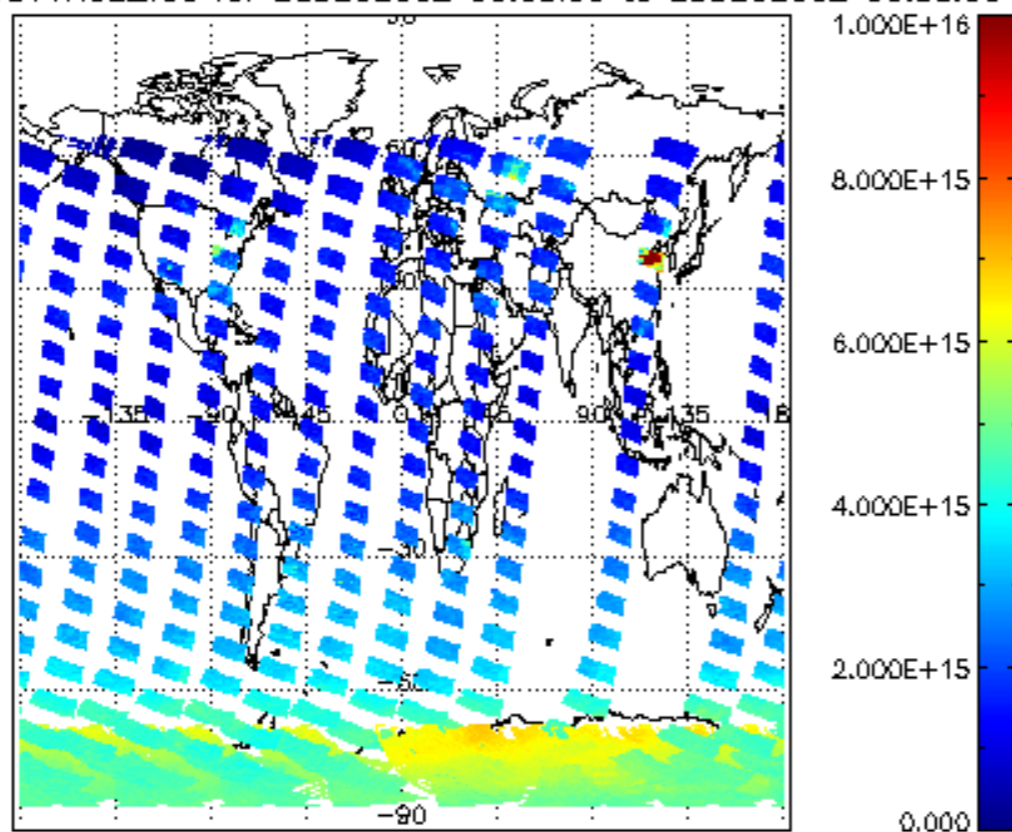
SCIOL2P_NADUV1NO2_vcd for 28DEC2002 00:00:00 to 29DEC2002 00:00:00
