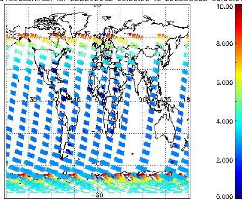
SCIOL2P_NADUV003_amf_sl for 28DEC2002 00:00:00 to 29DEC2002 00:00:00
