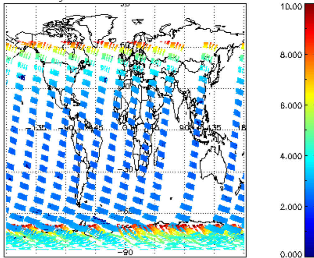
SCIOL2P_NADUV003_amf_gr for 28DEC2002 00:00:00 to 29DEC2002 00:00:00
