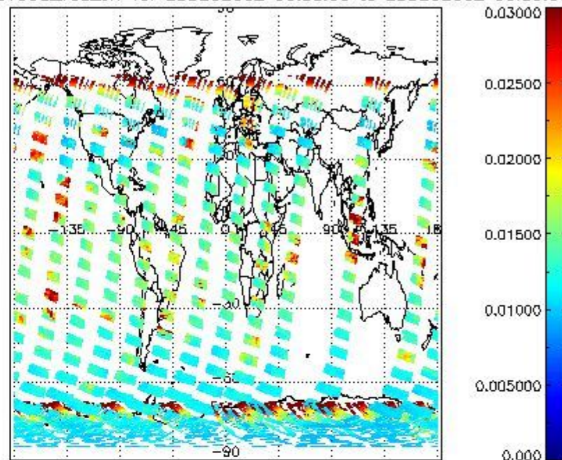
SCIOL2P_NADUV003_vcd_err for 28DEC2002 00:00:00 to 29DEC2002 00:00:00
