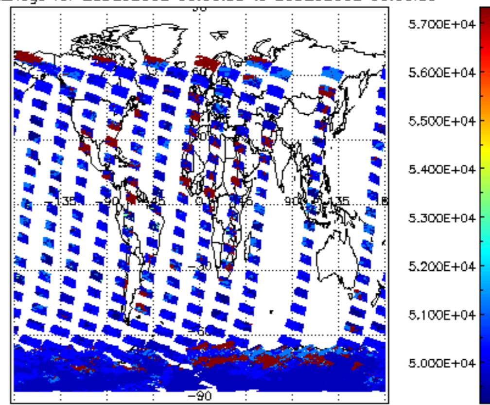
cloud_flags for 28DEC2002 00:00:00 to 29DEC2002 00:00:00
