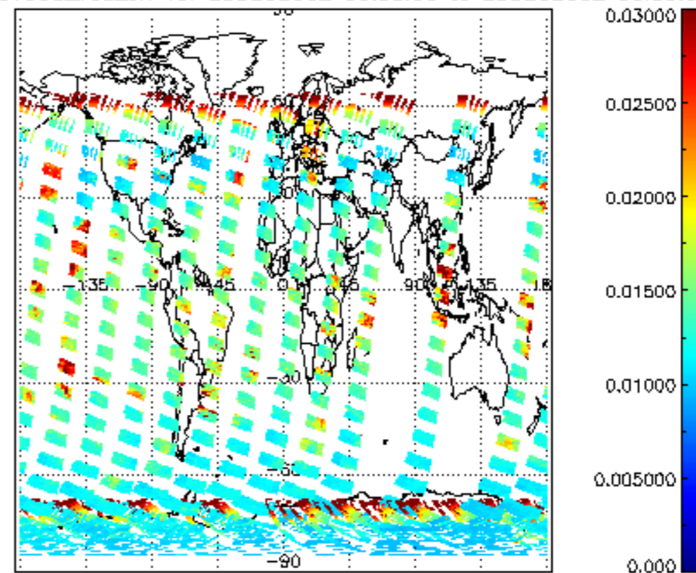
SCIOL2P_NADUV003_vcd_err for 28DEC2002 00:00:00 to 29DEC2002 00:00:00
