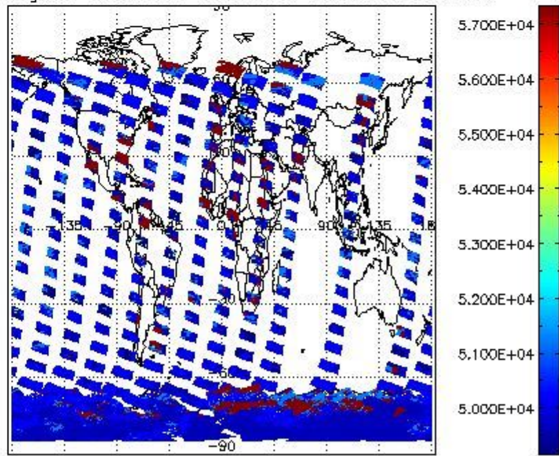
cloud_flags for 28DEC2002 00:00:00 to 29DEC2002 00:00:00
