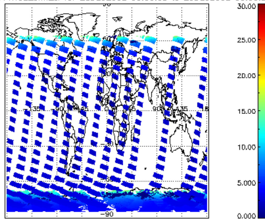
SCIOL2P_NADUV1NO2_amf_cl for 28DEC2002 00:00:00 to 29DEC2002 00:00:00
