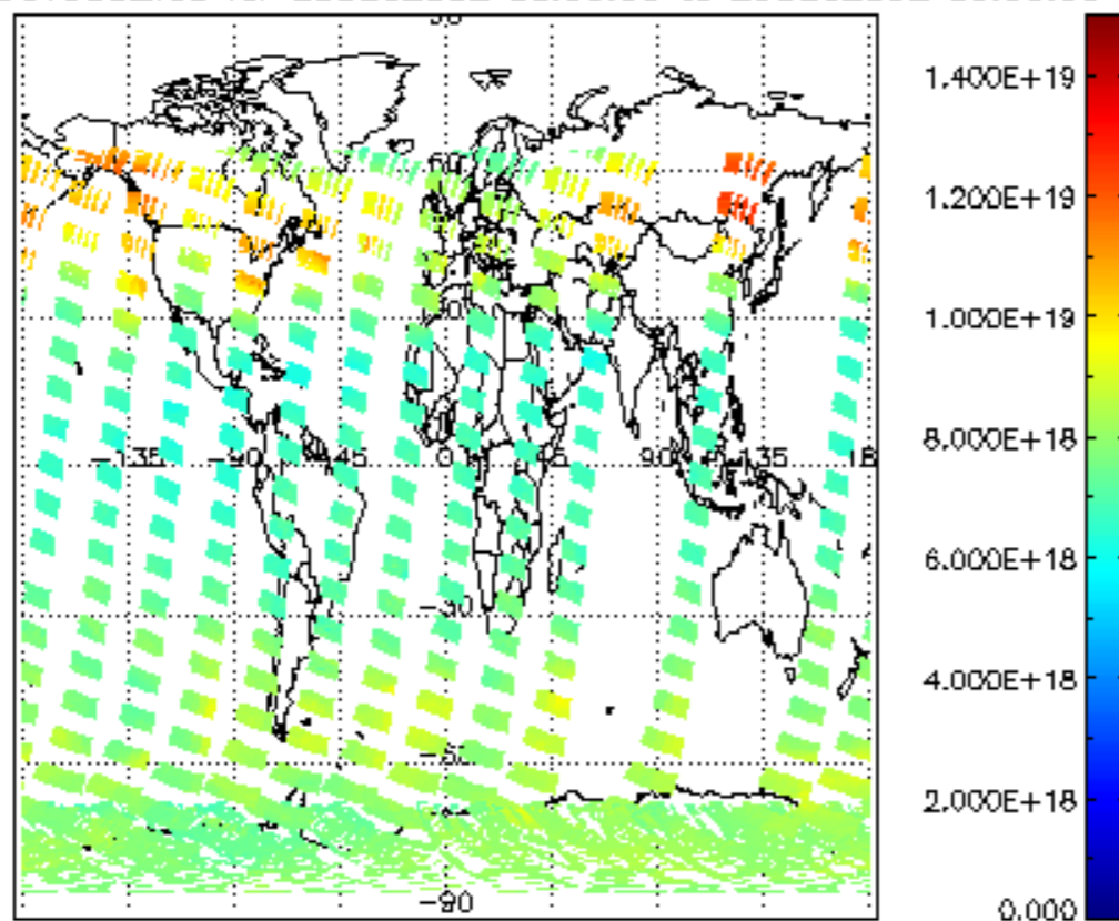
SCIOL2P_NADUV003_vcd for 28DEC2002 00:00:00 to 29DEC2002 00:00:00
