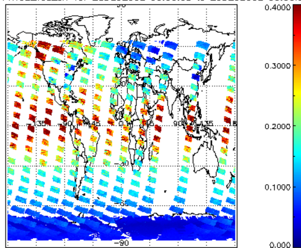
SCIOL2P_NADUV1NO2_vcd_err for 28DEC2002 00:00:00 to 29DEC2002 00:00:00
