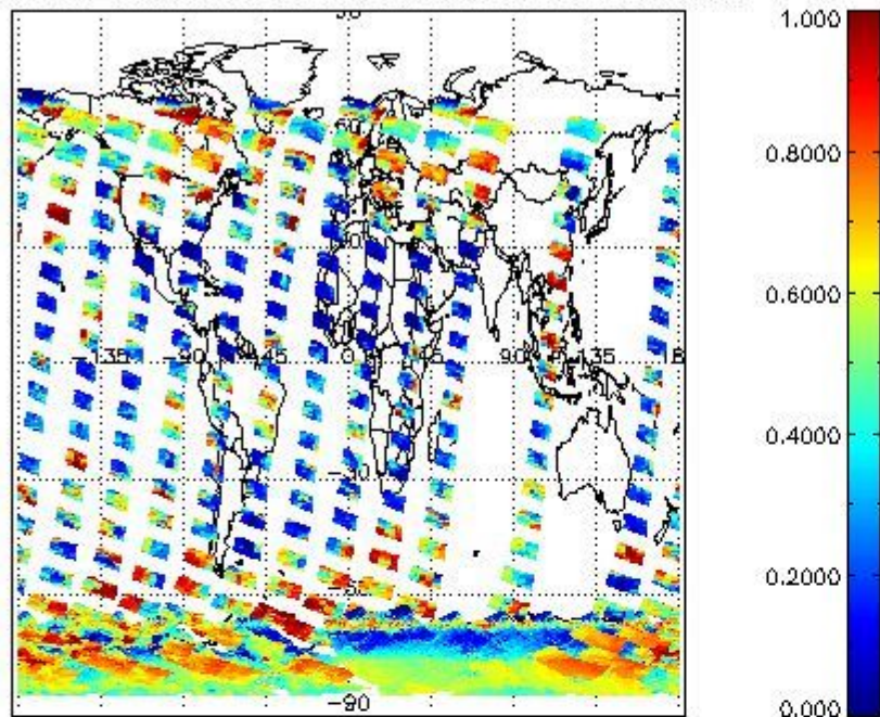
cL_frac for 28DEC2002 00:00:00 to 29DEC2002 00:00:00
