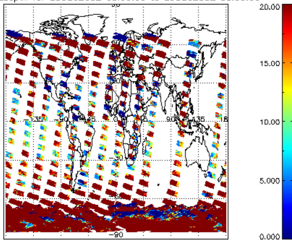
cI_opt_depth for 28DEC2002 00:00:00 to 29DEC2002 00:00:00
