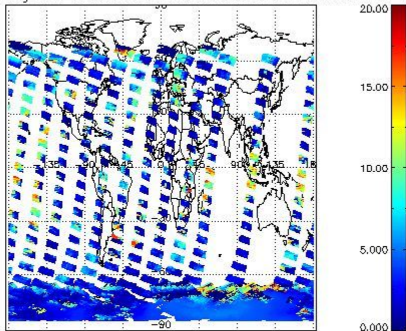
cL_top_height for 28DEC2002 00:00:00 to 29DEC2002 00:00:00
