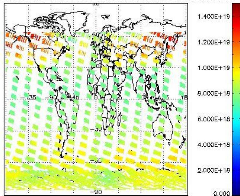
SCIOL2P_NADUV003_vcd for 22DEC2002 00:00:00 to 23DEC2002 00:00:00
