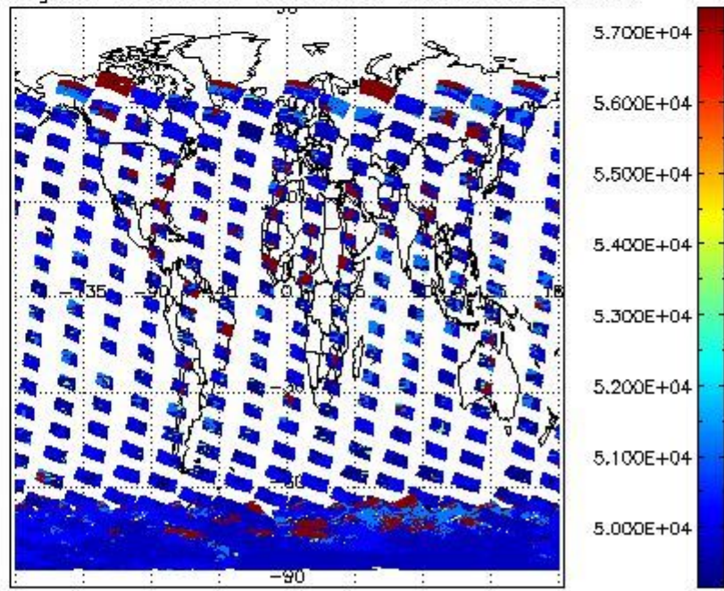
cloud_flags for 22DEC2002 00:00:00 to 23DEC2002 00:00:00
