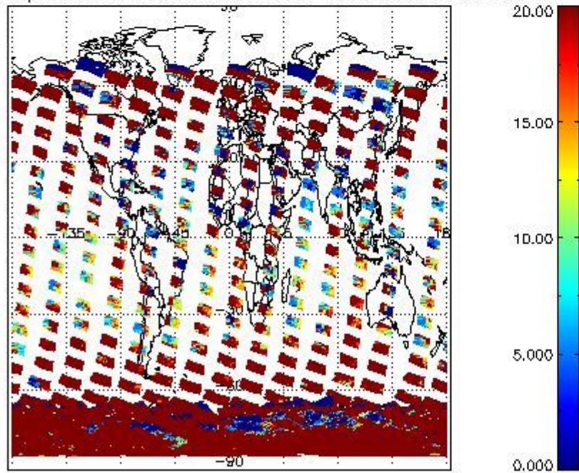
cL_opt_depth for 22DEC2002 00:00:00 to 23DEC2002 00:00:00
