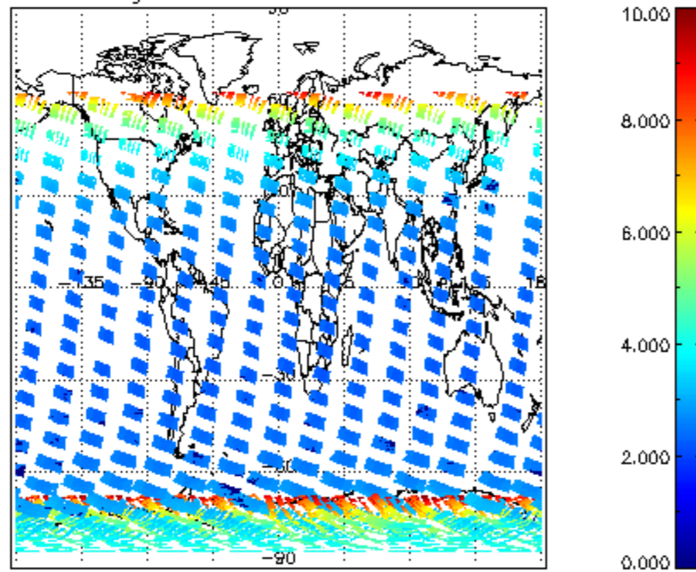
SCIOL2P_NADUV003_amf_gr for 22DEC2002 00:00:00 to 23DEC2002 00:00:00
