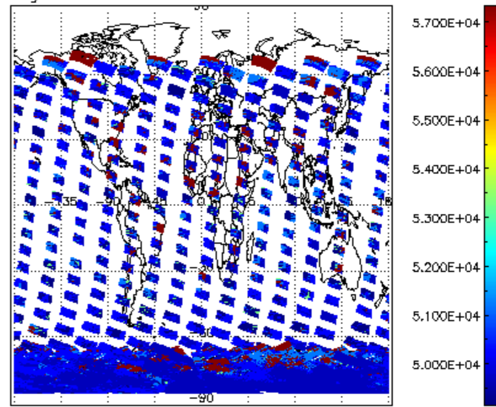
cloud_flags for 22DEC2002 00:00:00 to 23DEC2002 00:00:00
