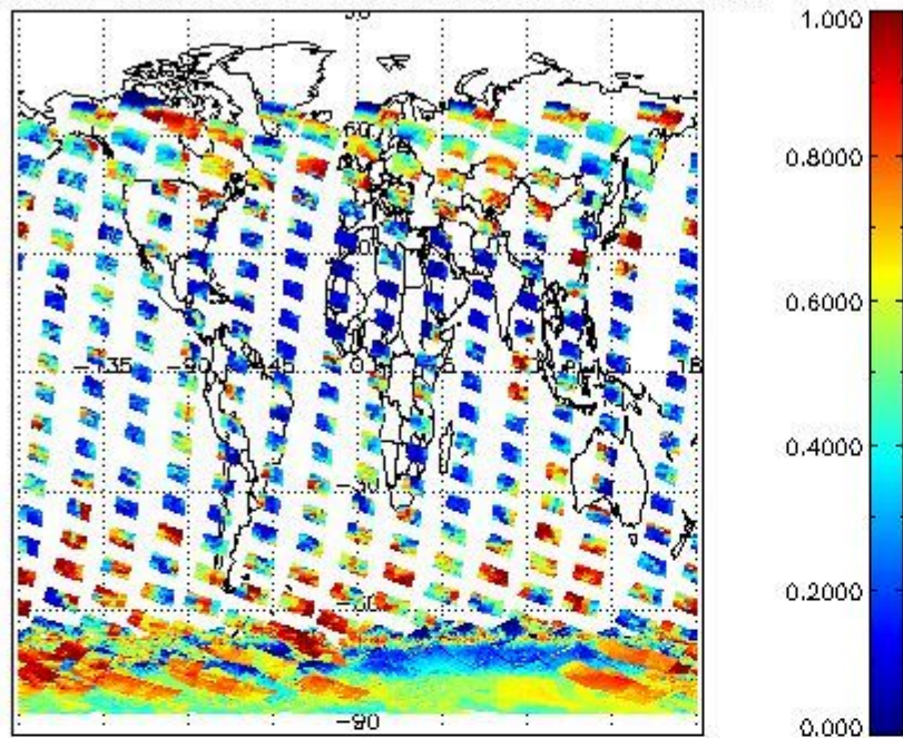
cL_frac for 22DEC2002 00:00:00 to 23DEC2002 00:00:00
