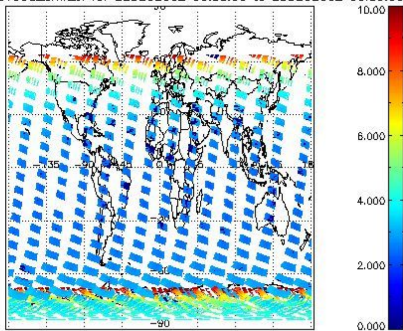
SCIOL2P_NADUV003_amf_sl for 22DEC2002 00:00:00 to 23DEC2002 00:00:00
