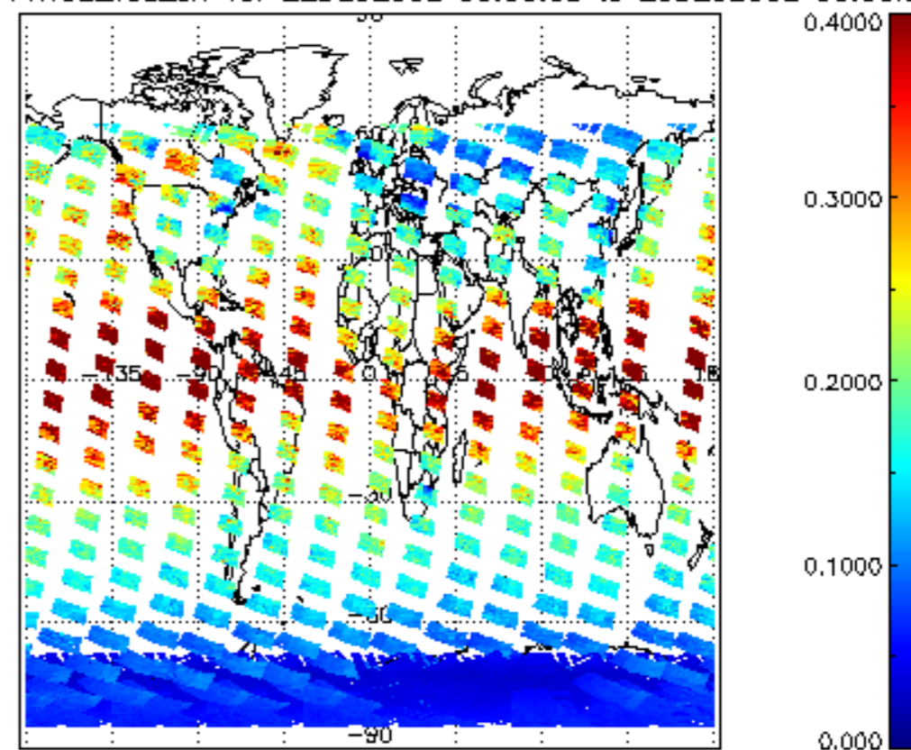
SCIOL2P_NADUV1NO2_vcd_err for 22DEC2002 00:00:00 to 23DEC2002 00:00:00
