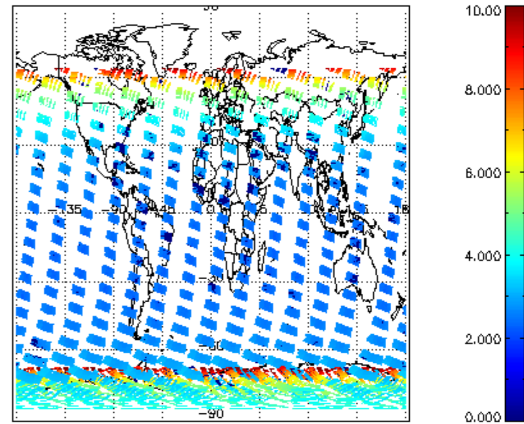
SCIOL2P_NADUV003_amf_cl for 22DEC2002 00:00:00 to 23DEC2002 00:00:00
