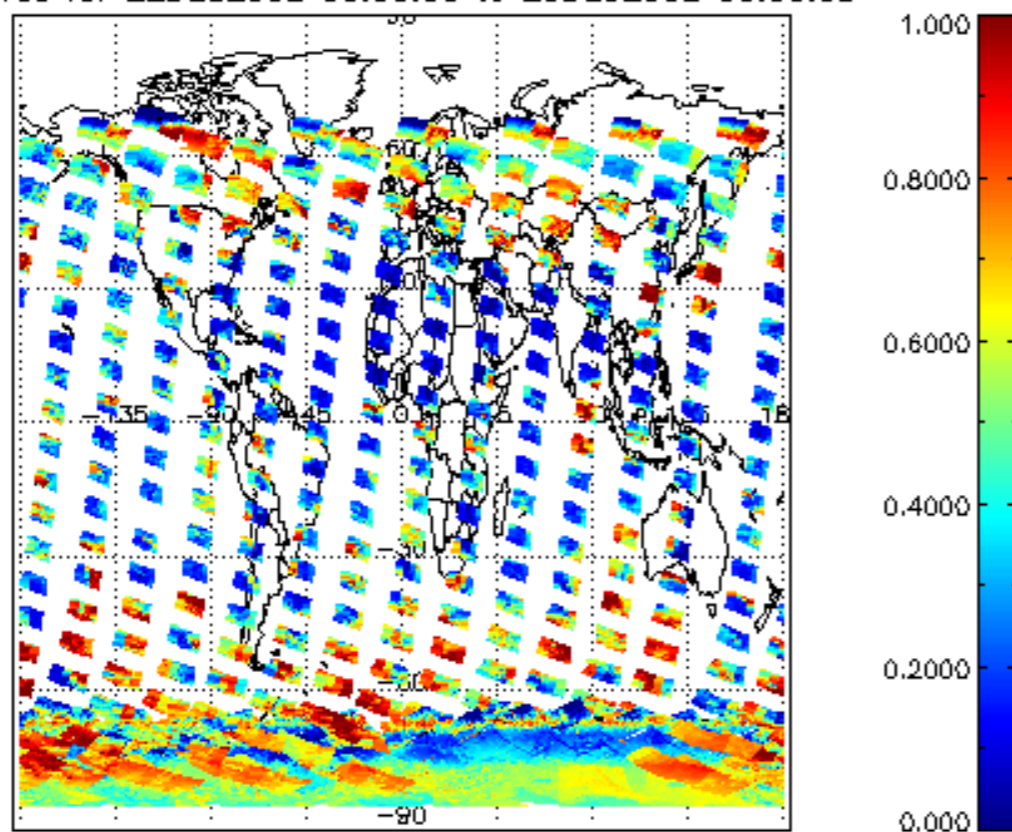
cl_frac for 22DEC2002 00:00:00 to 23DEC2002 00:00:00
