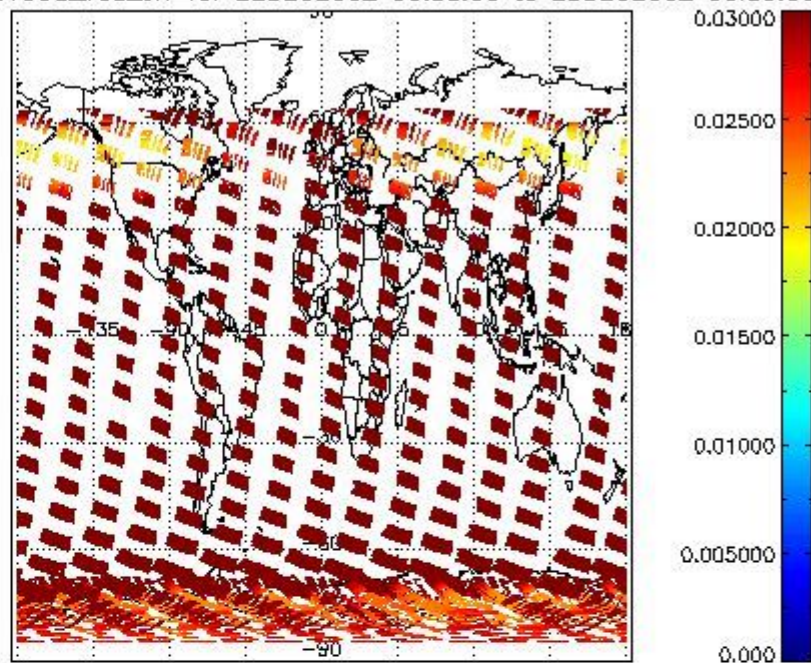
SCIOL2P_NADUV003_vcd_err for 22DEC2002 00:00:00 to 23DEC2002 00:00:00
