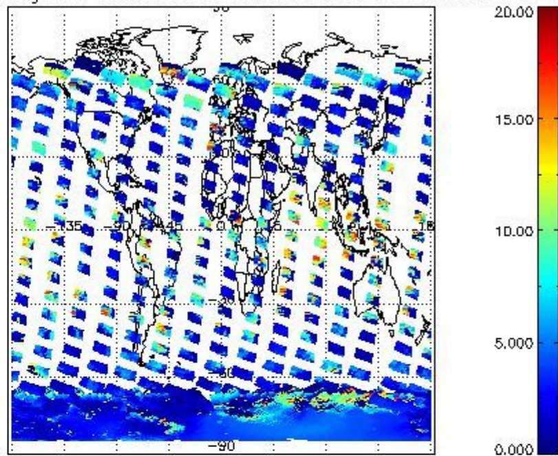
cL_top_height for 22DEC2002 00:00:00 to 23DEC2002 00:00:00
