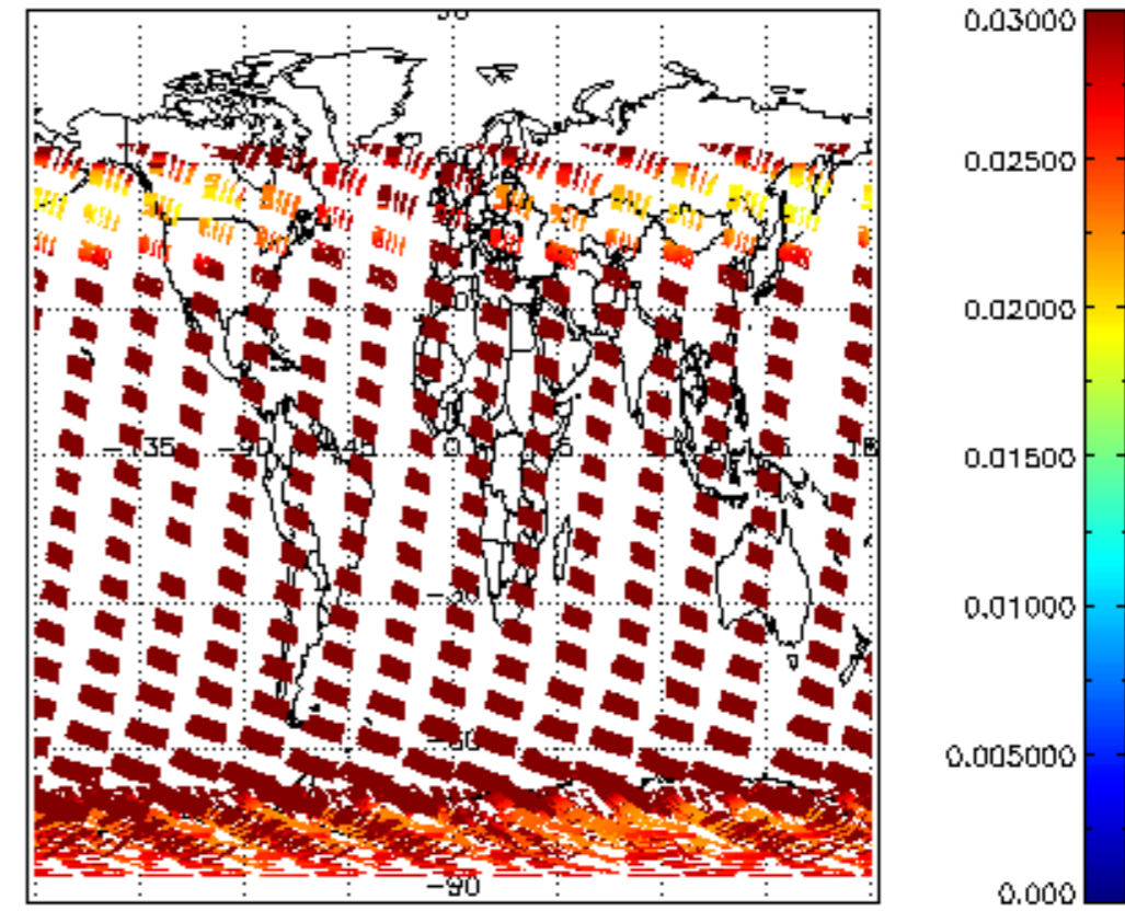
SCIOL2P_NADUV003_vcd_err for 22DEC2002 00:00:00 to 23DEC2002 00:00:00
