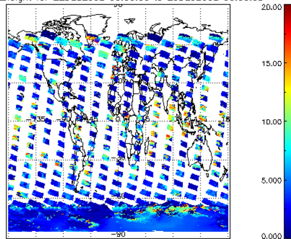
cl_top_height for 22DEC2002 00:00:00 to 23DEC2002 00:00:00
