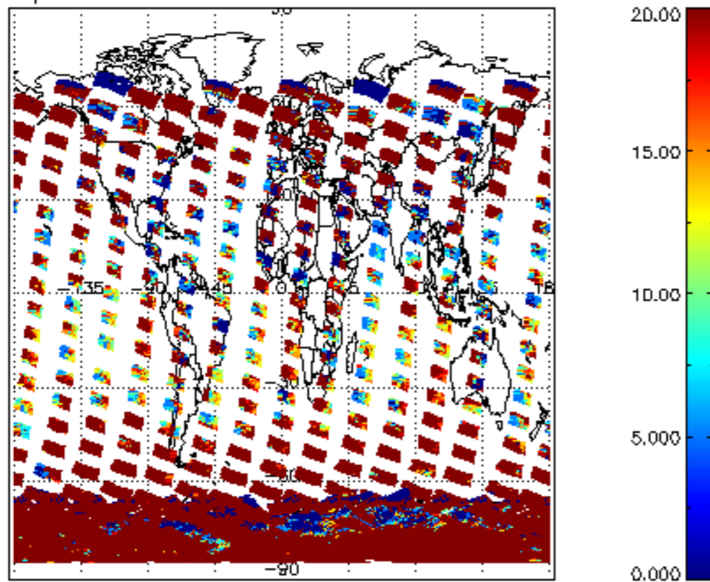
cl_opt_depth for 22DEC2002 00:00:00 to 23DEC2002 00:00:00
