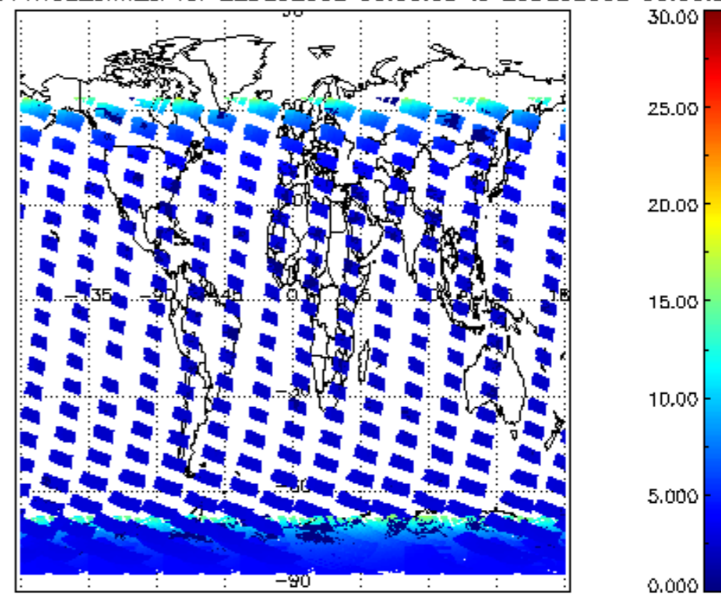
SCIOL2P_NADUV1NO2_amf_cl for 22DEC2002 00:00:00 to 23DEC2002 00:00:00
