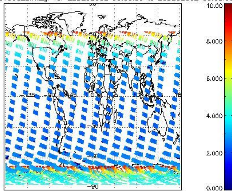
SCIOL2P_NADUV003_amf_gr for 22DEC2002 00:00:00 to 23DEC2002 00:00:00
