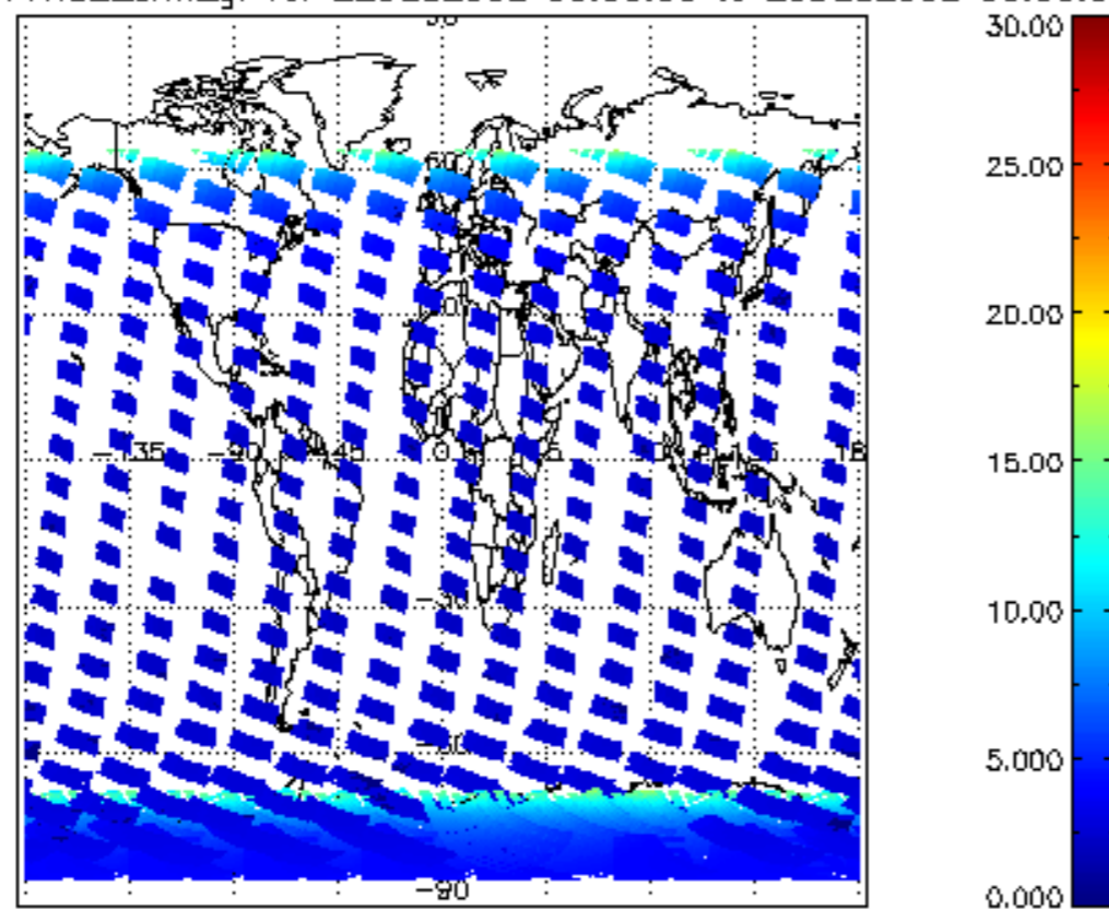
SCIOL2P_NADUV1NO2_amf_gr for 22DEC2002 00:00:00 to 23DEC2002 00:00:00
