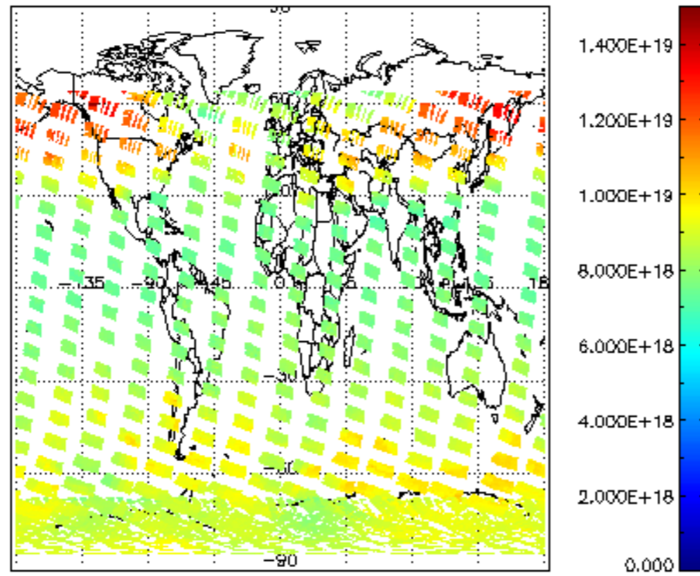
SCIOL2P_NADUV003_vcd for 22DEC2002 00:00:00 to 23DEC2002 00:00:00
