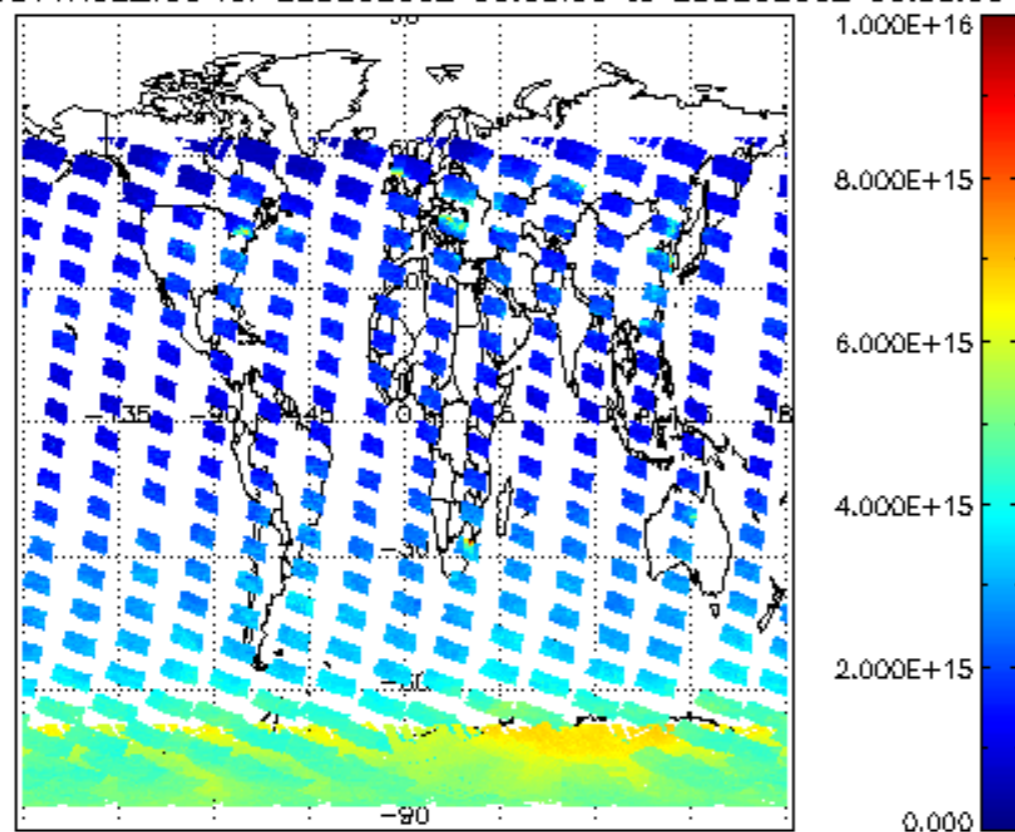
SCIOL2P_NADUV1NO2_vcd for 22DEC2002 00:00:00 to 23DEC2002 00:00:00
