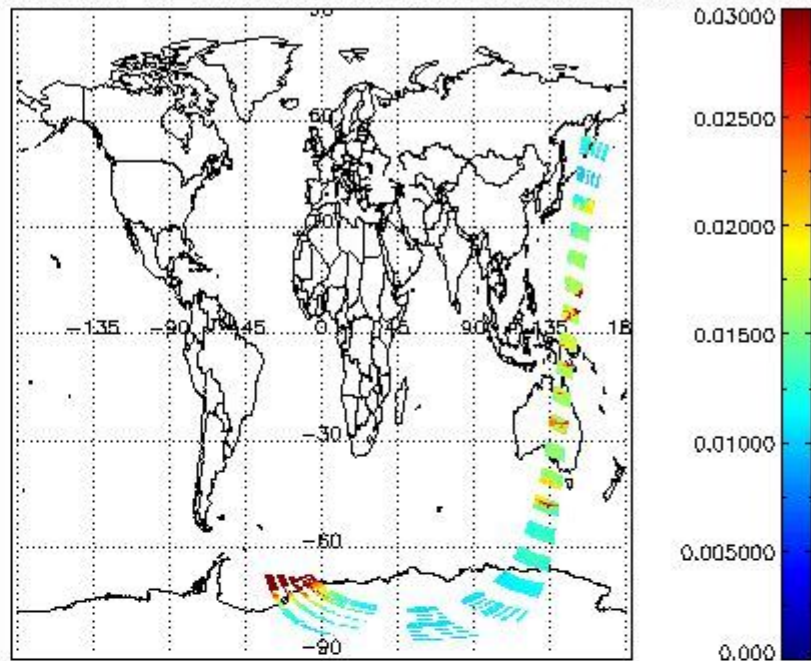
SCIOL2P_NADUV003_vcd_err for 20DEC2002 00:00:00 to 21DEC2002 00:00:00
