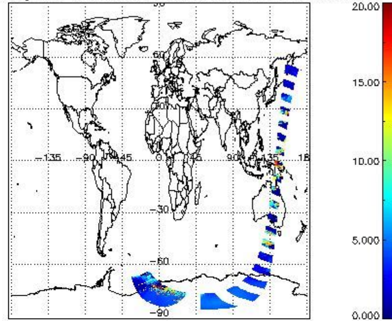
cl_top_height for 20DEC2002 00:00:00 to 21DEC2002 00:00:00
