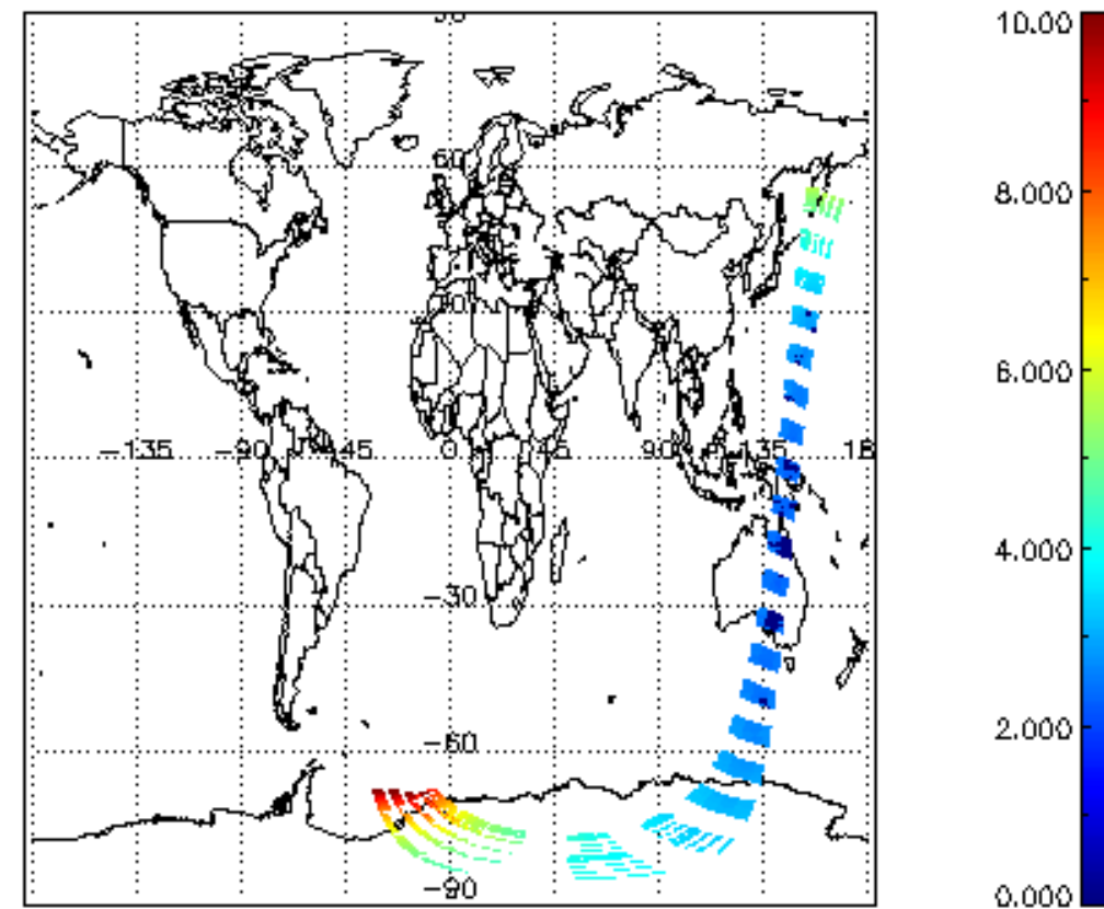
SCIOL2P_NADUV003_amf_cl for 20DEC2002 00:00:00 to 21DEC2002 00:00:00
