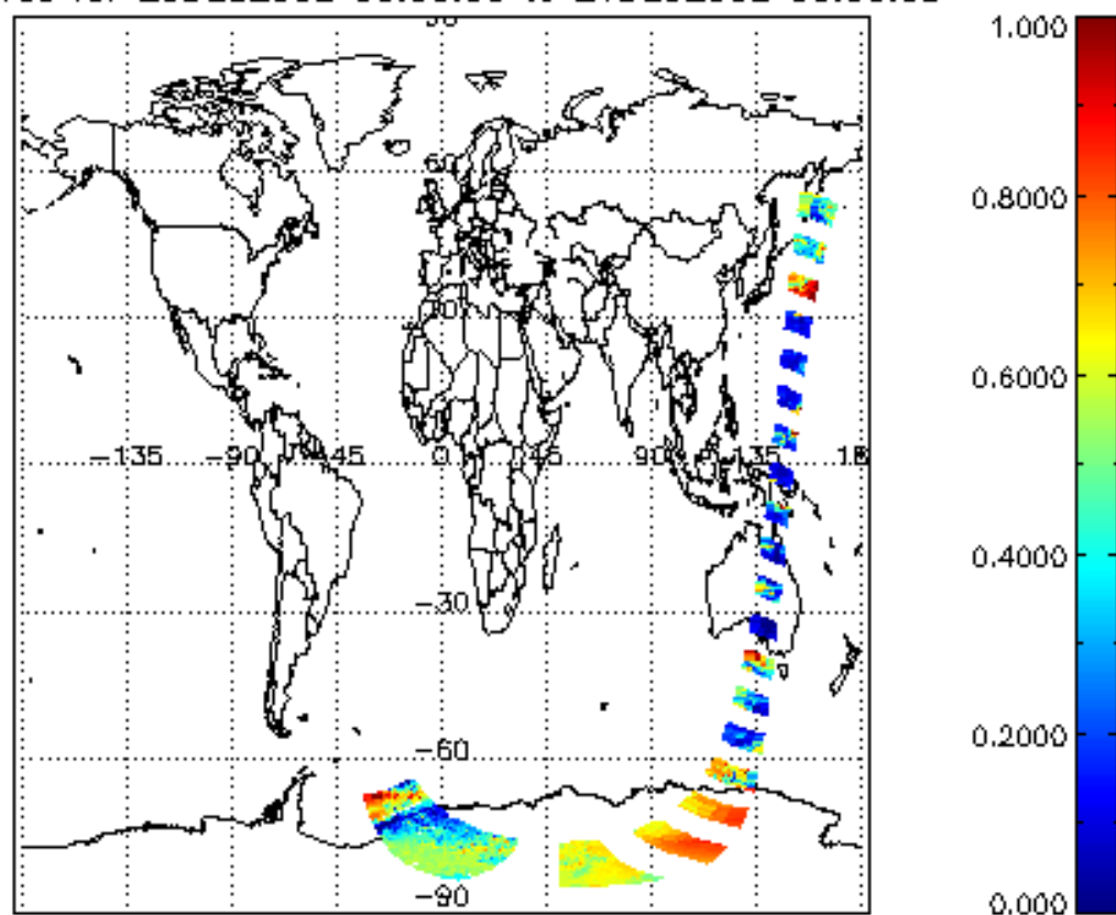
cl_frac for 20DEC2002 00:00:00 to 21DEC2002 00:00:00
