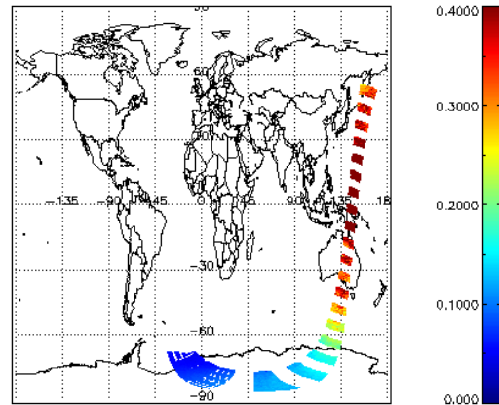
SCIOL2P_NADUV1NO2_vcd_err for 20DEC2002 00:00:00 to 21DEC2002 00:00:00
