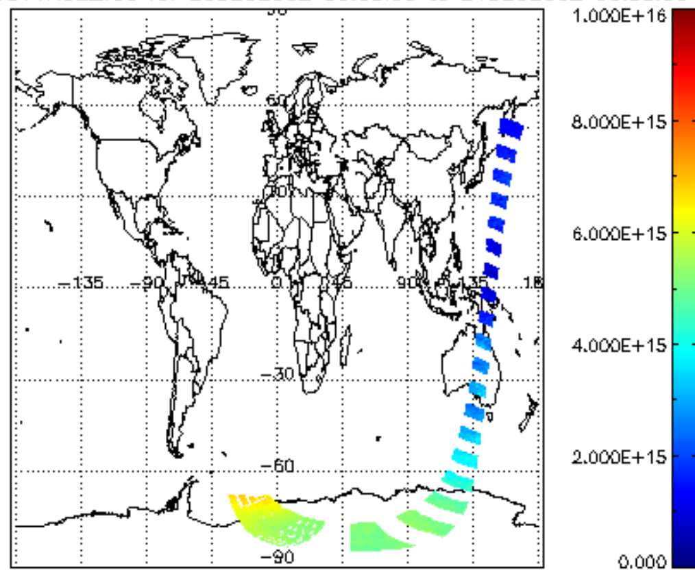
SCIOL2P_NADUV1NO2_vcd for 20DEC2002 00:00:00 to 21DEC2002 00:00:00
