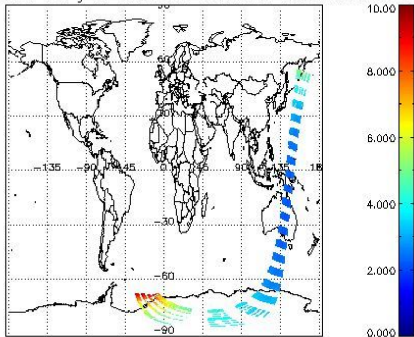
SCIOL2P_NADUV003_amf_gr for 20DEC2002 00:00:00 to 21DEC2002 00:00:00
