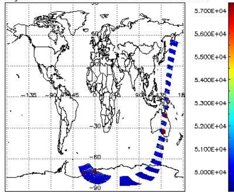
cloud_flags for 20DEC2002 00:00:00 to 21DEC2002 00:00:00
