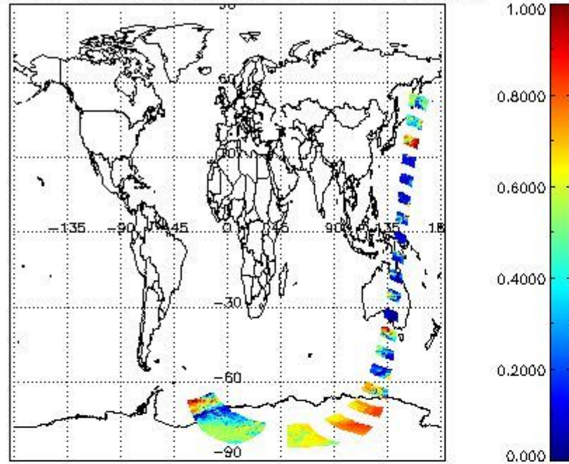
cl_frac for 20DEC2002 00:00:00 to 21DEC2002 00:00:00
