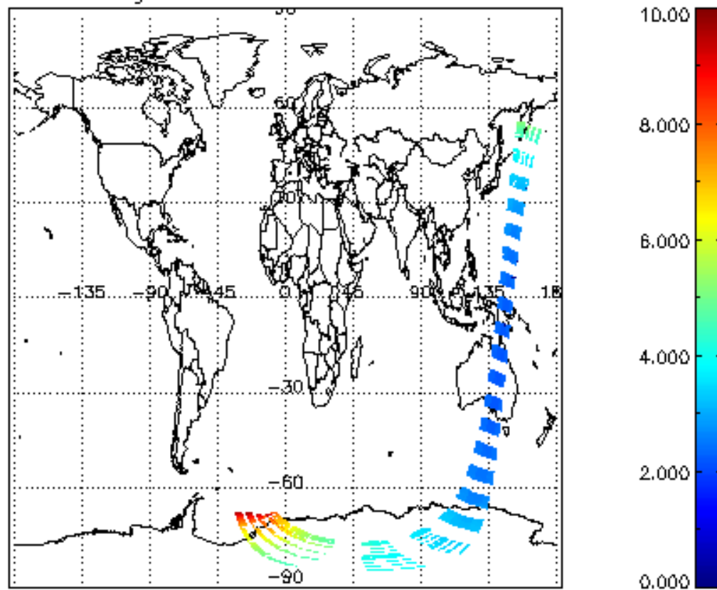
SCIOL2P_NADUV003_amf_gr for 20DEC2002 00:00:00 to 21DEC2002 00:00:00
