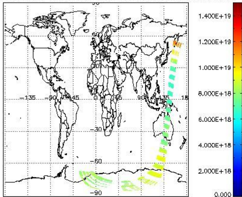
SCIOL2P_NADUV003_vcd for 20DEC2002 00:00:00 to 21DEC2002 00:00:00
