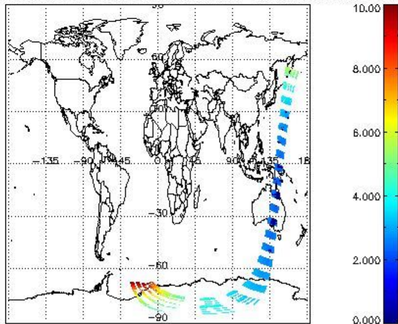
SCIOL2P_NADUV003_amf_cl for 20DEC2002 00:00:00 to 21DEC2002 00:00:00
