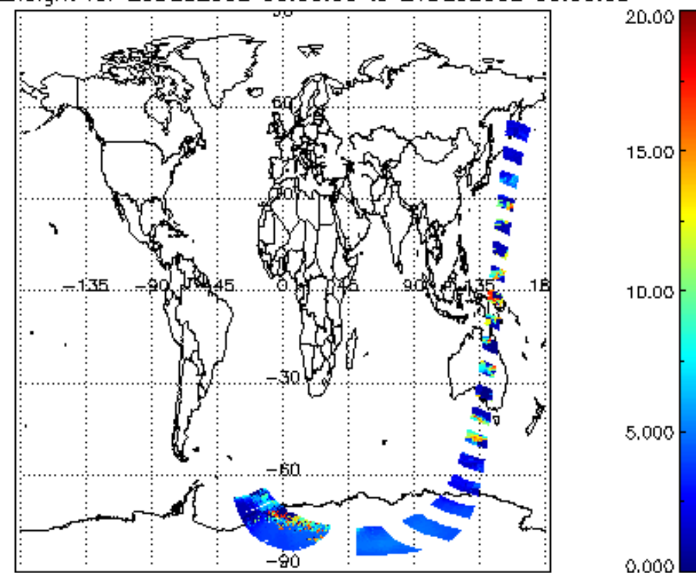
cl_top_height for 20DEC2002 00:00:00 to 21DEC2002 00:00:00
