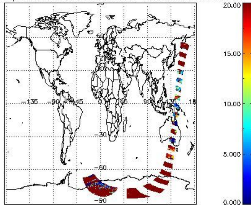
cl_opt_depth for 20DEC2002 00:00:00 to 21DEC2002 00:00:00
