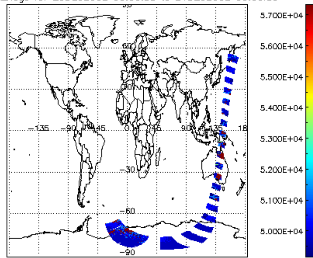
cloud_flags for 20DEC2002 00:00:00 to 21DEC2002 00:00:00
