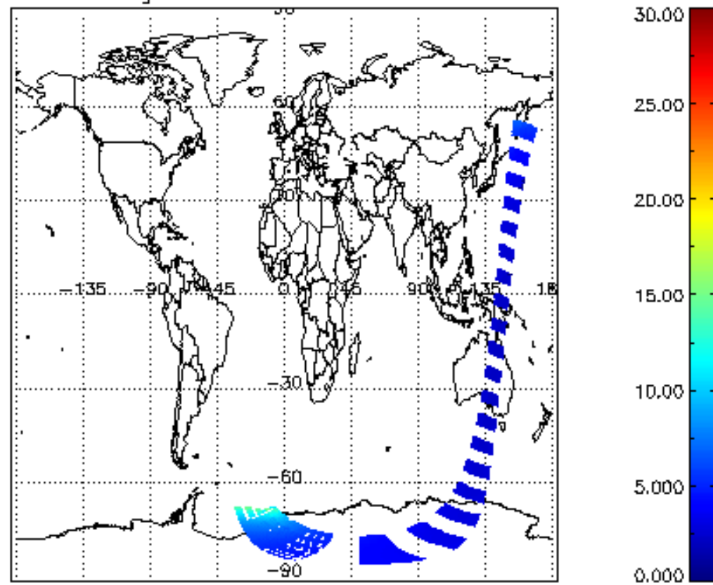
SCIOL2P_NADUV1NO2_amf_gr for 20DEC2002 00:00:00 to 21DEC2002 00:00:00
