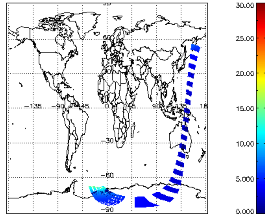
SCIOL2P_NADUV1NO2_amf_cl for 20DEC2002 00:00:00 to 21DEC2002 00:00:00
