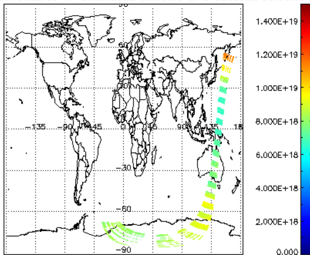
SCIOL2P_NADUV003_vcd for 20DEC2002 00:00:00 to 21DEC2002 00:00:00
