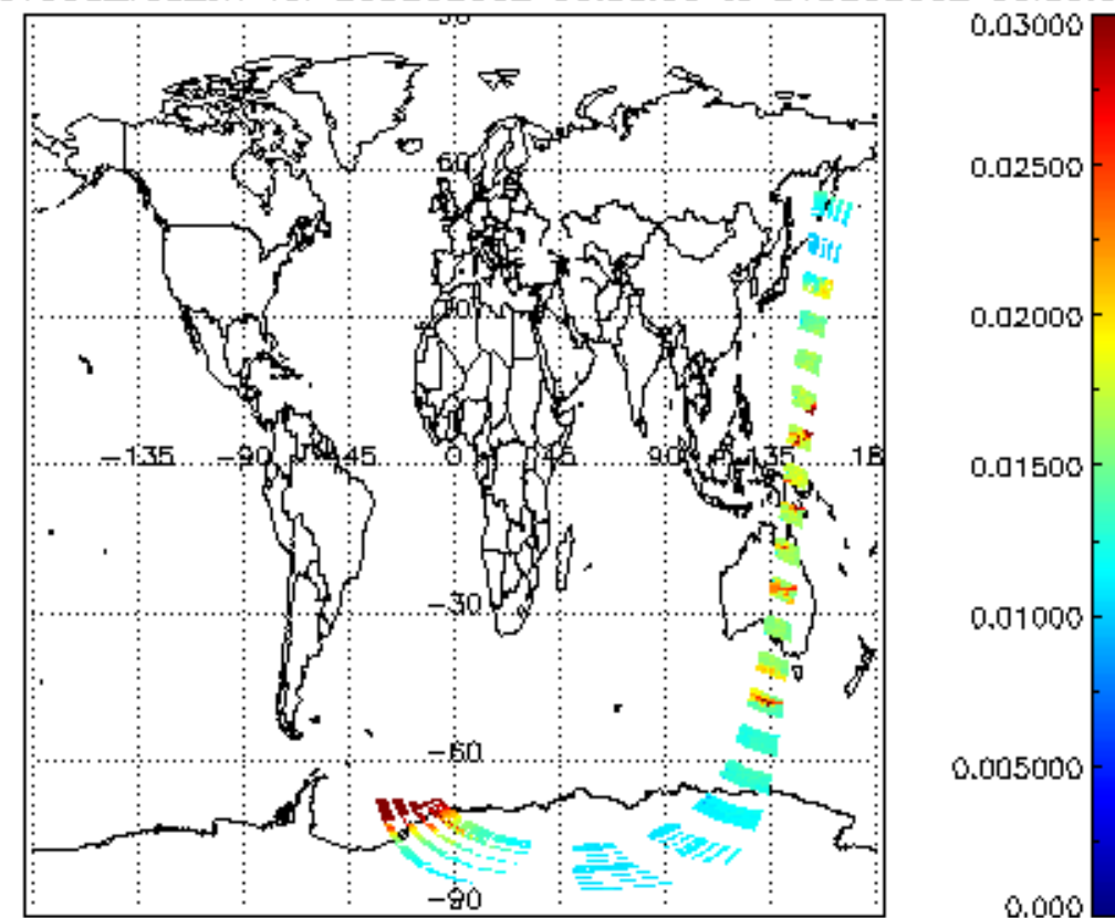
SCIOL2P_NADUV003_vcd_err for 20DEC2002 00:00:00 to 21DEC2002 00:00:00
