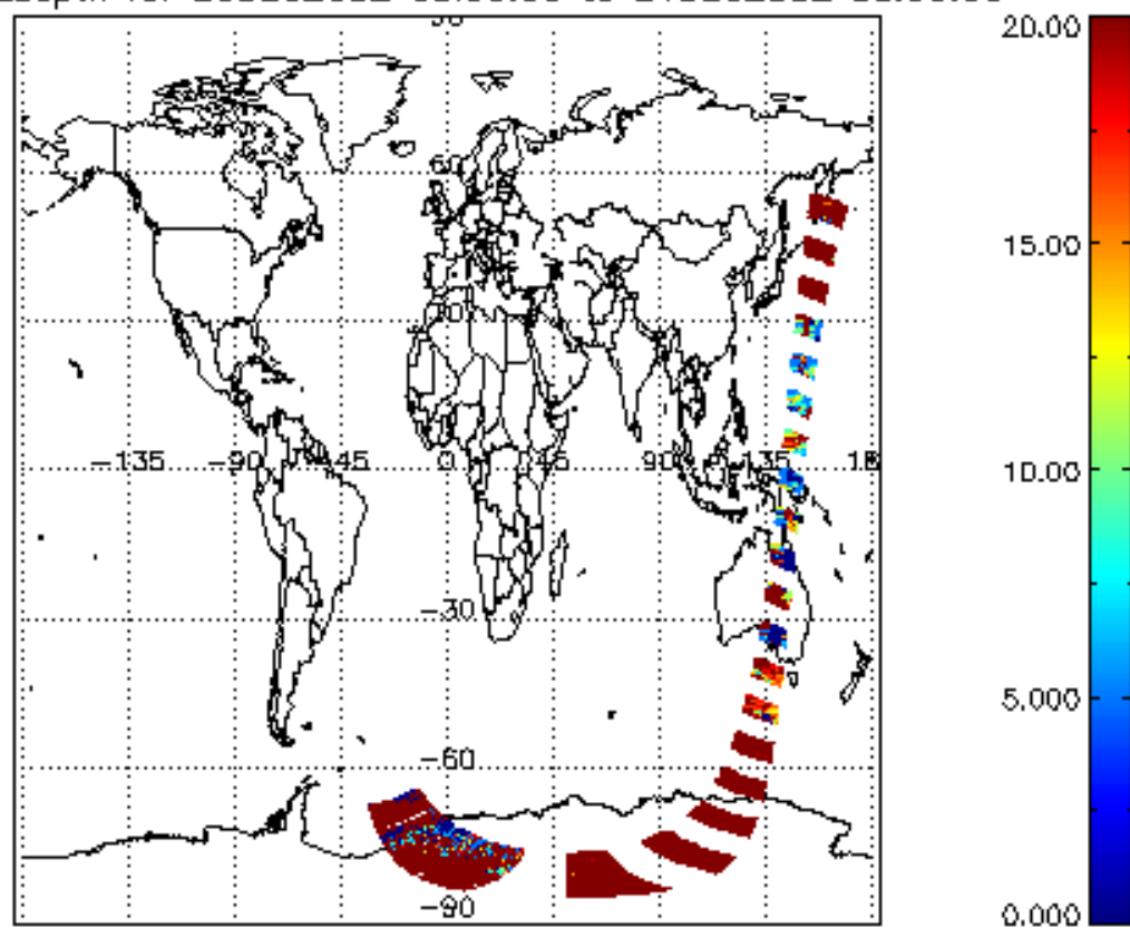
cl_opt_depth for 20DEC2002 00:00:00 to 21DEC2002 00:00:00
