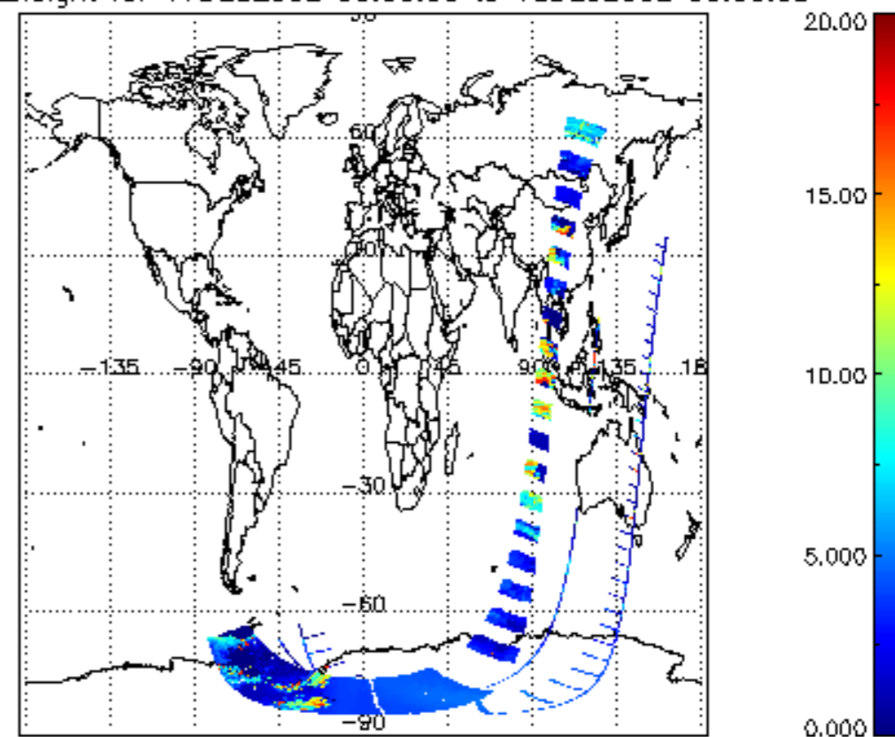
cl_top_height for 17DEC2002 00:00:00 to 18DEC2002 00:00:00
