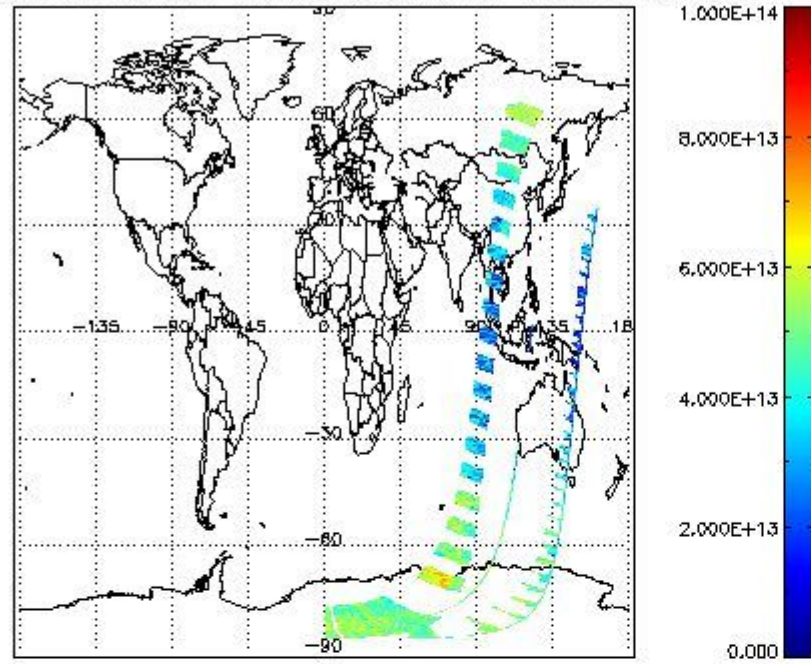
SCIOL2P_NADUV3BRO_vcd for 17DEC2002 00:00:00 to 18DEC2002 00:00:00
