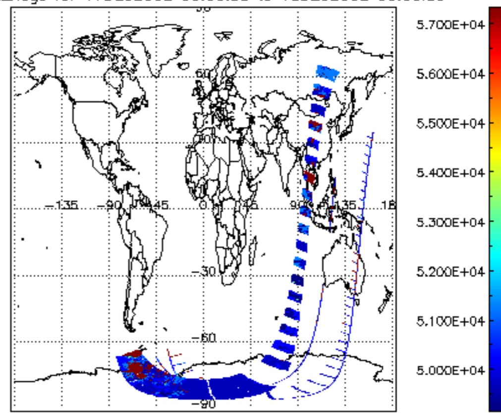
cloud_flags for 17DEC2002 00:00:00 to 18DEC2002 00:00:00
