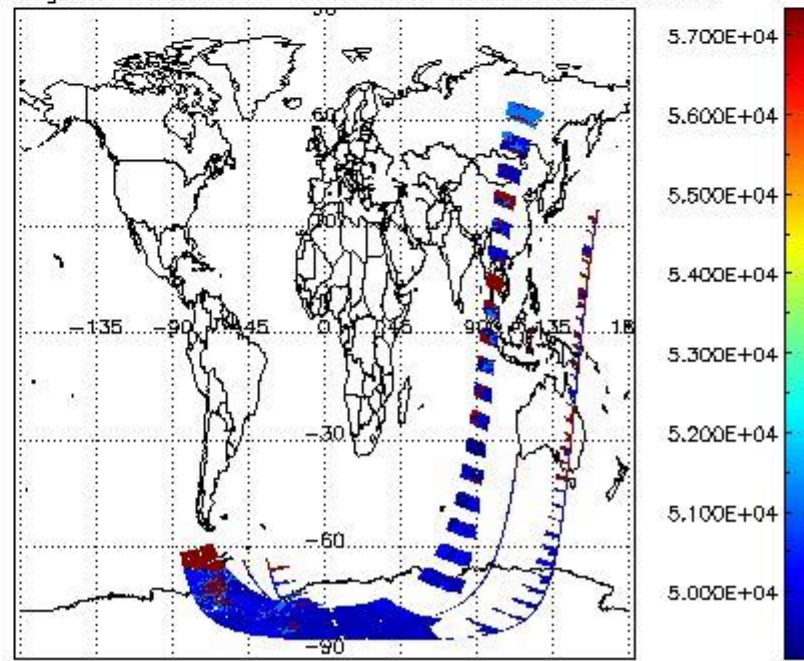
cloud_flags for 17DEC2002 00:00:00 to 18DEC2002 00:00:00
