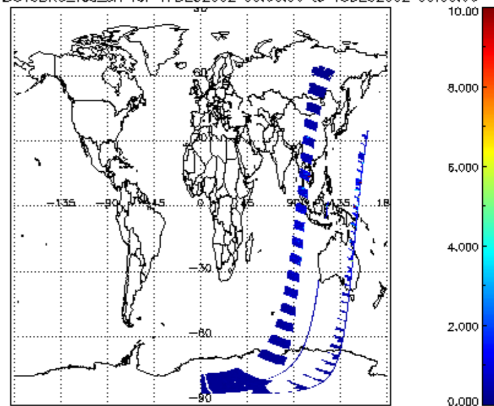
SCIOL2P_NADUV3BRO_vcd_err for 17DEC2002 00:00:00 to 18DEC2002 00:00:00
