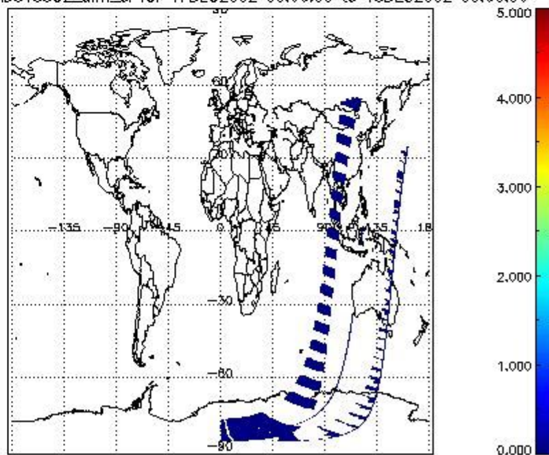
SCIOL2P_NADUV5S02_amf_cl for 17DEC2002 00:00:00 to 18DEC2002 00:00:00
