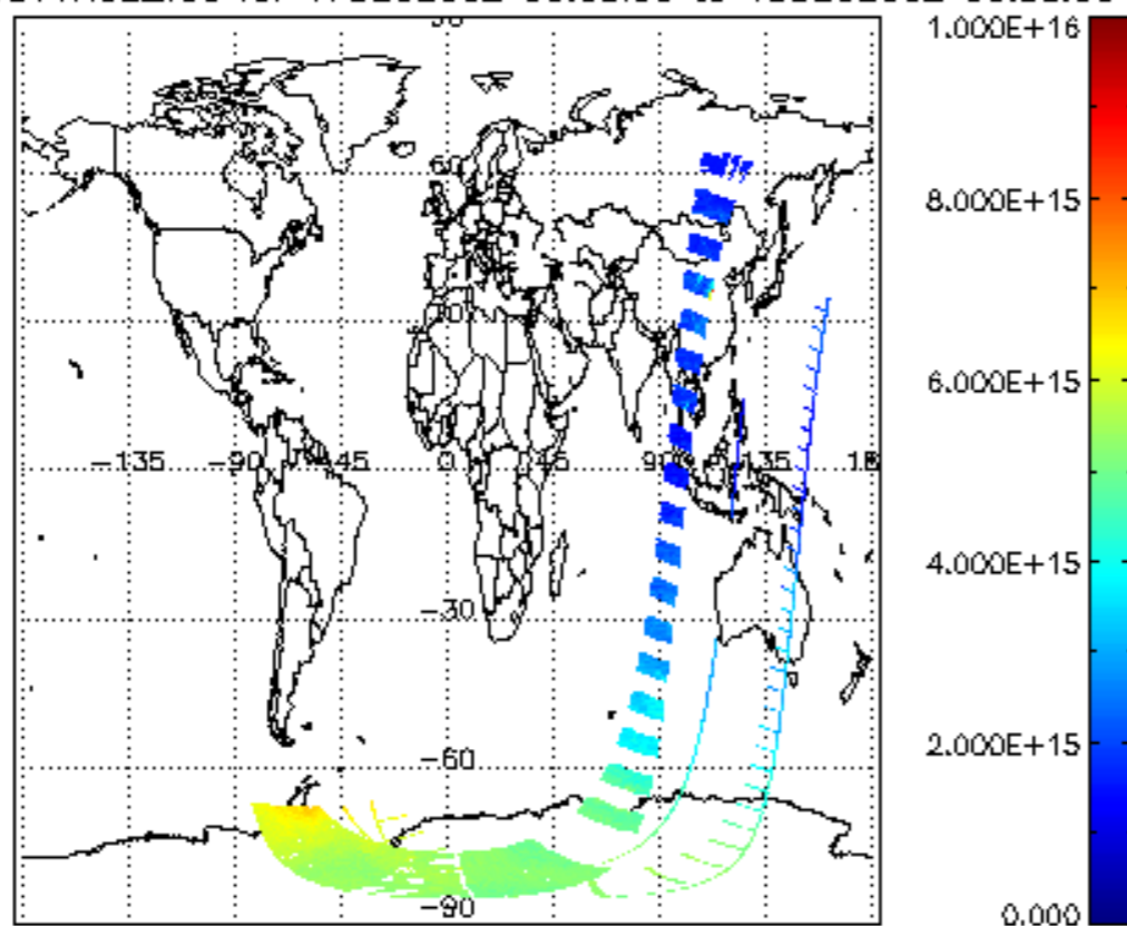
SCIOL2P_NADUV1NO2_vcd for 17DEC2002 00:00:00 to 18DEC2002 00:00:00
