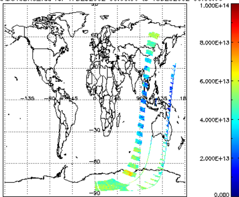
SCIOL2P_NADUV3BRO_vcd for 17DEC2002 00:00:00 to 18DEC2002 00:00:00
