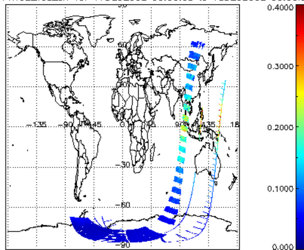
SCIOL2P_NADUV1NO2_vcd_err for 17DEC2002 00:00:00 to 18DEC2002 00:00:00
