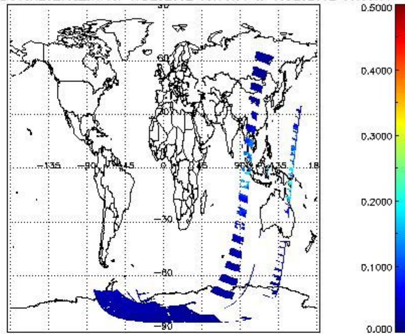
SCIOL2P_NADUV8H2O_vcd_err for 17DEC2002 00:00:00 to 18DEC2002 00:00:00
