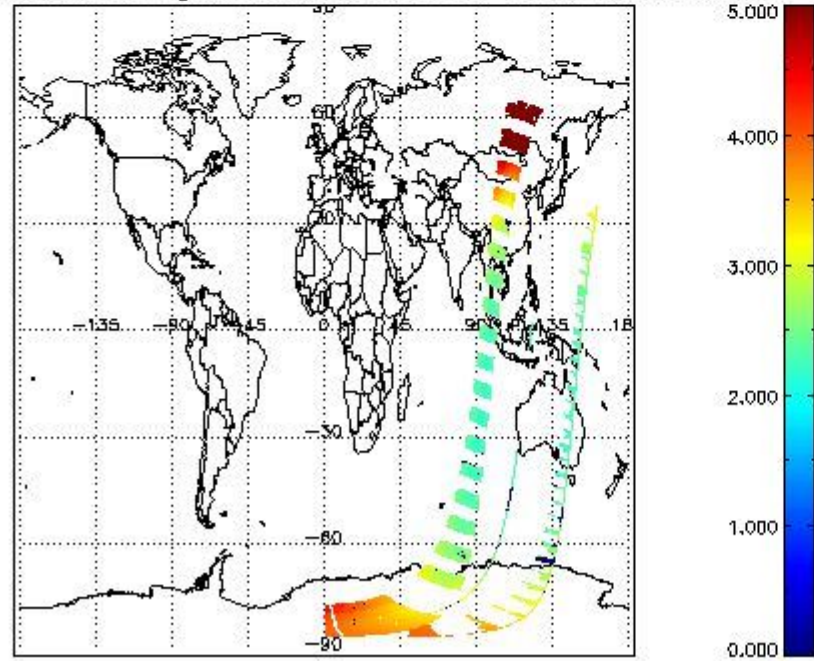
SCIOL2P_NADUV1N02_amf_gr for 17DEC2002 00:00:00 to 18DEC2002 00:00:00
