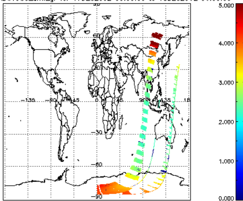
SCIOL2P_NADUV003_amf_gr for 17DEC2002 00:00:00 to 18DEC2002 00:00:00
