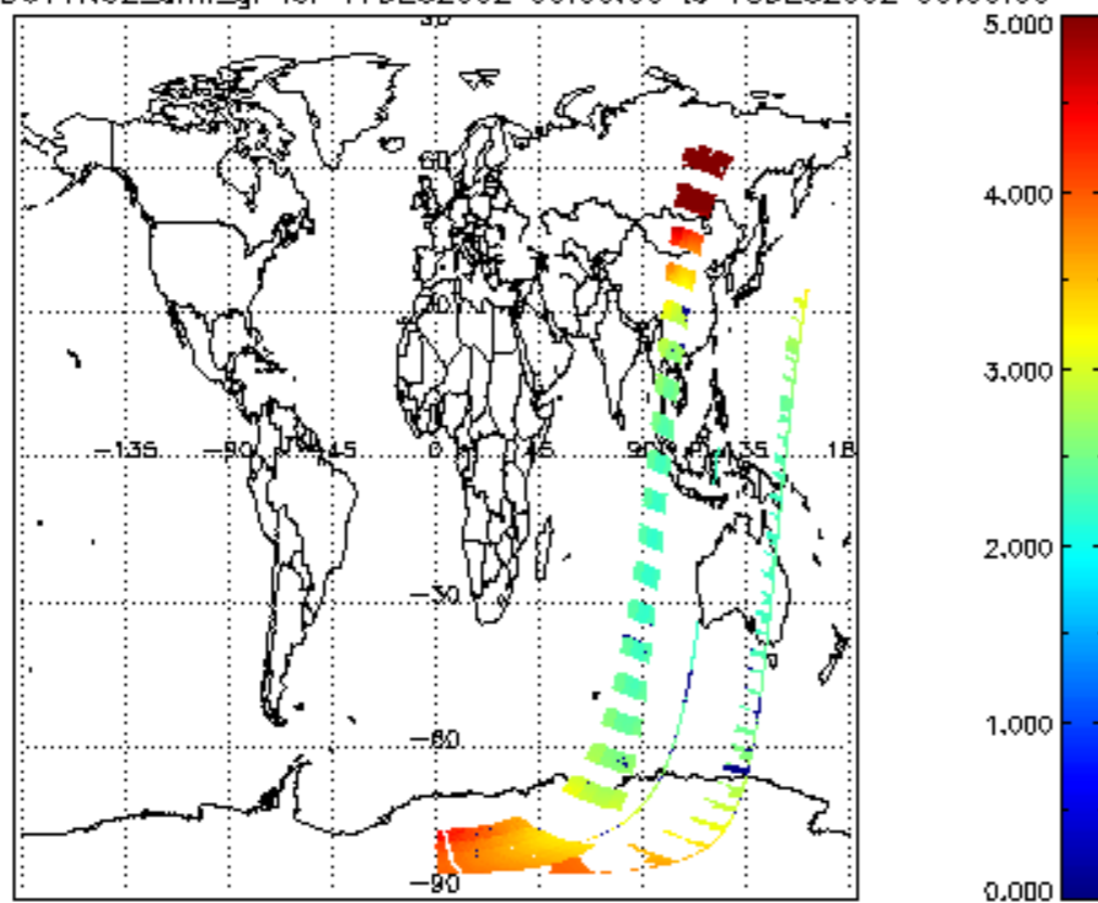
SCIOL2P_NADUV1NO2_amf_gr for 17DEC2002 00:00:00 to 18DEC2002 00:00:00
