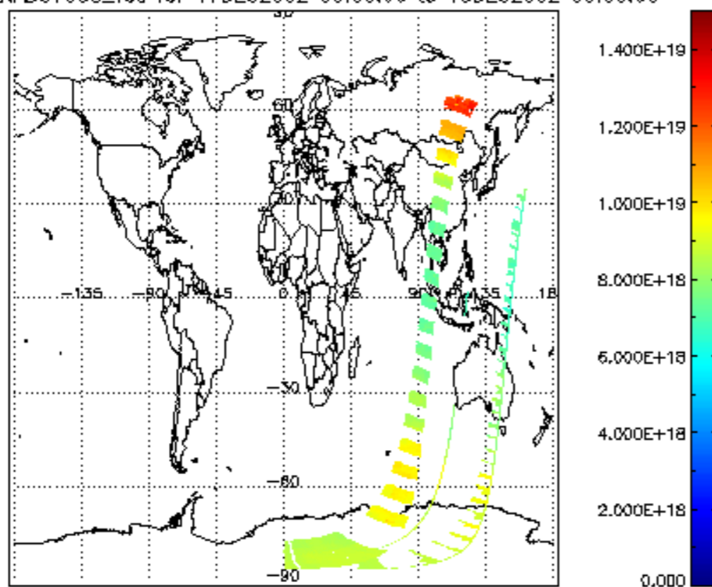
SCIOL2P_NADUV003_vcd for 17DEC2002 00:00:00 to 18DEC2002 00:00:00
