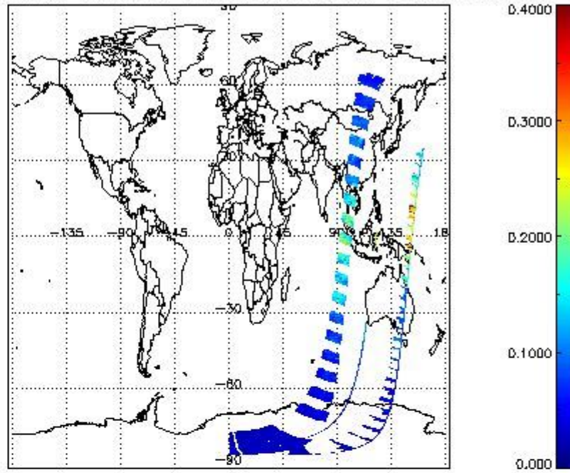
SCIOL2P_NADUV1N02_vcd_err for 17DEC2002 00:00:00 to 18DEC2002 00:00:00
