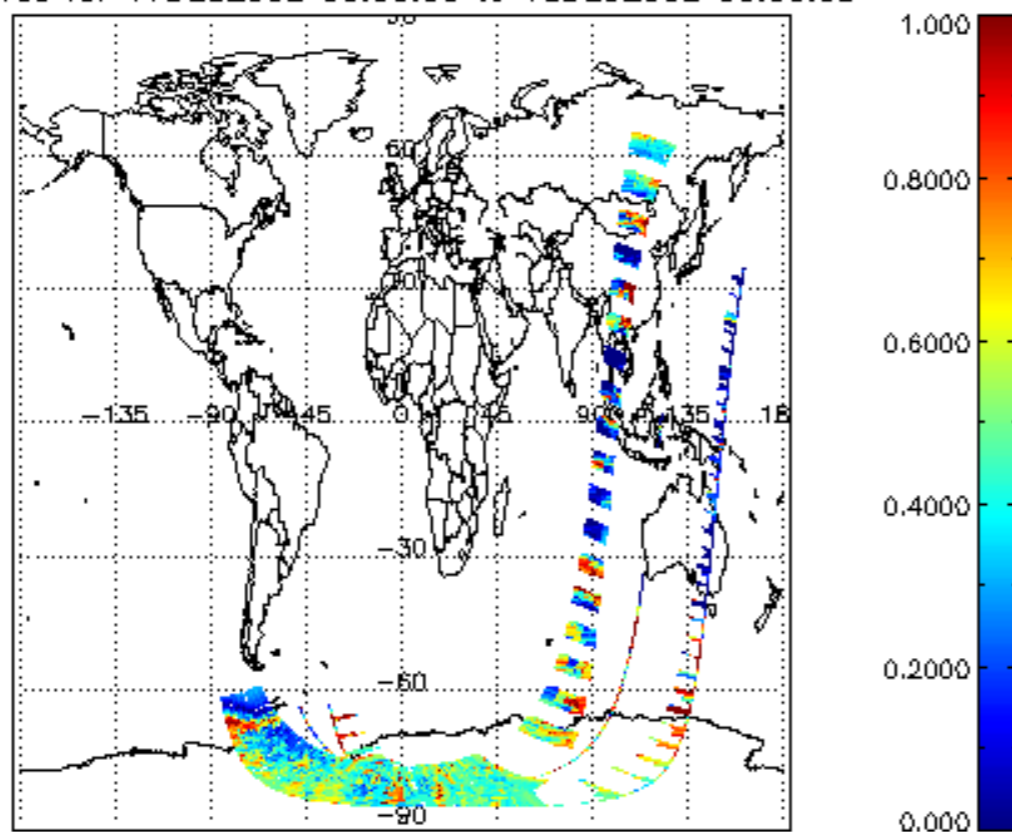
cl_frac for 17DEC2002 00:00:00 to 18DEC2002 00:00:00
