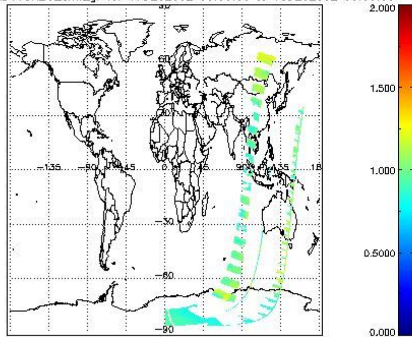
SCIOL2P_NADUV8H2O_amf_gr for 17DEC2002 00:00:00 to 18DEC2002 00:00:00
