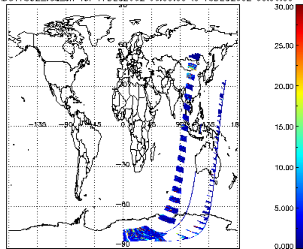
SCIOL2P_NADUV7S02_vcd_err for 17DEC2002 00:00:00 to 18DEC2002 00:00:00
