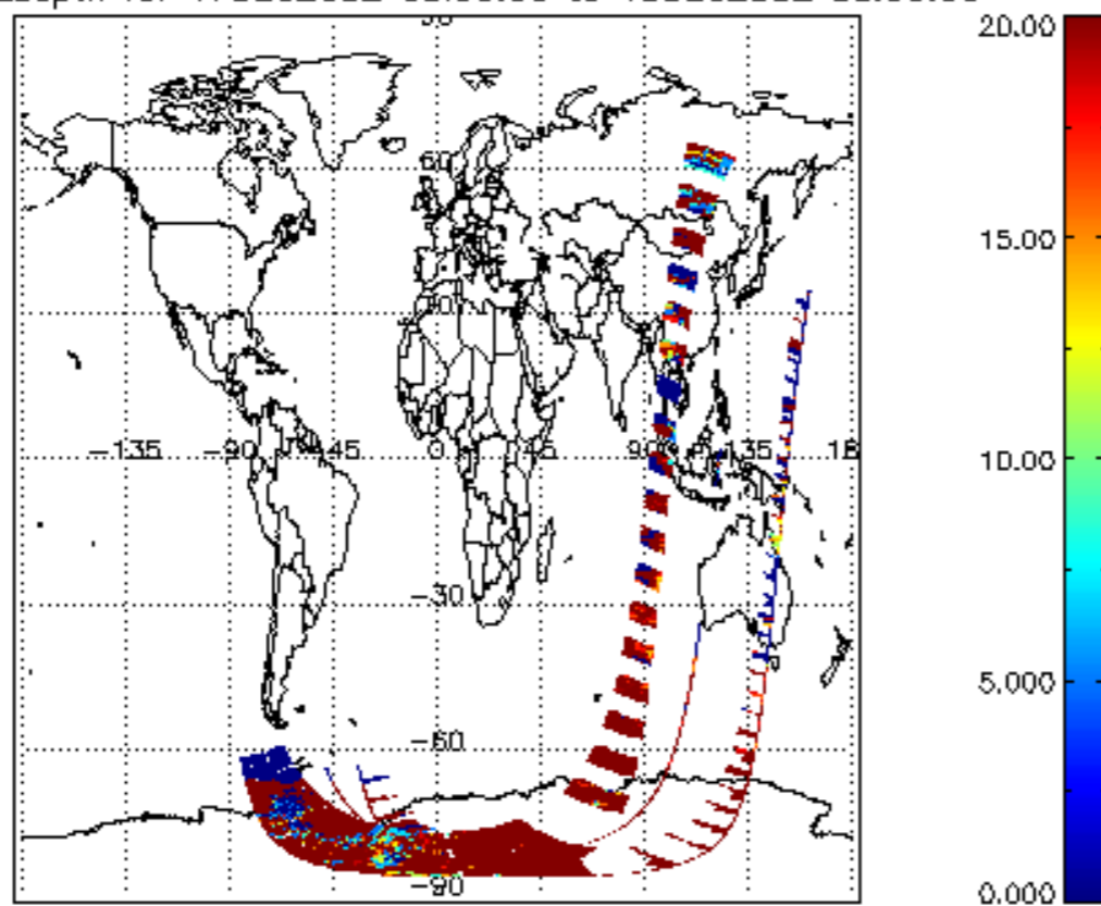
cl_opt_depth for 17DEC2002 00:00:00 to 18DEC2002 00:00:00
