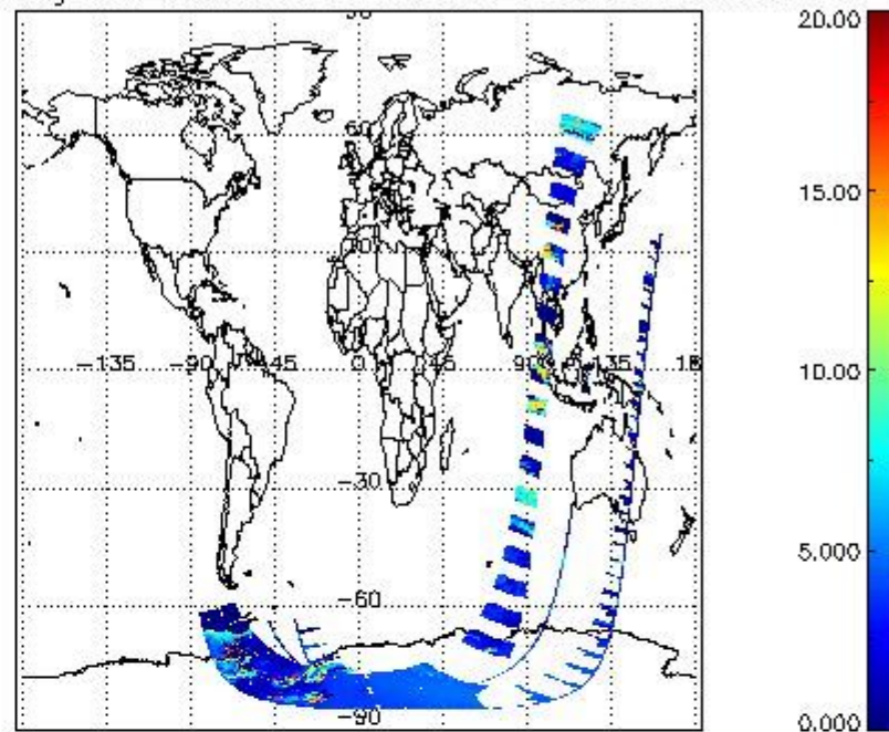
cL_top_height for 17DEC2002 00:00:00 to 18DEC2002 00:00:00
