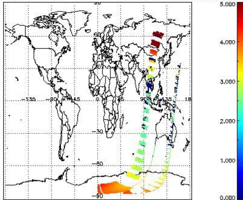
SCIOL2P_NADUV003_amf_cl for 17DEC2002 00:00:00 to 18DEC2002 00:00:00
