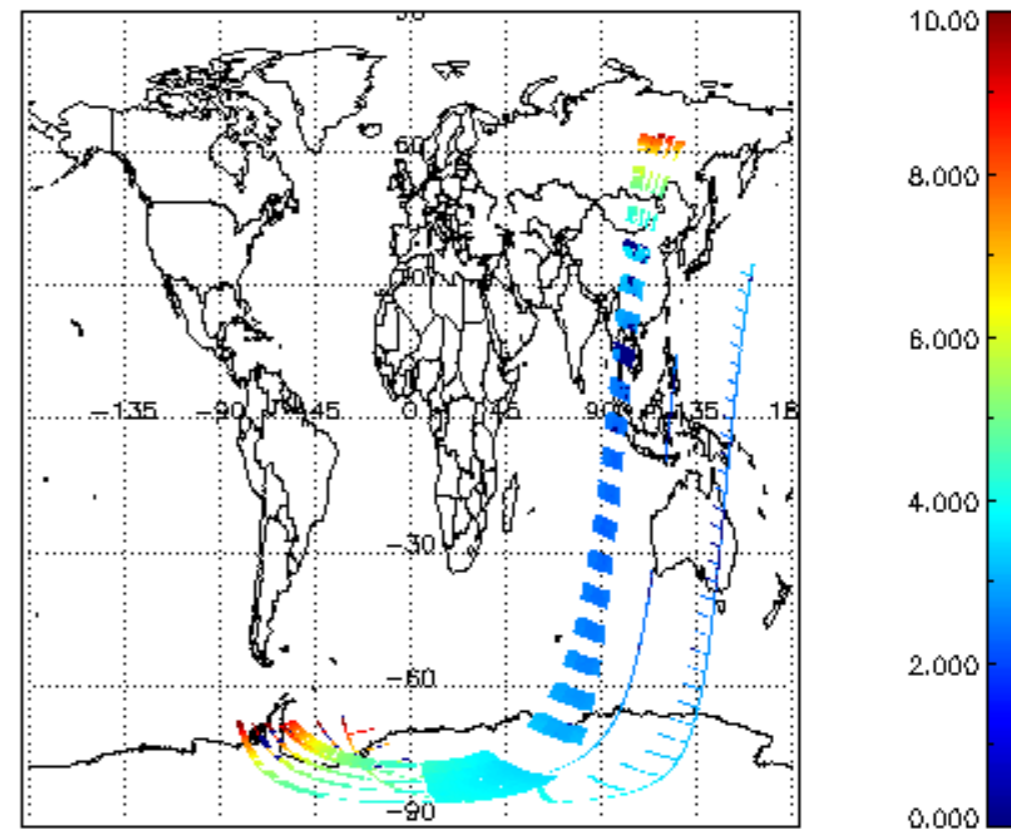
SCIOL2P_NADUV003_amf_cl for 17DEC2002 00:00:00 to 18DEC2002 00:00:00
