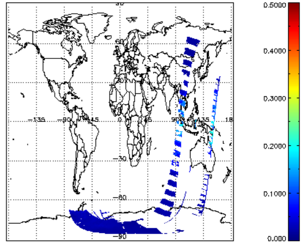
SCIOL2P_NADUV8H2O_vcd_err for 17DEC2002 00:00:00 to 18DEC2002 00:00:00
