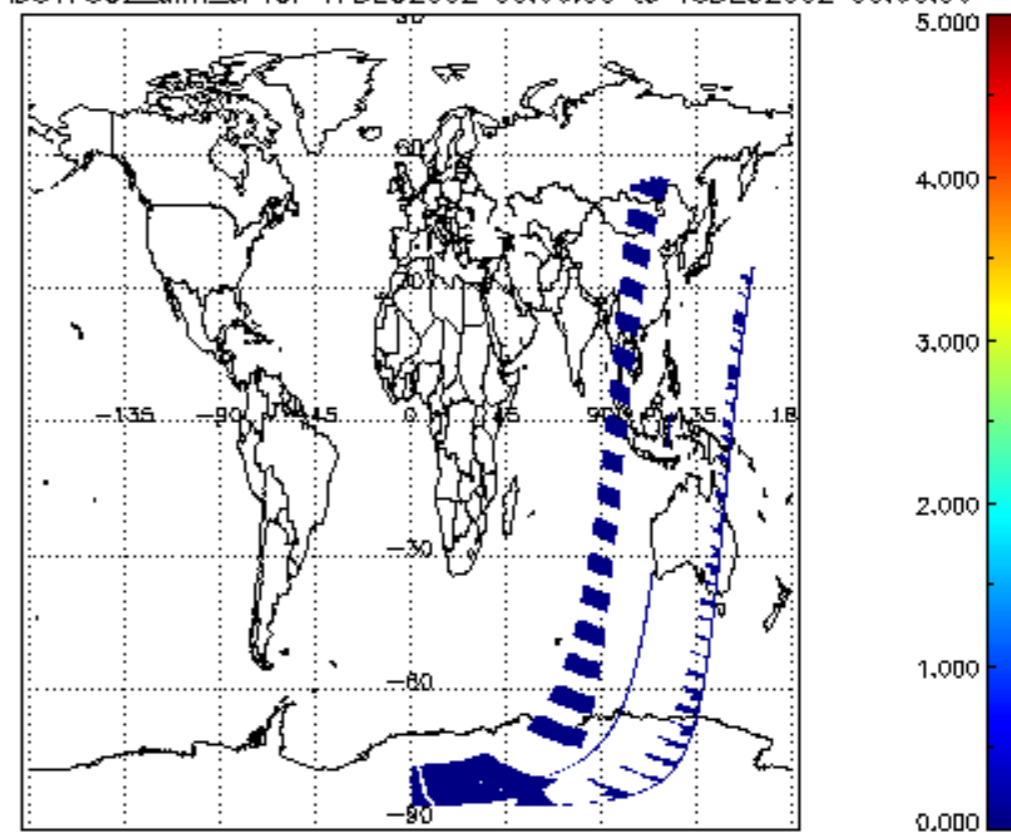
SCIOL2P_NADUV7S02_amf_cl for 17DEC2002 00:00:00 to 18DEC2002 00:00:00
