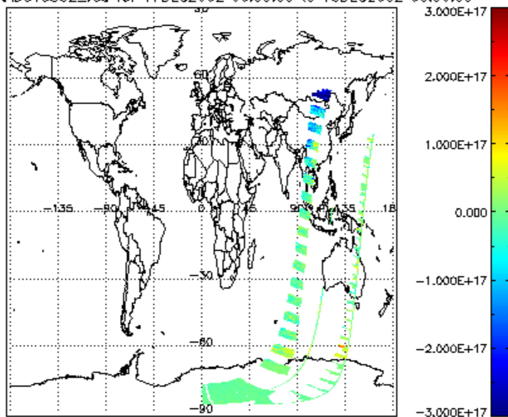
SCIOL2P_NADUV5SO2_vcd for 17DEC2002 00:00:00 to 18DEC2002 00:00:00
