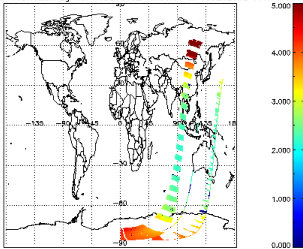
SCIOL2P_NADUV3BRO_amf_gr for 17DEC2002 00:00:00 to 18DEC2002 00:00:00
