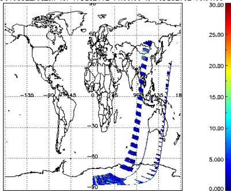
SCIOL2P_NADUV5S02_vcd_err for 17DEC2002 00:00:00 to 18DEC2002 00:00:00
