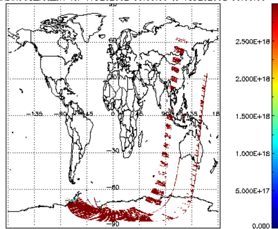
SCIOL2P_NADIR3CO_vcd_err for 17DEC2002 00:00:00 to 18DEC2002 00:00:00
