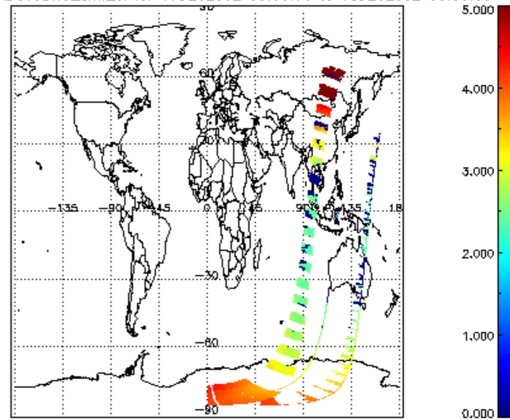
SCIOL2P_NADUV3BRO_amf_cl for 17DEC2002 00:00:00 to 18DEC2002 00:00:00
