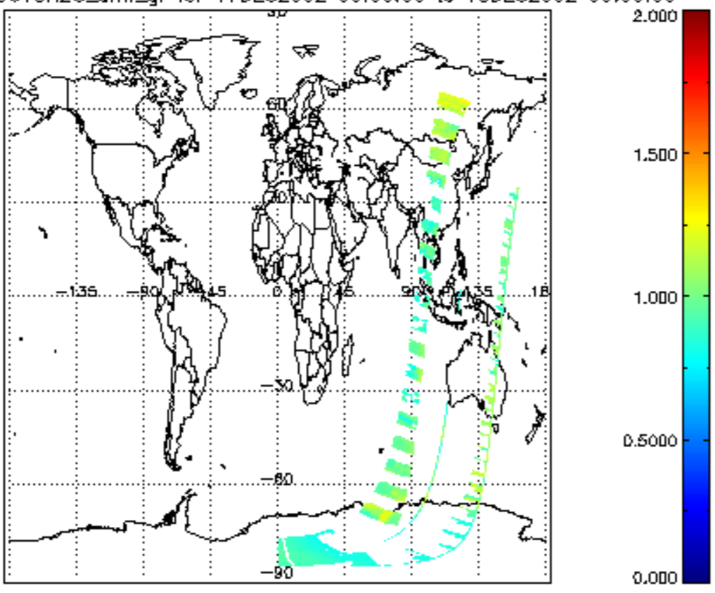
SCIOL2P_NADUV8H2O_amf_gr for 17DEC2002 00:00:00 to 18DEC2002 00:00:00
