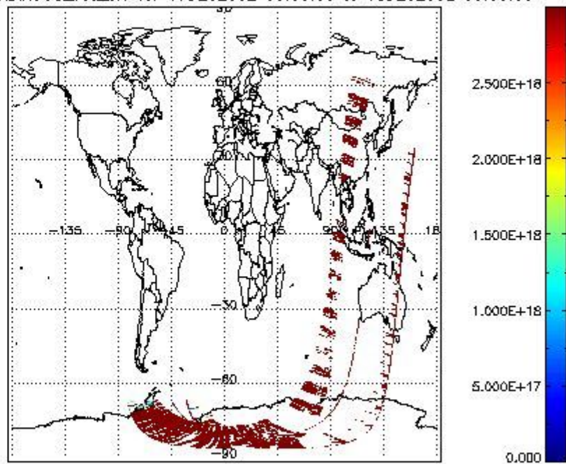
SCIDL2P_NADIR3CO_vcd_err for 17DEC2002 00:00:00 to 18DEC2002 00:00:00
