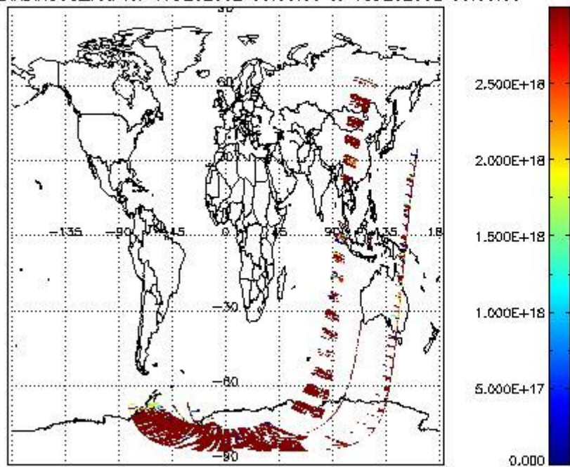
SCIDL2P_NADIR3CO_vcd for 17DEC2002 00:00:00 to 18DEC2002 00:00:00
