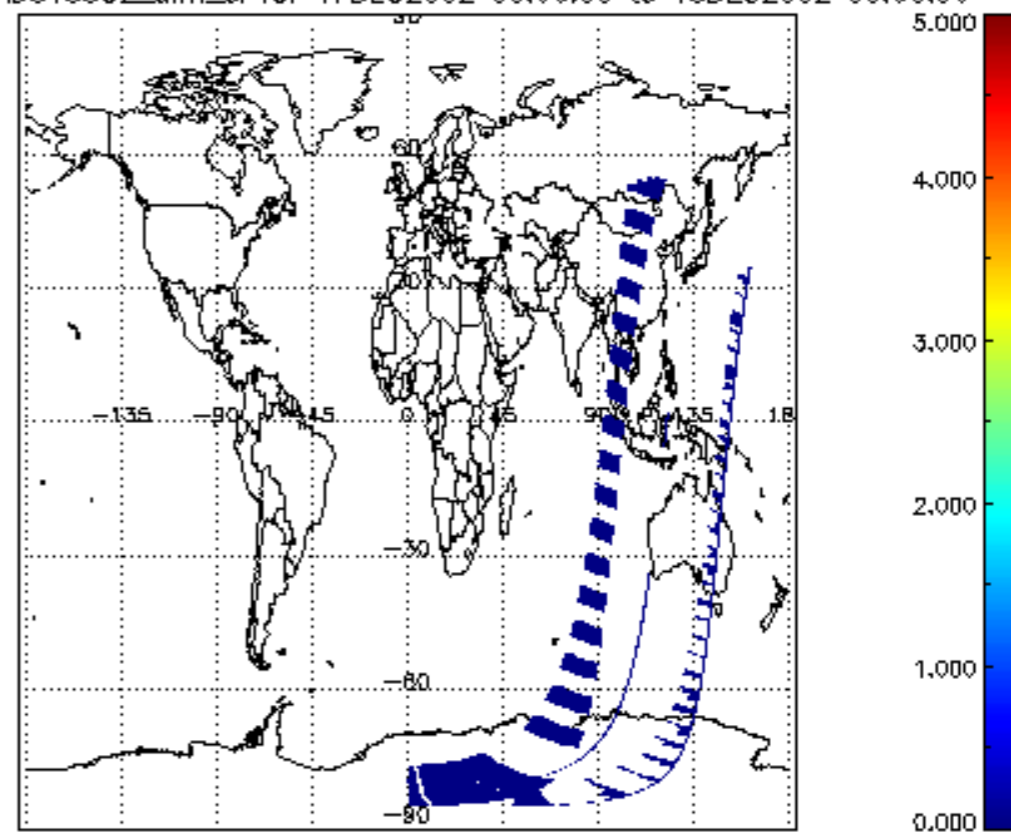
SCIOL2P_NADUV5SO2_amf_cl for 17DEC2002 00:00:00 to 18DEC2002 00:00:00
