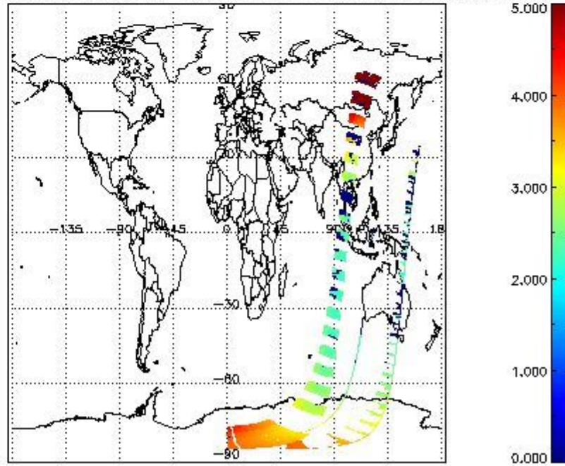
SCIOL2P_NADUV1N02_amf_cl for 17DEC2002 00:00:00 to 18DEC2002 00:00:00
