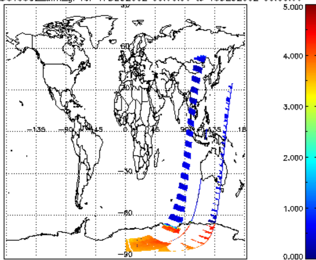
SCIOL2P_NADUV5SO2_amf_gr for 17DEC2002 00:00:00 to 18DEC2002 00:00:00
