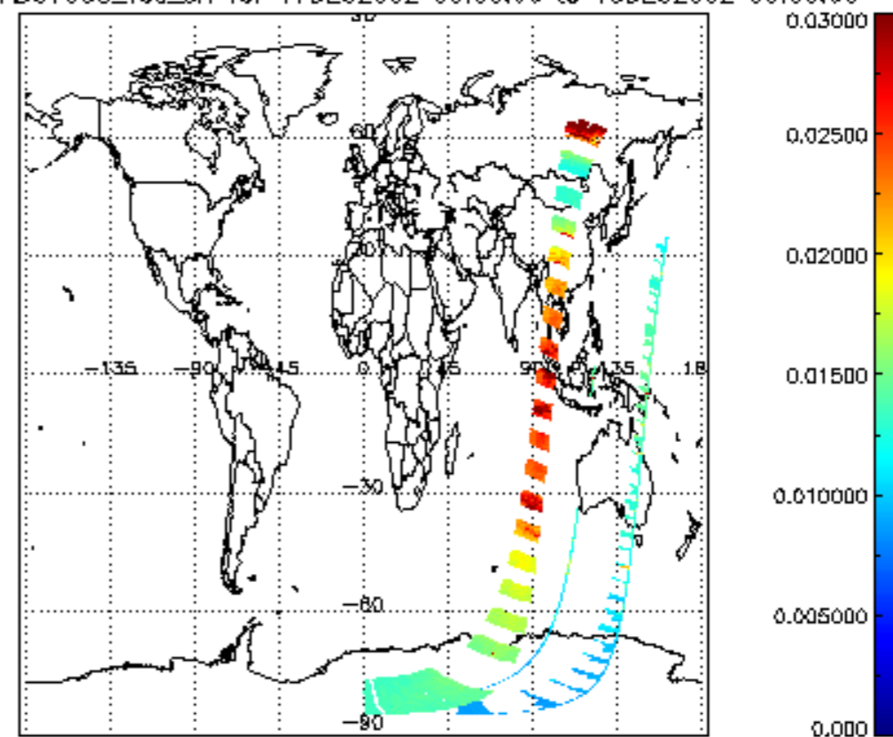
SCIOL2P_NADUV003_vcd_err for 17DEC2002 00:00:00 to 18DEC2002 00:00:00
