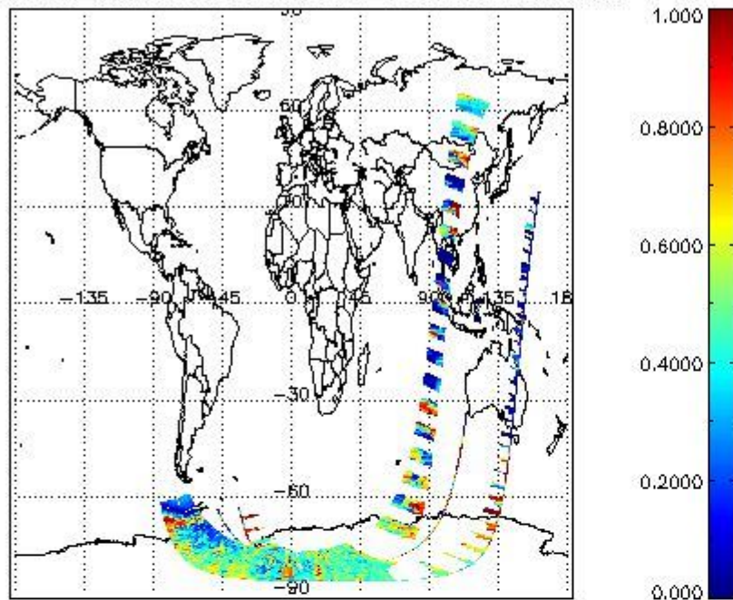
cL_frac for 17DEC2002 00:00:00 to 18DEC2002 00:00:00
