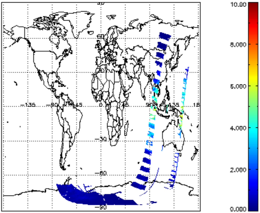
SCIOL2P_NADUV8H2O_vcd for 17DEC2002 00:00:00 to 18DEC2002 00:00:00
