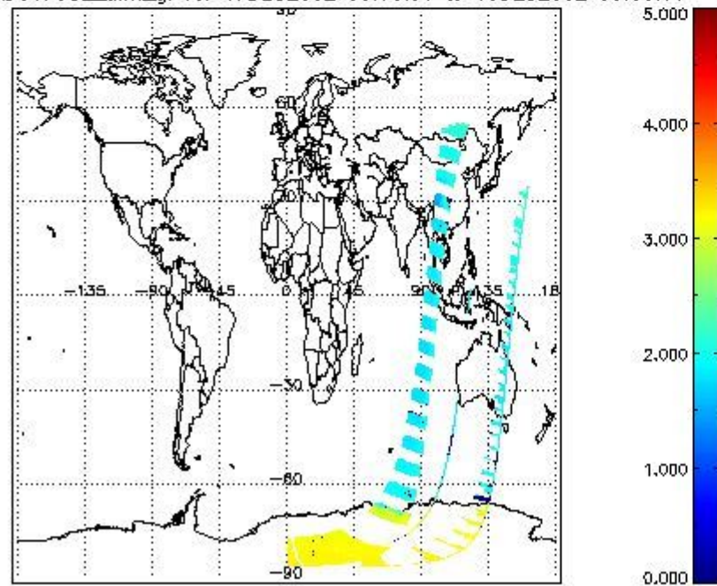
SCIOL2P_NADUV7S02_amf_gr for 17DEC2002 00:00:00 to 18DEC2002 00:00:00
