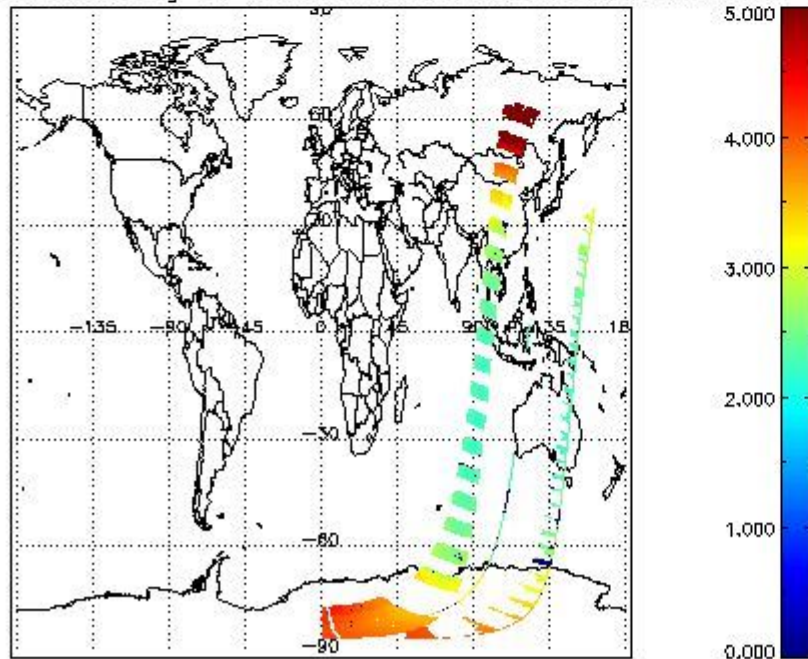
SCIOL2P_NADUV003_amf_gr for 17DEC2002 00:00:00 to 18DEC2002 00:00:00
