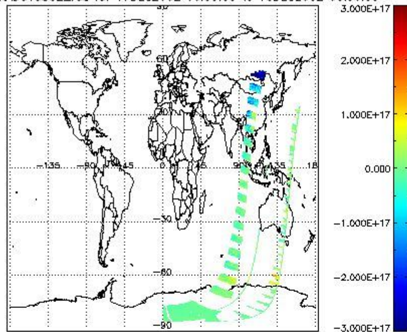
SCIOL2P_NADUV5S02_vcd for 17DEC2002 00:00:00 to 18DEC2002 00:00:00
