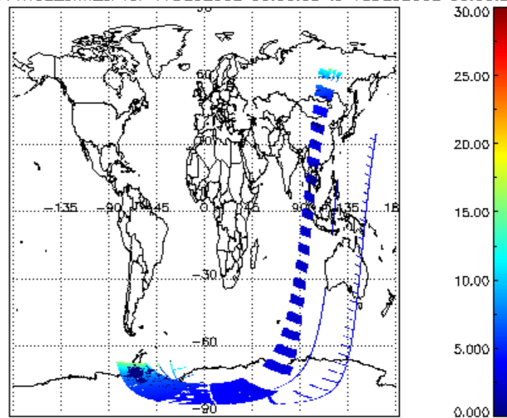
SCIOL2P_NADUV1NO2_amf_cl for 17DEC2002 00:00:00 to 18DEC2002 00:00:00
