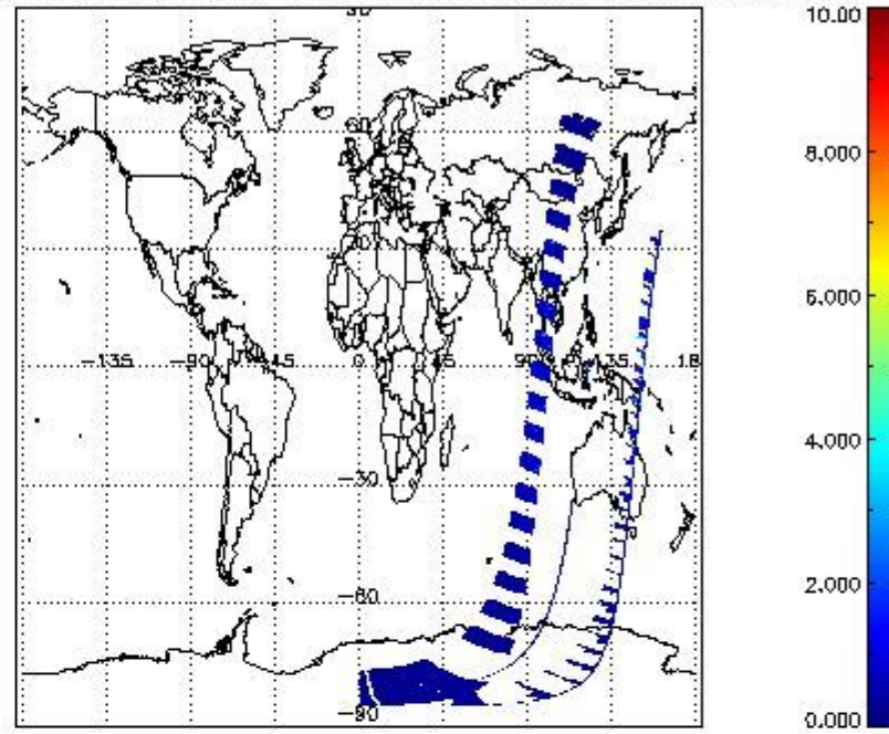
SCIOL2P_NADUV3BRO_vcd_err for 17DEC2002 00:00:00 to 18DEC2002 00:00:00
