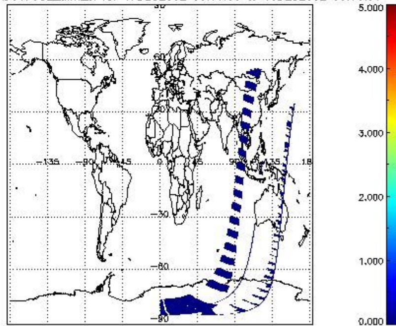
SCIOL2P_NADUV7S02_amf_cl for 17DEC2002 00:00:00 to 18DEC2002 00:00:00
