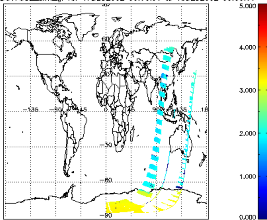
SCIOL2P_NADUV7S02_amf_gr for 17DEC2002 00:00:00 to 18DEC2002 00:00:00
