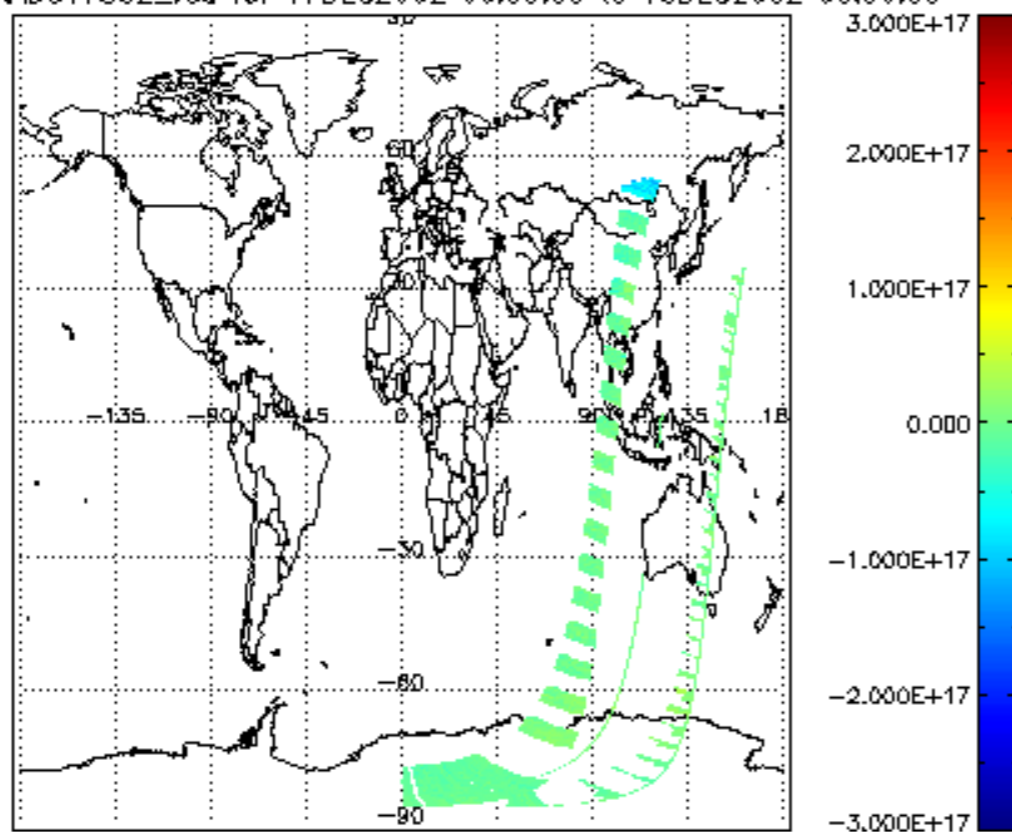
SCIOL2P_NADUV7S02_vcd for 17DEC2002 00:00:00 to 18DEC2002 00:00:00
