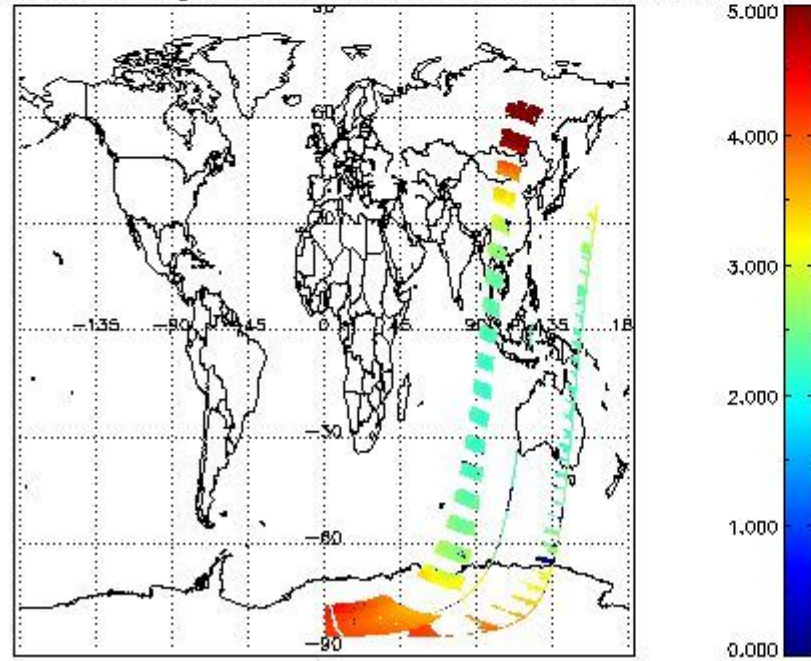
SCIOL2P_NADUV3BRO_amf_gr for 17DEC2002 00:00:00 to 18DEC2002 00:00:00
