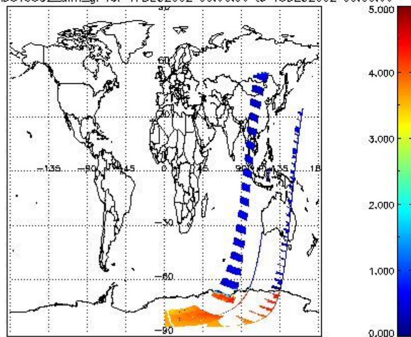
SCIOL2P_NADUV5S02_amf_gr for 17DEC2002 00:00:00 to 18DEC2002 00:00:00
