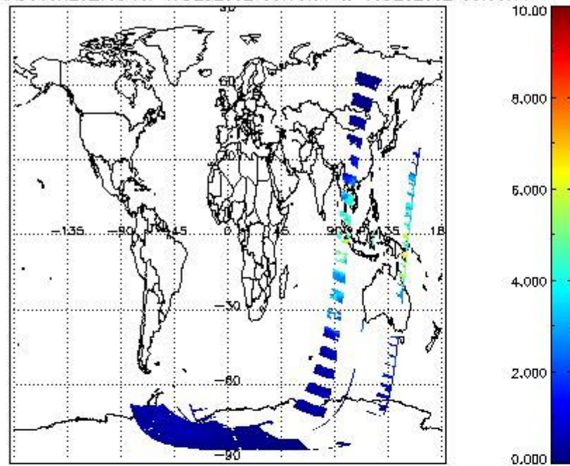
SCIOL2P_NADUV8H2O_vcd for 17DEC2002 00:00:00 to 18DEC2002 00:00:00
