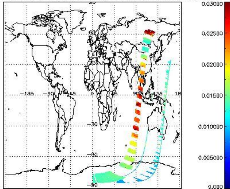
SCIOL2P_NADUV003_vcd_err for 17DEC2002 00:00:00 to 18DEC2002 00:00:00
