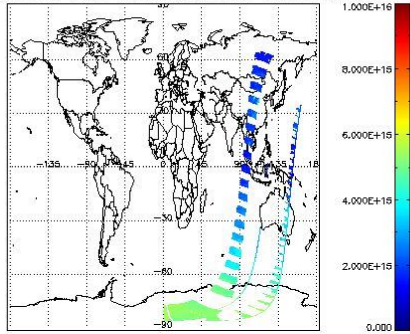
SCIOL2P_NADUV1N02_vcd for 17DEC2002 00:00:00 to 18DEC2002 00:00:00
