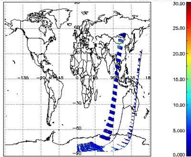
SCIOL2P_NADUV7S02_vcd_err for 17DEC2002 00:00:00 to 18DEC2002 00:00:00
