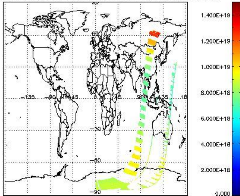
SCIOL2P_NADUV003_vcd for 17DEC2002 00:00:00 to 18DEC2002 00:00:00
