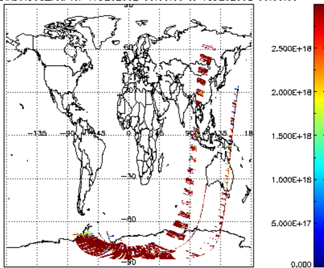
SCIOL2P_NADIR3CO_vcd for 17DEC2002 00:00:00 to 18DEC2002 00:00:00
