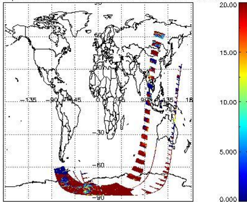
cL_opt_depth for 17DEC2002 00:00:00 to 18DEC2002 00:00:00
