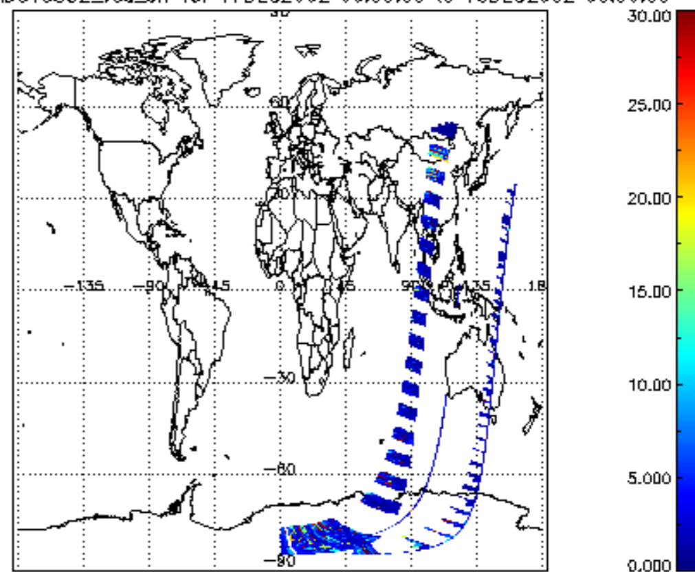
SCIOL2P_NADUV5SO2_vcd_err for 17DEC2002 00:00:00 to 18DEC2002 00:00:00
