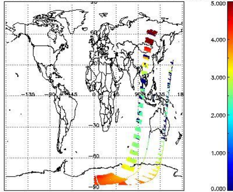
SCIOL2P_NADUV3BRO_amf_cl for 17DEC2002 00:00:00 to 18DEC2002 00:00:00
