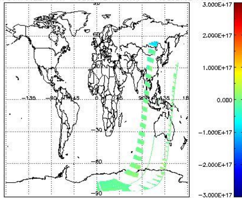
SCIOL2P_NADUV7S02_vcd for 17DEC2002 00:00:00 to 18DEC2002 00:00:00
