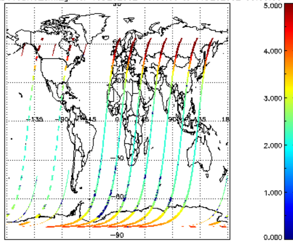
SCIOL2P_NADUV3BRO_amf_gr for 15DEC2002 00:00:00 to 16DEC2002 00:00:00
