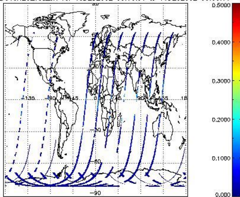
SCIOL2P_NADUV8H2O_vcd_err for 15DEC2002 00:00:00 to 16DEC2002 00:00:00
