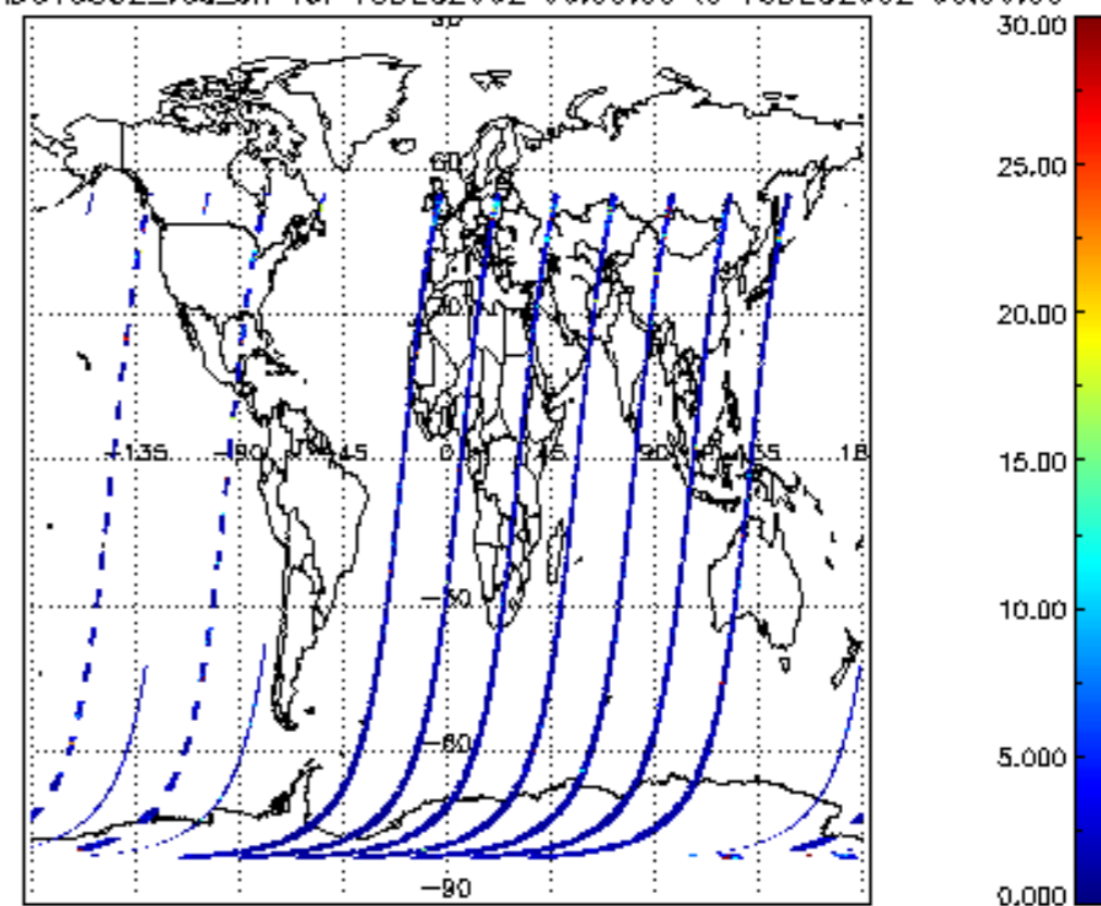
SCIOL2P_NADUV5S02_vcd_err for 15DEC2002 00:00:00 to 16DEC2002 00:00:00
