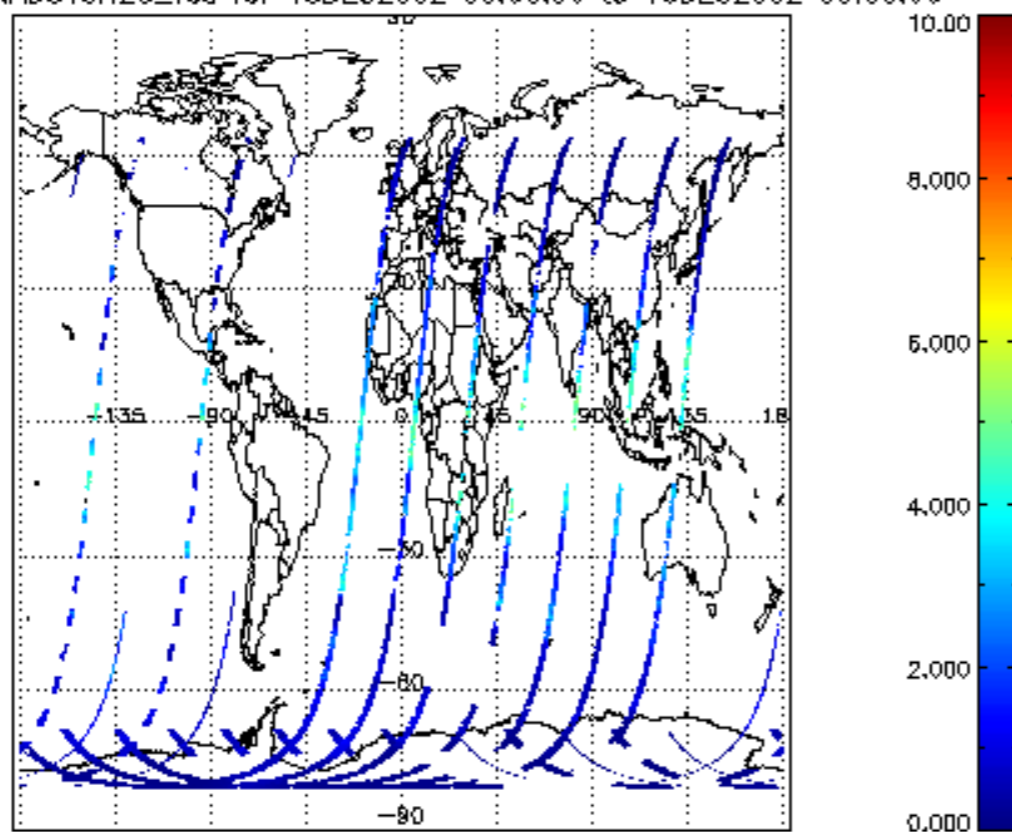
SCIOL2P_NADUV8H2O_vcd for 15DEC2002 00:00:00 to 16DEC2002 00:00:00
