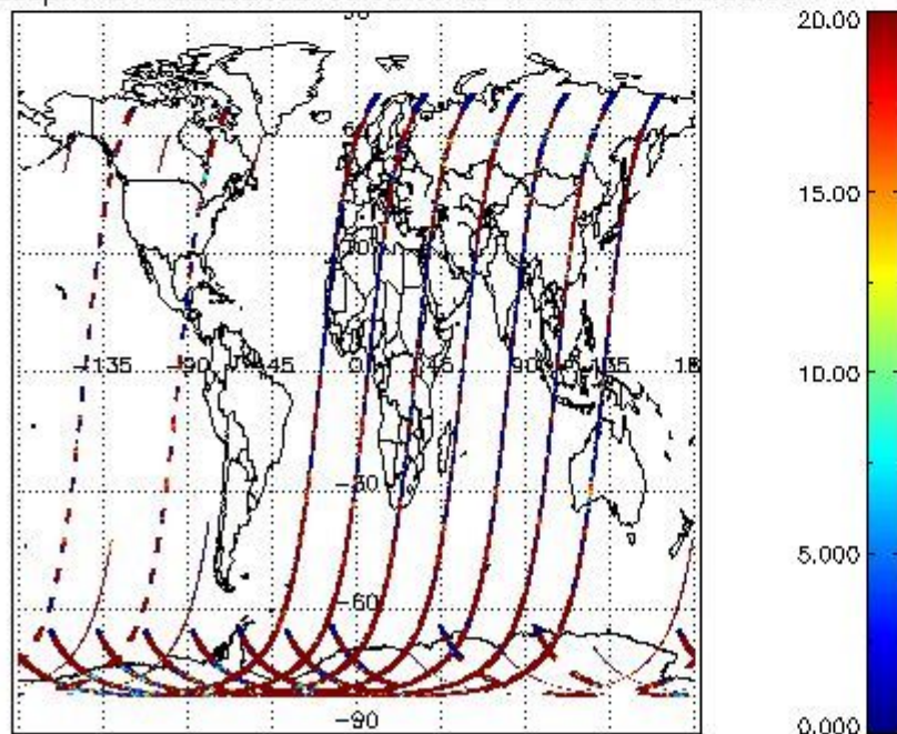
cL_opt_depth for 15DEC2002 00:00:00 to 16DEC2002 00:00:00
