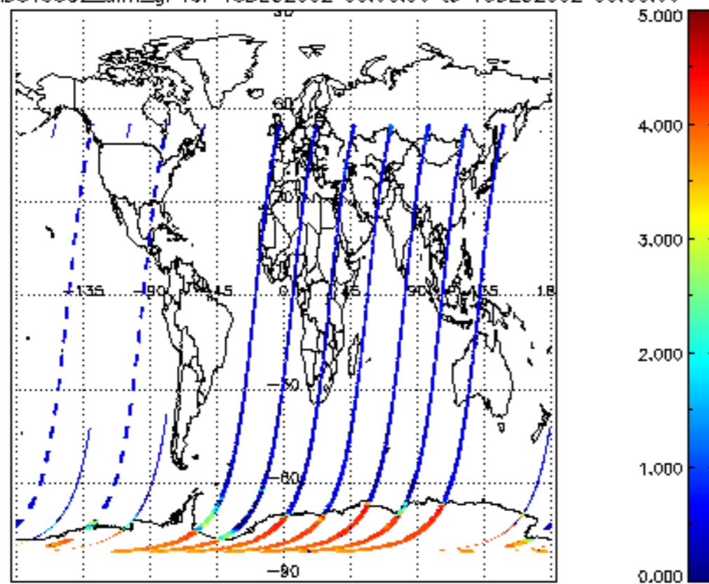
SCIOL2P_NADUV5S02_amf_gr for 15DEC2002 00:00:00 to 16DEC2002 00:00:00
