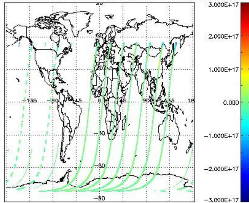
SCIOL2P_NADUV7S02_vcd for 15DEC2002 00:00:00 to 16DEC2002 00:00:00
