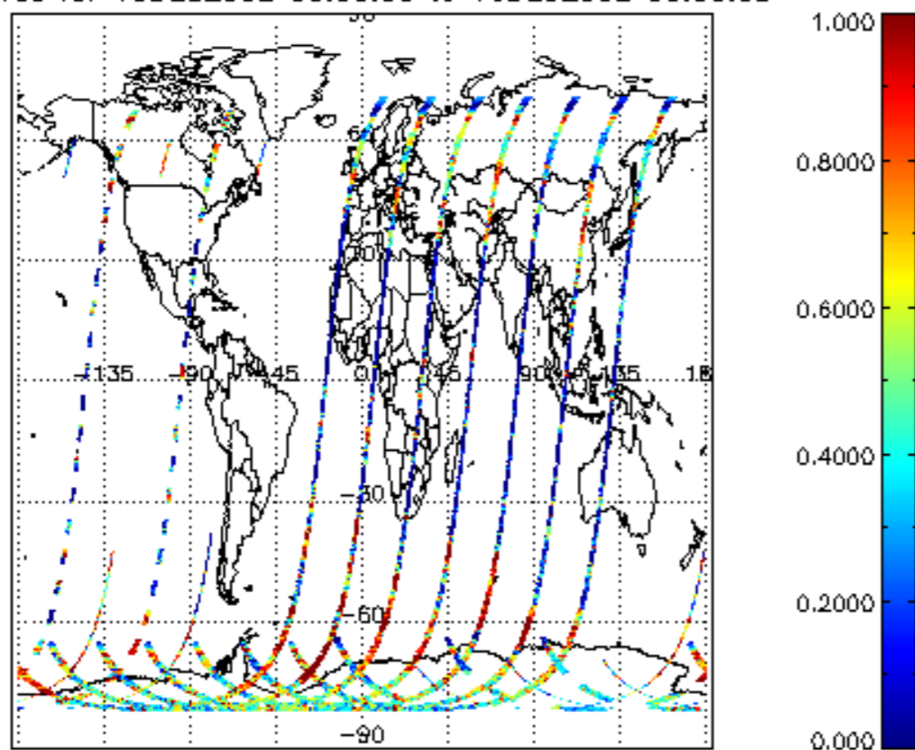
cL_frac for 15DEC2002 00:00:00 to 16DEC2002 00:00:00
