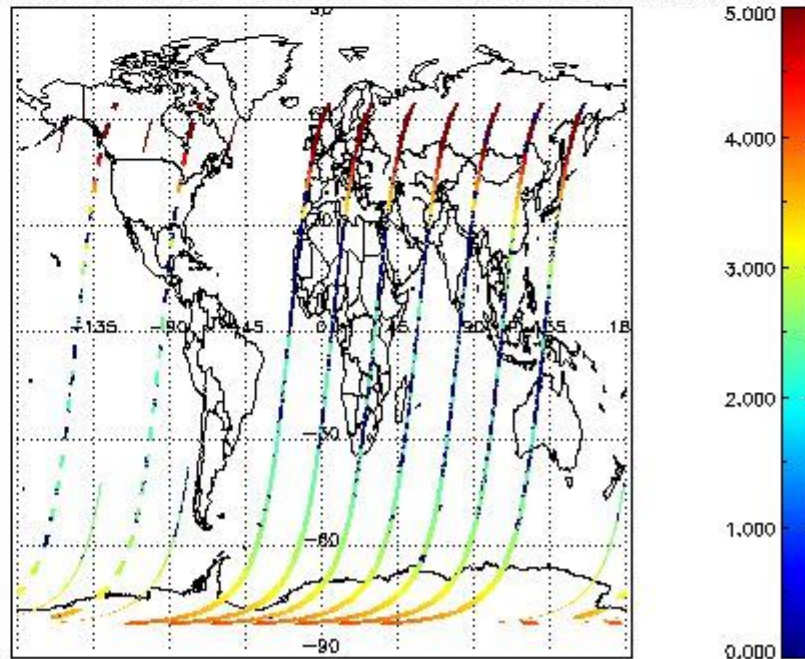
SCIOL2P_NADUV003_amf_cl for 15DEC2002 00:00:00 to 16DEC2002 00:00:00
