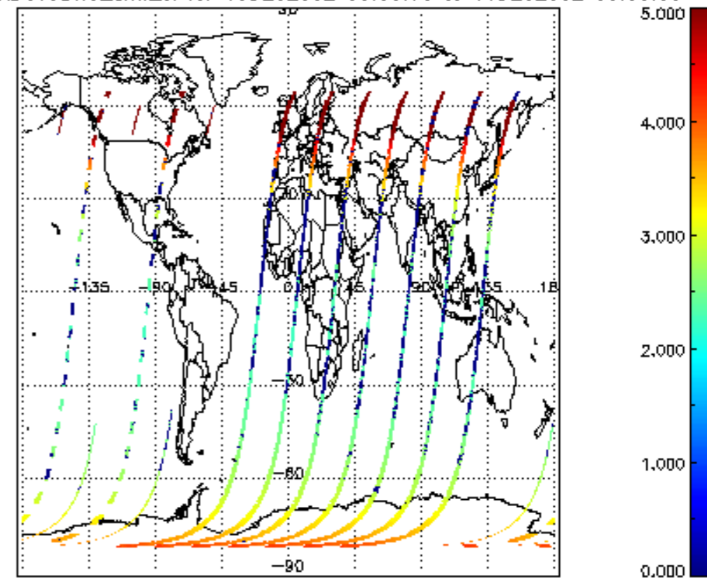
SCIOL2P_NADUV3BRO_amf_cl for 15DEC2002 00:00:00 to 16DEC2002 00:00:00
