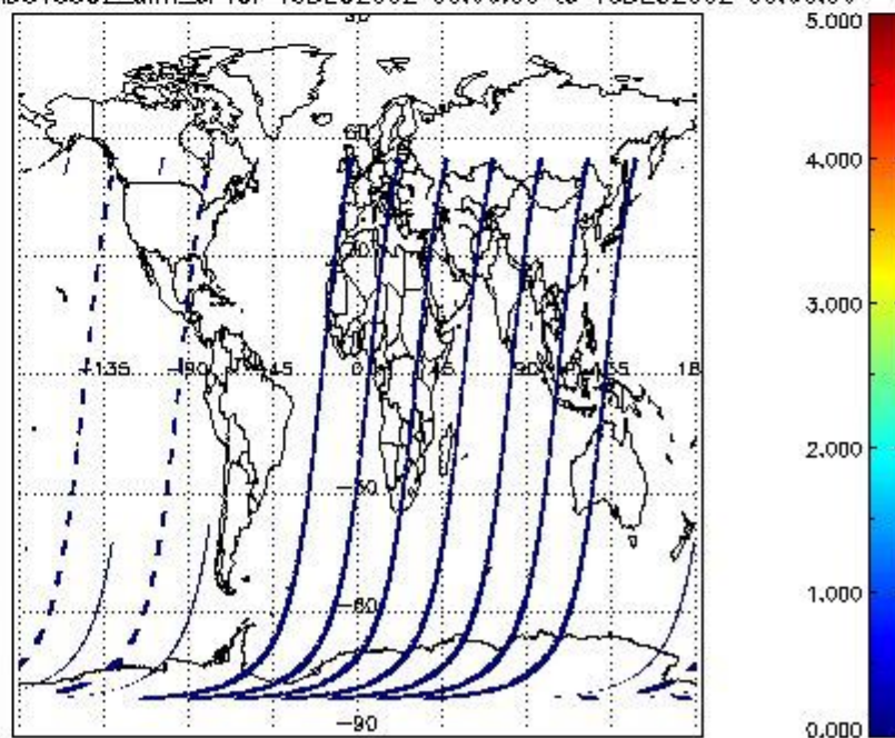
SCIOL2P_NADUV5S02_amf_cl for 15DEC2002 00:00:00 to 16DEC2002 00:00:00
