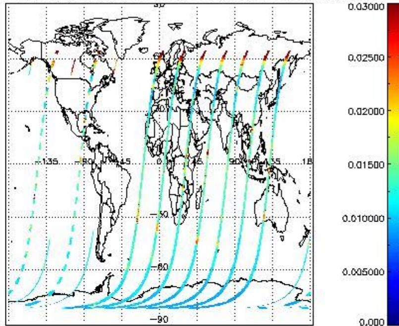
SCIOL2P_NADUV003_vcd_err for 15DEC2002 00:00:00 to 16DEC2002 00:00:00
