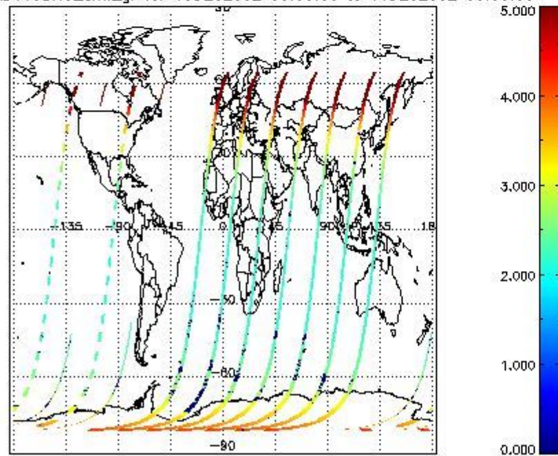
SCIOL2P_NADUV3BRO_amf_gr for 15DEC2002 00:00:00 to 16DEC2002 00:00:00
