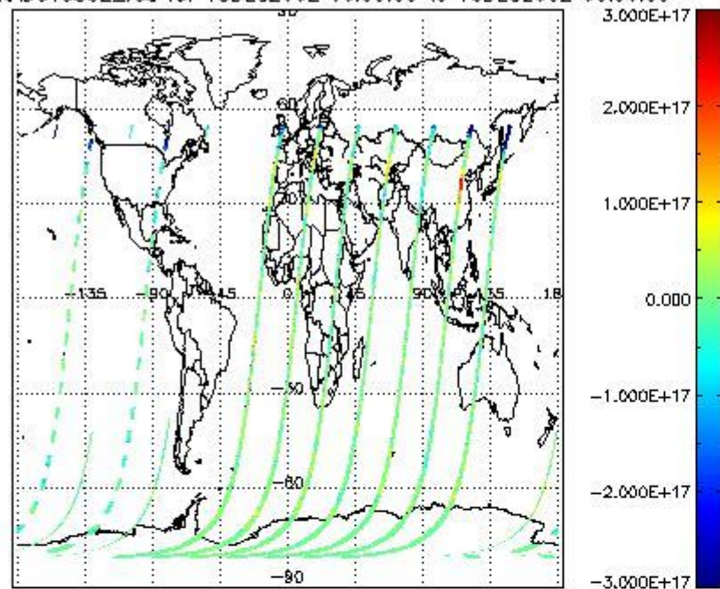
SCIOL2P_NADUV5S02_vcd for 15DEC2002 00:00:00 to 16DEC2002 00:00:00
