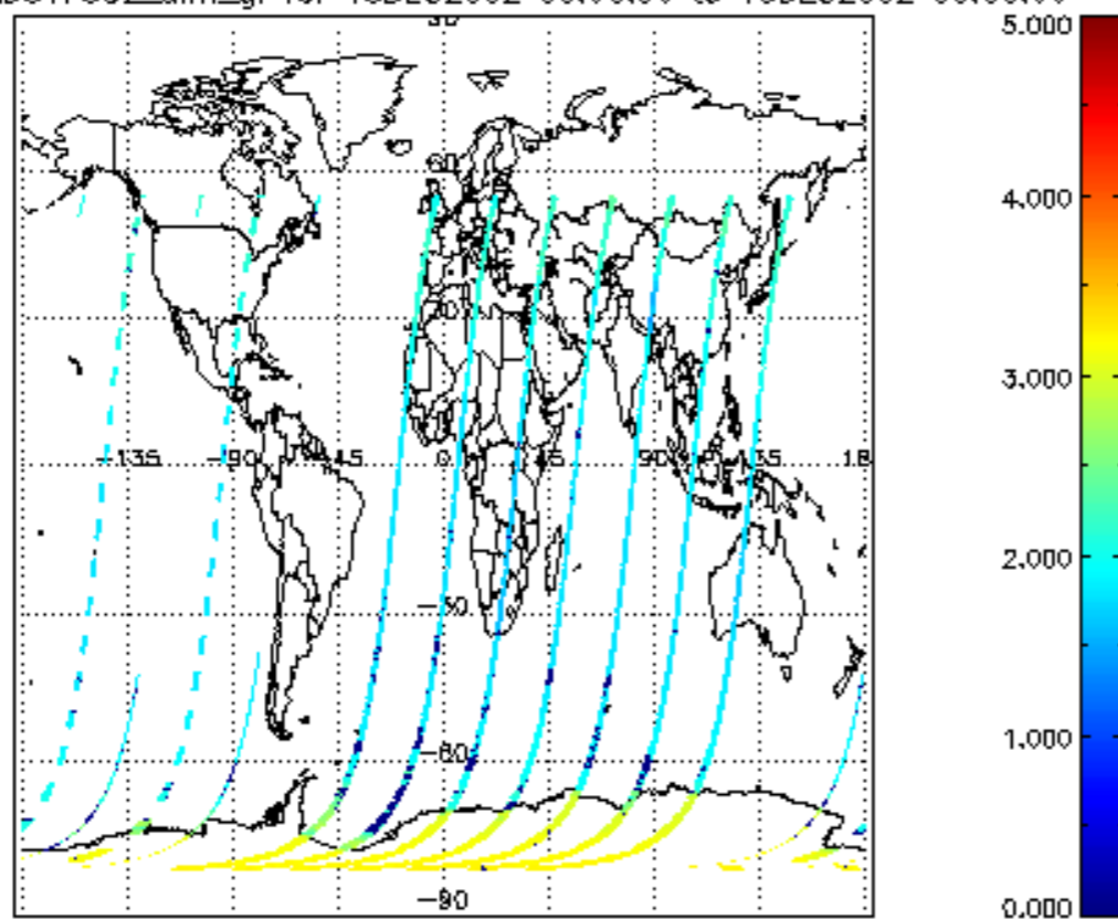
SCIOL2P_NADUV7S02_amf_gr for 15DEC2002 00:00:00 to 16DEC2002 00:00:00
