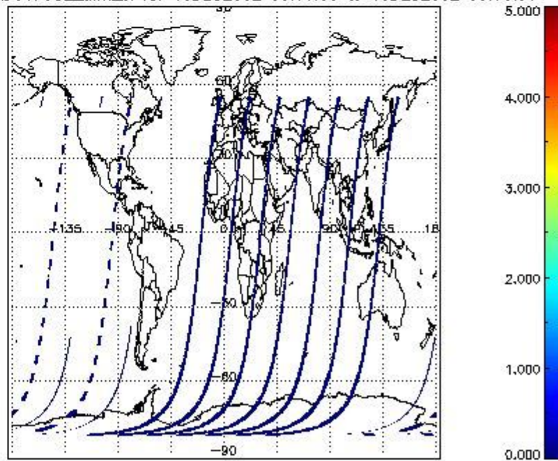
SCIOL2P_NADUV7S02_amf_cl for 15DEC2002 00:00:00 to 16DEC2002 00:00:00
