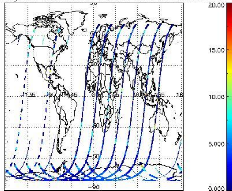
cL_top_height for 15DEC2002 00:00:00 to 16DEC2002 00:00:00
