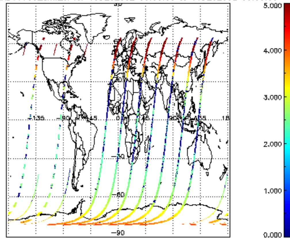
SCIOL2P_NADUV003_amf_cl for 15DEC2002 00:00:00 to 16DEC2002 00:00:00
