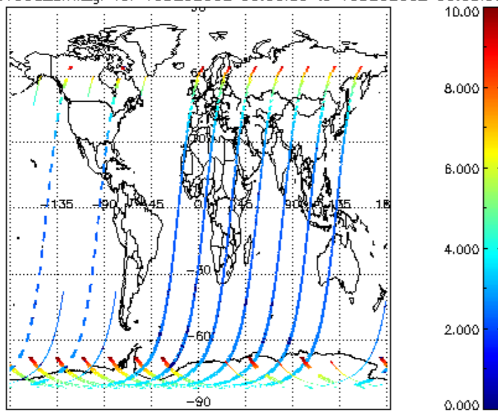
SCIOL2P_NADUV003_amf_gr for 15DEC2002 00:00:00 to 16DEC2002 00:00:00
