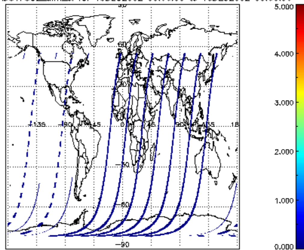
SCIOL2P_NADUV7S02_amf_cl for 15DEC2002 00:00:00 to 16DEC2002 00:00:00
