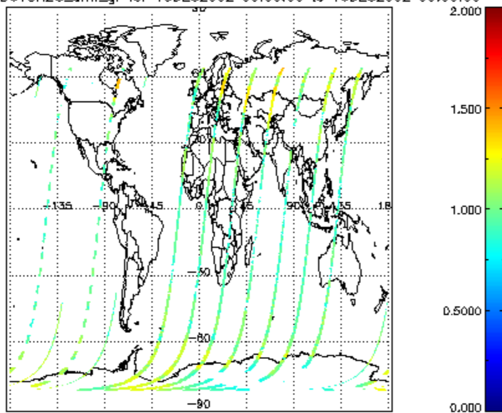
SCIOL2P_NADUV8H2O_amf_gr for 15DEC2002 00:00:00 to 16DEC2002 00:00:00
