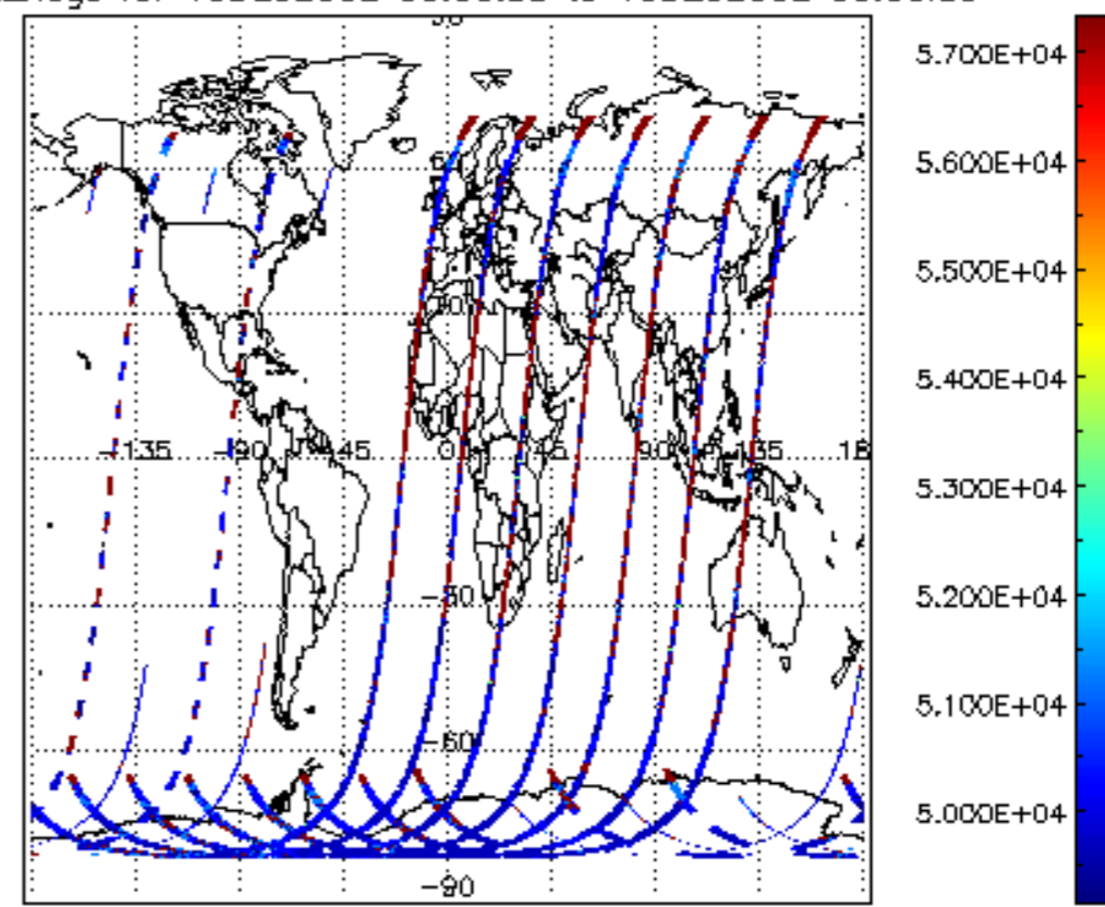
cloud_flags for 15DEC2002 00:00:00 to 16DEC2002 00:00:00
