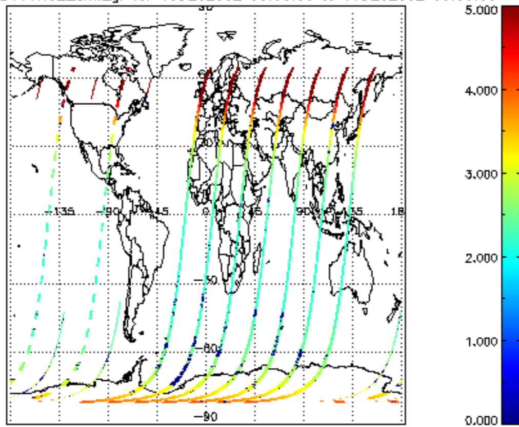
SCIOL2P_NADUV1N02_amf_gr for 15DEC2002 00:00:00 to 16DEC2002 00:00:00
