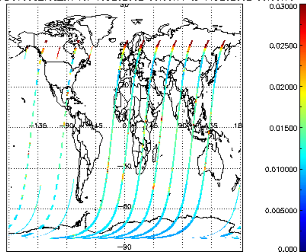
SCIOL2P_NADUV003_vcd_err for 15DEC2002 00:00:00 to 16DEC2002 00:00:00
