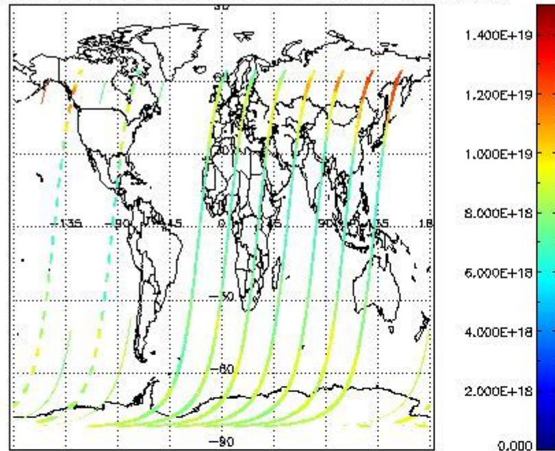
SCIOL2P_NADUV003_vcd for 15DEC2002 00:00:00 to 16DEC2002 00:00:00
