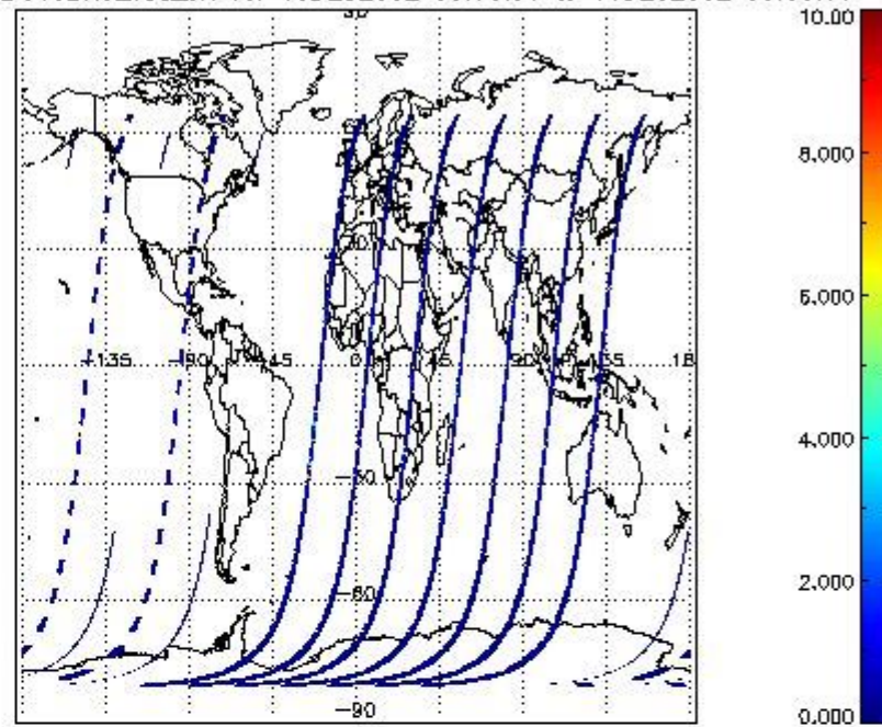
SCIOL2P_NADUV3BRO_vcd_err for 15DEC2002 00:00:00 to 16DEC2002 00:00:00
