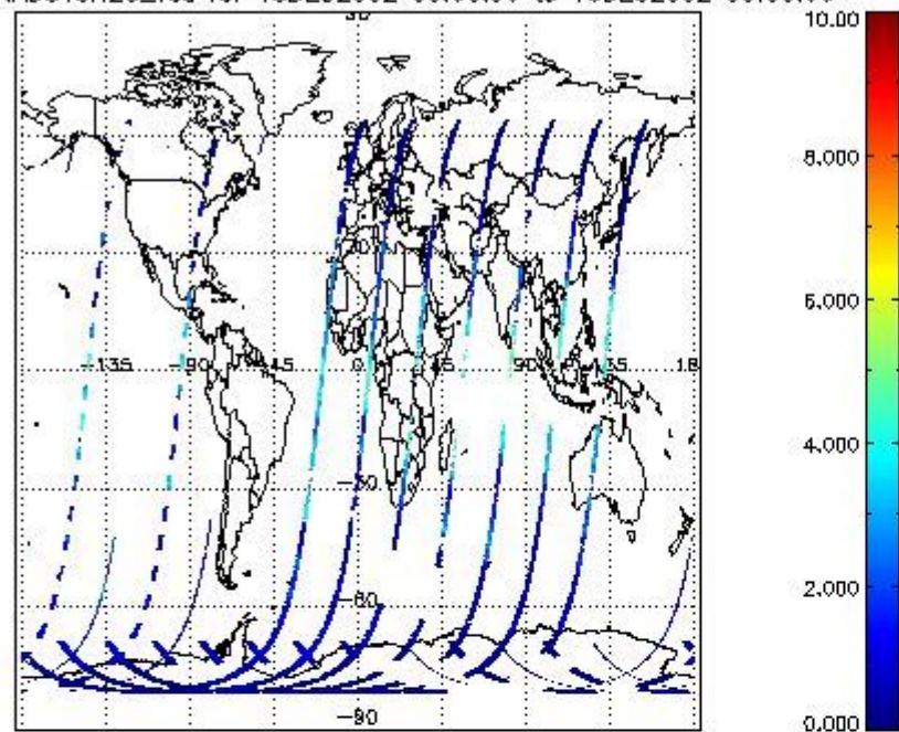
SCIOL2P_NADUV8H2O_vcd for 15DEC2002 00:00:00 to 16DEC2002 00:00:00
