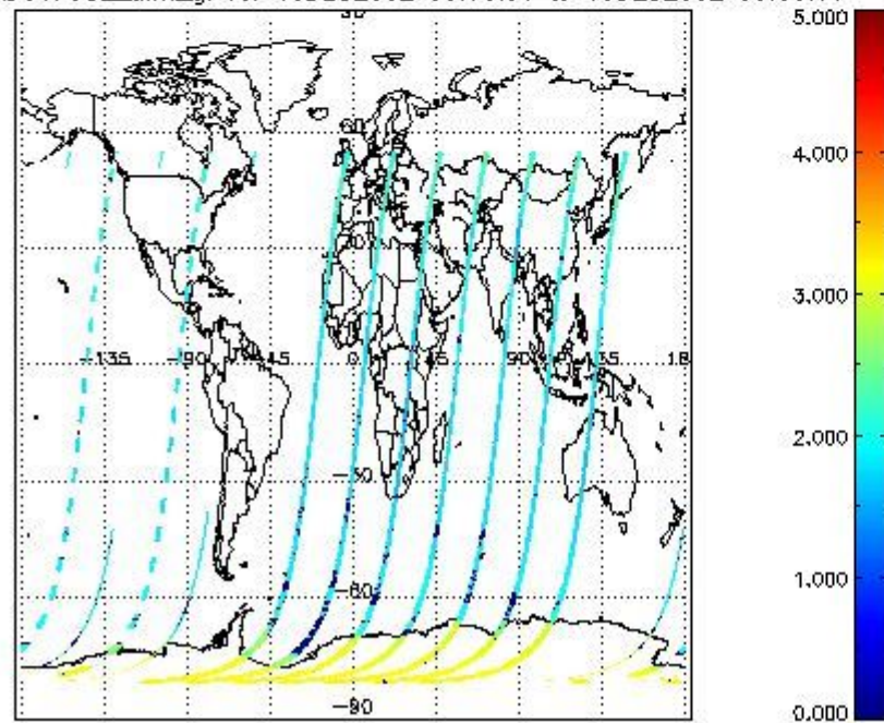
SCIOL2P_NADUV7S02_amf_gr for 15DEC2002 00:00:00 to 16DEC2002 00:00:00
