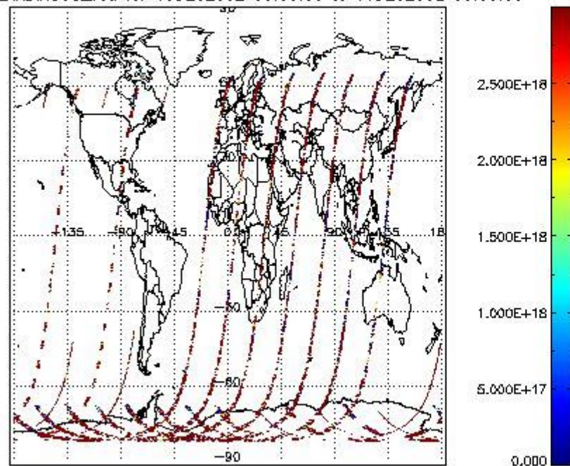
SCIDL2P_NADIR3CO_vcd for 15DEC2002 00:00:00 to 16DEC2002 00:00:00
