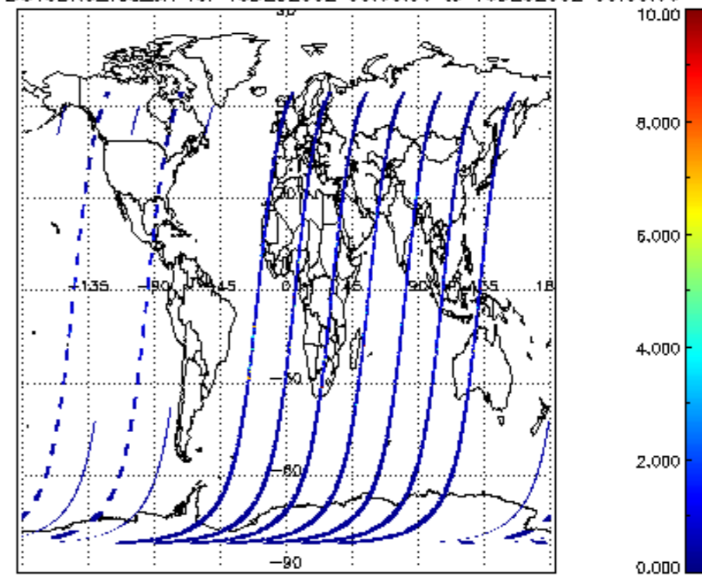
SCIOL2P_NADUV3BRO_vcd_err for 15DEC2002 00:00:00 to 16DEC2002 00:00:00
