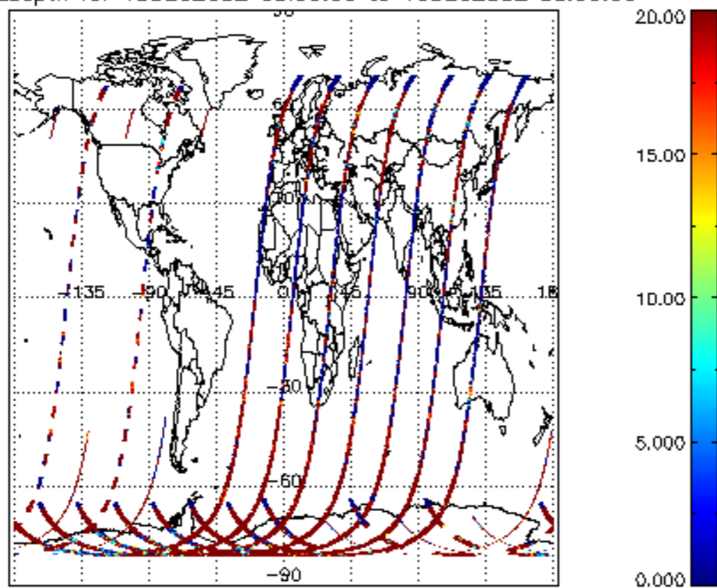
cL_opt_depth for 15DEC2002 00:00:00 to 16DEC2002 00:00:00
