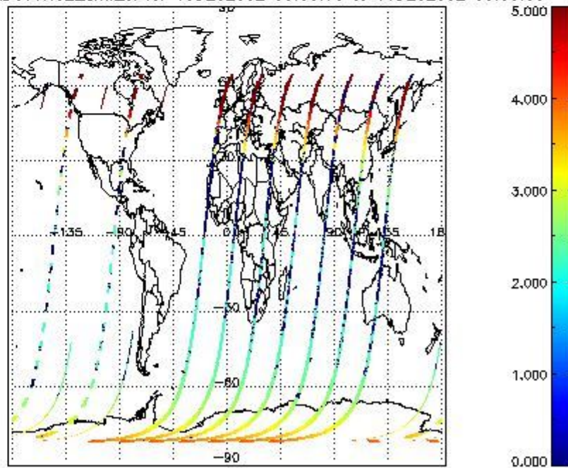
SCIOL2P_NADUV1N02_amf_cl for 15DEC2002 00:00:00 to 16DEC2002 00:00:00
