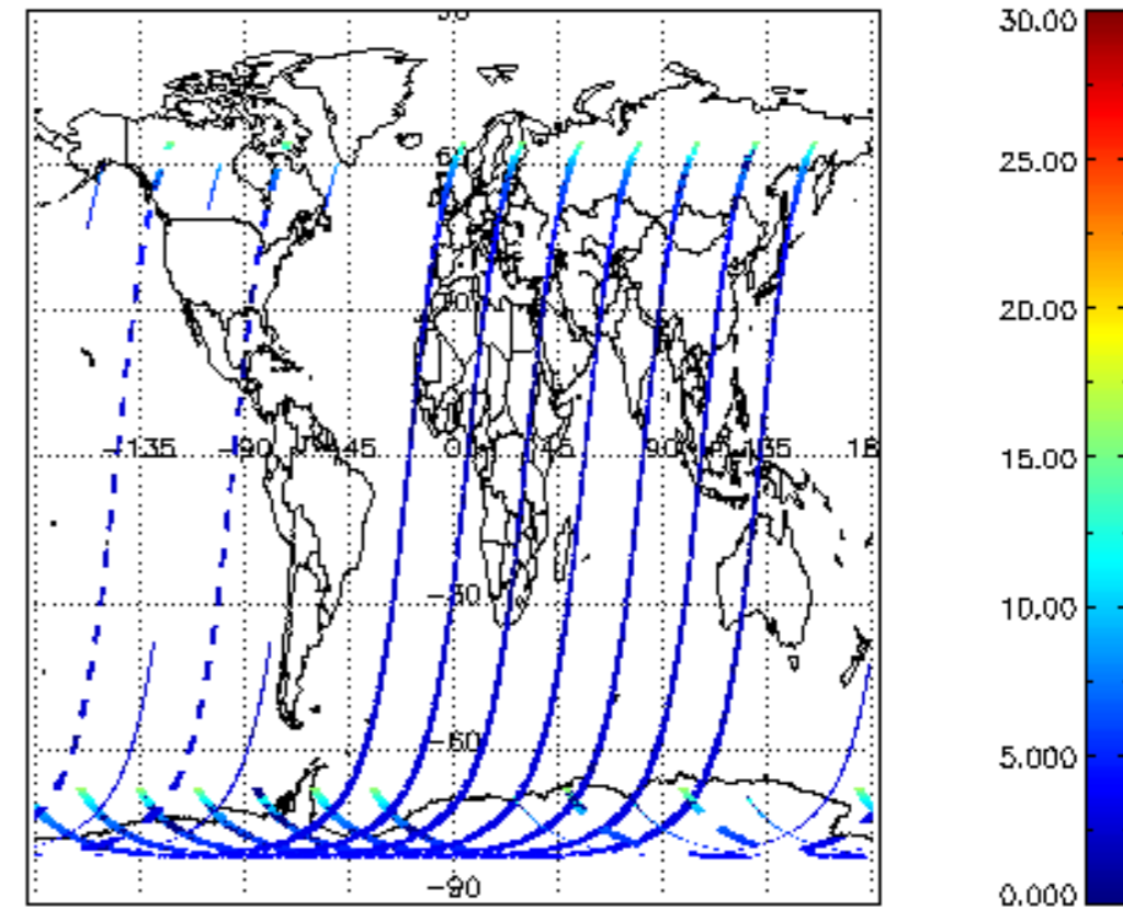
SCIOL2P_NADUV1NO2_amf_cl for 15DEC2002 00:00:00 to 16DEC2002 00:00:00
