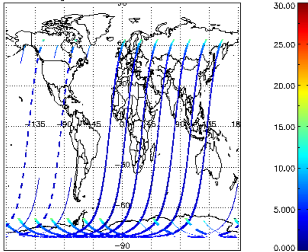
SCIOL2P_NADUV1NO2_amf_gr for 15DEC2002 00:00:00 to 16DEC2002 00:00:00
