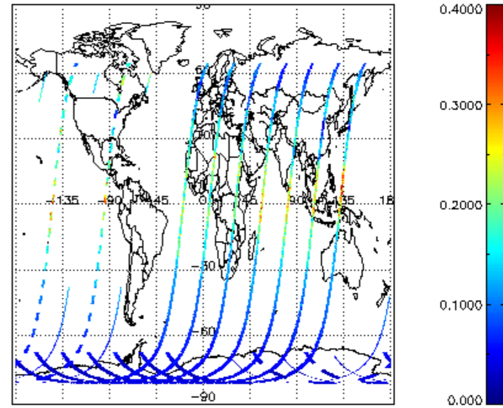
SCIOL2P_NADUV1NO2_vcd_err for 15DEC2002 00:00:00 to 16DEC2002 00:00:00
