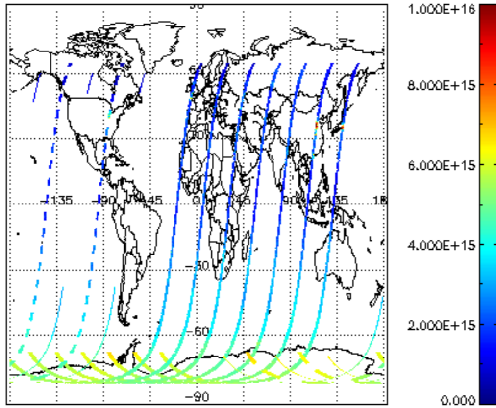
SCIOL2P_NADUV1NO2_vcd for 15DEC2002 00:00:00 to 16DEC2002 00:00:00
