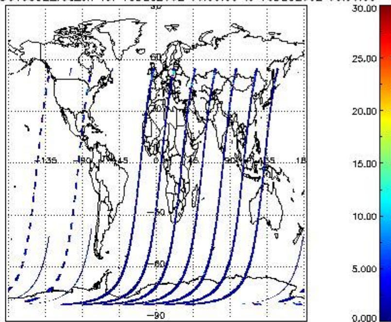
SCIOL2P_NADUV5S02_vcd_err for 15DEC2002 00:00:00 to 16DEC2002 00:00:00
