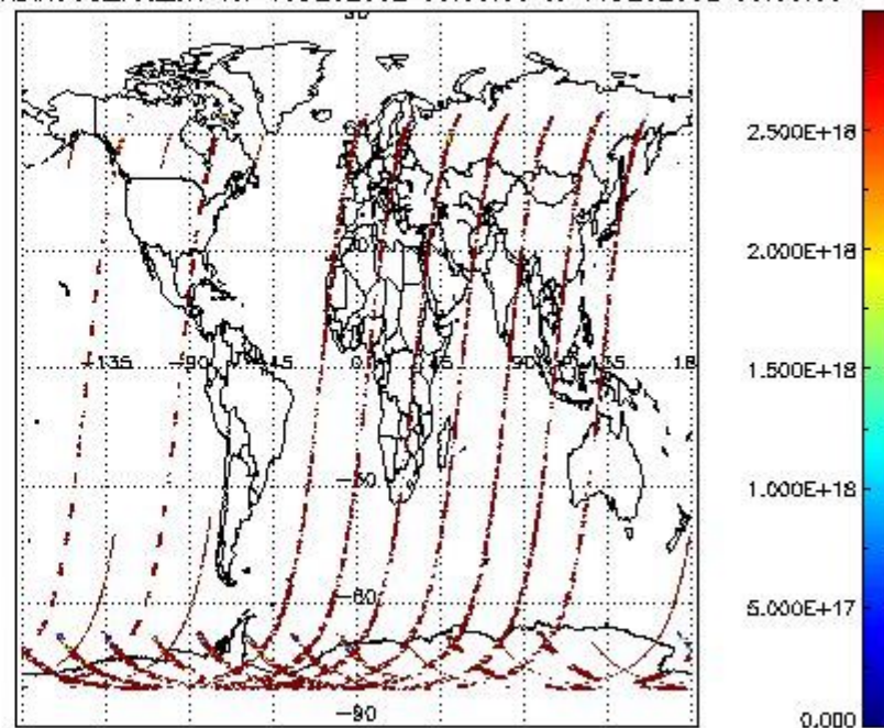
SCIDL2P_NADIR3CO_vcd_err for 15DEC2002 00:00:00 to 16DEC2002 00:00:00
