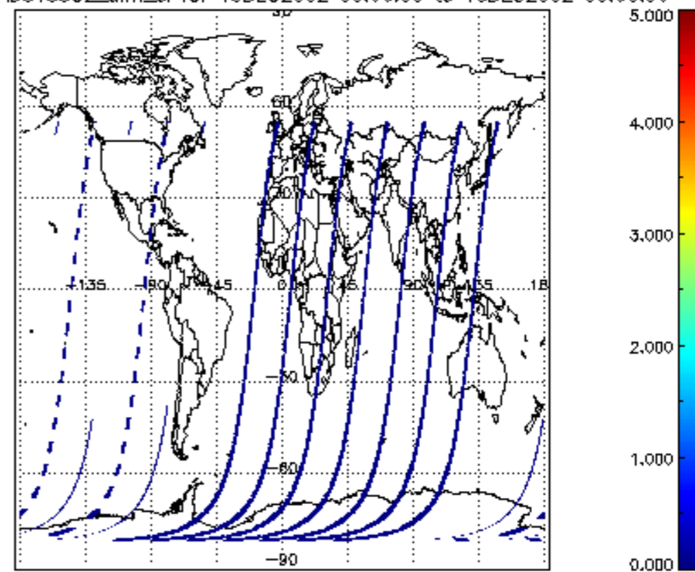
SCIOL2P_NADUV5S02_amf_cl for 15DEC2002 00:00:00 to 16DEC2002 00:00:00
