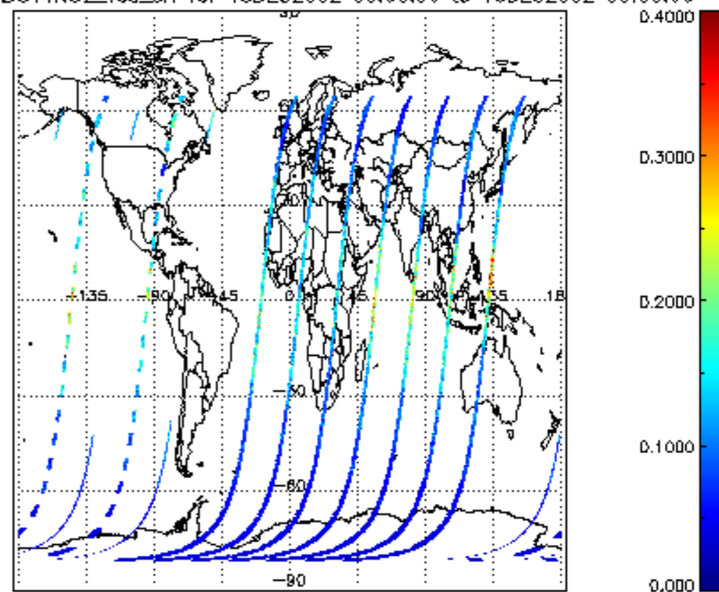
SCIOL2P_NADUV1N02_vcd_err for 15DEC2002 00:00:00 to 16DEC2002 00:00:00
