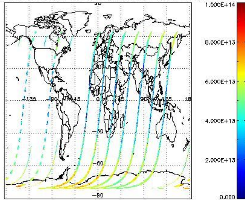
SCIOL2P_NADUV3BRO_vcd for 15DEC2002 00:00:00 to 16DEC2002 00:00:00
