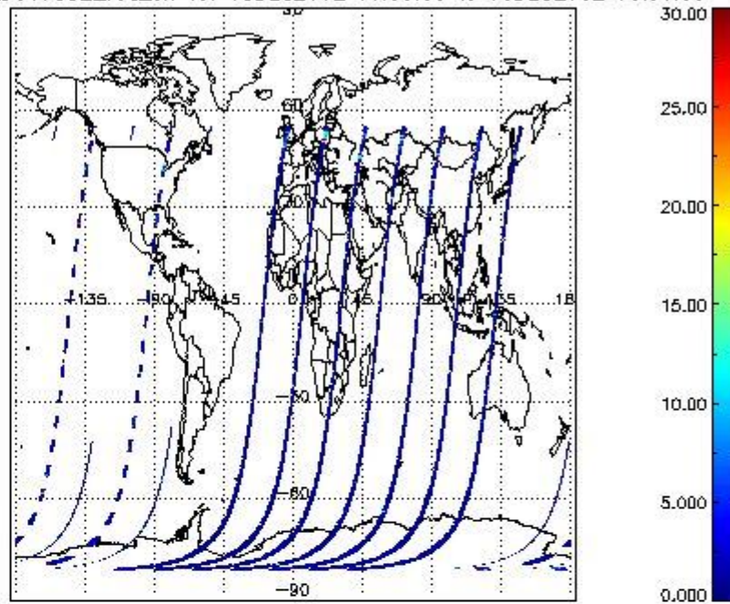
SCIOL2P_NADUV7S02_vcd_err for 15DEC2002 00:00:00 to 16DEC2002 00:00:00
