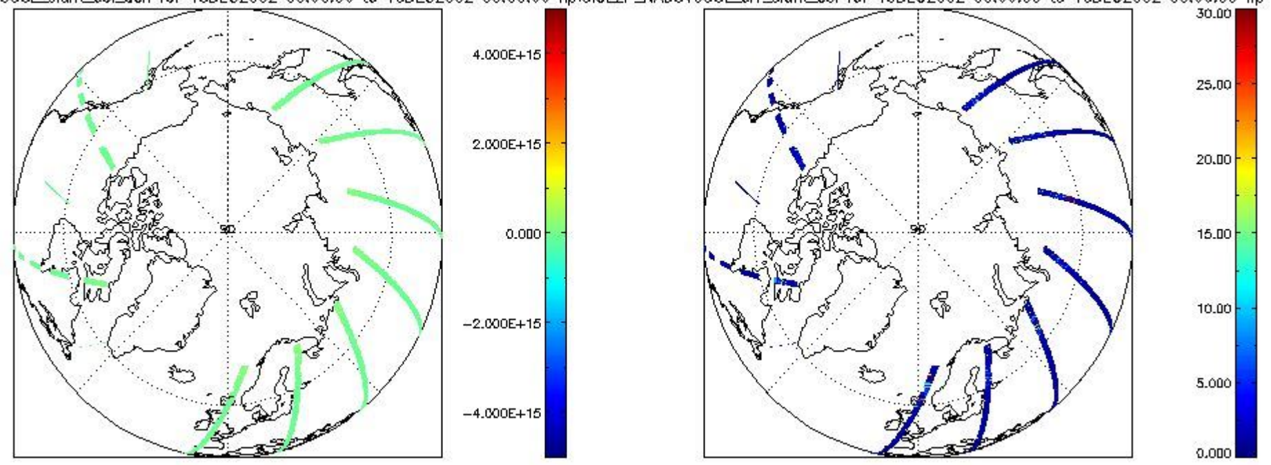
CIOL2P_NADUV60CL_slant_col_den for 15DEC2002 00:00:00 to 16DEC2002 00:00:00 np; CIOL2P_NADUV60CL_err_slant_col for 15DEC2002 00:00:00 to 16DEC2002 00:00:00 np
