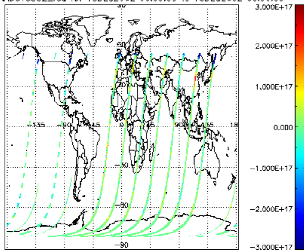
SCIOL2P_NADUV5S02_vcd for 15DEC2002 00:00:00 to 16DEC2002 00:00:00
