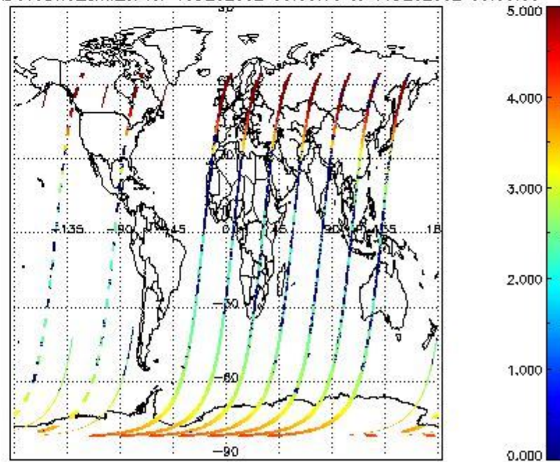
SCIOL2P_NADUV3BRO_amf_cl for 15DEC2002 00:00:00 to 16DEC2002 00:00:00
