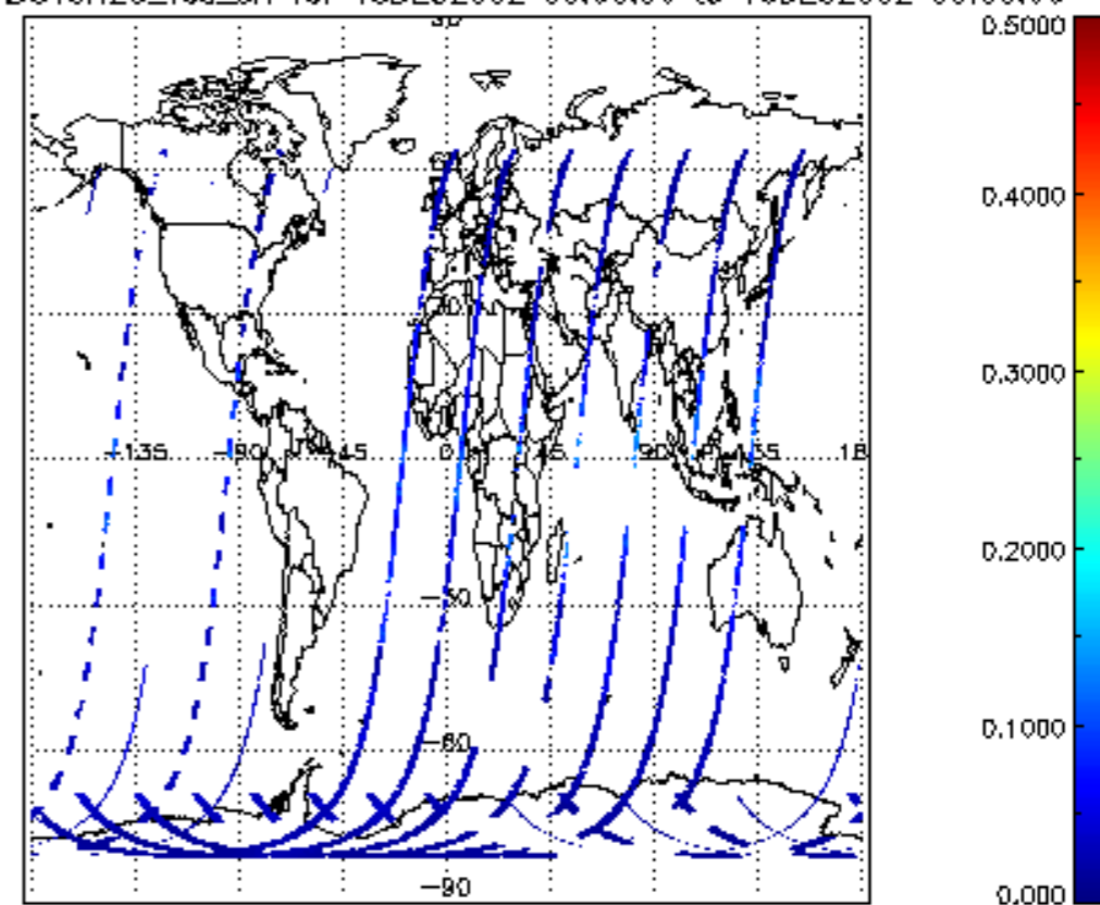
SCIOL2P_NADUV8H2O_vcd_err for 15DEC2002 00:00:00 to 16DEC2002 00:00:00
