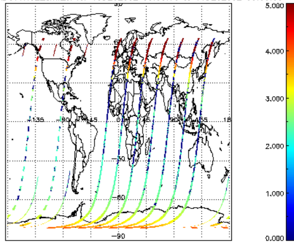
SCIOL2P_NADUV1N02_amf_cl for 15DEC2002 00:00:00 to 16DEC2002 00:00:00
