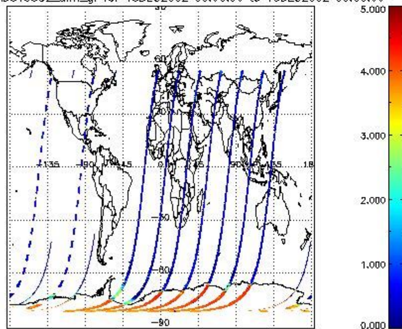
SCIOL2P_NADUV5S02_amf_gr for 15DEC2002 00:00:00 to 16DEC2002 00:00:00
