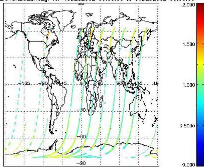
SCIOL2P_NADUV8H2O_amf_gr for 15DEC2002 00:00:00 to 16DEC2002 00:00:00
