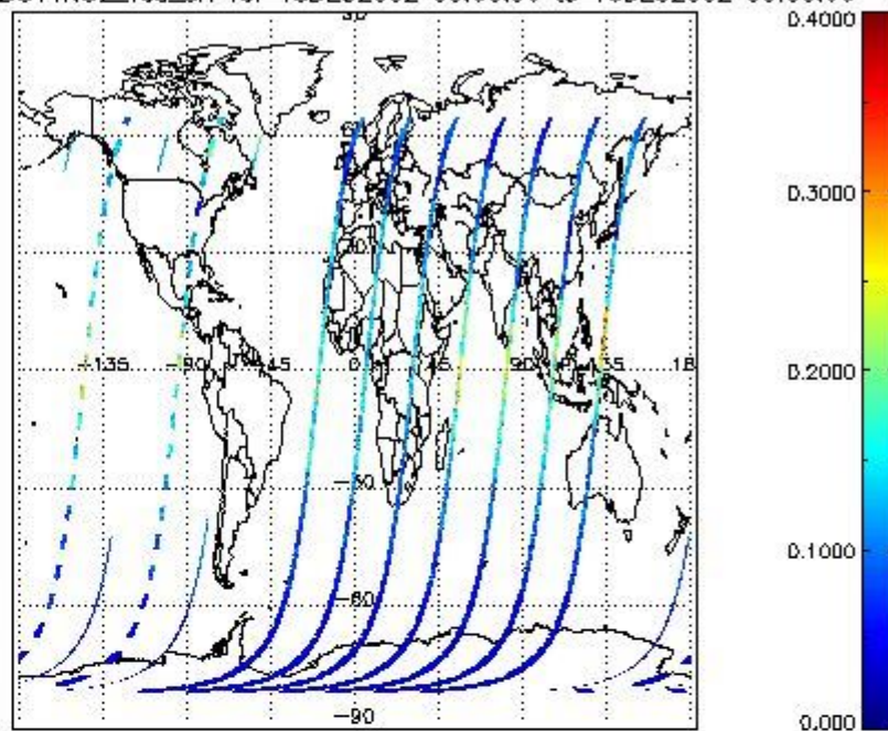
SCIOL2P_NADUV1N02_vcd_err for 15DEC2002 00:00:00 to 16DEC2002 00:00:00
