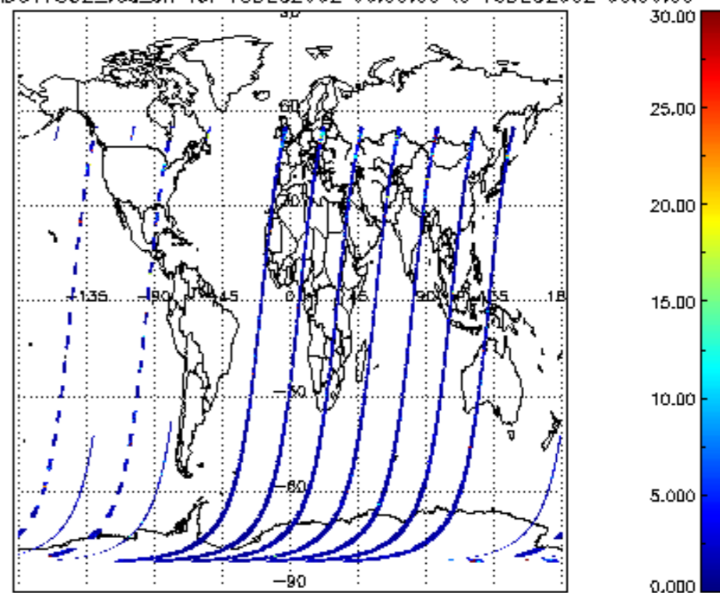
SCIOL2P_NADUV7S02_vcd_err for 15DEC2002 00:00:00 to 16DEC2002 00:00:00
