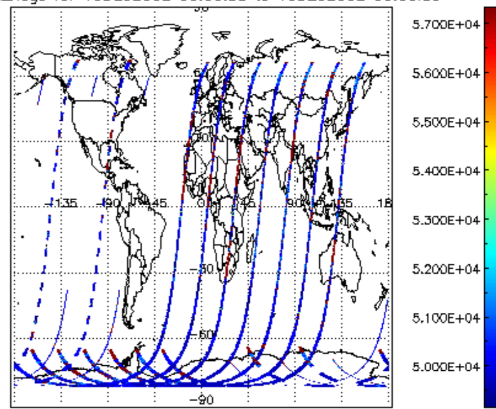
cloud_flags for 15DEC2002 00:00:00 to 16DEC2002 00:00:00
