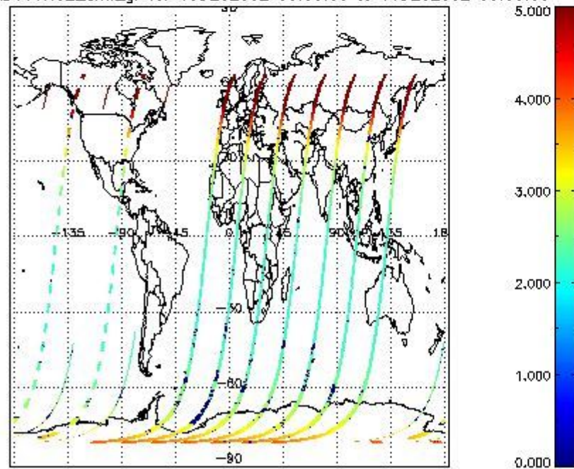
SCIOL2P_NADUV1N02_amf_gr for 15DEC2002 00:00:00 to 16DEC2002 00:00:00
