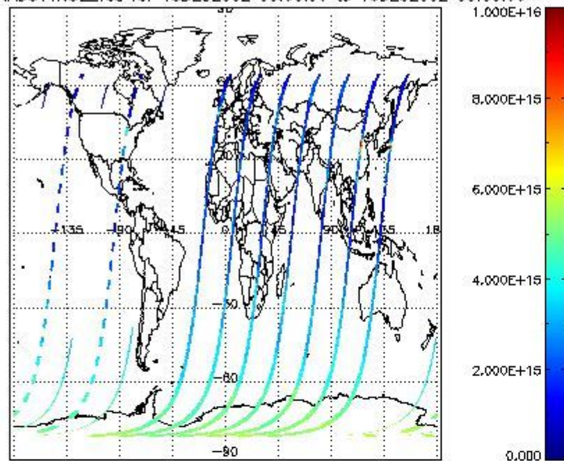
SCIOL2P_NADUV1N02_vcd for 15DEC2002 00:00:00 to 16DEC2002 00:00:00
