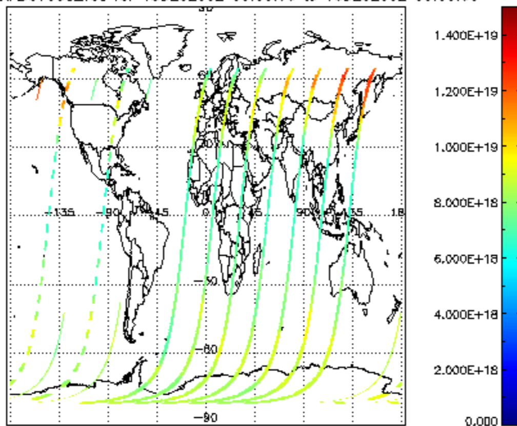
SCIOL2P_NADUV003_vcd for 15DEC2002 00:00:00 to 16DEC2002 00:00:00
