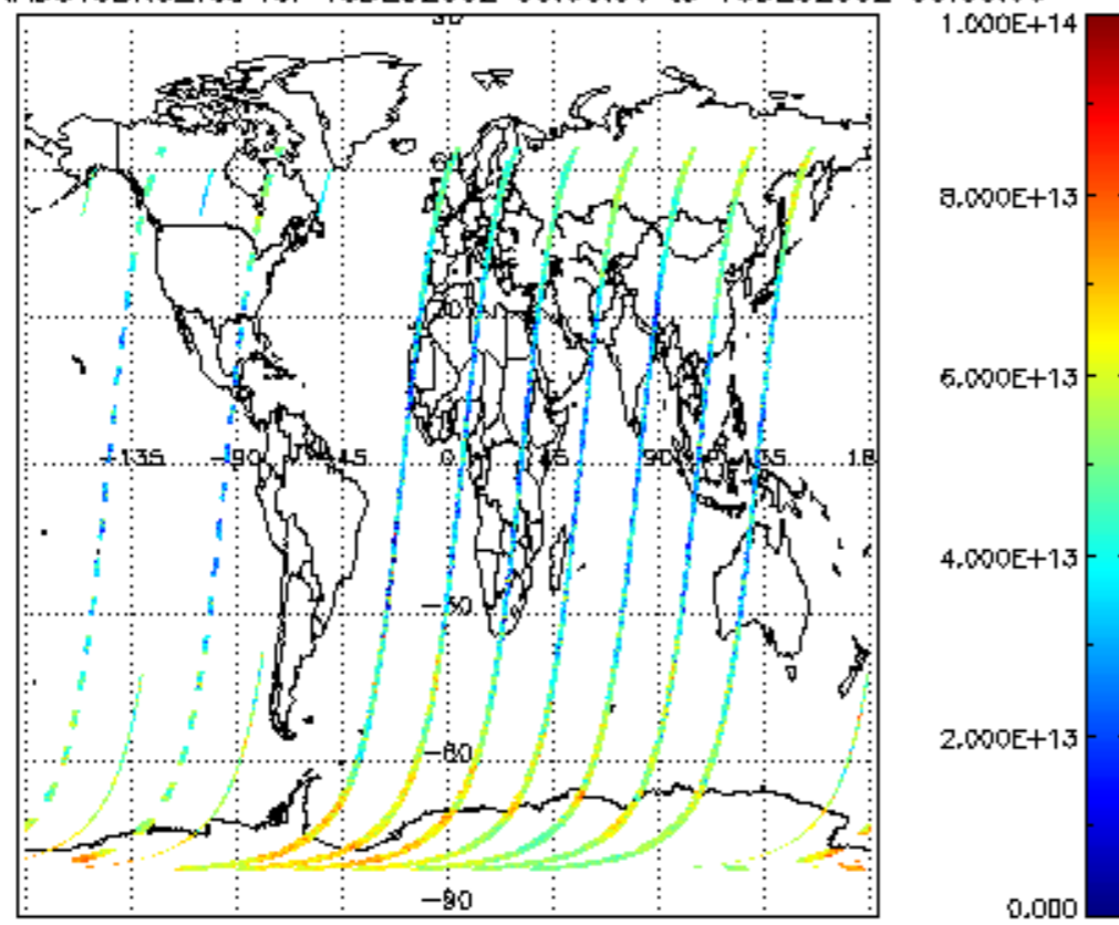
SCIOL2P_NADUV3BRO_vcd for 15DEC2002 00:00:00 to 16DEC2002 00:00:00
