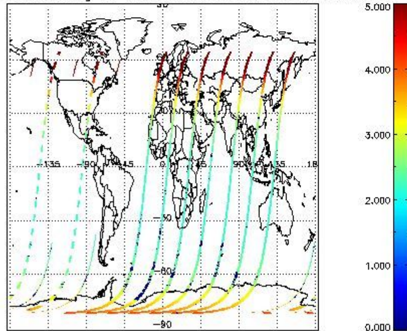
SCIOL2P_NADUV003_amf_gr for 15DEC2002 00:00:00 to 16DEC2002 00:00:00
