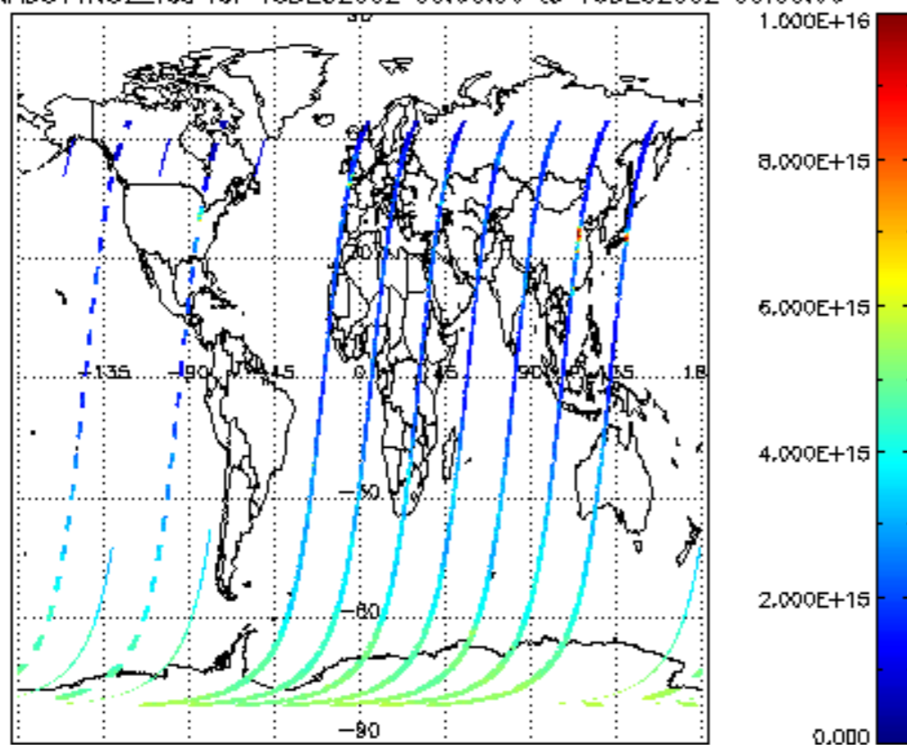
SCIOL2P_NADUV1N02_vcd for 15DEC2002 00:00:00 to 16DEC2002 00:00:00
