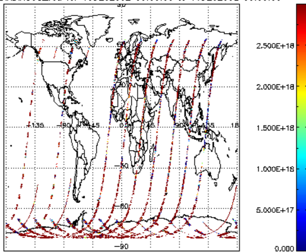
SCIOL2P_NADIR3CO_vcd for 15DEC2002 00:00:00 to 16DEC2002 00:00:00
