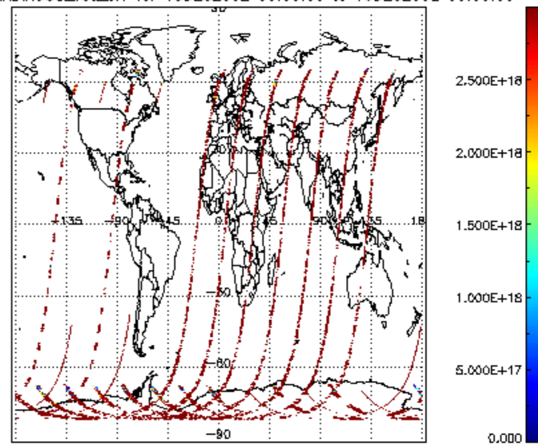
SCIOL2P_NADIR3CO_vcd_Lerr for 15DEC2002 00:00:00 to 16DEC2002 00:00:00
