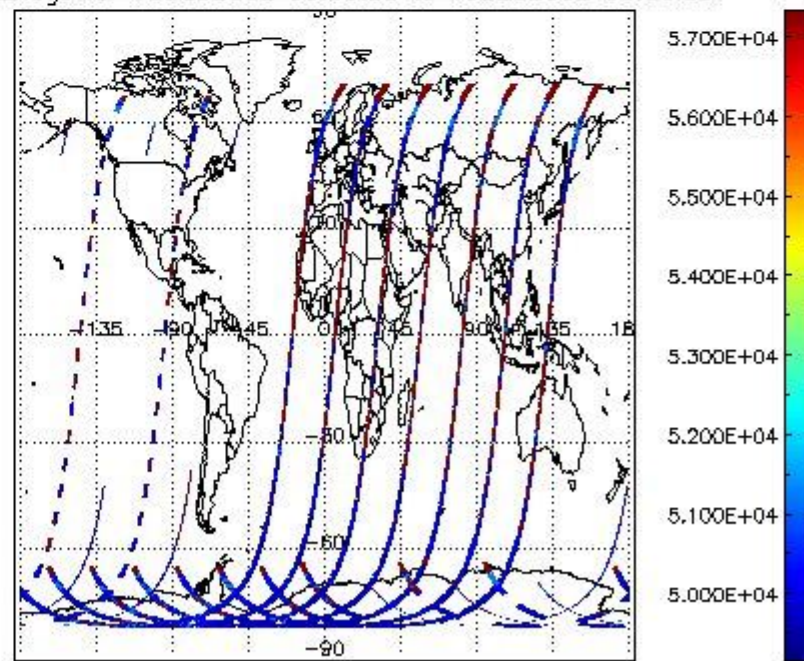
cloud_flags for 15DEC2002 00:00:00 to 16DEC2002 00:00:00
