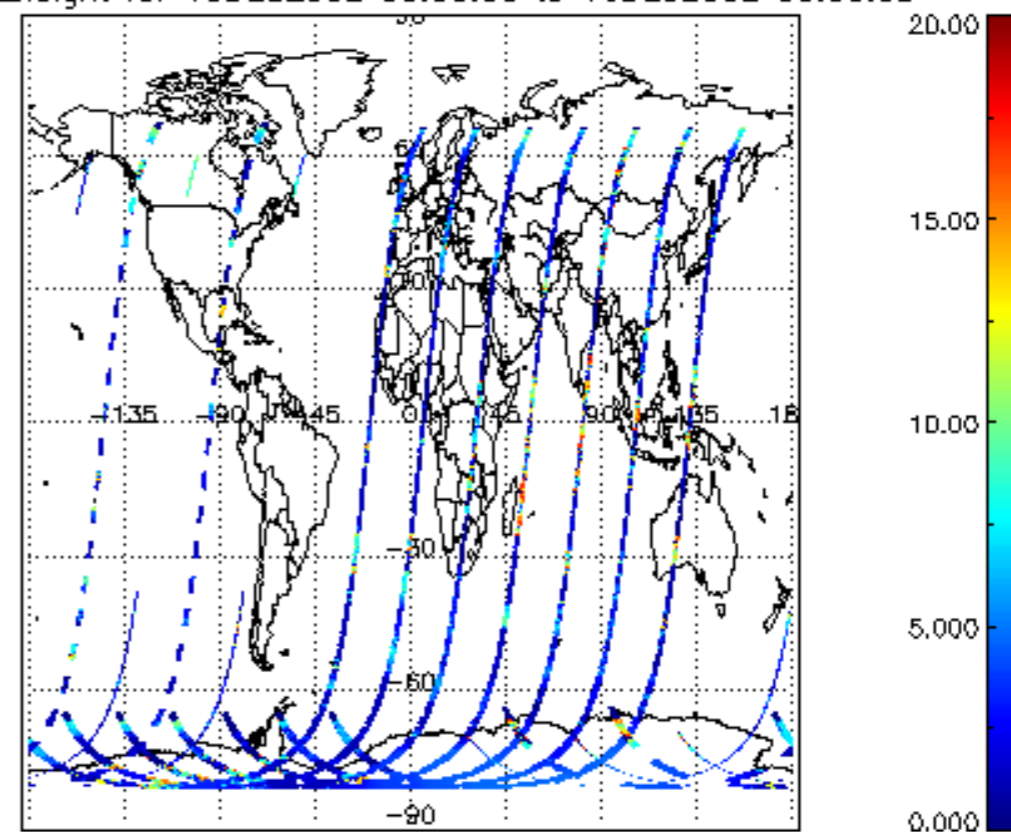
cL_top_height for 15DEC2002 00:00:00 to 16DEC2002 00:00:00
