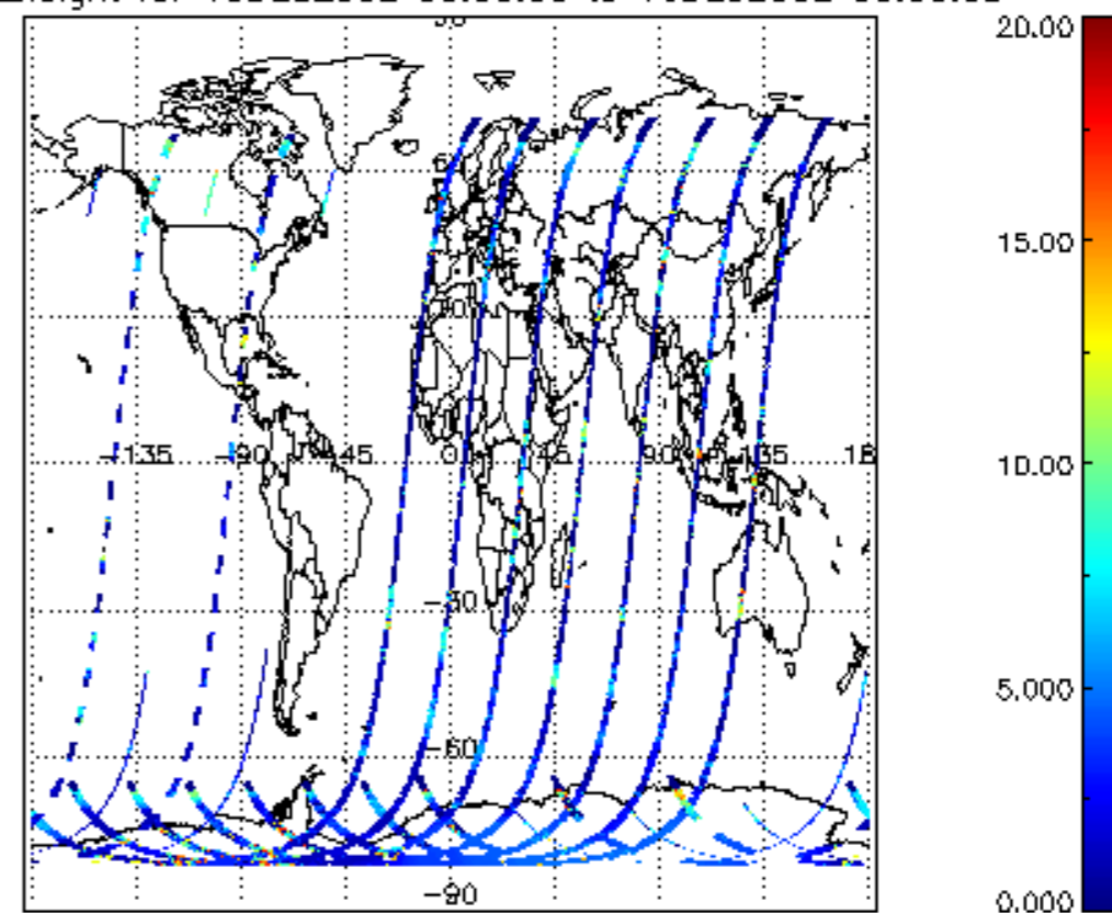
cL_top_height for 15DEC2002 00:00:00 to 16DEC2002 00:00:00
