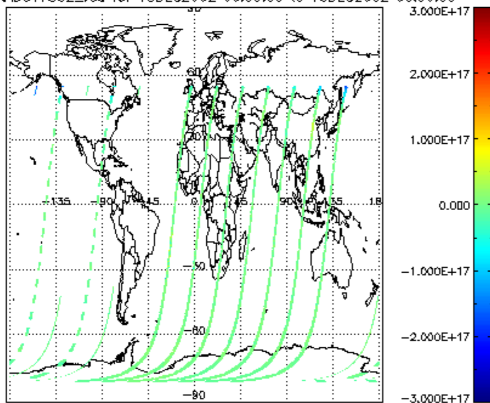
SCIOL2P_NADUV7S02_vcd for 15DEC2002 00:00:00 to 16DEC2002 00:00:00
