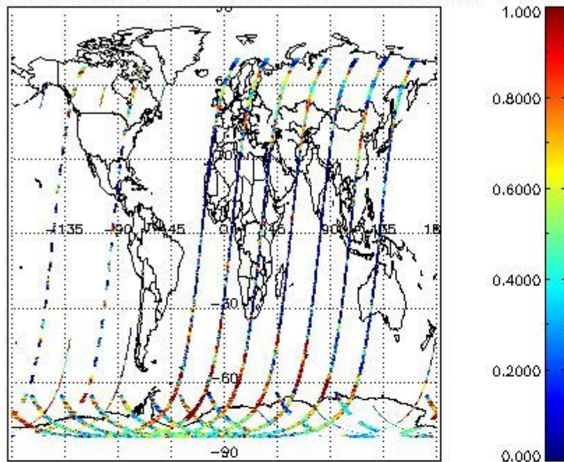
cL_frac for 15DEC2002 00:00:00 to 16DEC2002 00:00:00
