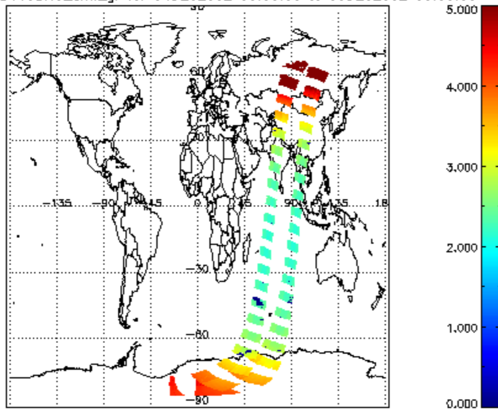
SCIOL2P_NADUV3BRO_amf_gr for 04DEC2002 00:00:00 to 05DEC2002 00:00:00
