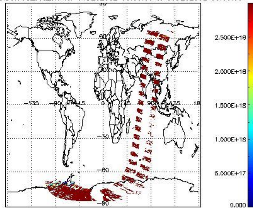
SCIDL2P_NADIR3CO_vcd_err for 04DEC2002 00:00:00 to 05DEC2002 00:00:00
