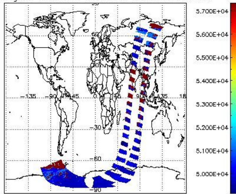
cloud_flags for 04DEC2002 00:00:00 to 05DEC2002 00:00:00
