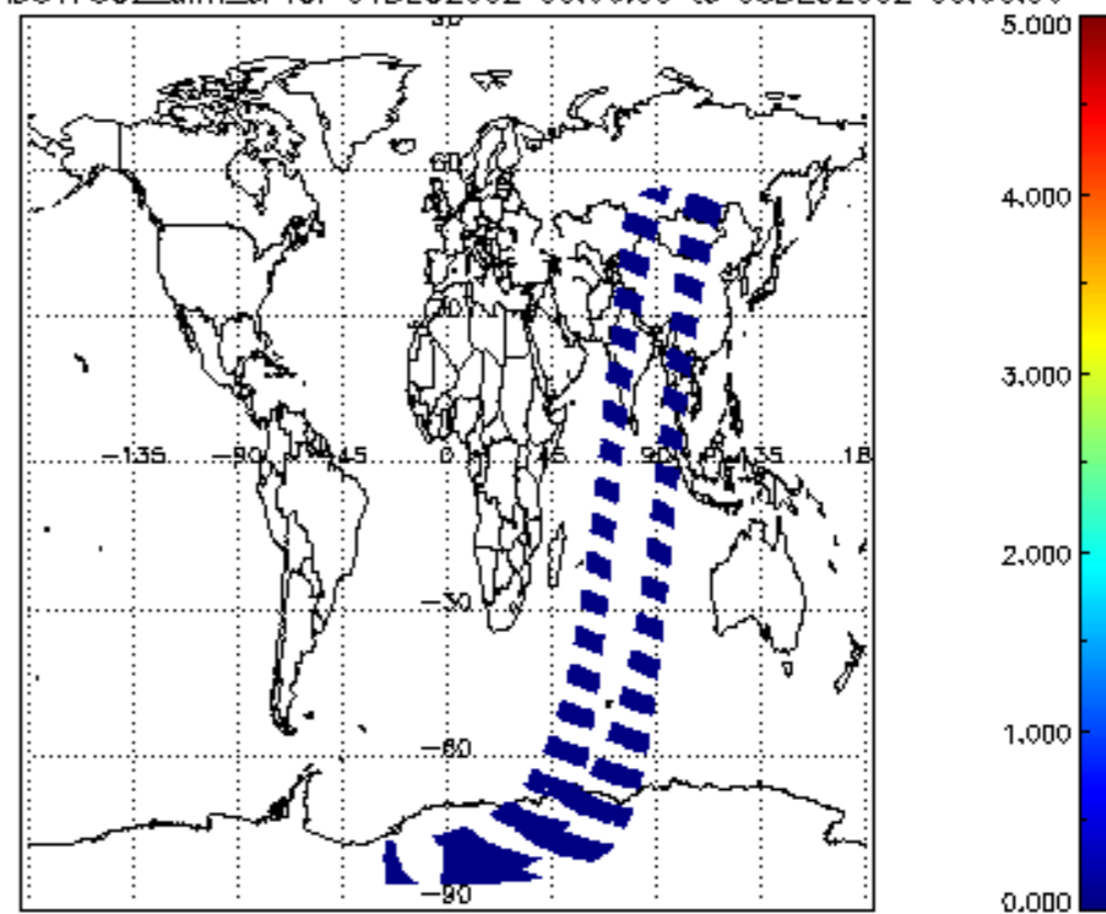
SCIOL2P_NADUV7S02_amf_cl for 04DEC2002 00:00:00 to 05DEC2002 00:00:00
