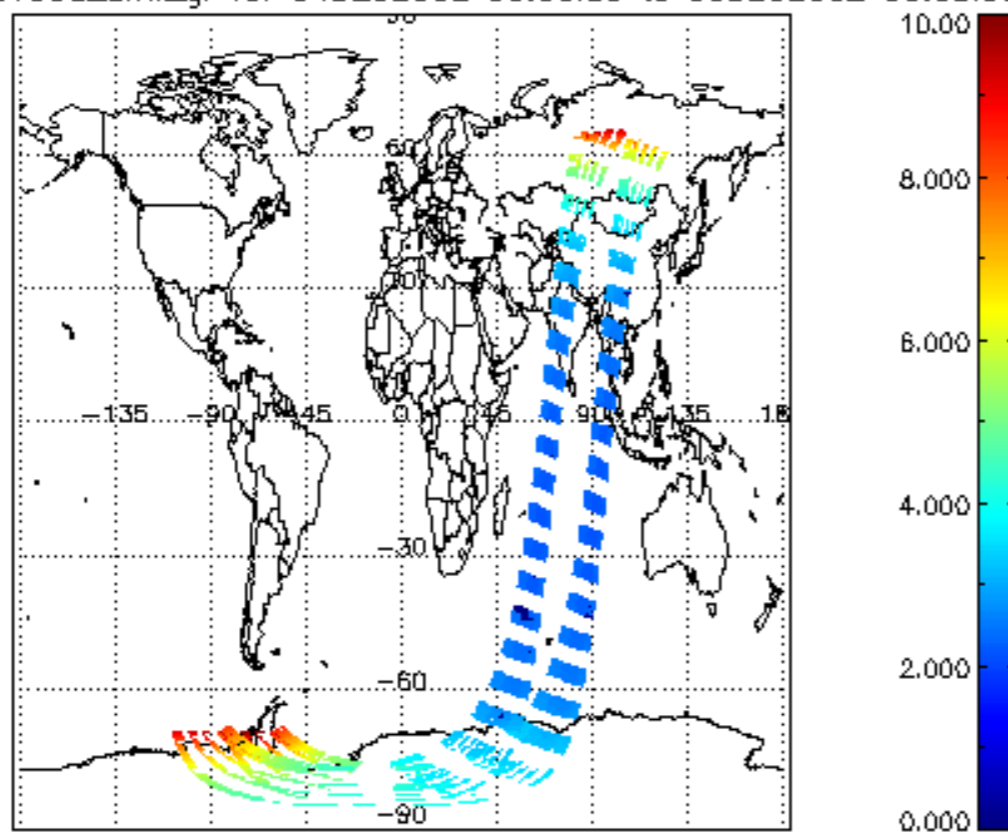
SCIOL2P_NADUV003_amf_gr for 04DEC2002 00:00:00 to 05DEC2002 00:00:00
