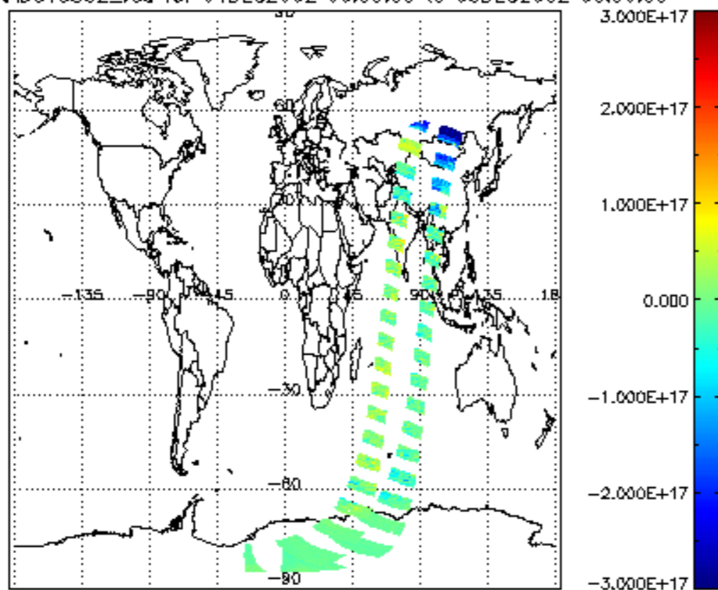
SCIOL2P_NADUV5S02_vcd for 04DEC2002 00:00:00 to 05DEC2002 00:00:00
