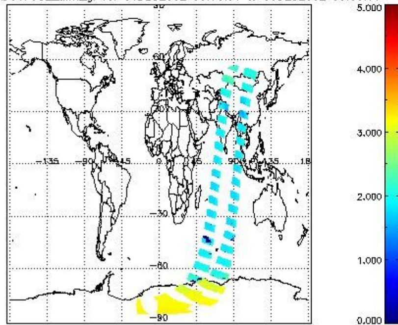
SCIOL2P_NADUV7S02_amf_gr for 04DEC2002 00:00:00 to 05DEC2002 00:00:00
