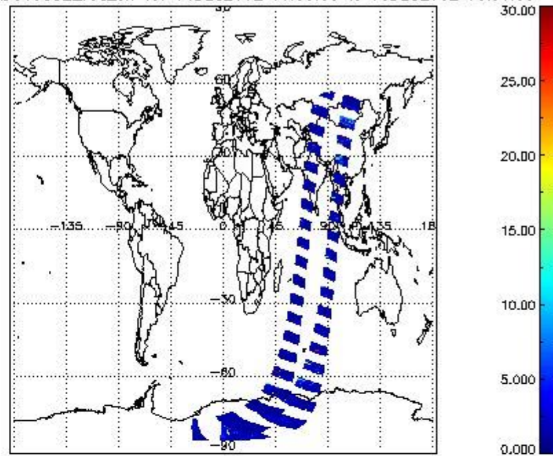
SCIOL2P_NADUV5SO2_vcd_err for 04DEC2002 00:00:00 to 05DEC2002 00:00:00
