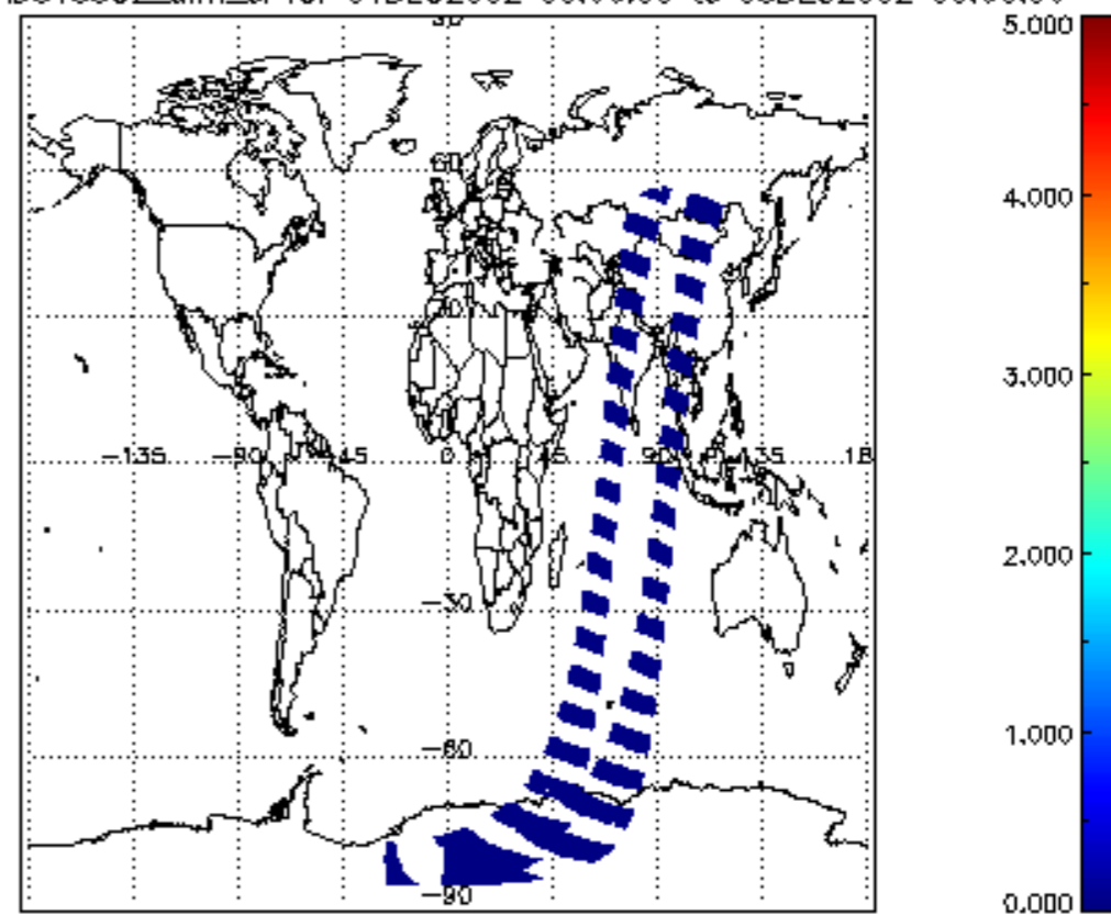
SCIOL2P_NADUV5S02_amf_cl for 04DEC2002 00:00:00 to 05DEC2002 00:00:00
