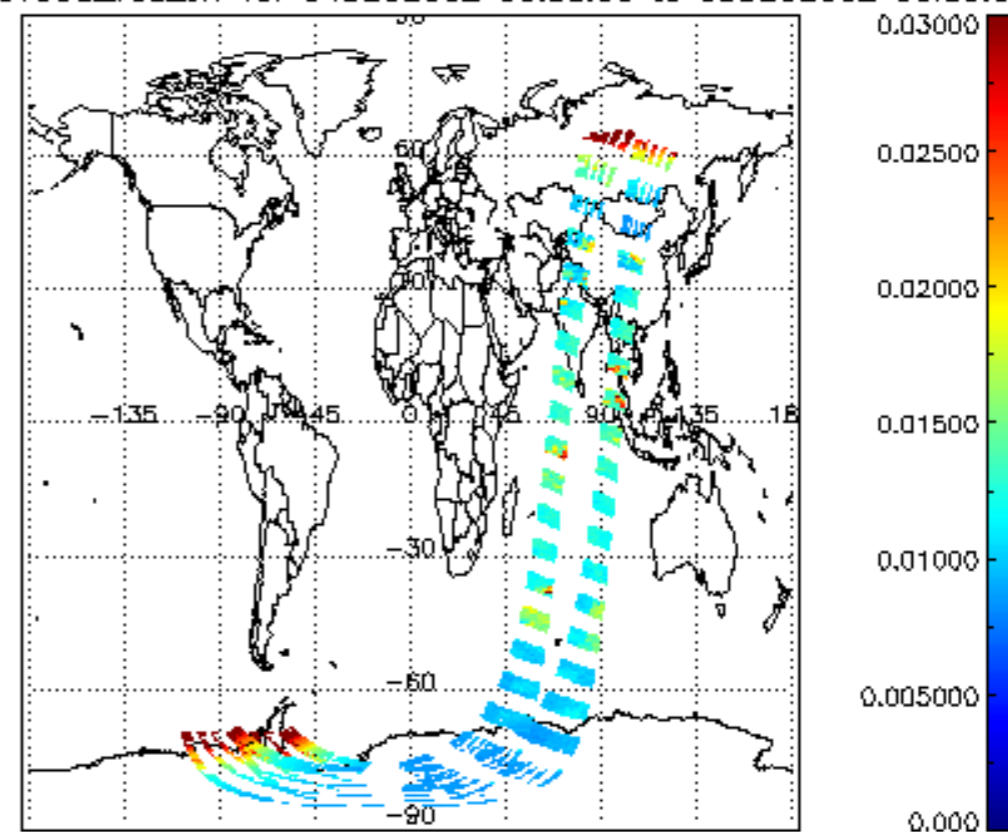
SCIOL2P_NADUV003_vcd_err for 04DEC2002 00:00:00 to 05DEC2002 00:00:00
