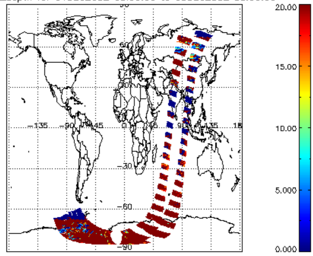
cl_opt_depth for 04DEC2002 00:00:00 to 05DEC2002 00:00:00
