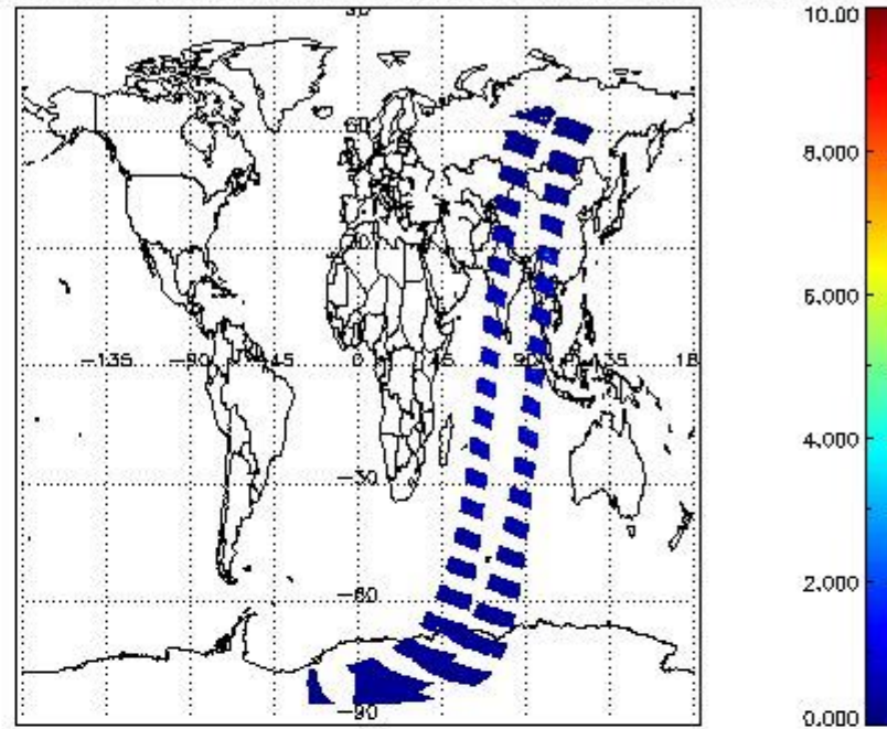
SCIOL2P_NADUV3BRO_vcd_err for 04DEC2002 00:00:00 to 05DEC2002 00:00:00
