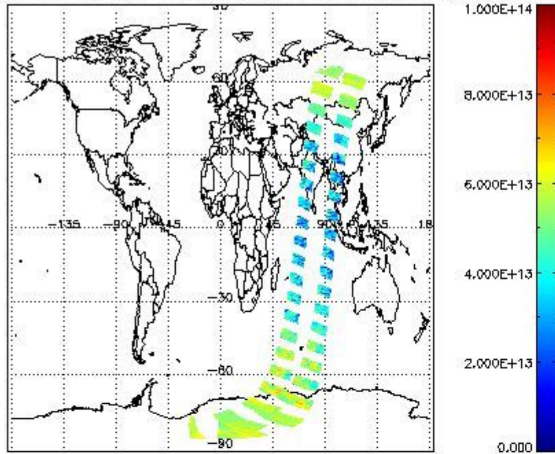
SCIOL2P_NADUV3BRO_vcd for 04DEC2002 00:00:00 to 05DEC2002 00:00:00
