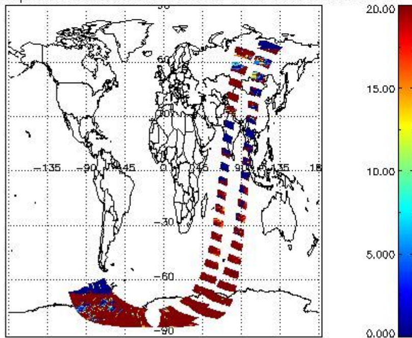
cL_opt_depth for 04DEC2002 00:00:00 to 05DEC2002 00:00:00
