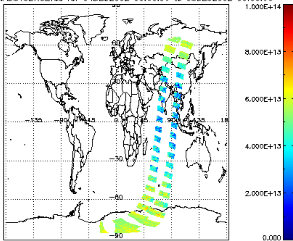
SCIOL2P_NADUV3BRO_vcd for 04DEC2002 00:00:00 to 05DEC2002 00:00:00
