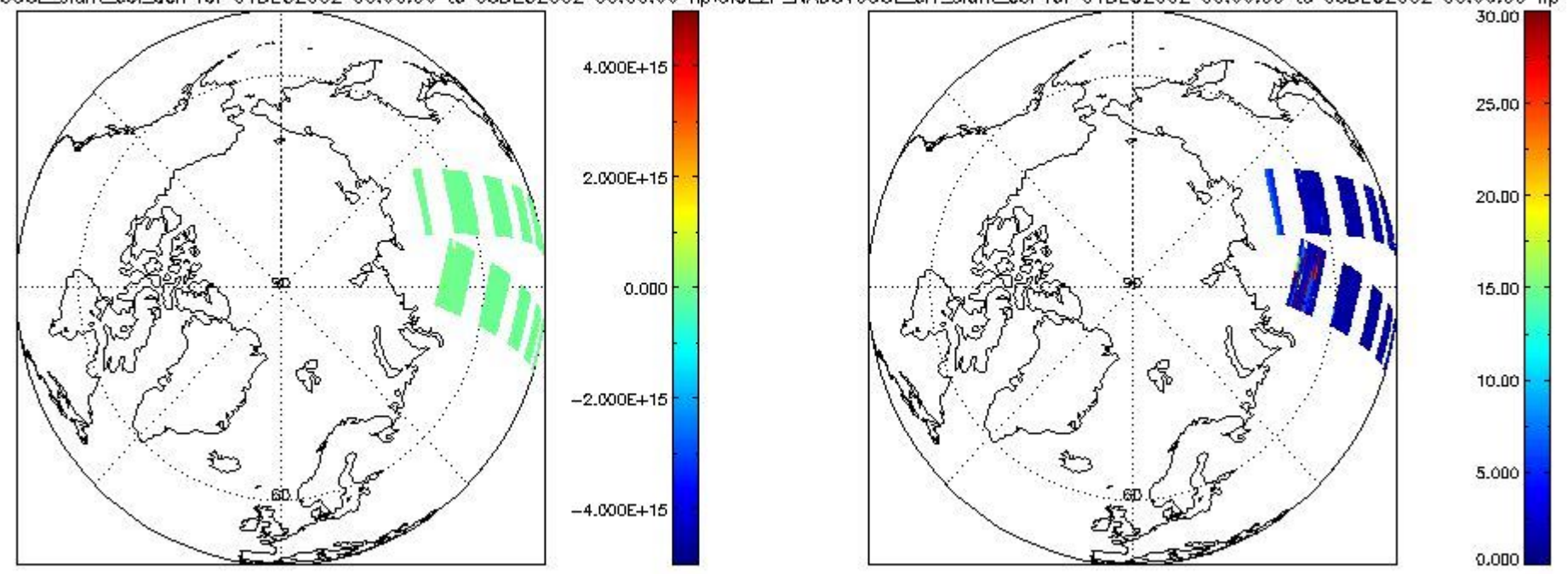
CIOL2P_NADUV60CL_slant_col_den for 04DEC2002 00:00:00 to 05DEC2002 00:00:00 np; CIOL2P_NADUV60CL_err_slant_col for 04DEC2002 00:00:00 to 05DEC2002 00:00:00 np
