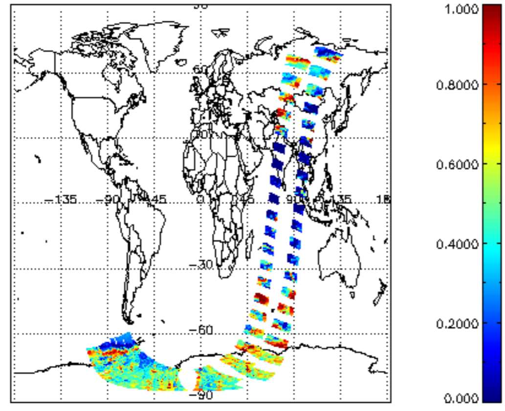
cl_frac for 04DEC2002 00:00:00 to 05DEC2002 00:00:00
