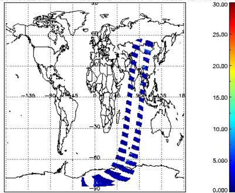
SCIOL2P_NADUV7S02_vcd_err for 04DEC2002 00:00:00 to 05DEC2002 00:00:00
