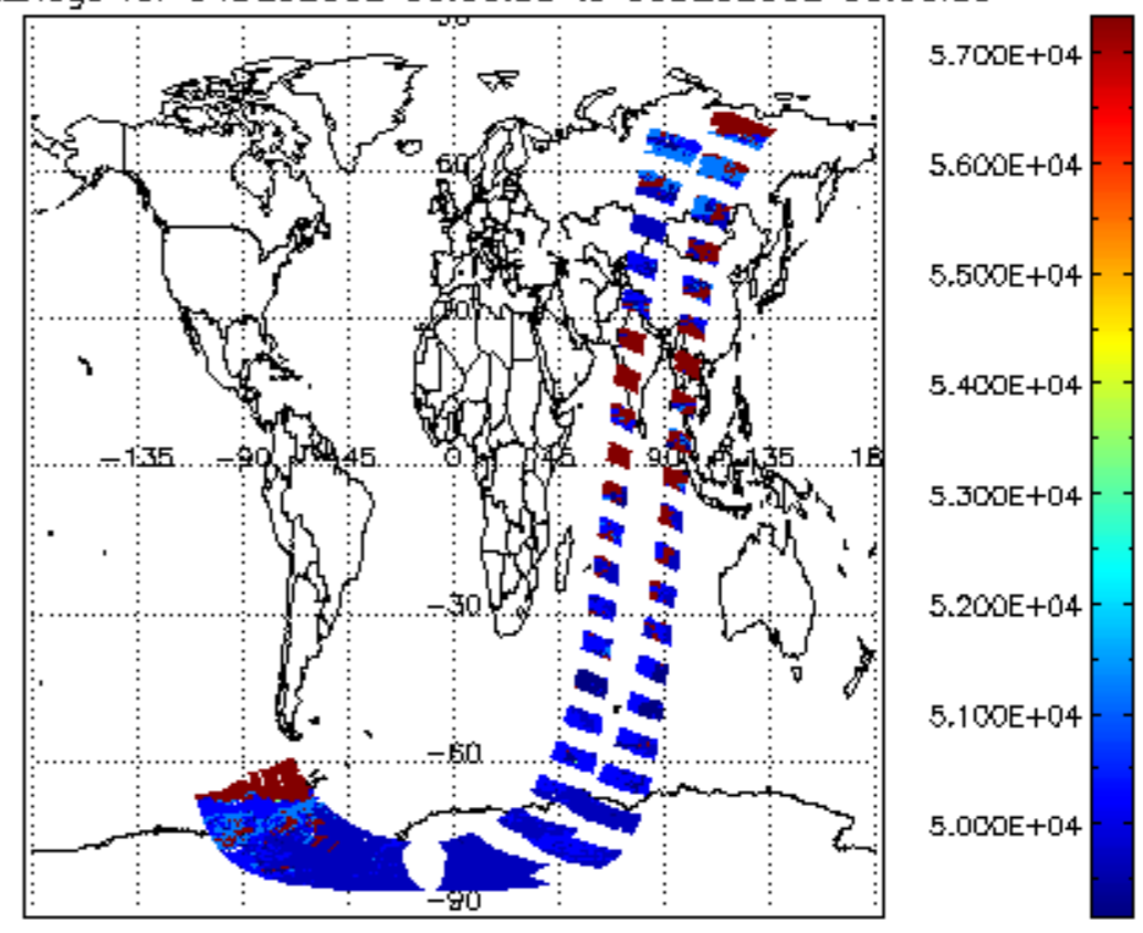
cloud_flags for 04DEC2002 00:00:00 to 05DEC2002 00:00:00
