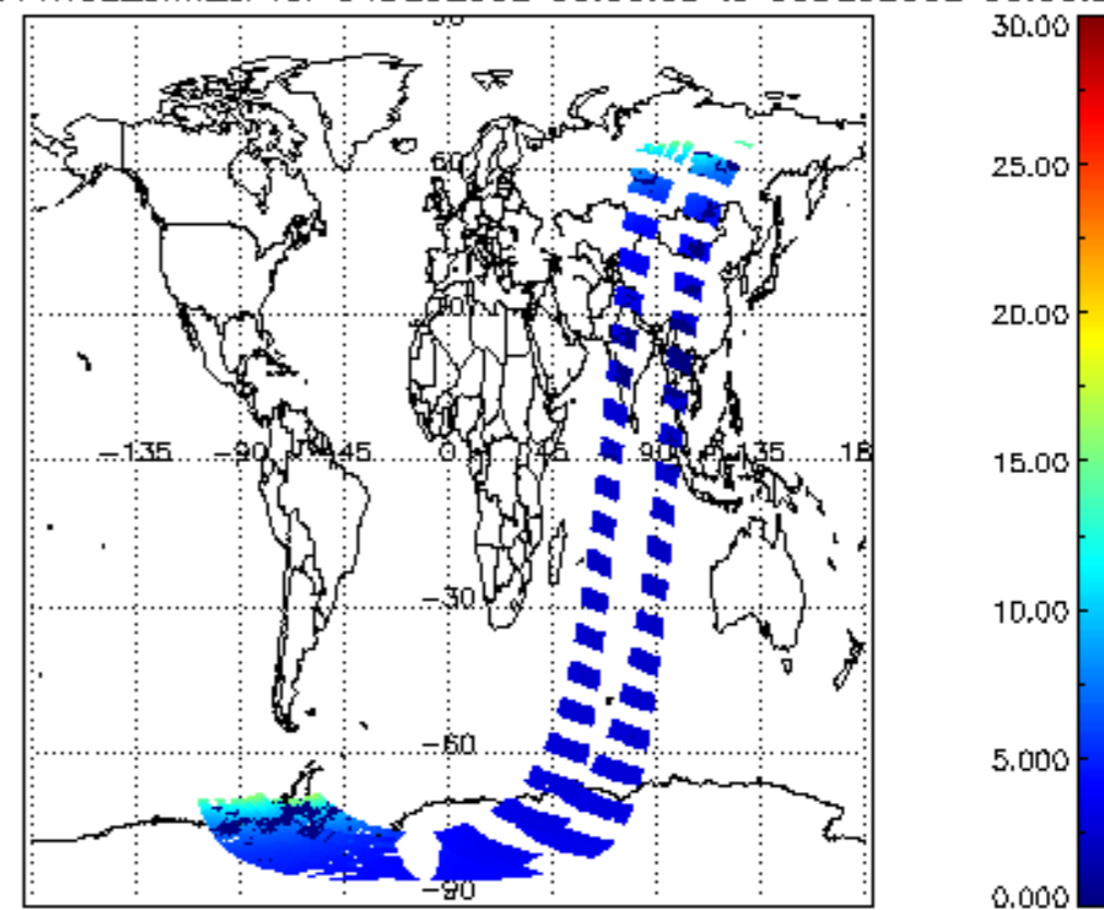
SCIOL2P_NADUV1NO2_amf_cl for 04DEC2002 00:00:00 to 05DEC2002 00:00:00
