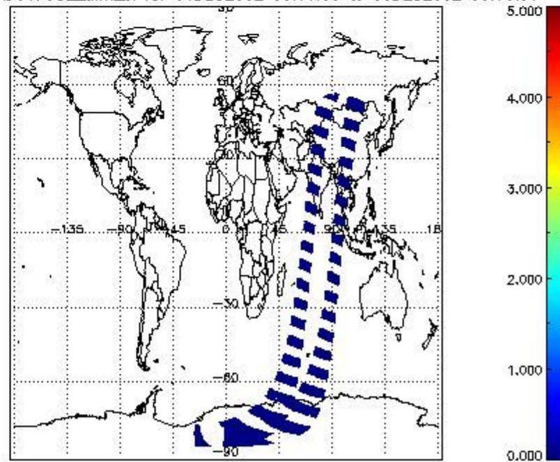
SCIOL2P_NADUV7S02_amf_cl for 04DEC2002 00:00:00 to 05DEC2002 00:00:00
