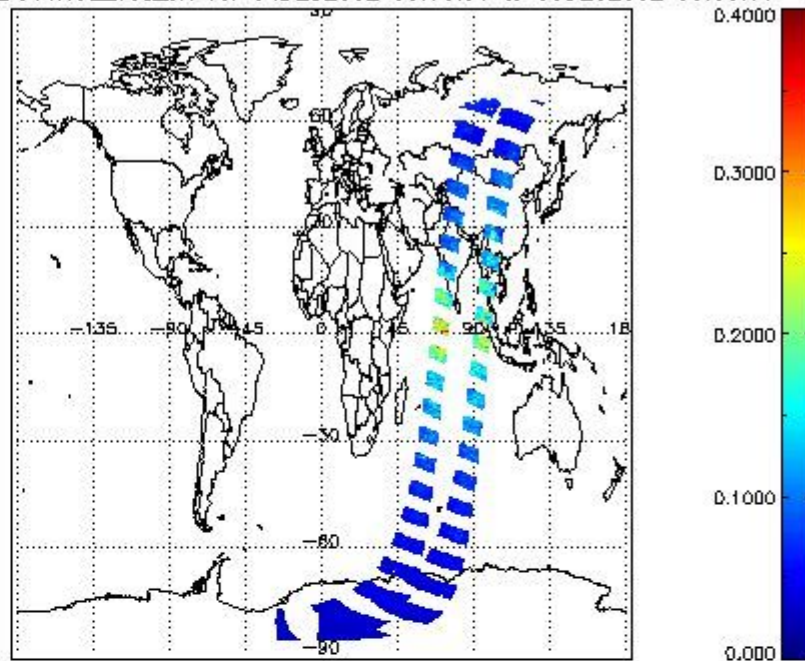
SCIOL2P_NADUV1N02_vcd_err for 04DEC2002 00:00:00 to 05DEC2002 00:00:00
