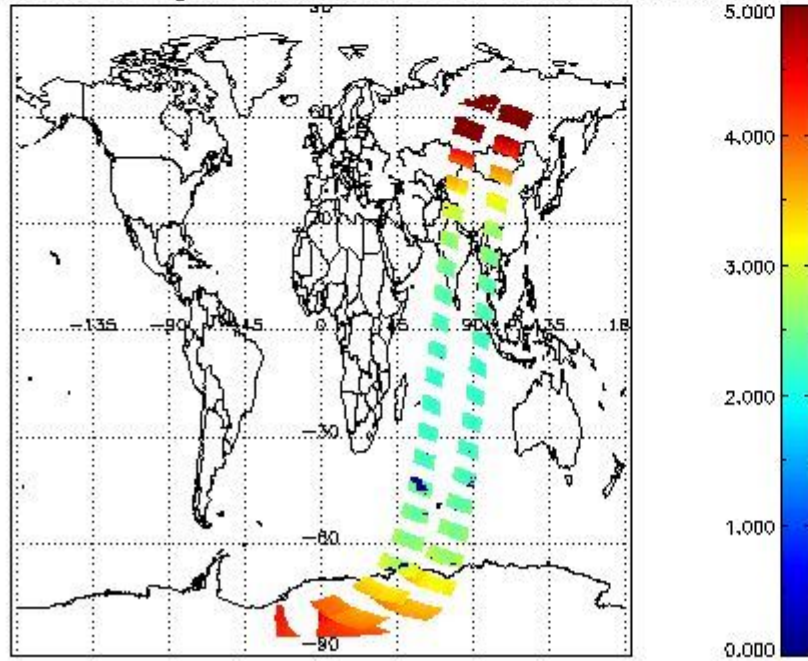
SCIOL2P_NADUV3BRO_amf_gr for 04DEC2002 00:00:00 to 05DEC2002 00:00:00
