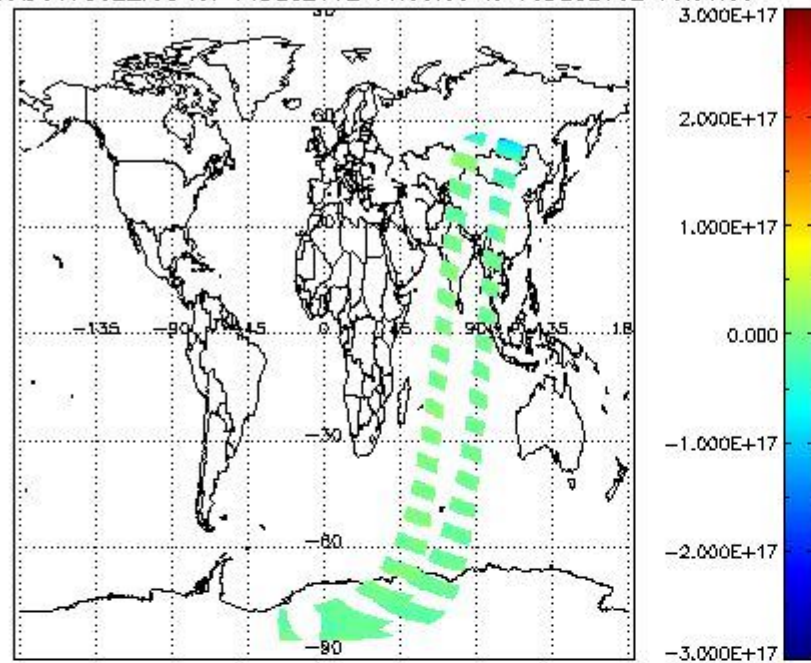
SCIOL2P_NADUV7S02_vcd for 04DEC2002 00:00:00 to 05DEC2002 00:00:00
