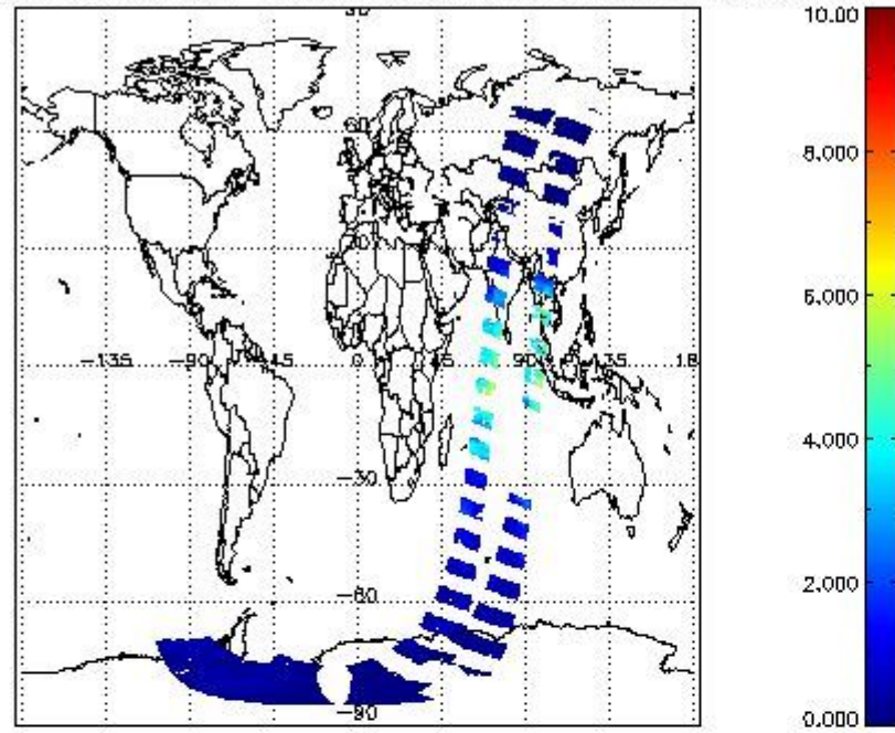
SCIOL2P_NADUV8H2O_vcd for 04DEC2002 00:00:00 to 05DEC2002 00:00:00
