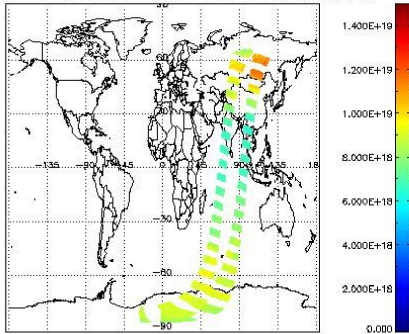
SCIOL2P_NADUV003_vcd for 04DEC2002 00:00:00 to 05DEC2002 00:00:00
