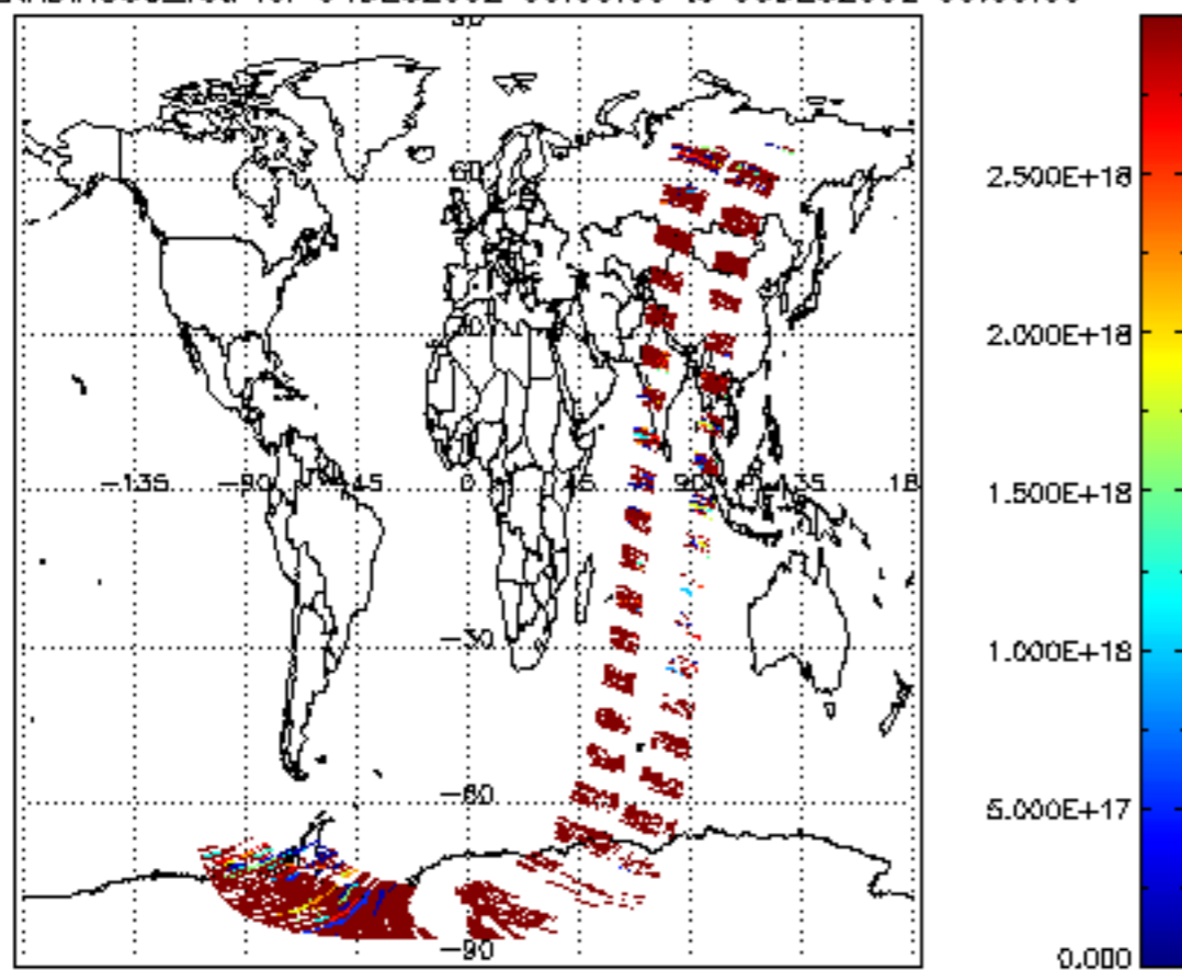
SCIOL2P_NADIR3CO_vcd for 04DEC2002 00:00:00 to 05DEC2002 00:00:00
