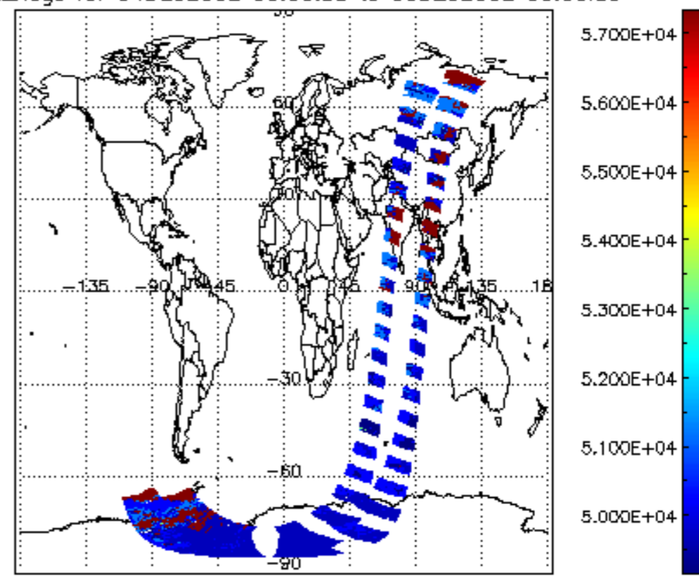
cloud_flags for 04DEC2002 00:00:00 to 05DEC2002 00:00:00
