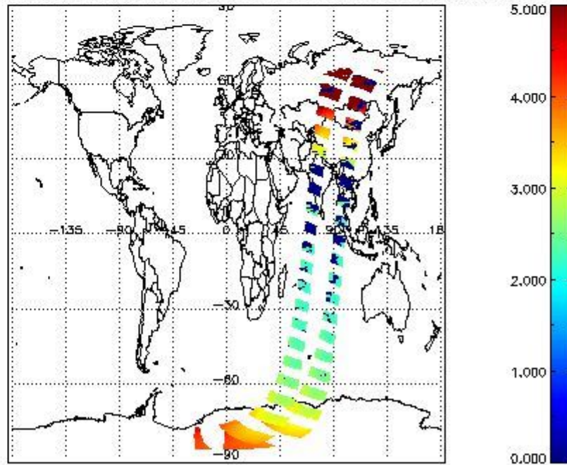
SCIOL2P_NADUV1N02_amf_cl for 04DEC2002 00:00:00 to 05DEC2002 00:00:00
