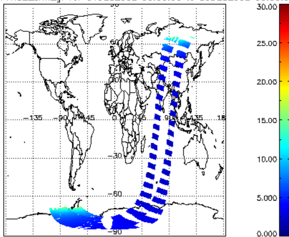
SCIOL2P_NADUV1NO2_amf_gr for 04DEC2002 00:00:00 to 05DEC2002 00:00:00
