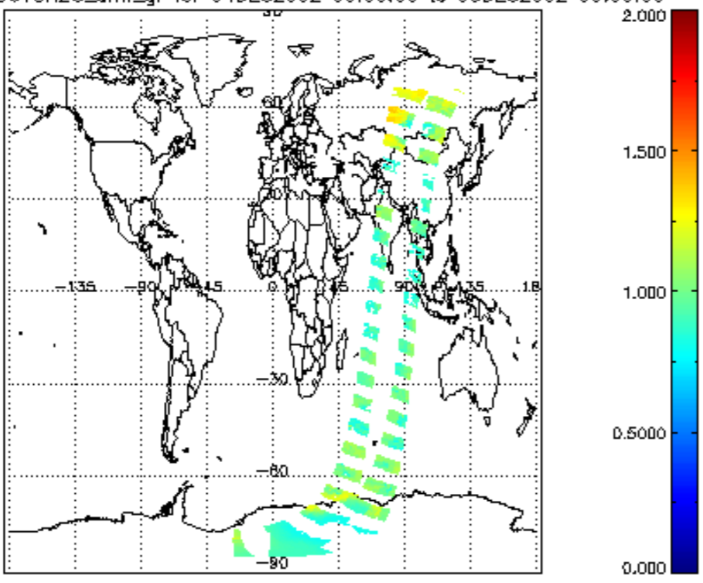
SCIOL2P_NADUV8H2O_amf_gr for 04DEC2002 00:00:00 to 05DEC2002 00:00:00
