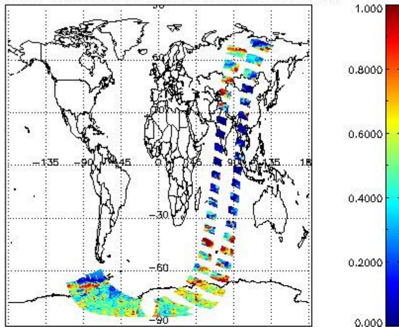
cL_frac for 04DEC2002 00:00:00 to 05DEC2002 00:00:00
