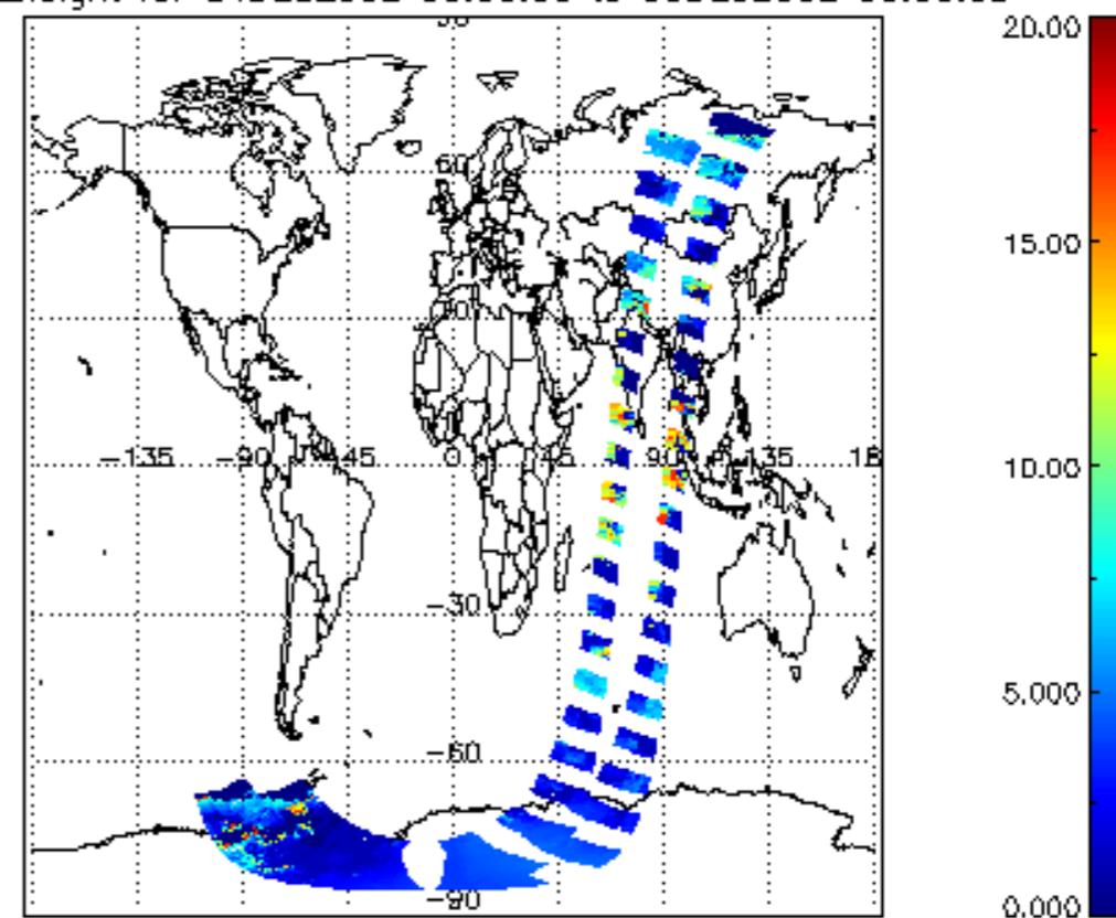
cl_top_height for 04DEC2002 00:00:00 to 05DEC2002 00:00:00
