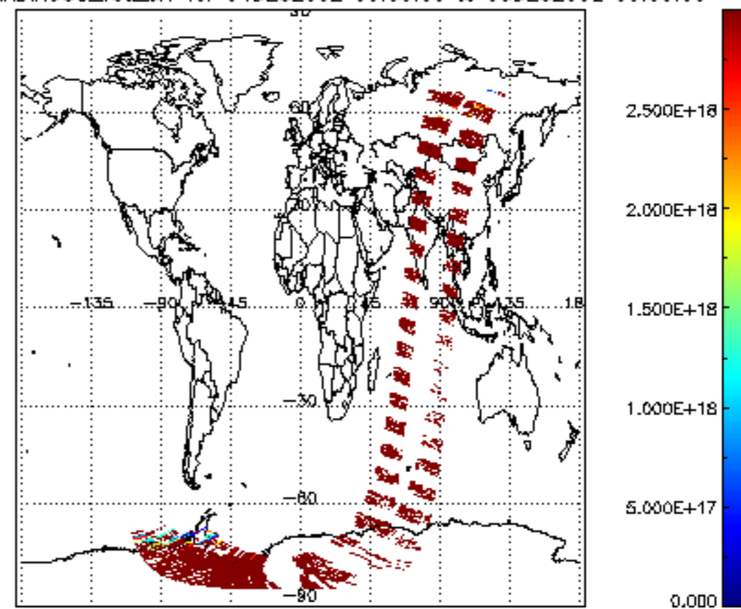
SCIOL2P_NADIR3CO_vcdLerr for 04DEC2002 00:00:00 to 05DEC2002 00:00:00
