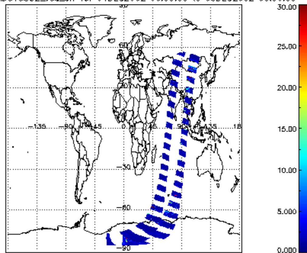
SCIOL2P_NADUV5S02_vcd_err for 04DEC2002 00:00:00 to 05DEC2002 00:00:00
