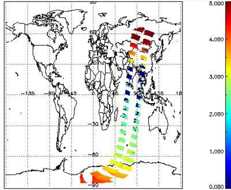
SCIOL2P_NADUV3BRO_amf_cl for 04DEC2002 00:00:00 to 05DEC2002 00:00:00
