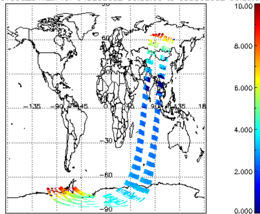
SCIOL2P_NADUV003_amf_cl for 04DEC2002 00:00:00 to 05DEC2002 00:00:00
