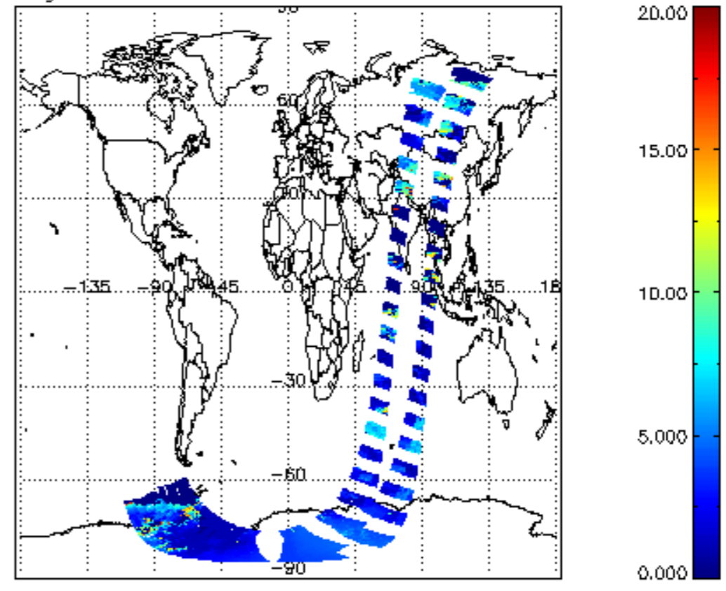
cl_top_height for 04DEC2002 00:00:00 to 05DEC2002 00:00:00
