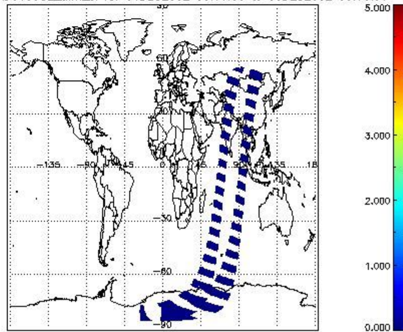
SCIOL2P_NADUV5SO2_amf_cl for 04DEC2002 00:00:00 to 05DEC2002 00:00:00
