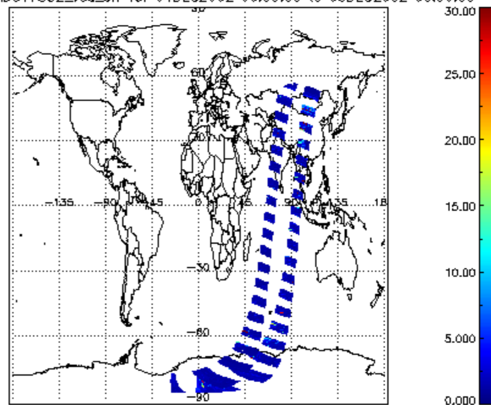
SCIOL2P_NADUV7S02_vcd_err for 04DEC2002 00:00:00 to 05DEC2002 00:00:00
