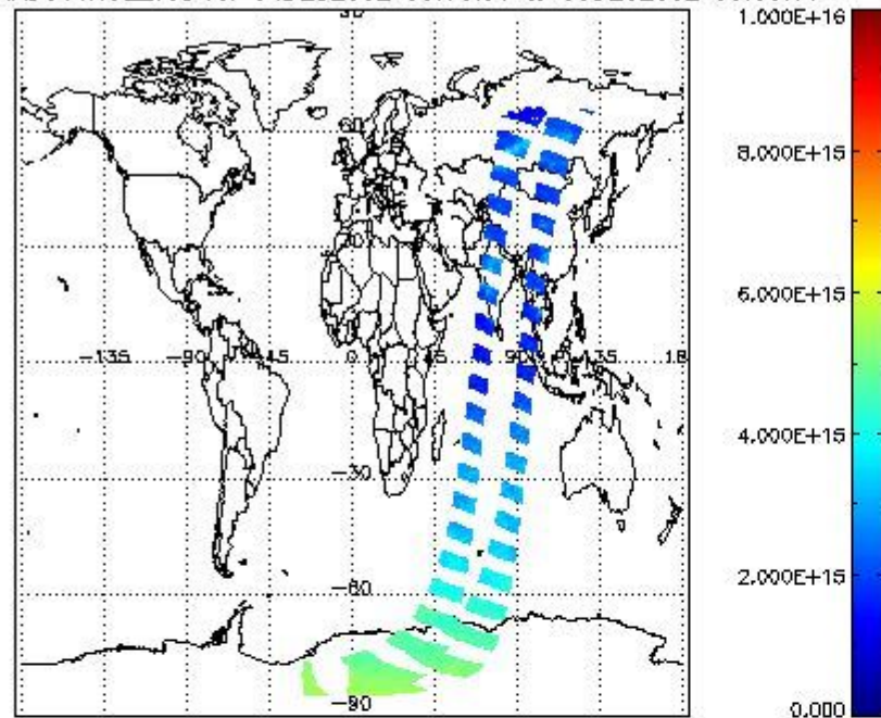
SCIOL2P_NADUV1N02_vcd for 04DEC2002 00:00:00 to 05DEC2002 00:00:00
