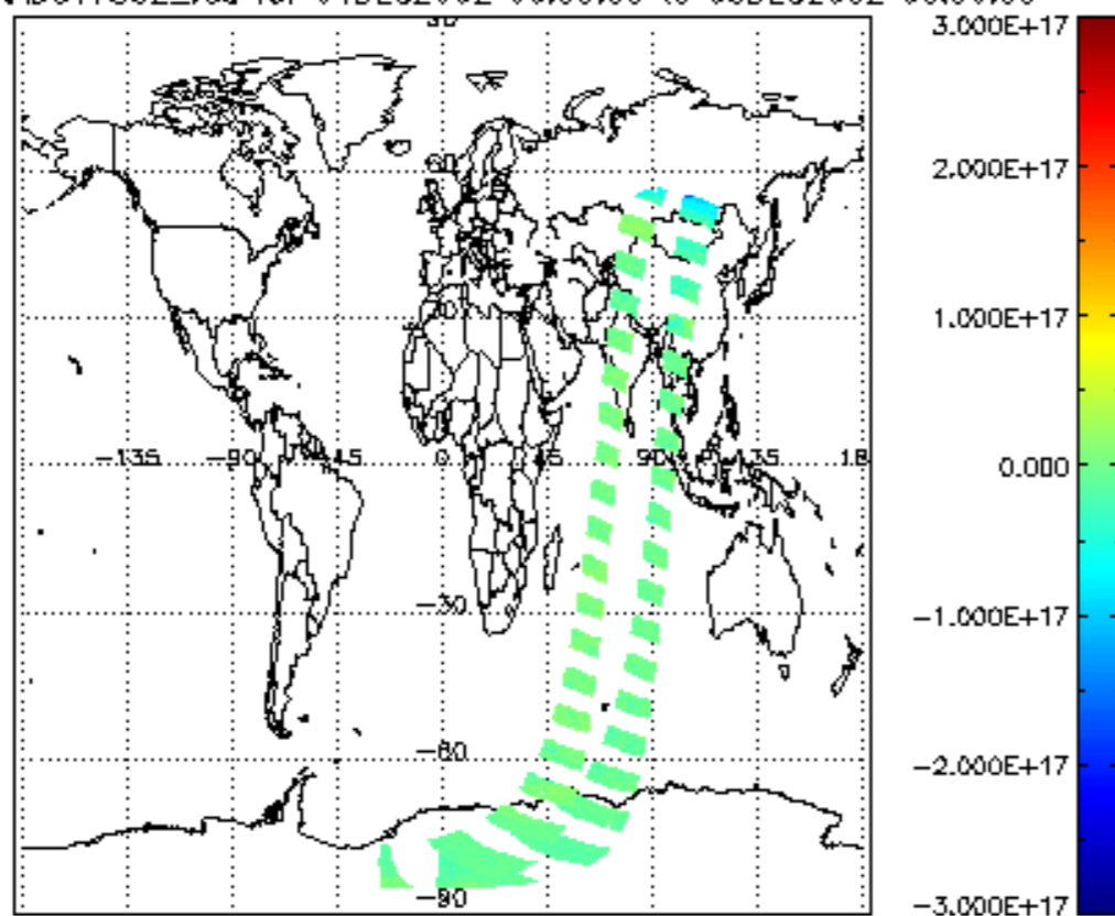
SCIOL2P_NADUV7S02_vcd for 04DEC2002 00:00:00 to 05DEC2002 00:00:00
