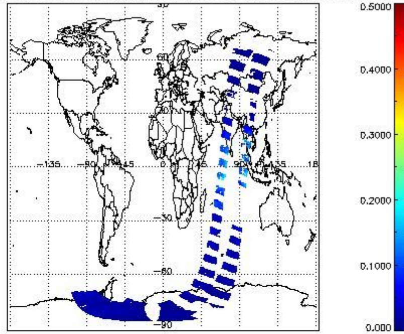
SCIOL2P_NADUV8H2O_vcd_err for 04DEC2002 00:00:00 to 05DEC2002 00:00:00
