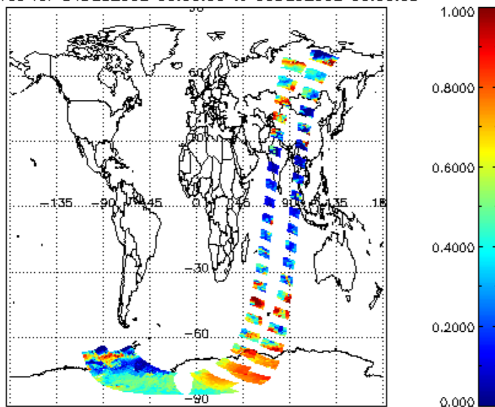
cl_frac for 04DEC2002 00:00:00 to 05DEC2002 00:00:00
