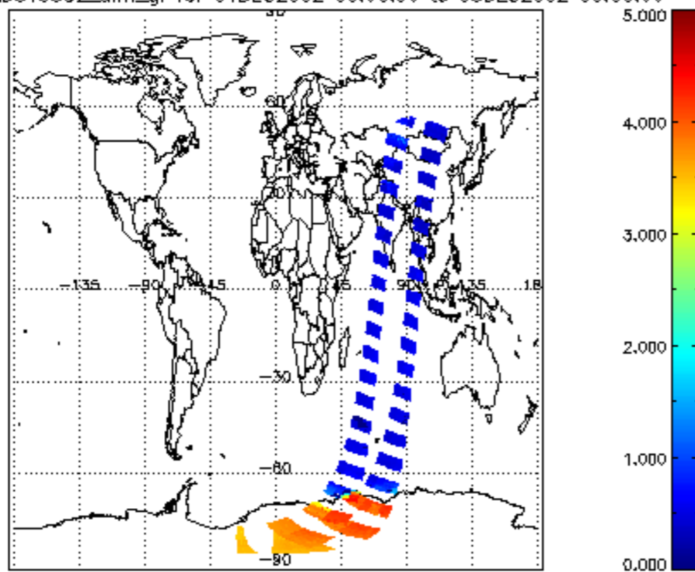
SCIOL2P_NADUV5S02_amf_gr for 04DEC2002 00:00:00 to 05DEC2002 00:00:00
