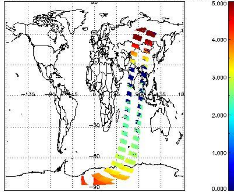
SCIOL2P_NADUV003_amf_cl for 04DEC2002 00:00:00 to 05DEC2002 00:00:00
