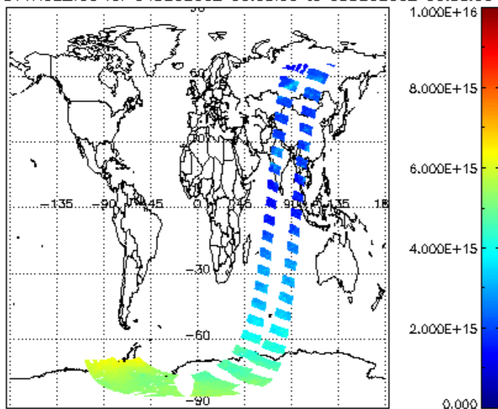
SCIOL2P_NADUV1NO2_vcd for 04DEC2002 00:00:00 to 05DEC2002 00:00:00
