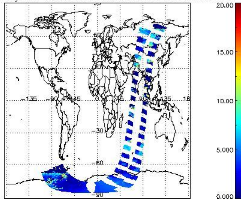
cL_top_height for 04DEC2002 00:00:00 to 05DEC2002 00:00:00
