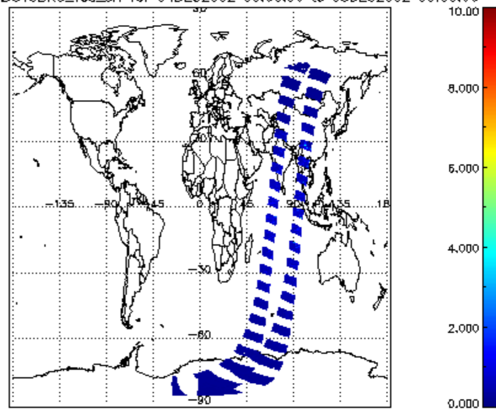
SCIOL2P_NADUV3BRO_vcd_err for 04DEC2002 00:00:00 to 05DEC2002 00:00:00
