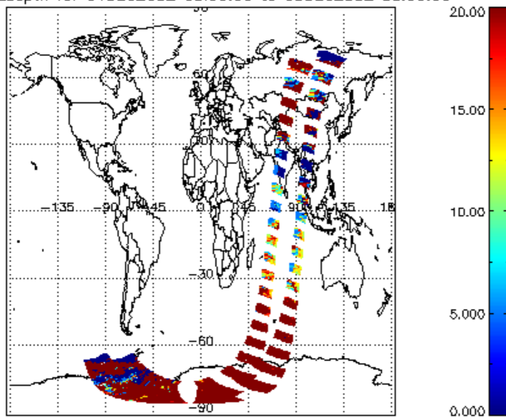
cl_opt_depth for 04DEC2002 00:00:00 to 05DEC2002 00:00:00
