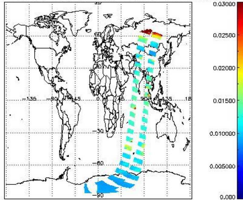
SCIOL2P_NADUV003_vcd_err for 04DEC2002 00:00:00 to 05DEC2002 00:00:00
