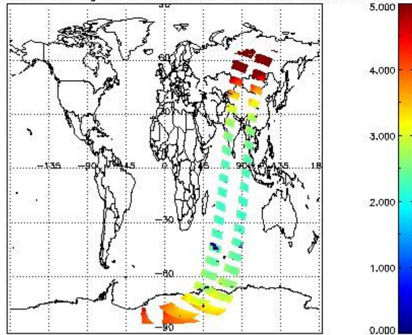
SCIOL2P_NADUV1N02_amf_gr for 04DEC2002 00:00:00 to 05DEC2002 00:00:00
