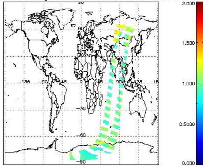
SCIOL2P_NADUV8H2O_amf_gr for 04DEC2002 00:00:00 to 05DEC2002 00:00:00
