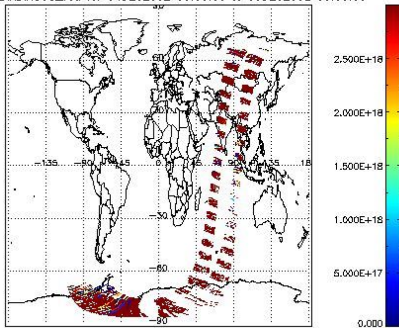
SCIDL2P_NADIR3CO_vcd for 04DEC2002 00:00:00 to 05DEC2002 00:00:00
