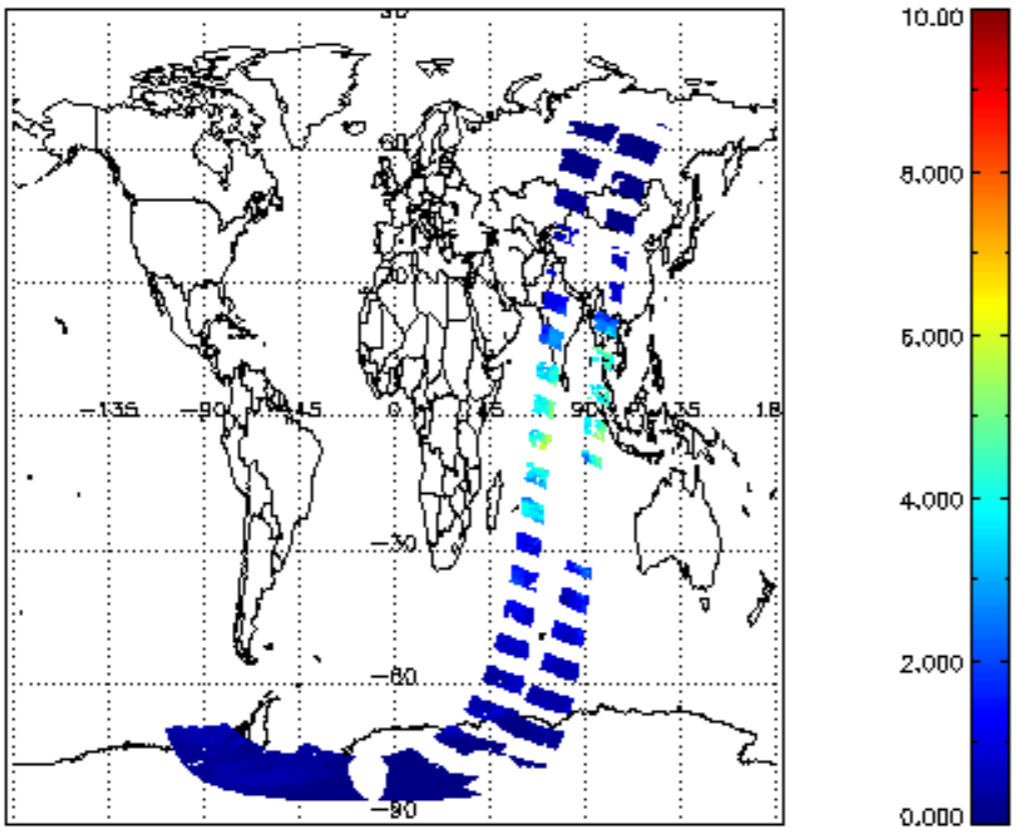
SCIOL2P_NADUV8H2O_vcd for 04DEC2002 00:00:00 to 05DEC2002 00:00:00
