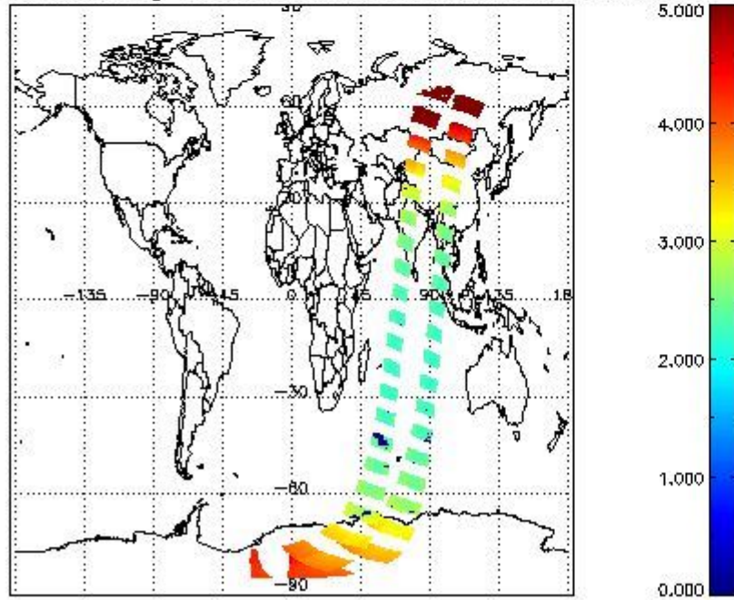
SCIOL2P_NADUV003_amf_gr for 04DEC2002 00:00:00 to 05DEC2002 00:00:00
