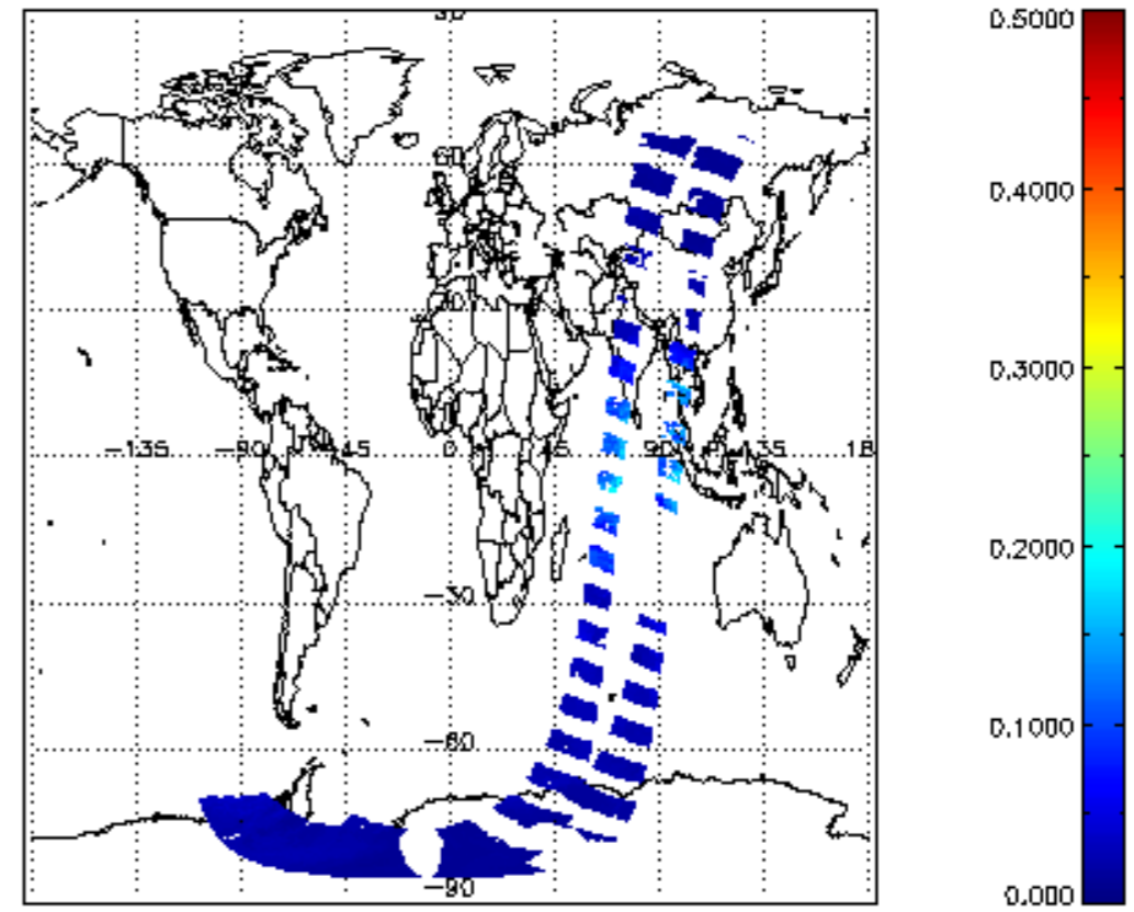
SCIOL2P_NADUV8H2O_vcd_err for 04DEC2002 00:00:00 to 05DEC2002 00:00:00
