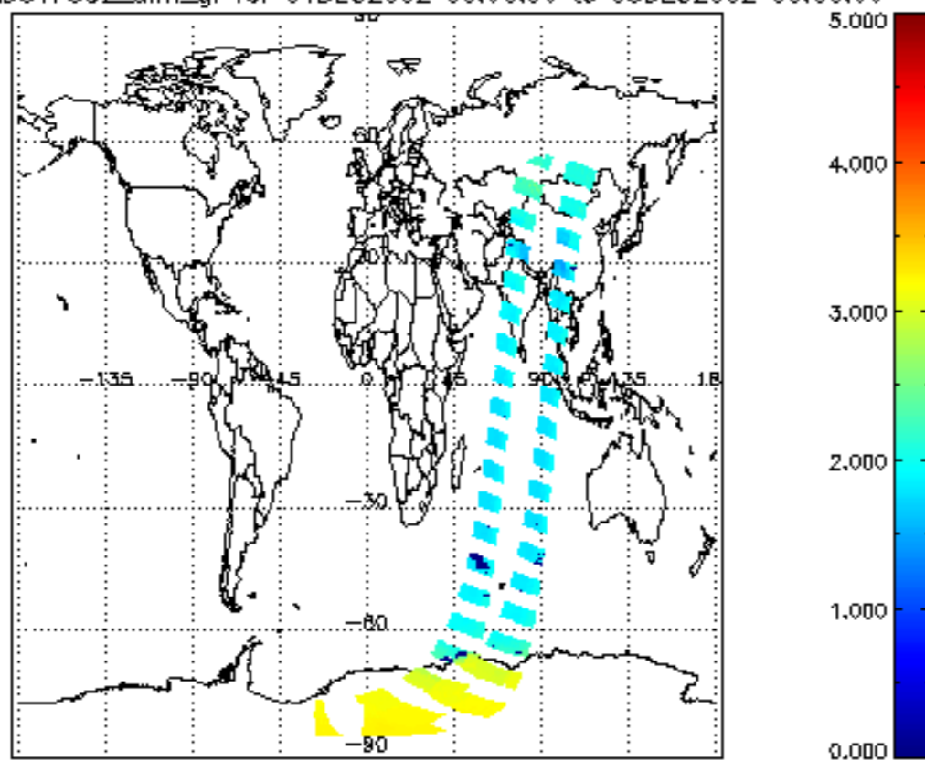
SCIOL2P_NADUV7S02_amf_gr for 04DEC2002 00:00:00 to 05DEC2002 00:00:00
