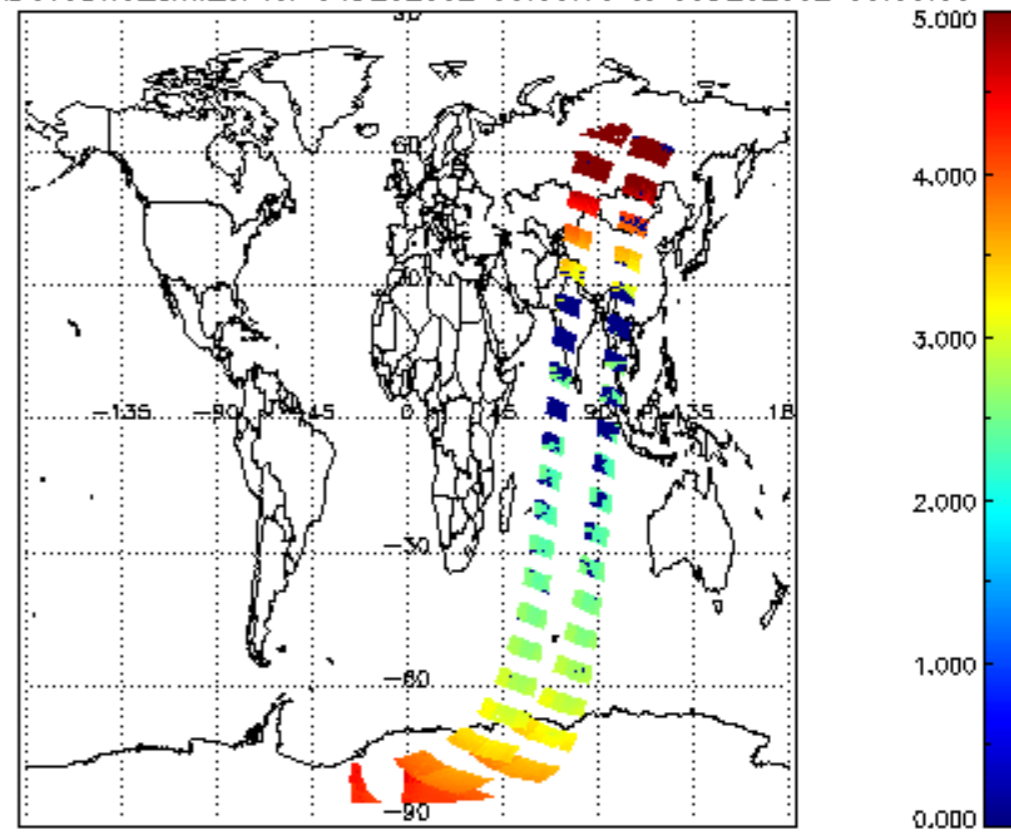
SCIOL2P_NADUV3BRO_amf_cl for 04DEC2002 00:00:00 to 05DEC2002 00:00:00
