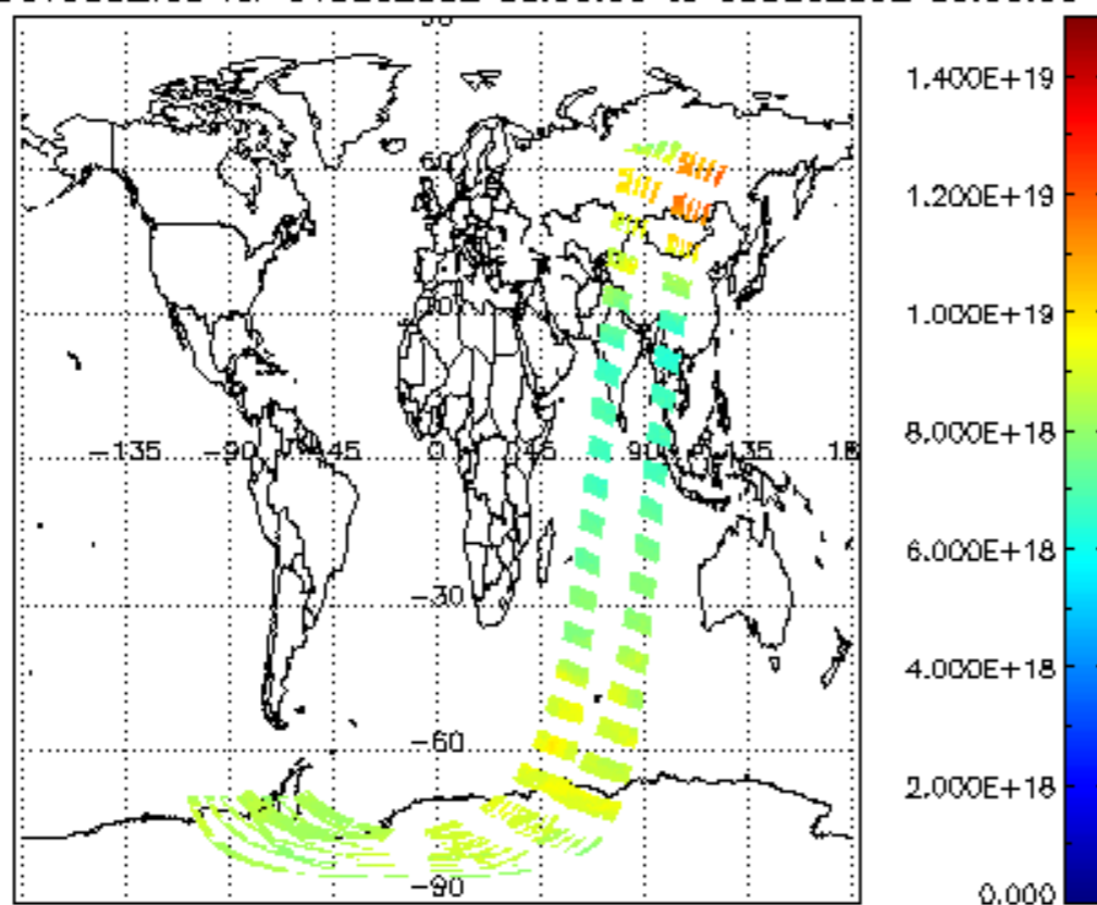
SCIOL2P_NADUV003_vcd for 04DEC2002 00:00:00 to 05DEC2002 00:00:00
