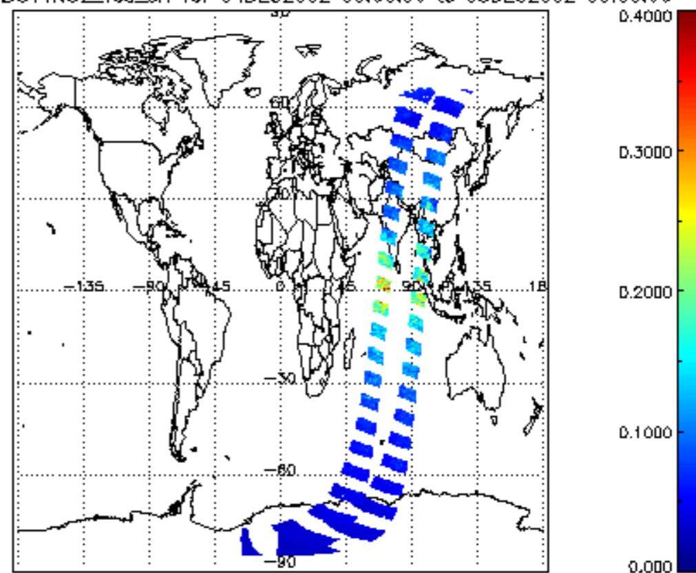
SCIOL2P_NADUV1NO2_vcd_err for 04DEC2002 00:00:00 to 05DEC2002 00:00:00
