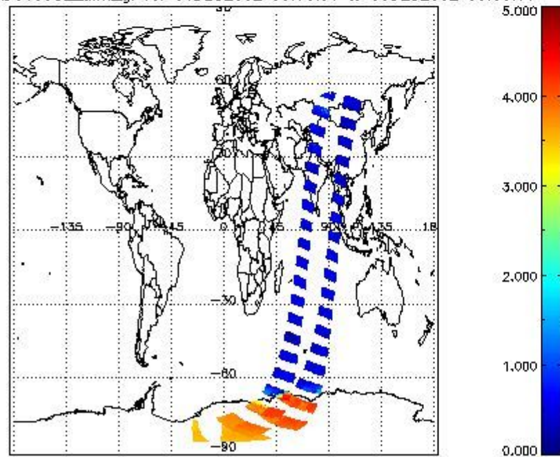
SCIOL2P_NADUV5SO2_amf_gr for 04DEC2002 00:00:00 to 05DEC2002 00:00:00
