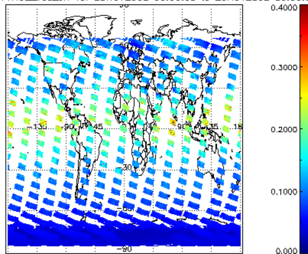
SCIOL2P_NADUV1NO2_vcd_err for 25NOV2002 00:00:00 to 26NOV2002 00:00:00
