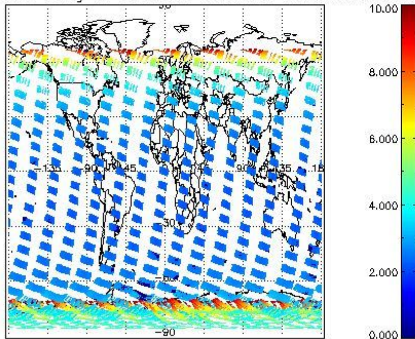
SCIOL2P_NADUV003_amf_gr for 25NOV2002 00:00:00 to 26NOV2002 00:00:00
