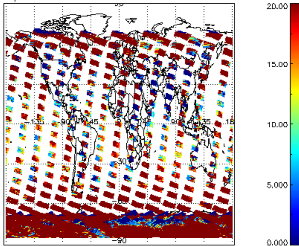
cL_opt_depth for 25NOV2002 00:00:00 to 26NOV2002 00:00:00
