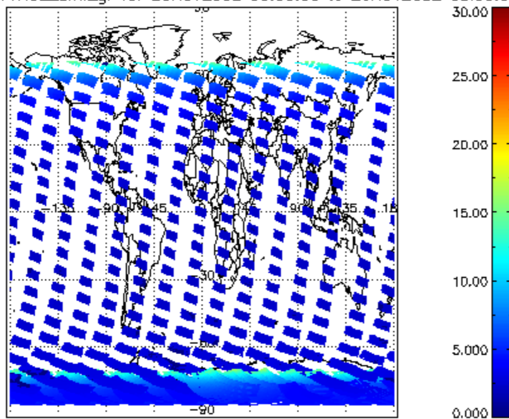
SCIOL2P_NADUV1NO2_amf_gr for 25NOV2002 00:00:00 to 26NOV2002 00:00:00
