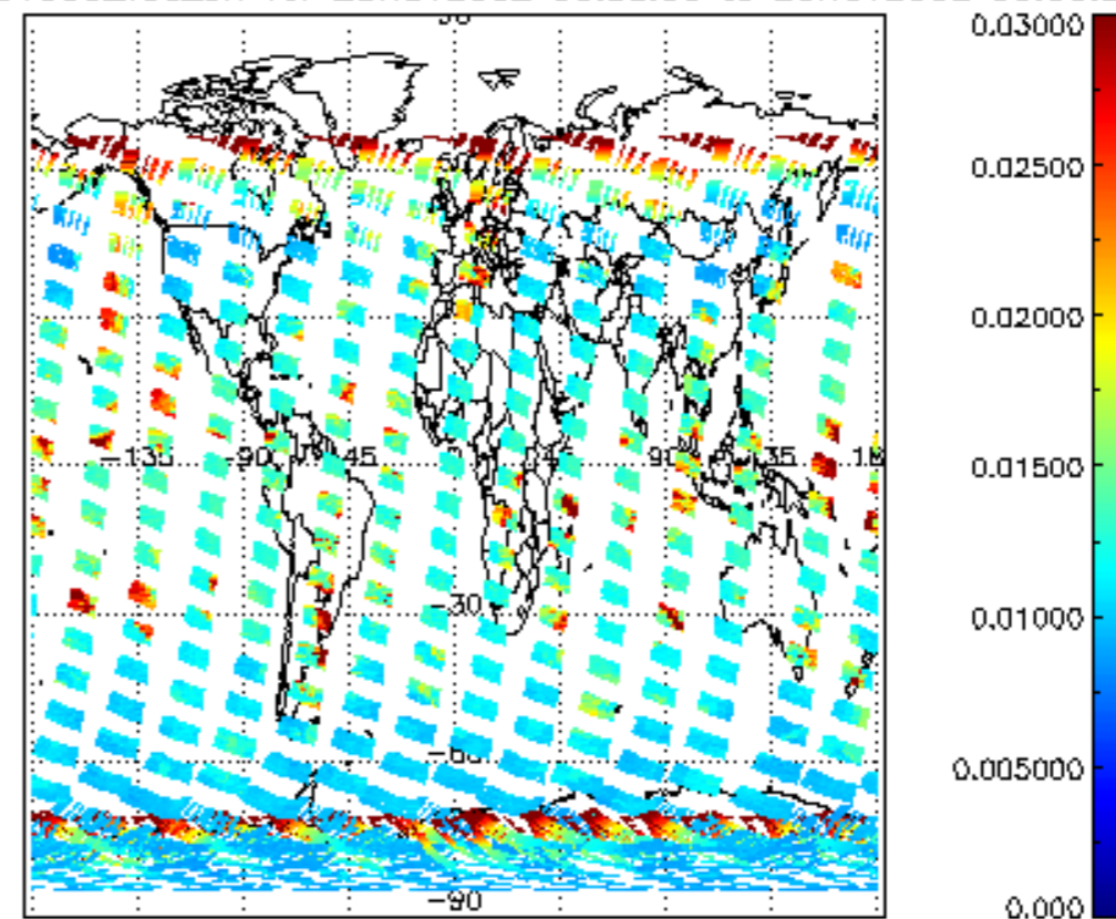
SCIOL2P_NADUV003_vcd_err for 25NOV2002 00:00:00 to 26NOV2002 00:00:00
