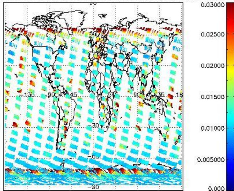
SCIOL2P_NADUV003_vcd_err for 25NOV2002 00:00:00 to 26NOV2002 00:00:00
