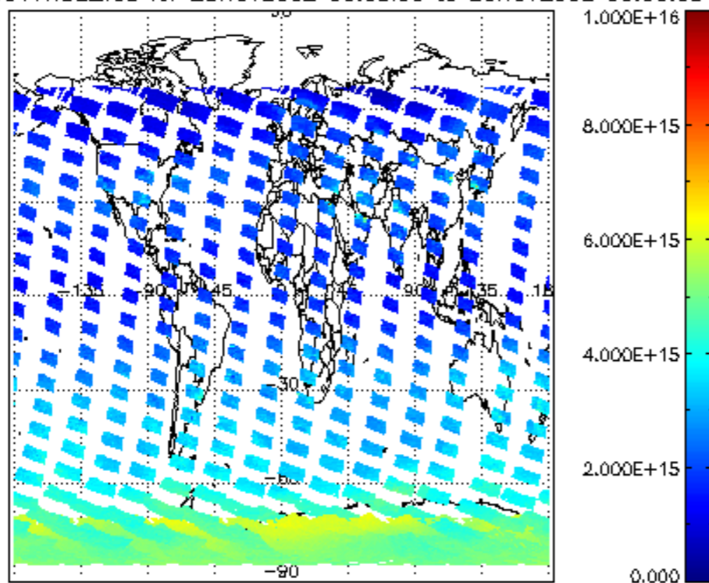
SCIOL2P_NADUV1NO2_vcd for 25NOV2002 00:00:00 to 26NOV2002 00:00:00
