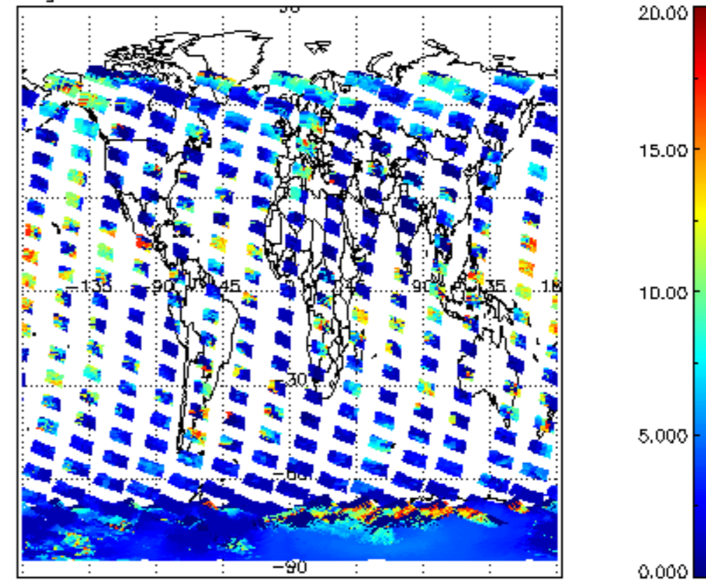
cL_top_height for 25NOV2002 00:00:00 to 26NOV2002 00:00:00
