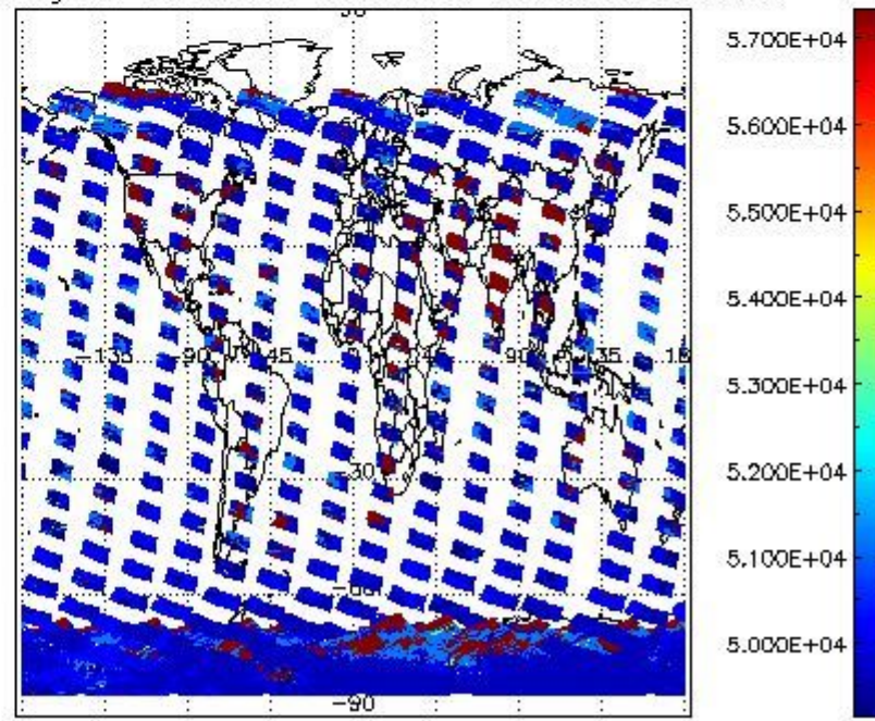
cloud_flags for 25NOV2002 00:00:00 to 26NOV2002 00:00:00
