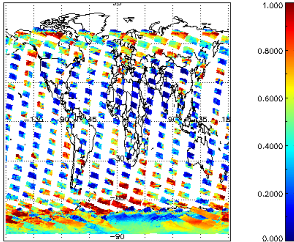
cLfrac for 25NOV2002 00:00:00 to 26NOV2002 00:00:00
