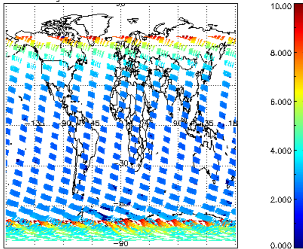
SCIOL2P_NADUV003_amf_gr for 25NOV2002 00:00:00 to 26NOV2002 00:00:00
