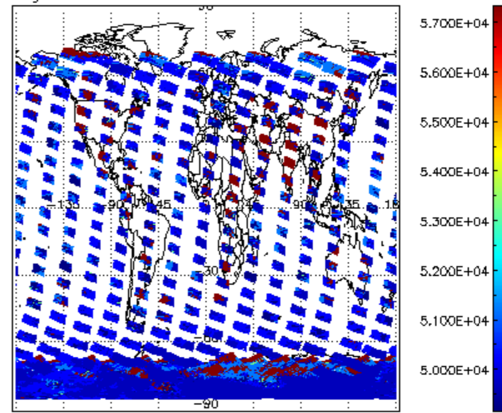
cloud_flags for 25NOV2002 00:00:00 to 26NOV2002 00:00:00
