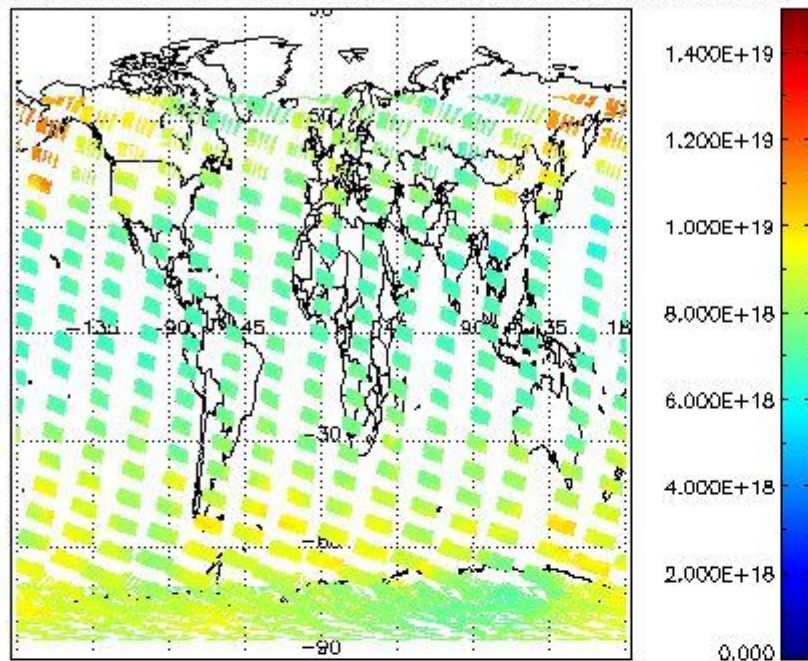
SCIOL2P_NADUV003_vcd for 25NOV2002 00:00:00 to 26NOV2002 00:00:00
