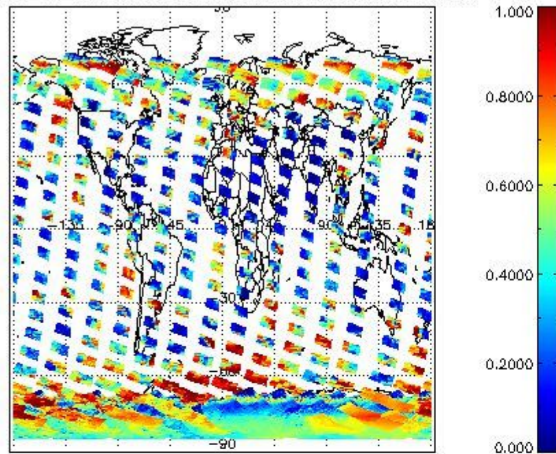
cLfrac for 25NOV2002 00:00:00 to 26NOV2002 00:00:00
