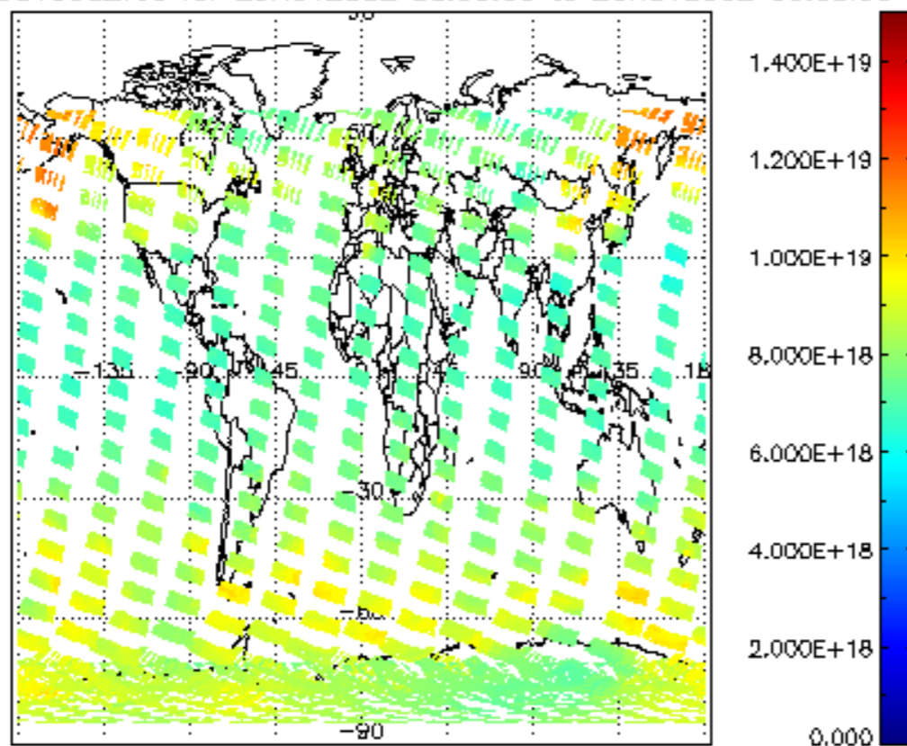
SCIOL2P_NADUV003_vcd for 25NOV2002 00:00:00 to 26NOV2002 00:00:00
