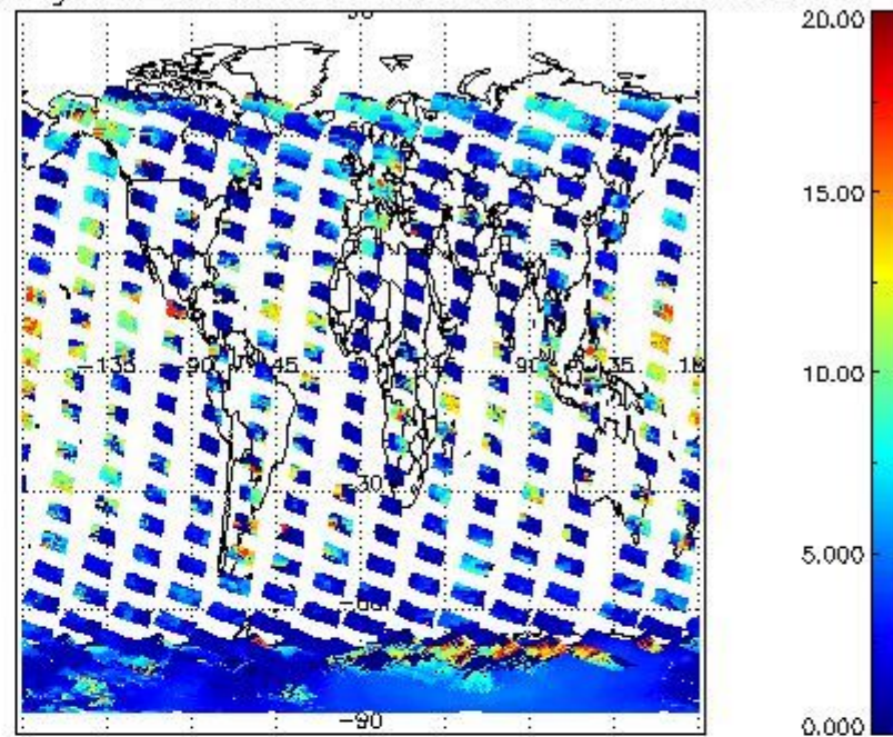
cL_top_height for 25NOV2002 00:00:00 to 26NOV2002 00:00:00
