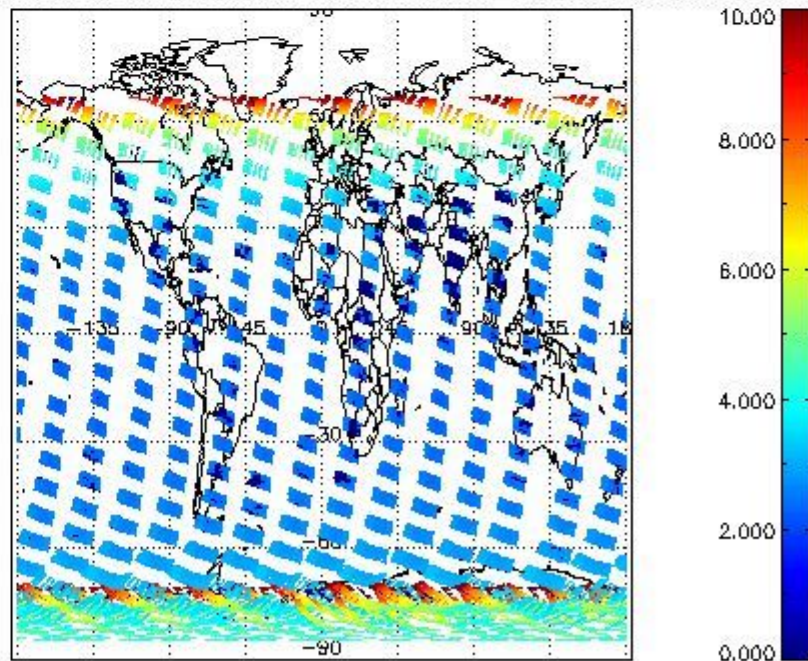
SCIOL2P_NADUV003_amf_cl for 25NOV2002 00:00:00 to 26NOV2002 00:00:00
