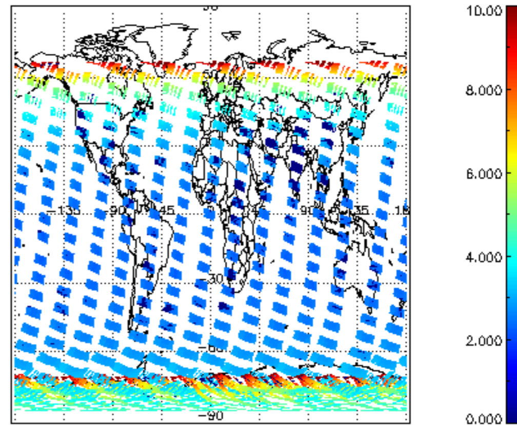
SCIOL2P_NADUV003_amf_cl for 25NOV2002 00:00:00 to 26NOV2002 00:00:00
