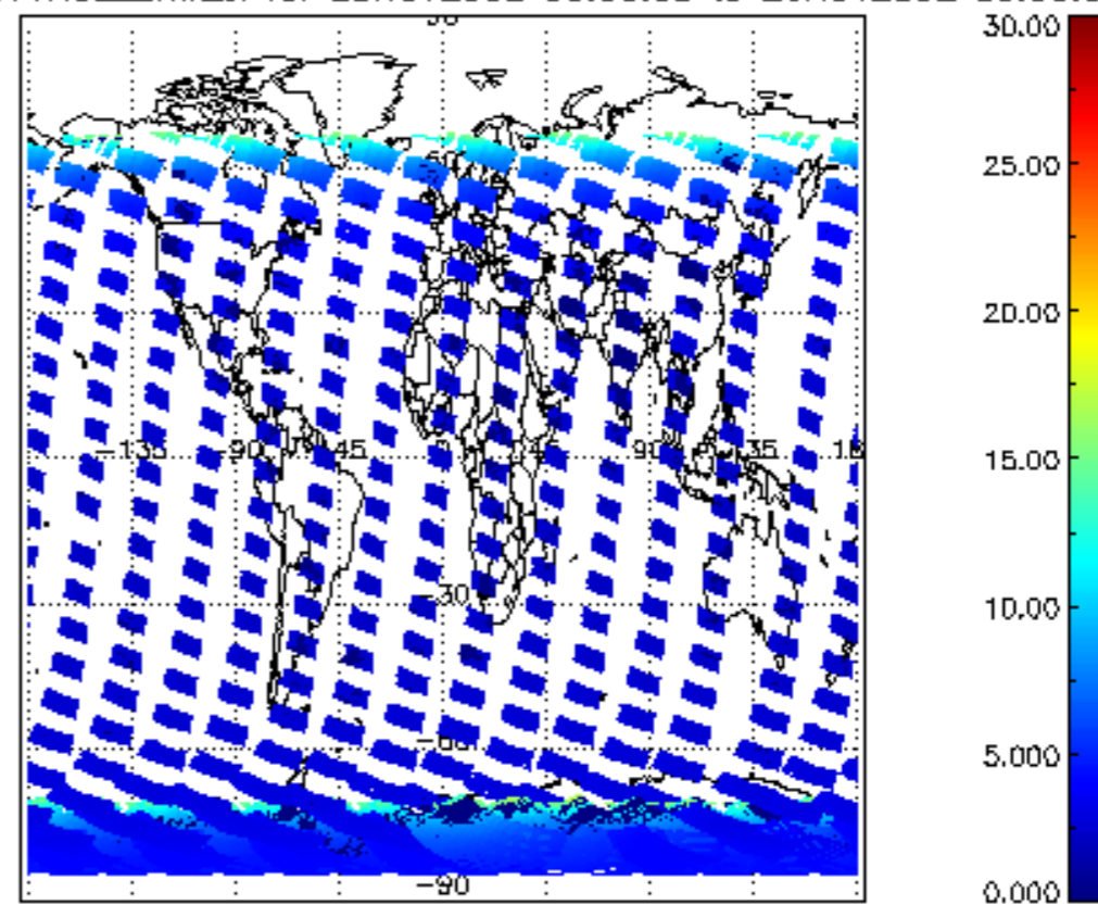
SCIOL2P_NADUV1NO2_amf_cl for 25NOV2002 00:00:00 to 26NOV2002 00:00:00
