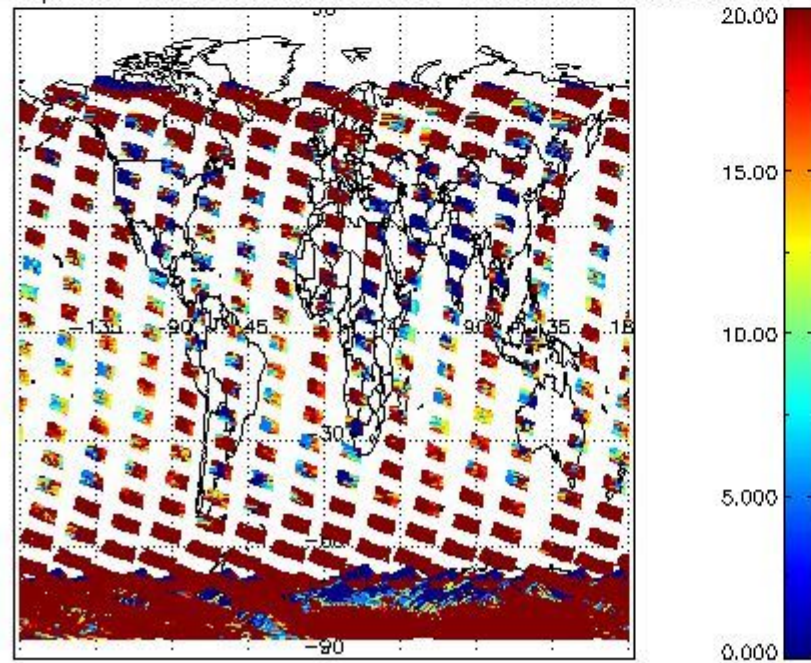
cL_opt_depth for 25NOV2002 00:00:00 to 26NOV2002 00:00:00
