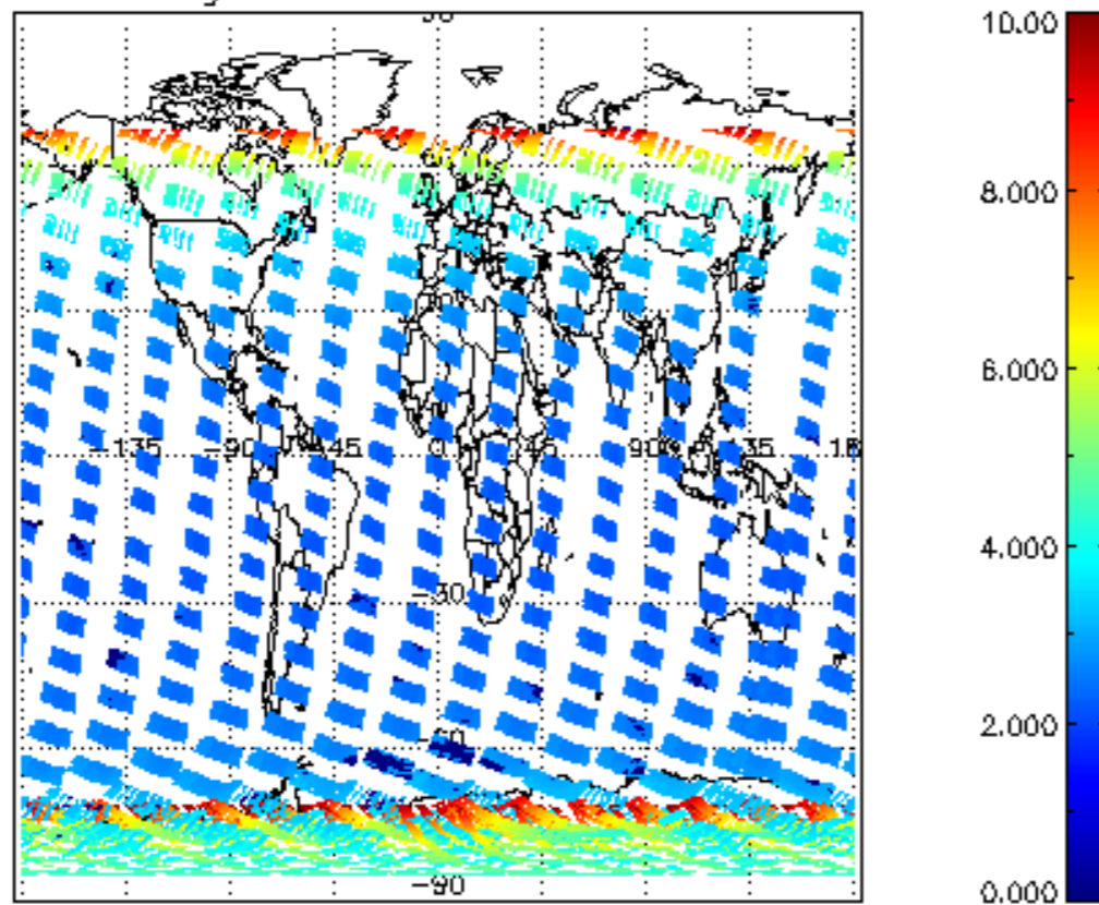
SCIOL2P_NADUV003_amf_gr for 22NOV2002 00:00:00 to 23NOV2002 00:00:00
