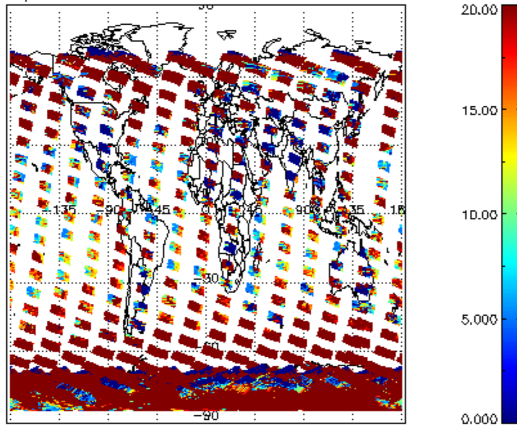
cL_opt_depth for 22NOV2002 00:00:00 to 23NOV2002 00:00:00
