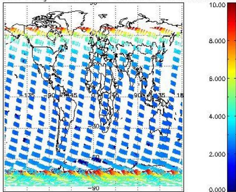
SCIOL2P_NADUV003_amf_gr for 22NOV2002 00:00:00 to 23NOV2002 00:00:00
