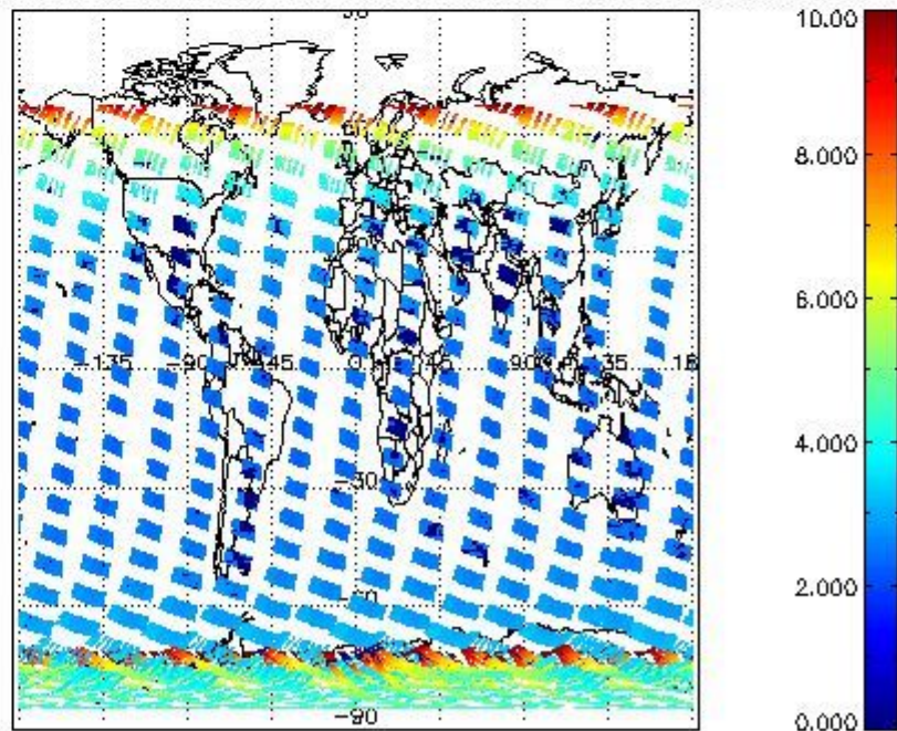
SCIOL2P_NADUV003_amf_cl for 22NOV2002 00:00:00 to 23NOV2002 00:00:00
