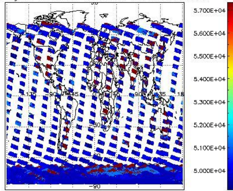
cloud_flags for 22NOV2002 00:00:00 to 23NOV2002 00:00:00
