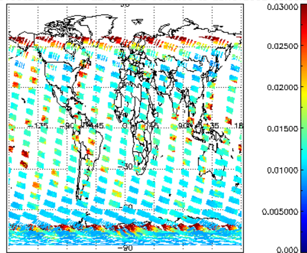
SCIOL2P_NADUV003_vcd_err for 22NOV2002 00:00:00 to 23NOV2002 00:00:00
