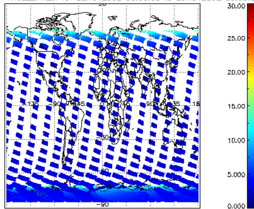
SCIOL2P_NADUV1NO2_amf_cl for 22NOV2002 00:00:00 to 23NOV2002 00:00:00
