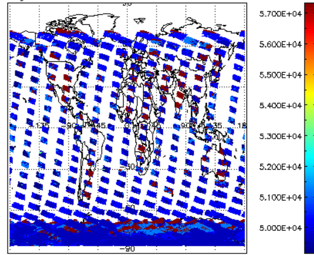
cloud_flags for 22NOV2002 00:00:00 to 23NOV2002 00:00:00
