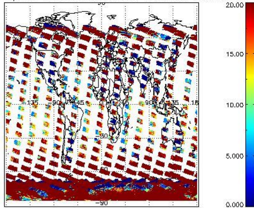
cL_opt_depth for 22NOV2002 00:00:00 to 23NOV2002 00:00:00
