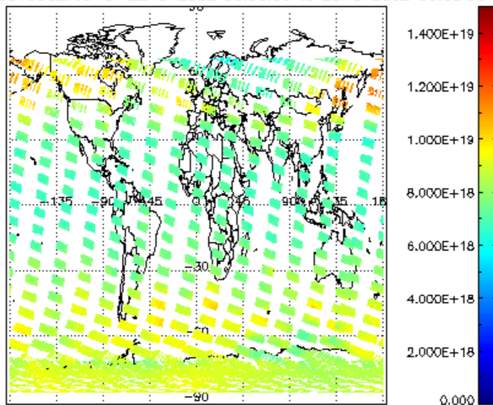
SCIOL2P_NADUV003_vcd for 22NOV2002 00:00:00 to 23NOV2002 00:00:00
