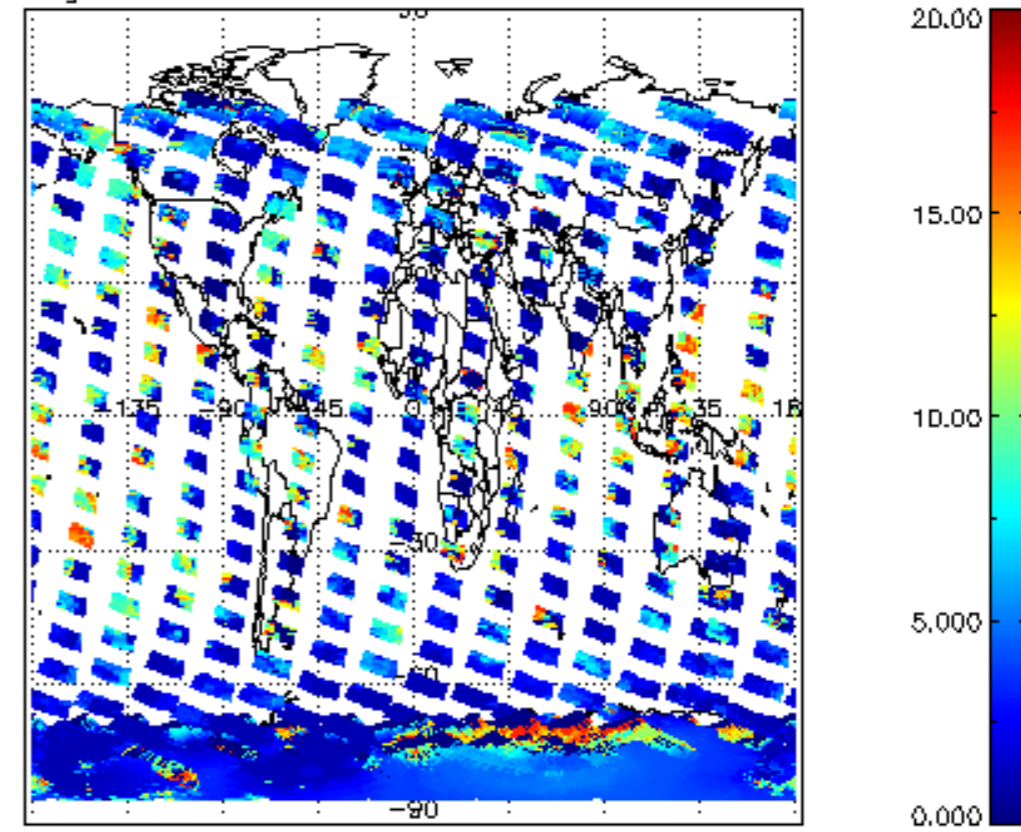
cL_top_height for 22NOV2002 00:00:00 to 23NOV2002 00:00:00
