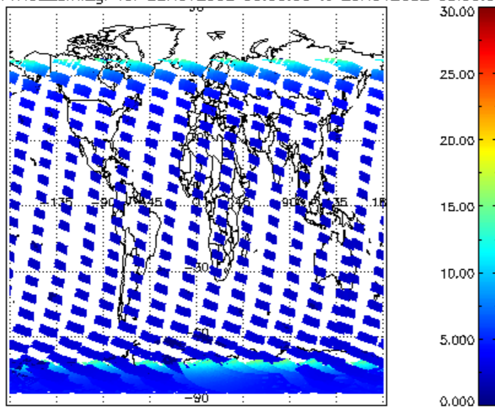
SCIOL2P_NADUV1NO2_amf_gr for 22NOV2002 00:00:00 to 23NOV2002 00:00:00
