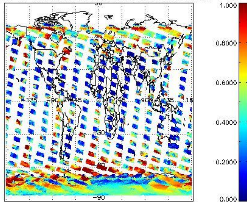
cLfrac for 22NOV2002 00:00:00 to 23NOV2002 00:00:00
