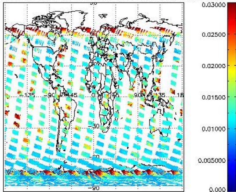
SCIOL2P_NADUV003_vcd_err for 22NOV2002 00:00:00 to 23NOV2002 00:00:00
