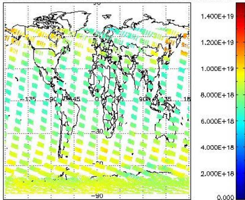
SCIOL2P_NADUV003_vcd for 22NOV2002 00:00:00 to 23NOV2002 00:00:00
