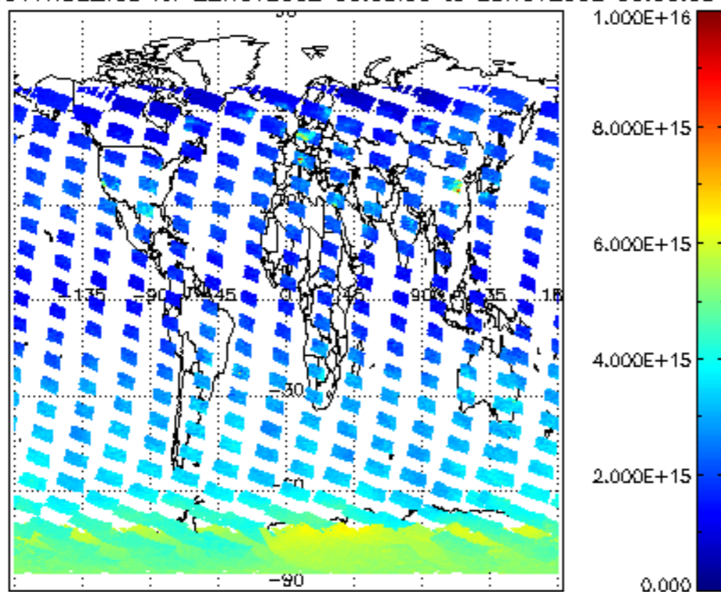
SCIOL2P_NADUV1NO2_vcd for 22NOV2002 00:00:00 to 23NOV2002 00:00:00
