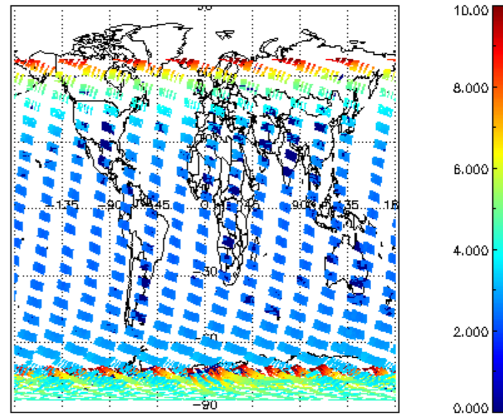
SCIOL2P_NADUV003_amf_cl for 22NOV2002 00:00:00 to 23NOV2002 00:00:00
