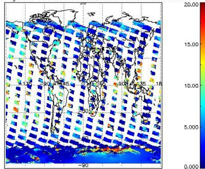
cL_top_height for 22NOV2002 00:00:00 to 23NOV2002 00:00:00
