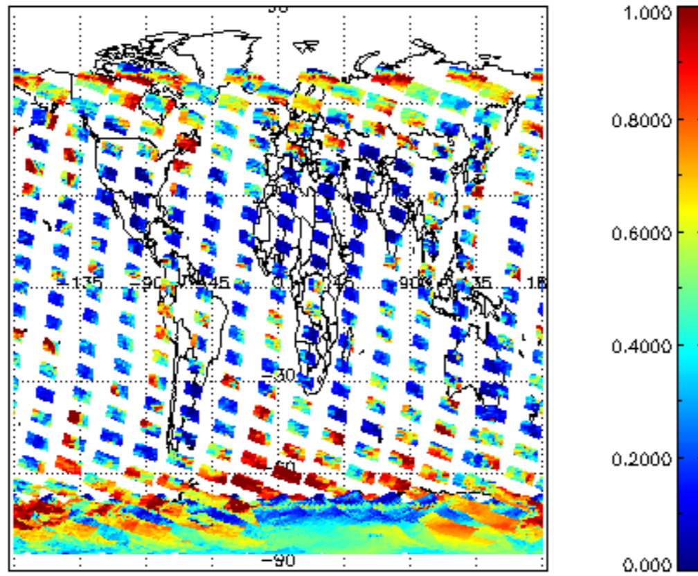
cLfrac for 22NOV2002 00:00:00 to 23NOV2002 00:00:00
