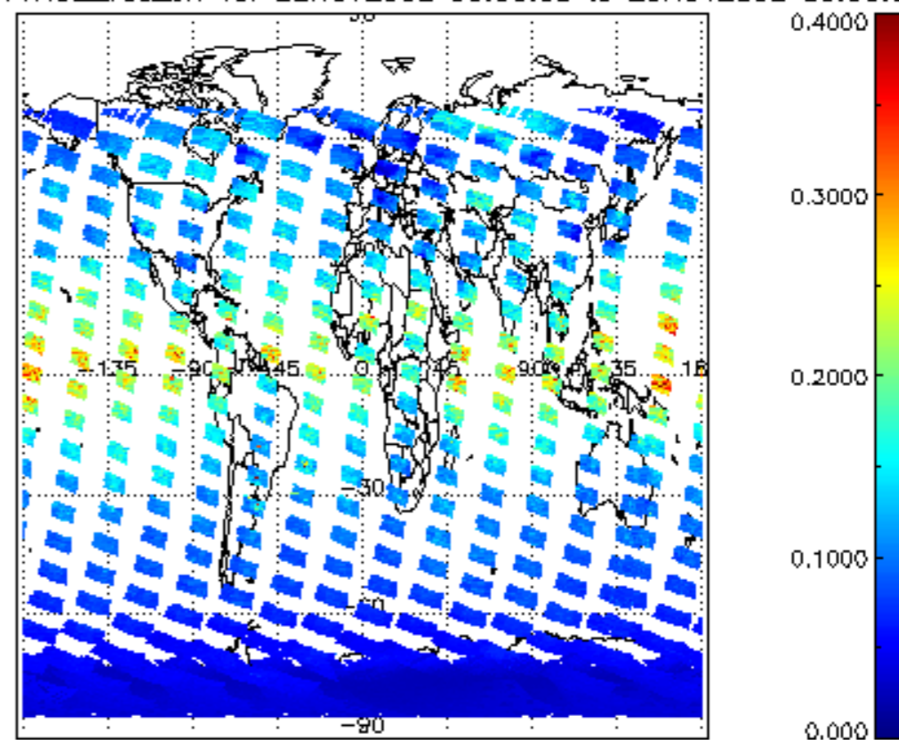
SCIOL2P_NADUV1NO2_vcd_err for 22NOV2002 00:00:00 to 23NOV2002 00:00:00
